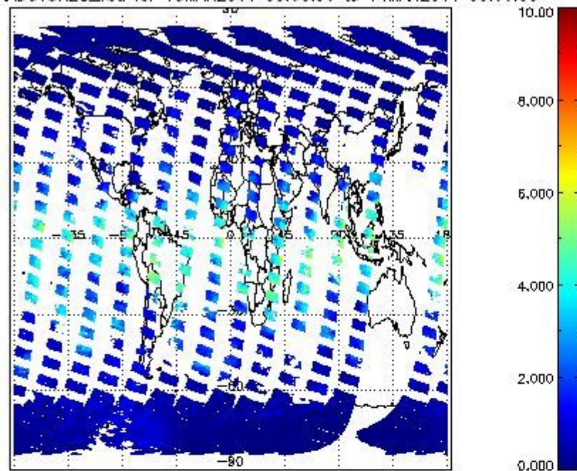
SCIOL2P_NADUV8H2O_vcd for 13MAR2011 00:00:00 to 14MAR2011 00:00:00
