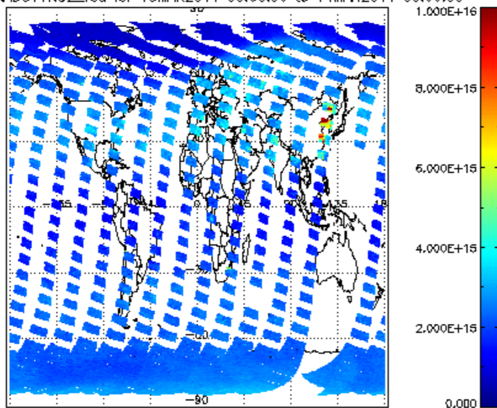
SCIOL2P_NADUV1NO2_vcd for 13MAR2011 00:00:00 to 14MAR2011 00:00:00
