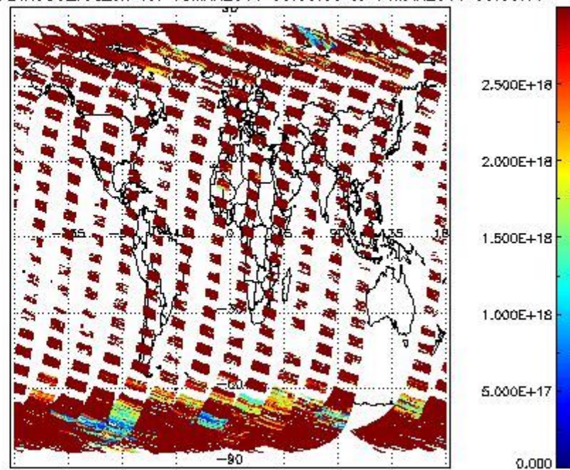
SCIDL2P_NADIR3CO_vcd_err for 13MAR2011 00:00:00 to 14MAR2011 00:00:00
