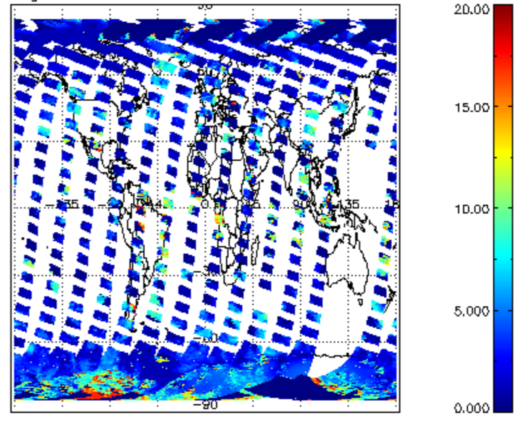
cL_top_height for 13MAR2011 00:00:00 to 14MAR2011 00:00:00
