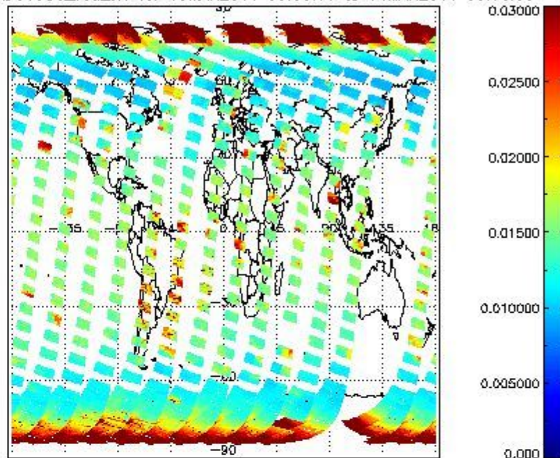
SCIOL2P_NADUV003_vcd_err for 13MAR2011 00:00:00 to 14MAR2011 00:00:00
