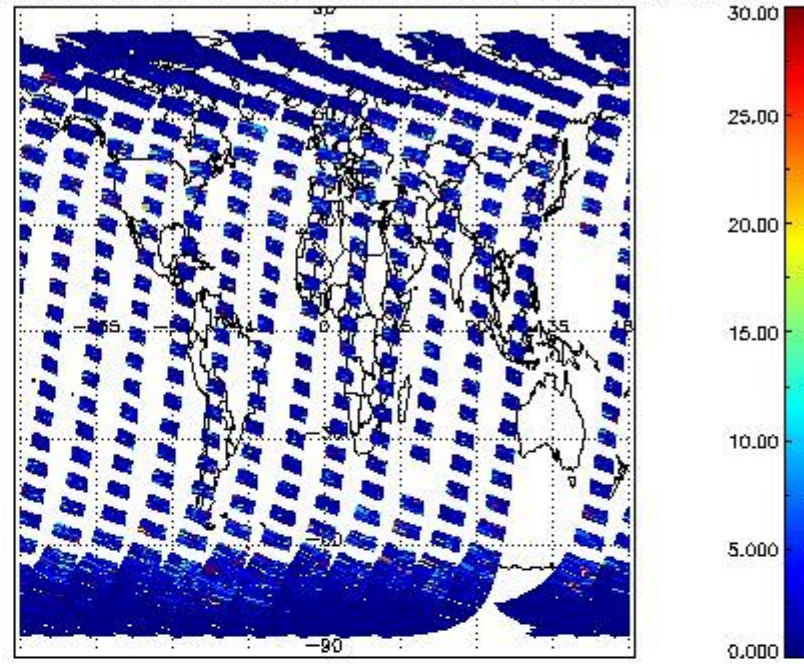
SCIOL2P_NADUV5S02_vcd_err for 13MAR2011 00:00:00 to 14MAR2011 00:00:00
