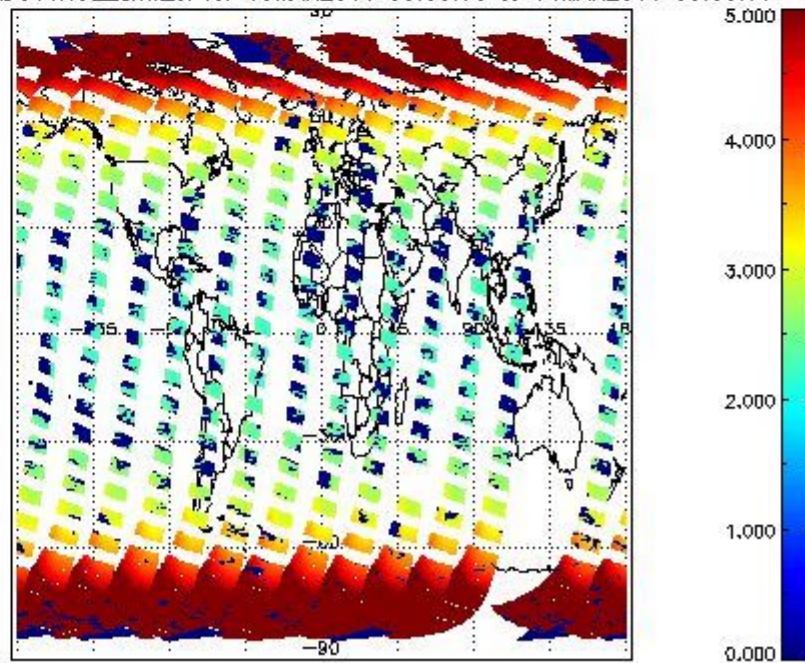
SCIOL2P_NADUV1NO2_amf_cl for 13MAR2011 00:00:00 to 14MAR2011 00:00:00
