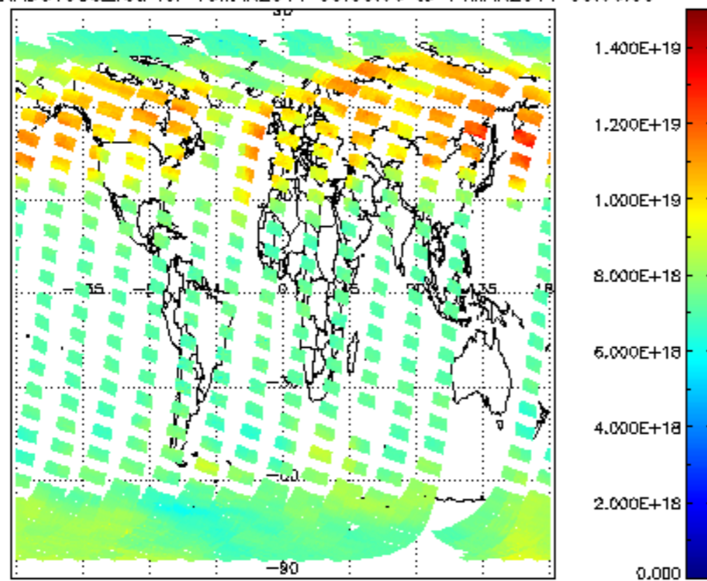
SCIOL2P_NADUV003_vcd for 13MAR2011 00:00:00 to 14MAR2011 00:00:00
