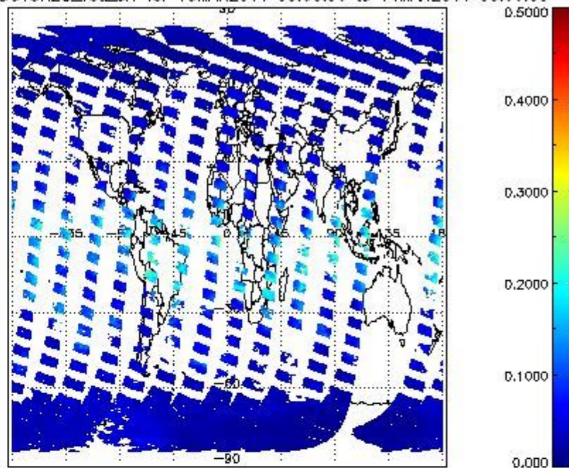
SCIOL2P_NADUV8H2O_vcd_err for 13MAR2011 00:00:00 to 14MAR2011 00:00:00
