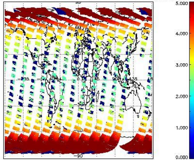
SCIOL2P_NADUV3BRO_amf_cl for 13MAR2011 00:00:00 to 14MAR2011 00:00:00
