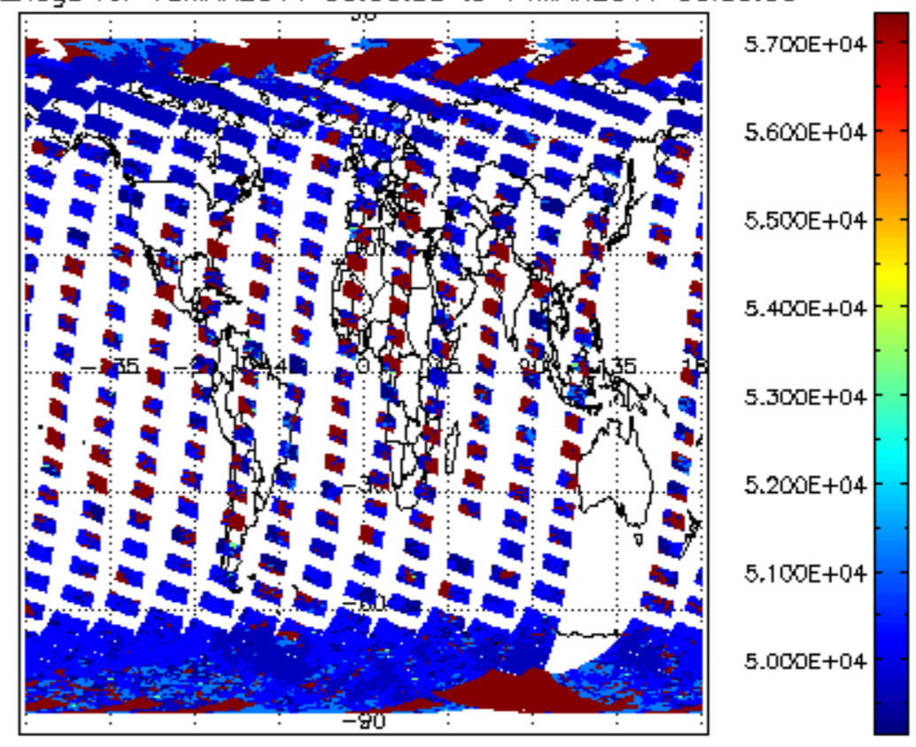
cloud_flags for 13MAR2011 00:00:00 to 14MAR2011 00:00:00
