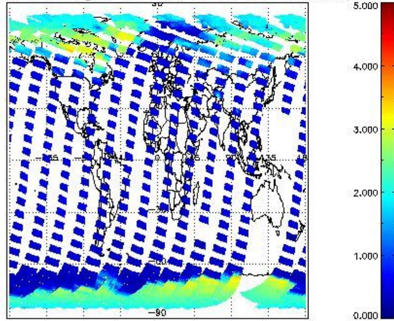
SCIOL2P_NADUV5S02_amf_gr for 13MAR2011 00:00:00 to 14MAR2011 00:00:00
