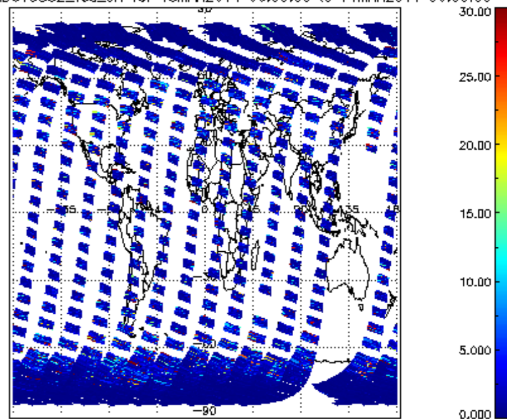
SCIOL2P_NADUV5S02_vcd_err for 13MAR2011 00:00:00 to 14MAR2011 00:00:00
