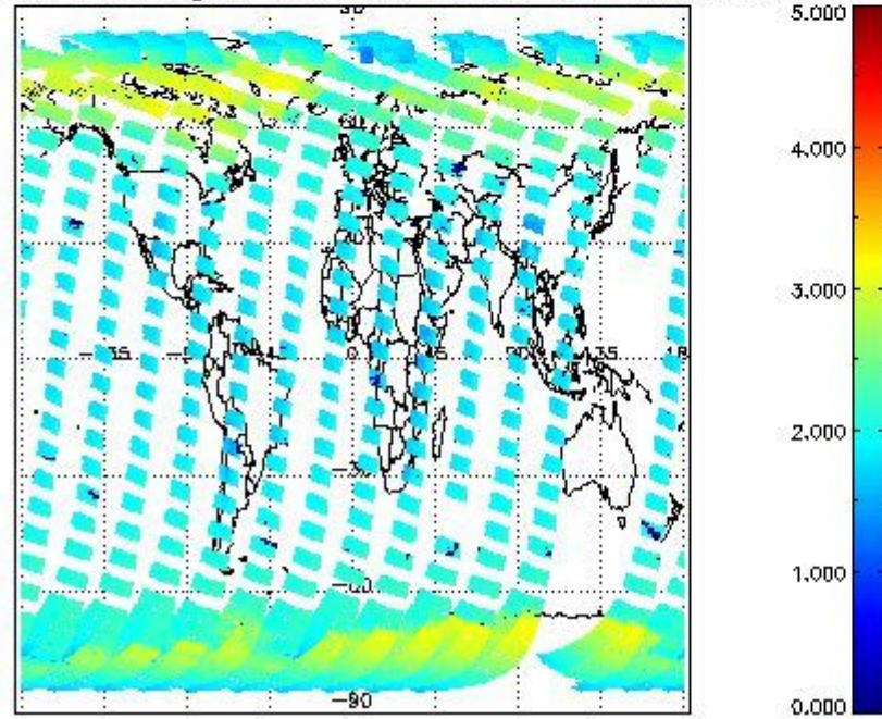
SCIOL2P_NADUV7S02_amf_gr for 13MAR2011 00:00:00 to 14MAR2011 00:00:00
