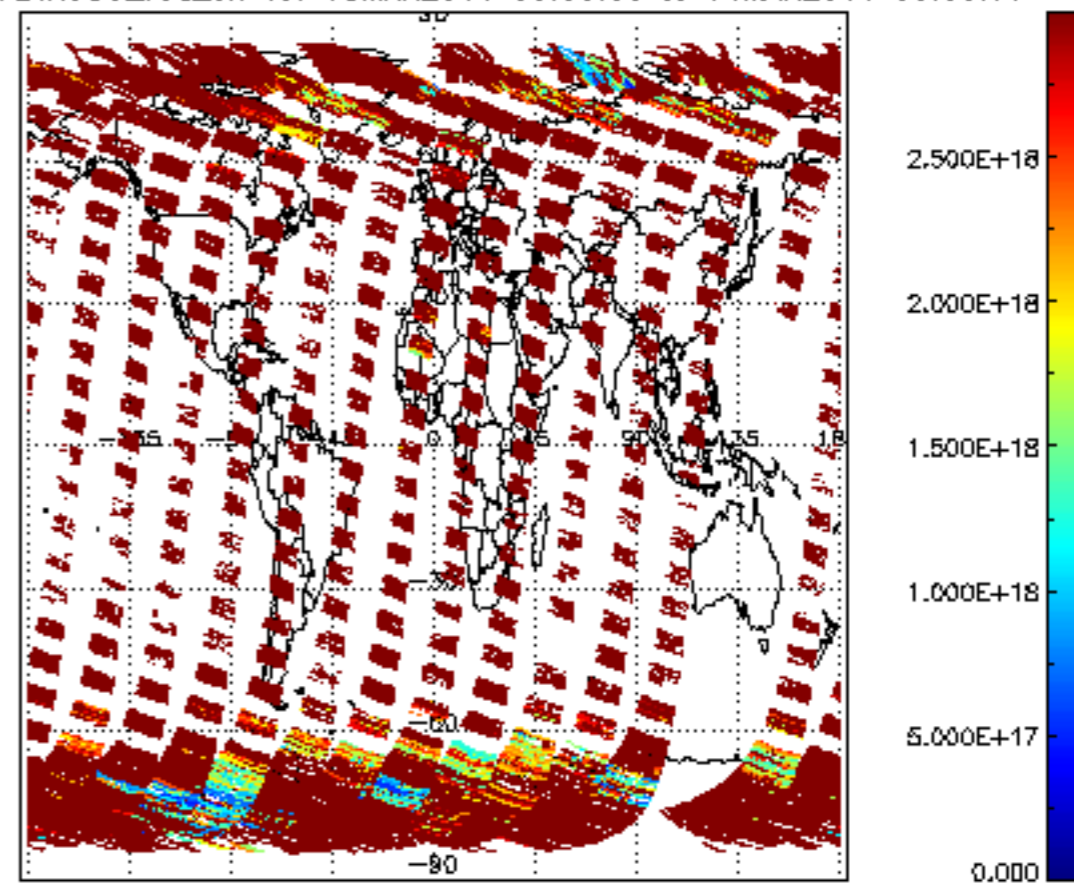
SCIOL2P_NADIR3CO_vcd_err for 13MAR2011 00:00:00 to 14MAR2011 00:00:00
