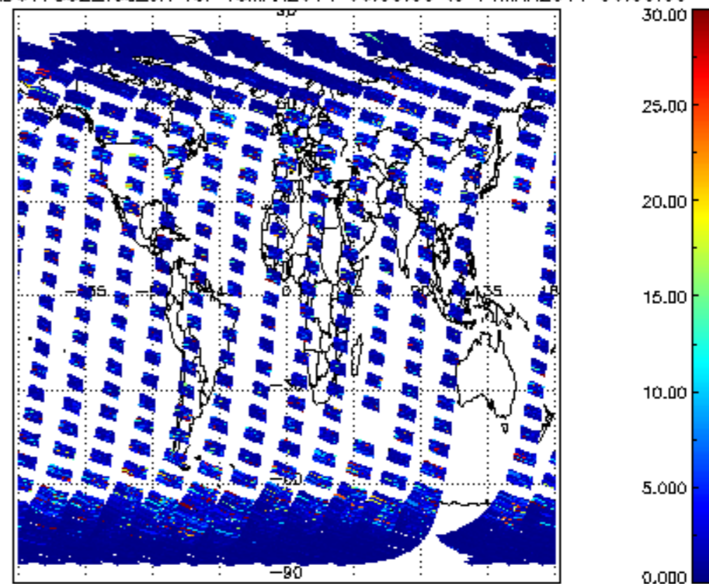
SCIOL2P_NADUV7S02_vcd_err for 13MAR2011 00:00:00 to 14MAR2011 00:00:00
