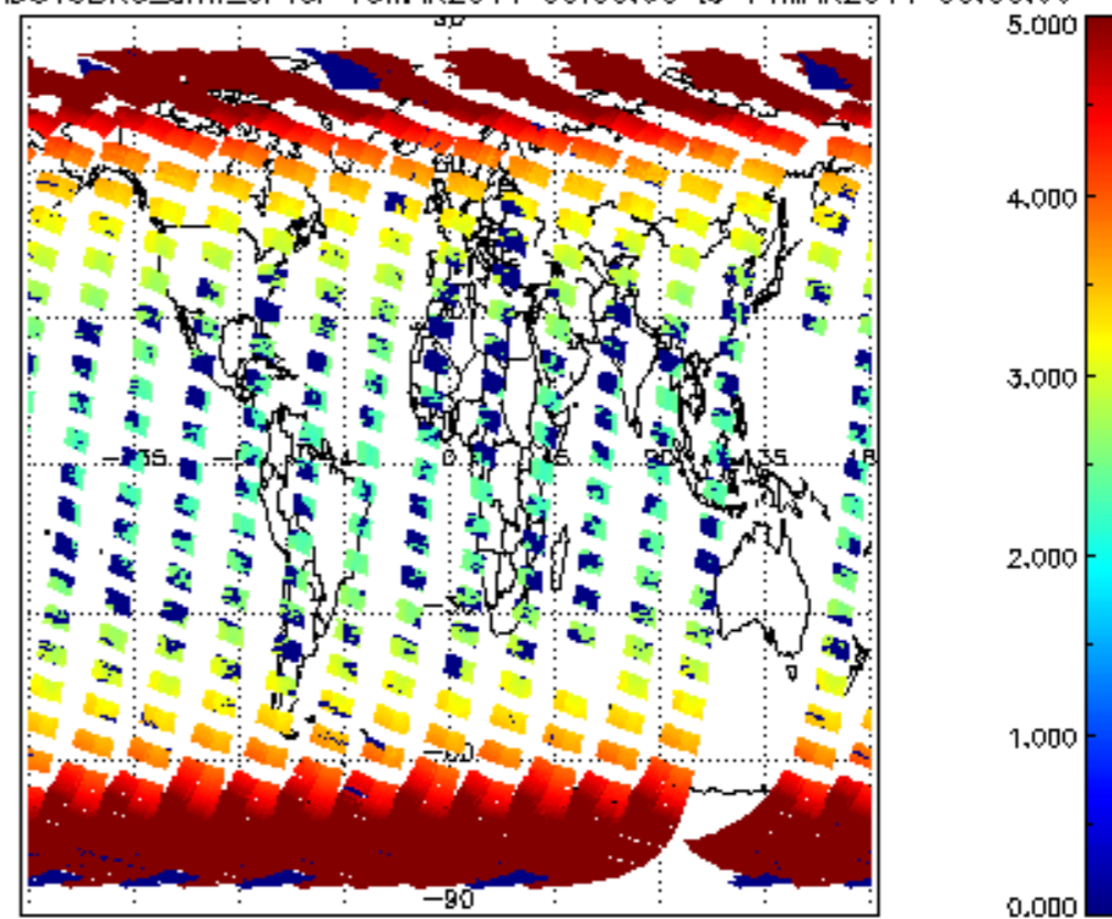
SCIOL2P_NADUV3BRO_amf_cl for 13MAR2011 00:00:00 to 14MAR2011 00:00:00
