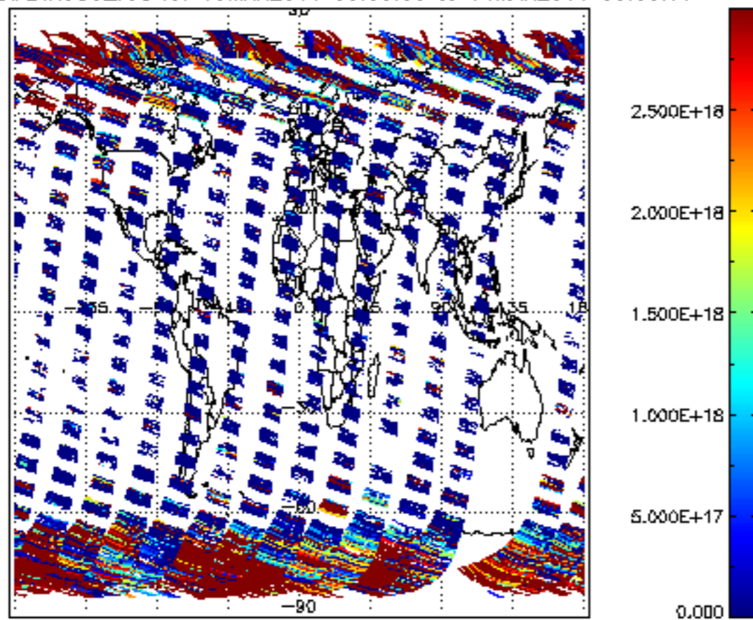
SCIOL2P_NADIR3CO_vcd for 13MAR2011 00:00:00 to 14MAR2011 00:00:00
