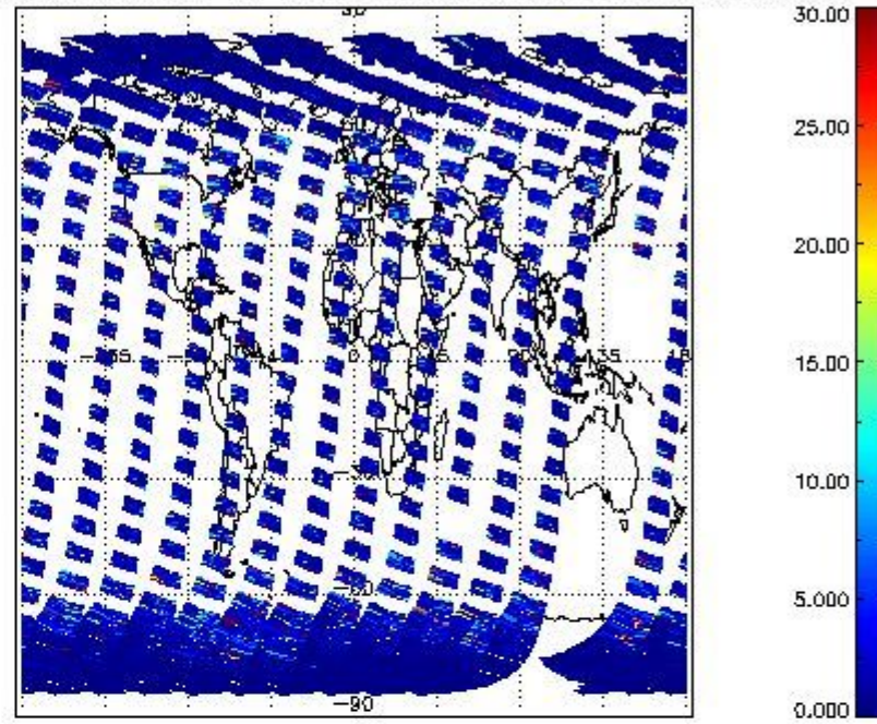
SCIOL2P_NADUV7S02_vcd_err for 13MAR2011 00:00:00 to 14MAR2011 00:00:00
