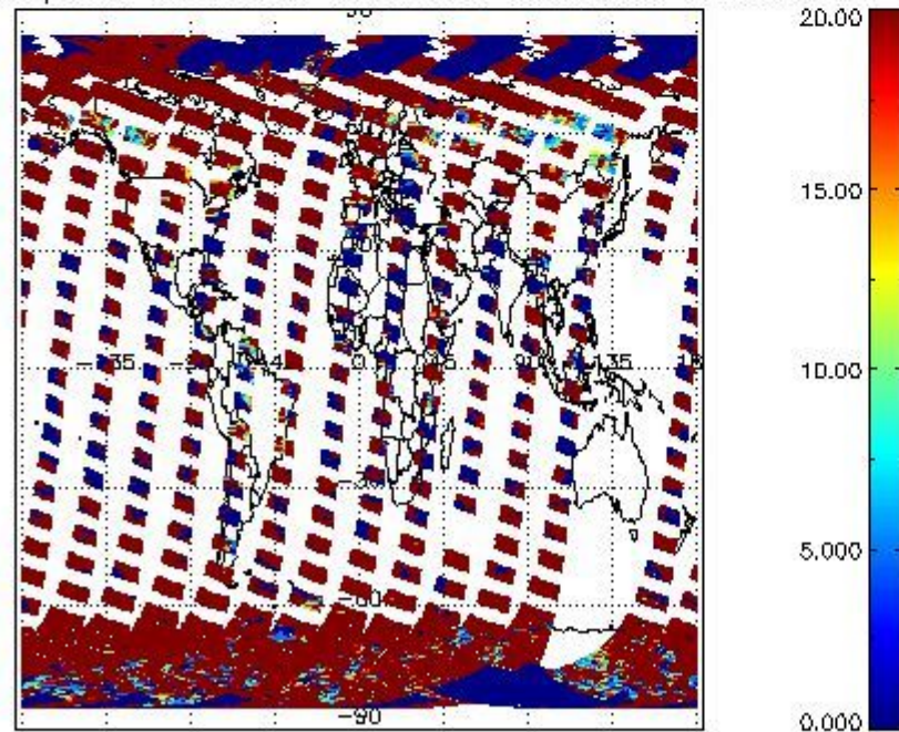
cL_opt_depth for 13MAR2011 00:00:00 to 14MAR2011 00:00:00
