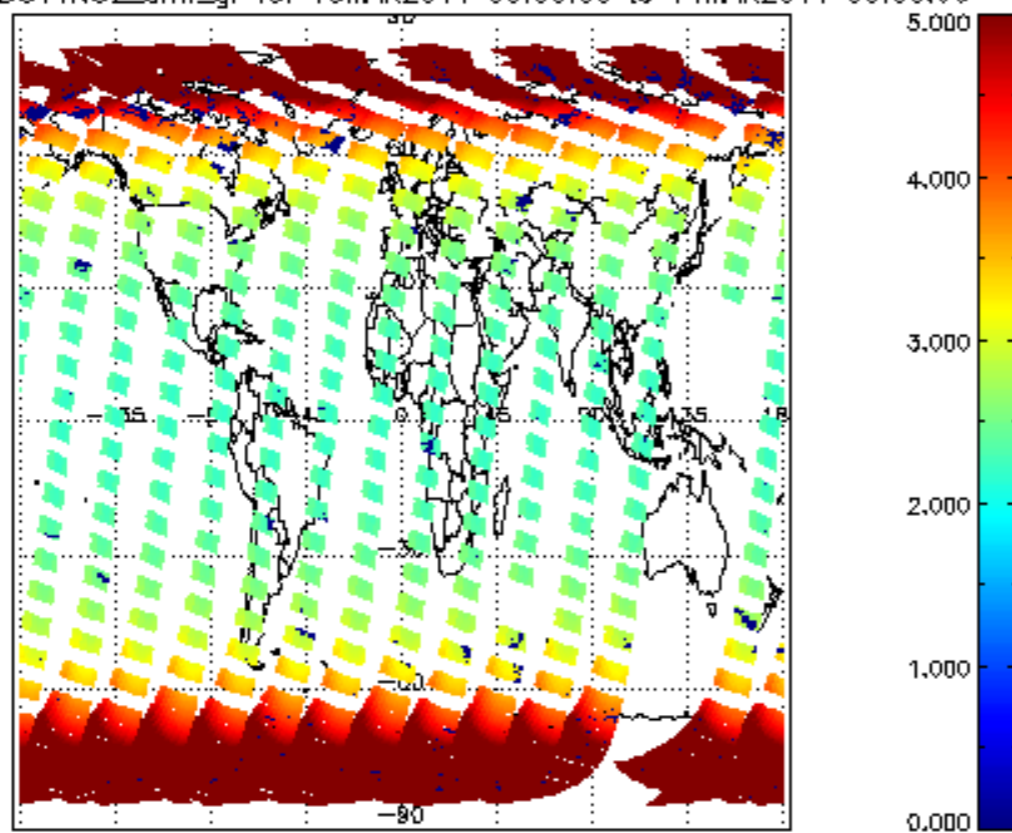
SCIOL2P_NADUV1NO2_amf_gr for 13MAR2011 00:00:00 to 14MAR2011 00:00:00
