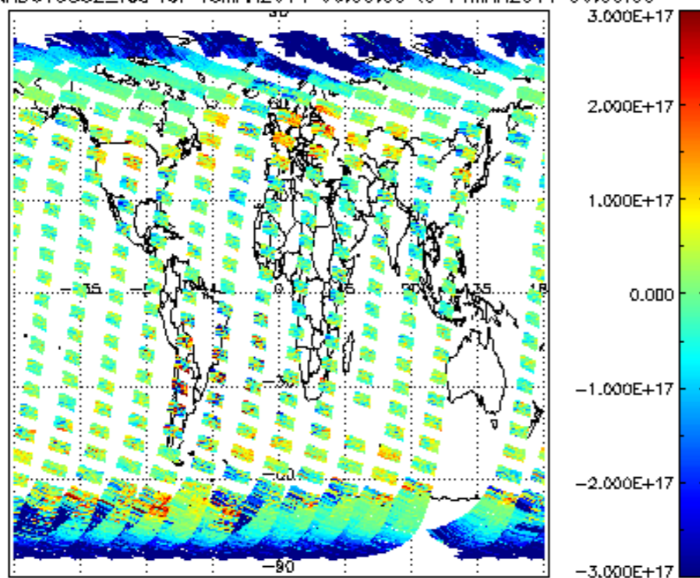
SCIOL2P_NADUV5S02_vcd for 13MAR2011 00:00:00 to 14MAR2011 00:00:00
