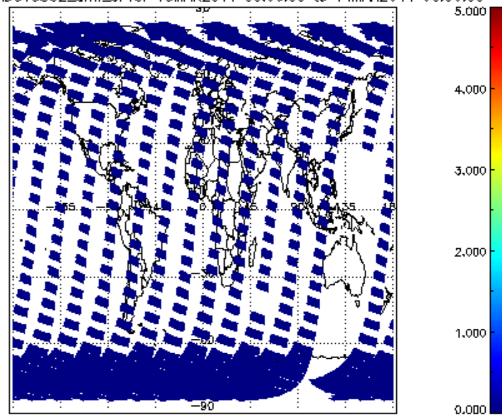
SCIOL2P_NADUV5S02_amf_cl for 13MAR2011 00:00:00 to 14MAR2011 00:00:00
