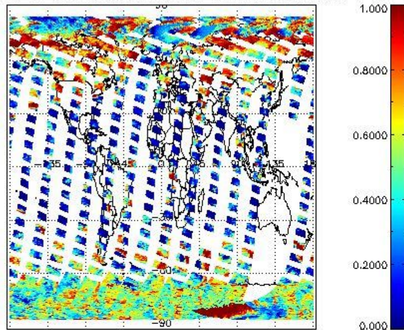
cL_frac for 13MAR2011 00:00:00 to 14MAR2011 00:00:00
