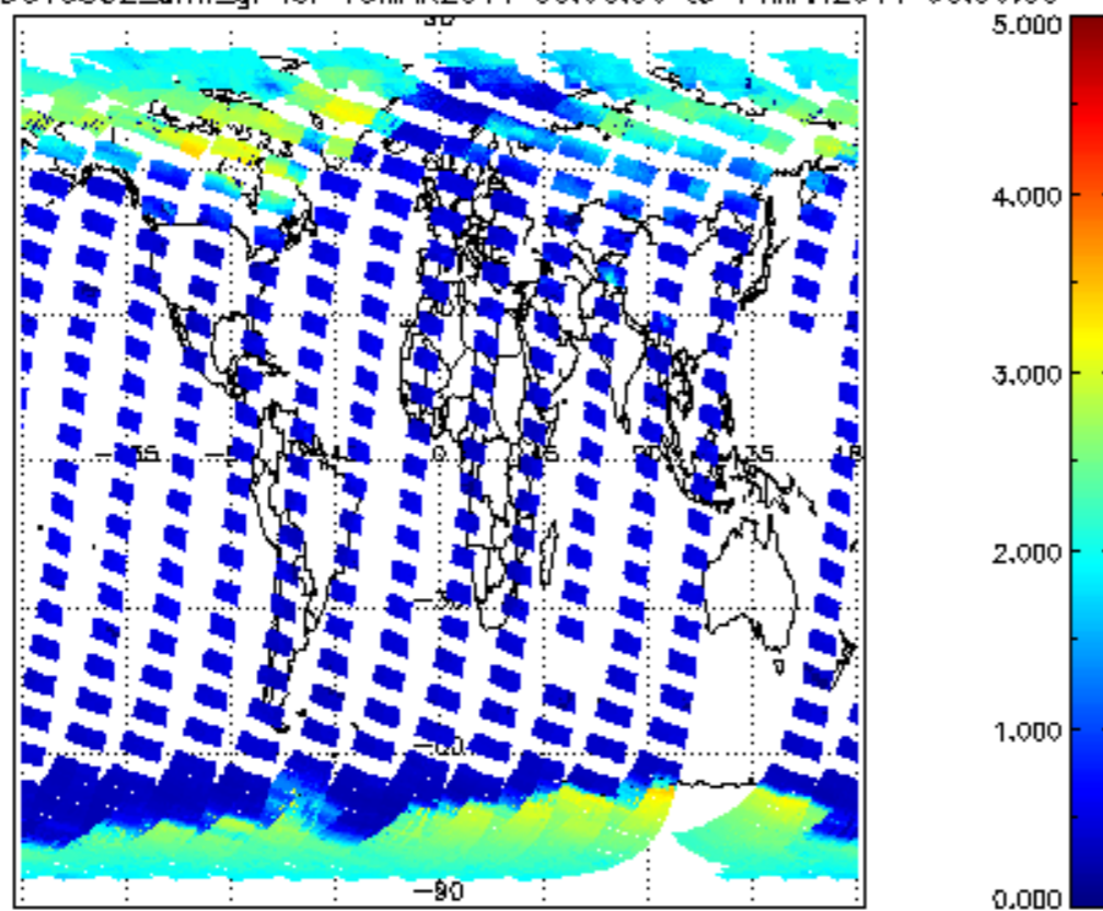
SCIOL2P_NADUV5S02_amf_gr for 13MAR2011 00:00:00 to 14MAR2011 00:00:00
