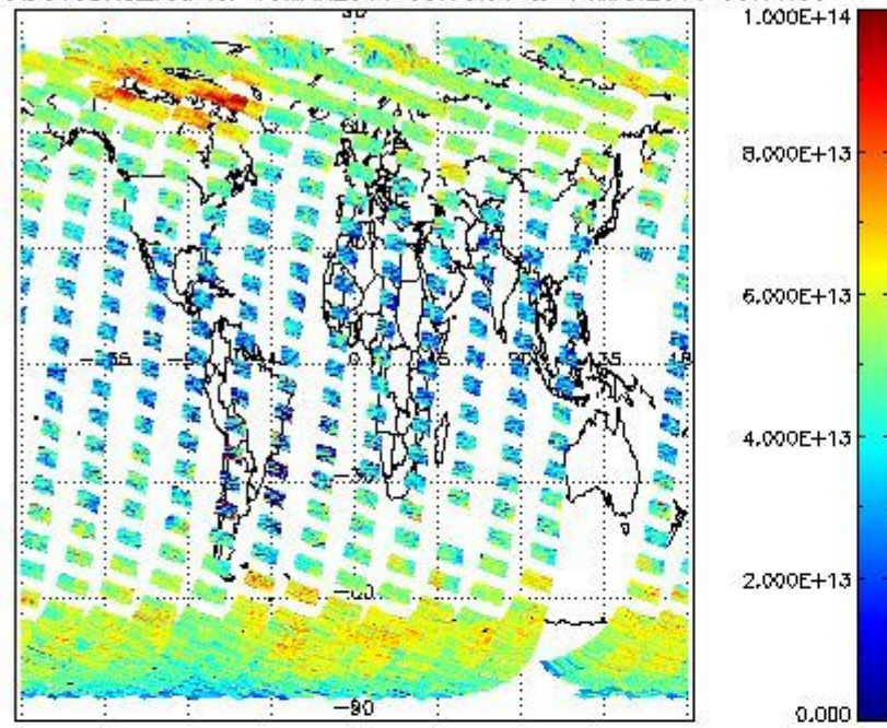
SCIOL2P_NADUV3BRO_vcd for 13MAR2011 00:00:00 to 14MAR2011 00:00:00
