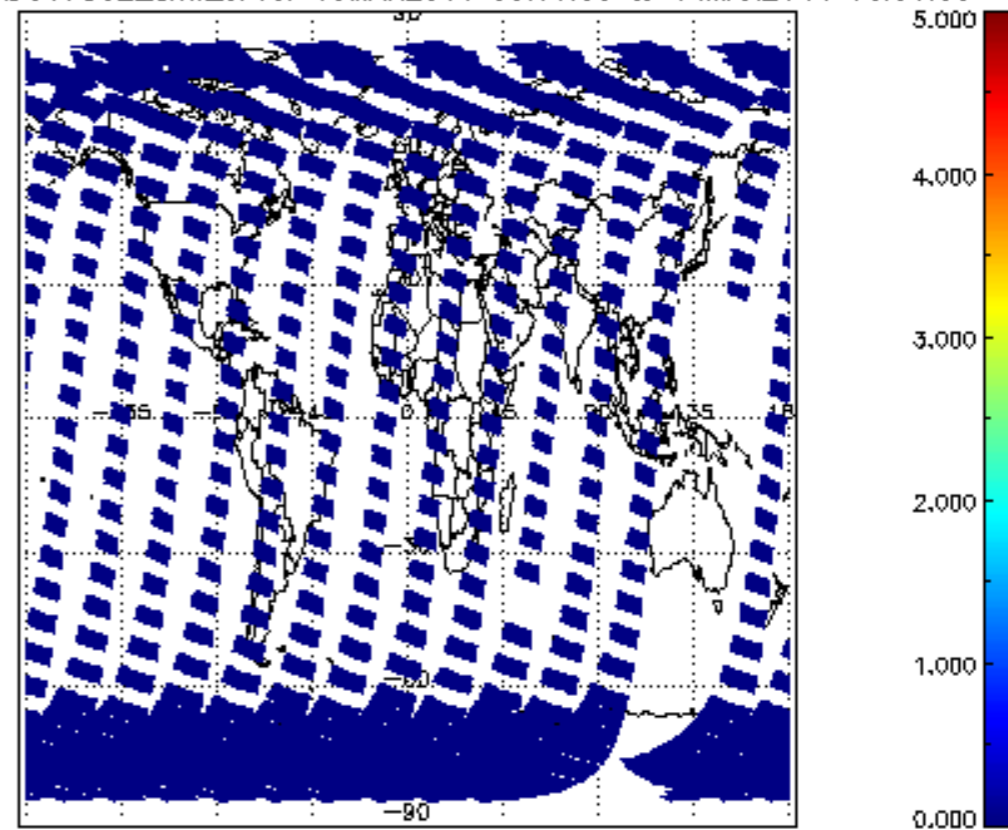
SCIOL2P_NADUV7S02_amf_cl for 13MAR2011 00:00:00 to 14MAR2011 00:00:00
