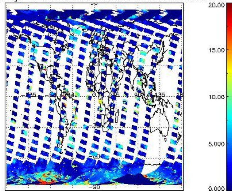
cL_top_height for 13MAR2011 00:00:00 to 14MAR2011 00:00:00
