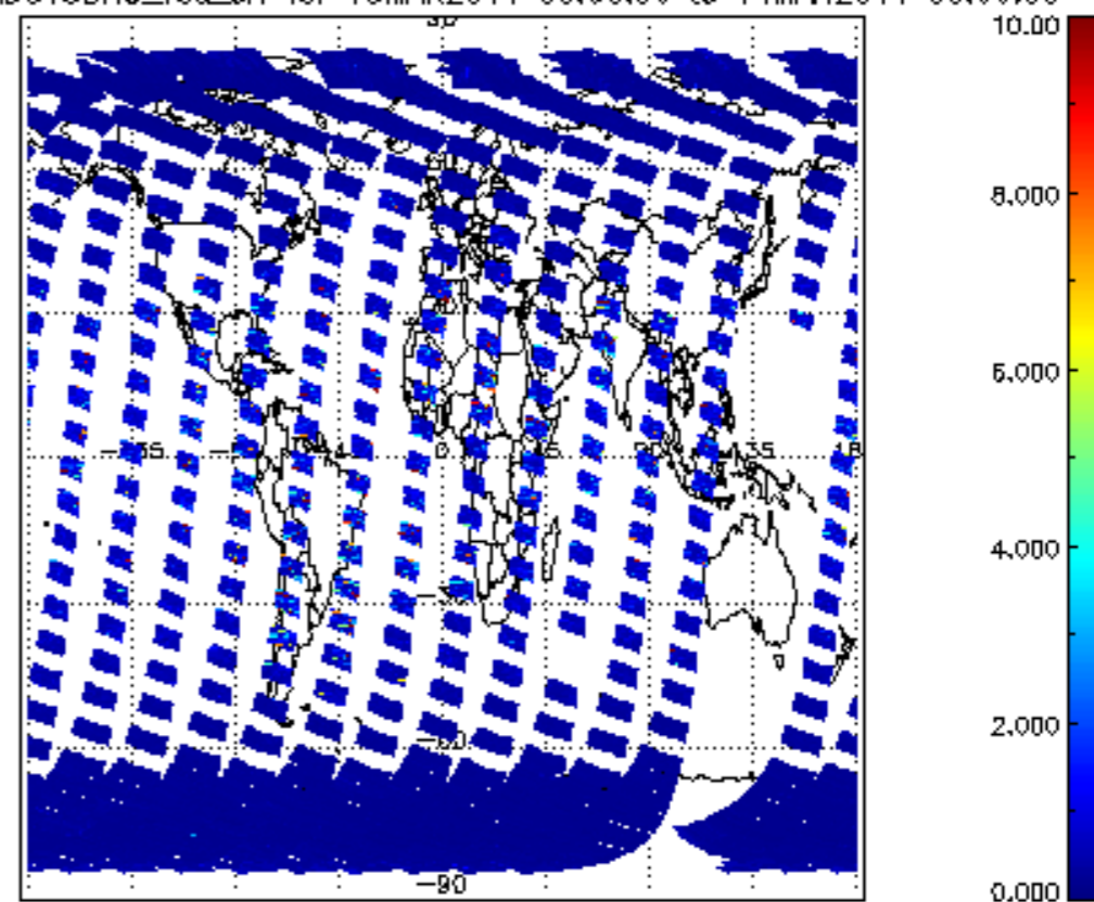
SCIOL2P_NADUV3BRO_vcd_err for 13MAR2011 00:00:00 to 14MAR2011 00:00:00
