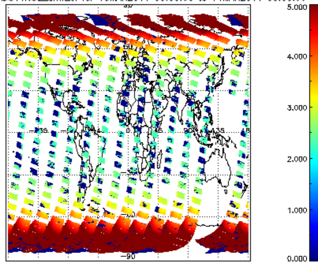
SCIOL2P_NADUV1NO2_amf_cl for 13MAR2011 00:00:00 to 14MAR2011 00:00:00
