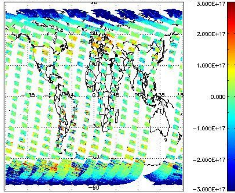
SCIOL2P_NADUV5S02_vcd for 13MAR2011 00:00:00 to 14MAR2011 00:00:00
