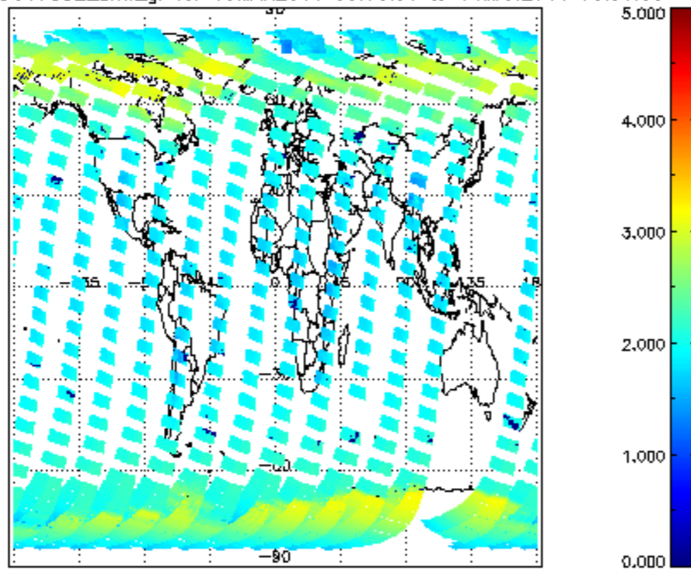
SCIOL2P_NADUV7S02_amf_gr for 13MAR2011 00:00:00 to 14MAR2011 00:00:00
