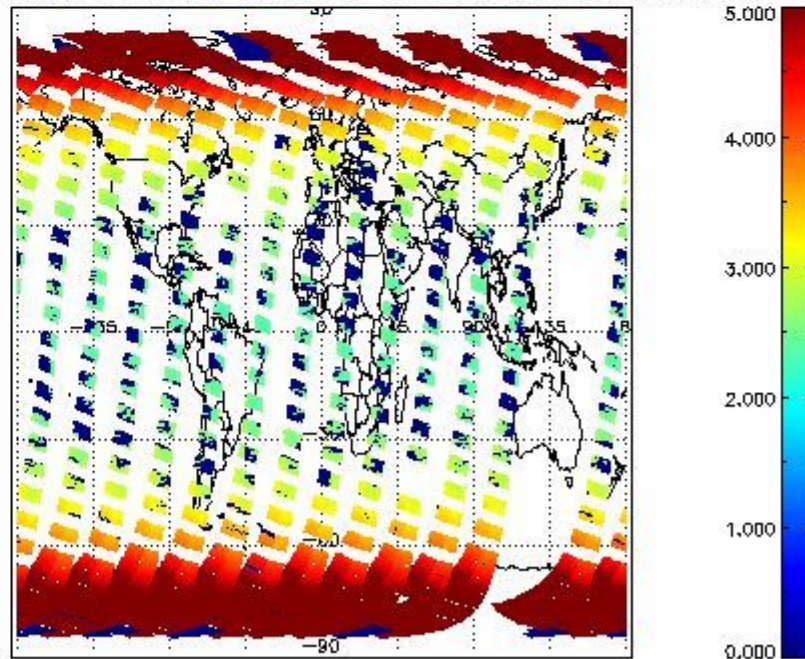
SCIOL2P_NADUV003_amf_cl for 13MAR2011 00:00:00 to 14MAR2011 00:00:00
