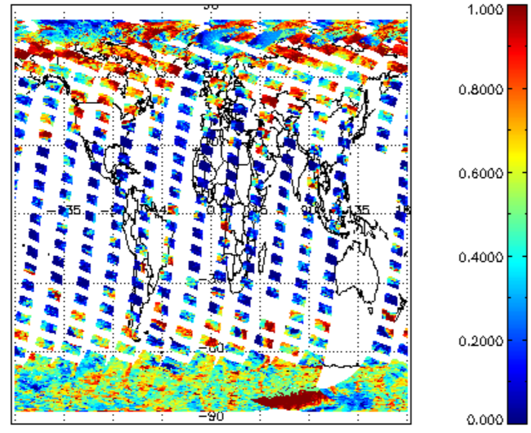
cLfrac for 13MAR2011 00:00:00 to 14MAR2011 00:00:00
