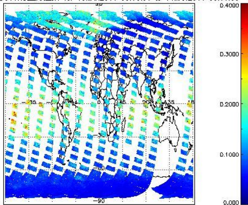
SCIOL2P_NADUV1NO2_vcd_err for 13MAR2011 00:00:00 to 14MAR2011 00:00:00
