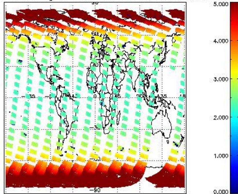
SCIOL2P_NADUV003_amf_gr for 13MAR2011 00:00:00 to 14MAR2011 00:00:00
