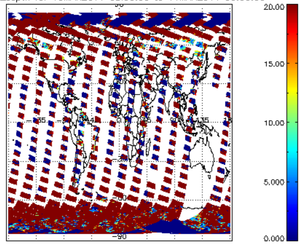
cL_opt_depth for 13MAR2011 00:00:00 to 14MAR2011 00:00:00
