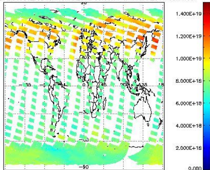
SCIOL2P_NADUV003_vcd for 13MAR2011 00:00:00 to 14MAR2011 00:00:00
