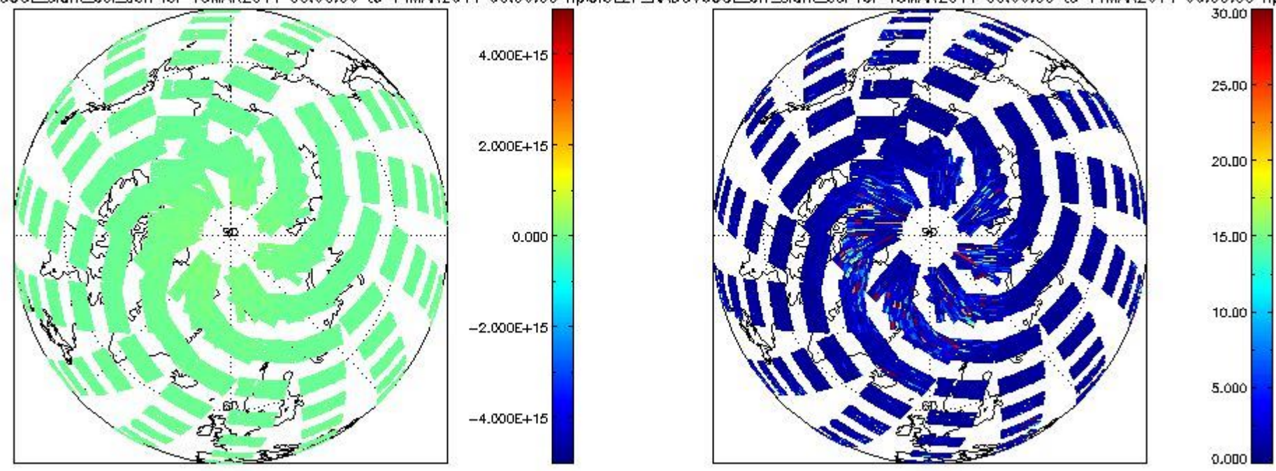
CIOL2P_NADUV6OCL_slant_col_den for 13MAR2011 00:00:00 to 14MAR2011 00:00:00 np CIOL2P_NADUV6OCL_err_slant_col for 13MAR2011 00:00:00 to 14MAR2011 00:00:00 np
