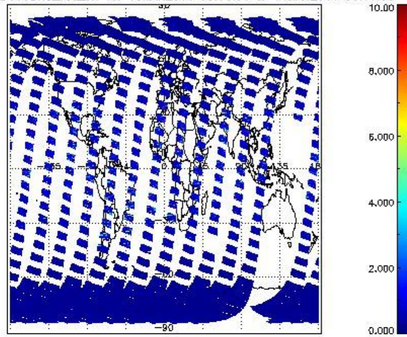
SCIOL2P_NADUV3BRO_vcd_err for 13MAR2011 00:00:00 to 14MAR2011 00:00:00
