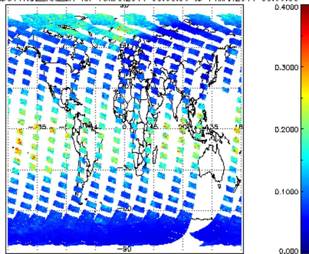
SCIOL2P_NADUV1NO2_vcd_err for 13MAR2011 00:00:00 to 14MAR2011 00:00:00
