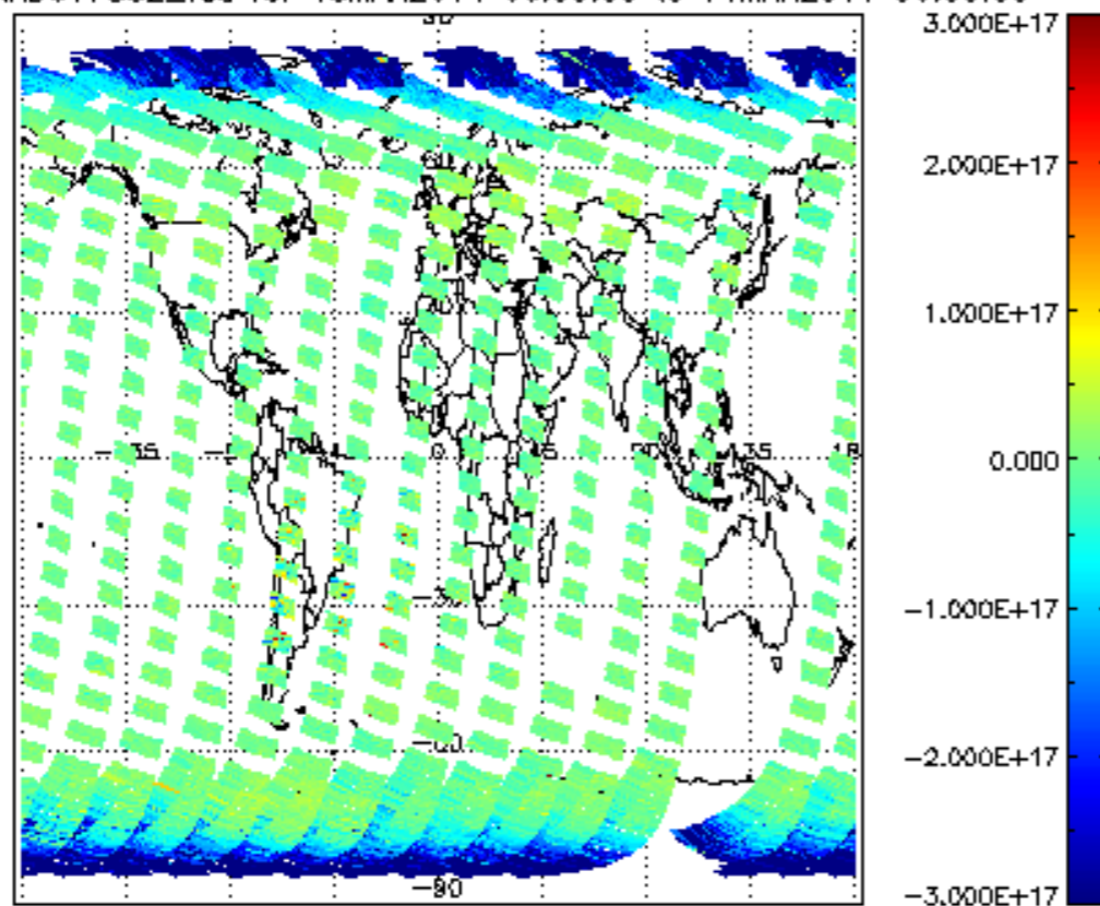
SCIOL2P_NADUV7S02_vcd for 13MAR2011 00:00:00 to 14MAR2011 00:00:00
