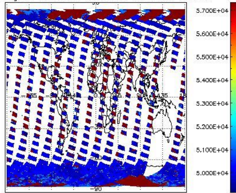
cloud_flags for 13MAR2011 00:00:00 to 14MAR2011 00:00:00
