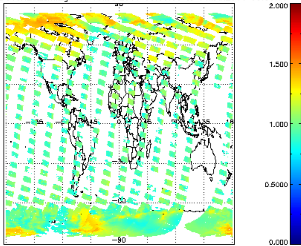
SCIOL2P_NADUV8H20_arnf_gr for 13MAR2011 00:00:00 to 14MAR2011 00:00:00
