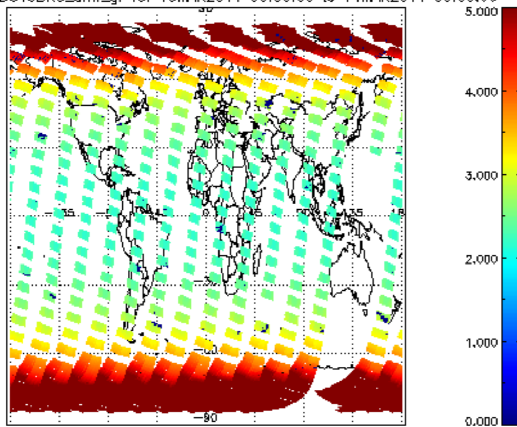
SCIOL2P_NADUV3BRO_amf_gr for 13MAR2011 00:00:00 to 14MAR2011 00:00:00
