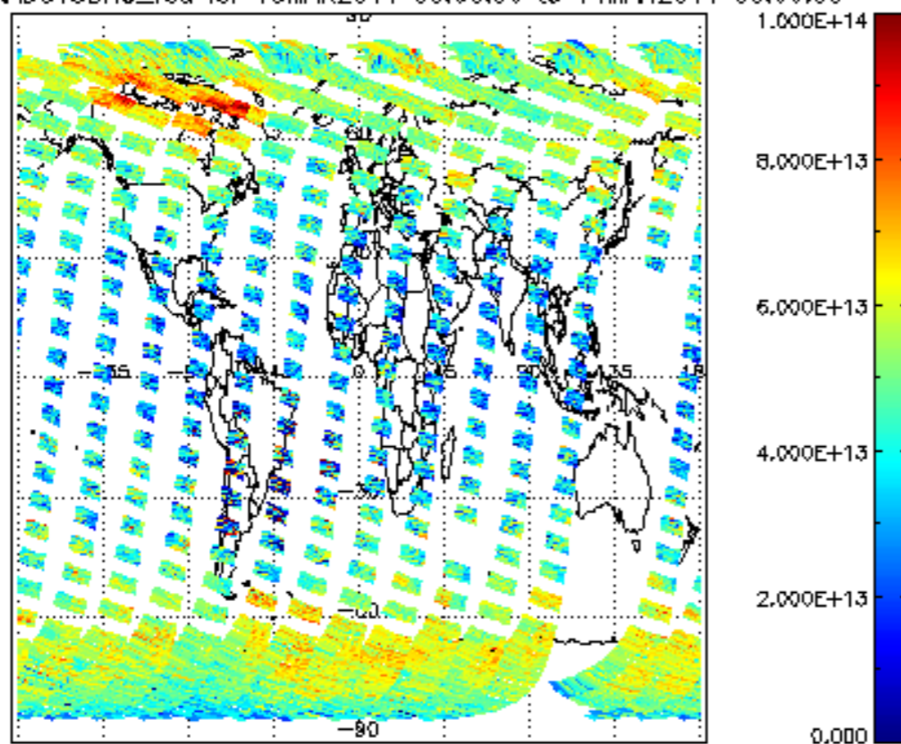
SCIOL2P_NADUV3BRO_vcd for 13MAR2011 00:00:00 to 14MAR2011 00:00:00
