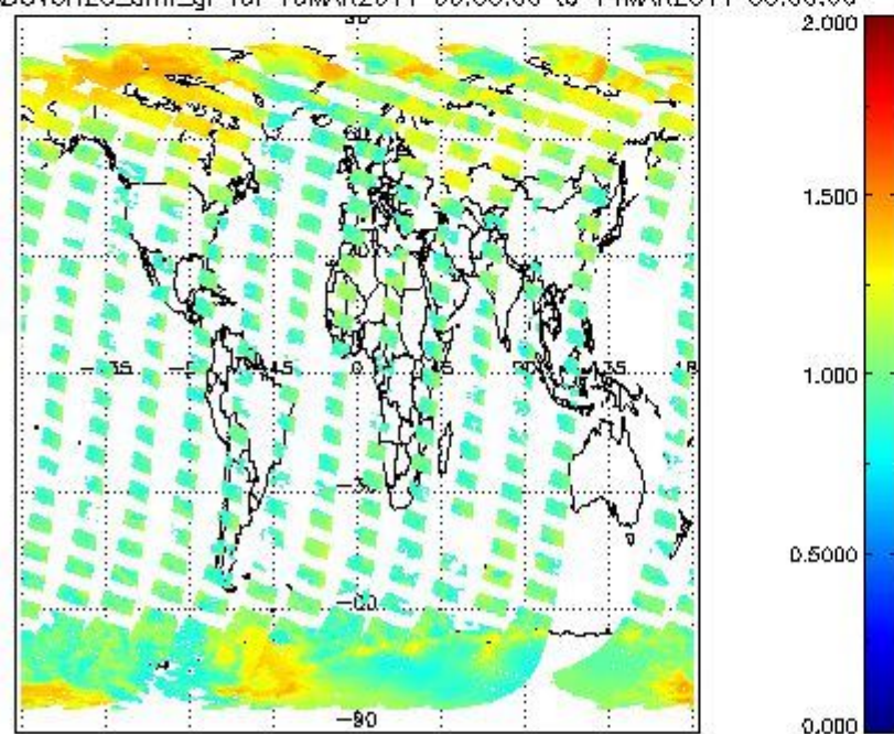
SCIOL2P_NADUV8H2O_arnf_gr for 13MAR2011 00:00:00 to 14MAR2011 00:00:00
