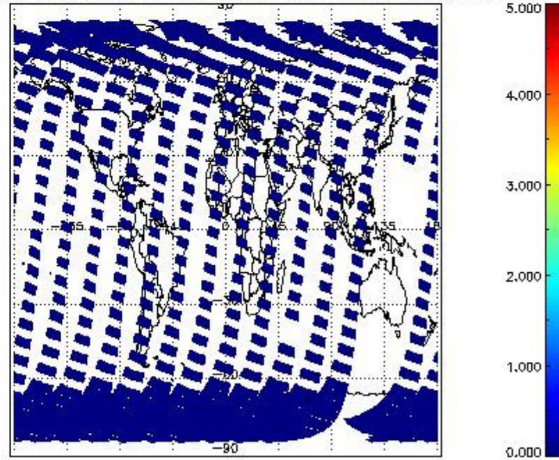
SCIOL2P_NADUV5S02_amf_cl for 13MAR2011 00:00:00 to 14MAR2011 00:00:00
