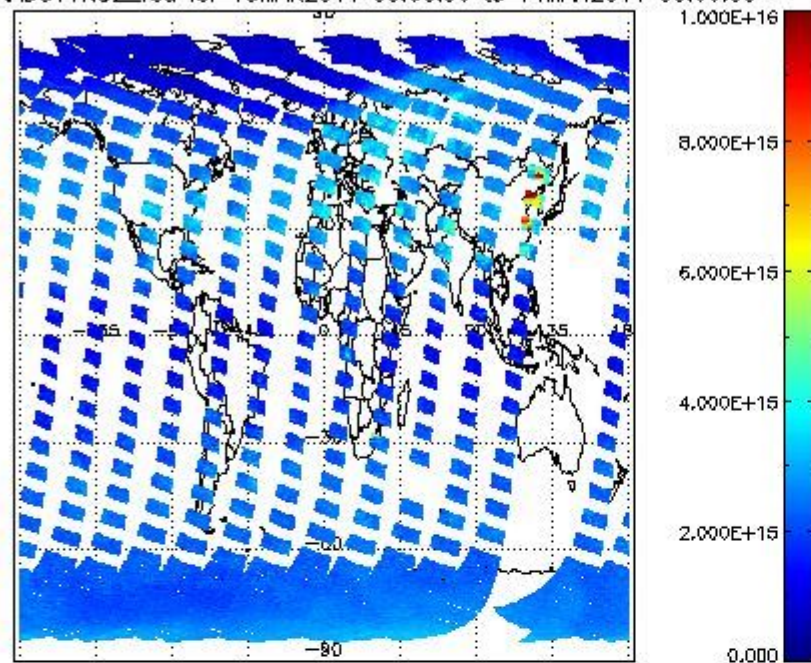
SCIOL2P_NADUV1NO2_vcd for 13MAR2011 00:00:00 to 14MAR2011 00:00:00
