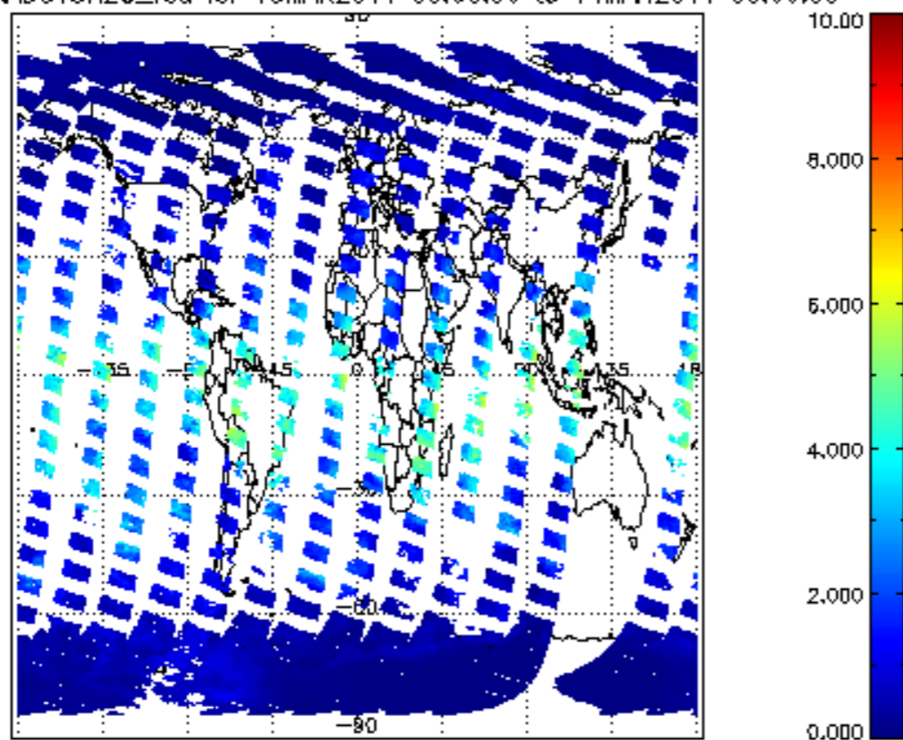
SCIOL2P_NADUV8H20_vcd for 13MAR2011 00:00:00 to 14MAR2011 00:00:00
