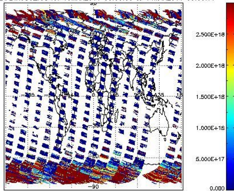
SCIDL2P_NADIR3CO_vcd for 13MAR2011 00:00:00 to 14MAR2011 00:00:00
