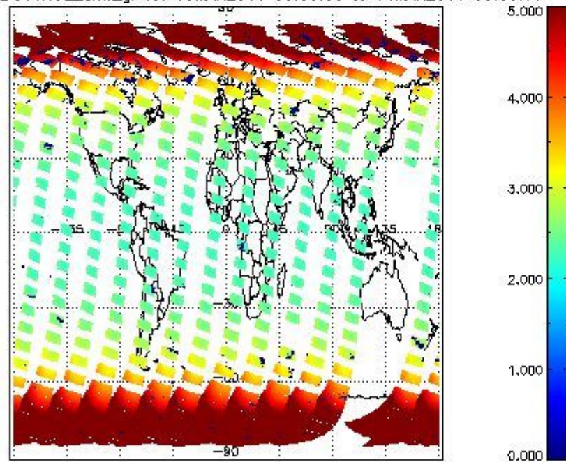
SCIOL2P_NADUV1NO2_amf_gr for 13MAR2011 00:00:00 to 14MAR2011 00:00:00
