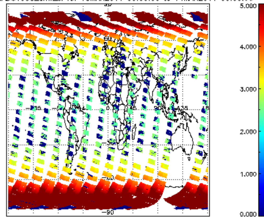
SCIOL2P_NADUV003_arnf_cl for 13MAR2011 00:00:00 to 14MAR2011 00:00:00
