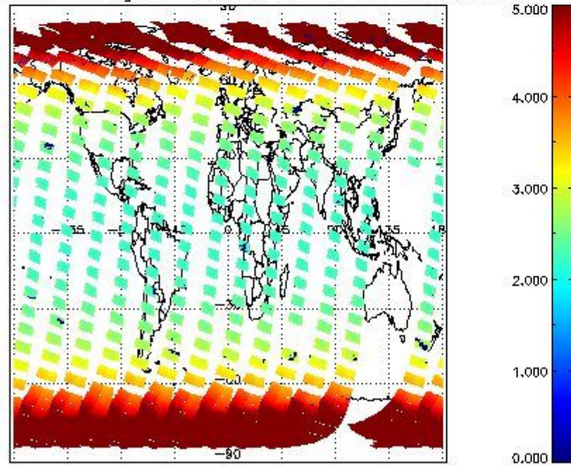
SCIOL2P_NADUV3BRO_amf_gr for 13MAR2011 00:00:00 to 14MAR2011 00:00:00
