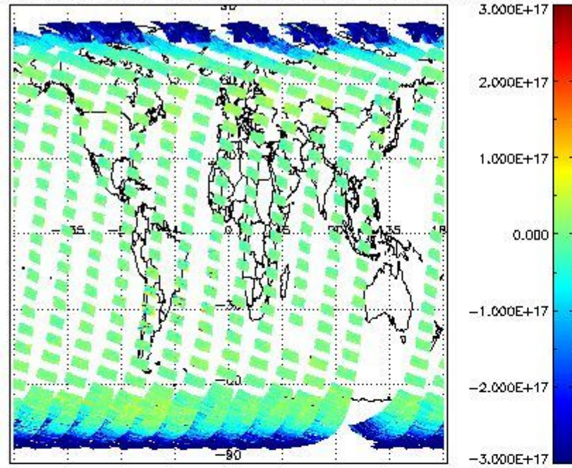
SCIOL2P_NADUV7S02_vcd for 13MAR2011 00:00:00 to 14MAR2011 00:00:00
