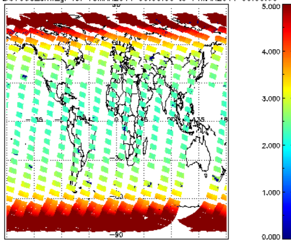
SCIOL2P_NADUV003_arnf_gr for 13MAR2011 00:00:00 to 14MAR2011 00:00:00
