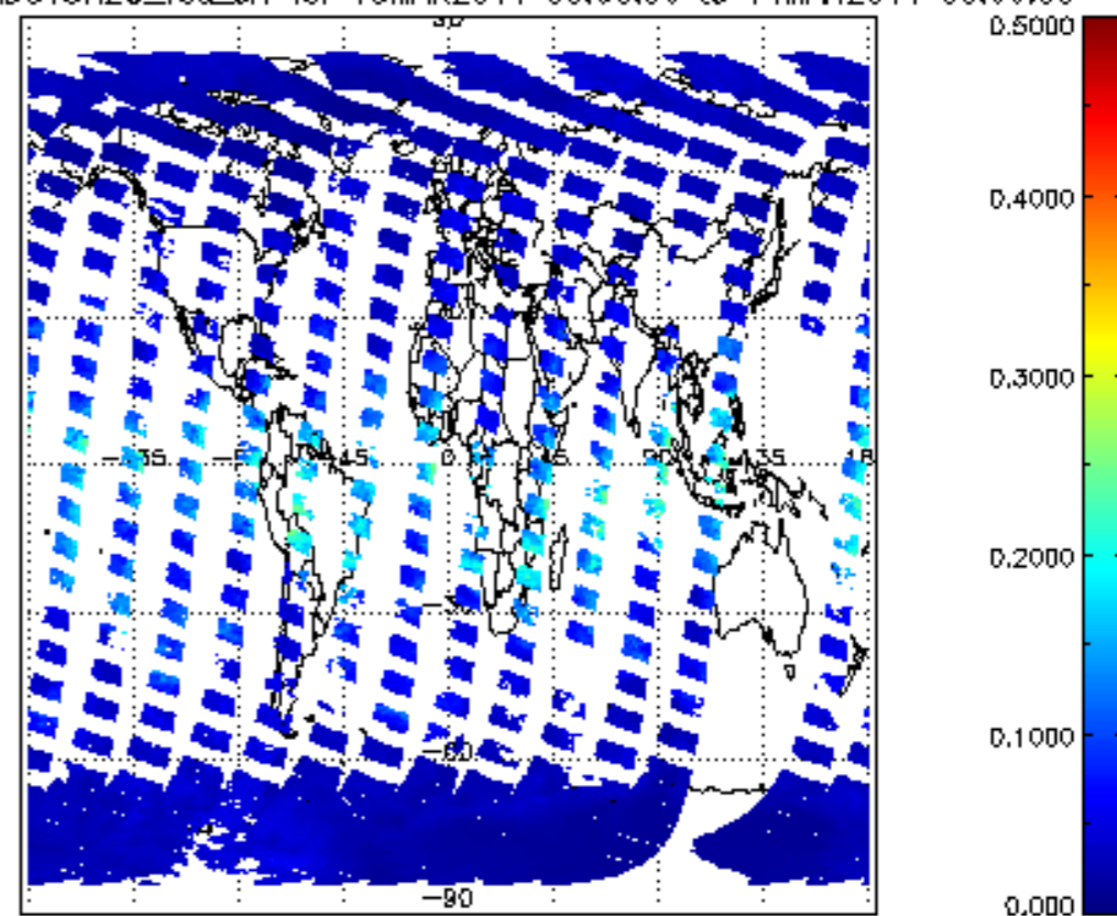
SCIOL2P_NADUV8H20_vcd_err for 13MAR2011 00:00:00 to 14MAR2011 00:00:00
