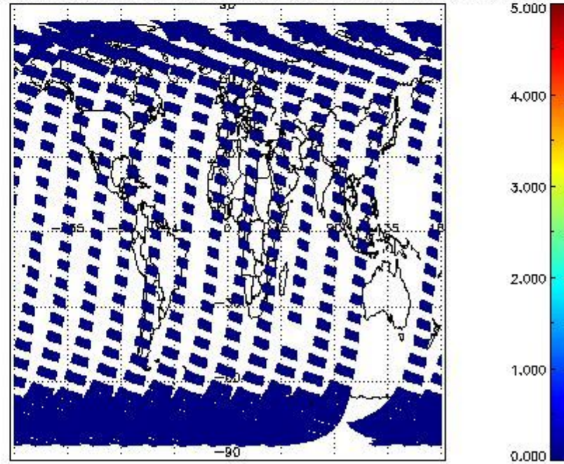
SCIOL2P_NADUV7S02_amf_cl for 13MAR2011 00:00:00 to 14MAR2011 00:00:00
