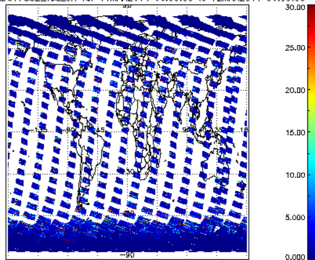
SCIOL2P_NADUV7S02_vcd_err for 11MAR2011 00:00:00 to 12MAR2011 00:00:00
