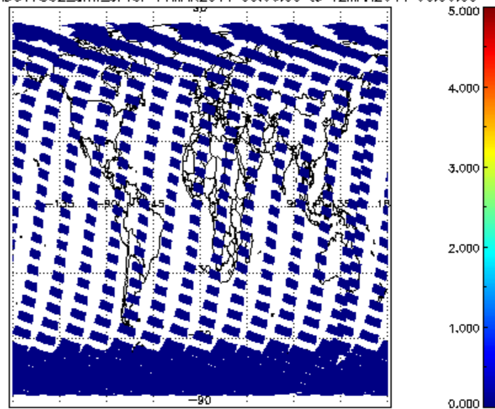
SCIOL2P_NADUV7S02_amf_cl for 11MAR2011 00:00:00 to 12MAR2011 00:00:00
