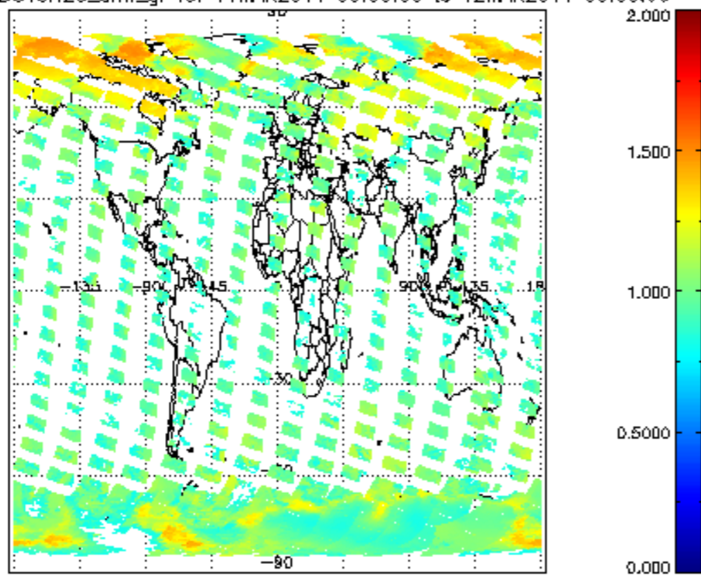
SCIOL2P_NADUV8H20_arnf_gr for 11MAR2011 00:00:00 to 12MAR2011 00:00:00
