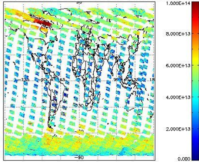
SCIOL2P_NADUV3BRO_vcd for 11MAR2011 00:00:00 to 12MAR2011 00:00:00
