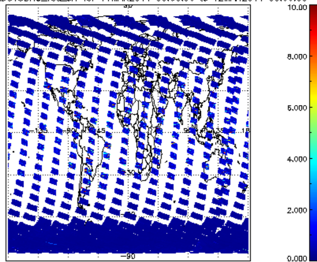
SCIOL2P_NADUV3BRO_vcd_err for 11MAR2011 00:00:00 to 12MAR2011 00:00:00
