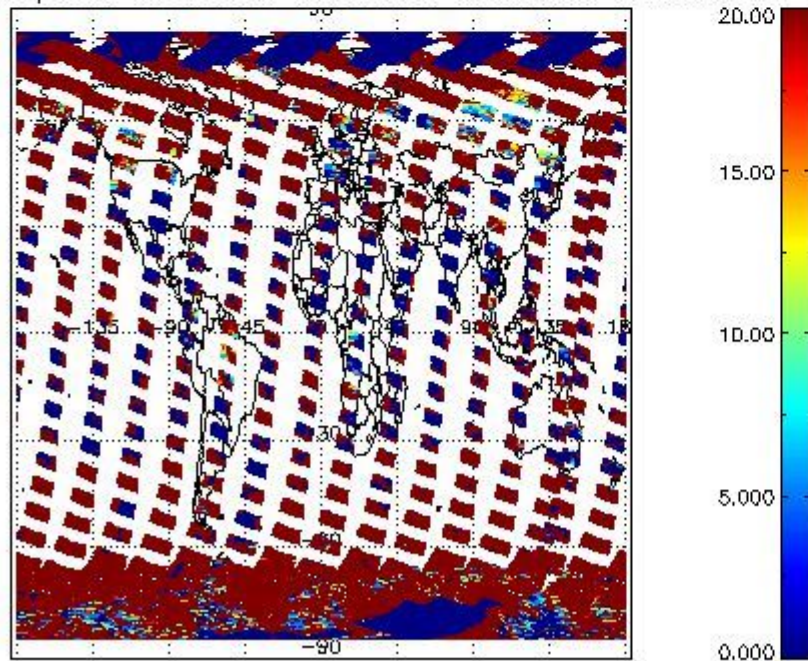
cL_opt_depth for 11MAR2011 00:00:00 to 12MAR2011 00:00:00
