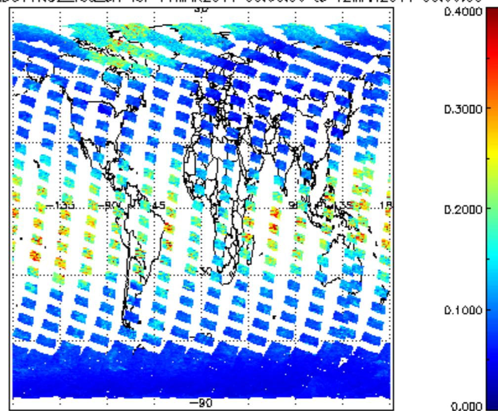
SCIOL2P_NADUV1NO2_vcd_err for 11MAR2011 00:00:00 to 12MAR2011 00:00:00
