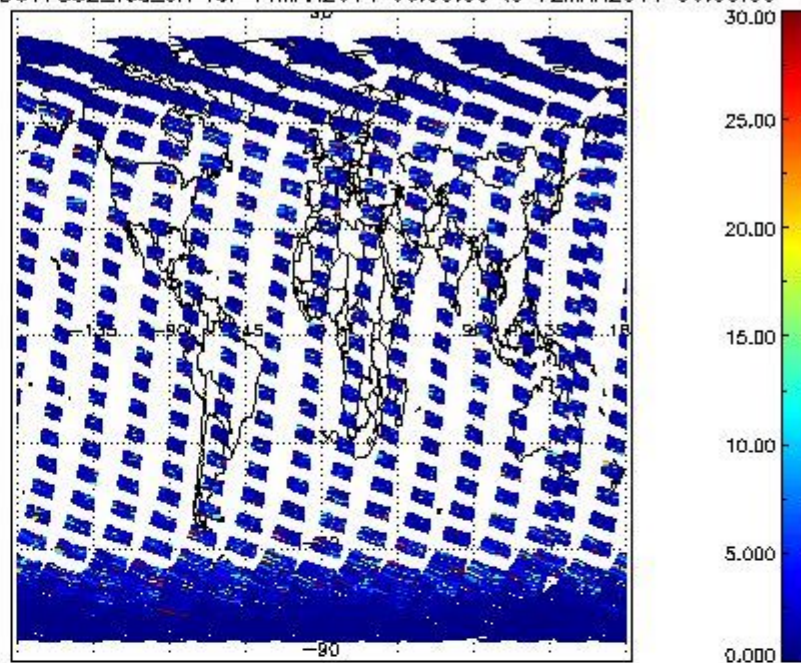
SCIOL2P_NADUV7S02_vcd_err for 11MAR2011 00:00:00 to 12MAR2011 00:00:00
