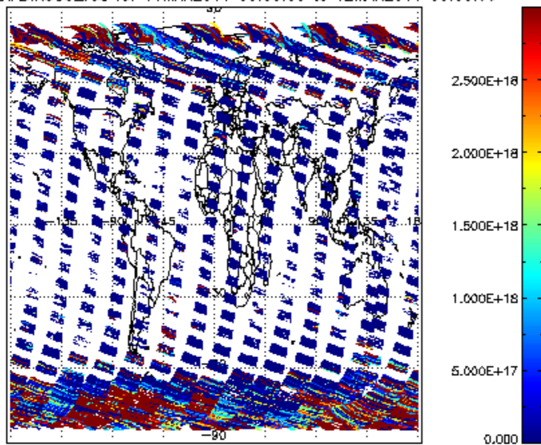
SCIOL2P_NADIR3CO_vcd for 11MAR2011 00:00:00 to 12MAR2011 00:00:00
