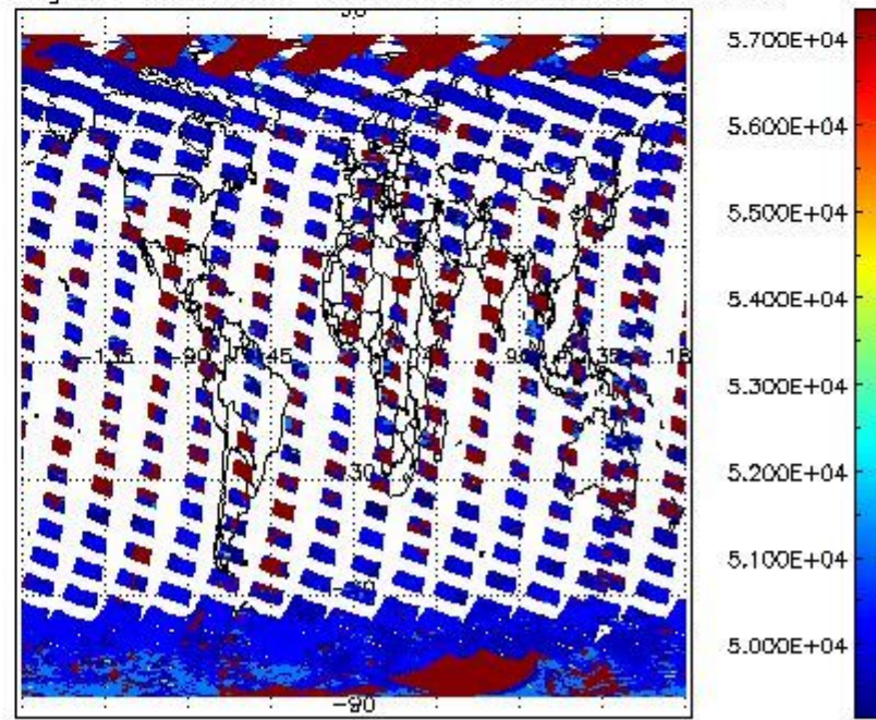
cloud_flags for 11MAR2011 00:00:00 to 12MAR2011 00:00:00
