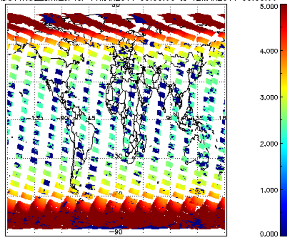
SCIOL2P_NADUV1NO2_amf_cl for 11MAR2011 00:00:00 to 12MAR2011 00:00:00
