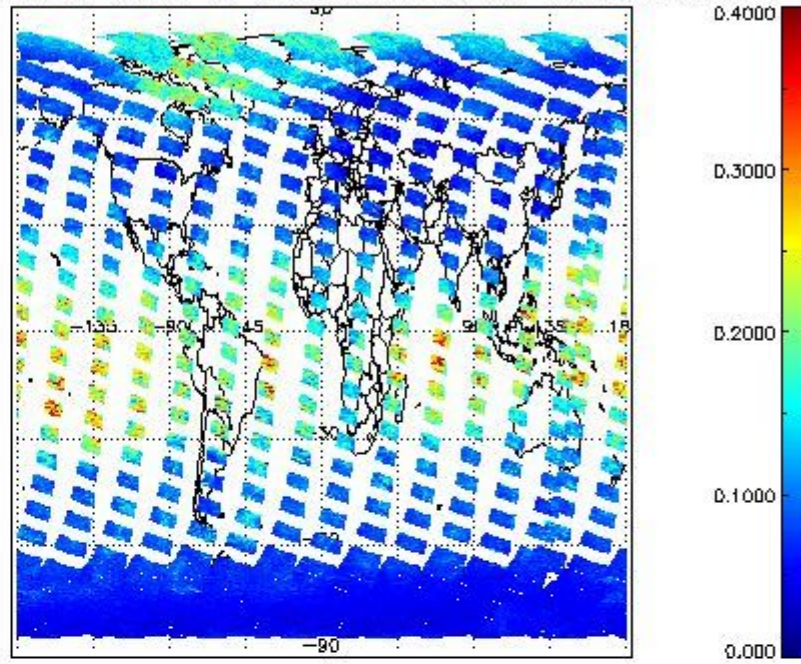
SCIOL2P_NADUV1NO2_vcd_err for 11MAR2011 00:00:00 to 12MAR2011 00:00:00
