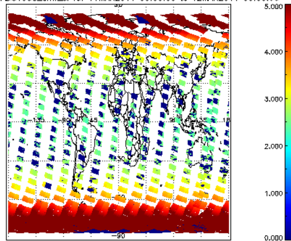
SCIOL2P_NADUV003_amf_cl for 11MAR2011 00:00:00 to 12MAR2011 00:00:00
