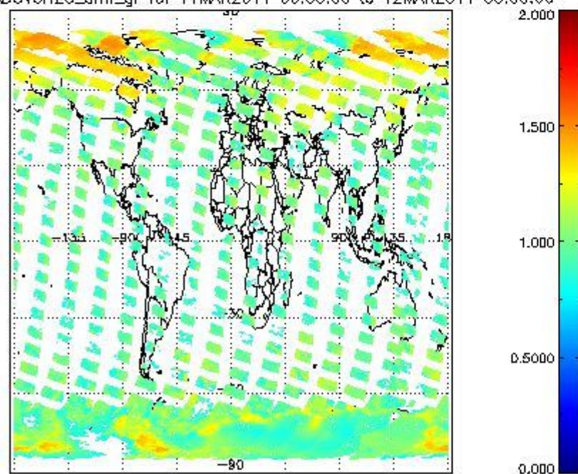
SCIOL2P_NADUV8H2O_amf_gr for 11MAR2011 00:00:00 to 12MAR2011 00:00:00
