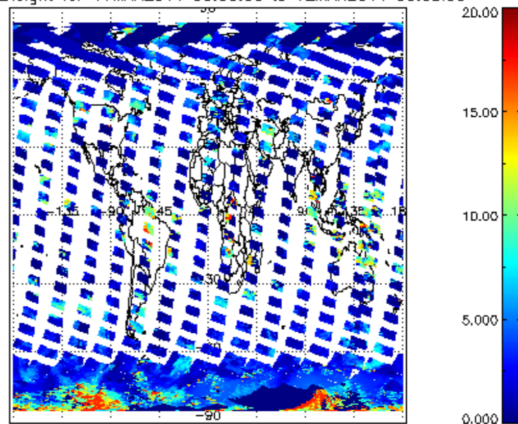
cL_top_height for 11MAR2011 00:00:00 to 12MAR2011 00:00:00
