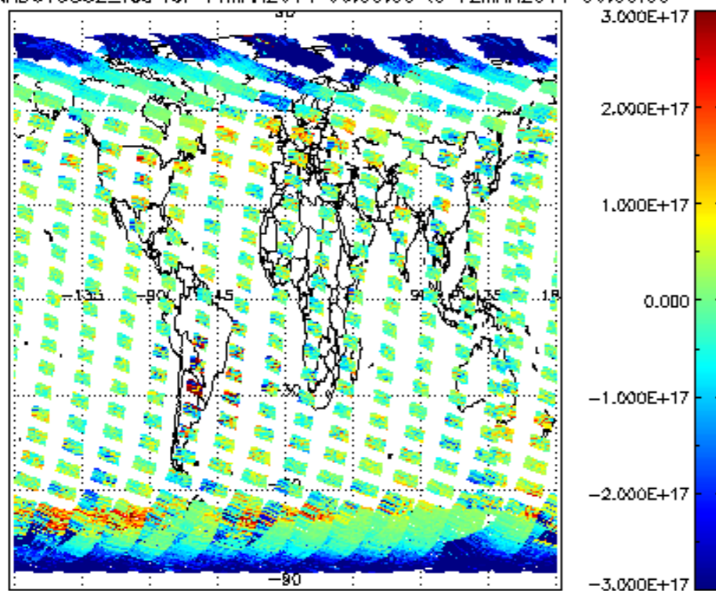
SCIOL2P_NADUV5S02_vcd for 11MAR2011 00:00:00 to 12MAR2011 00:00:00
