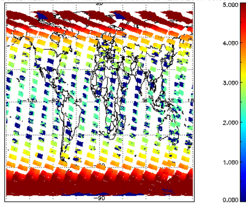
SCIOL2P_NADUV3BRO_amf_cl for 11MAR2011 00:00:00 to 12MAR2011 00:00:00
