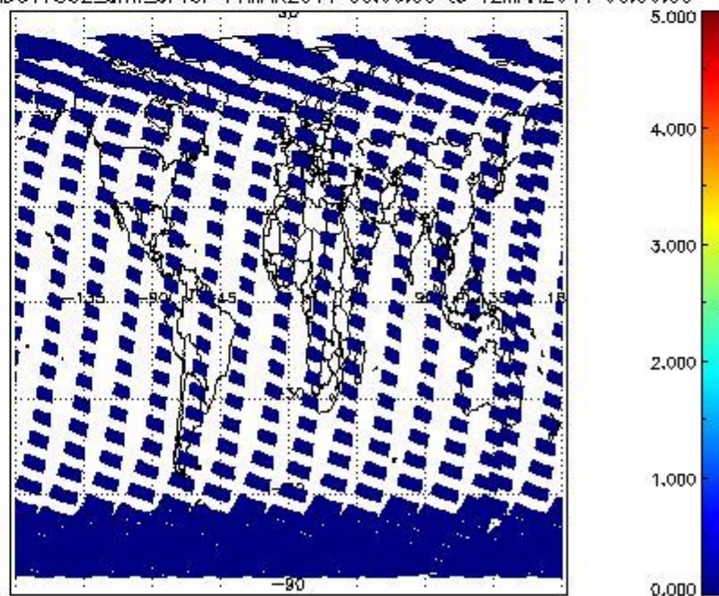
SCIOL2P_NADUV7S02_amf_cl for 11MAR2011 00:00:00 to 12MAR2011 00:00:00
