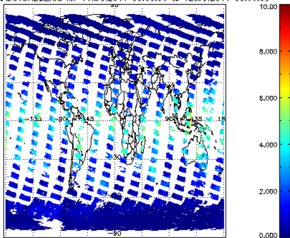
SCIOL2P_NADUV8H20_vcd for 11MAR2011 00:00:00 to 12MAR2011 00:00:00
