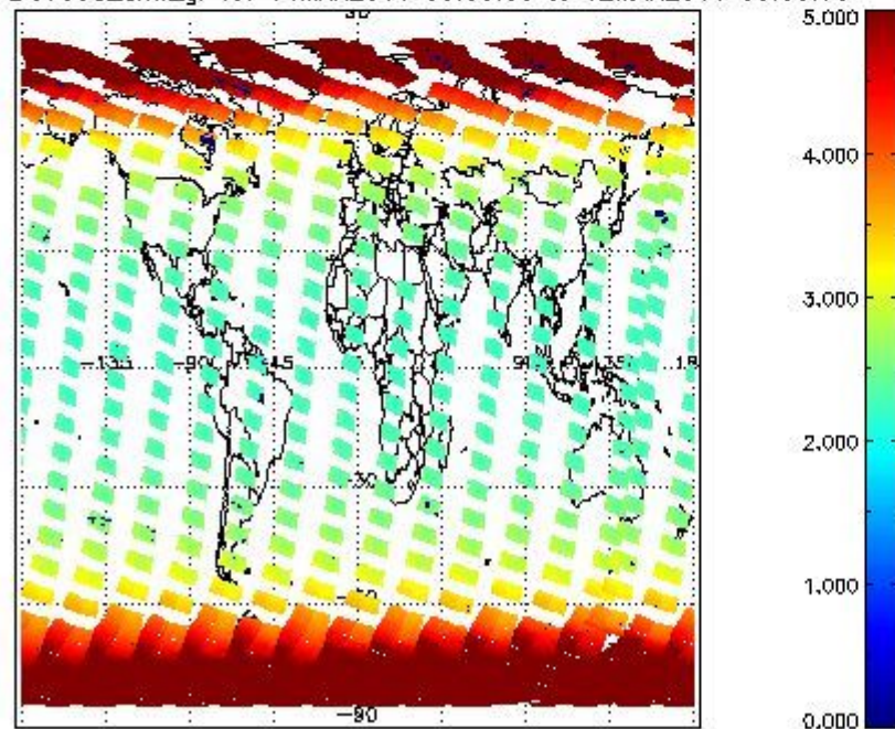
SCIOL2P_NADUV003_amf_gr for 11MAR2011 00:00:00 to 12MAR2011 00:00:00
