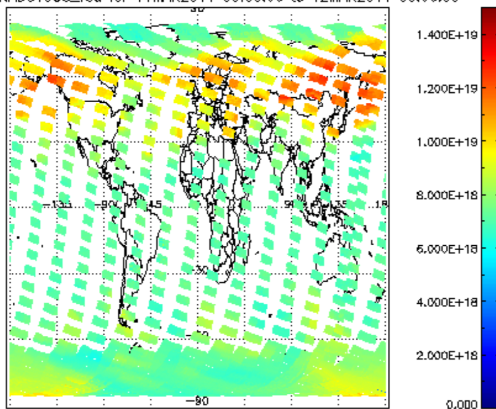
SCIOL2P_NADUV003_vcd for 11MAR2011 00:00:00 to 12MAR2011 00:00:00
