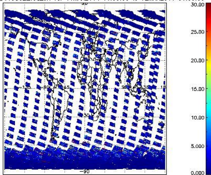
SCIOL2P_NADUV5SO2_vcd_err for 11MAR2011 00:00:00 to 12MAR2011 00:00:00
