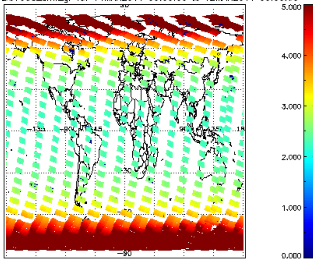
SCIOL2P_NADUV003_amf_gr for 11MAR2011 00:00:00 to 12MAR2011 00:00:00
