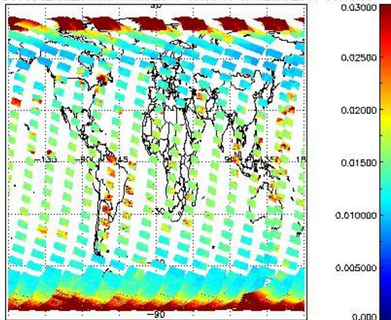
SCIOL2P_NADUV003_vcd_err for 11MAR2011 00:00:00 to 12MAR2011 00:00:00
