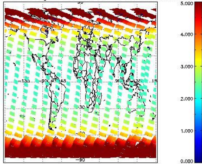
SCIOL2P_NADUV3BRO_amf_gr for 11MAR2011 00:00:00 to 12MAR2011 00:00:00
