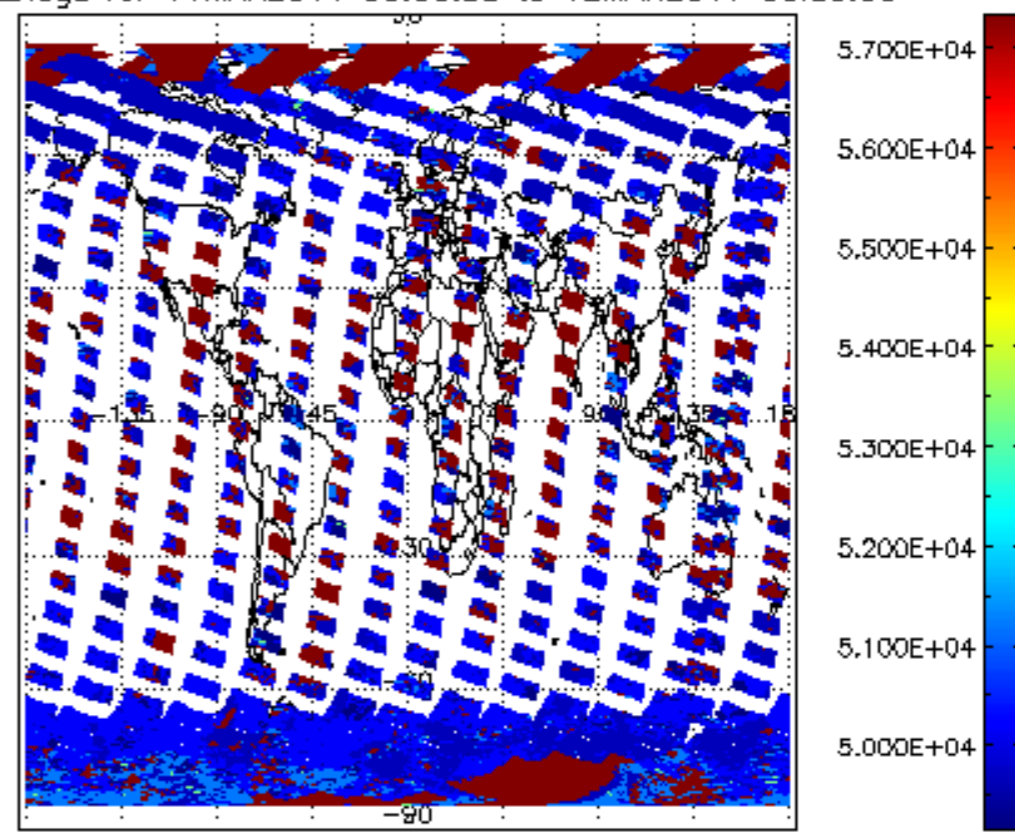
cloud_flags for 11MAR2011 00:00:00 to 12MAR2011 00:00:00
