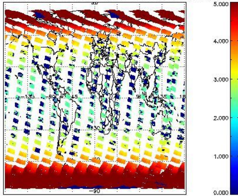
SCIOL2P_NADUV3BRO_amf_cl for 11MAR2011 00:00:00 to 12MAR2011 00:00:00
