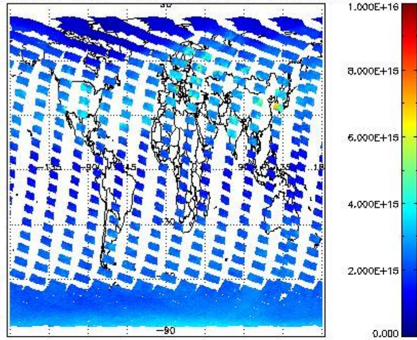
SCIOL2P_NADUV1NO2_vcd for 11MAR2011 00:00:00 to 12MAR2011 00:00:00
