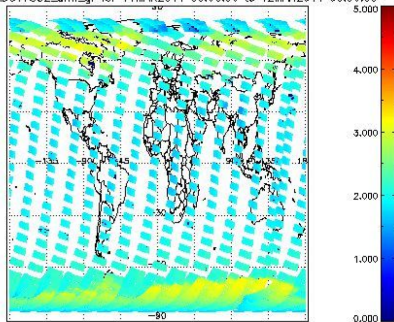
SCIOL2P_NADUV7S02_amf_gr for 11MAR2011 00:00:00 to 12MAR2011 00:00:00
