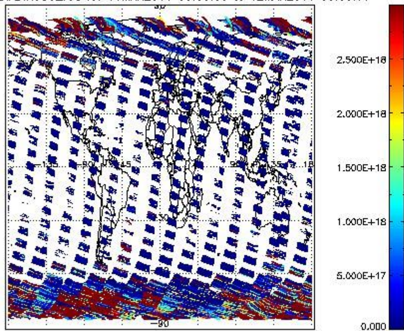
SCIDL2P_NADIR3CO_vcd for 11MAR2011 00:00:00 to 12MAR2011 00:00:00
