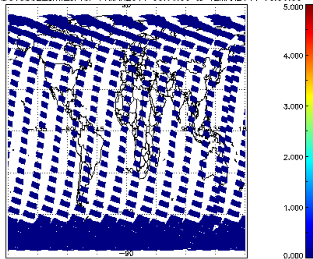
SCIOL2P_NADUV5S02_amf_cl for 11MAR2011 00:00:00 to 12MAR2011 00:00:00
