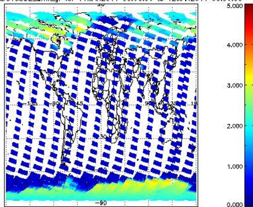
SCIOL2P_NADUV5SO2_amf_gr for 11MAR2011 00:00:00 to 12MAR2011 00:00:00
