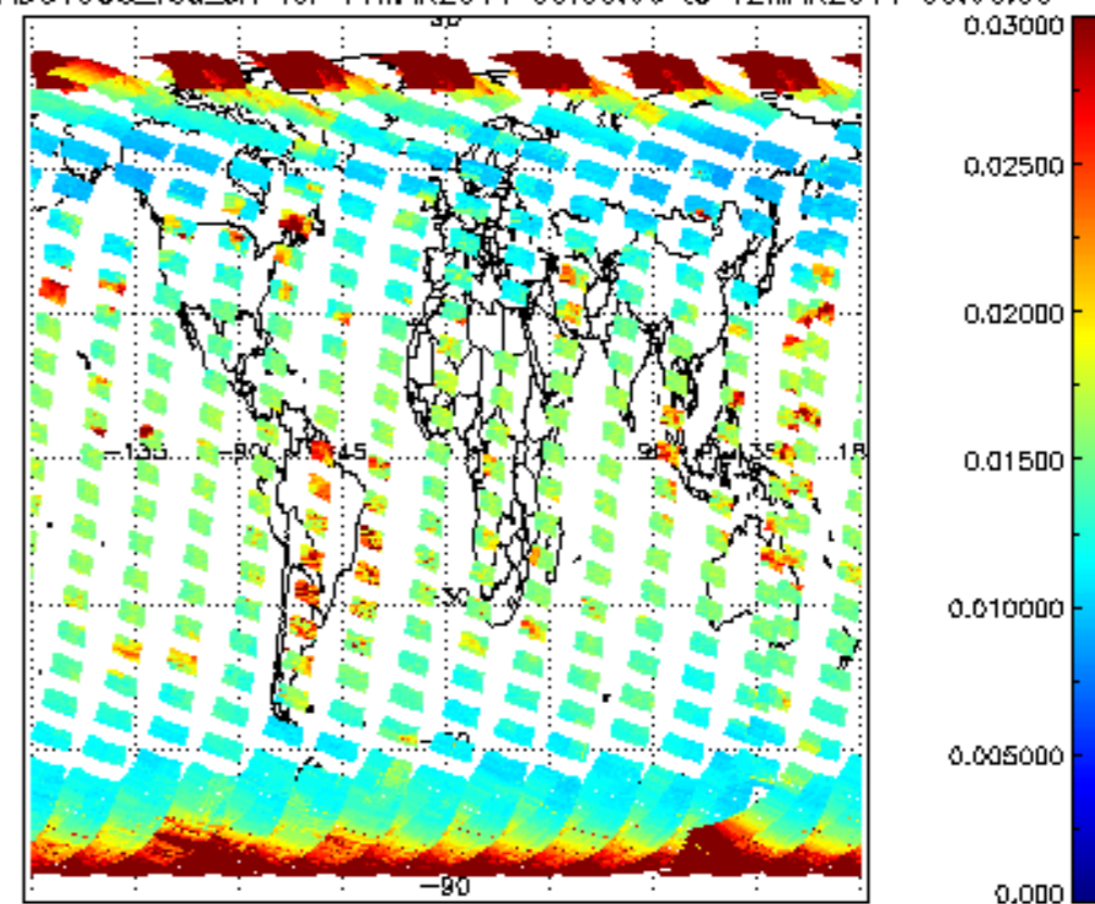
SCIOL2P_NADUV003_vcd_err for 11MAR2011 00:00:00 to 12MAR2011 00:00:00
