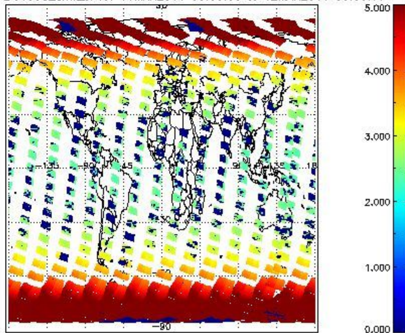
SCIOL2P_NADUV003_amf_cl for 11MAR2011 00:00:00 to 12MAR2011 00:00:00
