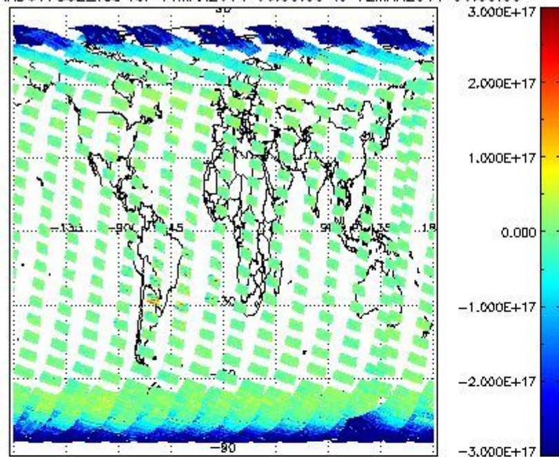
SCIOL2P_NADUV7S02_vcd for 11MAR2011 00:00:00 to 12MAR2011 00:00:00
