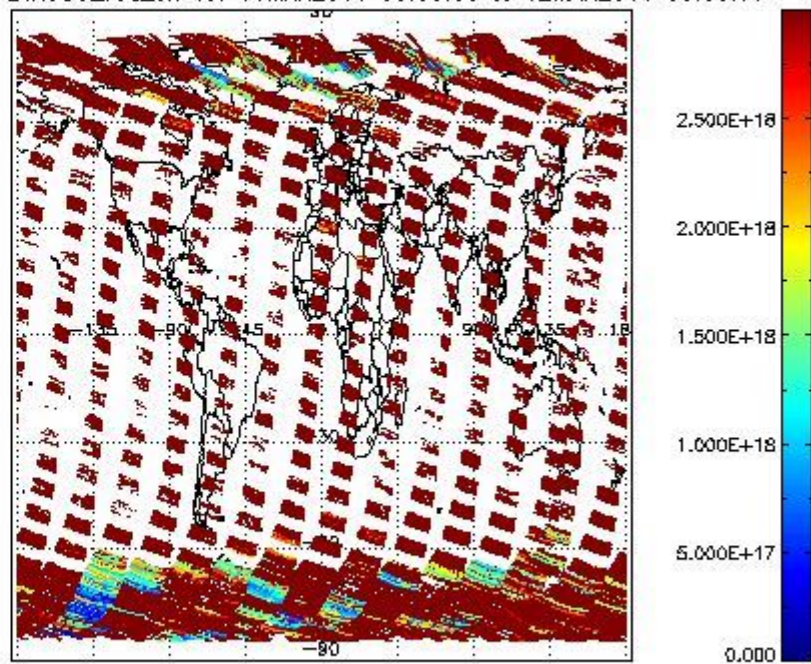
SCIDL2P_NADIR3CO_vcd_err for 11MAR2011 00:00:00 to 12MAR2011 00:00:00
