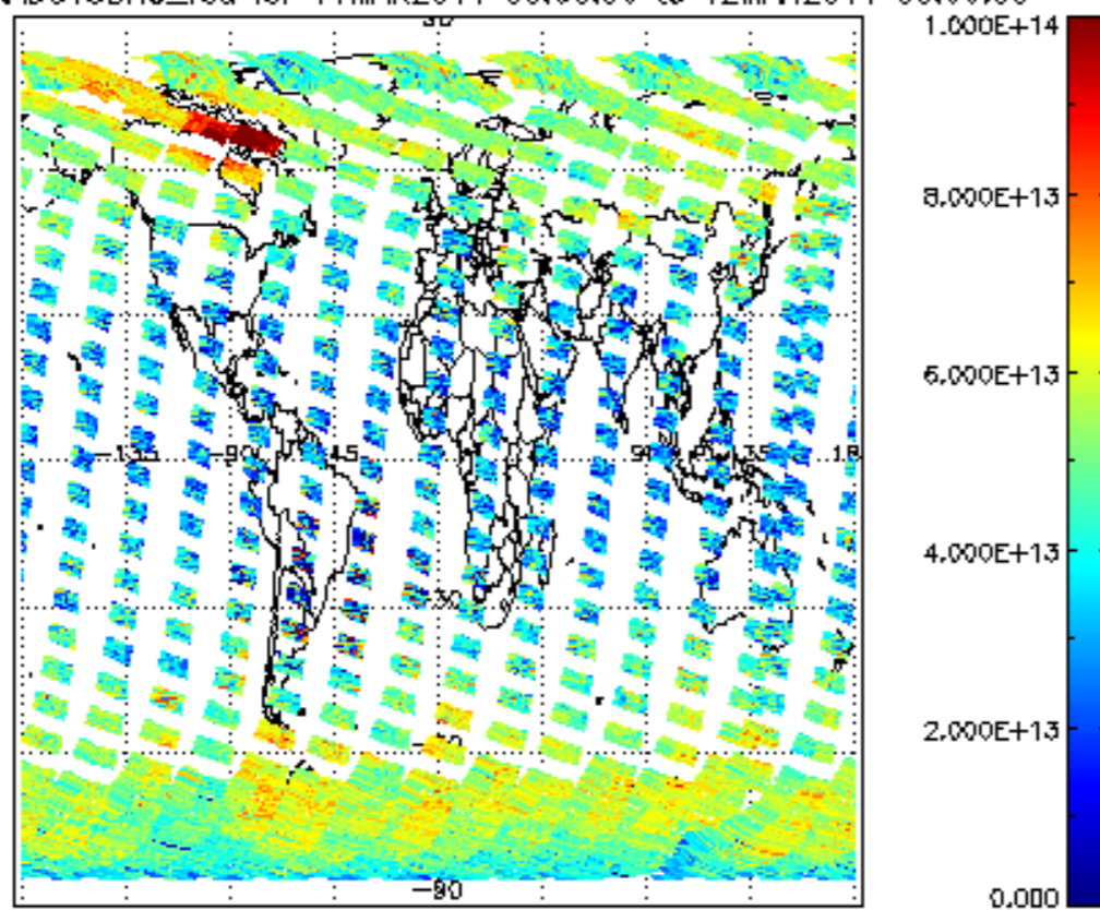
SCIOL2P_NADUV3BRO_vcd for 11MAR2011 00:00:00 to 12MAR2011 00:00:00
