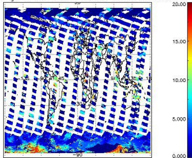
cL_top_height for 11MAR2011 00:00:00 to 12MAR2011 00:00:00
