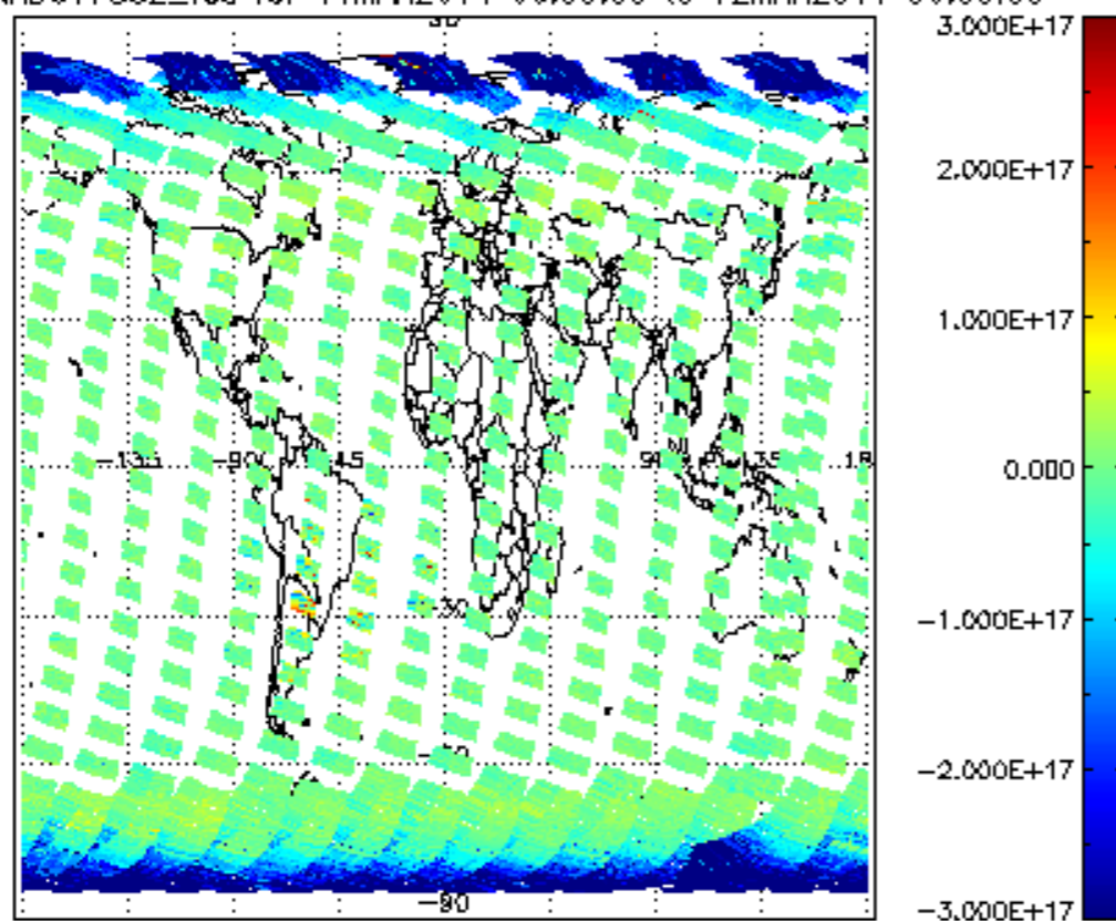
SCIOL2P_NADUV7S02_vcd for 11MAR2011 00:00:00 to 12MAR2011 00:00:00
