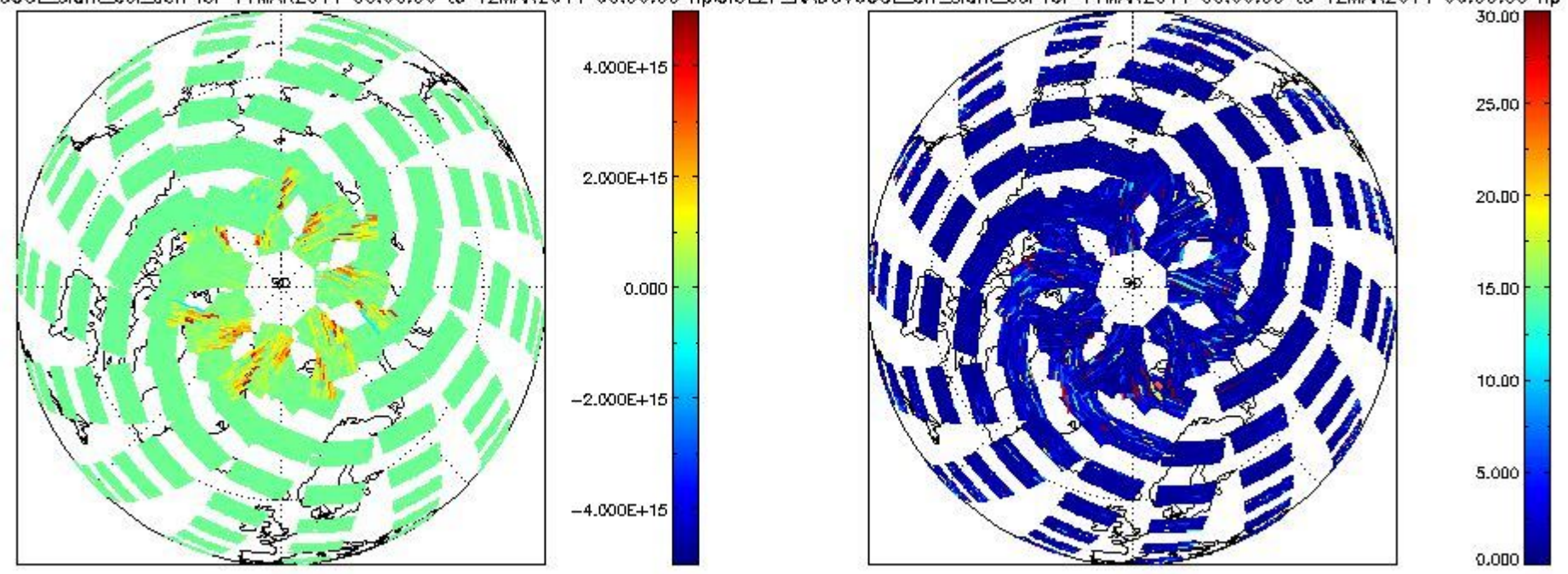
CIOL2P_NADUV6OCL_slant_col_den for 11MAR2011 00:00:00 to 12MAR2011 00:00:00 npCIOL2P_NADUV6OCL_err_slant_col for 11MAR2011 00:00:00 to 12MAR2011 00:00:00 np
