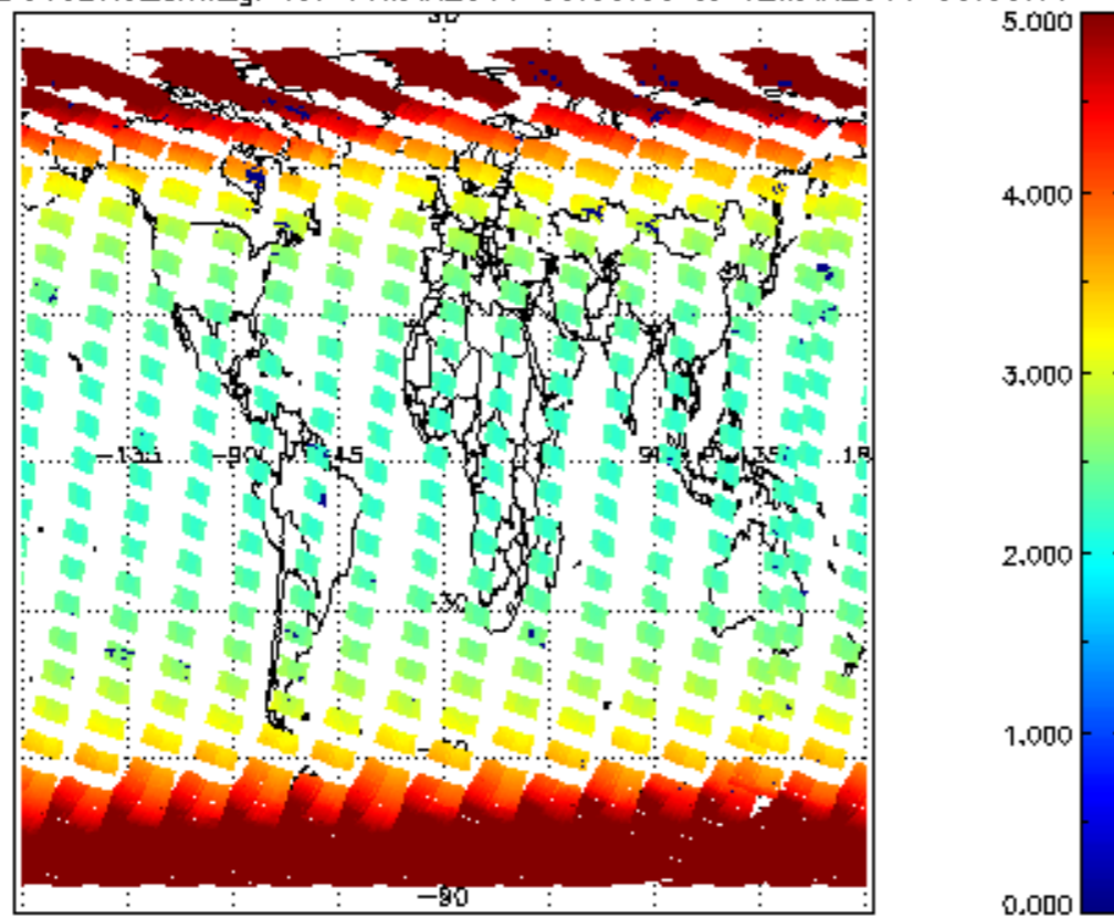
SCIOL2P_NADUV3BRO_amf_gr for 11MAR2011 00:00:00 to 12MAR2011 00:00:00
