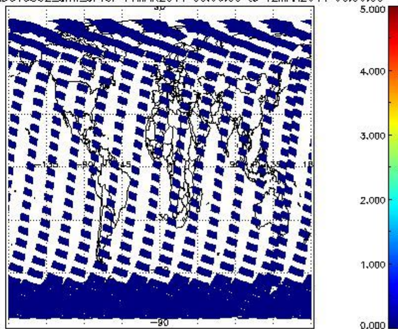
SCIOL2P_NADUV5SO2_amf_cl for 11MAR2011 00:00:00 to 12MAR2011 00:00:00
