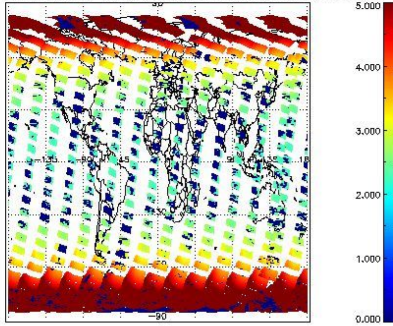
SCIOL2P_NADUV1NO2_amf_cl for 11MAR2011 00:00:00 to 12MAR2011 00:00:00
