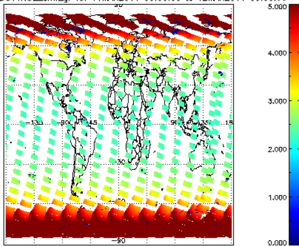
SCIOL2P_NADUV1NO2_amf_gr for 11MAR2011 00:00:00 to 12MAR2011 00:00:00
