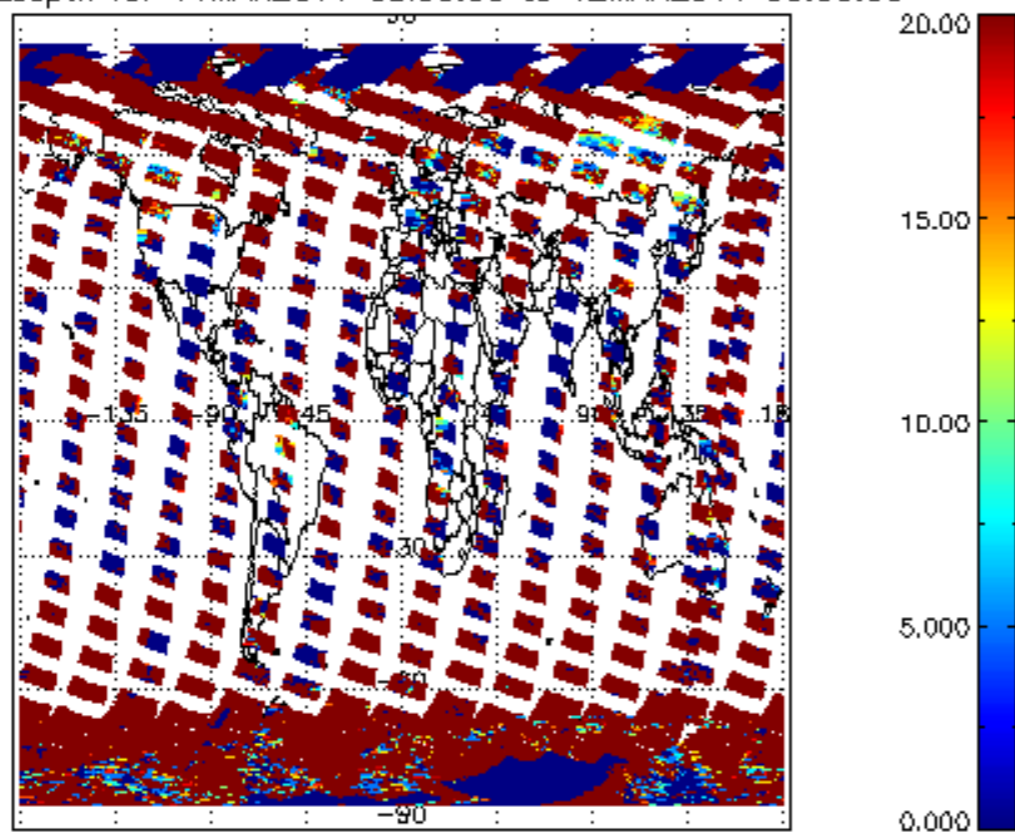
cL_opt_depth for 11MAR2011 00:00:00 to 12MAR2011 00:00:00
