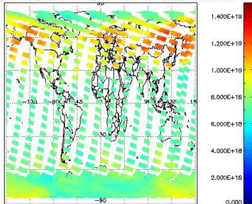
SCIOL2P_NADUV003_vcd for 11MAR2011 00:00:00 to 12MAR2011 00:00:00
