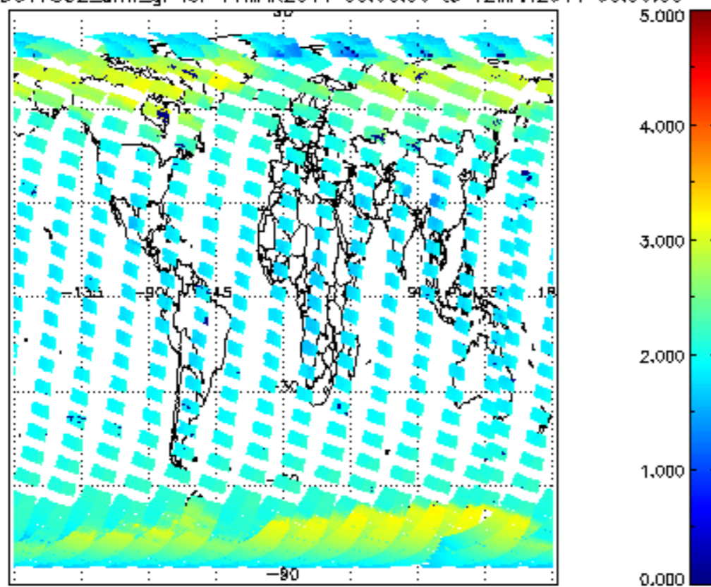
SCIOL2P_NADUV7S02_amf_gr for 11MAR2011 00:00:00 to 12MAR2011 00:00:00
