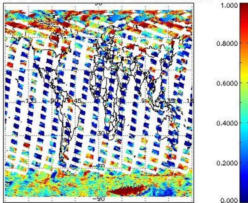
cL_frac for 11MAR2011 00:00:00 to 12MAR2011 00:00:00
