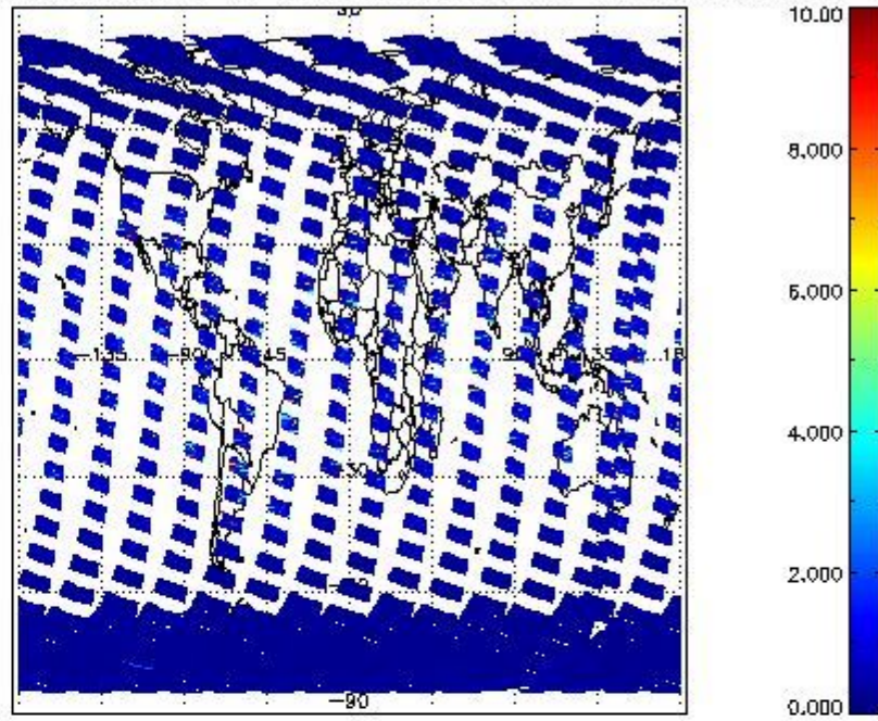
SCIOL2P_NADUV3BRO_vcd_err for 11MAR2011 00:00:00 to 12MAR2011 00:00:00
