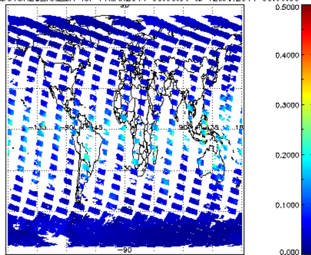
SCIOL2P_NADUV8H20_vcd_err for 11MAR2011 00:00:00 to 12MAR2011 00:00:00
