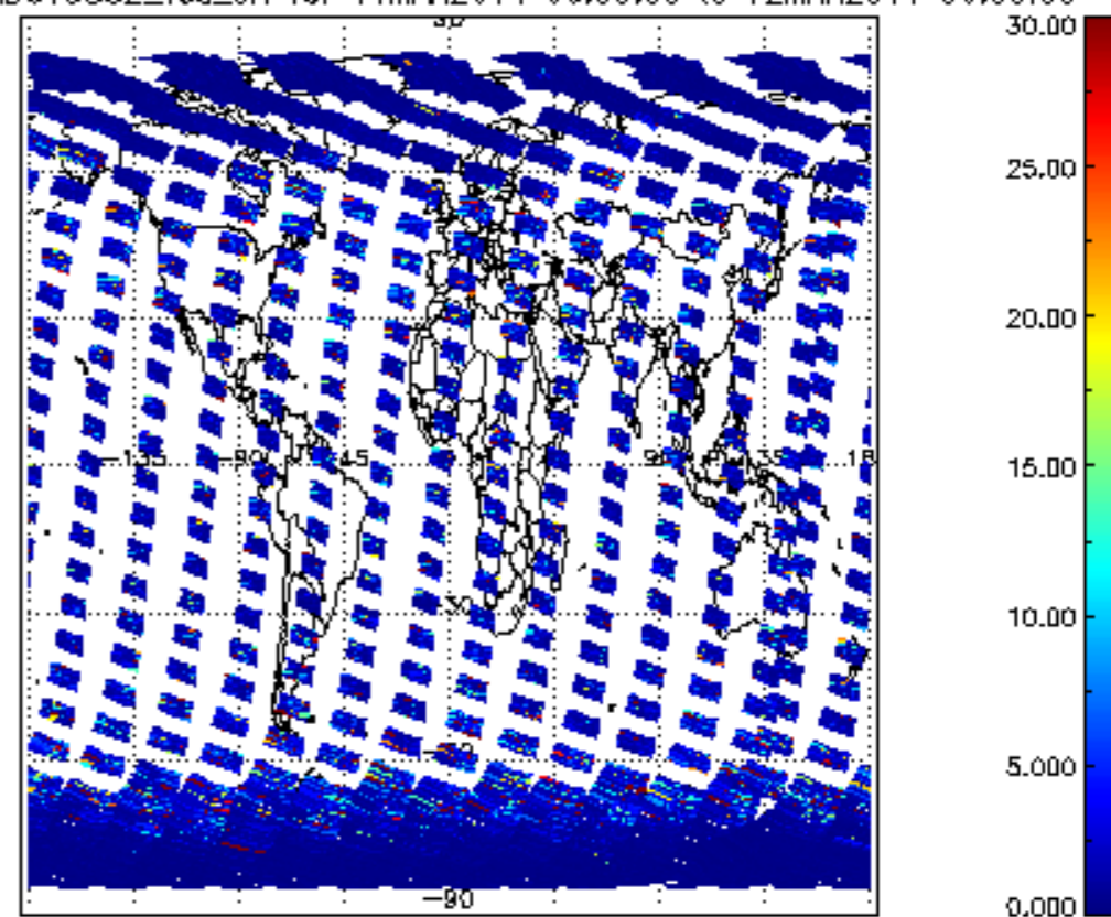
SCIOL2P_NADUV5S02_vcd_err for 11MAR2011 00:00:00 to 12MAR2011 00:00:00
