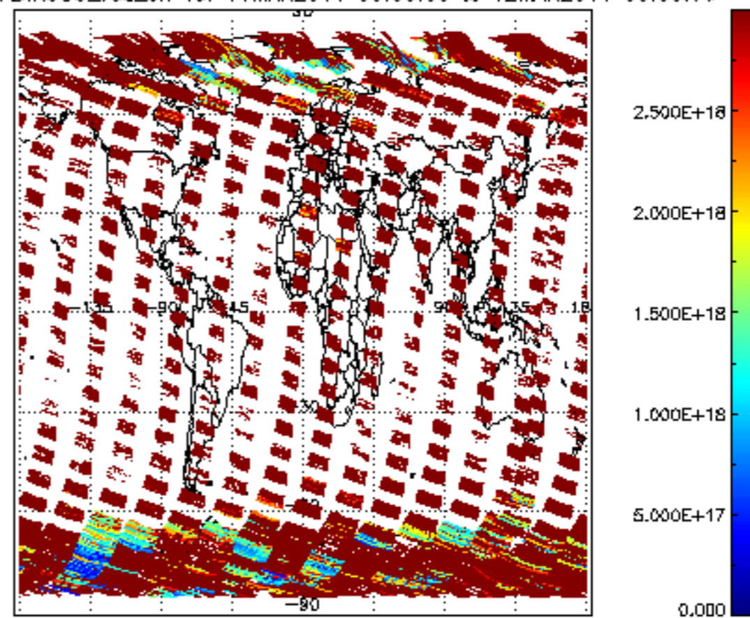
SCIOL2P_NADIR3CO_vcd_err for 11MAR2011 00:00:00 to 12MAR2011 00:00:00
