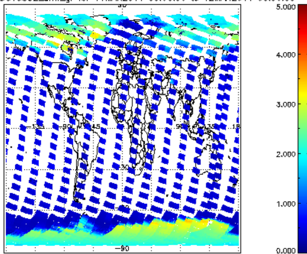
SCIOL2P_NADUV5S02_amf_gr for 11MAR2011 00:00:00 to 12MAR2011 00:00:00
