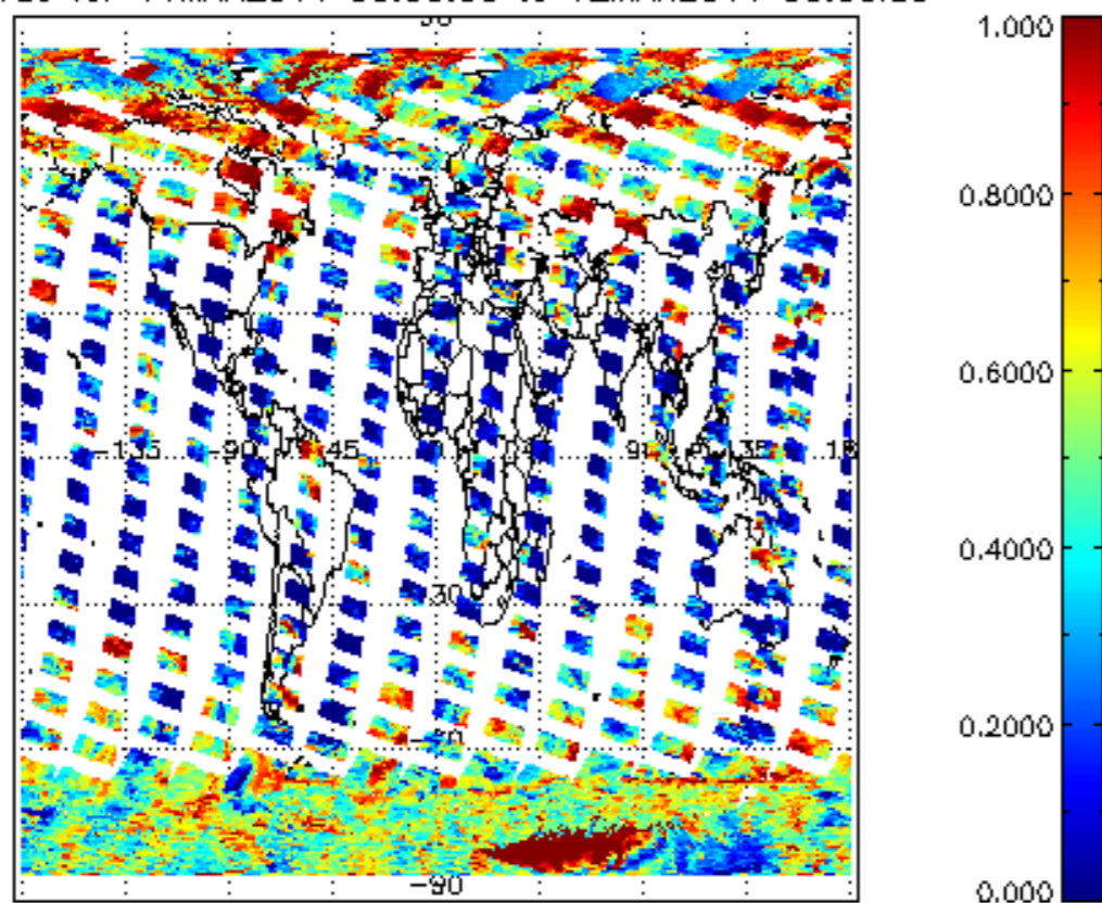
cLfrac for 11MAR2011 00:00:00 to 12MAR2011 00:00:00
