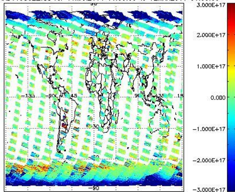
SCIOL2P_NADUV5SO2_vcd for 11MAR2011 00:00:00 to 12MAR2011 00:00:00
