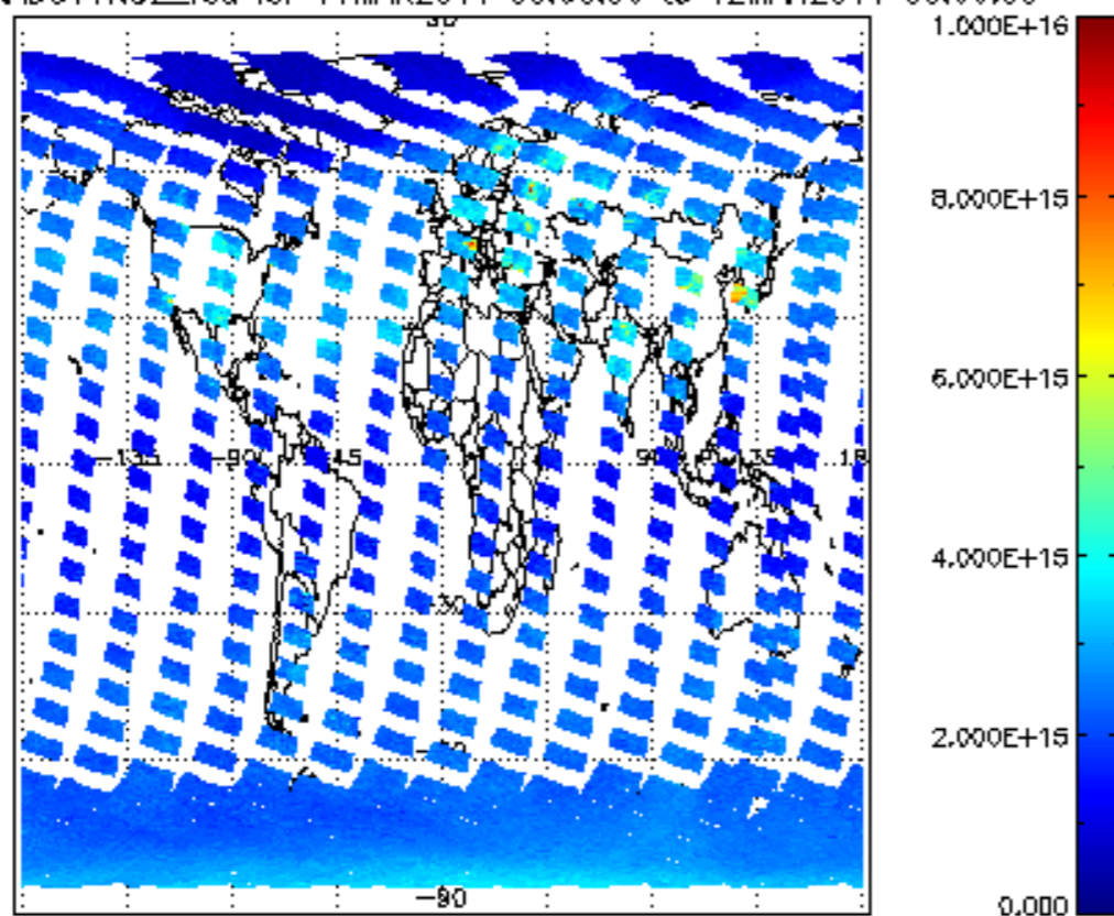
SCIOL2P_NADUV1NO2_vcd for 11MAR2011 00:00:00 to 12MAR2011 00:00:00
