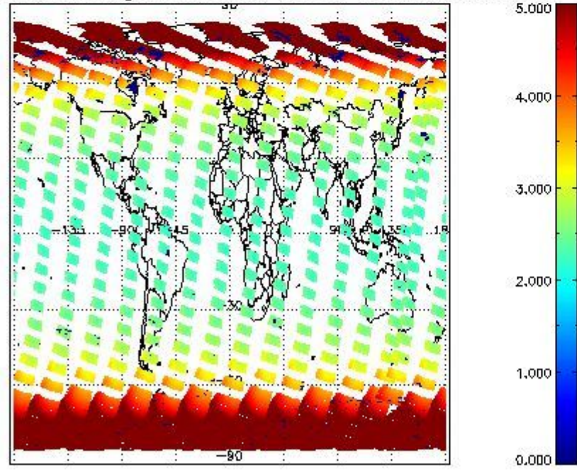
SCIOL2P_NADUV1NO2_amf_gr for 11MAR2011 00:00:00 to 12MAR2011 00:00:00
