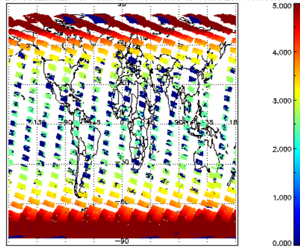
SCIOL2P_NADUV003_arnf_cl for 09MAR2011 00:00:00 to 10MAR2011 00:00:00
