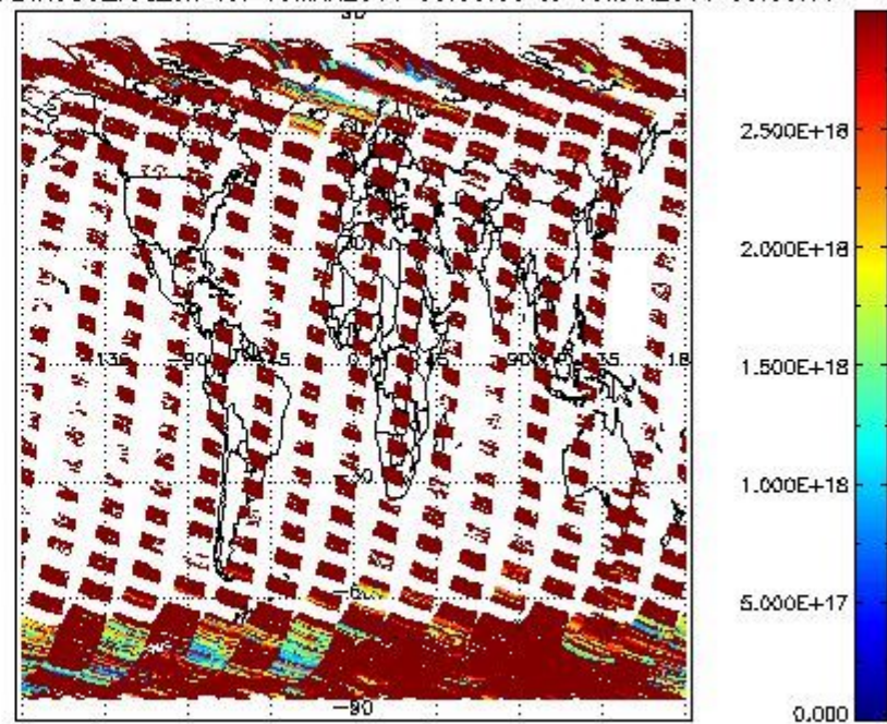
SCIDL2P_NADIR3CO_vcd_err for 09MAR2011 00:00:00 to 10MAR2011 00:00:00
