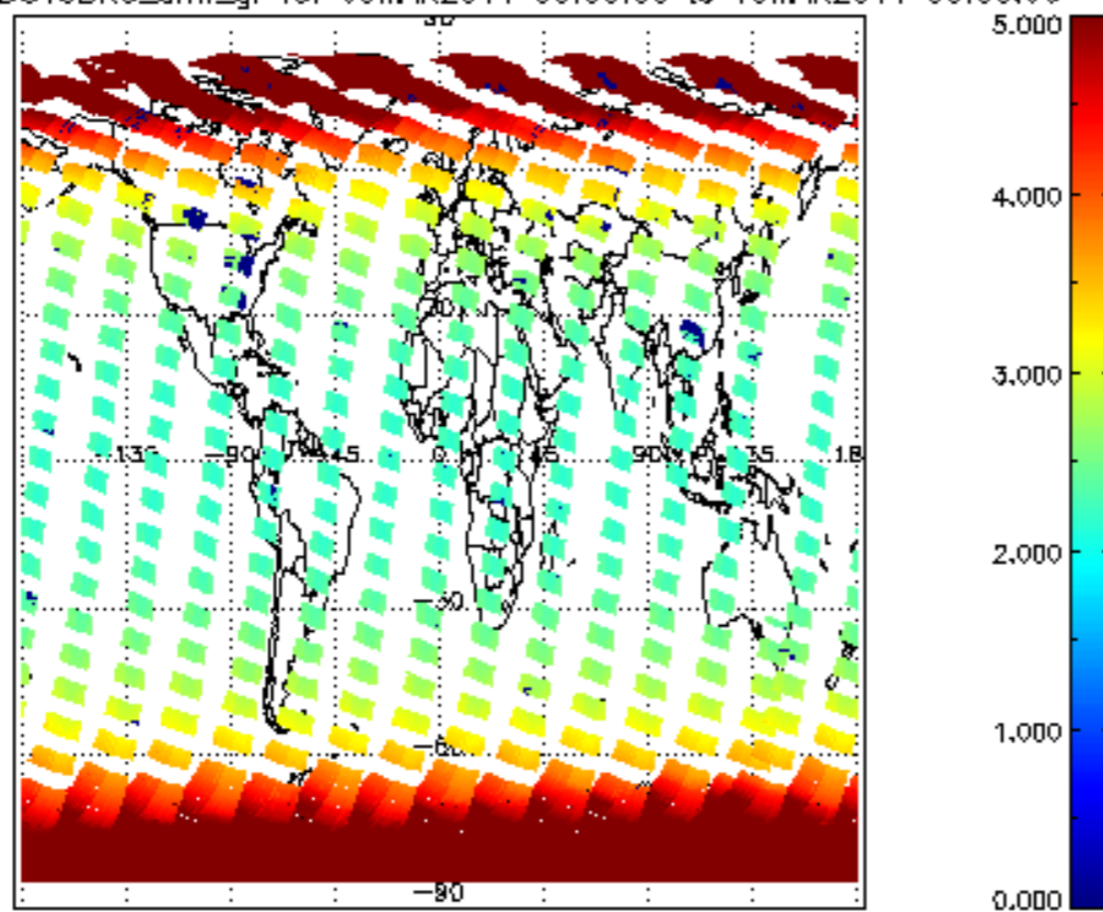
SCIOL2P_NADUV3BRO_amf_gr for 09MAR2011 00:00:00 to 10MAR2011 00:00:00
