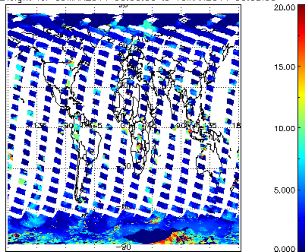
cL_top_height for 09MAR2011 00:00:00 to 10MAR2011 00:00:00
