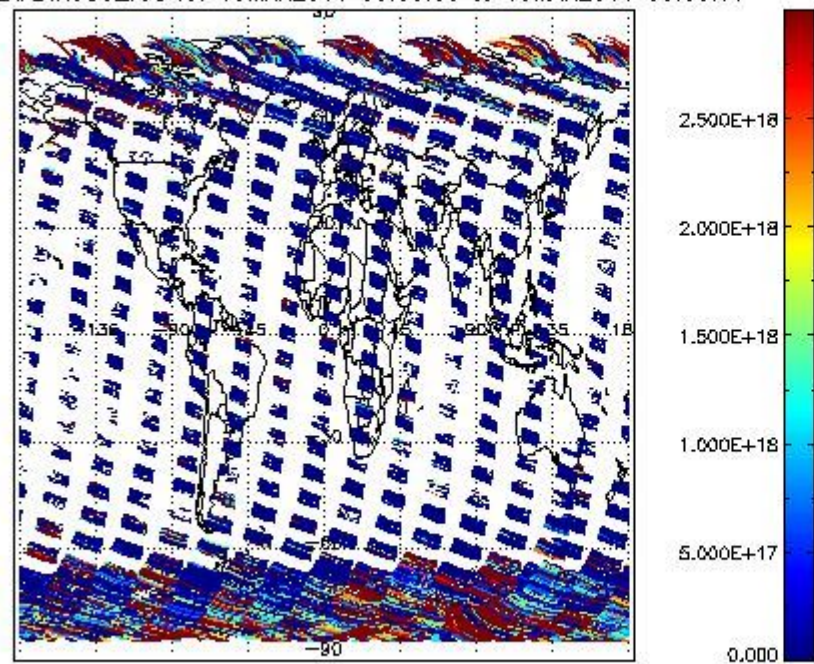
SCIDL2P_NADIR3CO_vcd for 09MAR2011 00:00:00 to 10MAR2011 00:00:00
