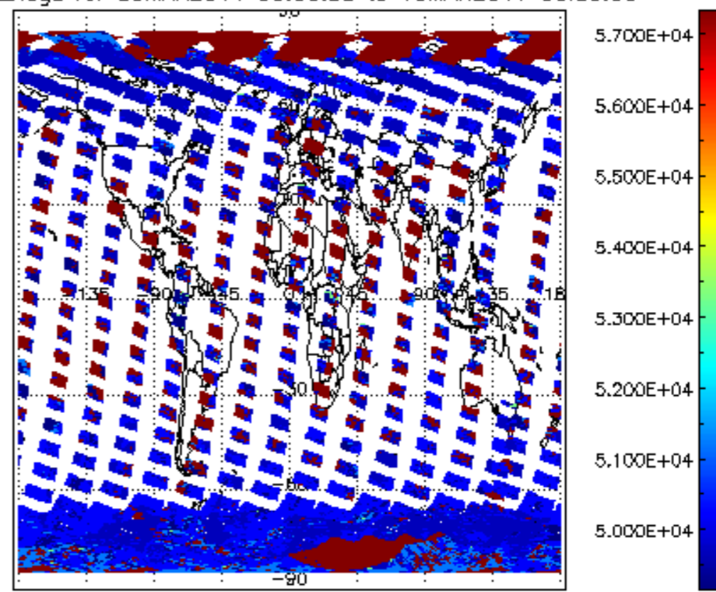
cloud_flags for 09MAR2011 00:00:00 to 10MAR2011 00:00:00
