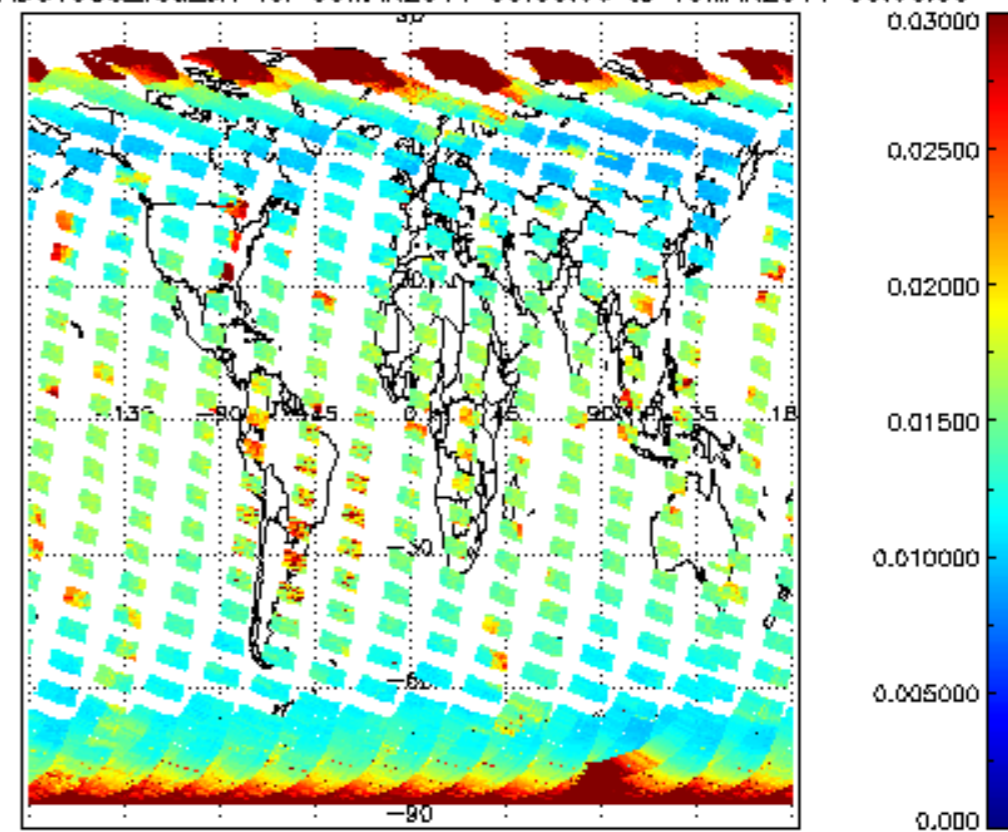
SCIOL2P_NADUV003_vcd_err for 09MAR2011 00:00:00 to 10MAR2011 00:00:00
