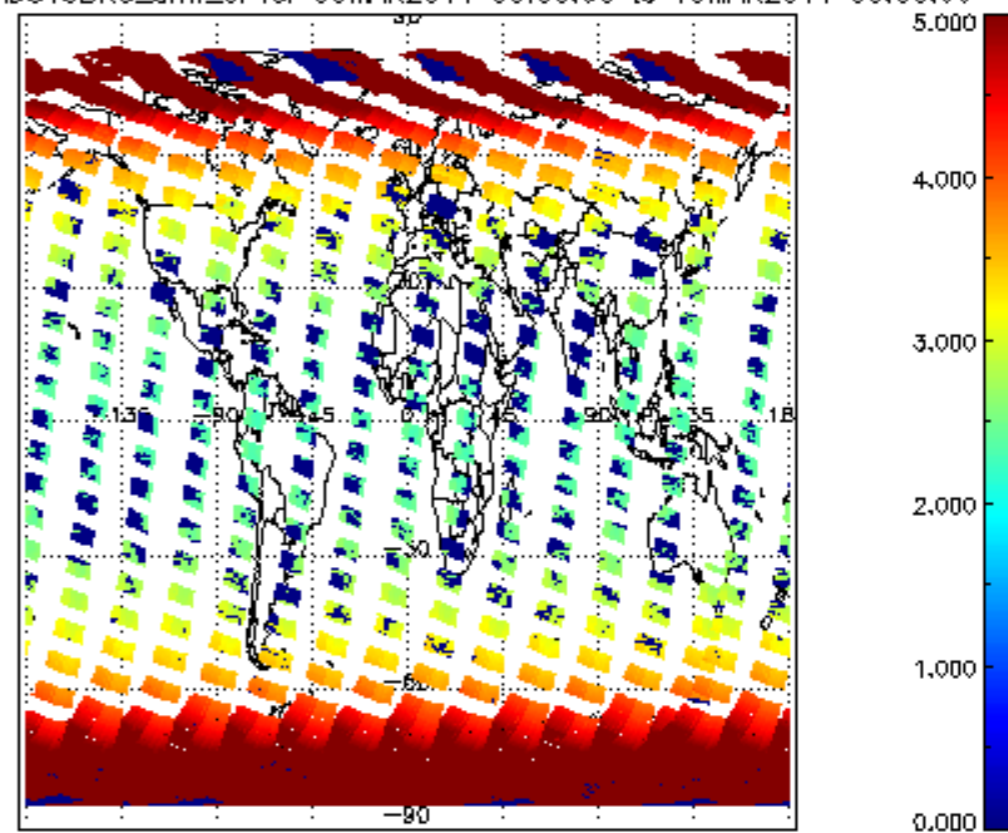
SCIOL2P_NADUV3BRO_amf_cl for 09MAR2011 00:00:00 to 10MAR2011 00:00:00
