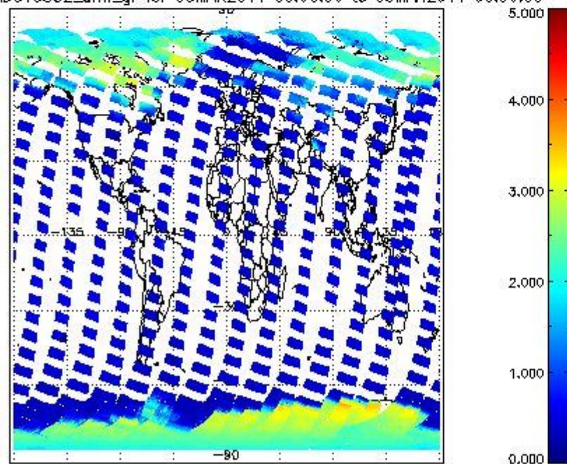
SCIOL2P_NADUV5S02_amf_gr for 08MAR2011 00:00:00 to 09MAR2011 00:00:00
