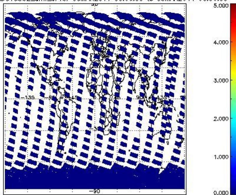
SCIOL2P_NADUV5S02_amf_cl for 08MAR2011 00:00:00 to 09MAR2011 00:00:00
