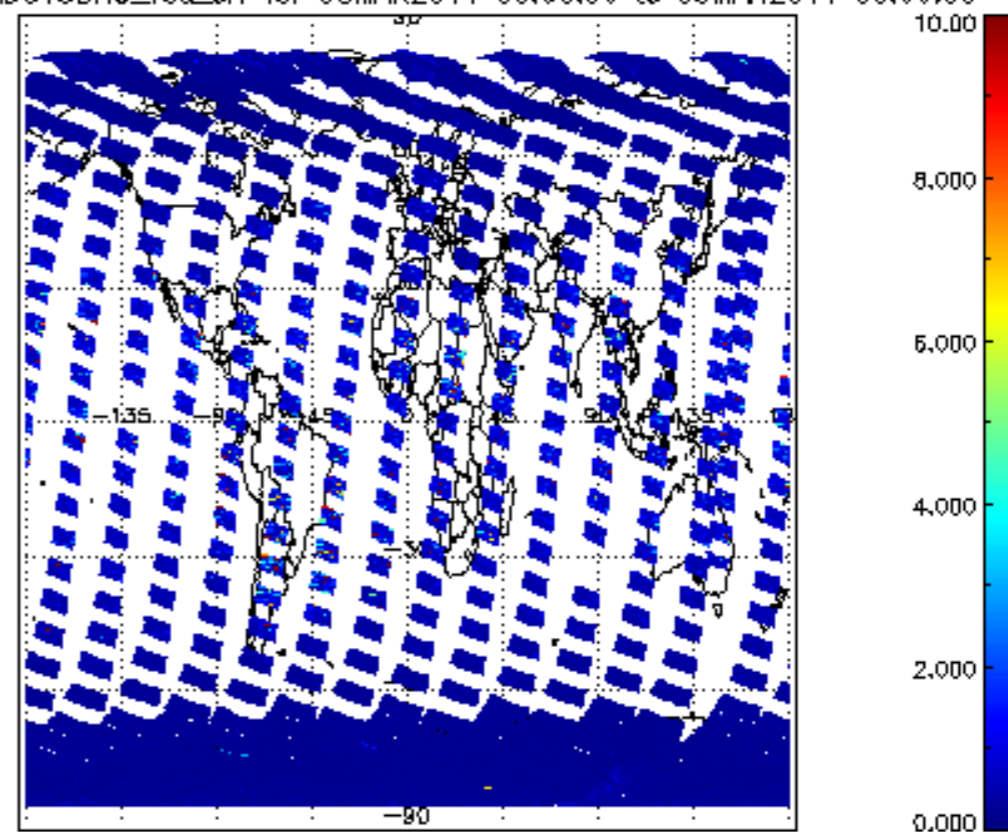
SCIOL2P_NADUV3BRO_vcd_err for 08MAR2011 00:00:00 to 09MAR2011 00:00:00
