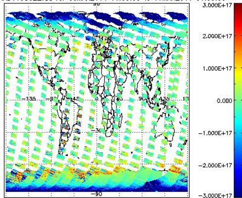
SCIOL2P_NADUV5S02_vcd for 08MAR2011 00:00:00 to 09MAR2011 00:00:00
