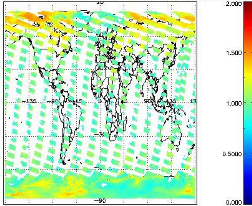
SCIOL2P_NADUV8H2O_amb_gr for 08MAR2011 00:00:00 to 09MAR2011 00:00:00
