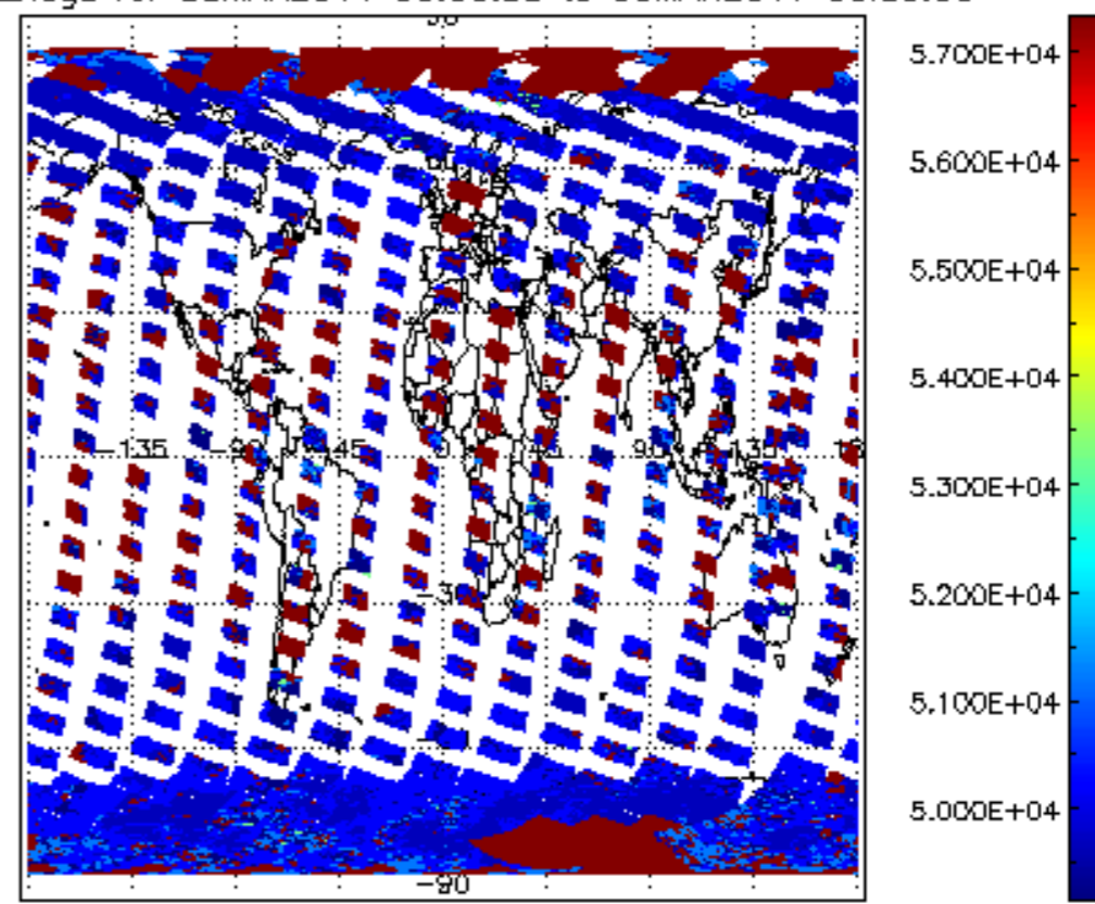
cloud_flags for 08MAR2011 00:00:00 to 09MAR2011 00:00:00
