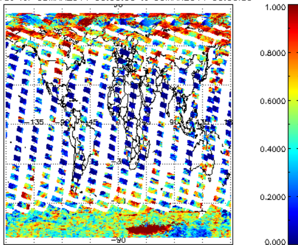
cL_frac for 08MAR2011 00:00:00 to 09MAR2011 00:00:00
