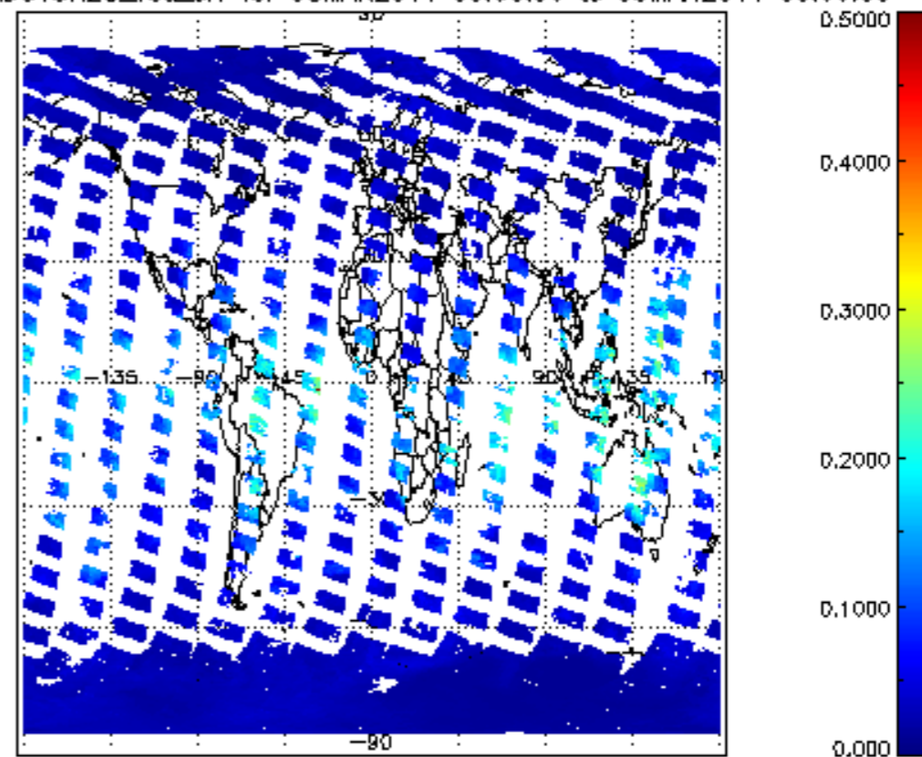
SCIOL2P_NADUV8H20_vcd_err for 08MAR2011 00:00:00 to 09MAR2011 00:00:00
