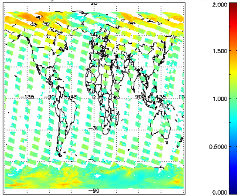
SCIOL2P_NADUV8H20_arnf_gr for 08MAR2011 00:00:00 to 09MAR2011 00:00:00
