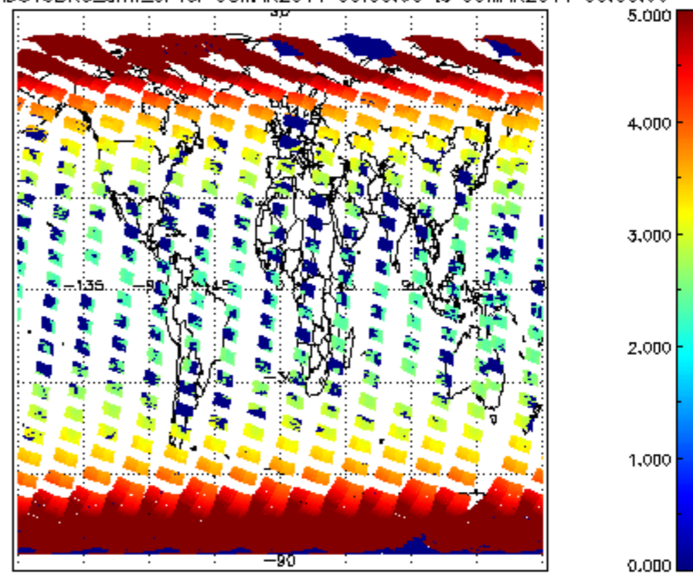
SCIOL2P_NADUV3BRO_amf_cl for 08MAR2011 00:00:00 to 09MAR2011 00:00:00
