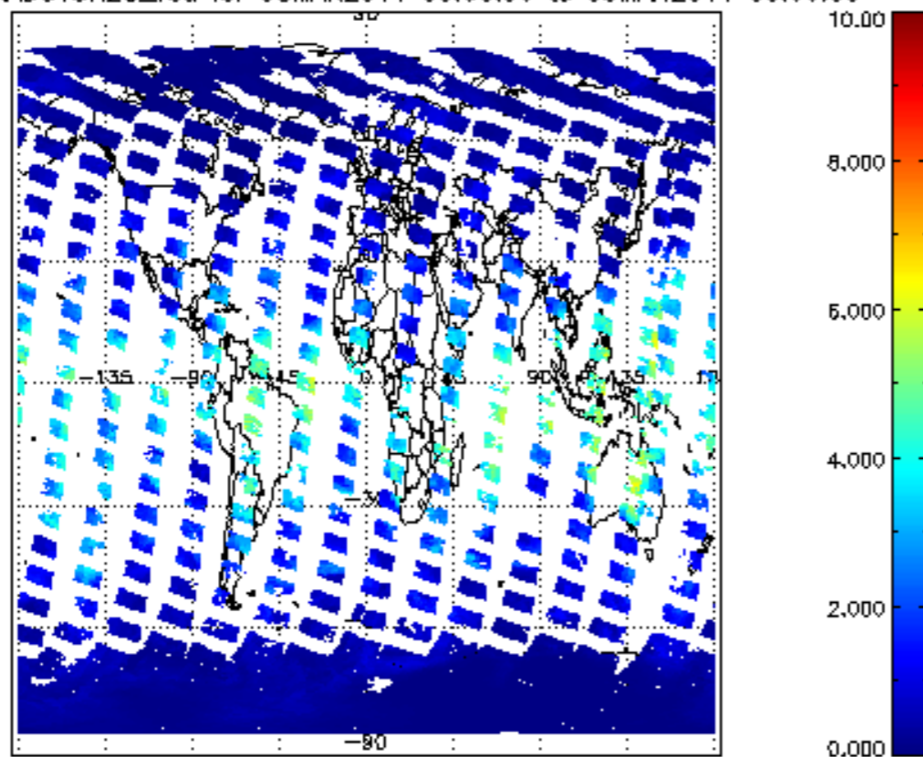
SCIOL2P_NADUV8H20_vcd for 08MAR2011 00:00:00 to 09MAR2011 00:00:00
