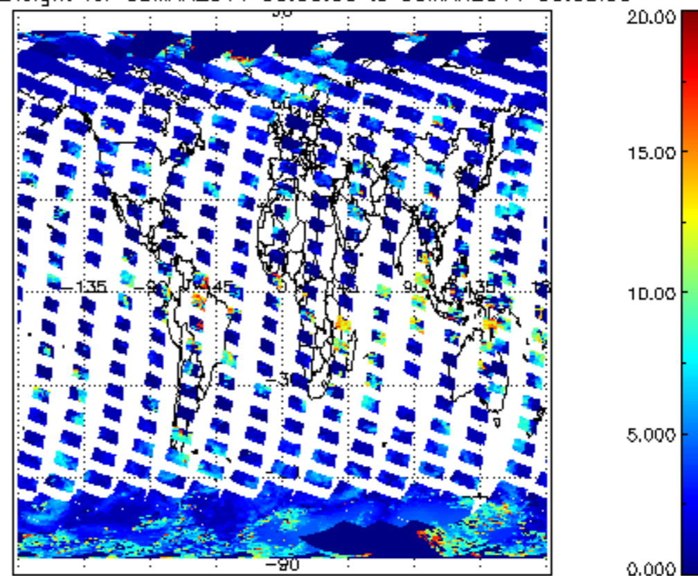
cL_top_height for 08MAR2011 00:00:00 to 09MAR2011 00:00:00
