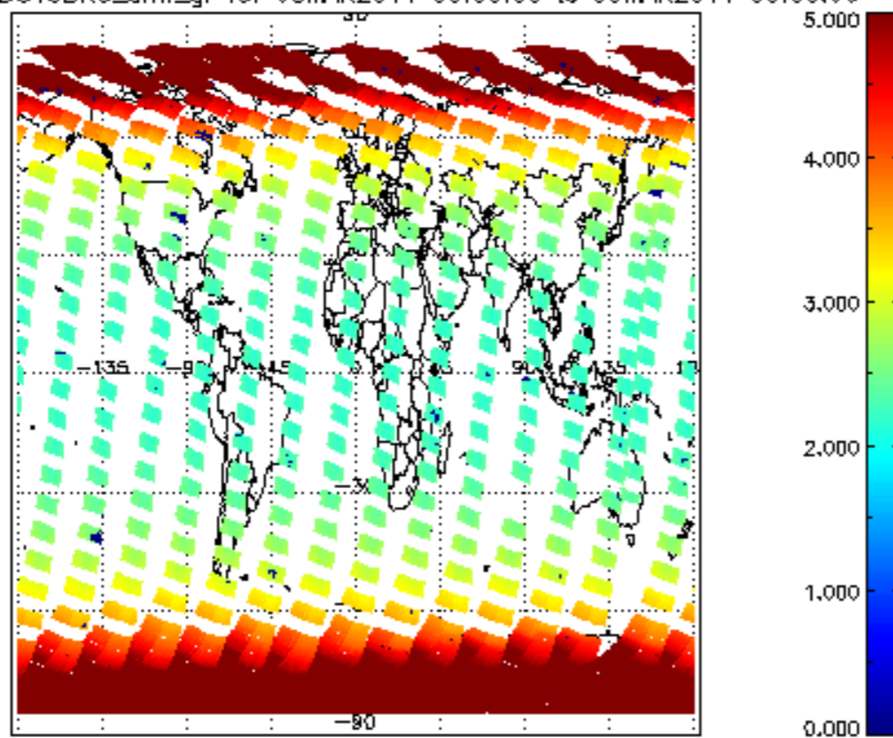
SCIOL2P_NADUV3BRO_amf_gr for 08MAR2011 00:00:00 to 09MAR2011 00:00:00
