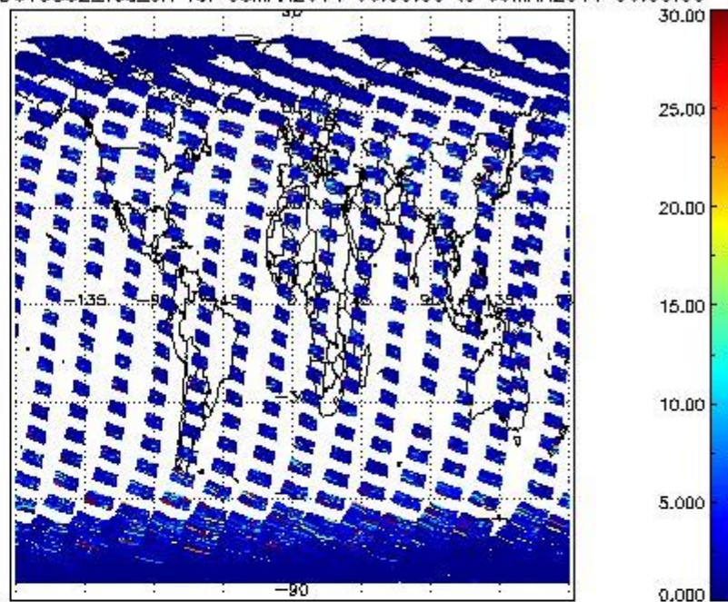
SCIOL2P_NADUV5S02_vcd_err for 08MAR2011 00:00:00 to 09MAR2011 00:00:00
