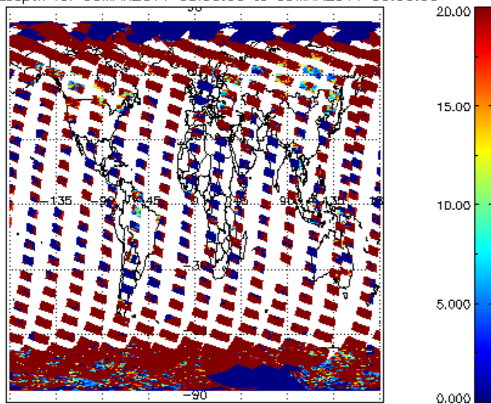
cL_opt_depth for 08MAR2011 00:00:00 to 09MAR2011 00:00:00
