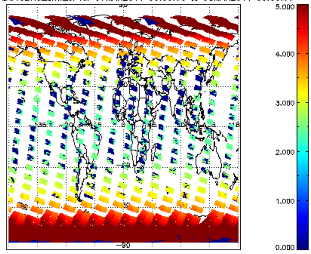
SCIOL2P_NADUV3BRO_arnf_cl for 07MAR2011 00:00:00 to 08MAR2011 00:00:00
