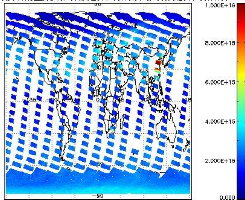
SCIOL2P_NADUV1NO2_vcd for 07MAR2011 00:00:00 to 06MAR2011 00:00:00
