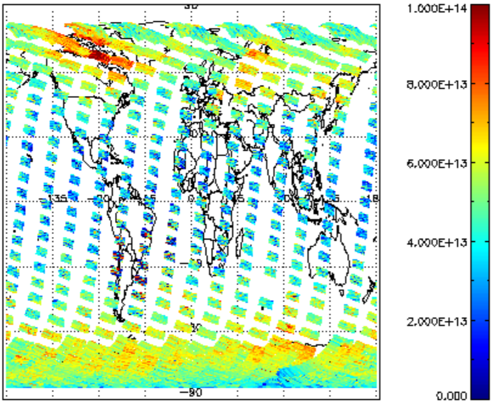
SCIOL2P_NADUV3BRO_vcd for 07MAR2011 00:00:00 to 08MAR2011 00:00:00
