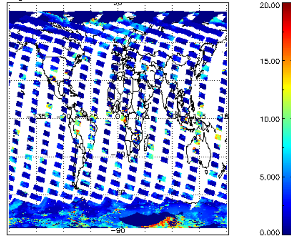
cL_top_height for 07MAR2011 00:00:00 to 08MAR2011 00:00:00
