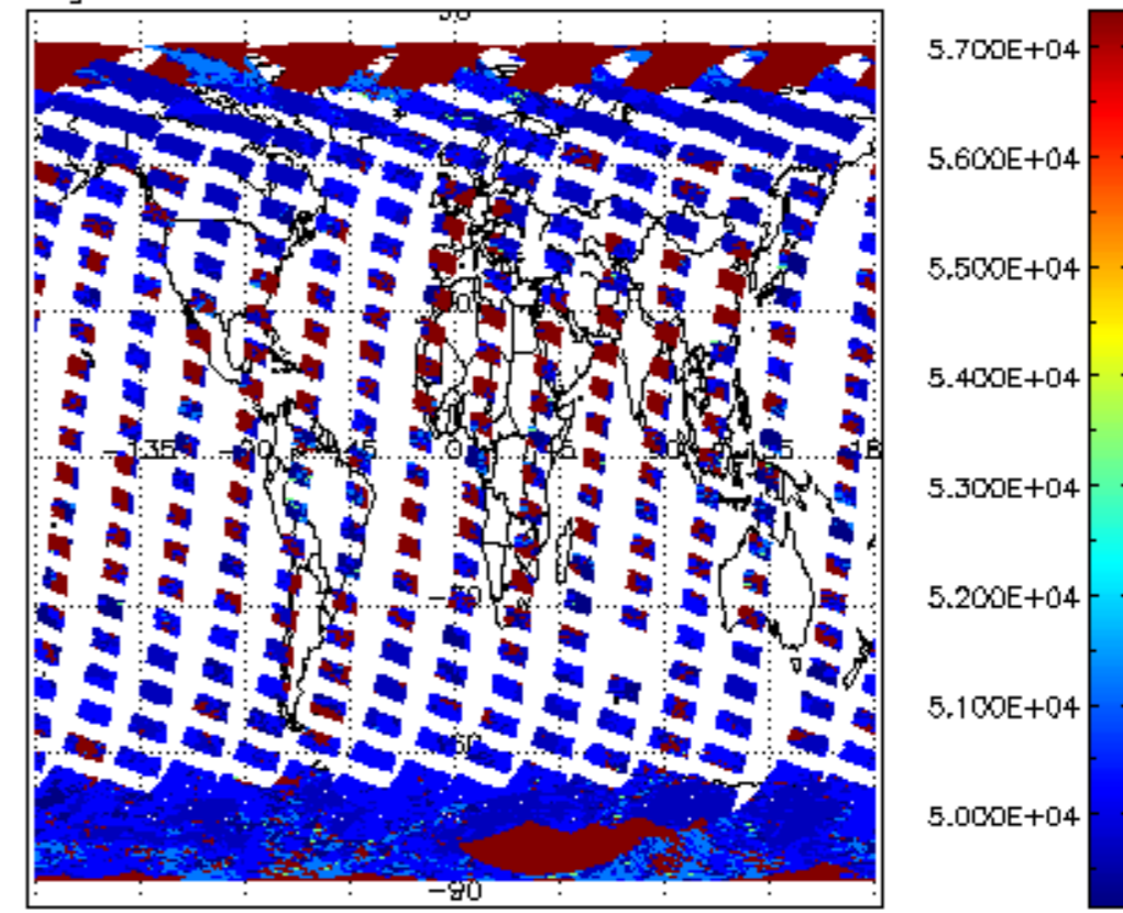
cloud_flags for 07MAR2011 00:00:00 to 08MAR2011 00:00:00
