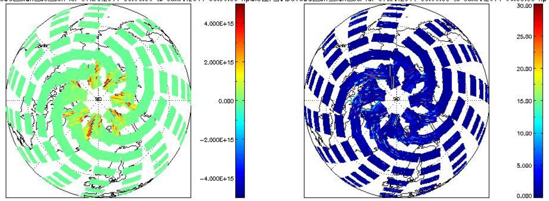
CIOL2P_NADUV6OCL_slant_col_den for 07MAR2011 00:00:00 to 08MAR2011 00:00:00 np CIOL2P_NADUV6OCL_err_slant_col for 07MAR2011 00:00:00 to 08MAR2011 00:00:00 np
