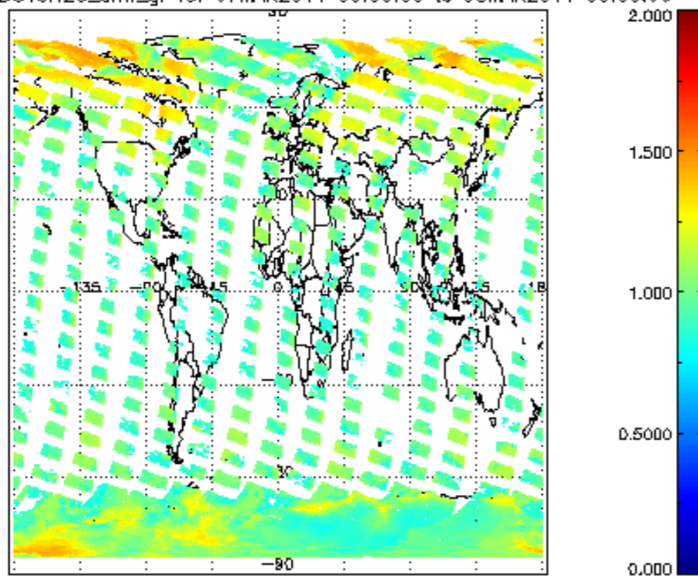
SCIOL2P_NADUV8H20_arnf_gr for 07MAR2011 00:00:00 to 08MAR2011 00:00:00
