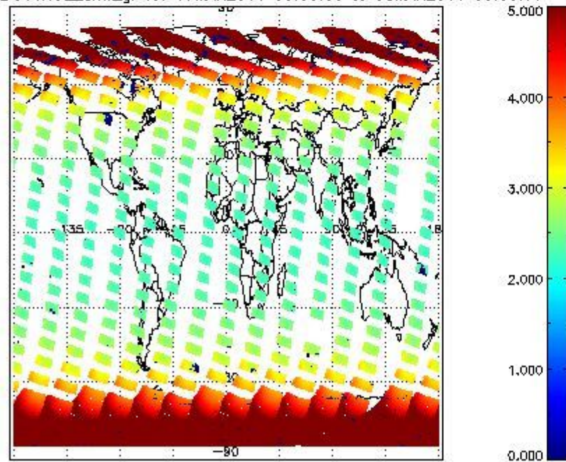
SCIOL2P_NADUV1NO2_amf_gr for 07MAR2011 00:00:00 to 08MAR2011 00:00:00
