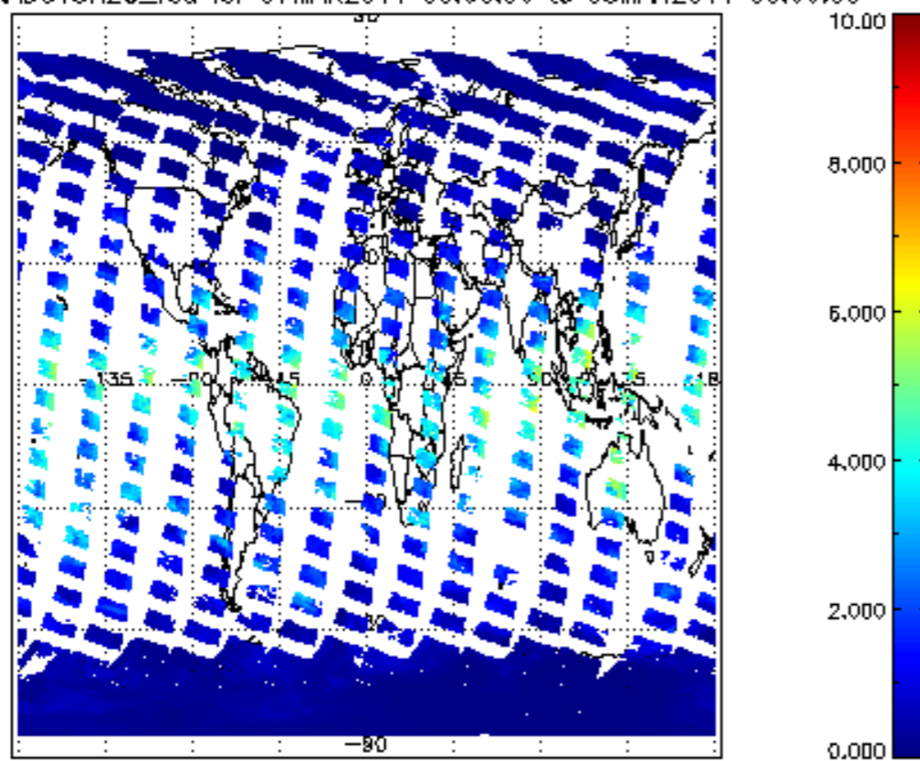
SCIOL2P_NADUV8H20_vcd for 07MAR2011 00:00:00 to 08MAR2011 00:00:00
