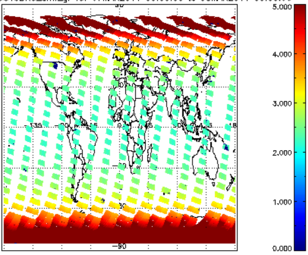
SCIOL2P_NADUV3BRO_arnf_gr for 07MAR2011 00:00:00 to 08MAR2011 00:00:00
