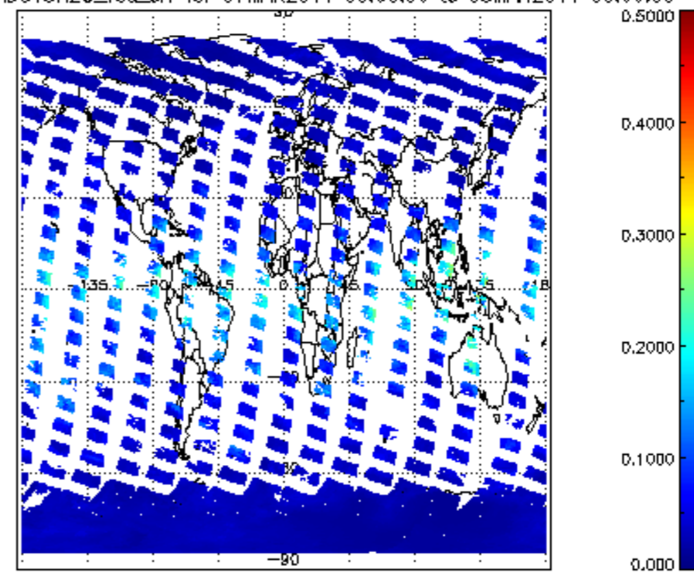
SCIOL2P_NADUV8H20_vcd_err for 07MAR2011 00:00:00 to 08MAR2011 00:00:00
