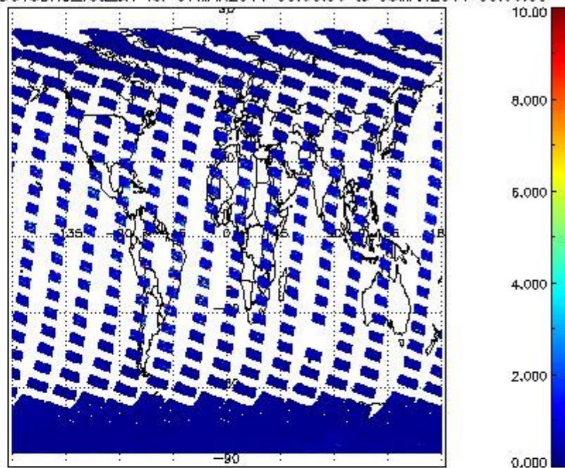
SCIOL2P_NADUV3BRO_vcd_err for 07MAR2011 00:00:00 to 06MAR2011 00:00:00
