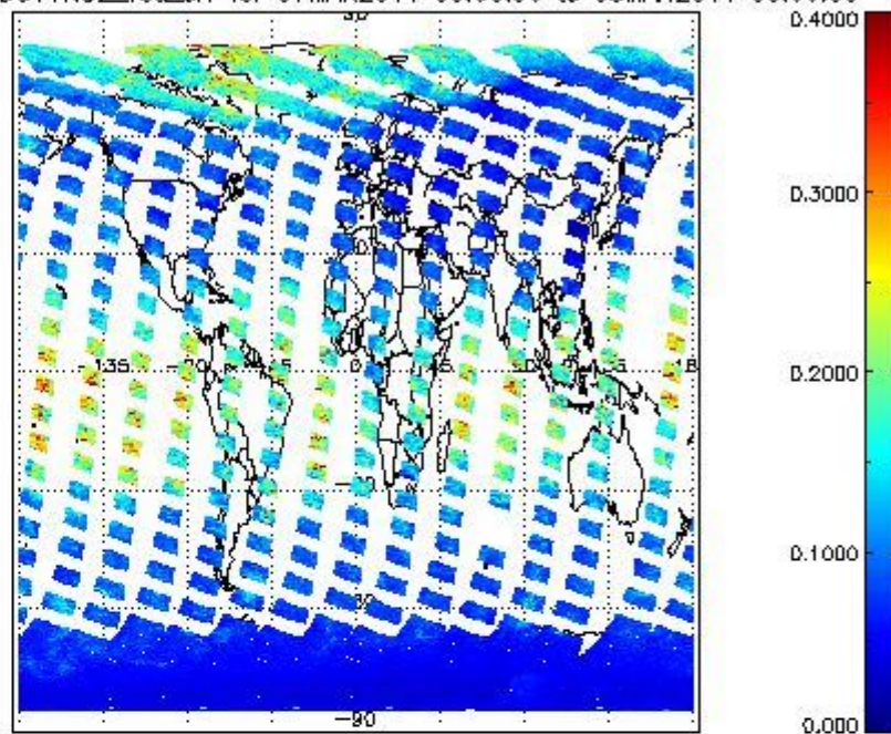
SCIOL2P_NADUV1NO2_vcd_err for 07MAR2011 00:00:00 to 06MAR2011 00:00:00
