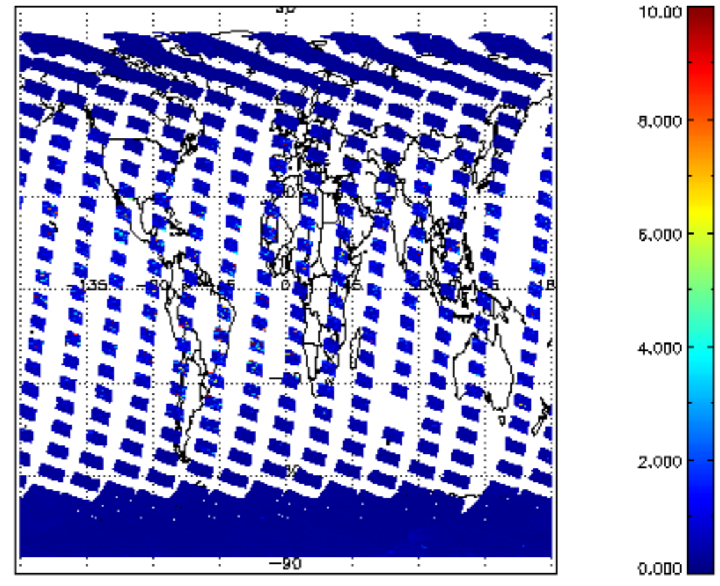
SCIOL2P_NADUV3BRO_vcd_Lerr for 07MAR2011 00:00:00 to 08MAR2011 00:00:00
