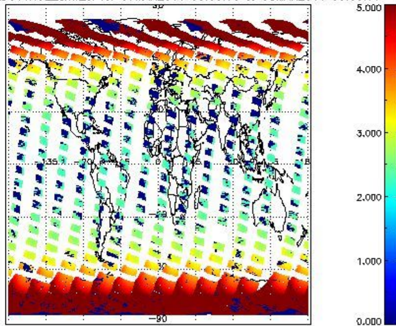
SCIOL2P_NADUV1NO2_amf_cl for 07MAR2011 00:00:00 to 08MAR2011 00:00:00
