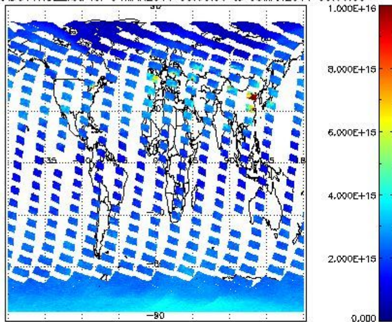
SCIOL2P_NADUV1NO2_vcd for 04MAR2011 00:00:00 to 05MAR2011 00:00:00
