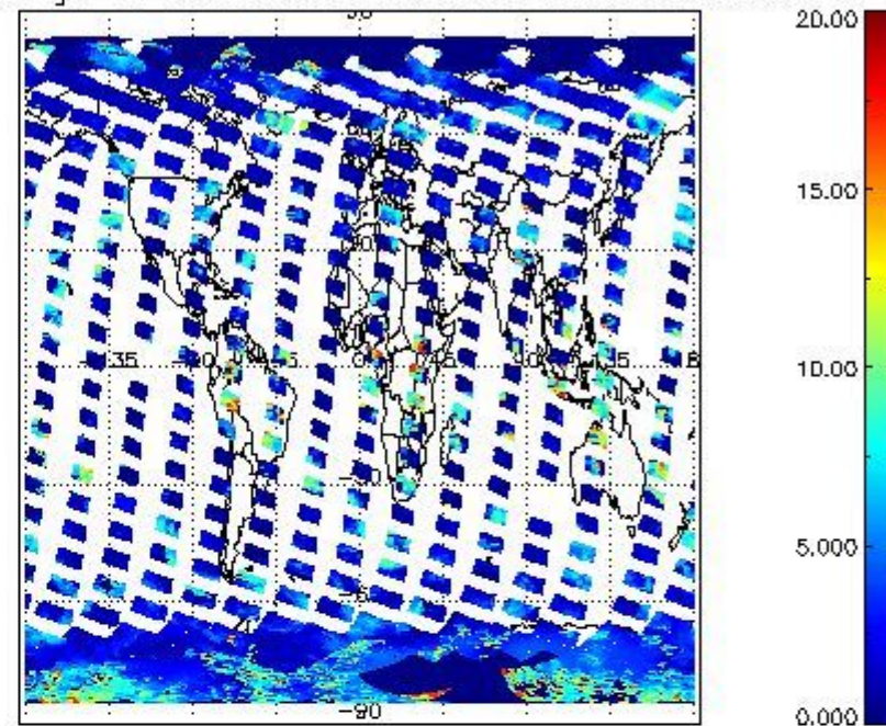
cL_top_height for 04MAR2011 00:00:00 to 05MAR2011 00:00:00
