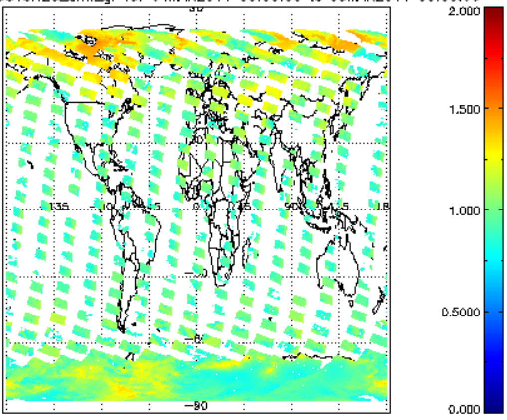
SCIOL2P_NADUV8H20_arnf_gr for 04MAR2011 00:00:00 to 05MAR2011 00:00:00
