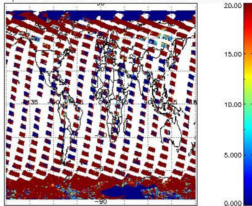
cL_opt_depth for 04MAR2011 00:00:00 to 05MAR2011 00:00:00
