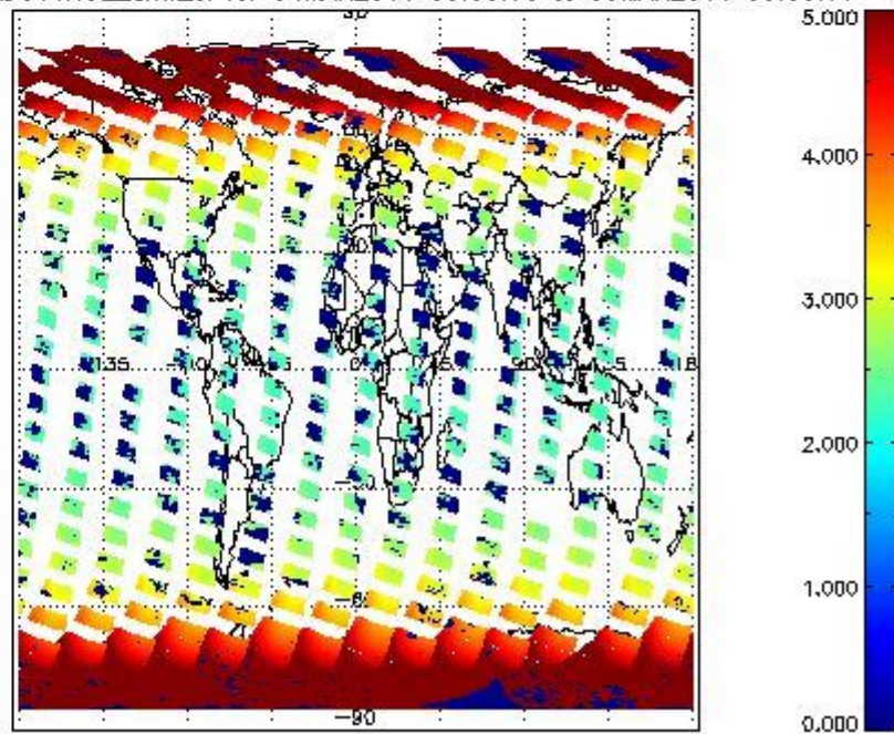
SCIOL2P_NADUV1NO2_amf_cl for 04MAR2011 00:00:00 to 05MAR2011 00:00:00
