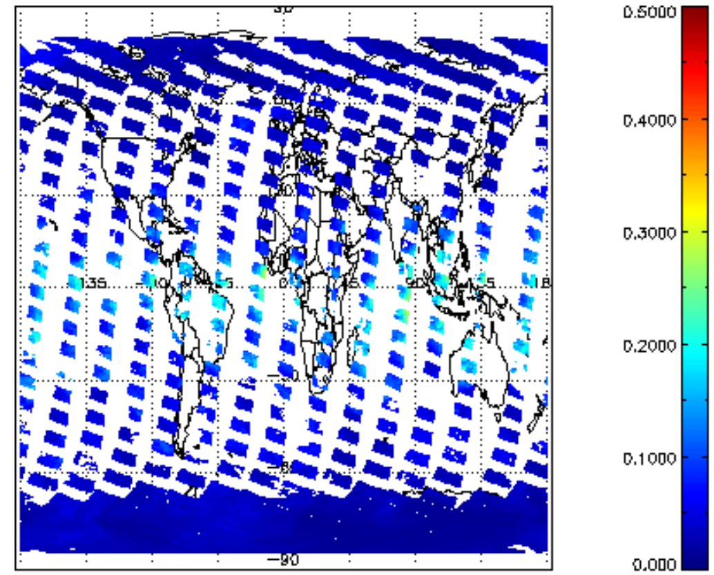
SCIOL2P_NADUV8H20_vcd_Lerr for 04MAR2011 00:00:00 to 05MAR2011 00:00:00
