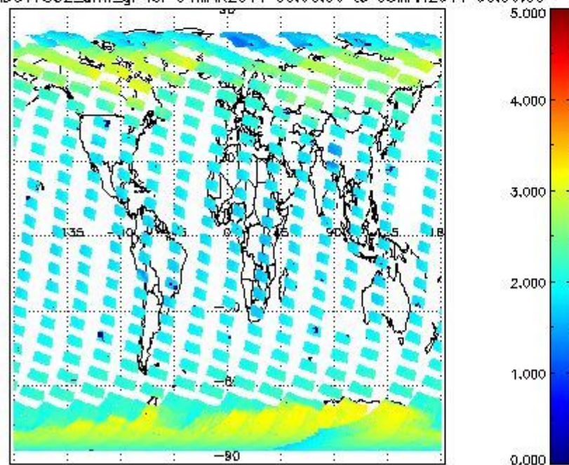
SCIOL2P_NADUV7S02_amf_gr for 04MAR2011 00:00:00 to 05MAR2011 00:00:00
