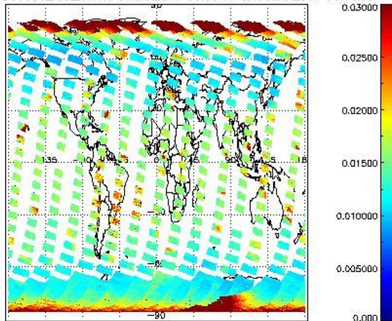
SCIOL2P_NADUV003_vcd_err for 04MAR2011 00:00:00 to 05MAR2011 00:00:00
