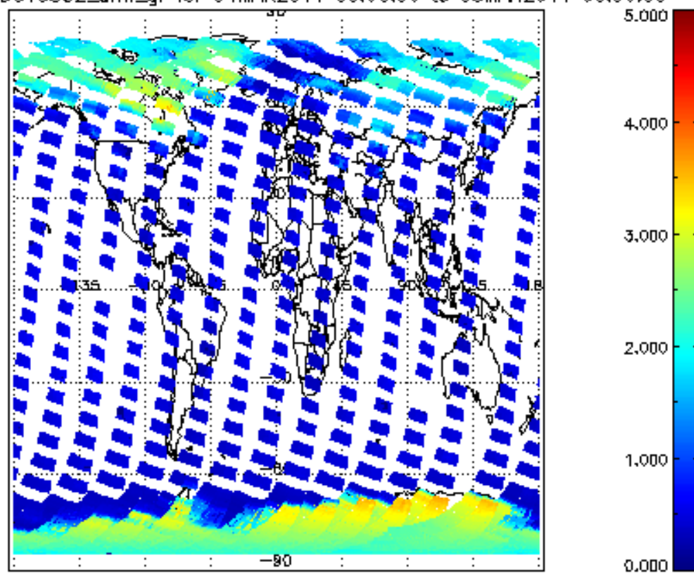
SCIOL2P_NADUV5S02_amf_gr for 04MAR2011 00:00:00 to 05MAR2011 00:00:00
