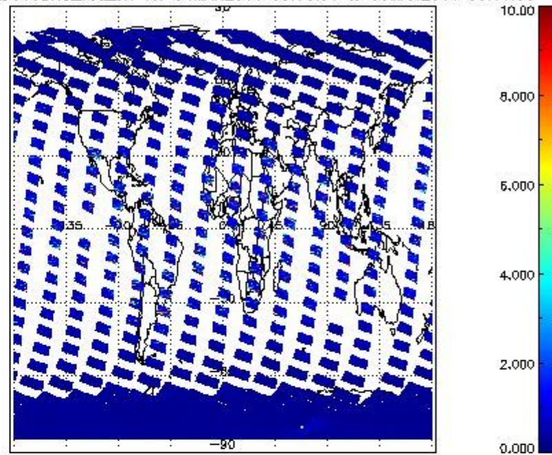
SCIOL2P_NADUV3BRO_vcd_err for 04MAR2011 00:00:00 to 05MAR2011 00:00:00
