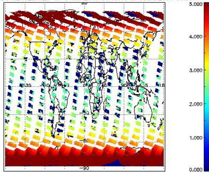
SCIOL2P_NADUV3BRO_amf_cl for 04MAR2011 00:00:00 to 05MAR2011 00:00:00
