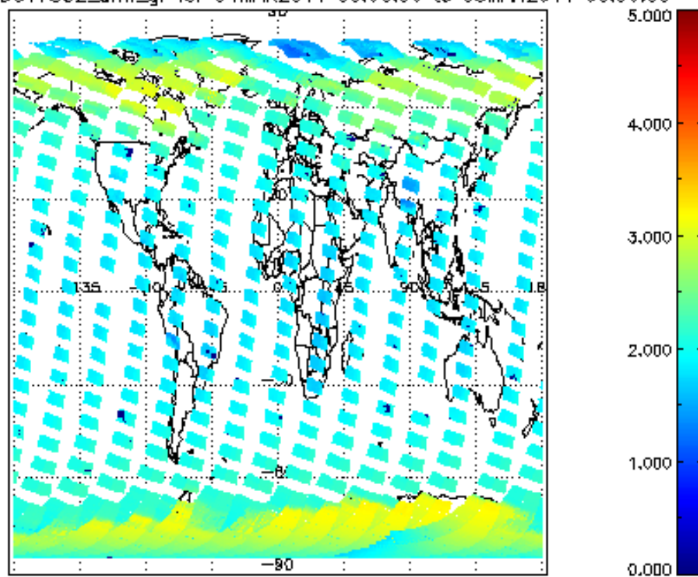
SCIOL2P_NADUV7S02_amf_gr for 04MAR2011 00:00:00 to 05MAR2011 00:00:00
