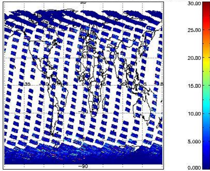
SCIOL2P_NADUV5SO2_vcd_err for 04MAR2011 00:00:00 to 05MAR2011 00:00:00
