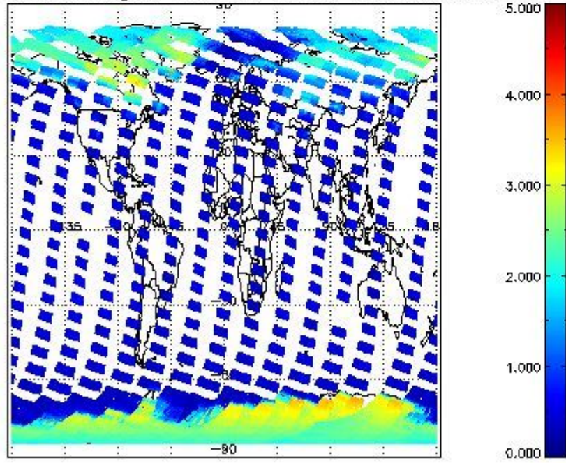
SCIOL2P_NADUV5SO2_amf_gr for 04MAR2011 00:00:00 to 05MAR2011 00:00:00
