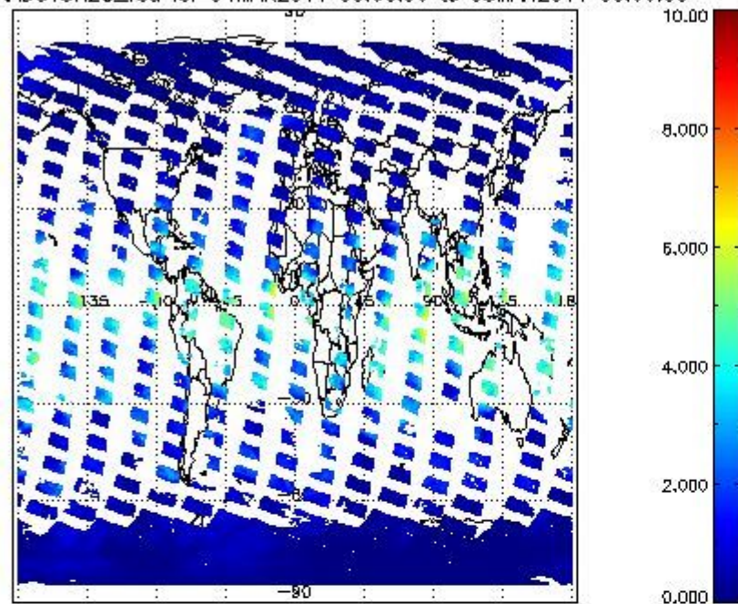
SCIOL2P_NADUV8H2O_vcd for 04MAR2011 00:00:00 to 05MAR2011 00:00:00
