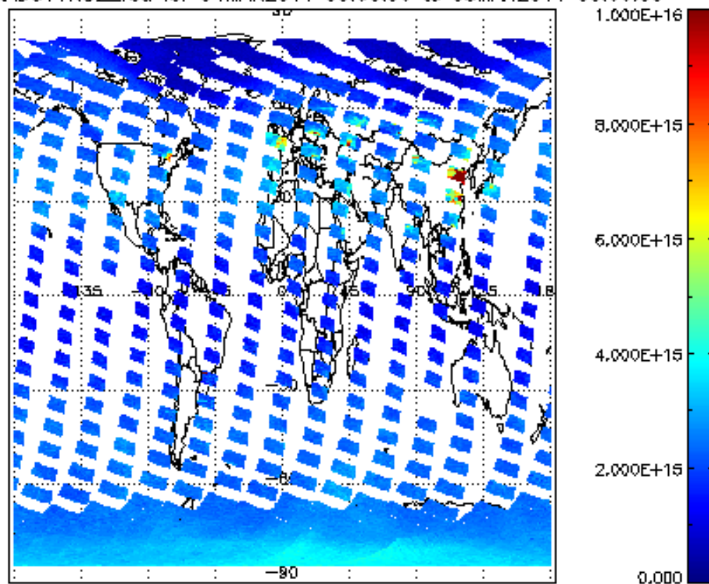
SCIOL2P_NADUV1NO2_vcd for 04MAR2011 00:00:00 to 05MAR2011 00:00:00
