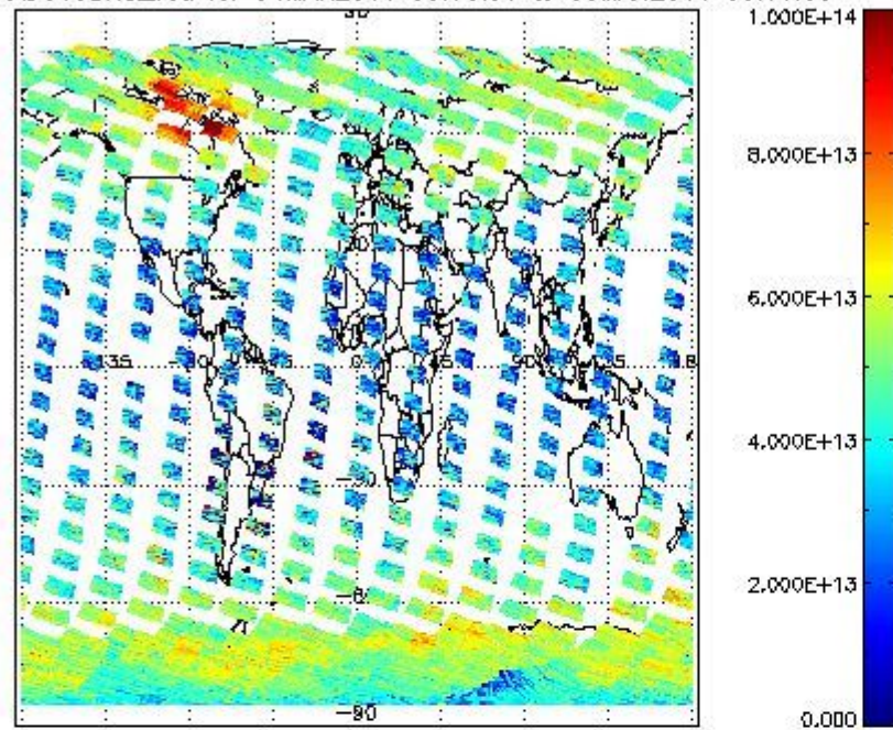
SCIOL2P_NADUV3BRO_vcd for 04MAR2011 00:00:00 to 05MAR2011 00:00:00
