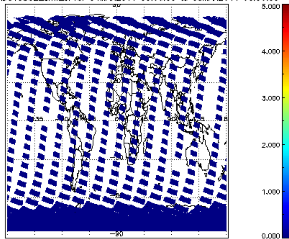
SCIOL2P_NADUV5S02_amf_cl for 04MAR2011 00:00:00 to 05MAR2011 00:00:00
