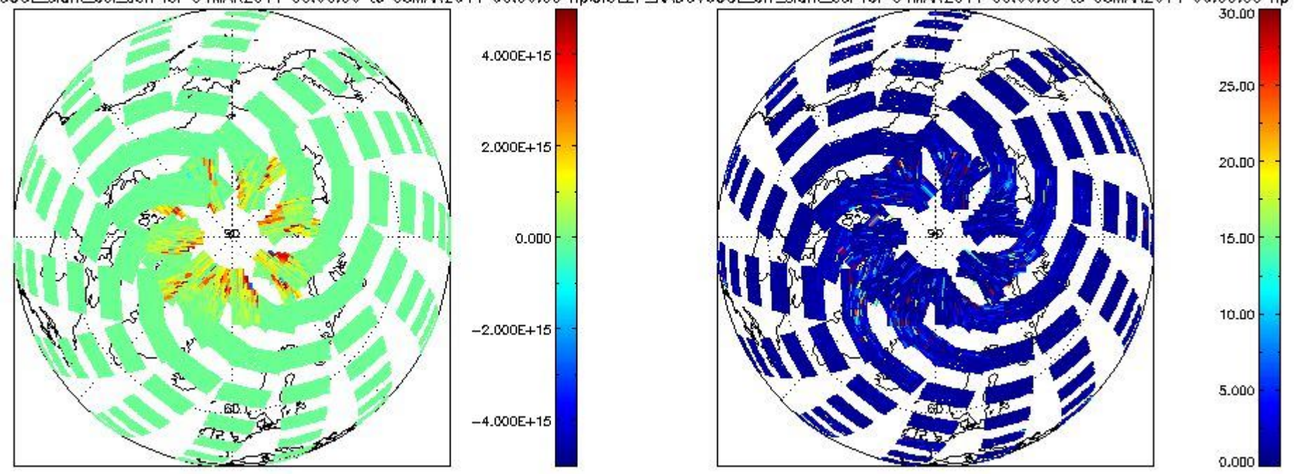
CIOL2P_NADUV6OCL_slant_col_den for 04MAR2011 00:00:00 to 05MAR2011 00:00:00 np CIOL2P_NADUV6OCL_err_slant_col for 04MAR2011 00:00:00 to 05MAR2011 00:00:00 np
