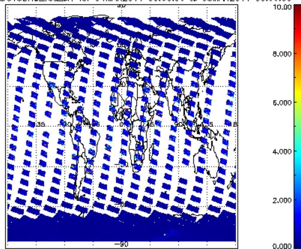
SCIOL2P_NADUV3BRO_vcd_err for 04MAR2011 00:00:00 to 05MAR2011 00:00:00
