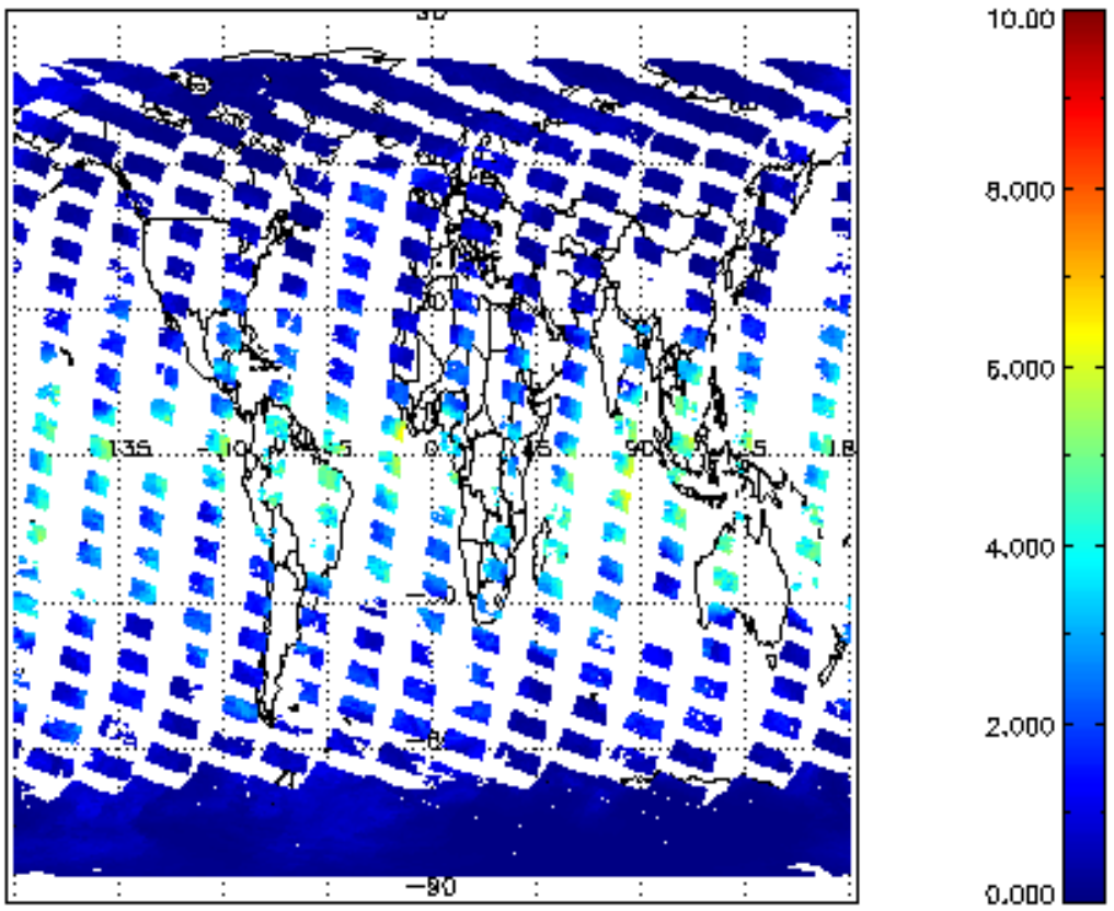
SCIOL2P_NADUV8H20_vcd for 04MAR2011 00:00:00 to 05MAR2011 00:00:00
