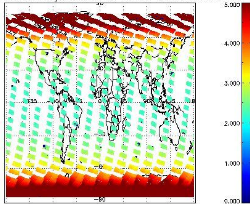
SCIOL2P_NADUV3BRO_amf_gr for 04MAR2011 00:00:00 to 05MAR2011 00:00:00
