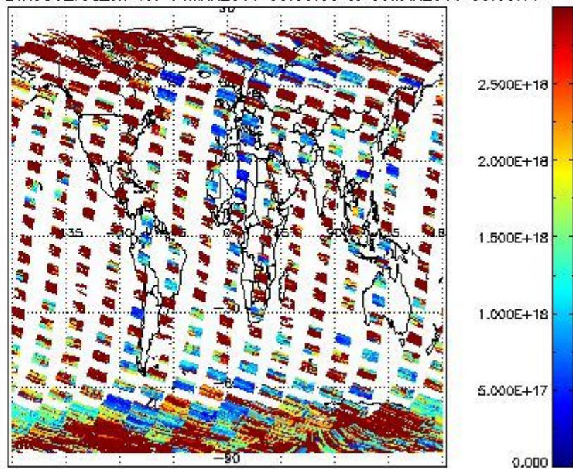
SCIDL2P_NADIR3CO_vcd_err for 04MAR2011 00:00:00 to 05MAR2011 00:00:00
