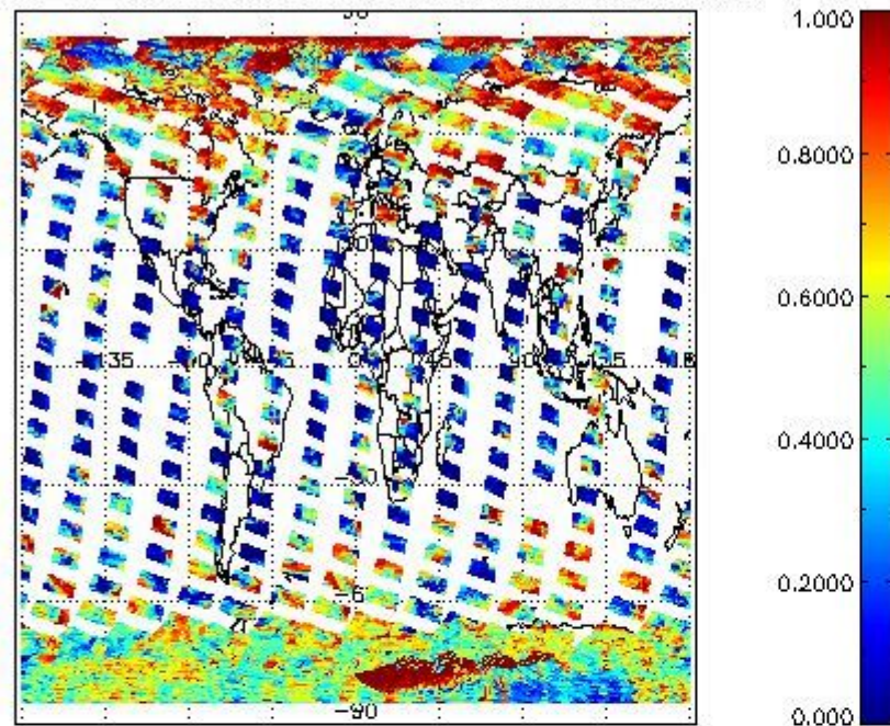
cL_frac for 04MAR2011 00:00:00 to 05MAR2011 00:00:00
