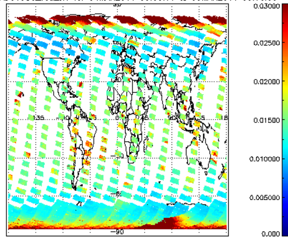
SCIOL2P_NADUV003_vcd_err for 04MAR2011 00:00:00 to 05MAR2011 00:00:00
