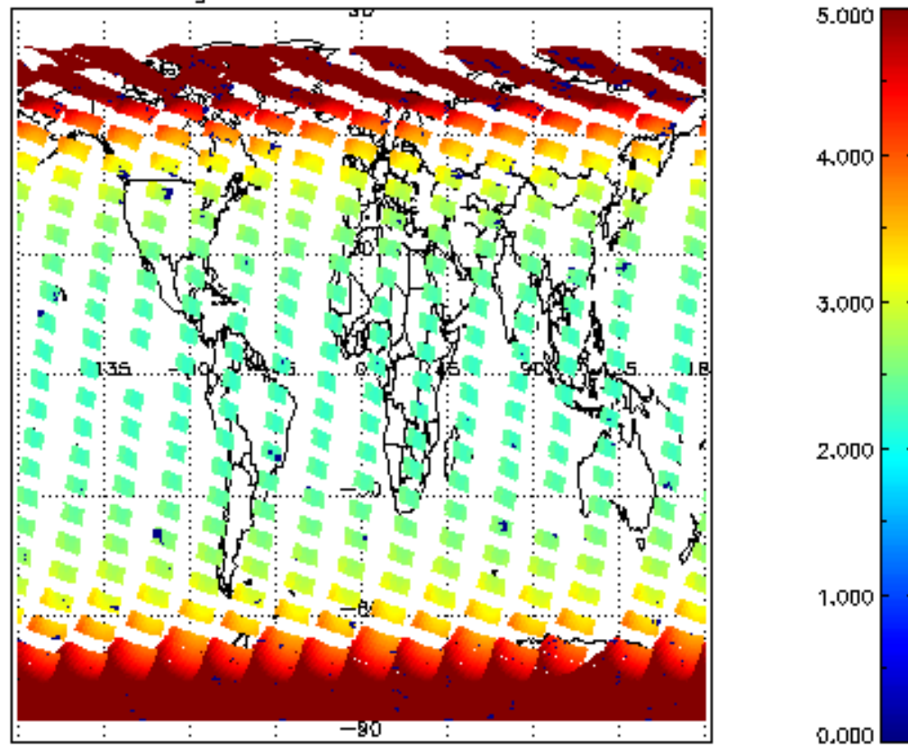
SCIOL2P_NADUV1NO2_amf_gr for 04MAR2011 00:00:00 to 05MAR2011 00:00:00
