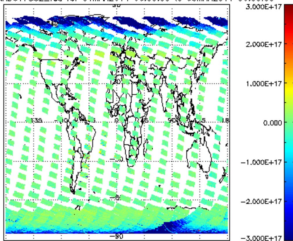
SCIOL2P_NADUV7S02_vcd for 04MAR2011 00:00:00 to 05MAR2011 00:00:00
