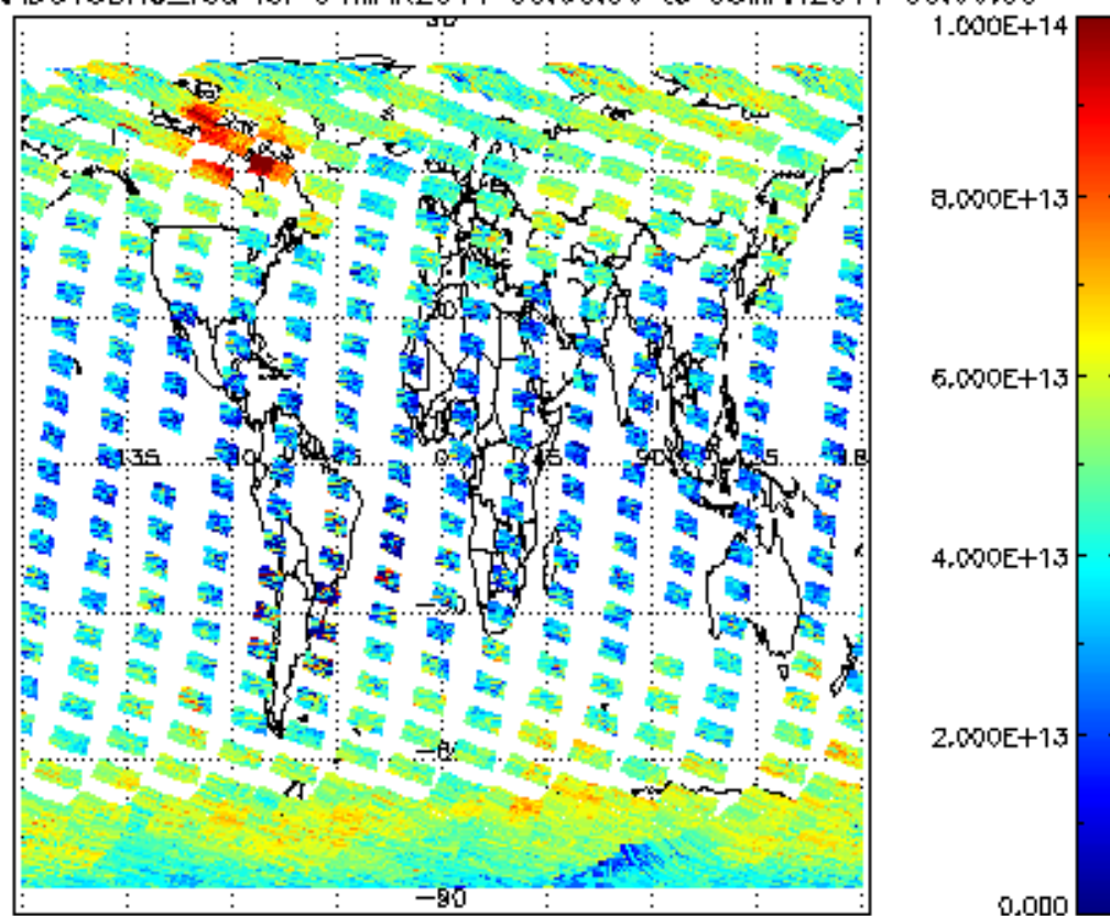
SCIOL2P_NADUV3BRO_vcd for 04MAR2011 00:00:00 to 05MAR2011 00:00:00
