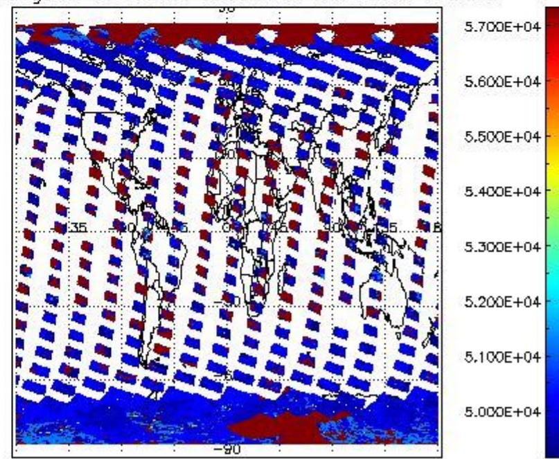
cloud_flags for 04MAR2011 00:00:00 to 05MAR2011 00:00:00
