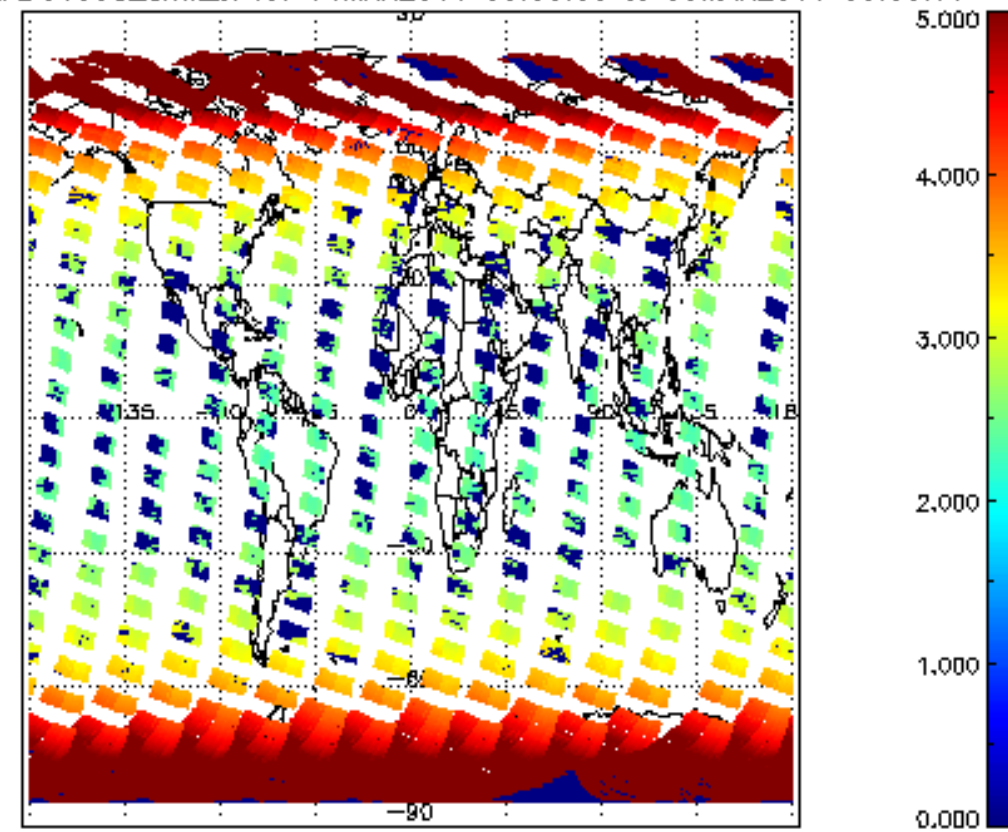
SCIOL2P_NADUV003_amf_cl for 04MAR2011 00:00:00 to 05MAR2011 00:00:00
