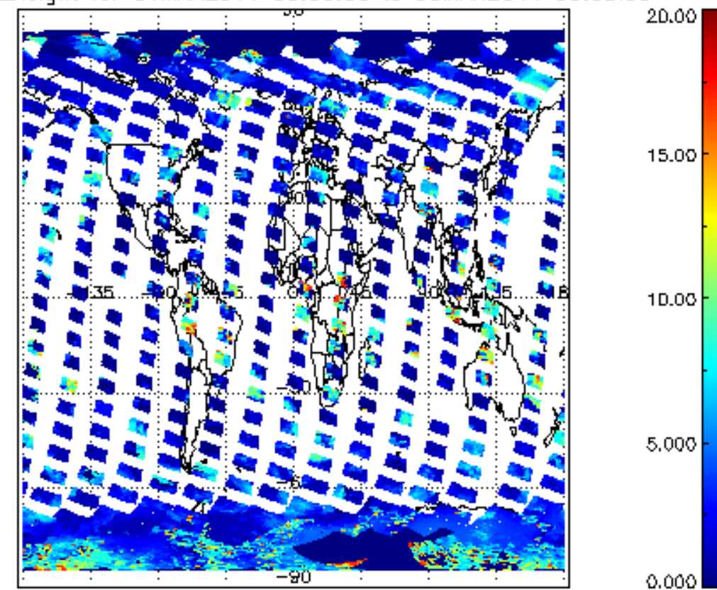
cL_top_height for 04MAR2011 00:00:00 to 05MAR2011 00:00:00
