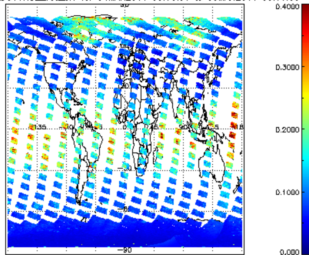
SCIOL2P_NADUV1NO2_vcd_err for 04MAR2011 00:00:00 to 05MAR2011 00:00:00
