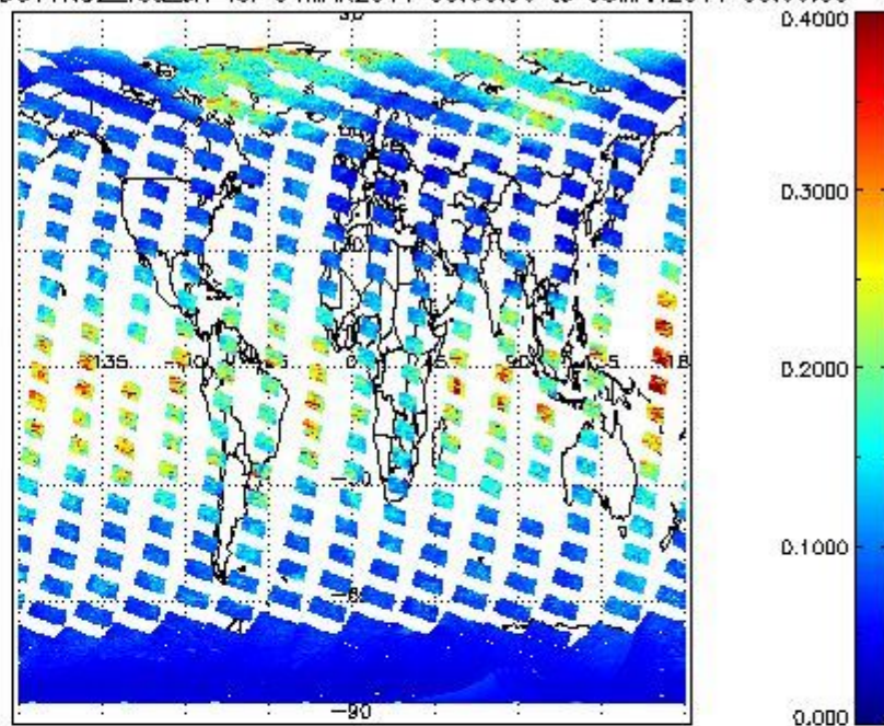
SCIOL2P_NADUV1NO2_vcd_err for 04MAR2011 00:00:00 to 05MAR2011 00:00:00
