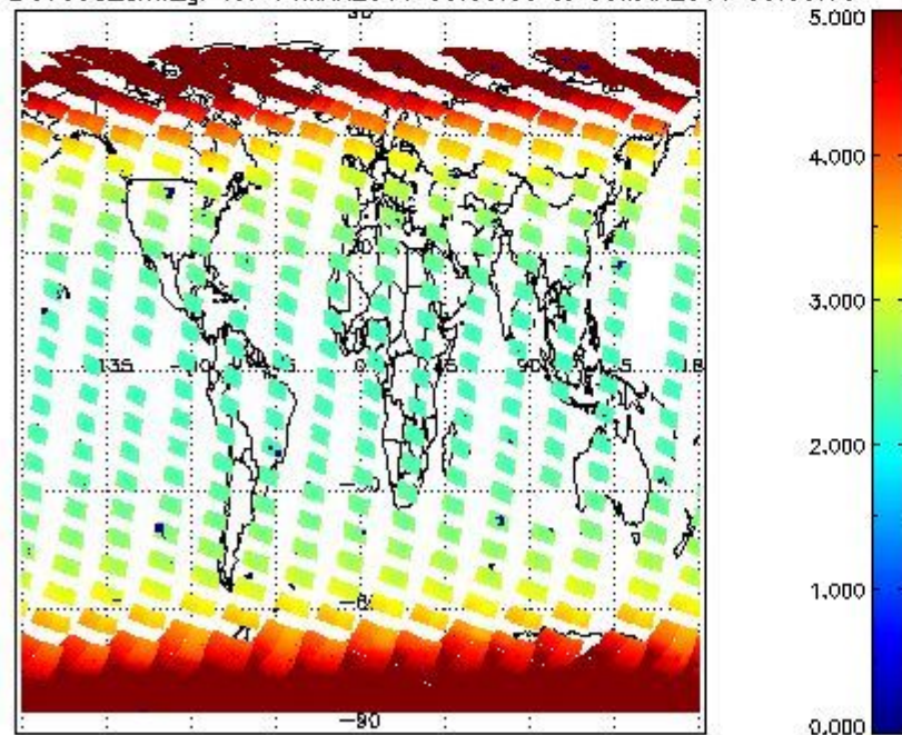
SCIOL2P_NADUV003_amf_gr for 04MAR2011 00:00:00 to 05MAR2011 00:00:00
