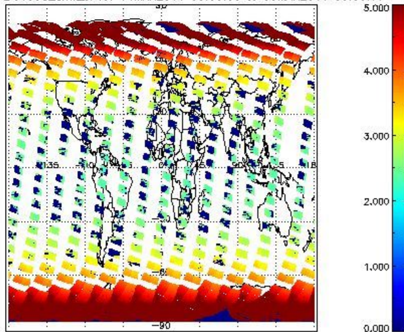
SCIOL2P_NADUV003_amf_cl for 04MAR2011 00:00:00 to 05MAR2011 00:00:00
