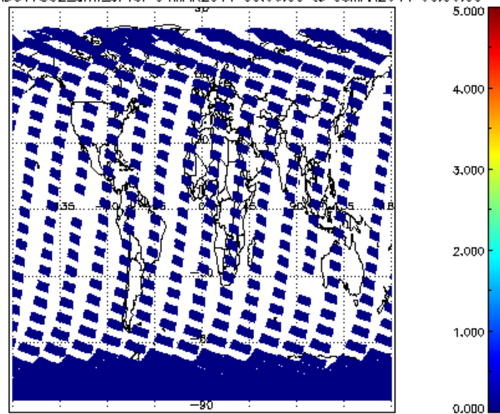
SCIOL2P_NADUV7S02_amf_cl for 04MAR2011 00:00:00 to 05MAR2011 00:00:00
