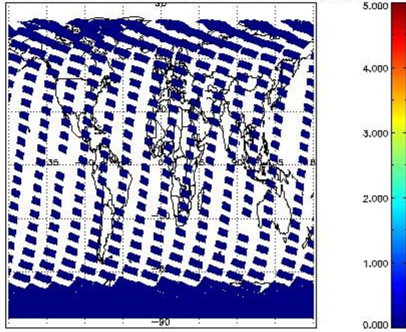
SCIOL2P_NADUV5SO2_amf_cl for 04MAR2011 00:00:00 to 05MAR2011 00:00:00
