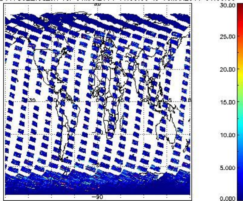
SCIOL2P_NADUV7S02_vcd_err for 04MAR2011 00:00:00 to 05MAR2011 00:00:00
