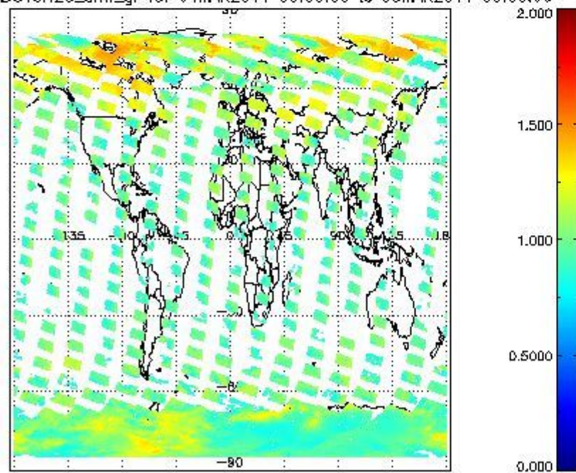
SCIOL2P_NADUV8H2O_arnf_gr for 04MAR2011 00:00:00 to 05MAR2011 00:00:00
