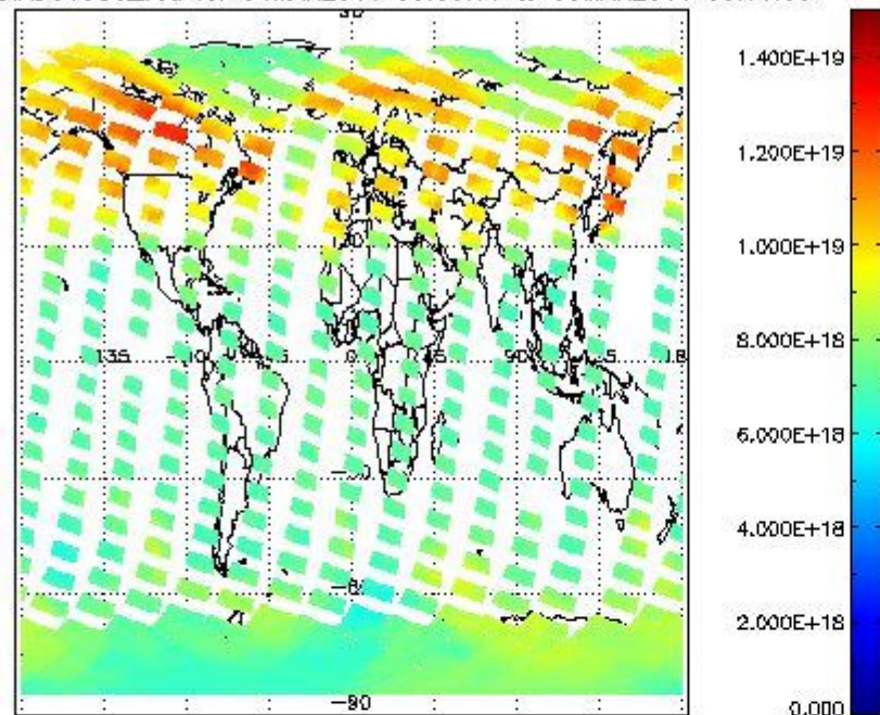
SCIOL2P_NADUV003_vcd for 04MAR2011 00:00:00 to 05MAR2011 00:00:00
