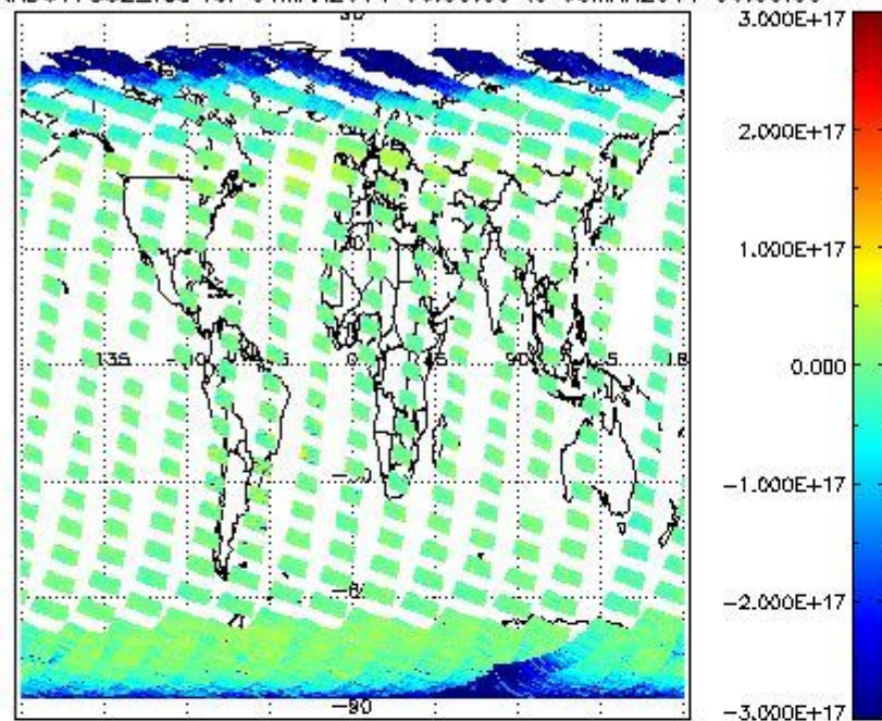
SCIOL2P_NADUV7S02_vcd for 04MAR2011 00:00:00 to 05MAR2011 00:00:00
