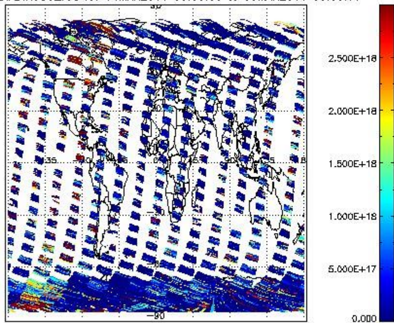
SCIDL2P_NADIR3CO_vcd for 04MAR2011 00:00:00 to 05MAR2011 00:00:00
