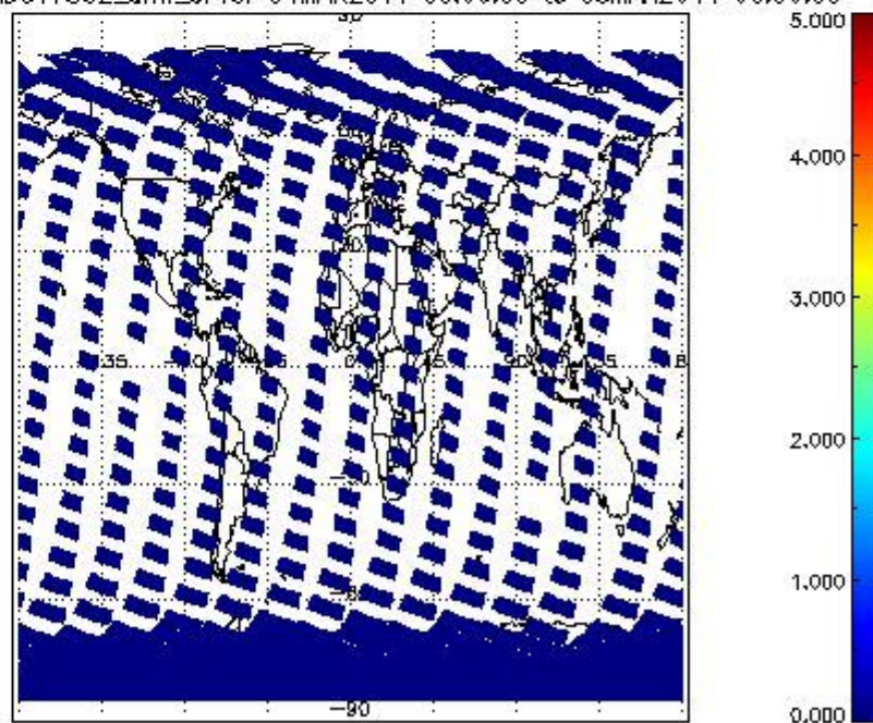
SCIOL2P_NADUV7S02_amf_cl for 04MAR2011 00:00:00 to 05MAR2011 00:00:00
