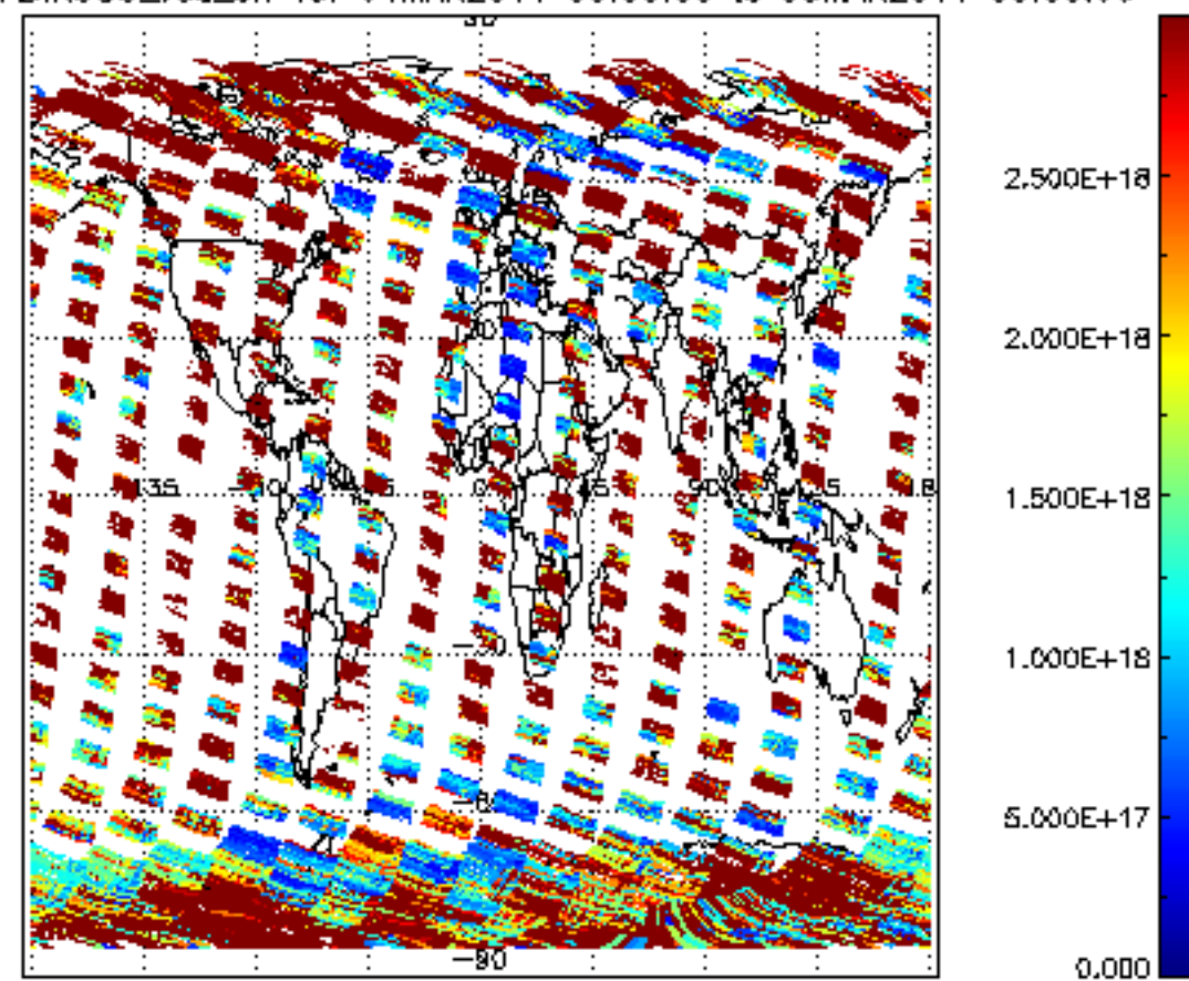
SCIOL2P_NADIR3CO_vcd_err for 04MAR2011 00:00:00 to 05MAR2011 00:00:00
