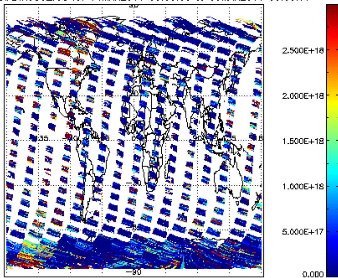
SCIOL2P_NADIR3CO_vcd for 04MAR2011 00:00:00 to 05MAR2011 00:00:00
