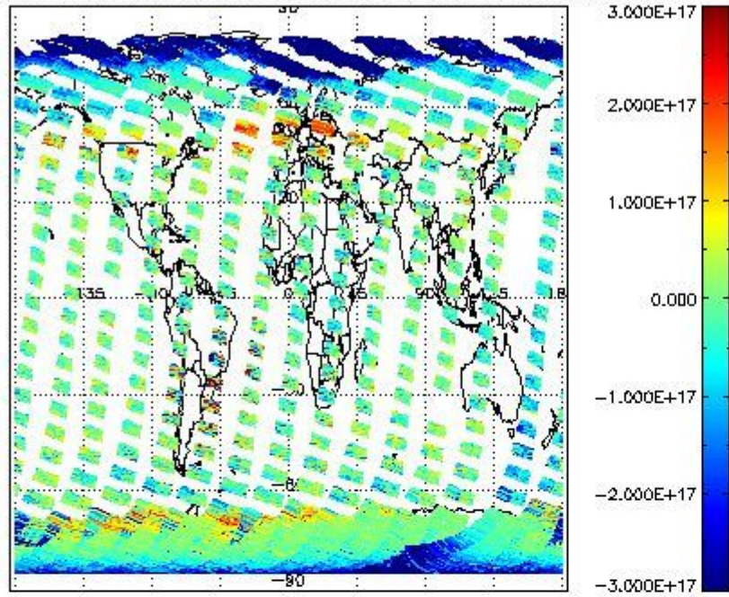
SCIOL2P_NADUV5SO2_vcd for 04MAR2011 00:00:00 to 05MAR2011 00:00:00
