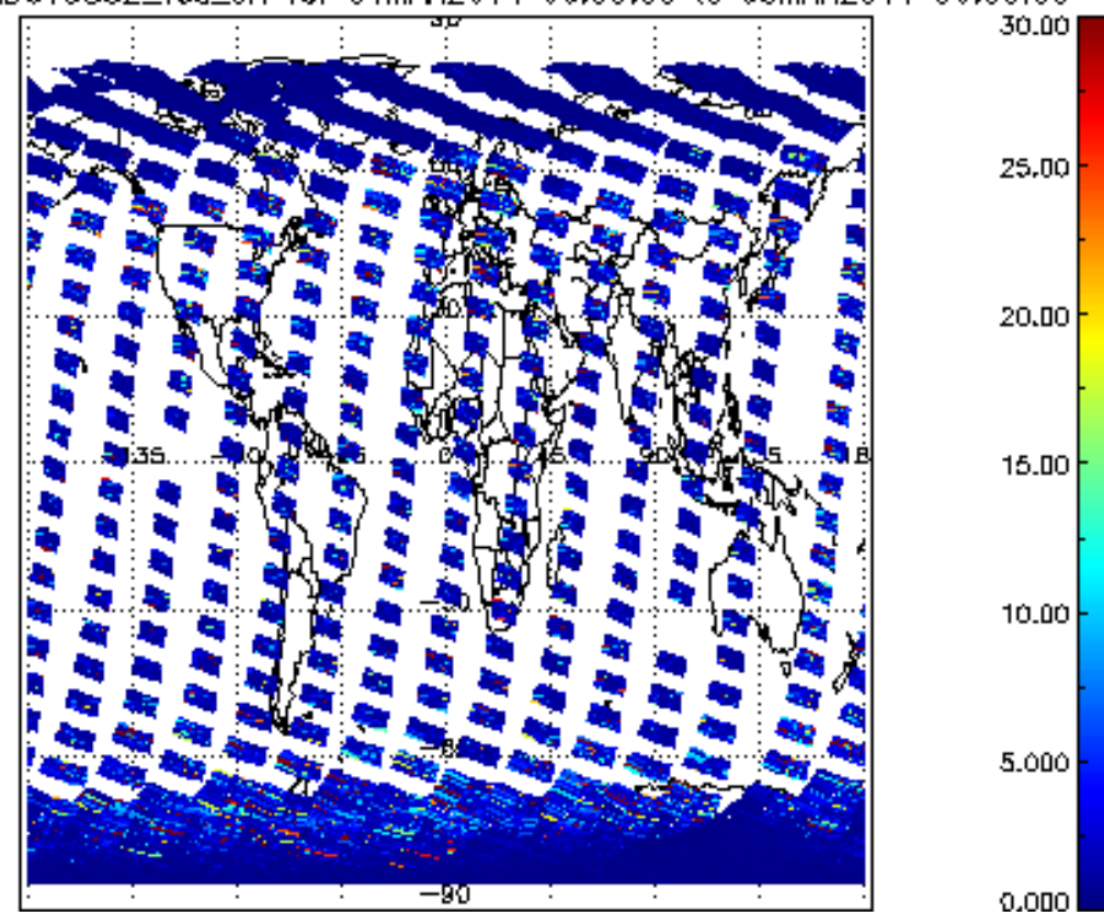
SCIOL2P_NADUV5S02_vcd_err for 04MAR2011 00:00:00 to 05MAR2011 00:00:00
