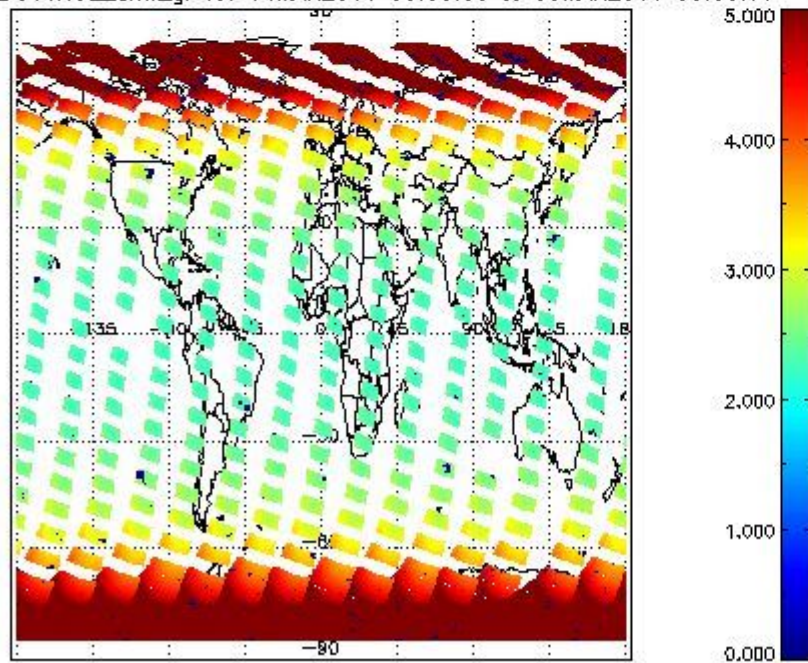
SCIOL2P_NADUV1NO2_amf_gr for 04MAR2011 00:00:00 to 05MAR2011 00:00:00
