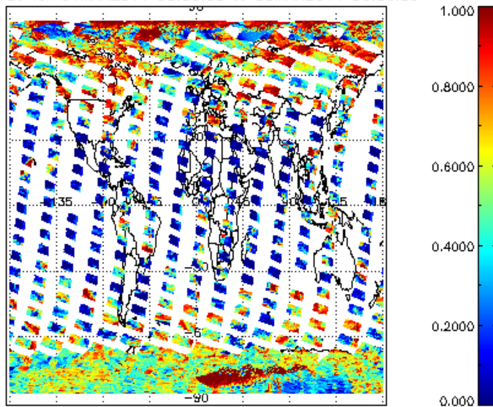
cL_frac for 04MAR2011 00:00:00 to 05MAR2011 00:00:00
