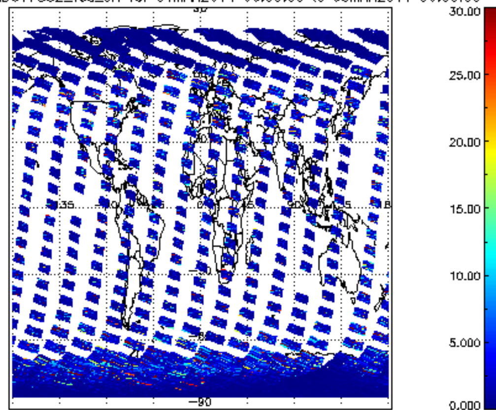
SCIOL2P_NADUV7S02_vcd_err for 04MAR2011 00:00:00 to 05MAR2011 00:00:00
