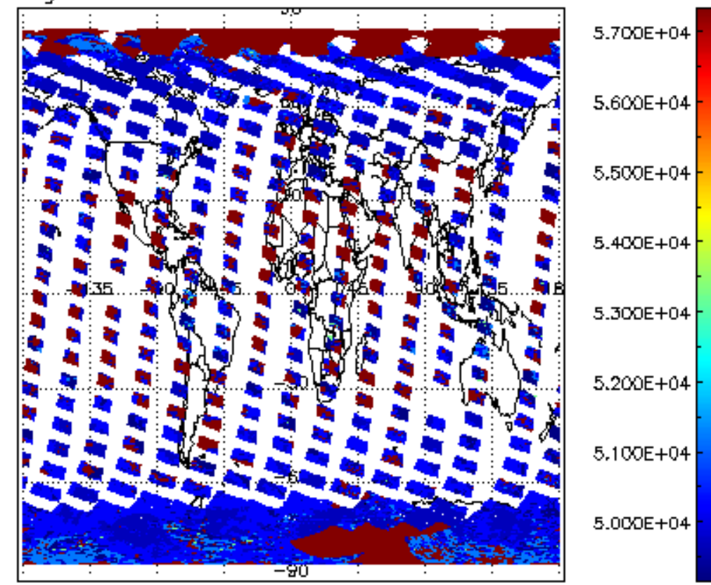
cloud_flags for 04MAR2011 00:00:00 to 05MAR2011 00:00:00
