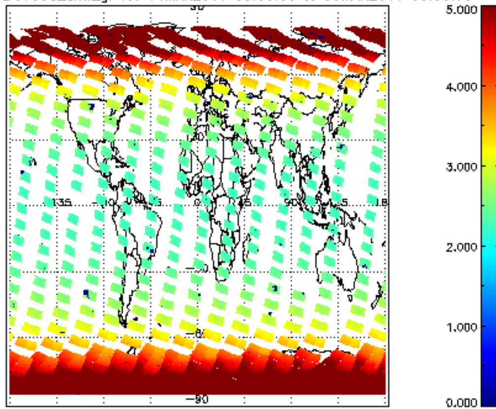
SCIOL2P_NADUV003_amf_gr for 04MAR2011 00:00:00 to 05MAR2011 00:00:00
