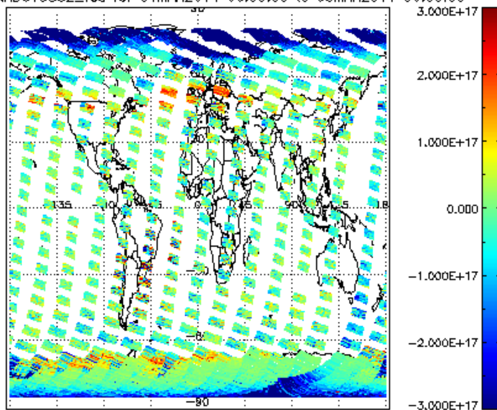
SCIOL2P_NADUV5S02_vcd for 04MAR2011 00:00:00 to 05MAR2011 00:00:00
