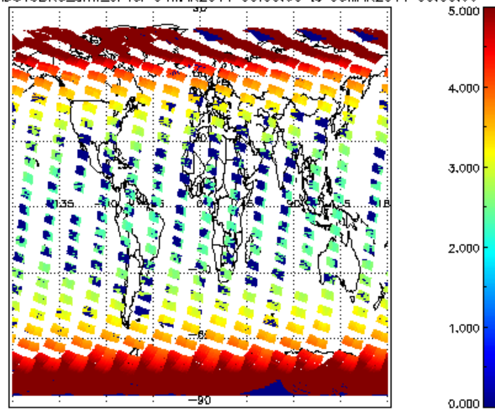
SCIOL2P_NADUV3BRO_amf_cl for 04MAR2011 00:00:00 to 05MAR2011 00:00:00
