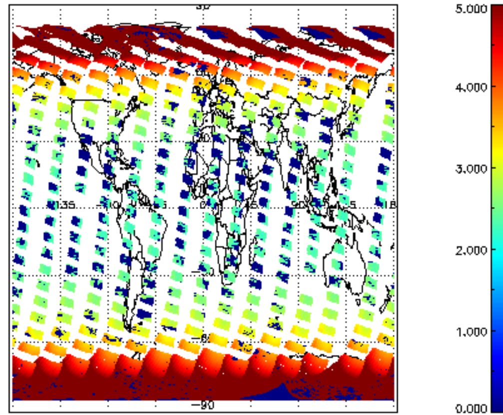
SCIOL2P_NADUV1NO2_amf_cl for 04MAR2011 00:00:00 to 05MAR2011 00:00:00
