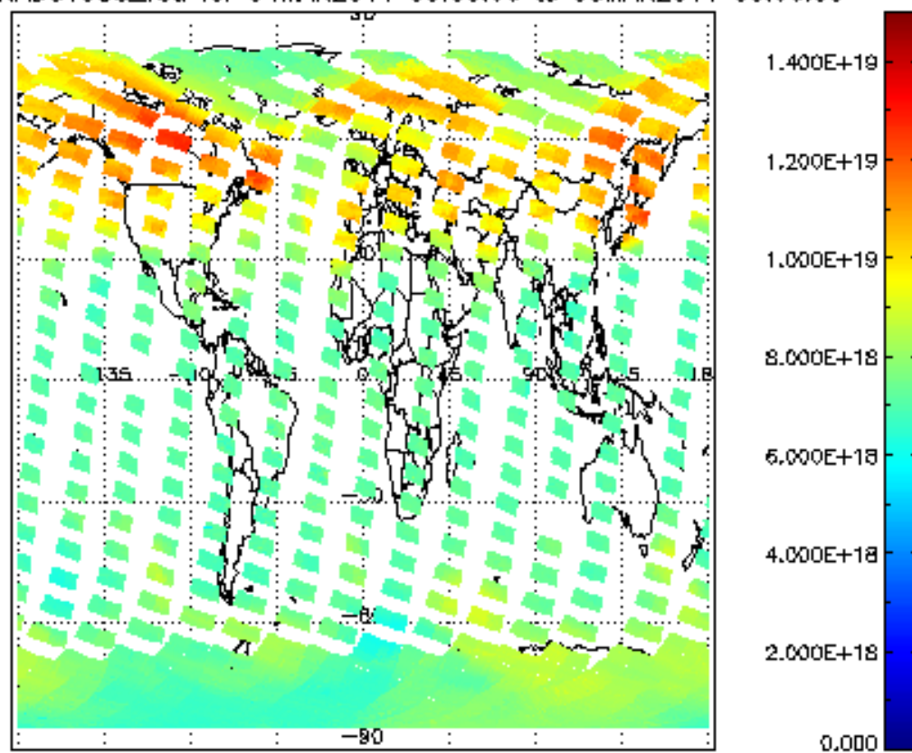
SCIOL2P_NADUV003_vcd for 04MAR2011 00:00:00 to 05MAR2011 00:00:00
