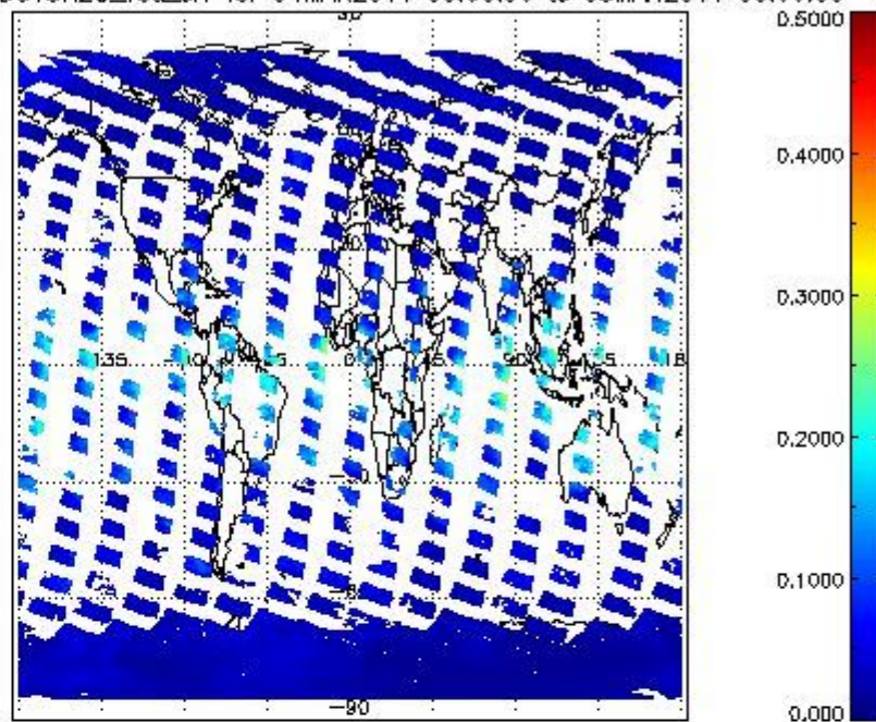
SCIOL2P_NADUV8H2O_vcd_err for 04MAR2011 00:00:00 to 05MAR2011 00:00:00
