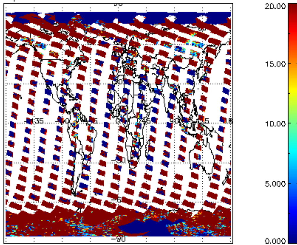
cL_opt_depth for 04MAR2011 00:00:00 to 05MAR2011 00:00:00
