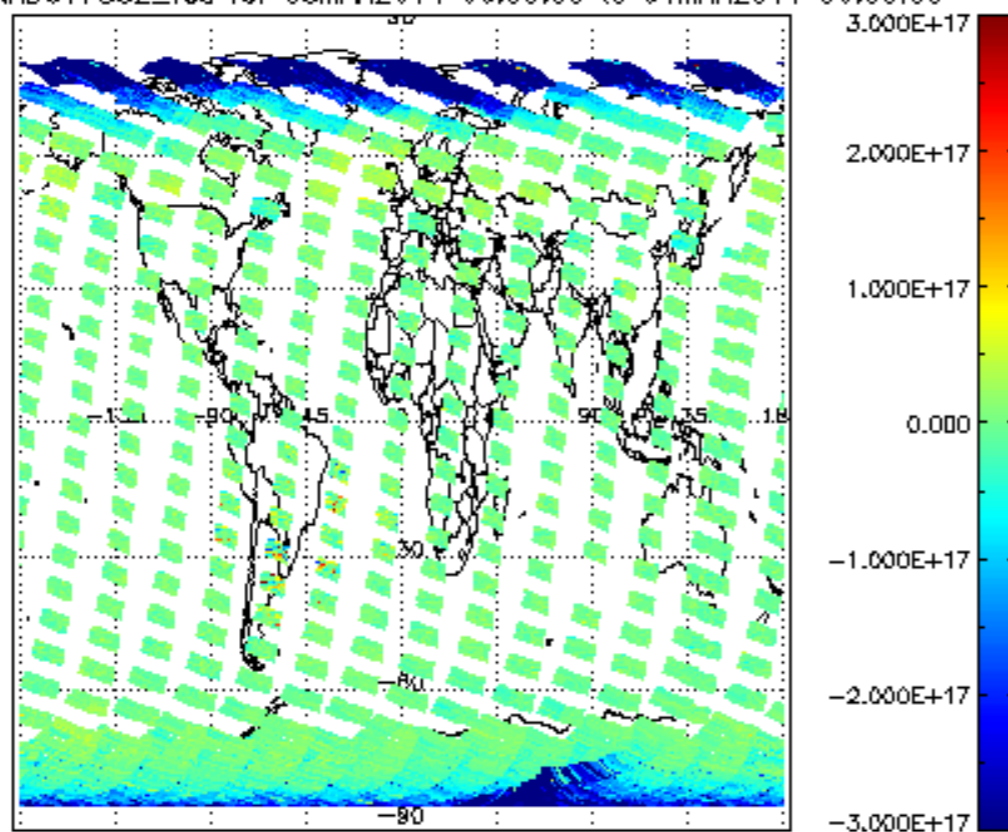
SCIOL2P_NADUV7S02_vcd for 03MAR2011 00:00:00 to 04MAR2011 00:00:00
