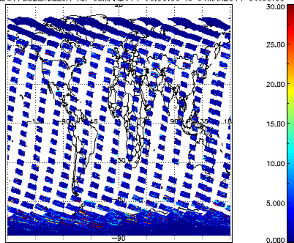
SCIOL2P_NADUV7S02_vcd_err for 03MAR2011 00:00:00 to 04MAR2011 00:00:00
