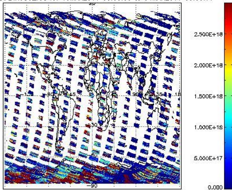
SCIOL2P_NADIR3CO_vcd for 03MAR2011 00:00:00 to 04MAR2011 00:00:00
