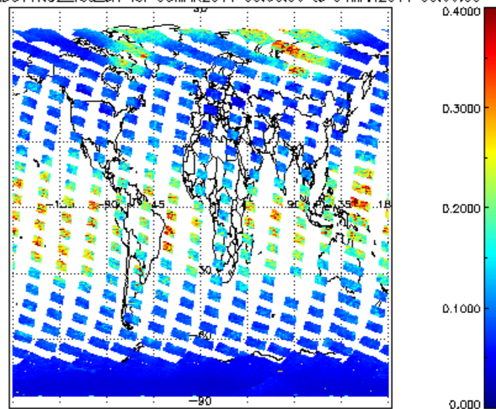
SCIOL2P_NADUV1NO2_vcd_err for 03MAR2011 00:00:00 to 04MAR2011 00:00:00
