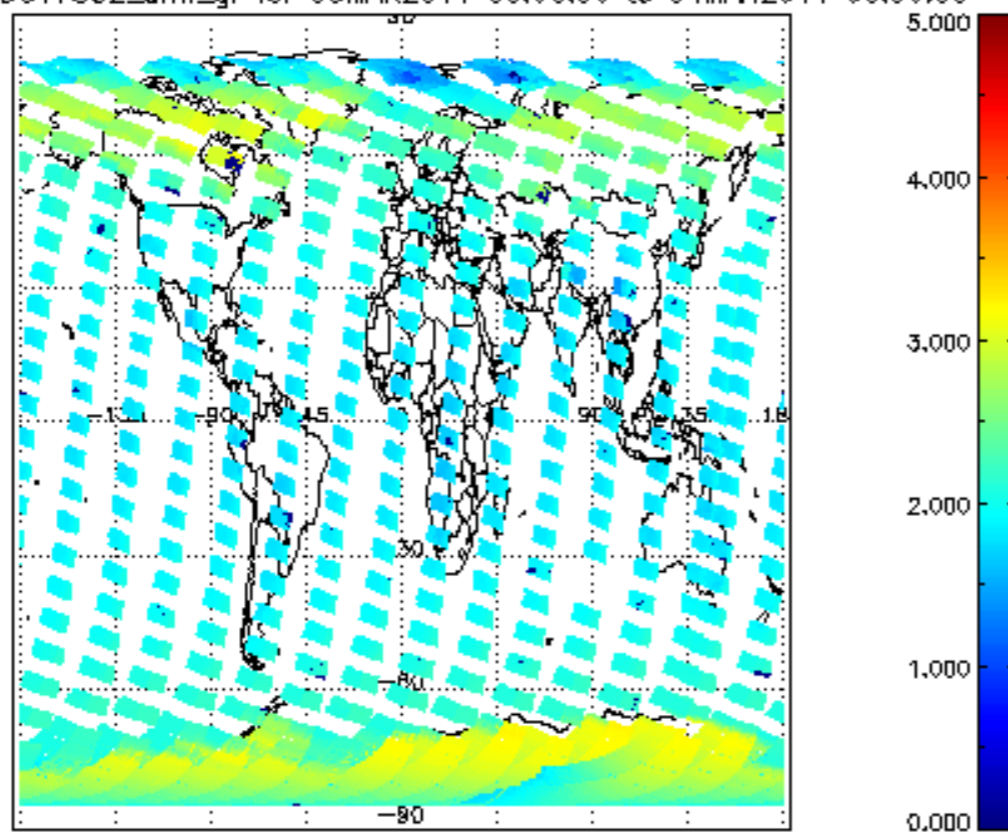
SCIOL2P_NADUV7S02_amf_gr for 03MAR2011 00:00:00 to 04MAR2011 00:00:00
