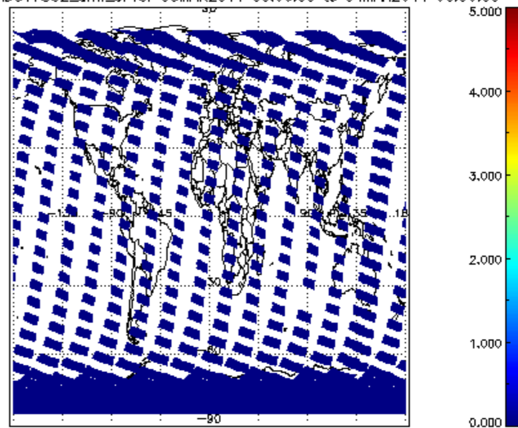
SCIOL2P_NADUV7S02_amf_cl for 03MAR2011 00:00:00 to 04MAR2011 00:00:00
