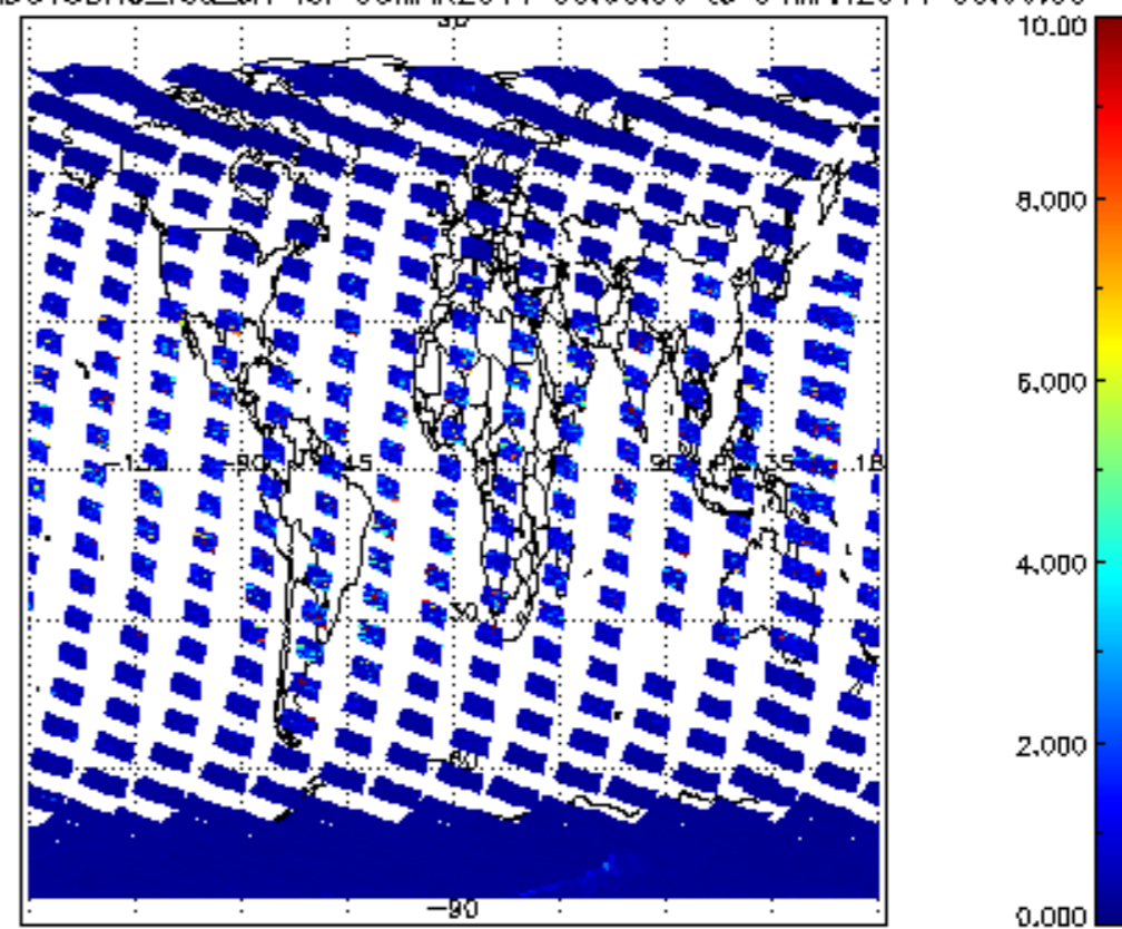
SCIOL2P_NADUV3BRO_vcd_Lerr for 03MAR2011 00:00:00 to 04MAR2011 00:00:00
