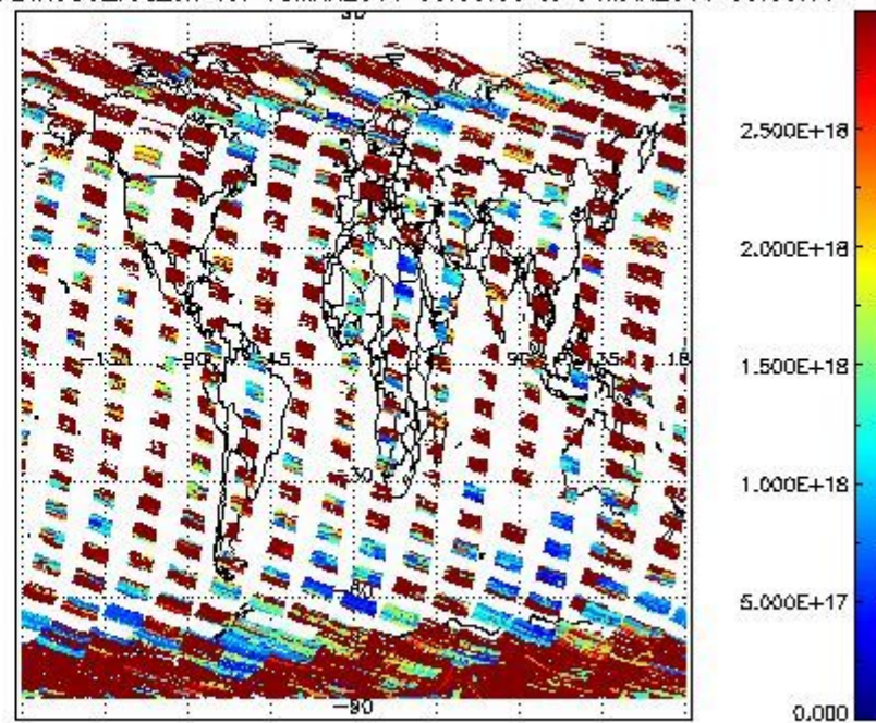
SCIOL2P_NADIR3CO_vcd_err for 03MAR2011 00:00:00 to 04MAR2011 00:00:00
