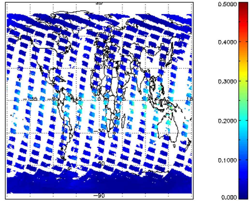
SCIOL2P_NADUV8H20_vcd_err for 02MAR2011 00:00:00 to 03MAR2011 00:00:00
