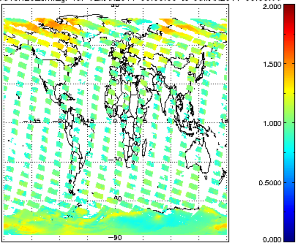
SCIOL2P_NADUV8H20_arnf_gr for 02MAR2011 00:00:00 to 03MAR2011 00:00:00
