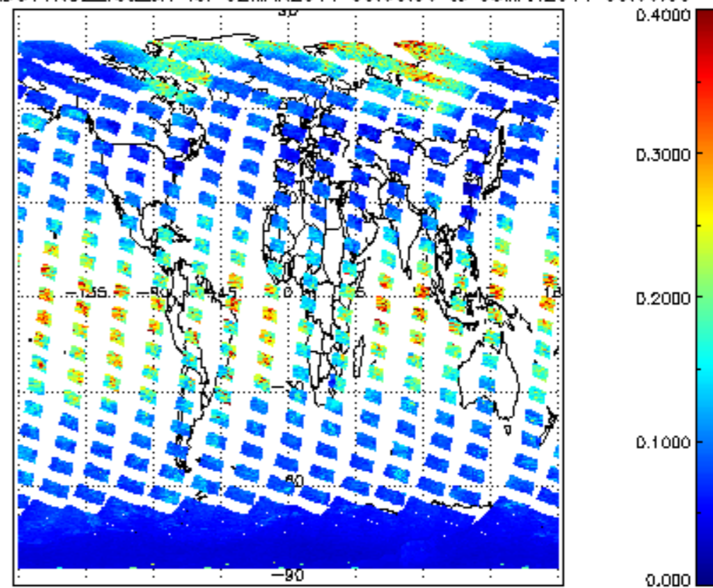
SCIOL2P_NADUV1NO2_vcd_err for 02MAR2011 00:00:00 to 03MAR2011 00:00:00
