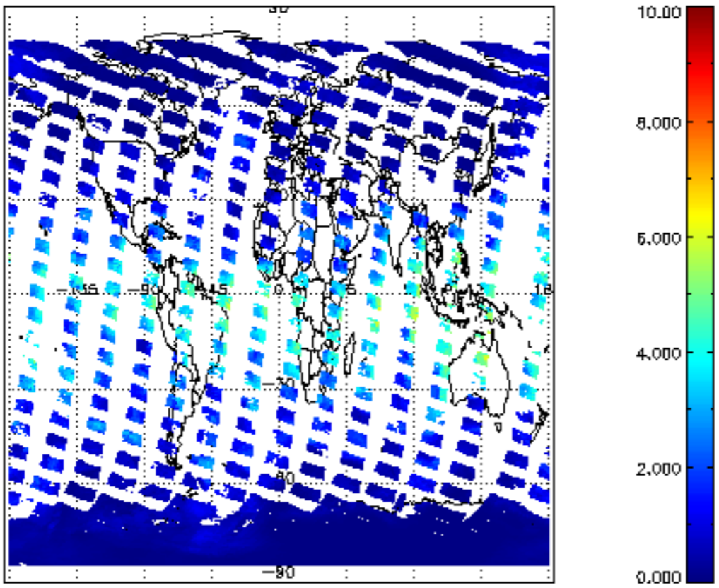
SCIOL2P_NADUV8H20_vcd for 02MAR2011 00:00:00 to 03MAR2011 00:00:00
