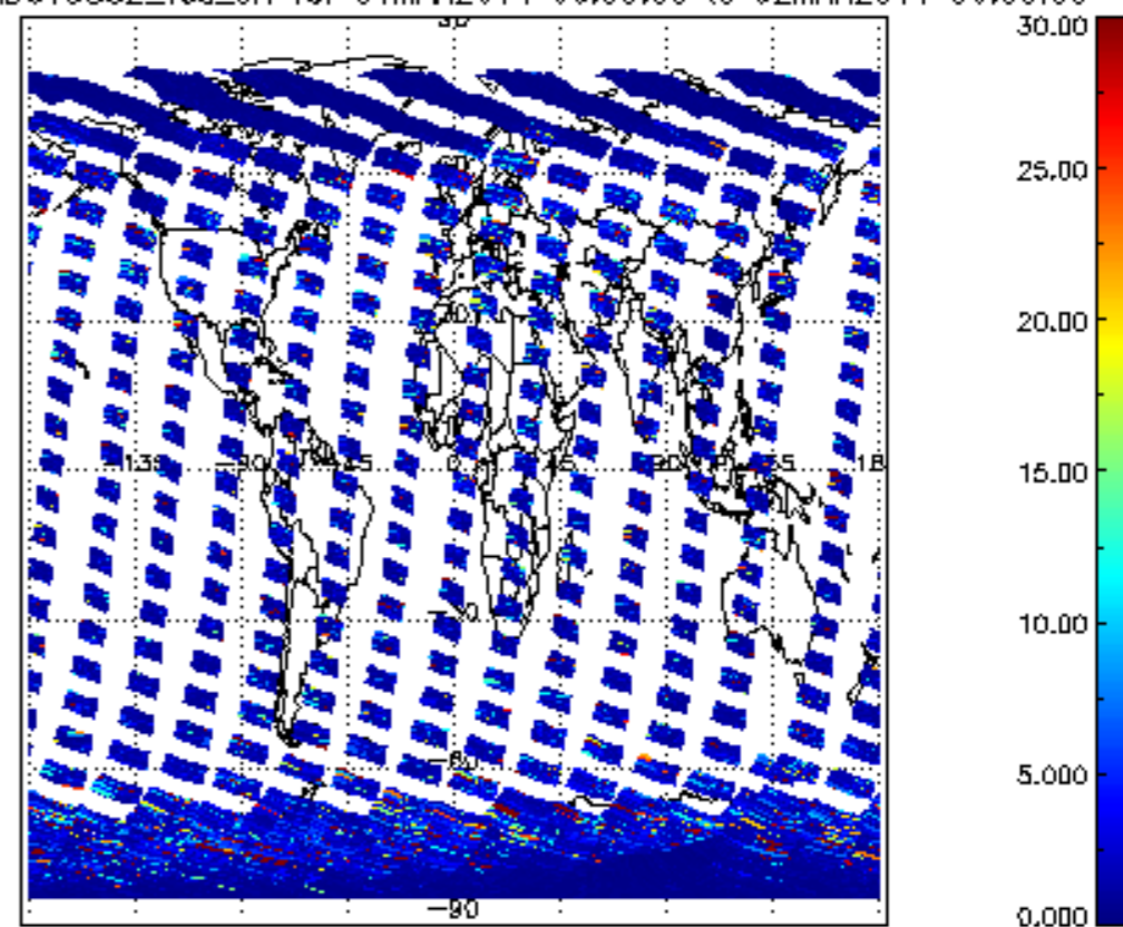
SCIOL2P_NADUV5S02_vcd_err for 01MAR2011 00:00:00 to 02MAR2011 00:00:00
