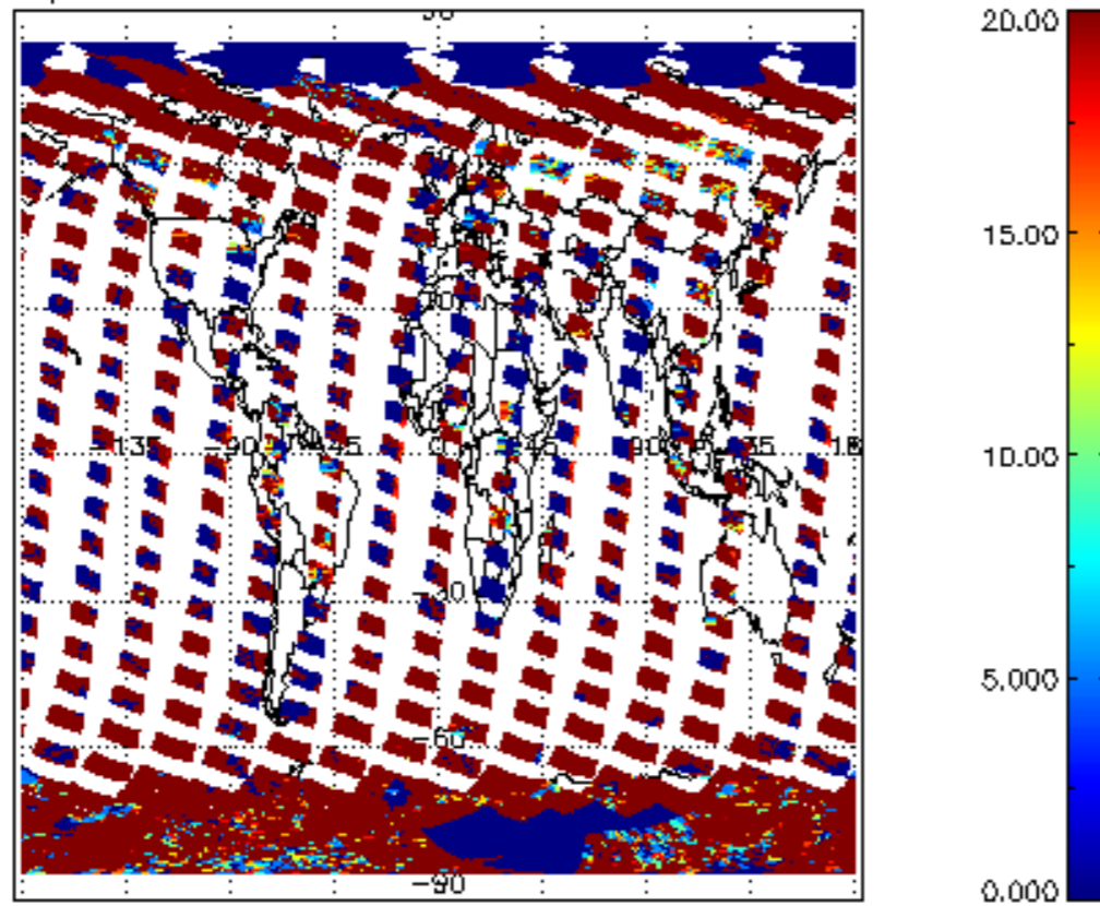
cL_opt_depth for 01MAR2011 00:00:00 to 02MAR2011 00:00:00
