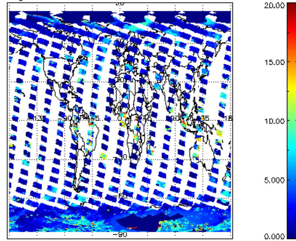
cL_top_height for 01MAR2011 00:00:00 to 02MAR2011 00:00:00
