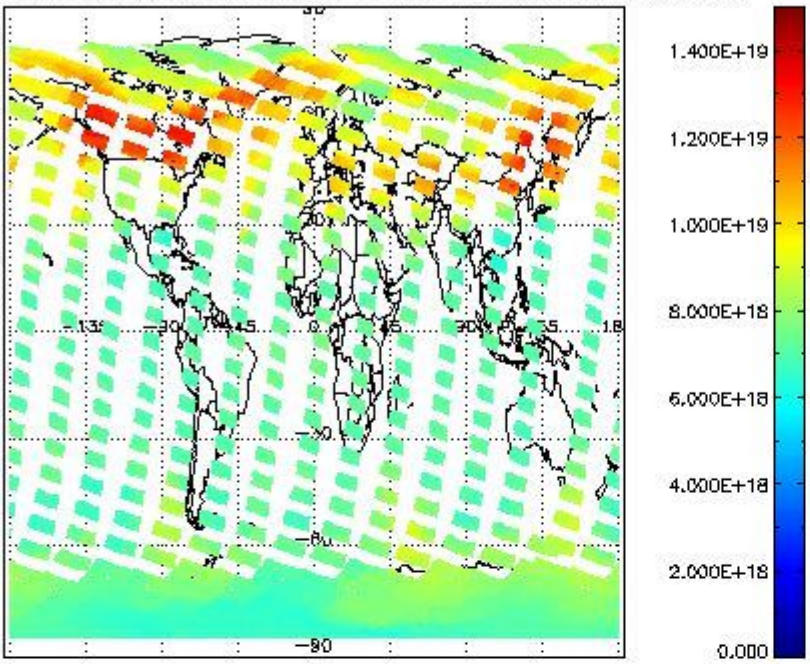
SCIOL2P_NADUV003_vcd for 01MAR2011 00:00:00 to 02MAR2011 00:00:00
