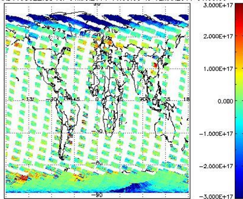
SCIOL2P_NADUV5SO2_vcd for 01MAR2011 00:00:00 to 02MAR2011 00:00:00
