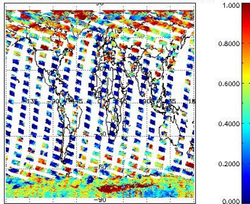
cL_frac for 01MAR2011 00:00:00 to 02MAR2011 00:00:00
