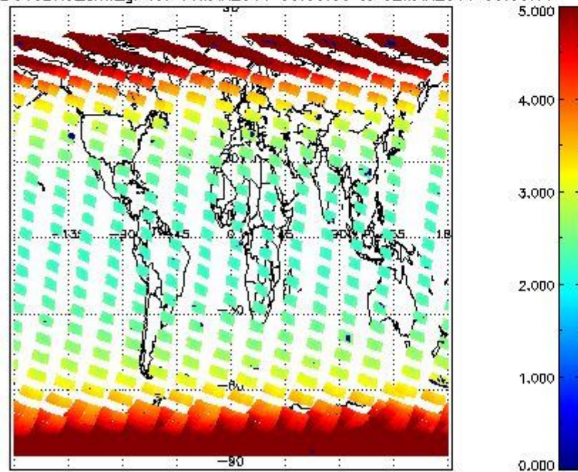
SCIOL2P_NADUV3BRO_amf_gr for 01MAR2011 00:00:00 to 02MAR2011 00:00:00
