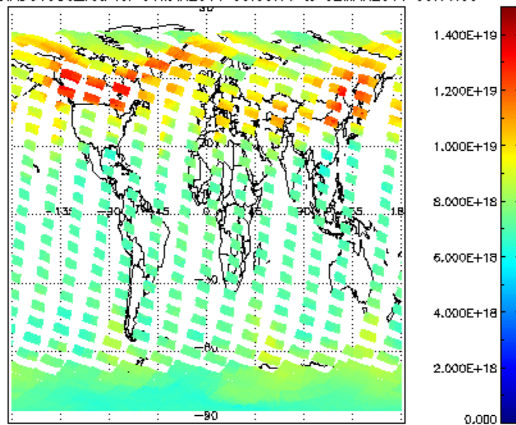
SCIOL2P_NADUV003_vcd for 01MAR2011 00:00:00 to 02MAR2011 00:00:00
