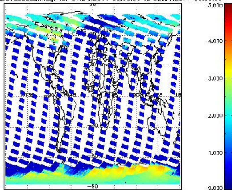
SCIOL2P_NADUV5SO2_amf_gr for 01MAR2011 00:00:00 to 02MAR2011 00:00:00
