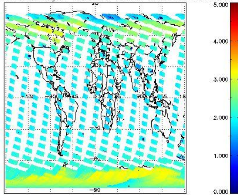
SCIOL2P_NADUV7S02_amf_gr for 01MAR2011 00:00:00 to 02MAR2011 00:00:00
