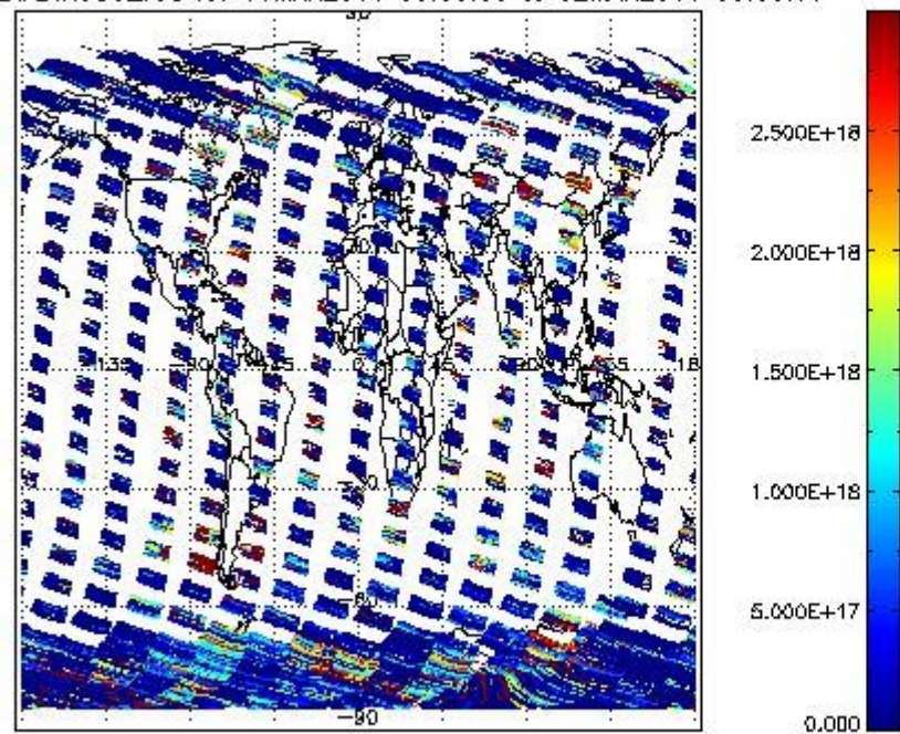
SCIDL2P_NADIR3CO_vcd for 01MAR2011 00:00:00 to 02MAR2011 00:00:00
