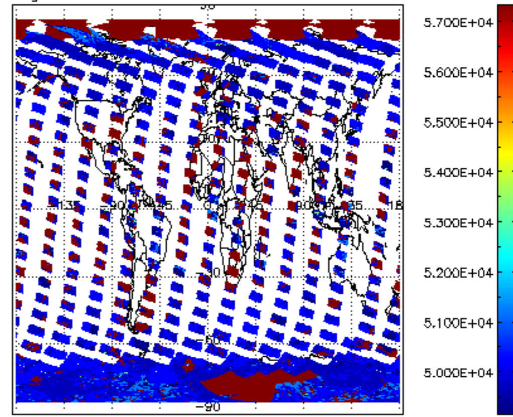
cloud_flags for 01MAR2011 00:00:00 to 02MAR2011 00:00:00
