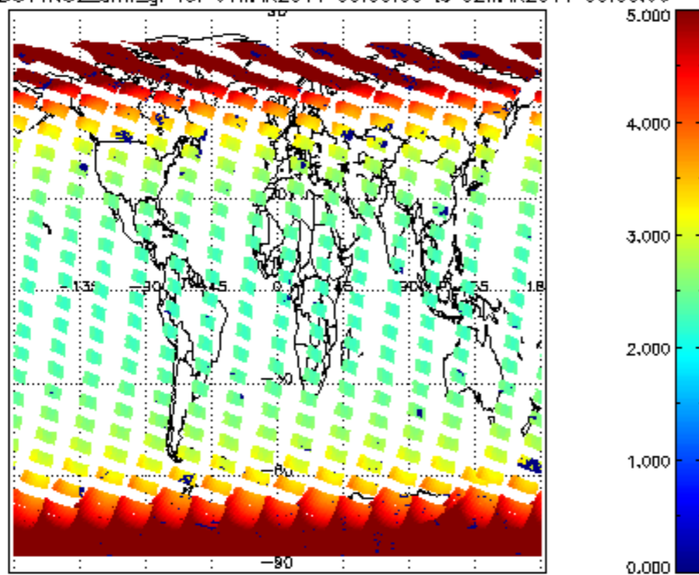
SCIOL2P_NADUV1NO2_amf_gr for 01MAR2011 00:00:00 to 02MAR2011 00:00:00
