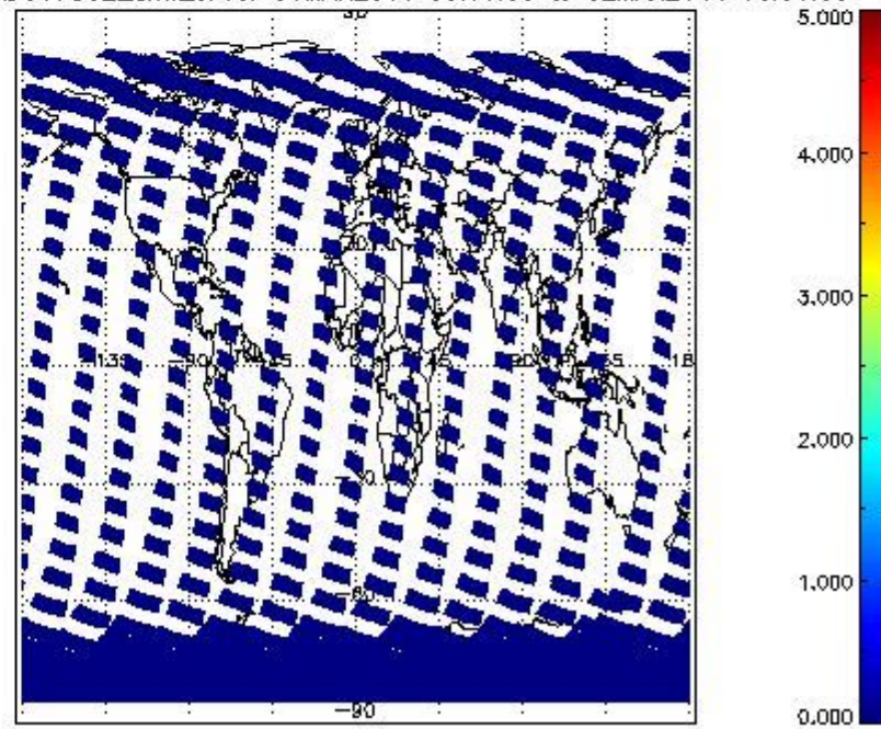
SCIOL2P_NADUV7S02_amf_cl for 01MAR2011 00:00:00 to 02MAR2011 00:00:00
