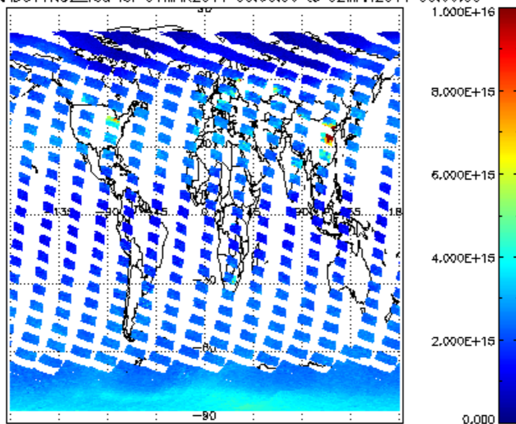
SCIOL2P_NADUV1NO2_vcd for 01MAR2011 00:00:00 to 02MAR2011 00:00:00
