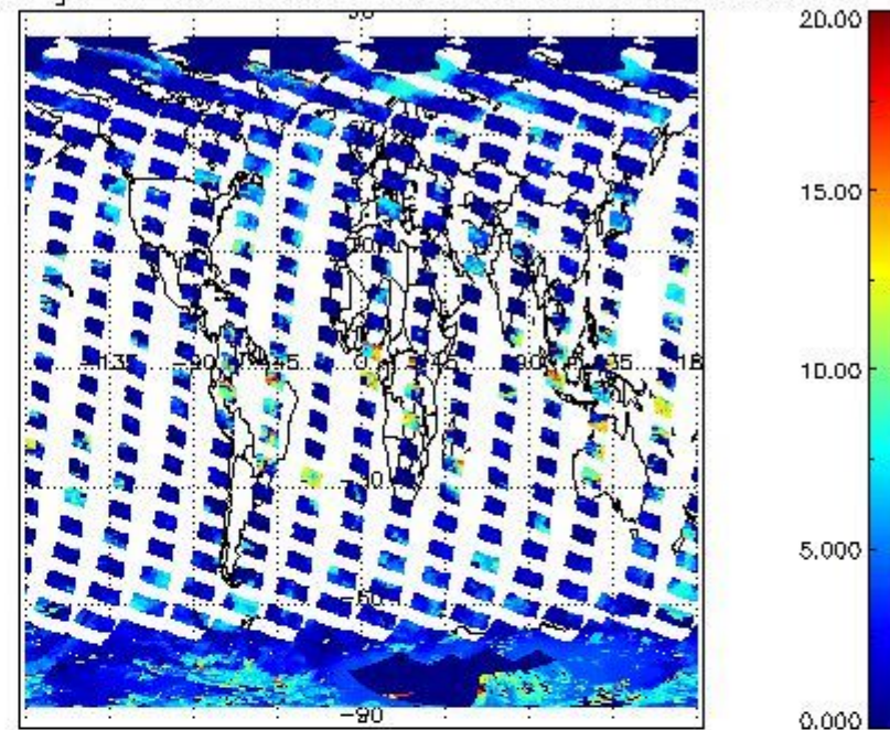
cL_top_height for 01MAR2011 00:00:00 to 02MAR2011 00:00:00
