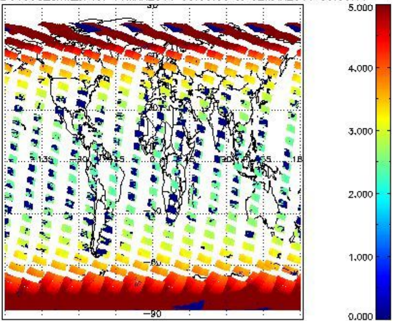
SCIOL2P_NADUV003_amf_cl for 01MAR2011 00:00:00 to 02MAR2011 00:00:00
