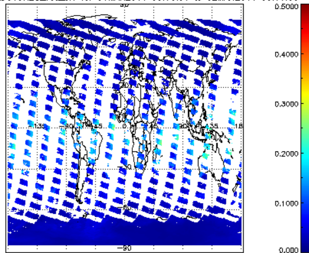
SCIOL2P_NADUV8H2O_vcd_Lerr for 01MAR2011 00:00:00 to 02MAR2011 00:00:00
