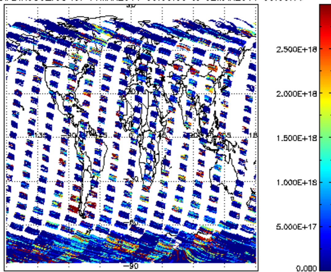
SCIOL2P_NADIR3CO_vcd for 01MAR2011 00:00:00 to 02MAR2011 00:00:00
