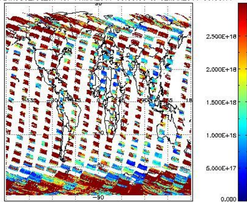
SCIDL2P_NADIR3CO_vcd_err for 01MAR2011 00:00:00 to 02MAR2011 00:00:00
