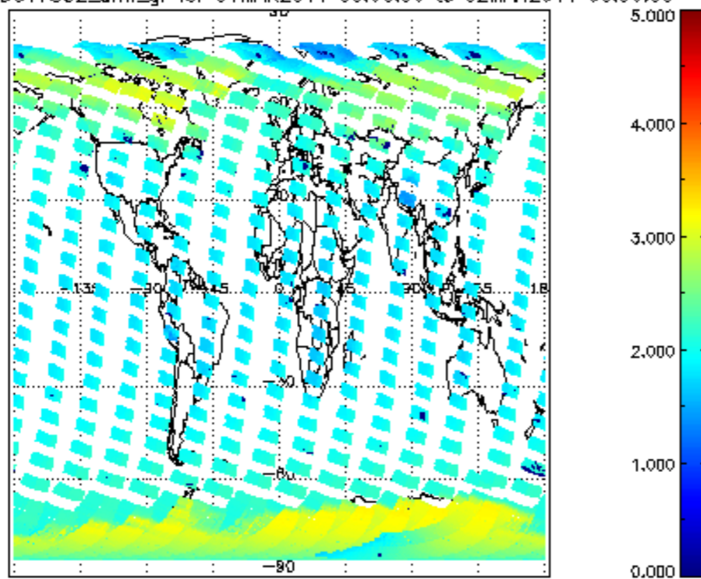
SCIOL2P_NADUV7S02_amf_gr for 01MAR2011 00:00:00 to 02MAR2011 00:00:00
