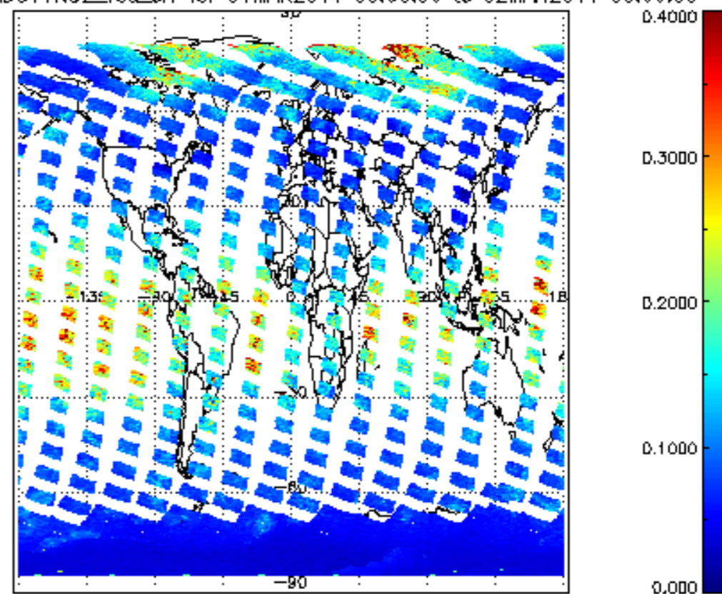
SCIOL2P_NADUV1NO2_vcdLerr for 01MAR2011 00:00:00 to 02MAR2011 00:00:00
