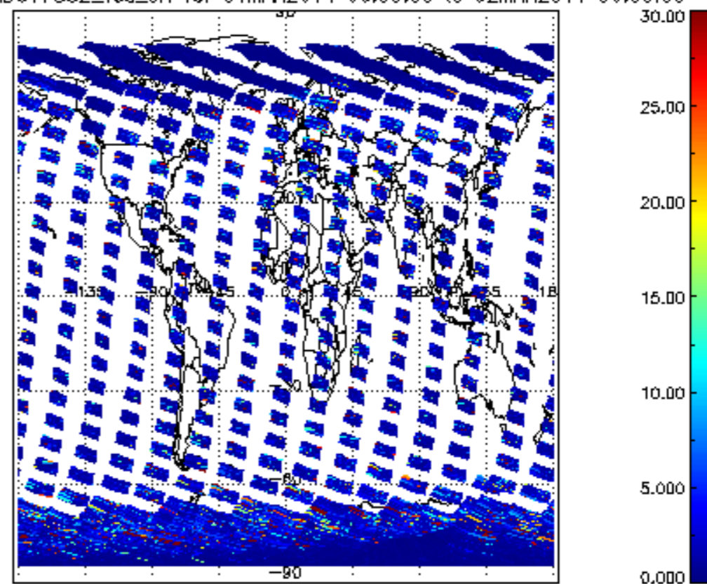
SCIOL2P_NADUV7S02_vcd_err for 01MAR2011 00:00:00 to 02MAR2011 00:00:00
