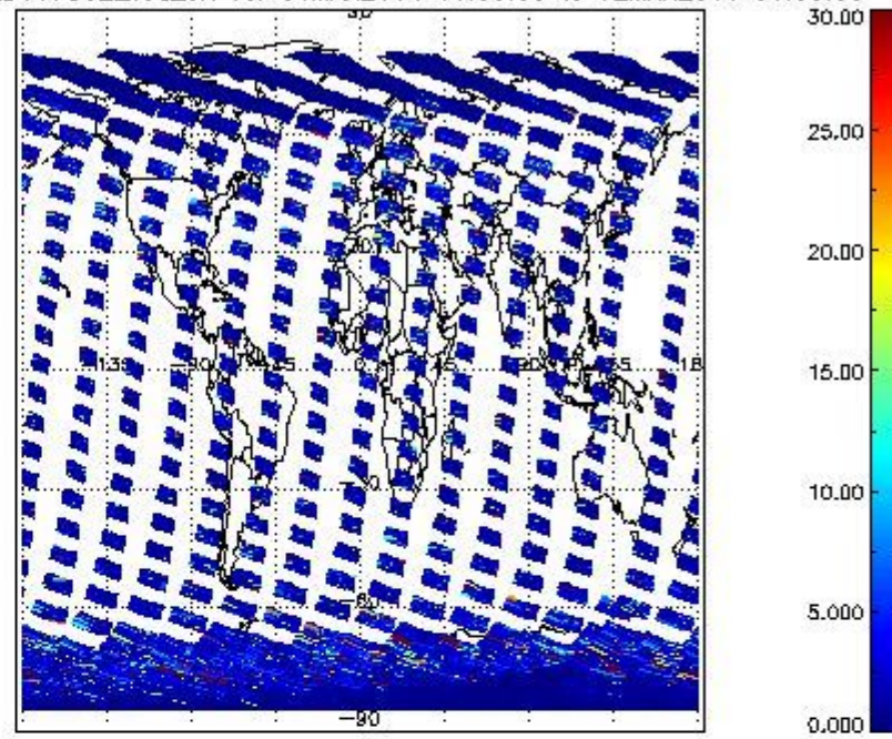
SCIOL2P_NADUV7S02_vcd_err for 01MAR2011 00:00:00 to 02MAR2011 00:00:00
