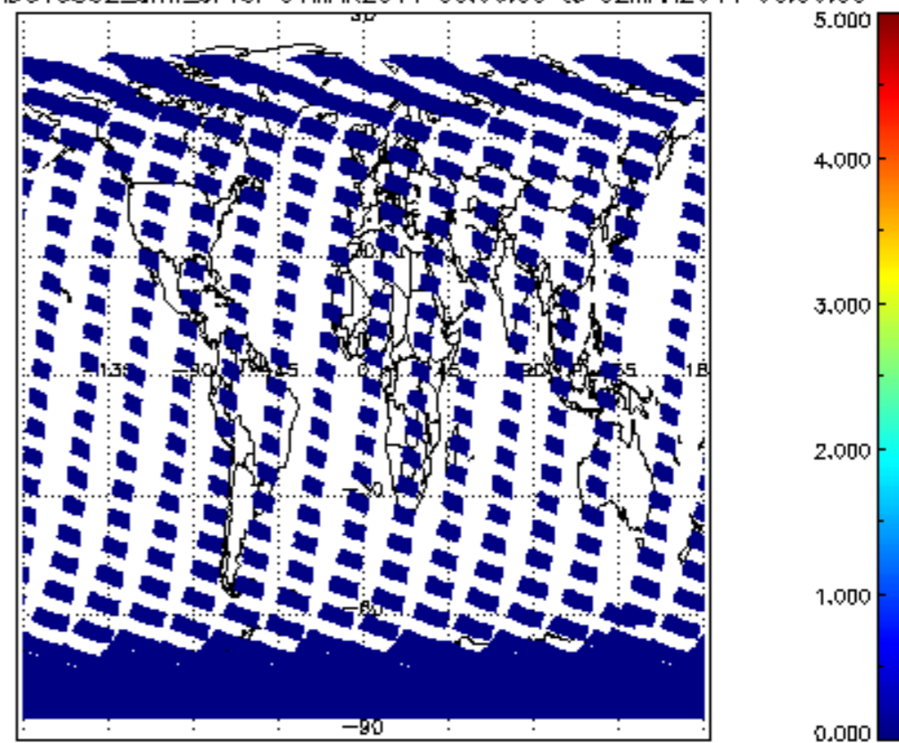
SCIOL2P_NADUV5S02_amf_cl for 01MAR2011 00:00:00 to 02MAR2011 00:00:00
