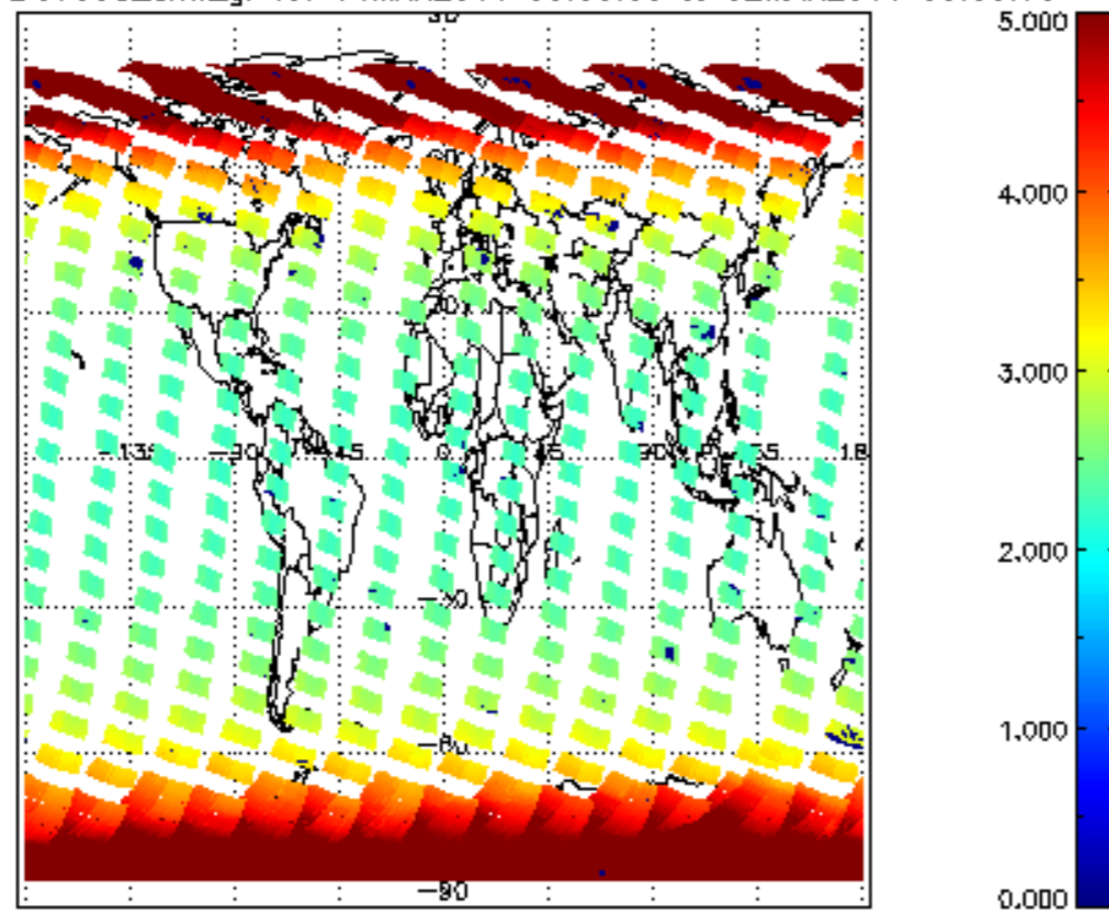
SCIOL2P_NADUV003_amf_gr for 01MAR2011 00:00:00 to 02MAR2011 00:00:00
