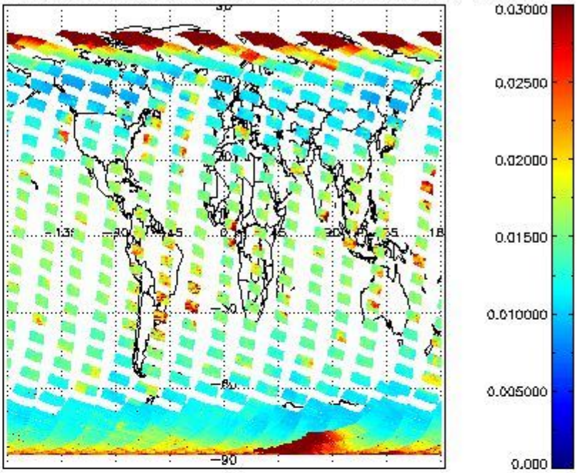
SCIOL2P_NADUV003_vcd_err for 01MAR2011 00:00:00 to 02MAR2011 00:00:00
