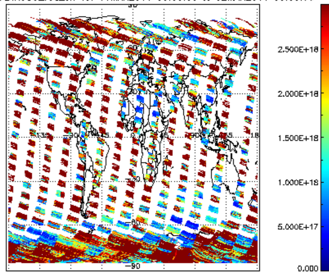
SCIOL2P_NADIR3CO_vcd_err for 01MAR2011 00:00:00 to 02MAR2011 00:00:00
