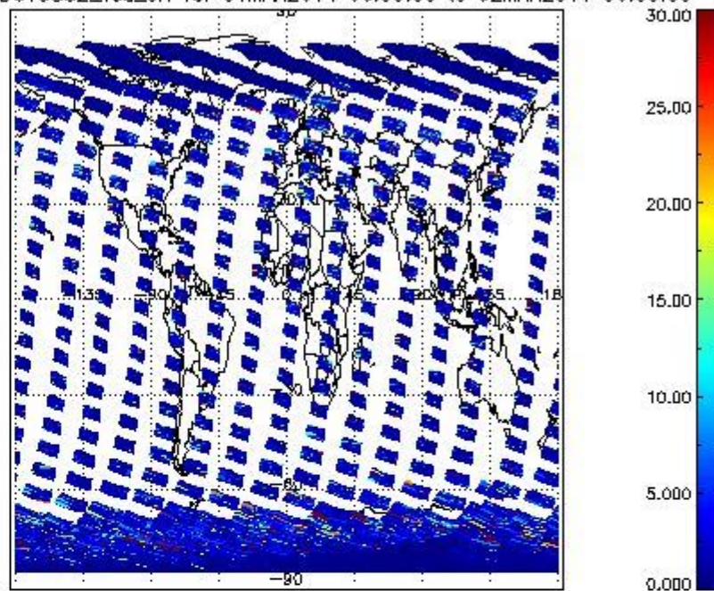
SCIOL2P_NADUV5SO2_vcd_err for 01MAR2011 00:00:00 to 02MAR2011 00:00:00
