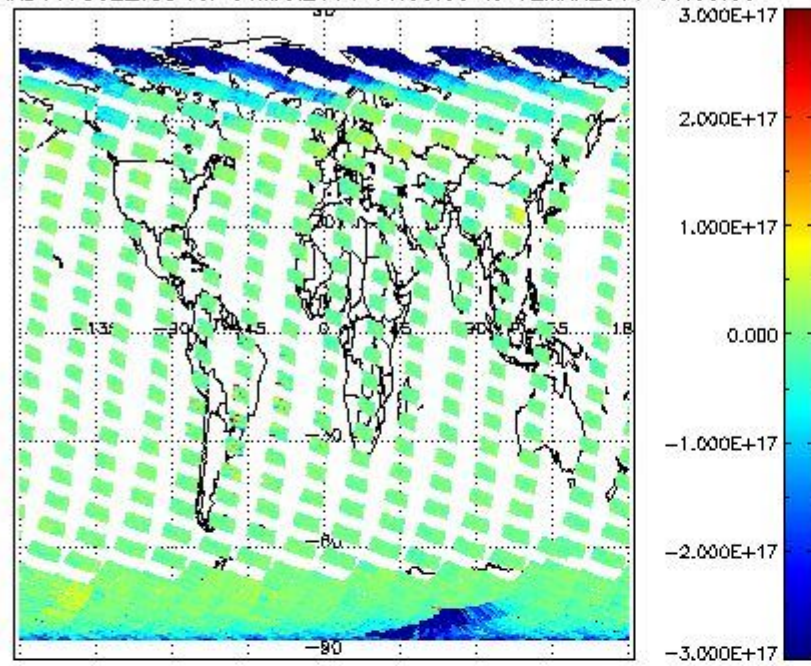
SCIOL2P_NADUV7S02_vcd for 01MAR2011 00:00:00 to 02MAR2011 00:00:00
