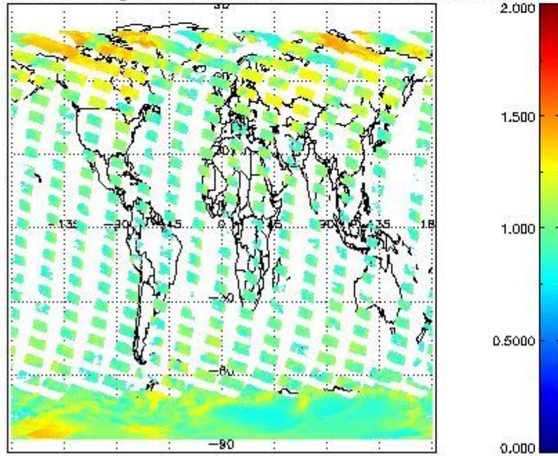
SCIOL2P_NADUV8H2O_amf_gr for 01MAR2011 00:00:00 to 02MAR2011 00:00:00
