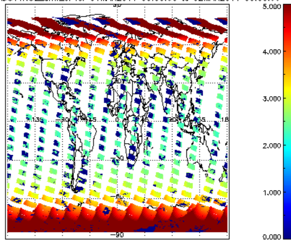
SCIOL2P_NADUV1NO2_amf_cl for 01MAR2011 00:00:00 to 02MAR2011 00:00:00
