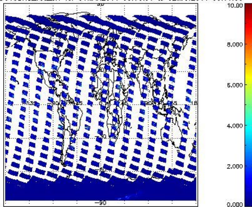
SCIOL2P_NADUV3BRO_vcd_err for 01MAR2011 00:00:00 to 02MAR2011 00:00:00
