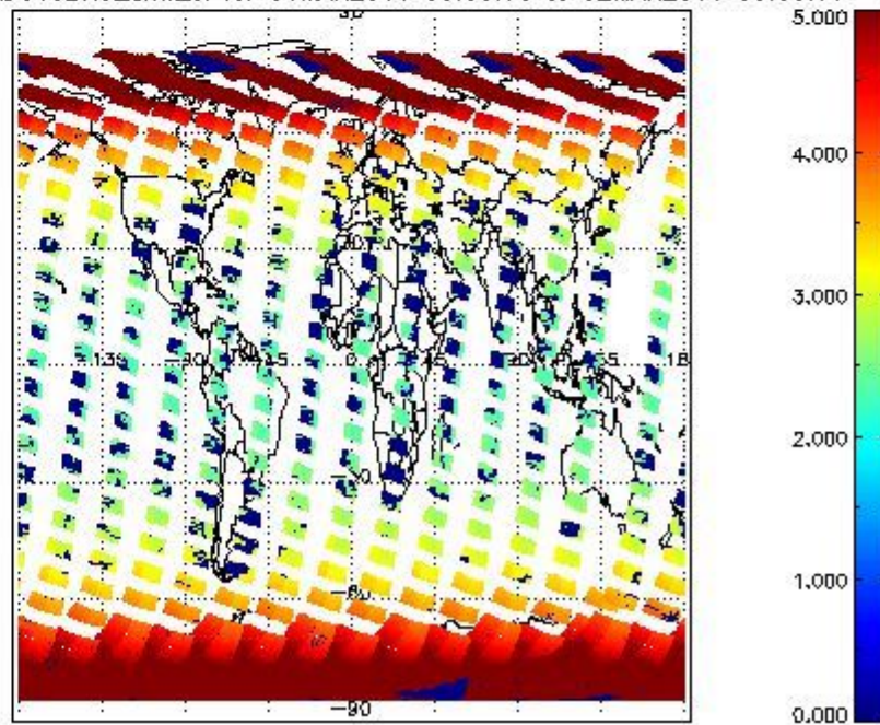
SCIOL2P_NADUV3BRO_amf_cl for 01MAR2011 00:00:00 to 02MAR2011 00:00:00
