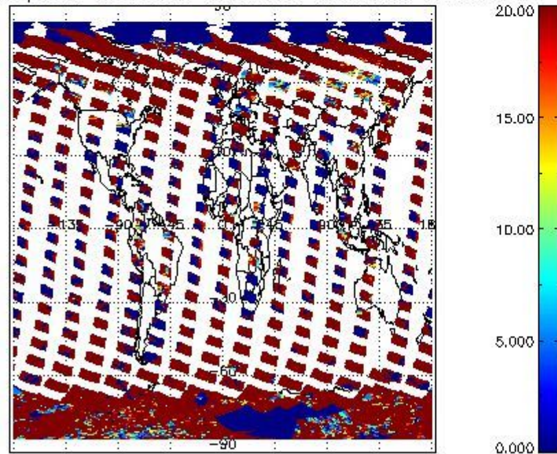
cL_opt_depth for 01MAR2011 00:00:00 to 02MAR2011 00:00:00
