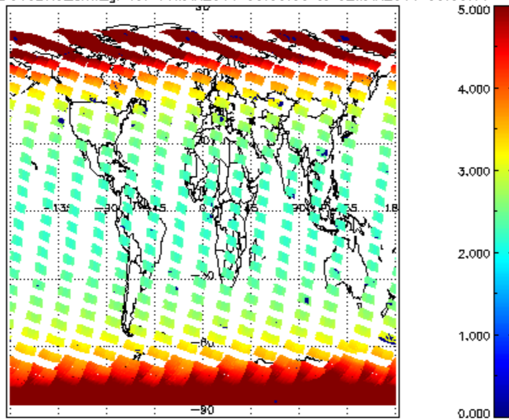
SCIOL2P_NADUV3BRO_arnf_gr for 01MAR2011 00:00:00 to 02MAR2011 00:00:00
