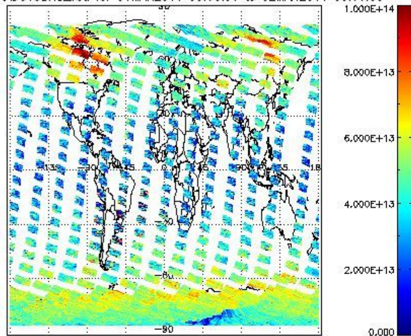
SCIOL2P_NADUV3BRO_vcd for 01MAR2011 00:00:00 to 02MAR2011 00:00:00
