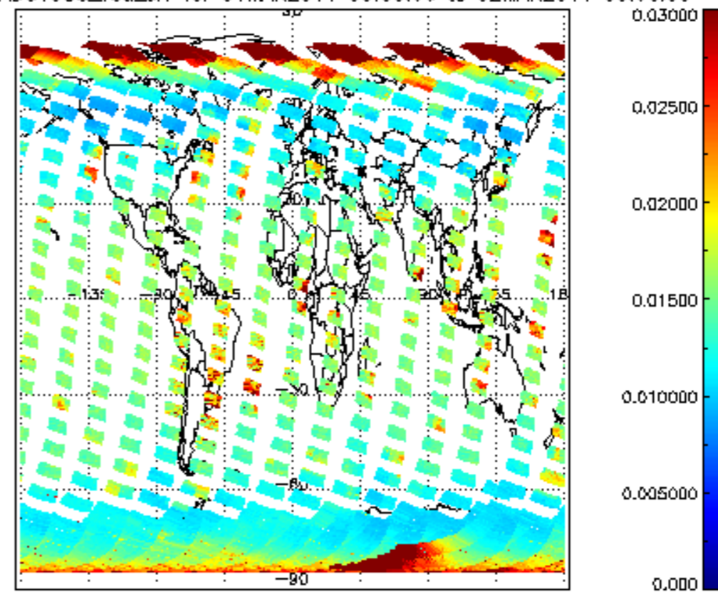
SCIOL2P_NADUV003_vcd_err for 01MAR2011 00:00:00 to 02MAR2011 00:00:00
