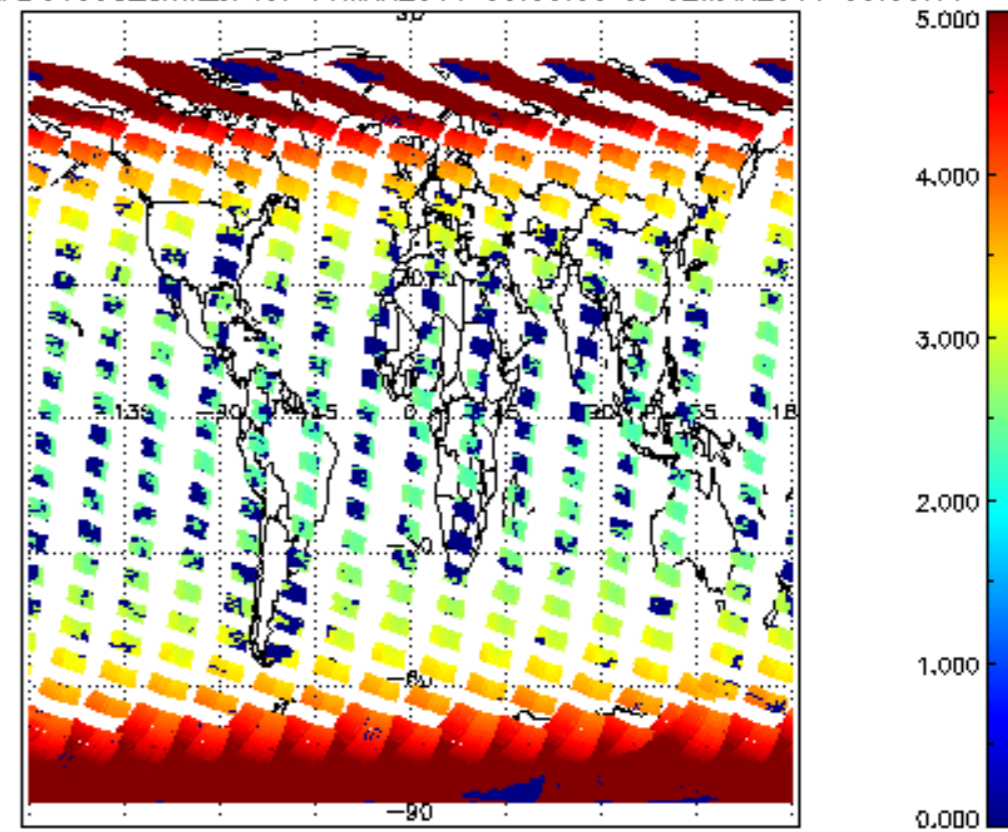
SCIOL2P_NADUV003_amf_cl for 01MAR2011 00:00:00 to 02MAR2011 00:00:00
