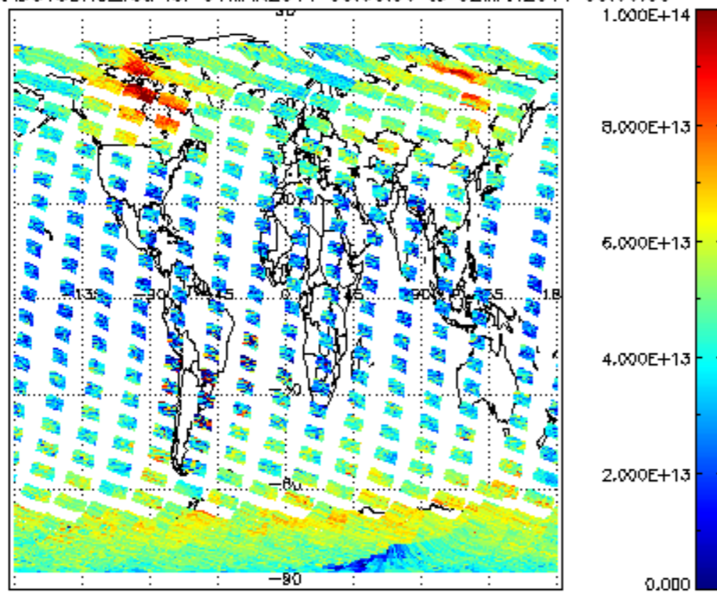
SCIOL2P_NADUV3BRO_vcd for 01MAR2011 00:00:00 to 02MAR2011 00:00:00
