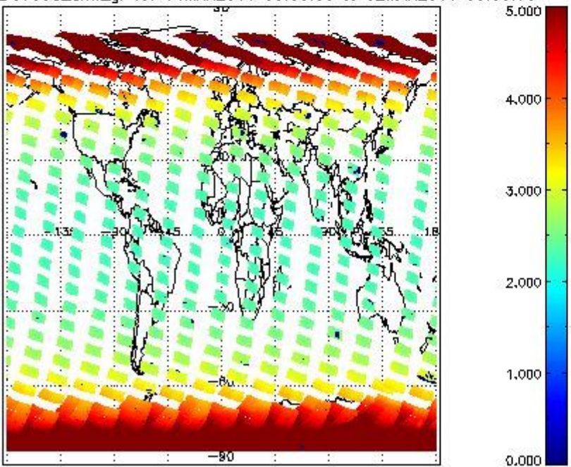
SCIOL2P_NADUV003_amf_gr for 01MAR2011 00:00:00 to 02MAR2011 00:00:00
