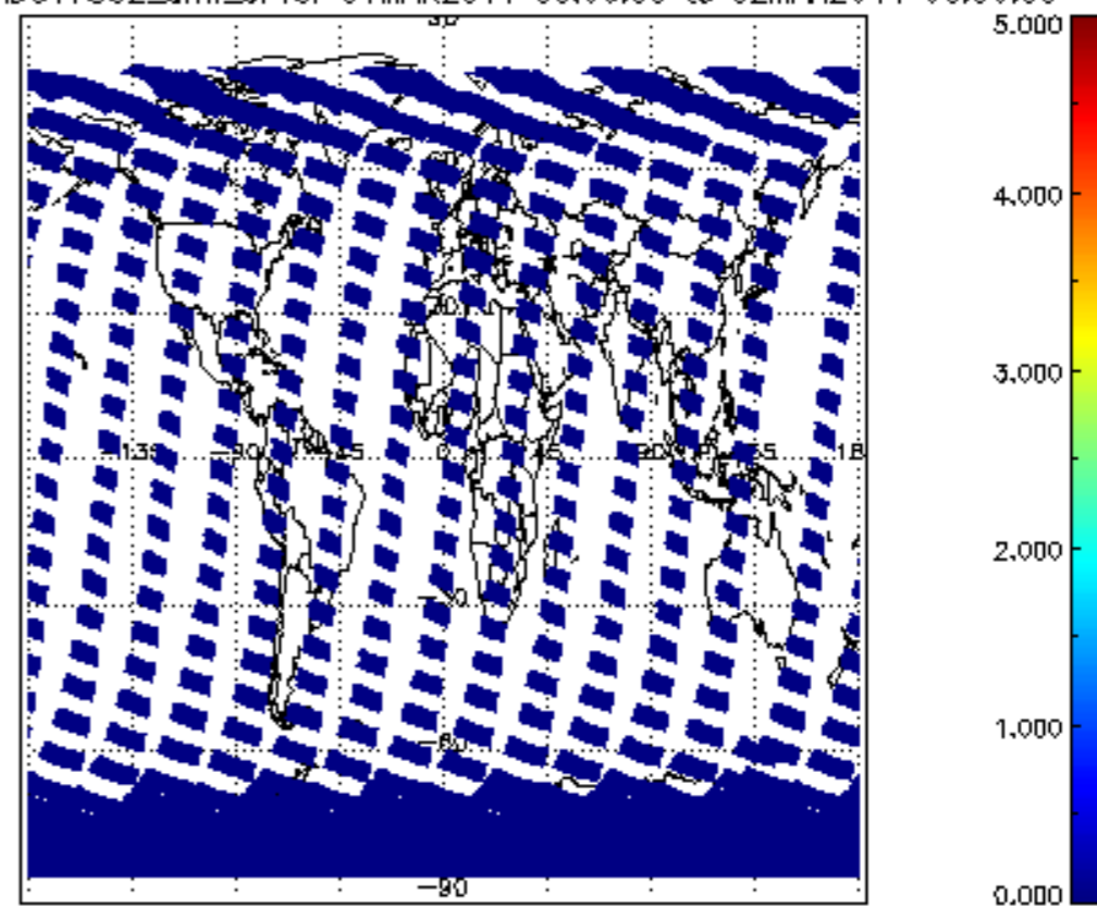
SCIOL2P_NADUV7S02_amf_cl for 01MAR2011 00:00:00 to 02MAR2011 00:00:00
