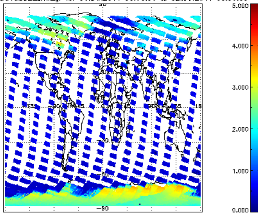
SCIOL2P_NADUV5S02_amf_gr for 01MAR2011 00:00:00 to 02MAR2011 00:00:00
