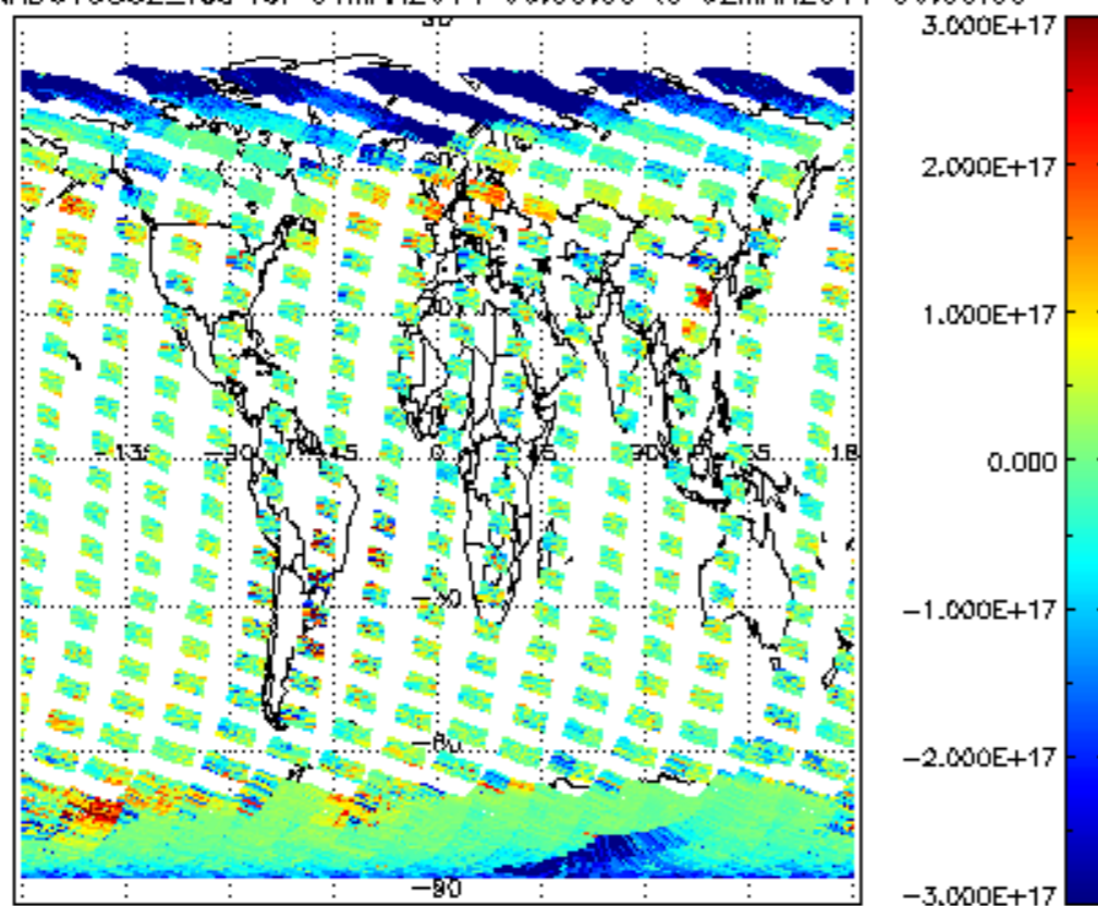
SCIOL2P_NADUV5S02_vcd for 01MAR2011 00:00:00 to 02MAR2011 00:00:00
