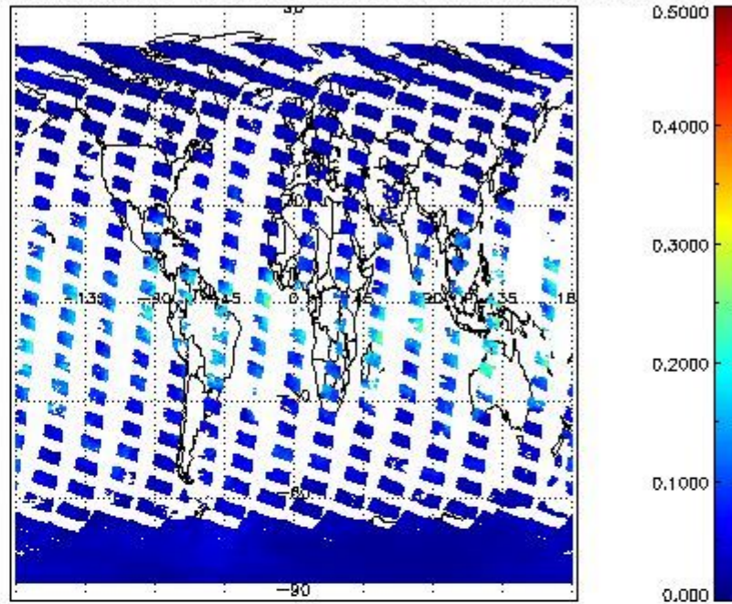
SCIOL2P_NADUV8H2O_vcd_err for 01MAR2011 00:00:00 to 02MAR2011 00:00:00
