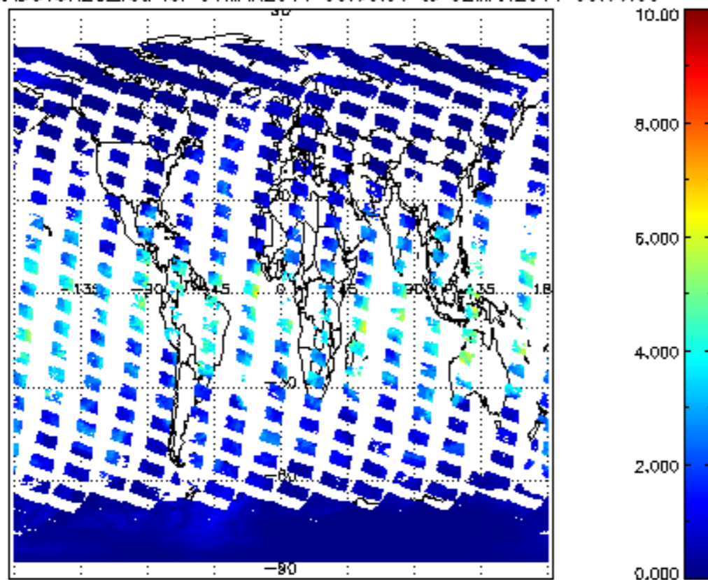
SCIOL2P_NADUV8H2O_vcd for 01MAR2011 00:00:00 to 02MAR2011 00:00:00
