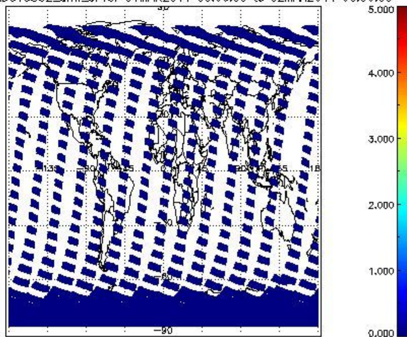
SCIOL2P_NADUV5SO2_amf_cl for 01MAR2011 00:00:00 to 02MAR2011 00:00:00
