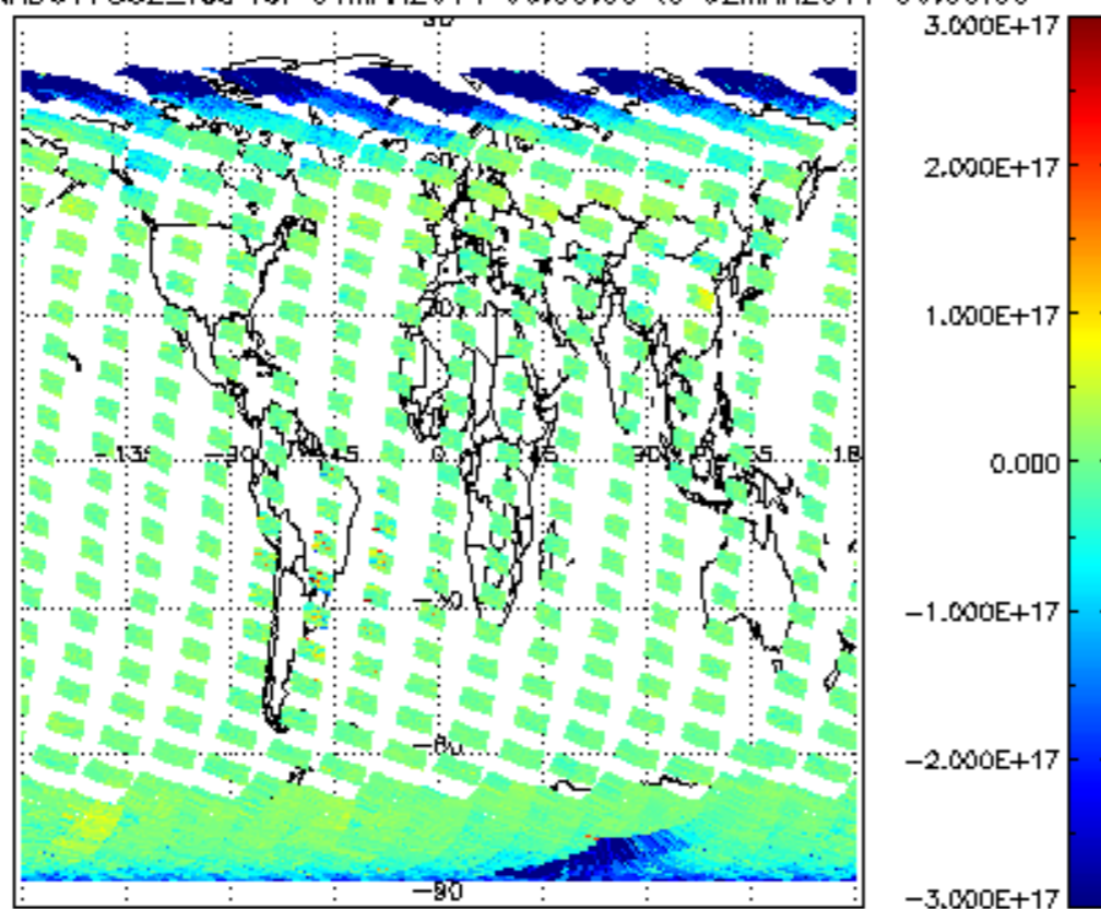
SCIOL2P_NADUV7S02_vcd for 01MAR2011 00:00:00 to 02MAR2011 00:00:00
