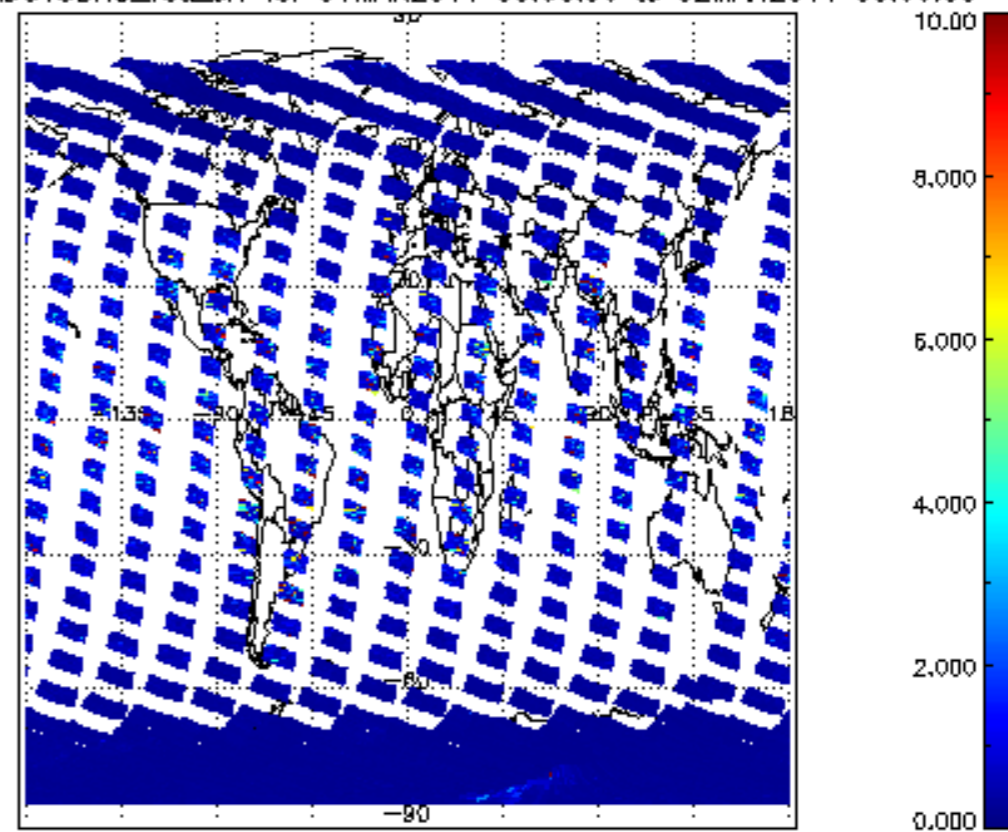
SCIOL2P_NADUV3BRO_vcd_Lerr for 01MAR2011 00:00:00 to 02MAR2011 00:00:00
