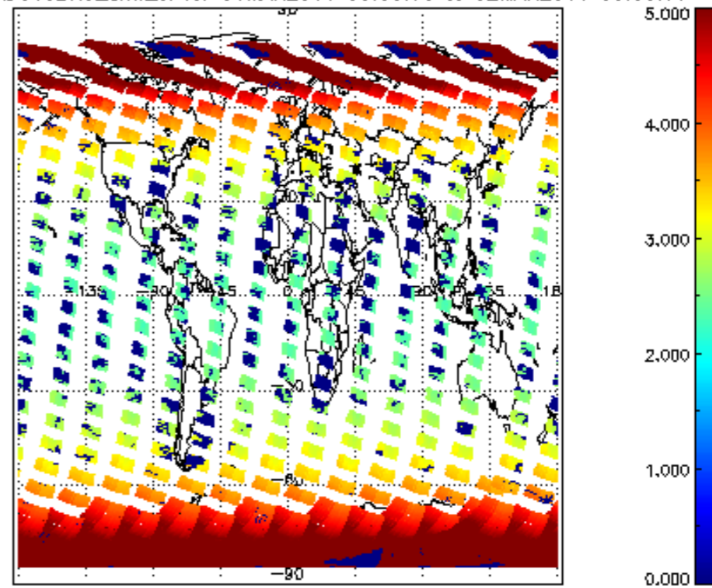
SCIOL2P_NADUV3BRO_arnf_cl for 01MAR2011 00:00:00 to 02MAR2011 00:00:00
