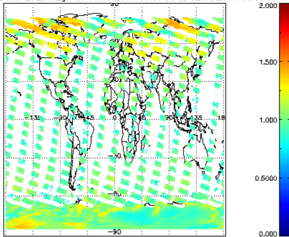
SCIOL2P_NADUV8H2O_arnf_gr for 01MAR2011 00:00:00 to 02MAR2011 00:00:00
