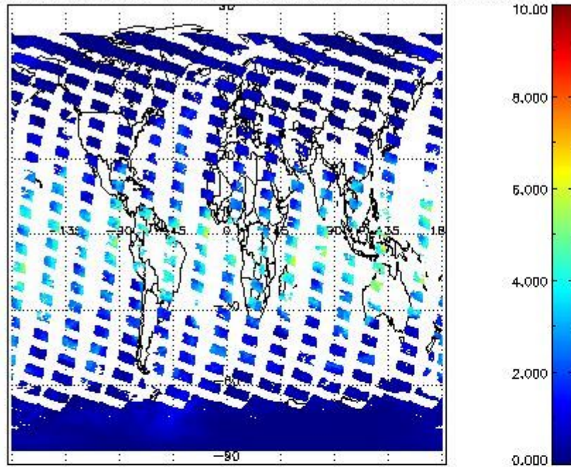
SCIOL2P_NADUV8H2O_vcd for 01MAR2011 00:00:00 to 02MAR2011 00:00:00
