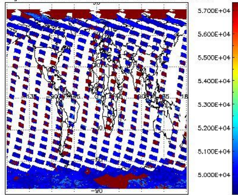
cloud_flags for 01MAR2011 00:00:00 to 02MAR2011 00:00:00
