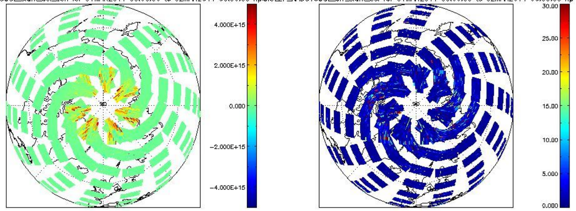
CIOL2P_NADUV6OCL_slant_col_den for 01MAR2011 00:00:00 to 02MAR2011 00:00:00 np CIOL2P_NADUV6OCL_err_slant_col for 01MAR2011 00:00:00 to 02MAR2011 00:00:00 np
