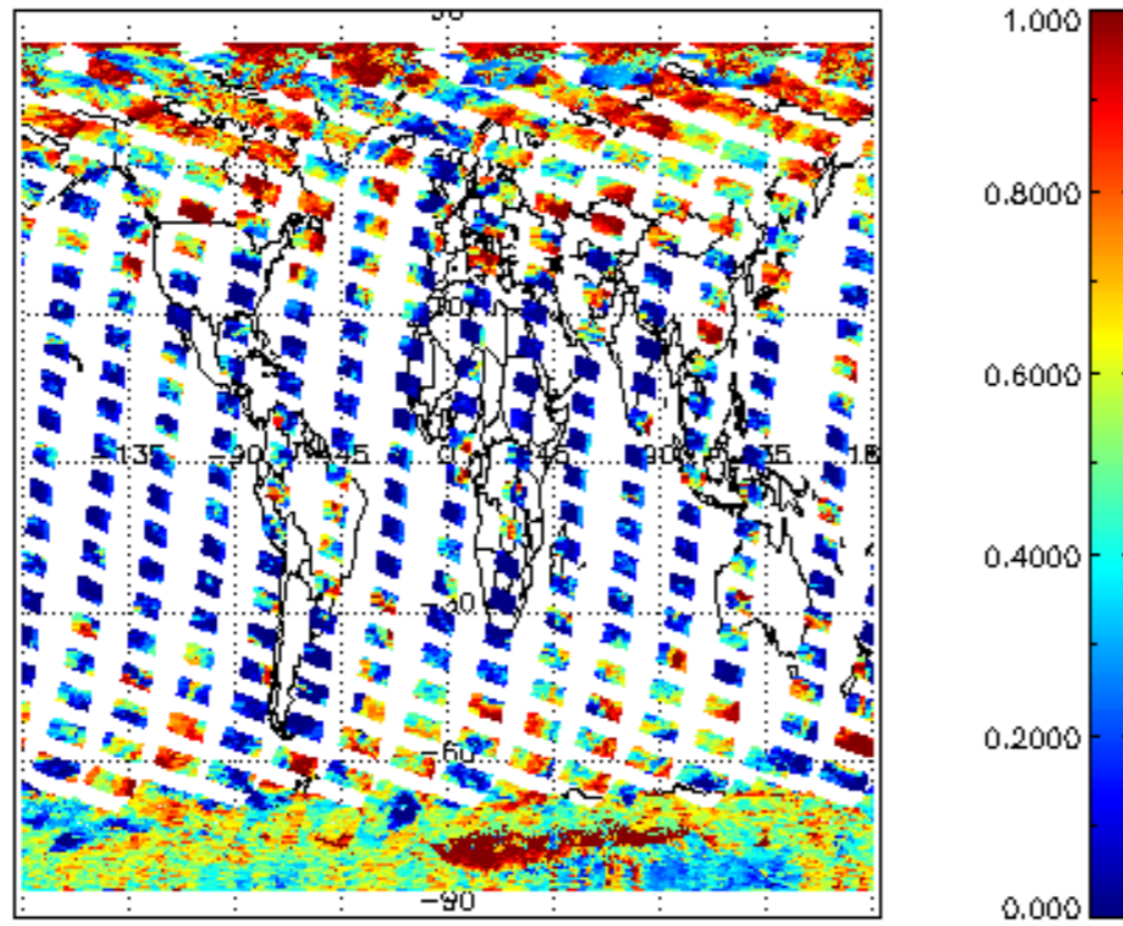
cL_frac for 01MAR2011 00:00:00 to 02MAR2011 00:00:00
