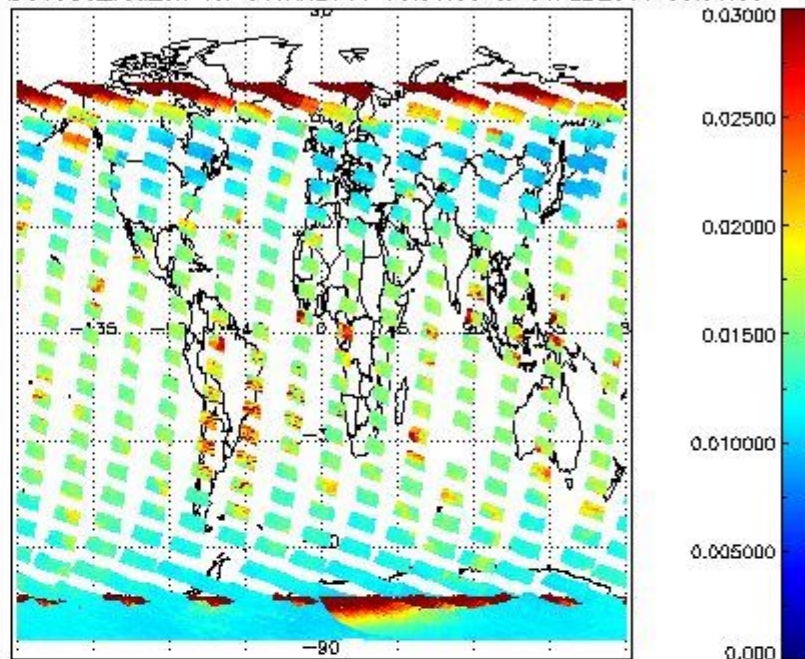
SCIOL2P_NADUV003_vcd_err for 31JAN2011 00:00:00 to 01FEB2011 00:00:00
