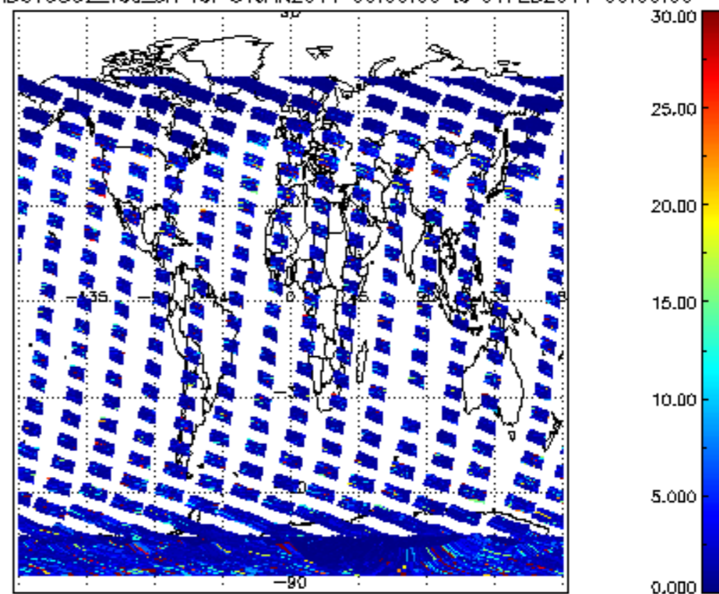
SCIOL2P_NADUV5S02_vcd_err for 31JAN2011 00:00:00 to 01FEB2011 00:00:00
