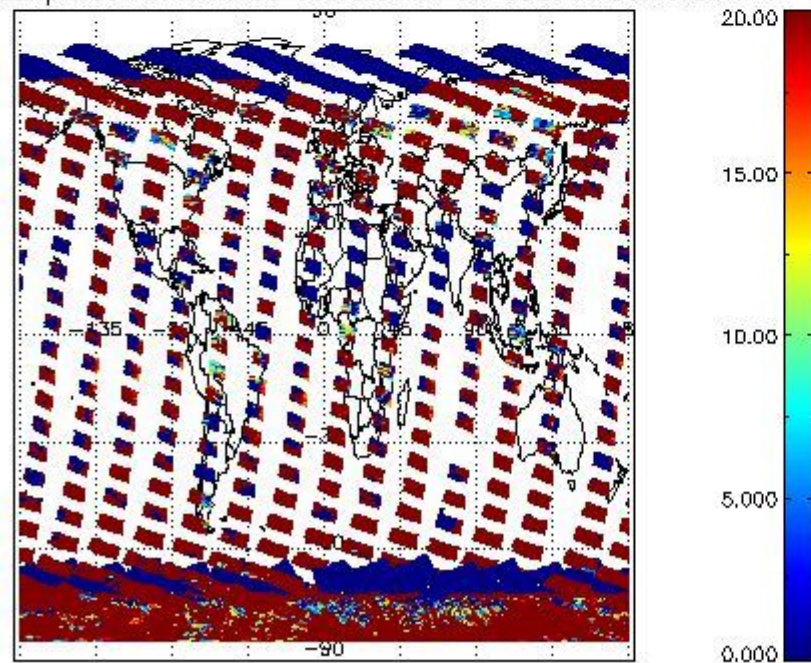
cL_opt_depth for 31JAN2011 00:00:00 to 01FEB2011 00:00:00
