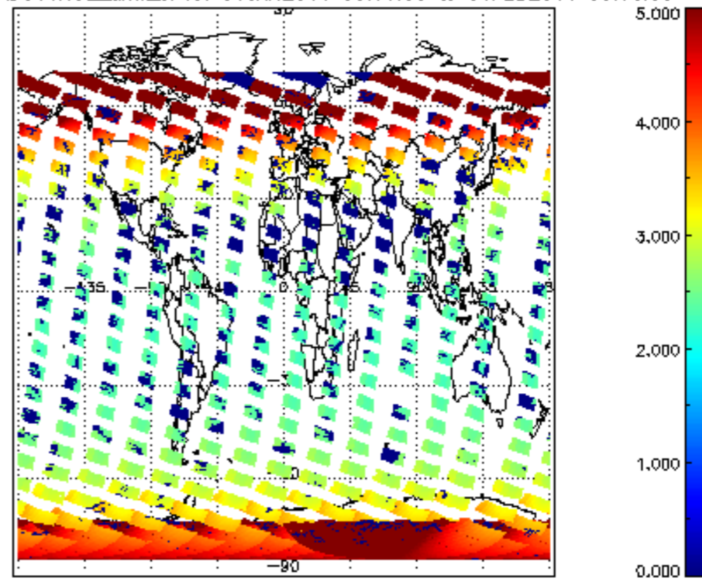
SCIOL2P_NADUV1NO2_amf_sl for 31JAN2011 00:00:00 to 01FEB2011 00:00:00
