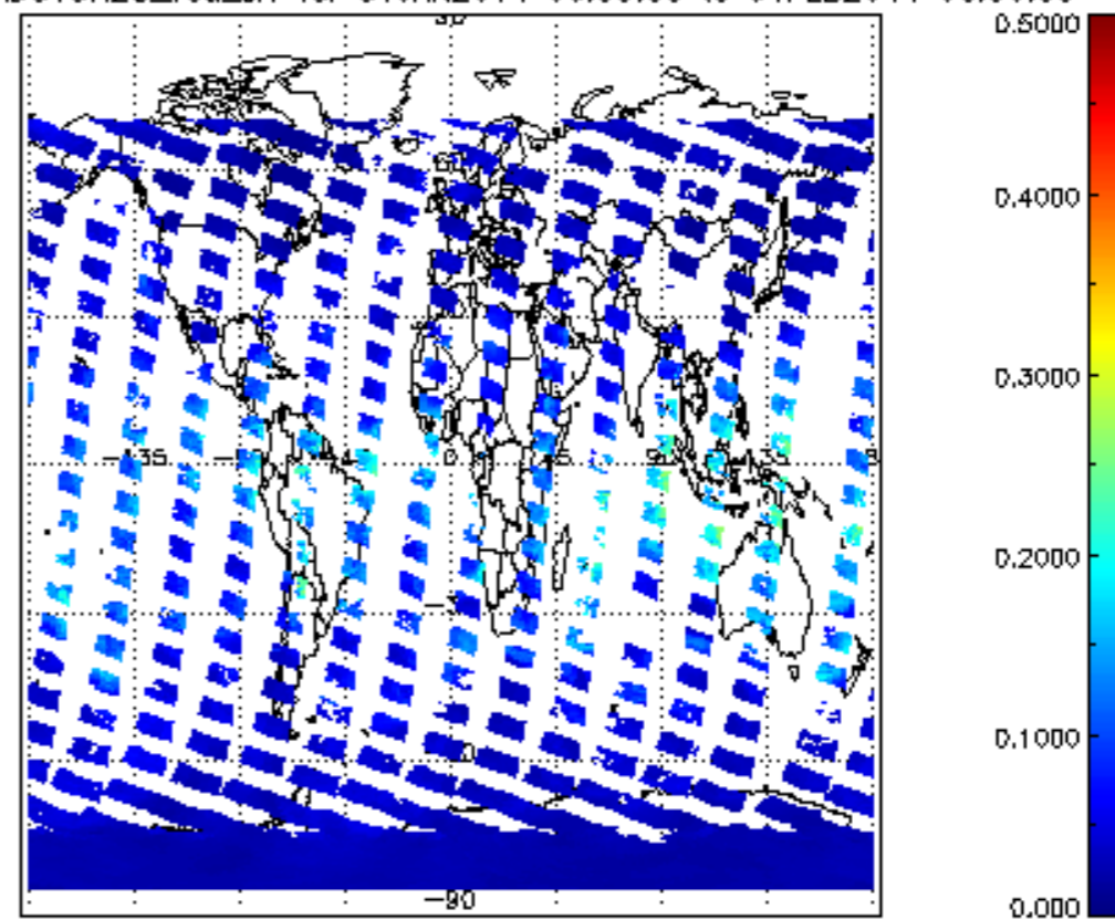
SCIOL2P_NADUV8H20_vcd_err for 31JAN2011 00:00:00 to 01FEB2011 00:00:00
