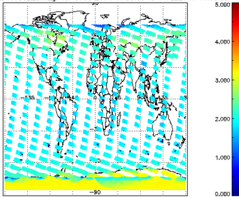
SCIOL2P_NADUV7S02_amf_gr for 31JAN2011 00:00:00 to 01FEB2011 00:00:00
