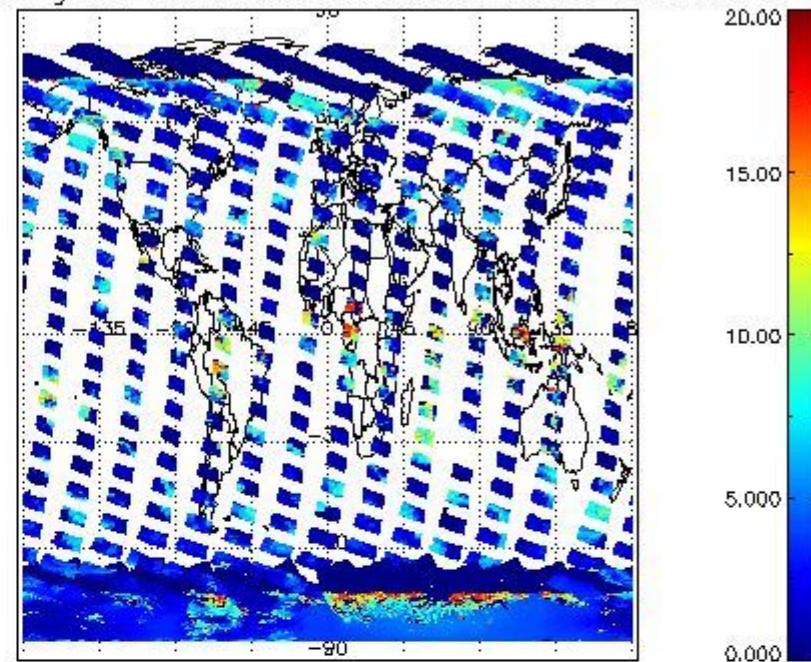
cL_top_height for 31JAN2011 00:00:00 to 01FEB2011 00:00:00
