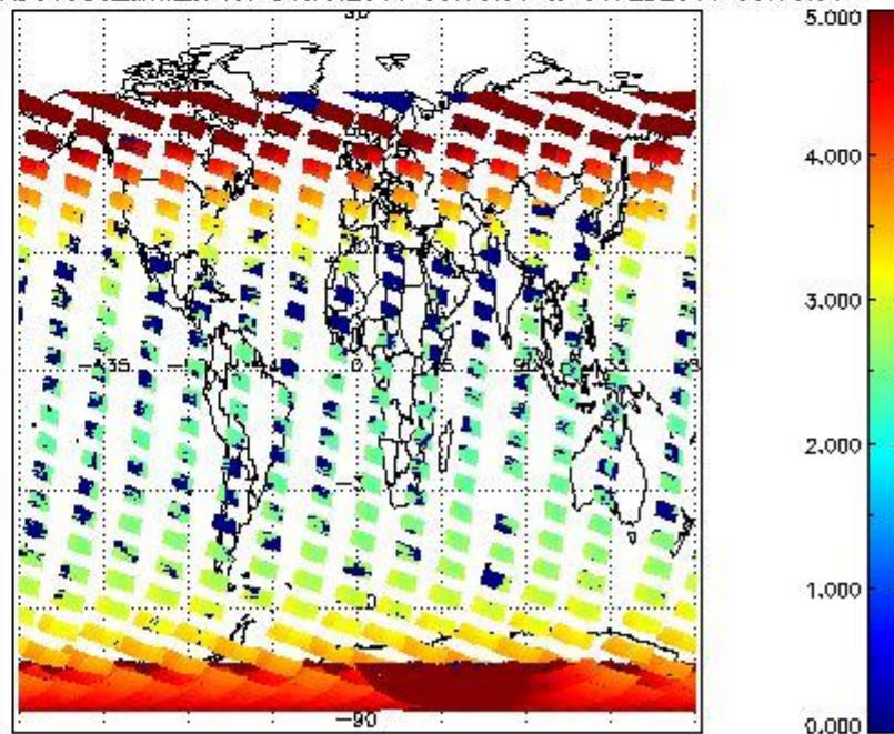
SCIOL2P_NADUV003_amf_cl for 31JAN2011 00:00:00 to 01FEB2011 00:00:00
