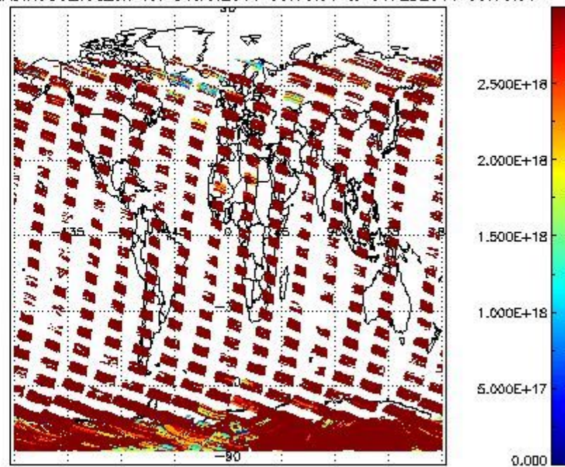
SCIDL2P_NADIR3CO_vcd_err for 31JAN2011 00:00:00 to 01FEB2011 00:00:00
