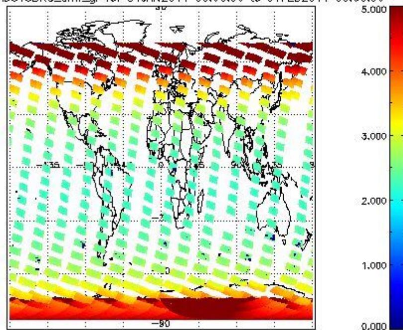
SCIOL2P_NADUV3BRO_amf_gr for 31JAN2011 00:00:00 to 01FEB2011 00:00:00
