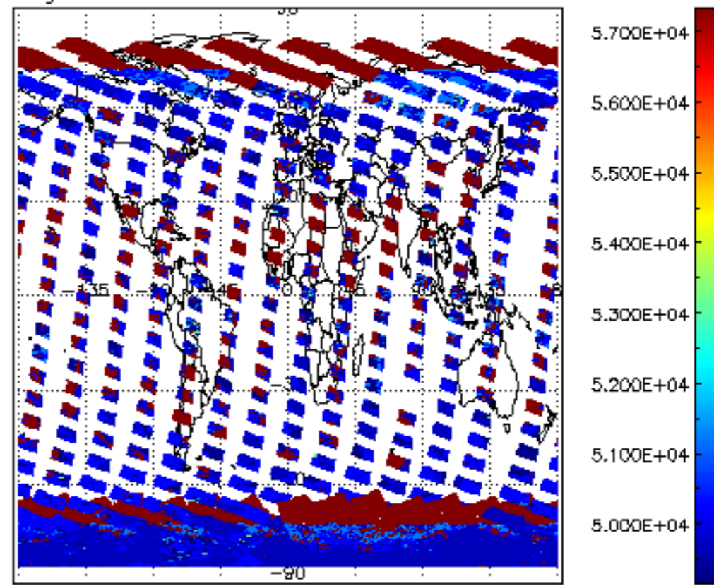
cloud_flags for 31JAN2011 00:00:00 to 01FEB2011 00:00:00
