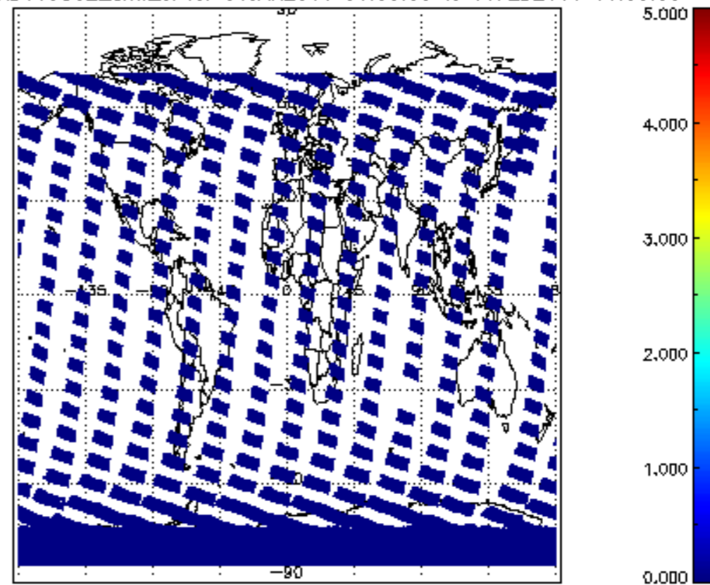
SCIOL2P_NADUV5S02_amf_cl for 31JAN2011 00:00:00 to 01FEB2011 00:00:00
