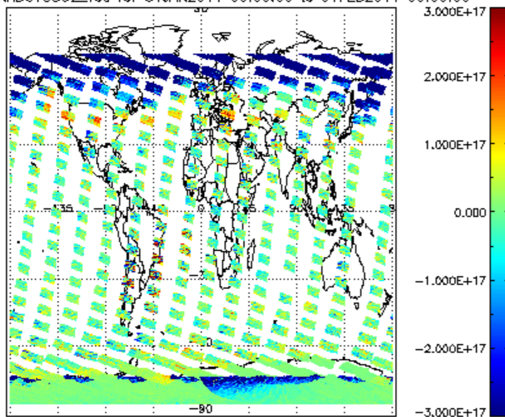
SCIOL2P_NADUV5S02_vcd for 31JAN2011 00:00:00 to 01FEB2011 00:00:00
