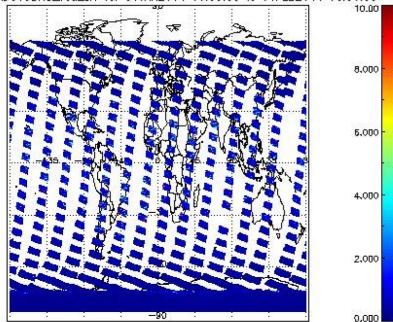
SCIOL2P_NADUV3BRO_vcd_err for 31JAN2011 00:00:00 to 01FEB2011 00:00:00
