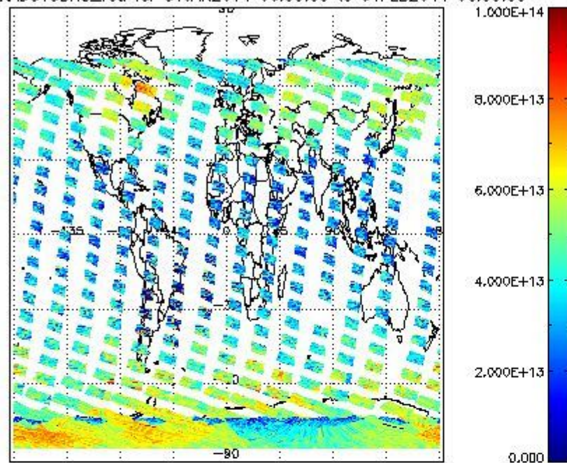
SCIOL2P_NADUV3BRO_vcd for 31JAN2011 00:00:00 to 01FEB2011 00:00:00
