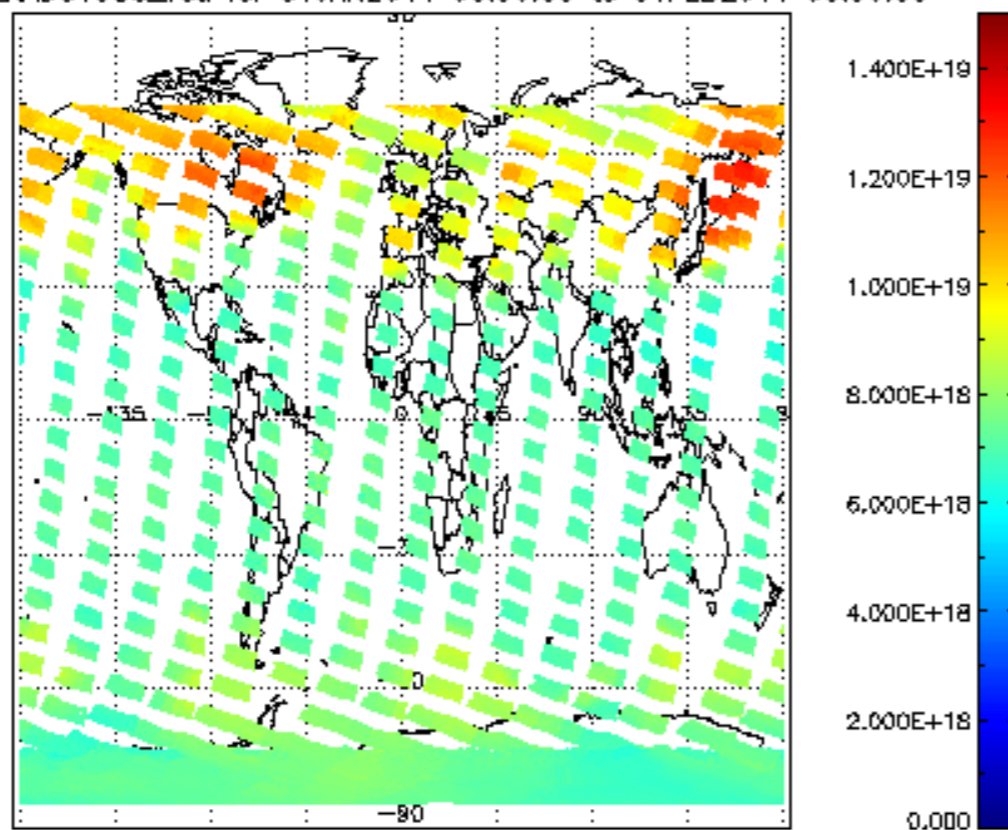
SCIOL2P_NADUV003_vcd for 31JAN2011 00:00:00 to 01FEB2011 00:00:00
