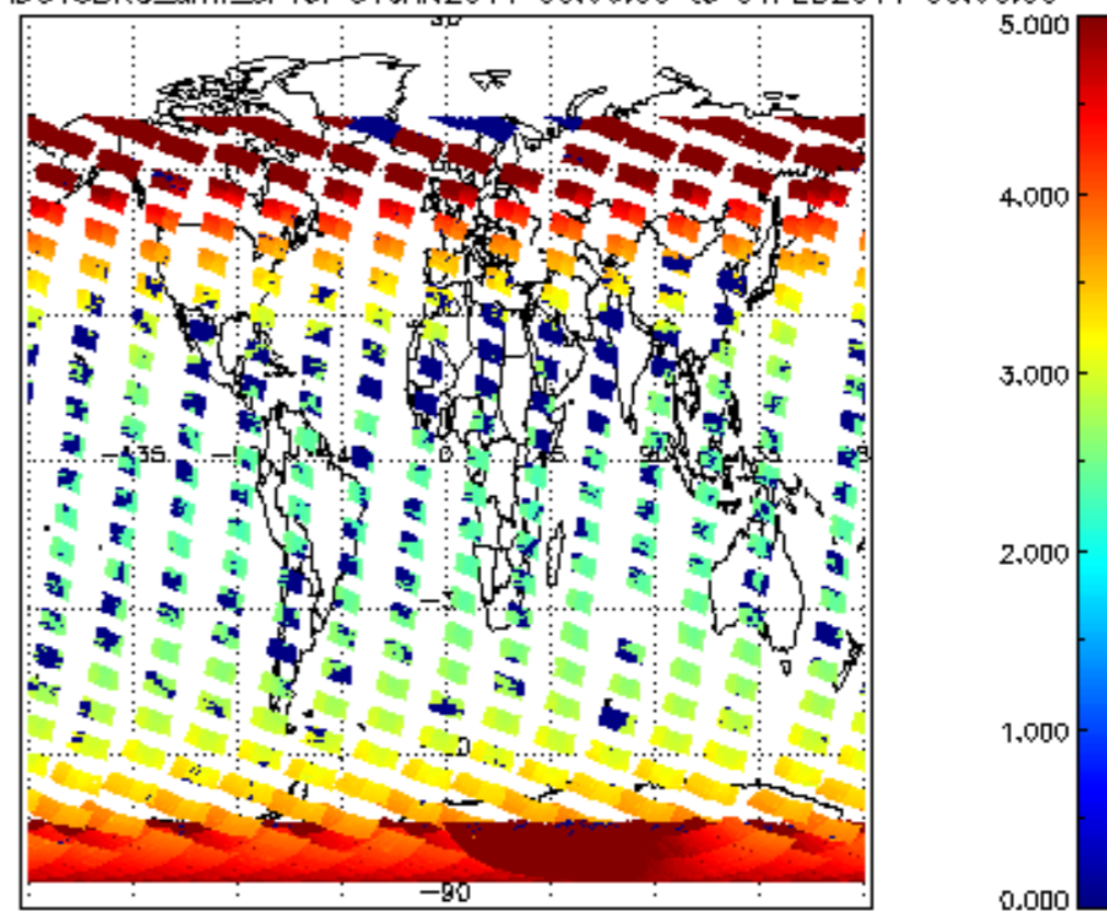
SCIOL2P_NADUV3BRO_amf_sl for 31JAN2011 00:00:00 to 01FEB2011 00:00:00
