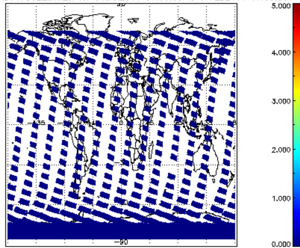
SCIOL2P_NADUV7S02_amf_cl for 31JAN2011 00:00:00 to 01FEB2011 00:00:00
