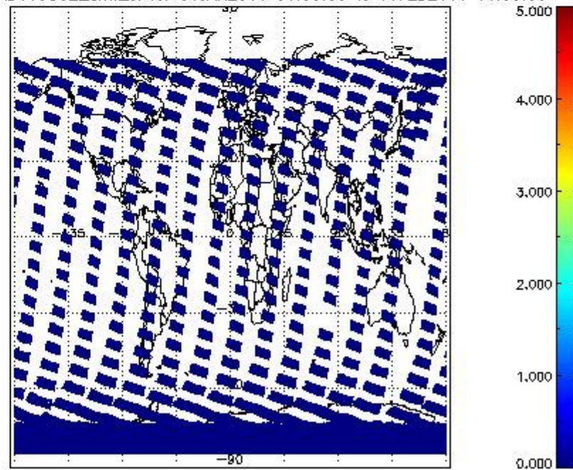
SCIOL2P_NADUV5S02_amf_cl for 31JAN2011 00:00:00 to 01FEB2011 00:00:00
