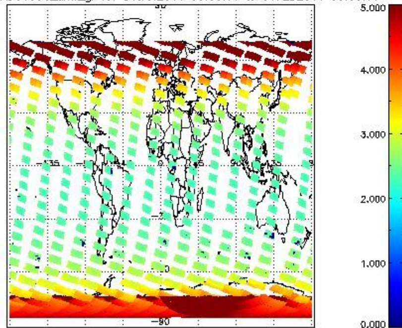
SCIOL2P_NADUV003_amf_gr for 31JAN2011 00:00:00 to 01FEB2011 00:00:00
