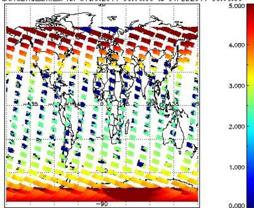
SCIOL2P_NADUV3BRO_amf_cl for 31JAN2011 00:00:00 to 01FEB2011 00:00:00
