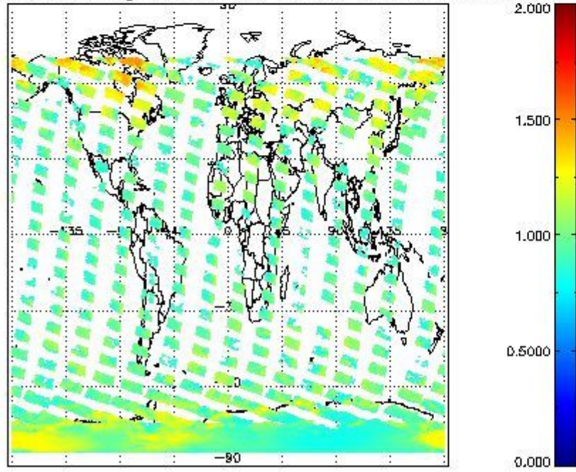
SCIOL2P_NADUV8H2O_amf_gr for 31JAN2011 00:00:00 to 01FEB2011 00:00:00
