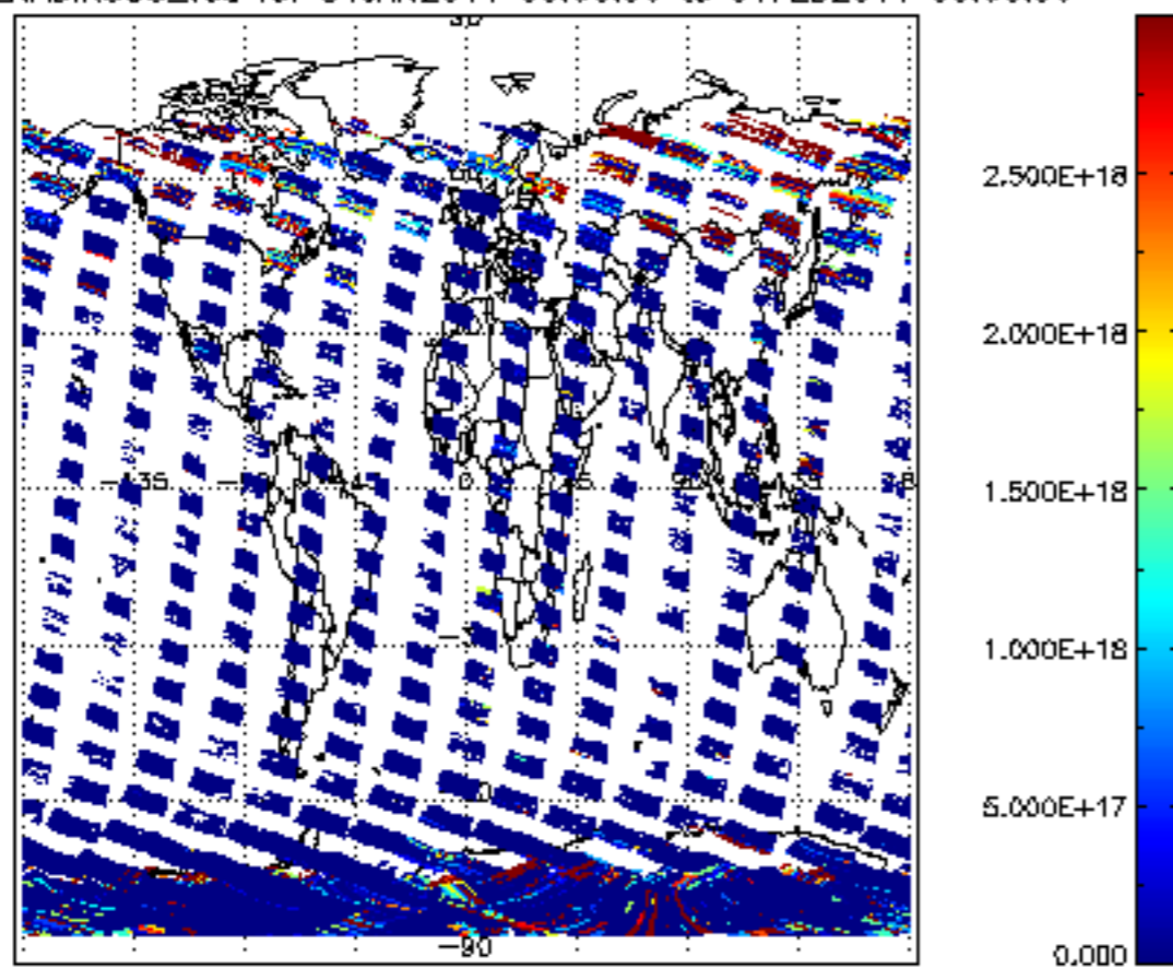
SCIOL2P_NADIR3CO_vcd for 31JAN2011 00:00:00 to 01FEB2011 00:00:00
