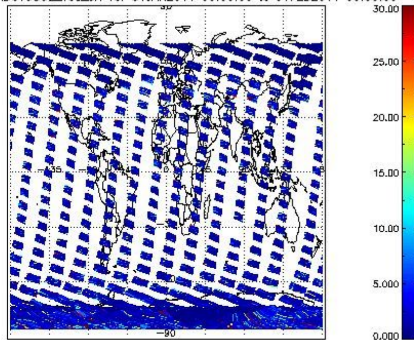
SCIOL2P_NADUV5S02_vcd_err for 31JAN2011 00:00:00 to 01FEB2011 00:00:00
