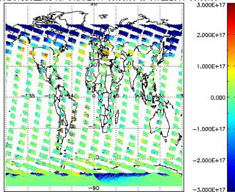
SCIOL2P_NADUV5S02_vcd for 31JAN2011 00:00:00 to 01FEB2011 00:00:00
