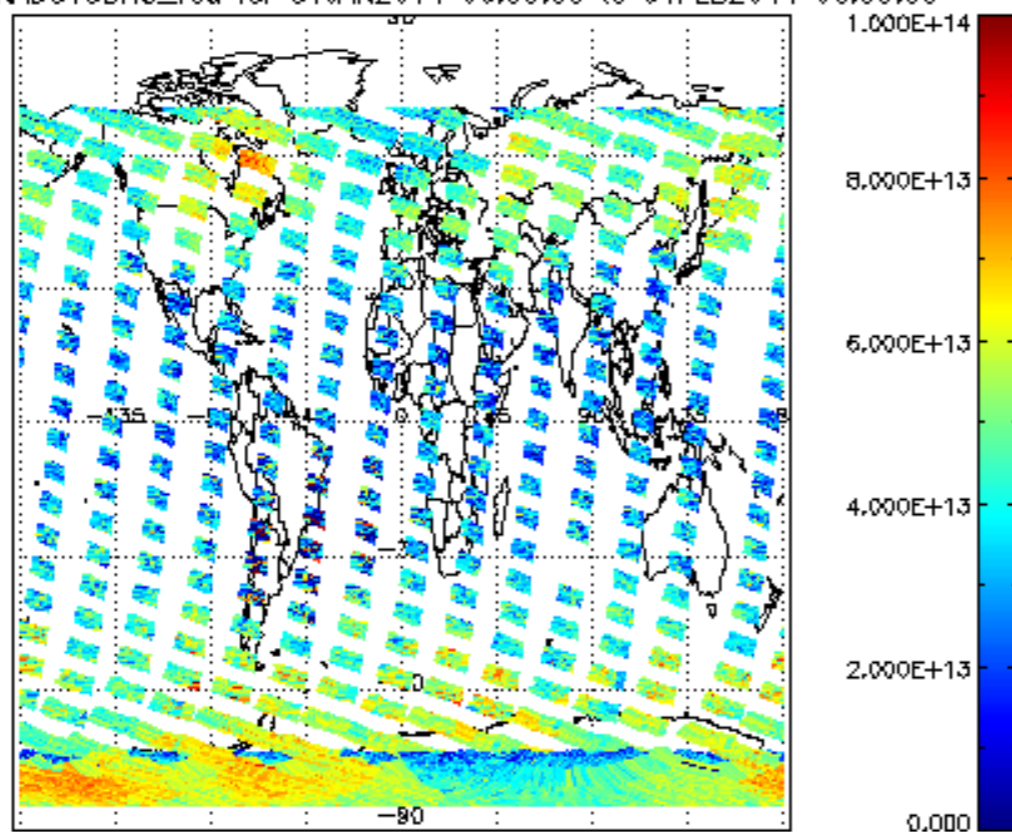
SCIOL2P_NADUV3BRO_vcd for 31JAN2011 00:00:00 to 01FEB2011 00:00:00
