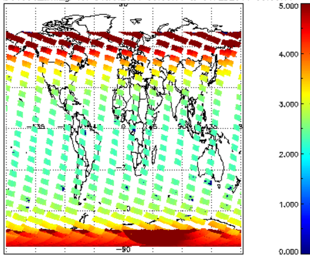
SCIOL2P_NADUV003_amf_gr for 31JAN2011 00:00:00 to 01FEB2011 00:00:00
