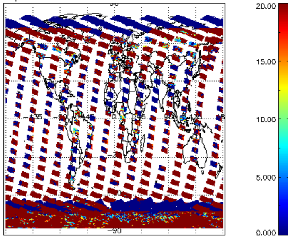
cl_opt_depth for 31JAN2011 00:00:00 to 01FEB2011 00:00:00
