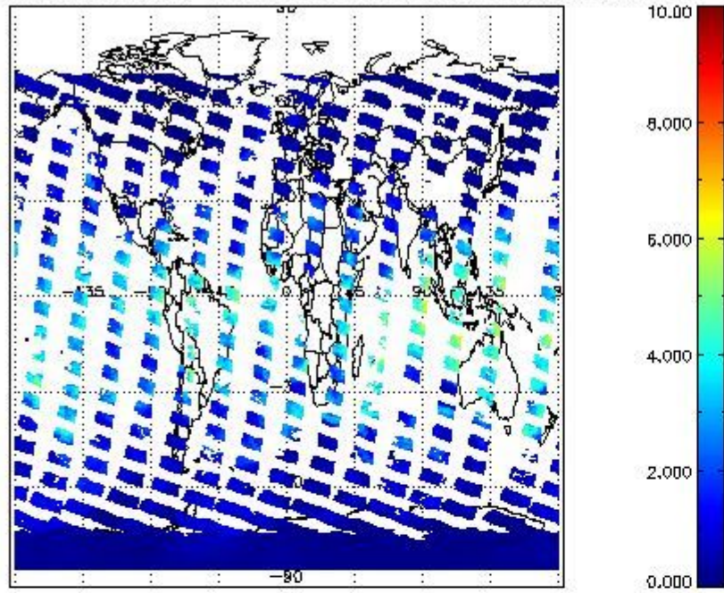
SCIOL2P_NADUV8H2O_vcd for 31JAN2011 00:00:00 to 01FEB2011 00:00:00
