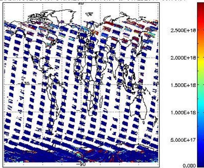
SCIDL2P_NADIR3CO_vcd for 31JAN2011 00:00:00 to 01FEB2011 00:00:00
