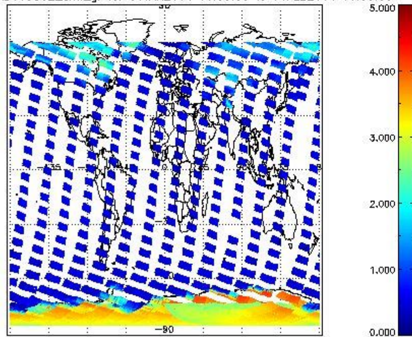
SCIOL2P_NADUV5S02_amf_gr for 31JAN2011 00:00:00 to 01FEB2011 00:00:00
