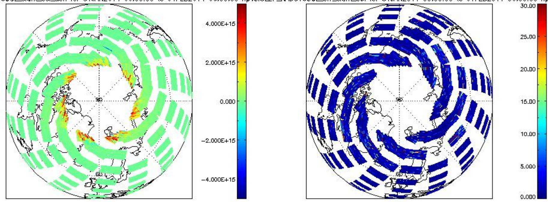
CIOL2P_NADUV60CLslant_col_den for 31JAN2011 00:00:00 to 01FEB2011 00:00:00 np; CIOL2P_NADUV60CLarr_slant_col for 31JAN2011 00:00:00 to 01FEB2011 00:00:00 np
