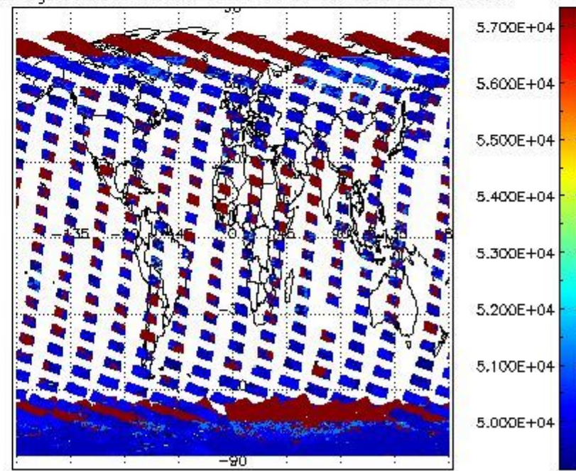
cloud_flags for 31JAN2011 00:00:00 to 01FEB2011 00:00:00
