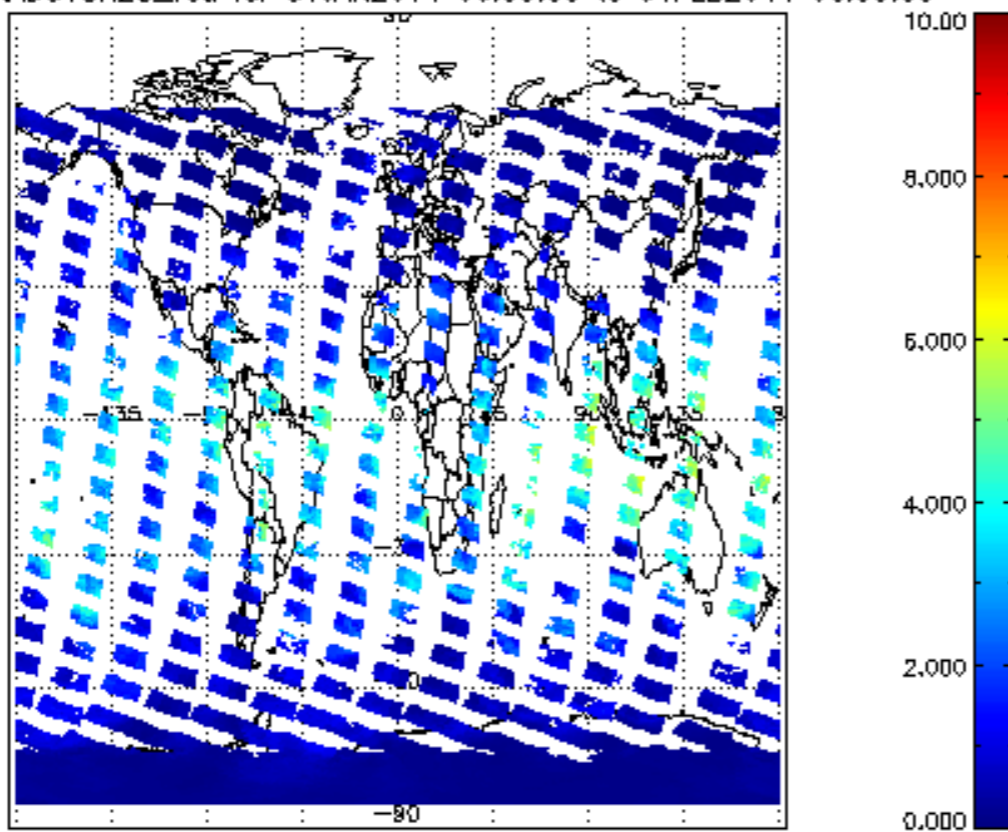
SCIOL2P_NADUV8H20_vcd for 31JAN2011 00:00:00 to 01FEB2011 00:00:00
