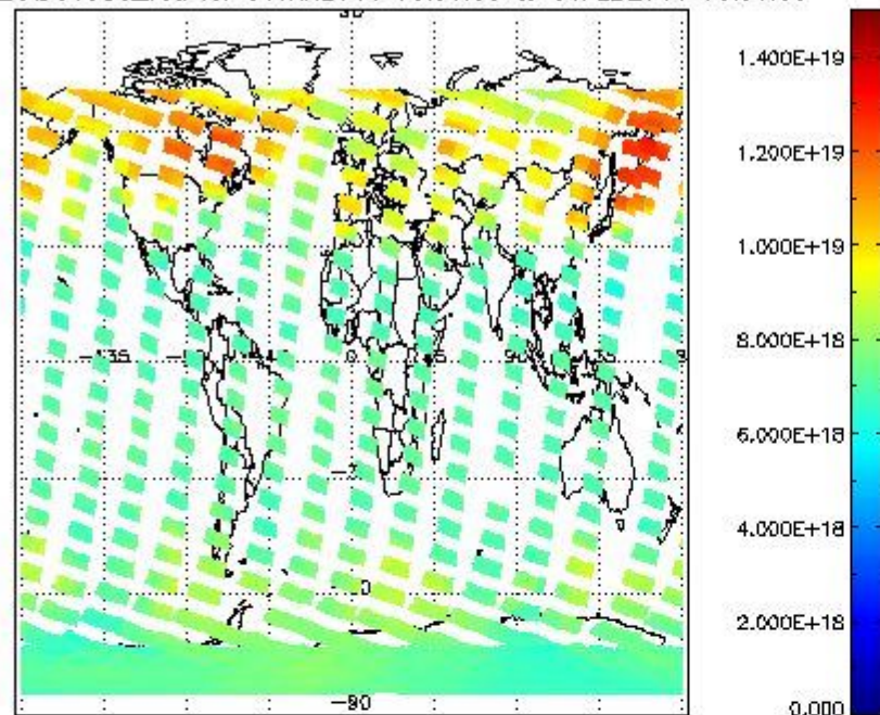
SCIOL2P_NADUV003_vcd for 31JAN2011 00:00:00 to 01FEB2011 00:00:00
