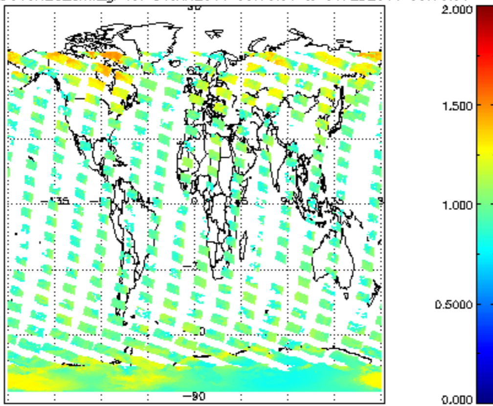
SCIOL2P_NADUV8H20_amf_gr for 31JAN2011 00:00:00 to 01FEB2011 00:00:00
