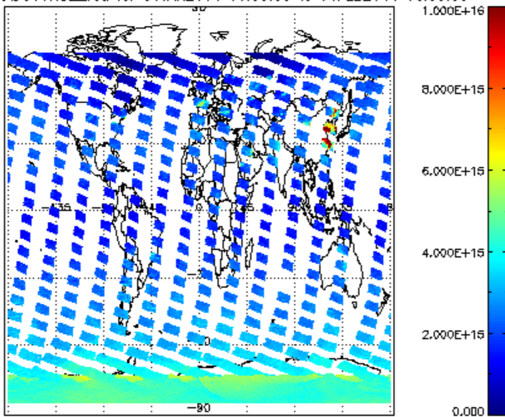
SCIOL2P_NADUV1NO2_vcd for 31JAN2011 00:00:00 to 01FEB2011 00:00:00
