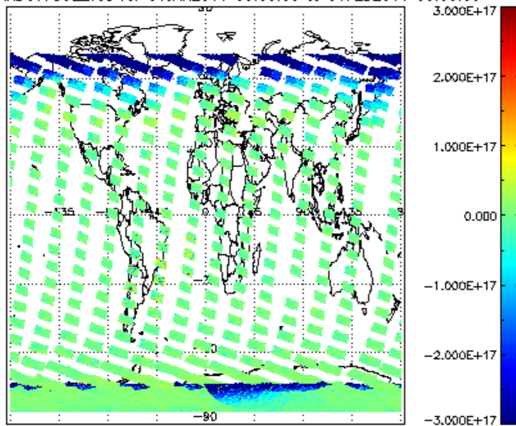
SCIOL2P_NADUV7S02_vcd for 31JAN2011 00:00:00 to 01FEB2011 00:00:00
