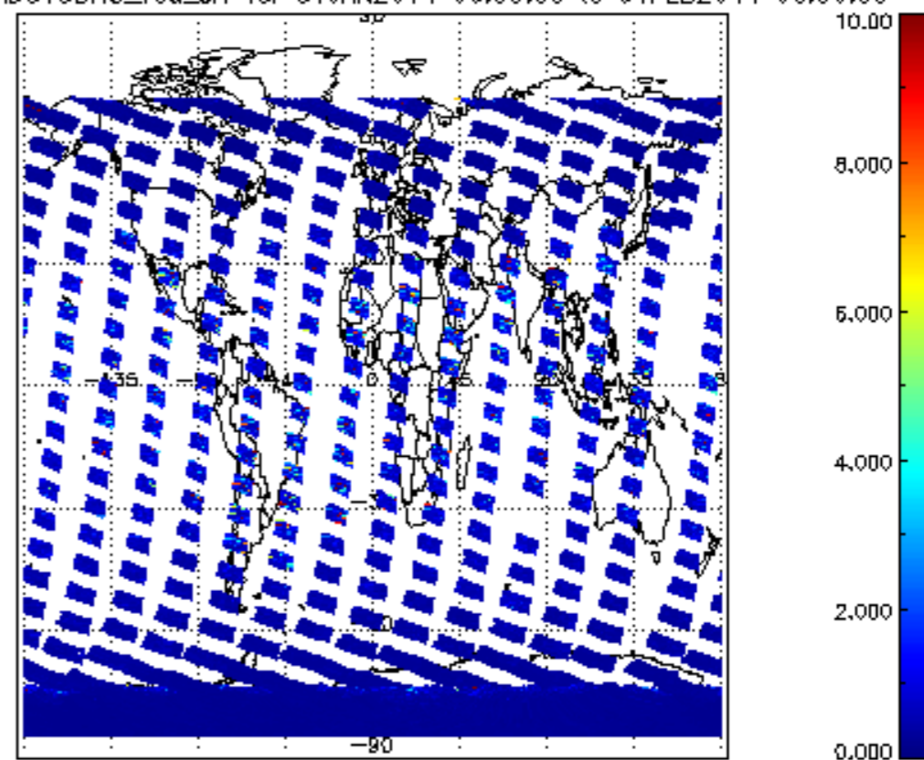
SCIOL2P_NADUV3BRO_vcd_err for 31JAN2011 00:00:00 to 01FEB2011 00:00:00
