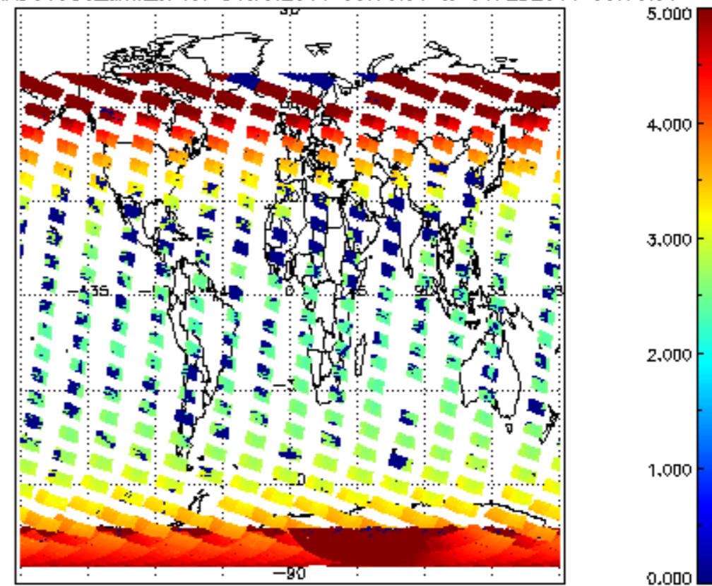
SCIOL2P_NADUV003_amf_cl for 31JAN2011 00:00:00 to 01FEB2011 00:00:00
