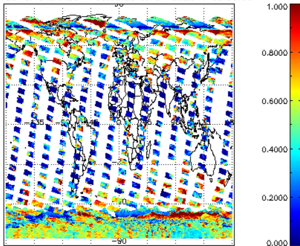
cl_frac for 31JAN2011 00:00:00 to 01FEB2011 00:00:00
