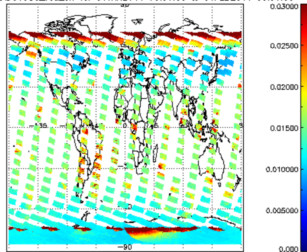
SCIOL2P_NADUV003_vcd_err for 31JAN2011 00:00:00 to 01FEB2011 00:00:00
