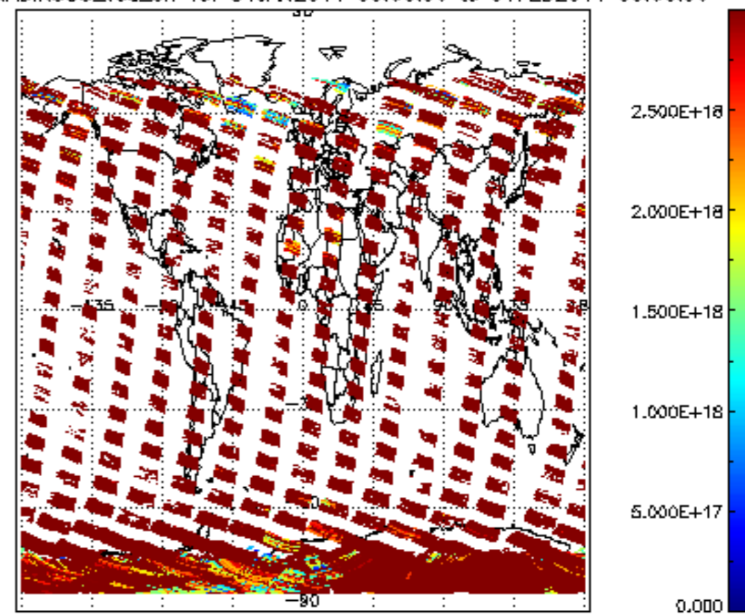
SCIOL2P_NADIR3CO_vcd_err for 31JAN2011 00:00:00 to 01FEB2011 00:00:00
