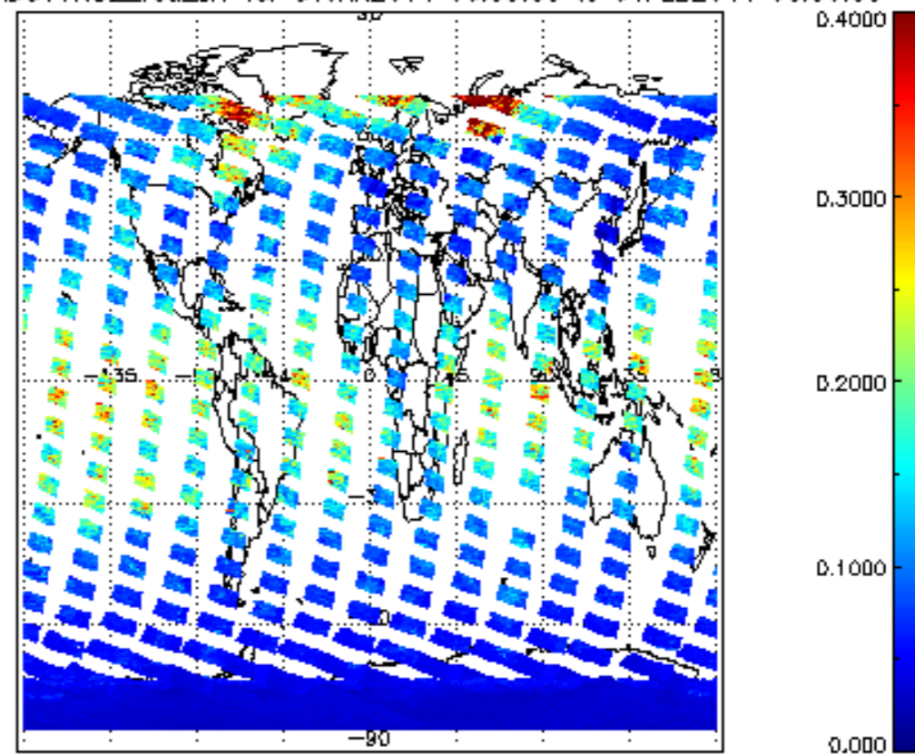
SCIOL2P_NADUV1NO2_vcd_err for 31JAN2011 00:00:00 to 01FEB2011 00:00:00
