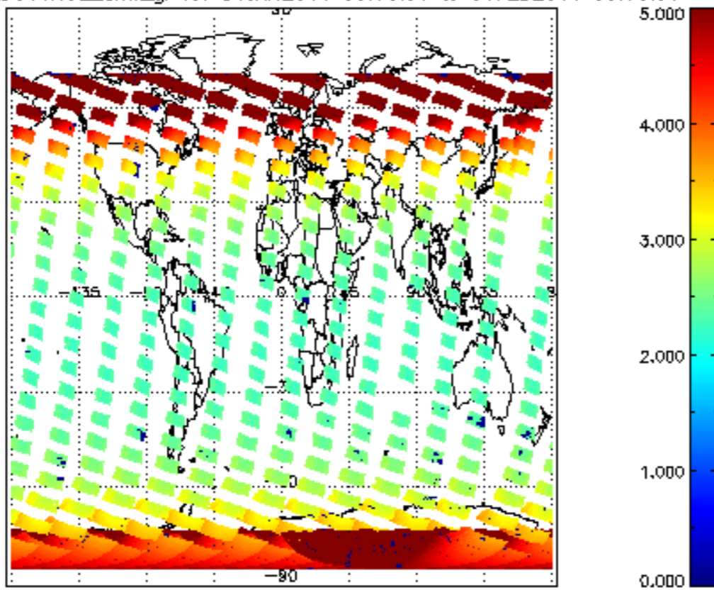
SCIOL2P_NADUV1NO2_amf_gr for 31JAN2011 00:00:00 to 01FEB2011 00:00:00
