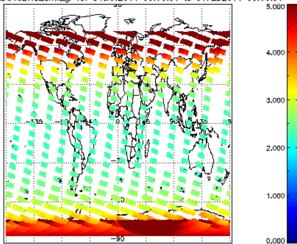
SCIOL2P_NADUV3BRO_amf_gr for 31JAN2011 00:00:00 to 01FEB2011 00:00:00
