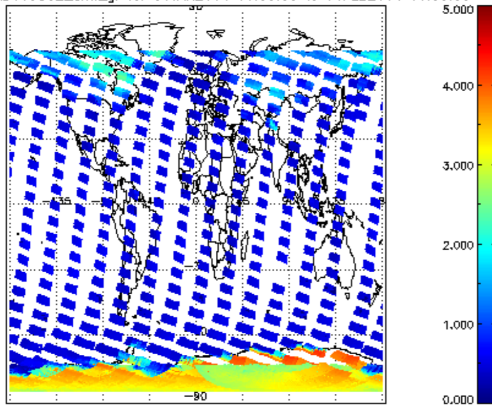
SCIOL2P_NADUV5S02_amf_gr for 31JAN2011 00:00:00 to 01FEB2011 00:00:00
