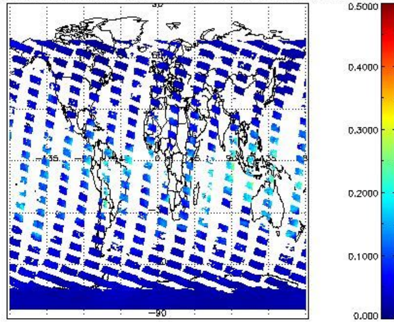
SCIOL2P_NADUV8H2O_vcd_err for 31JAN2011 00:00:00 to 01FEB2011 00:00:00
