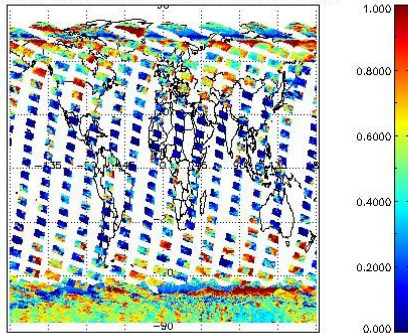
cL_frac for 31JAN2011 00:00:00 to 01FEB2011 00:00:00
