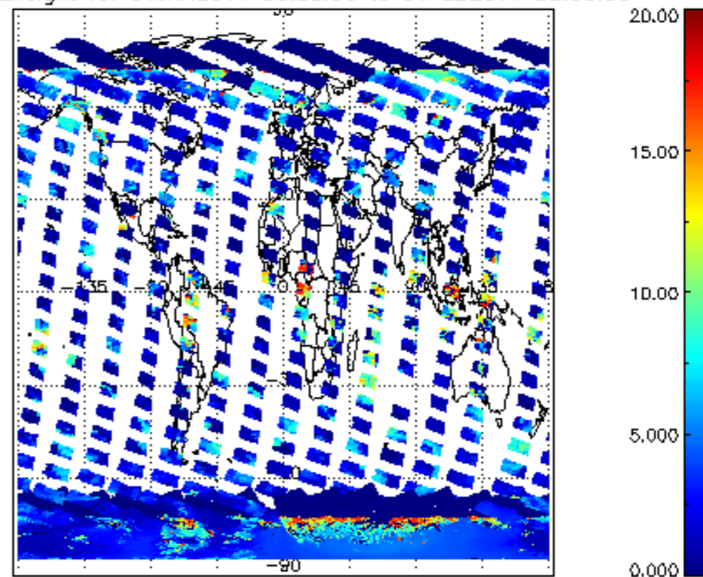
cl_top_height for 31JAN2011 00:00:00 to 01FEB2011 00:00:00
