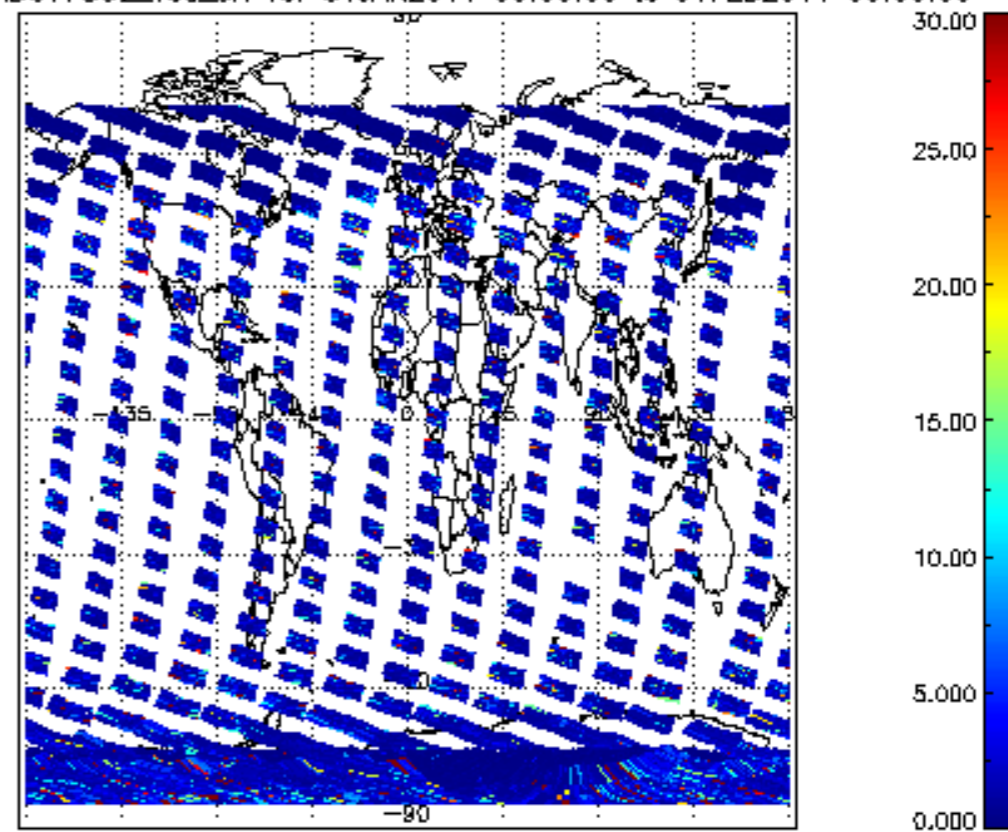
SCIOL2P_NADUV7S02_vcd_err for 31JAN2011 00:00:00 to 01FEB2011 00:00:00
