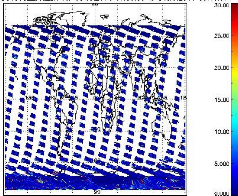
SCIOL2P_NADUV5SO2_vcd_err for 30JAN2011 00:00:00 to 31JAN2011 00:00:00
