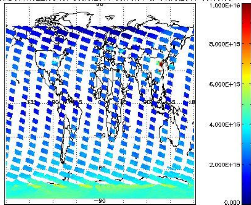
SCIOL2P_NADUV1NO2_vcd for 30JAN2011 00:00:00 to 31JAN2011 00:00:00
