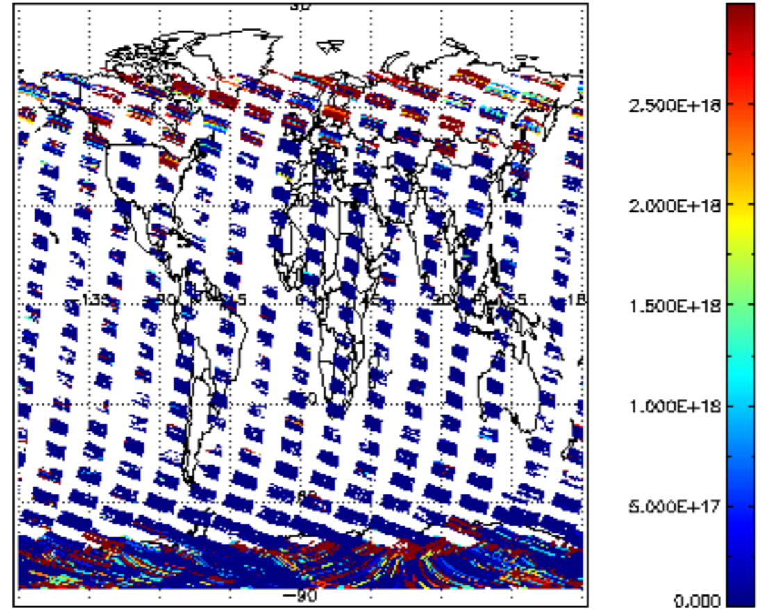
SCIOL2P_NADIR3CO_vcd for 30JAN2011 00:00:00 to 31JAN2011 00:00:00
