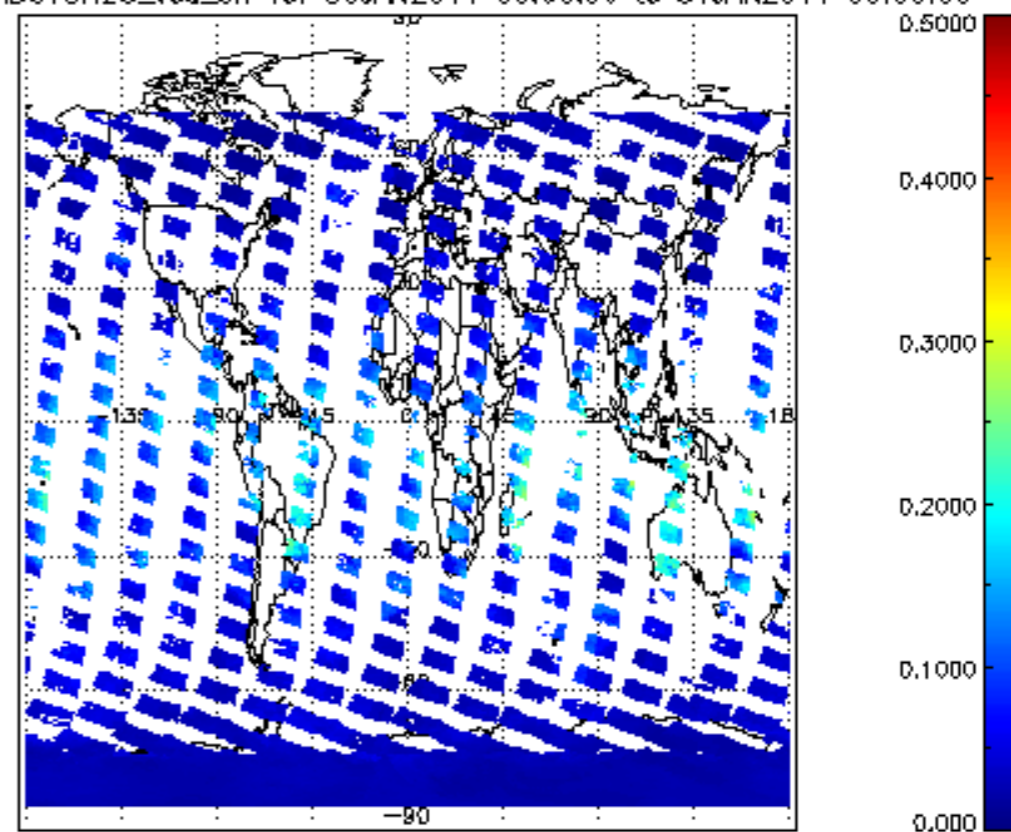
SCIOL2P_NADUVBH20_vcd_err for 30JAN2011 00:00:00 to 31JAN2011 00:00:00
