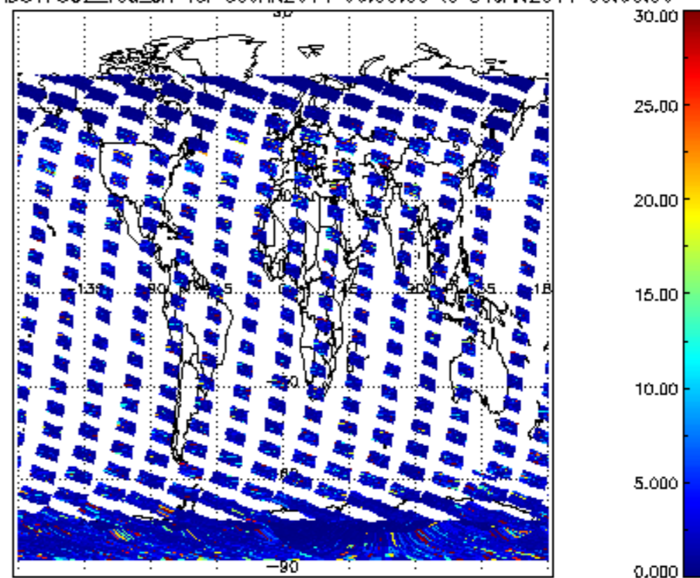
SCIOL2P_NADUV7S02_vcd_err for 30JAN2011 00:00:00 to 31JAN2011 00:00:00
