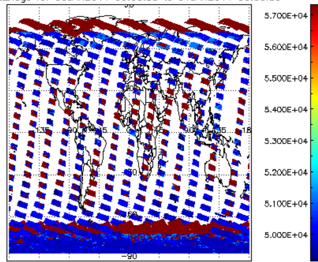
cloud_flags for 30JAN2011 00:00:00 to 31JAN2011 00:00:00
