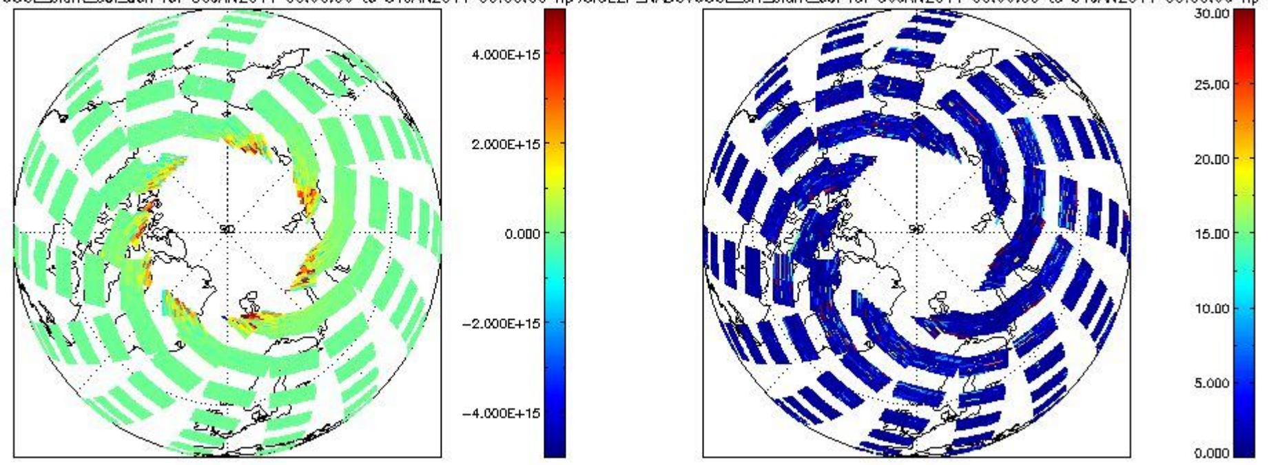
SCIOI2P_NADUV60CL_slant_col_den for 30JAN2011 00:00:00 to 31JAN2011 00:00:00 np; SCIOI2P_NADUV60CL_err_slant_col for 30JAN2011 00:00:00 to 31JAN2011 00:00:00 np
