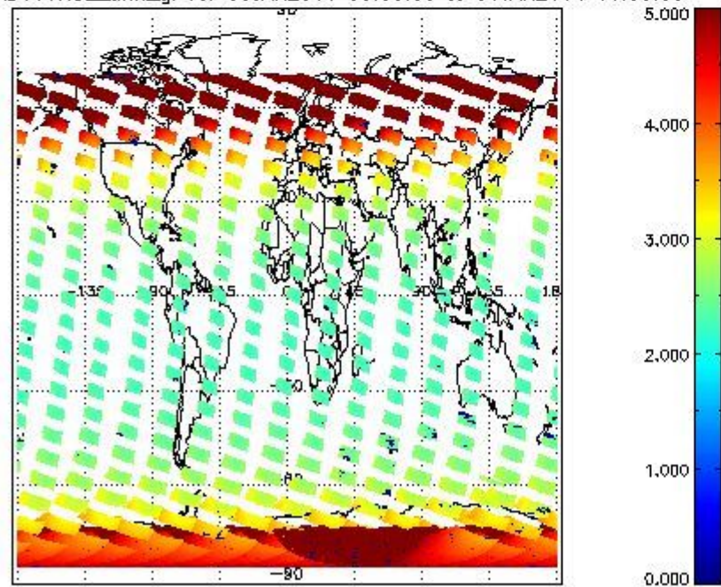
SCIOL2P_NADUV1NO2_amf_gr for 30JAN2011 00:00:00 to 31JAN2011 00:00:00
