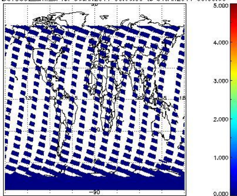
SCIOL2P_NADUV5SO2_amf_cl for 30JAN2011 00:00:00 to 31JAN2011 00:00:00
