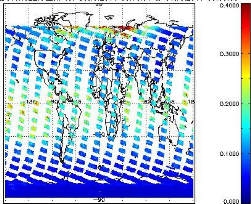
SCIOL2P_NADUV1NO2_vcd_err for 30JAN2011 00:00:00 to 31JAN2011 00:00:00
