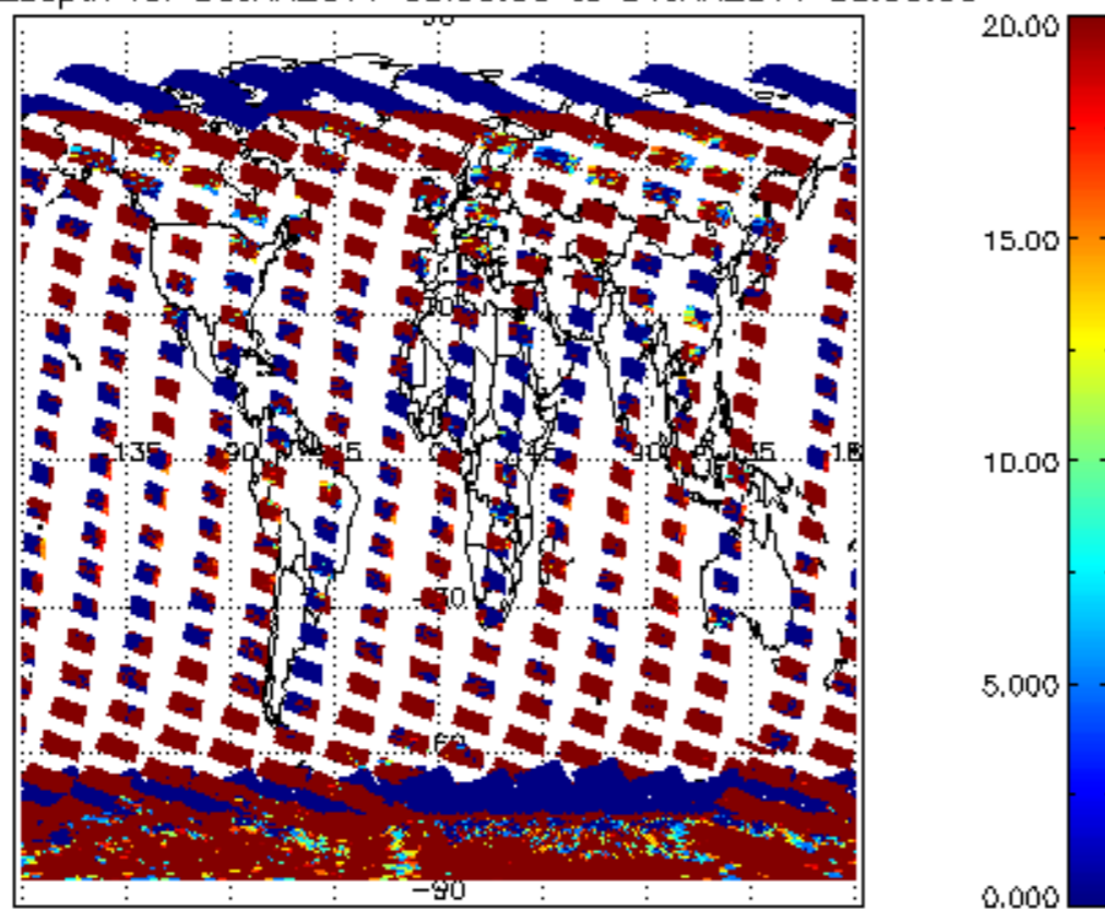
cLopt_depth for 30JAN2011 00:00:00 to 31JAN2011 00:00:00
