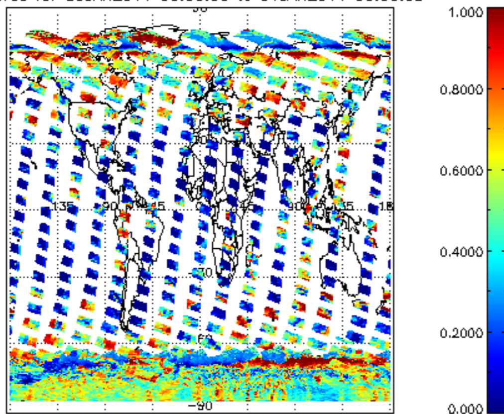
cL_frac for 30JAN2011 00:00:00 to 31JAN2011 00:00:00
