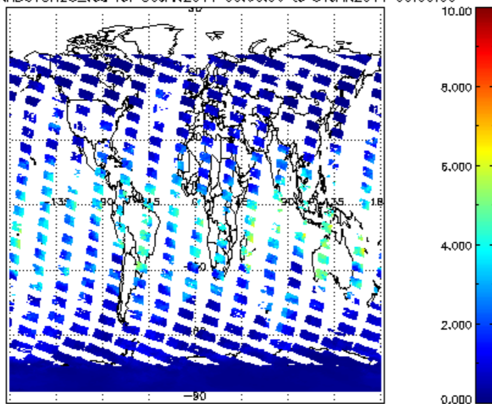
SCIOL2P_NADUVBH20_vcd for 30JAN2011 00:00:00 to 31JAN2011 00:00:00
