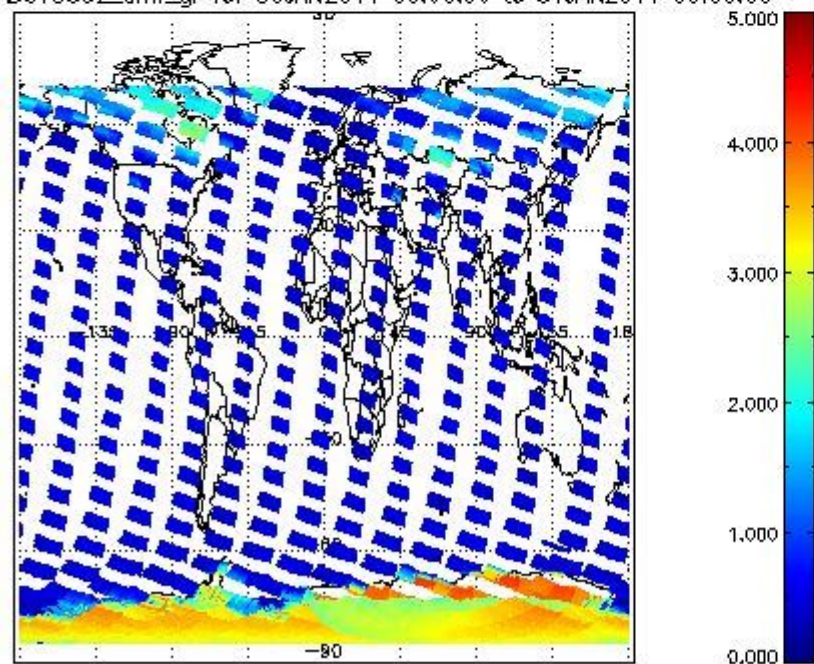
SCIOL2P_NADUV5SO2_amf_gr for 30JAN2011 00:00:00 to 31JAN2011 00:00:00
