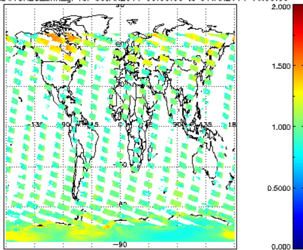
SCIOL2P_NADUVBH20_amf_gr for 30JAN2011 00:00:00 to 31JAN2011 00:00:00
