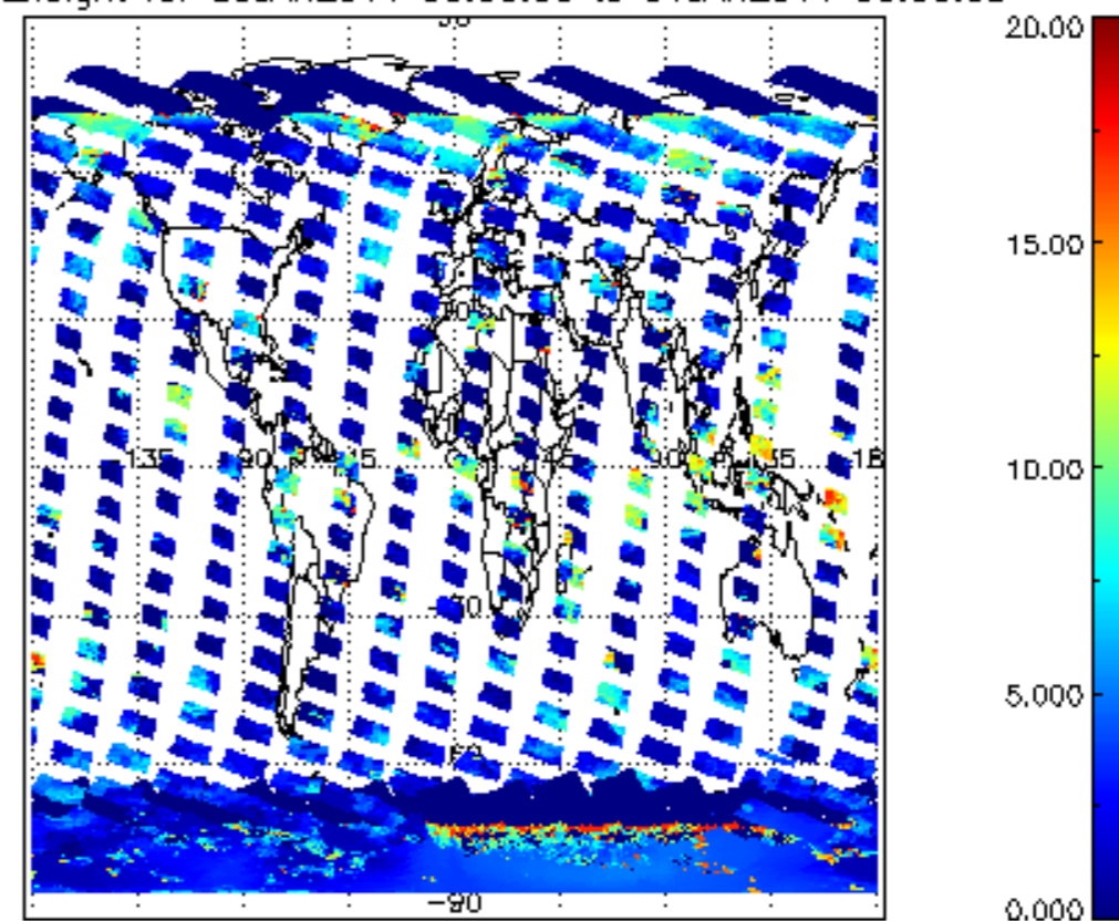
cL_top_height for 30JAN2011 00:00:00 to 31JAN2011 00:00:00
