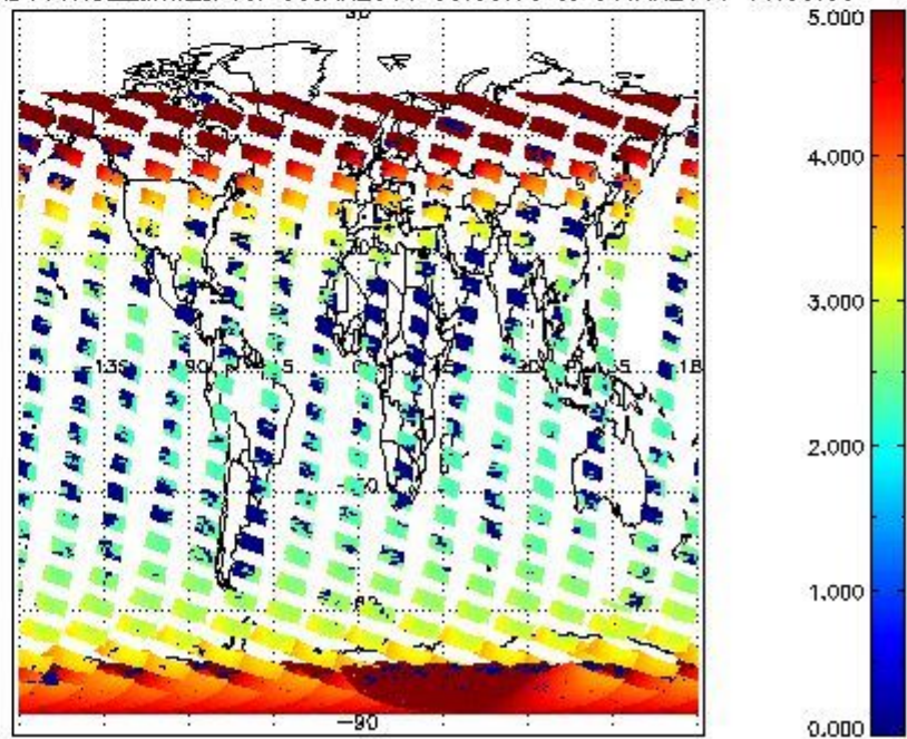
SCIOL2P_NADUV1NO2_amf_cl for 30JAN2011 00:00:00 to 31JAN2011 00:00:00
