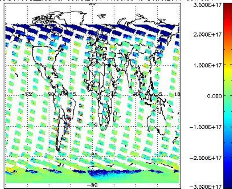
SCIOL2P_NADUV5SO2_vcd for 30JAN2011 00:00:00 to 31JAN2011 00:00:00
