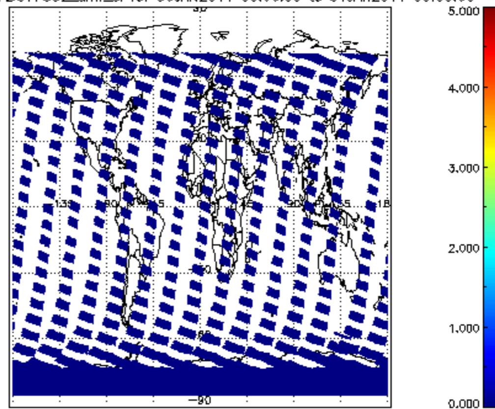
SCIOL2P_NADUV7S02_amf_sl for 30JAN2011 00:00:00 to 31JAN2011 00:00:00
