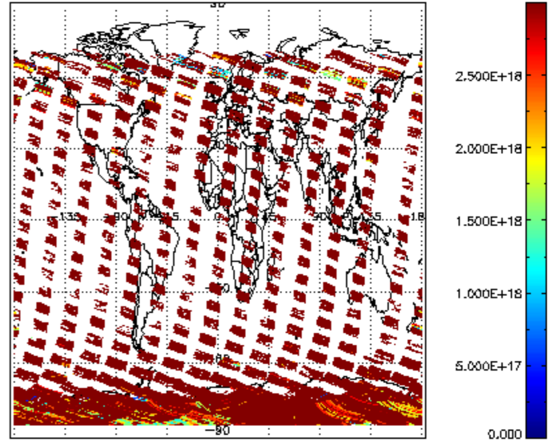
SCIOL2P_NADIR3CO_vcd_err for 30JAN2011 00:00:00 to 31JAN2011 00:00:00
