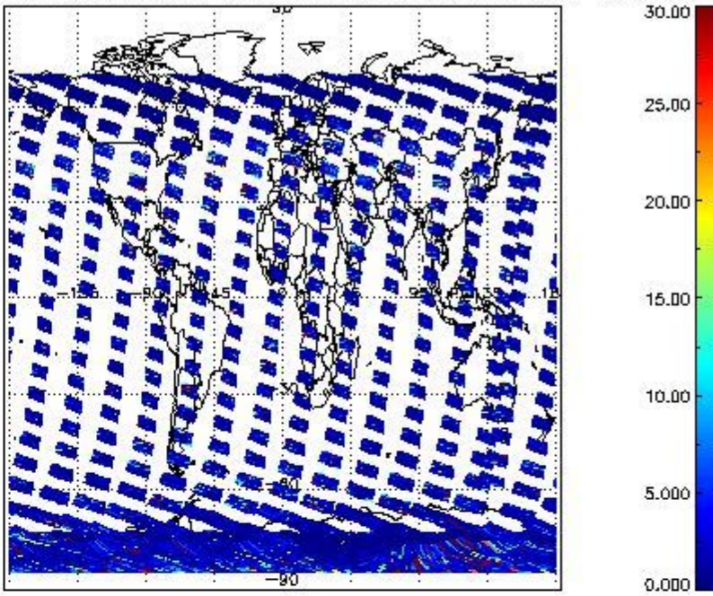
SCIOL2P_NADUV5SO2_vcd_err for 29JAN2011 00:00:00 to 30JAN2011 00:00:00
