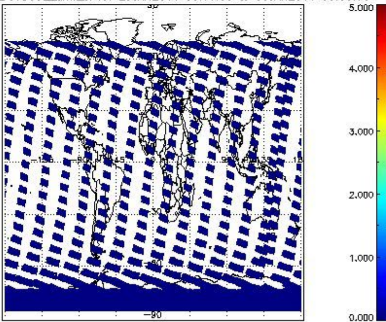
SCIOL2P_NADUV5SO2_amf_cl for 29JAN2011 00:00:00 to 30JAN2011 00:00:00
