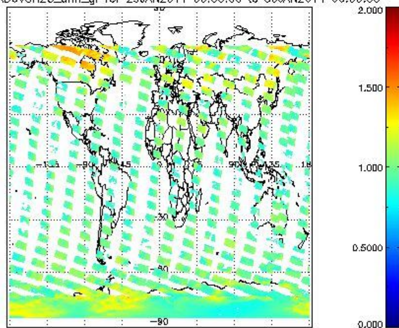
SCIOL2P_NADUV8H20_amf_gr for 29JAN2011 00:00:00 to 30JAN2011 00:00:00
