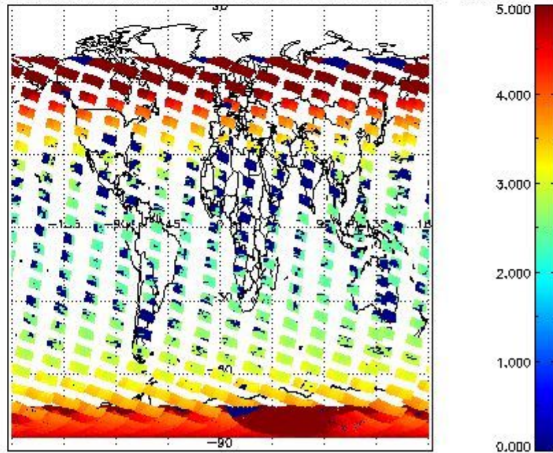
SCIOL2P_NADUV3BRO_amf_cl for 29JAN2011 00:00:00 to 30JAN2011 00:00:00
