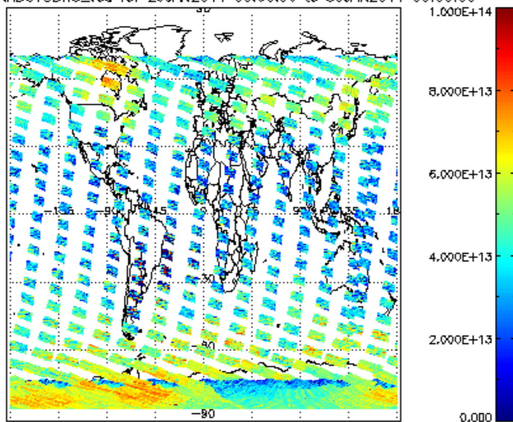
SCIOL2P_NADUV3BRO_vcd for 29JAN2011 00:00:00 to 30JAN2011 00:00:00
