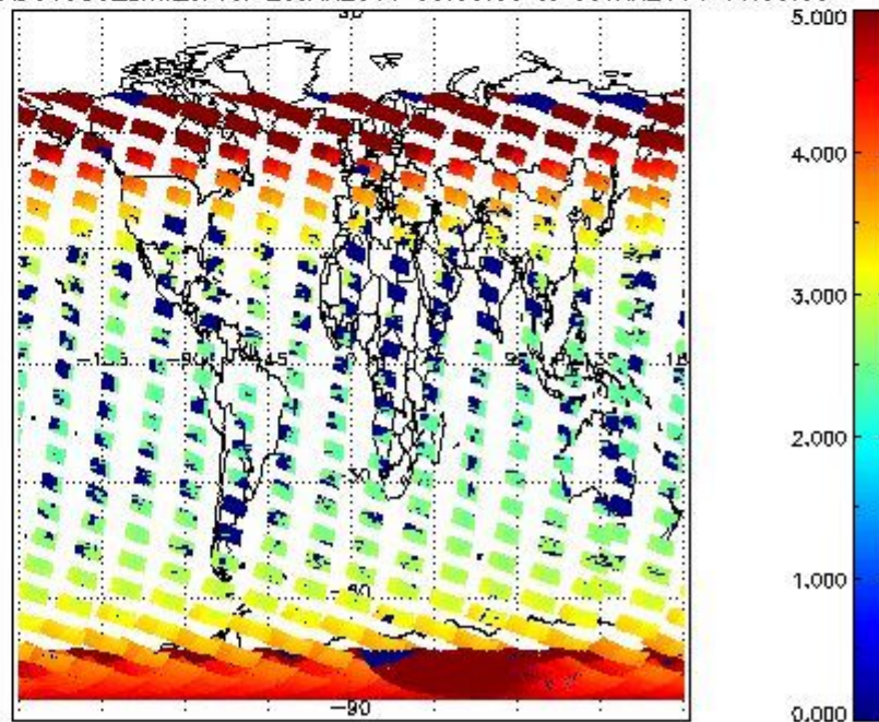
SCIOL2P_NADUV003_amf_cl for 29JAN2011 00:00:00 to 30JAN2011 00:00:00
