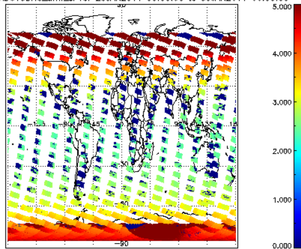
SCIOL2P_NADUV3BRO_amf_cl for 29JAN2011 00:00:00 to 30JAN2011 00:00:00
