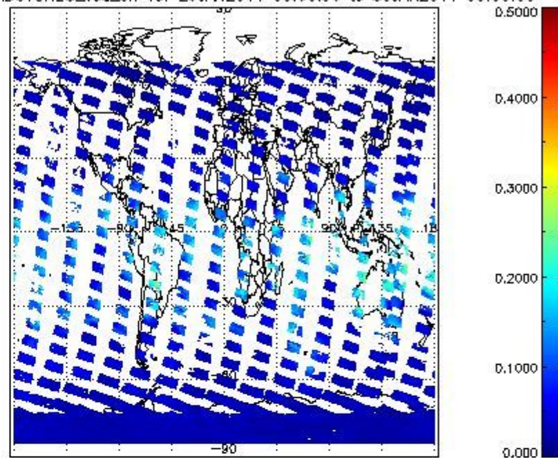
SCIOL2P_NADUV8H20_vcd_err for 29JAN2011 00:00:00 to 30JAN2011 00:00:00
