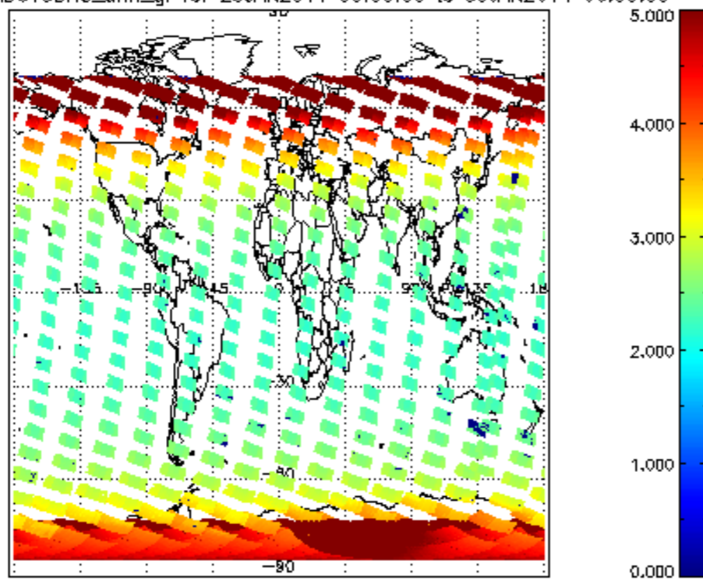
SCIOL2P_NADUV3BRO_amf_gr for 29JAN2011 00:00:00 to 30JAN2011 00:00:00
