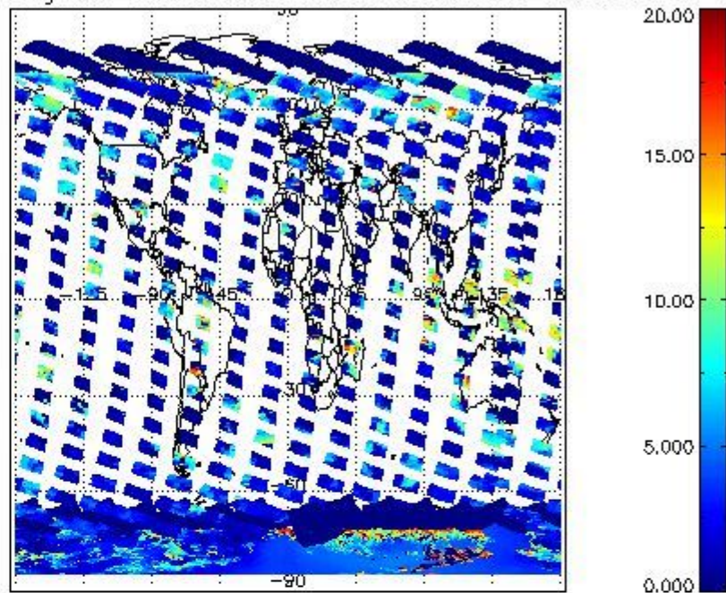
cL_top_height for 29JAN2011 00:00:00 to 30JAN2011 00:00:00
