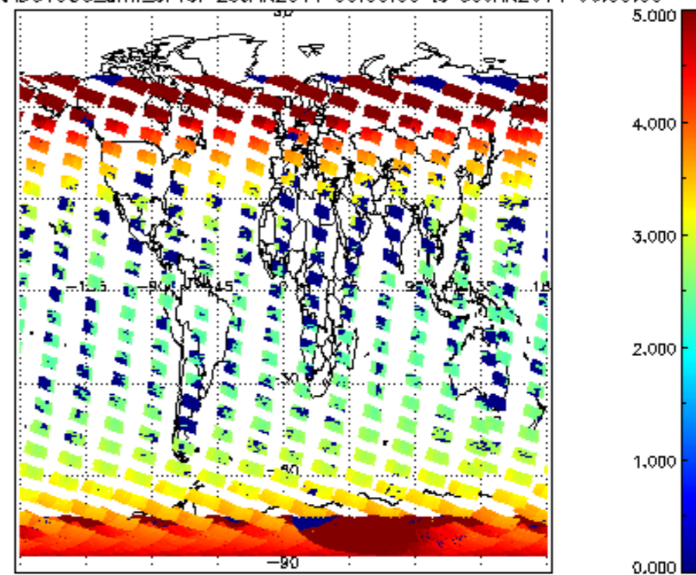
SCIOL2P_NADUV003_amf_cl for 29JAN2011 00:00:00 to 30JAN2011 00:00:00
