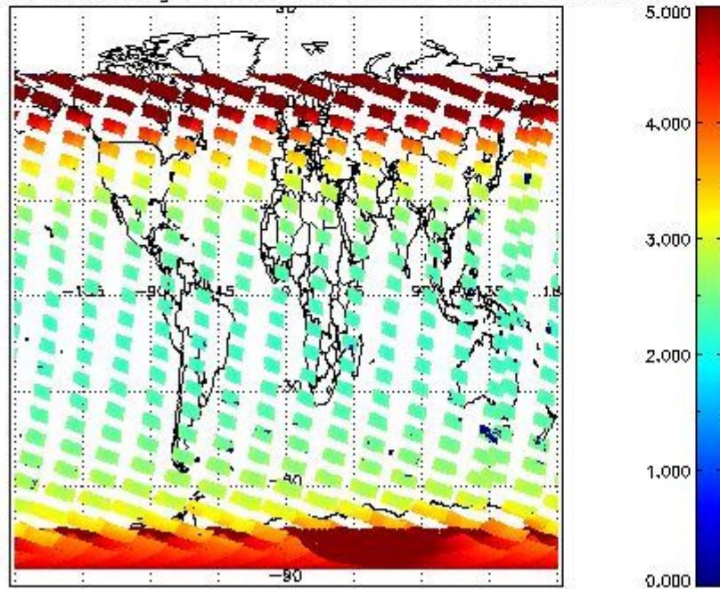
SCIOL2P_NADUV3BRO_amf_gr for 29JAN2011 00:00:00 to 30JAN2011 00:00:00
