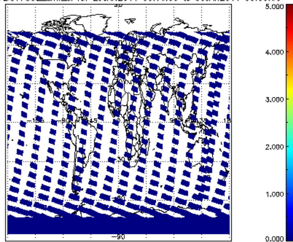
SCIOL2P_NADUV7S02_amf_cl for 29JAN2011 00:00:00 to 30JAN2011 00:00:00
