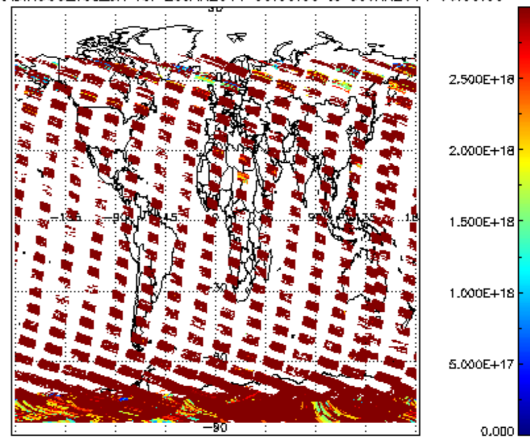
SCIOL2P_NADIR3CO_vcd_err for 29JAN2011 00:00:00 to 30JAN2011 00:00:00
