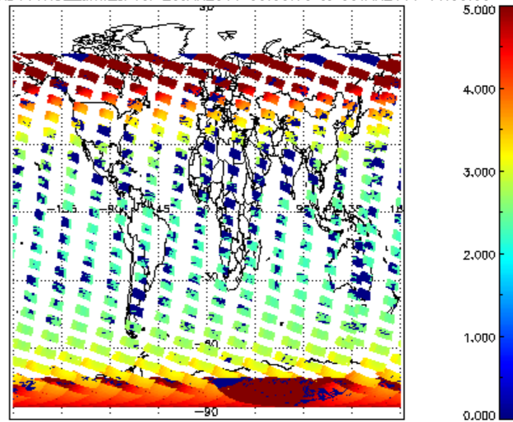
SCIOL2P_NADUV1NO2_amf_cl for 29JAN2011 00:00:00 to 30JAN2011 00:00:00
