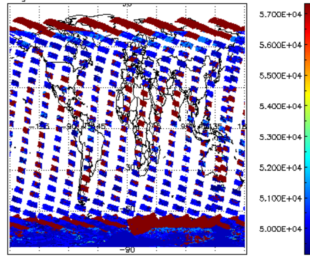
cloud_flags for 29JAN2011 00:00:00 to 30JAN2011 00:00:00
