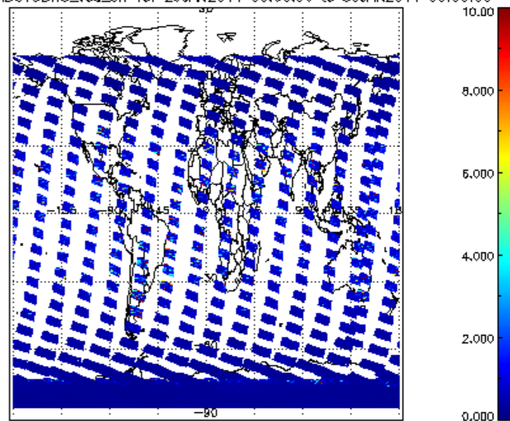
SCIOL2P_NADUV3BRO_vcd_err for 29JAN2011 00:00:00 to 30JAN2011 00:00:00
