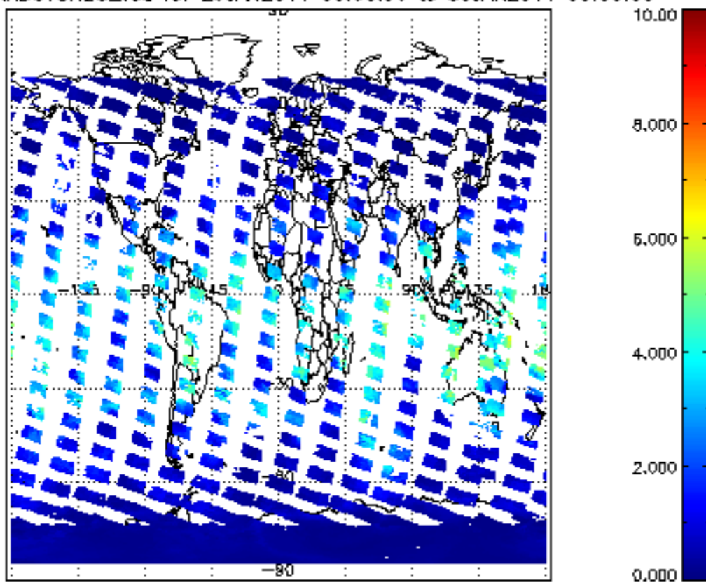
SCIOL2P_NADUVBH20_vcd for 29JAN2011 00:00:00 to 30JAN2011 00:00:00
