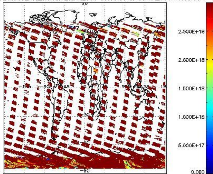
SCIDL2P_NADIR3CO_vcd_err for 29JAN2011 00:00:00 to 30JAN2011 00:00:00
