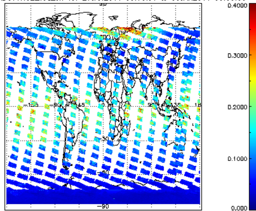
SCIOL2P_NADUV1NO2_vcd_err for 29JAN2011 00:00:00 to 30JAN2011 00:00:00
