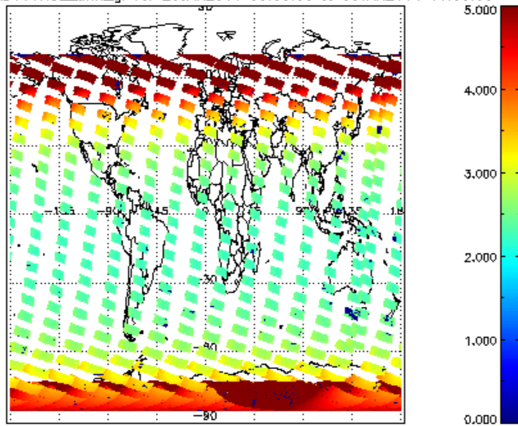
SCIOL2P_NADUV1NO2_amf_gr for 29JAN2011 00:00:00 to 30JAN2011 00:00:00
