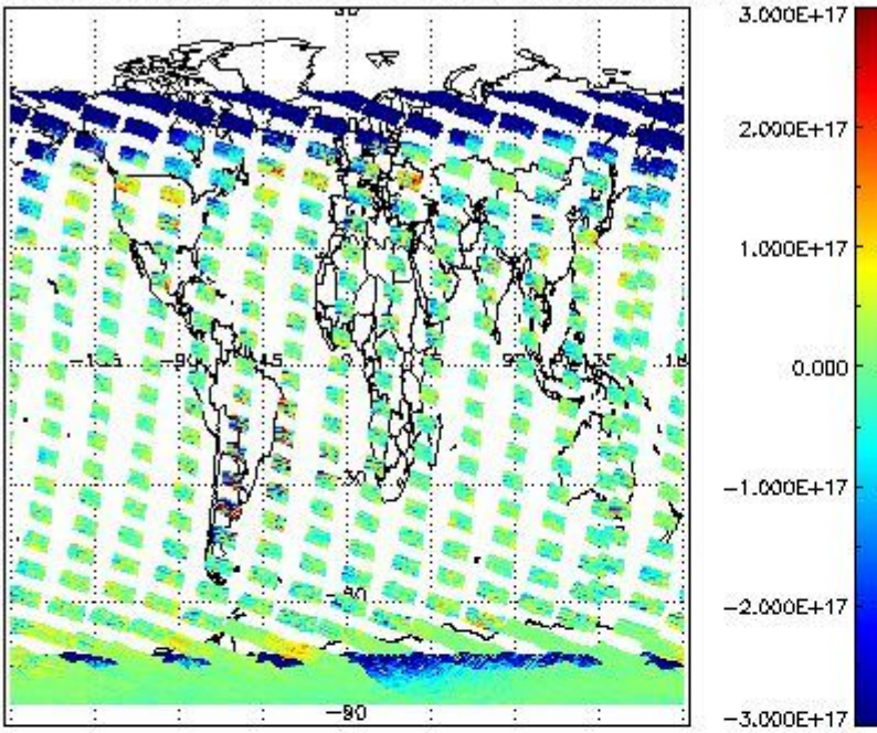
SCIOL2P_NADUV5SO2_vcd for 29JAN2011 00:00:00 to 30JAN2011 00:00:00
