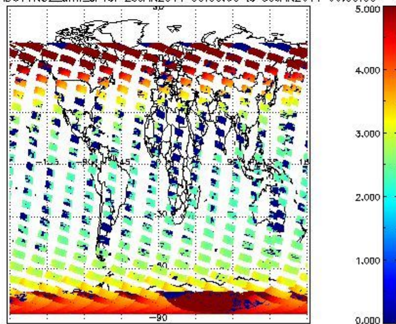
SCIOL2P_NADUV1NO2_amf_cl for 29JAN2011 00:00:00 to 30JAN2011 00:00:00
