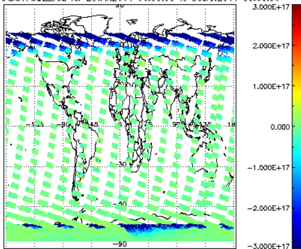
SCIOL2P_NADUV7S02_vcd for 29JAN2011 00:00:00 to 30JAN2011 00:00:00
