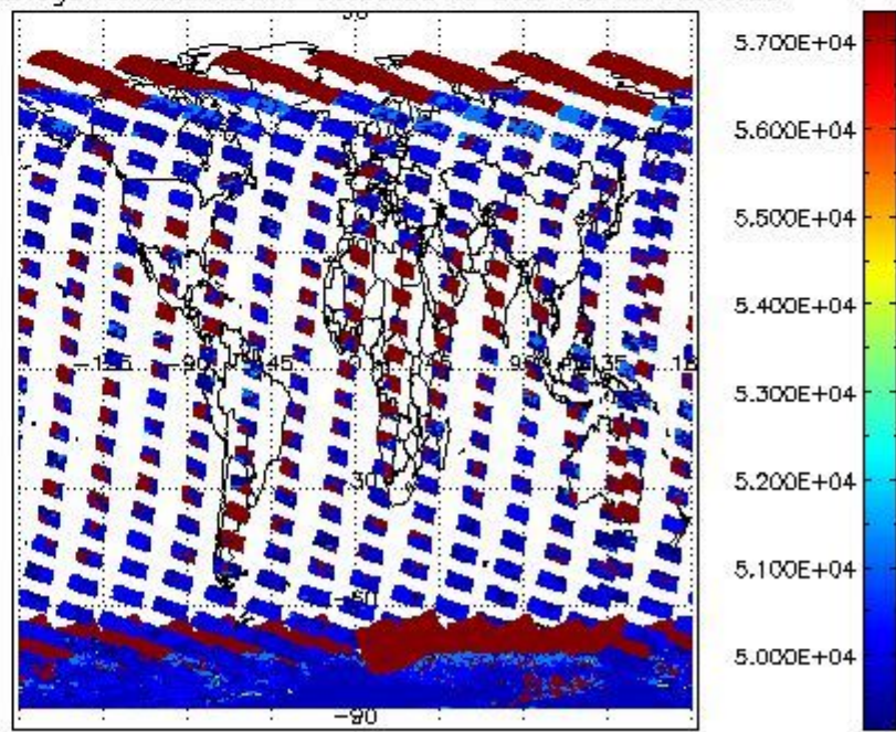
cloud_flags for 29JAN2011 00:00:00 to 30JAN2011 00:00:00
