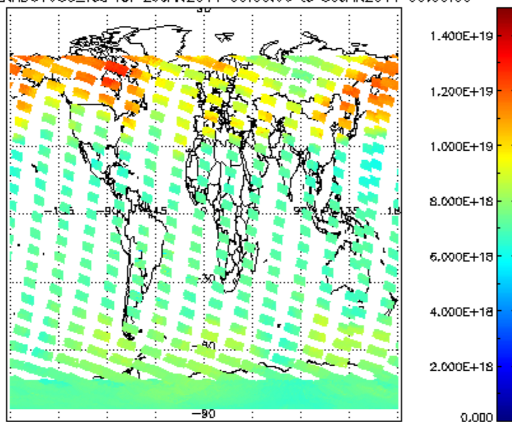
SCIOL2P_NADUV003_vcd for 29JAN2011 00:00:00 to 30JAN2011 00:00:00
