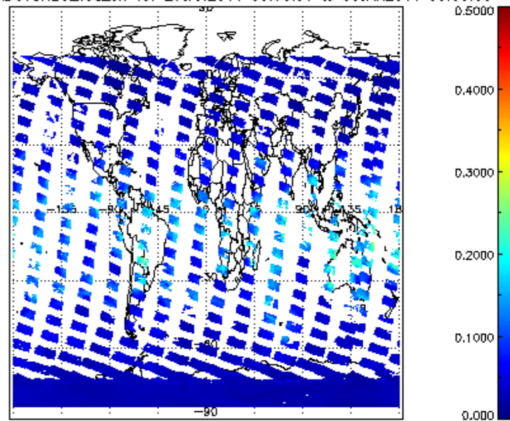
SCIOL2P_NADUVBH20_vcd_err for 29JAN2011 00:00:00 to 30JAN2011 00:00:00
