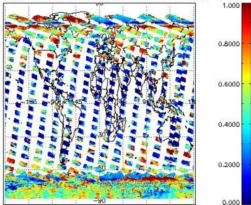
cL_frac for 29JAN2011 00:00:00 to 30JAN2011 00:00:00
