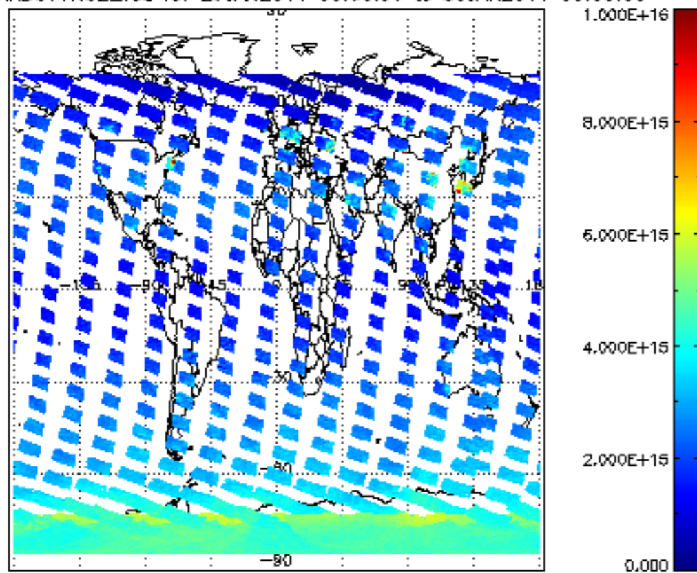
SCIOL2P_NADUV1NO2_vcd for 29JAN2011 00:00:00 to 30JAN2011 00:00:00
