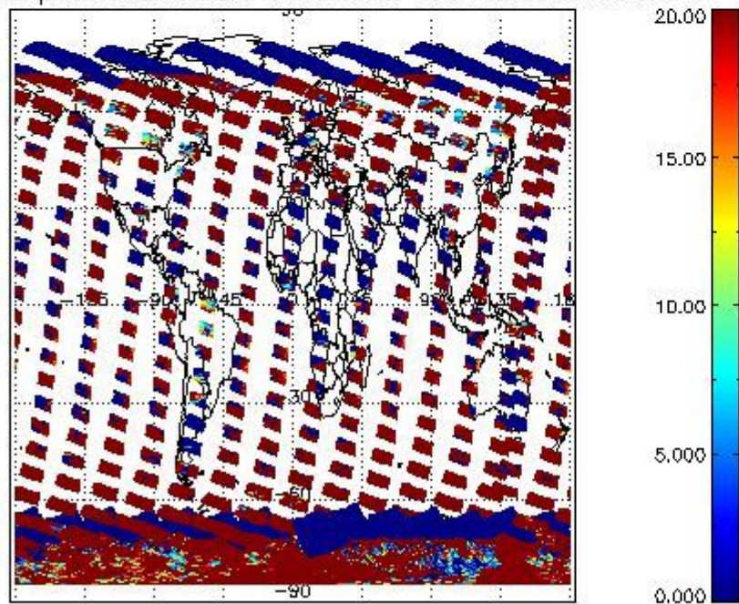
cLopt_depth for 29JAN2011 00:00:00 to 30JAN2011 00:00:00
