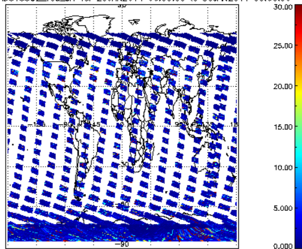
SCIOL2P_NADUV5S02_vcd_err for 29JAN2011 00:00:00 to 30JAN2011 00:00:00
