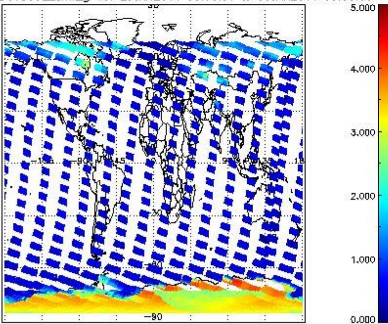
SCIOL2P_NADUV5SO2_amf_gr for 29JAN2011 00:00:00 to 30JAN2011 00:00:00
