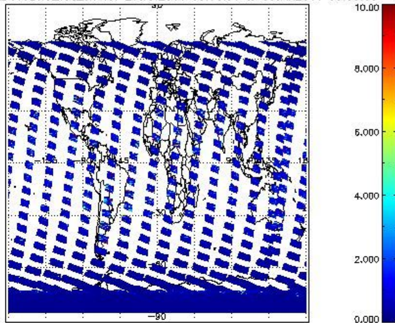
SCIOL2P_NADUV3BRO_vcd_err for 29JAN2011 00:00:00 to 30JAN2011 00:00:00
