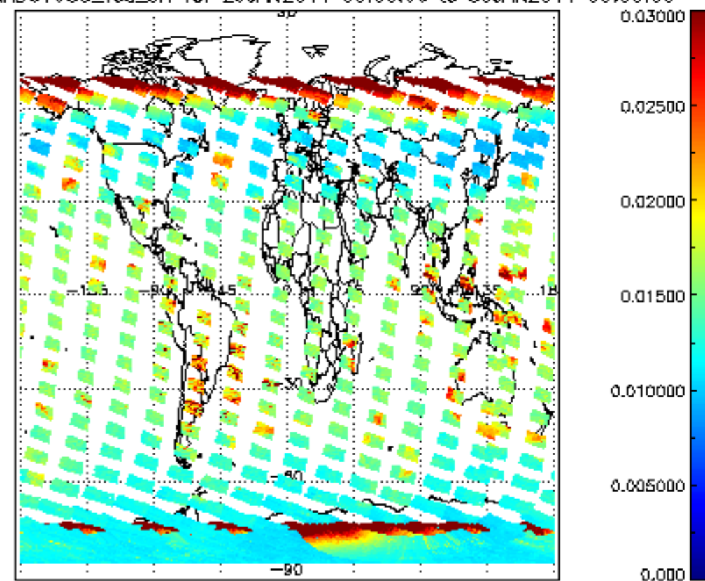
SCIOL2P_NADUV003_vcd_err for 29JAN2011 00:00:00 to 30JAN2011 00:00:00
