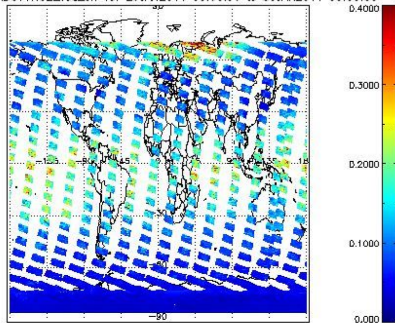
SCIOL2P_NADUV1NO2_vcd_err for 29JAN2011 00:00:00 to 30JAN2011 00:00:00
