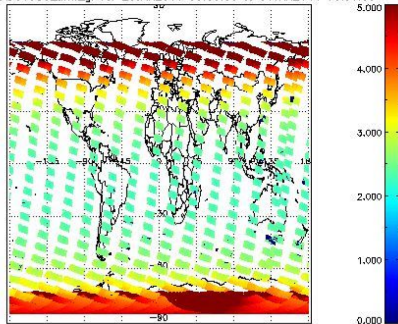
SCIOL2P_NADUV003_amf_gr for 29JAN2011 00:00:00 to 30JAN2011 00:00:00
