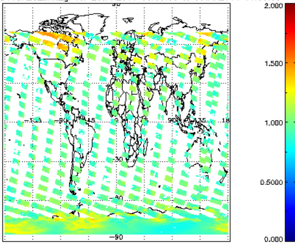
SCIOL2P_NADUVBH20_amf_gr for 29JAN2011 00:00:00 to 30JAN2011 00:00:00
