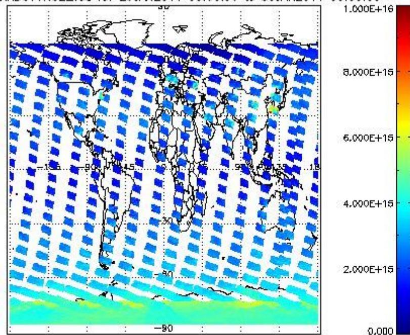
SCIOL2P_NADUV1NO2_vcd for 29JAN2011 00:00:00 to 30JAN2011 00:00:00
