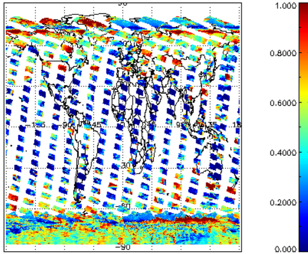
cL_frac for 29JAN2011 00:00:00 to 30JAN2011 00:00:00
