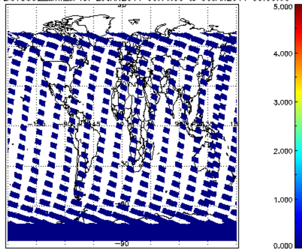
SCIOL2P_NADUV5S02_amf_cl for 29JAN2011 00:00:00 to 30JAN2011 00:00:00
