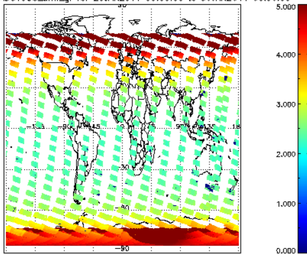
SCIOL2P_NADUV003_amf_gr for 29JAN2011 00:00:00 to 30JAN2011 00:00:00
