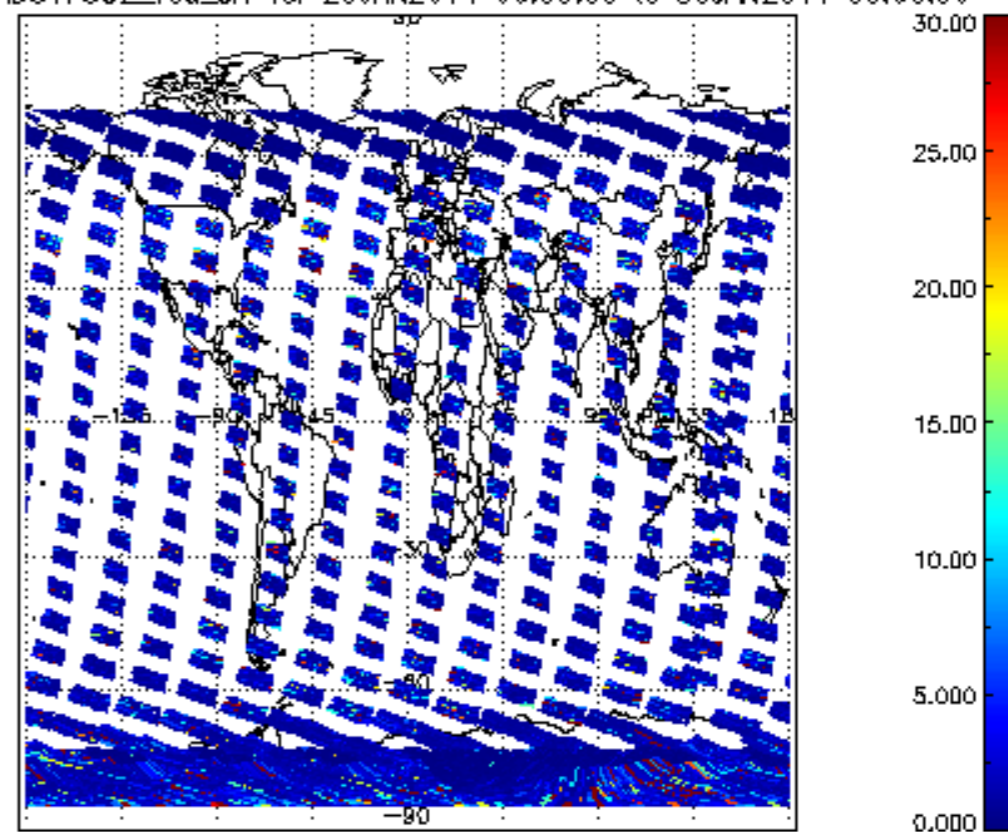
SCIOL2P_NADUV7S02_vcd_err for 29JAN2011 00:00:00 to 30JAN2011 00:00:00
