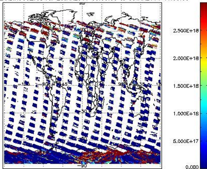
SCIDL2P_NADIR3CO_vcd for 29JAN2011 00:00:00 to 30JAN2011 00:00:00
