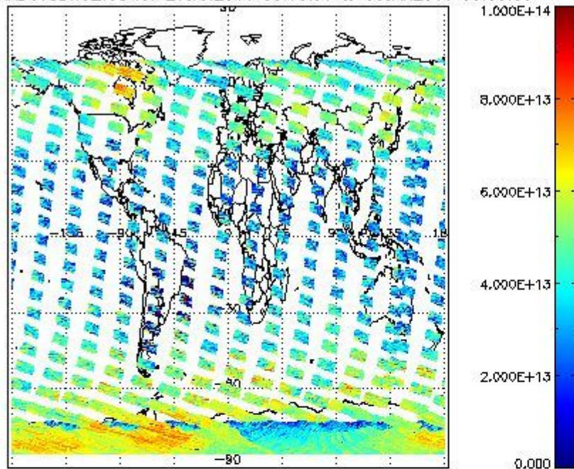
SCIOL2P_NADUV3BRO_vcd for 29JAN2011 00:00:00 to 30JAN2011 00:00:00
