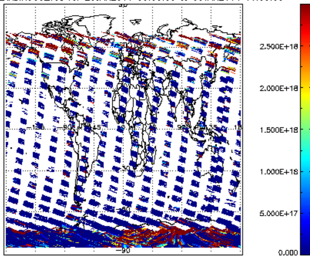
SCIOL2P_NADIR3CO_vcd for 29JAN2011 00:00:00 to 30JAN2011 00:00:00
