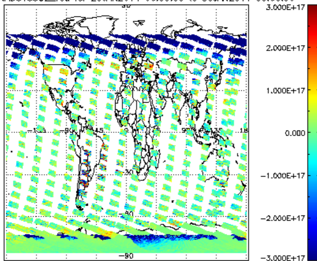
SCIOL2P_NADUV5S02_vcd for 29JAN2011 00:00:00 to 30JAN2011 00:00:00
