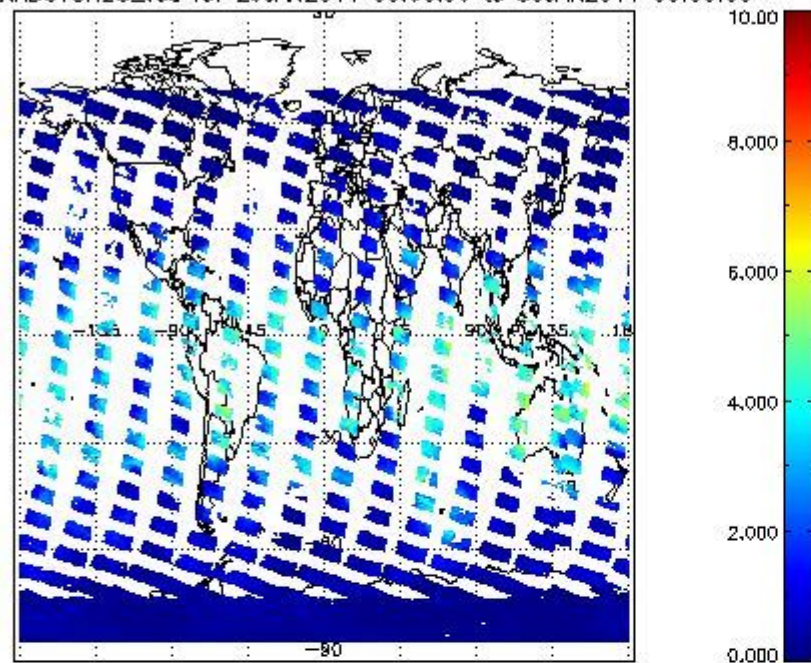
SCIOL2P_NADUV8H20_vcd for 29JAN2011 00:00:00 to 30JAN2011 00:00:00
