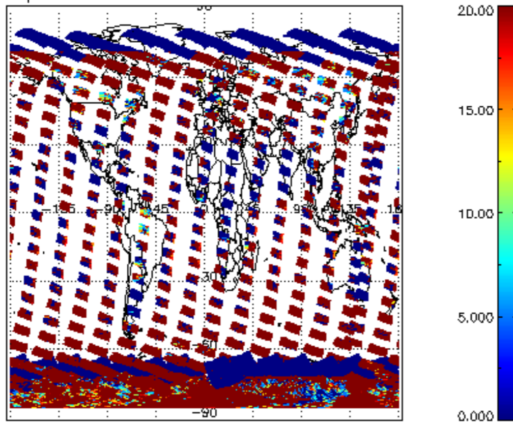
cLopt_depth for 29JAN2011 00:00:00 to 30JAN2011 00:00:00
