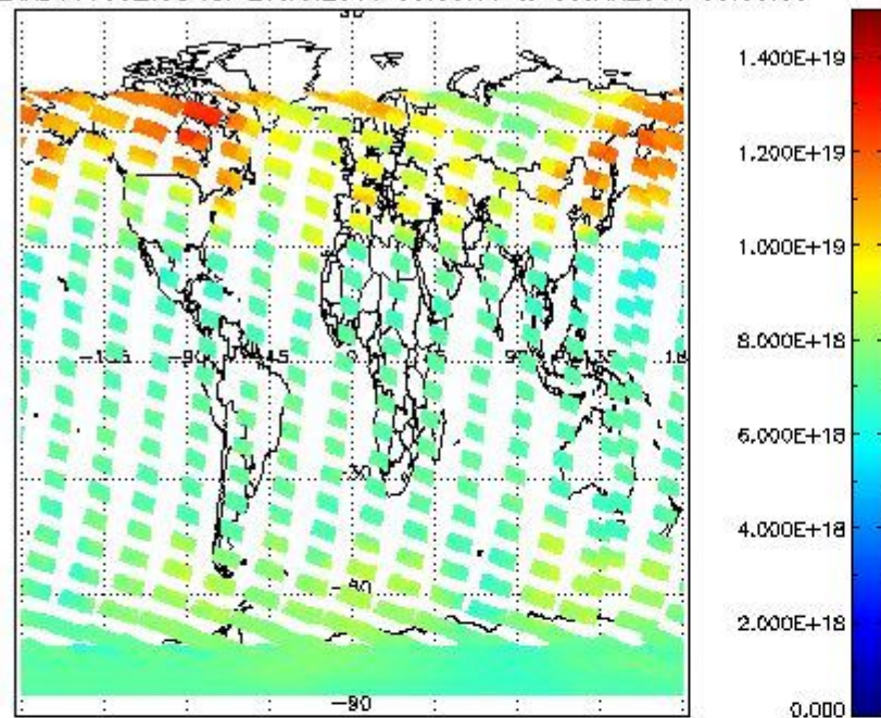
SCIOL2P_NADUV003_vcd for 29JAN2011 00:00:00 to 30JAN2011 00:00:00
