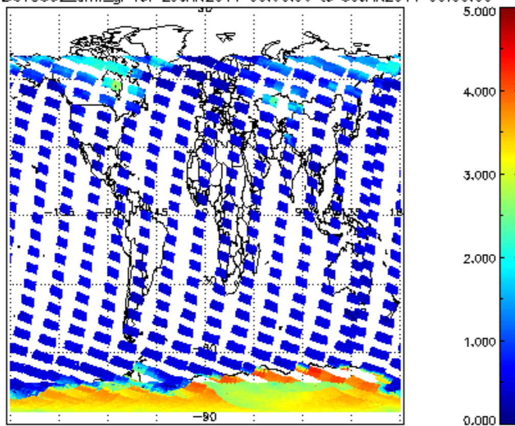
SCIOL2P_NADUV5S02_amf_gr for 29JAN2011 00:00:00 to 30JAN2011 00:00:00
