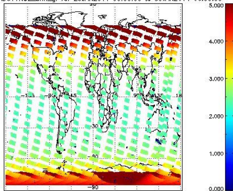
SCIOL2P_NADUV1NO2_amf_gr for 29JAN2011 00:00:00 to 30JAN2011 00:00:00
