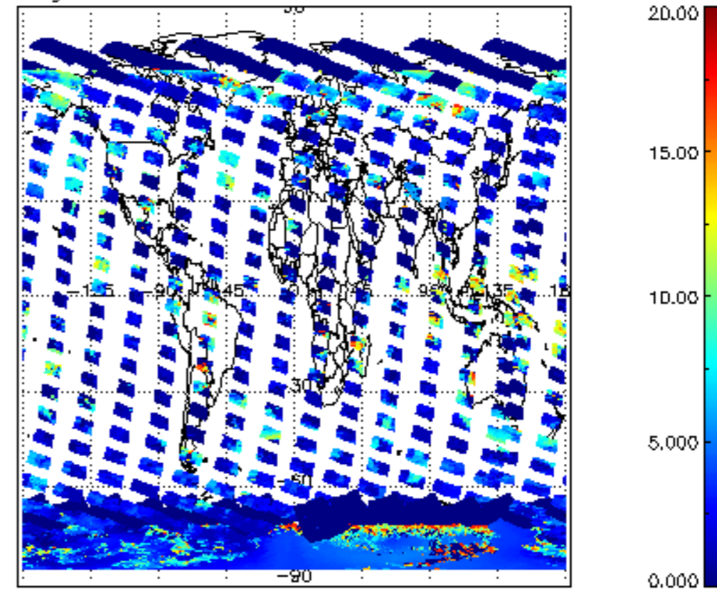
cL_top_height for 29JAN2011 00:00:00 to 30JAN2011 00:00:00
