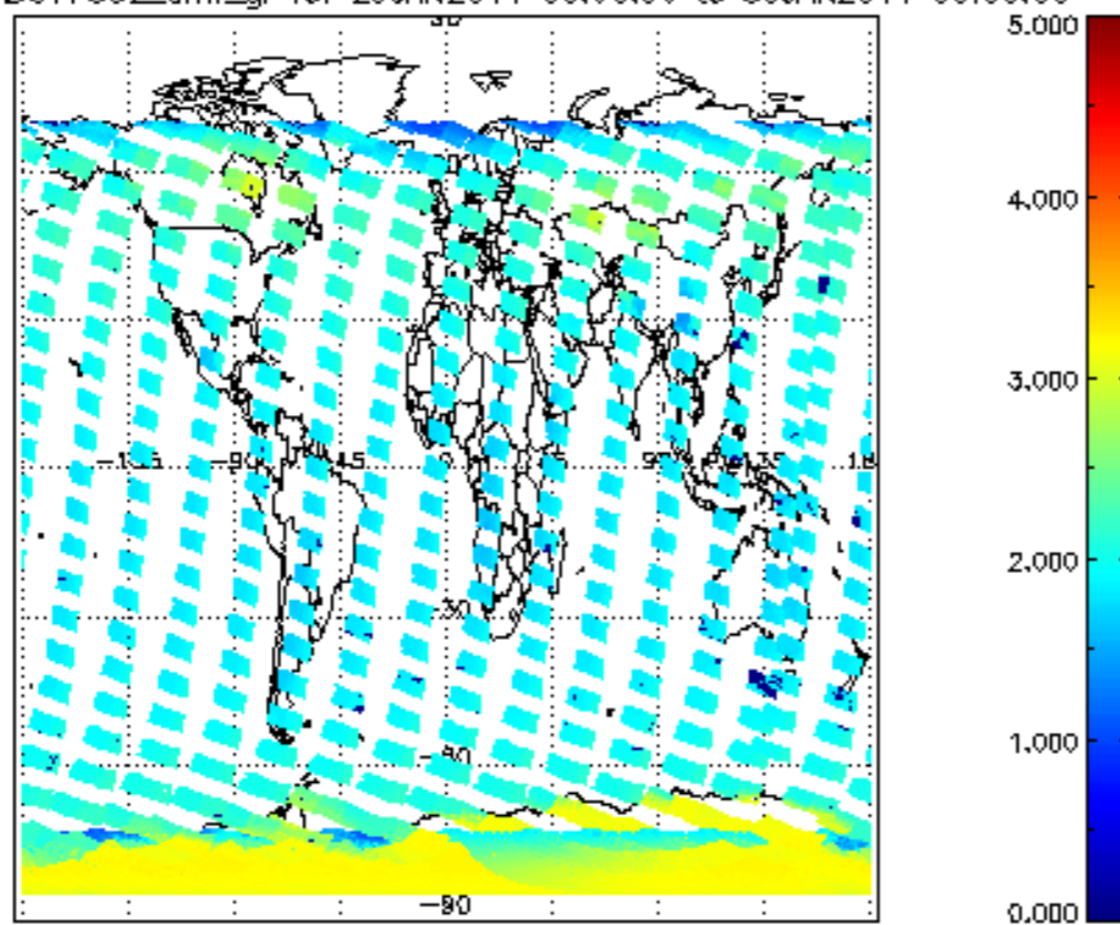
SCIOL2P_NADUV7S02_amf_gr for 29JAN2011 00:00:00 to 30JAN2011 00:00:00
