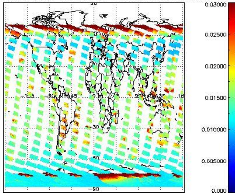
SCIOL2P_NADUV003_vcd_err for 29JAN2011 00:00:00 to 30JAN2011 00:00:00
