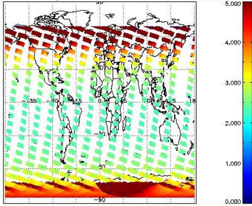
SCIOL2P_NADUV1NO2_amf_gr for 25JAN2011 00:00:00 to 26JAN2011 00:00:00
