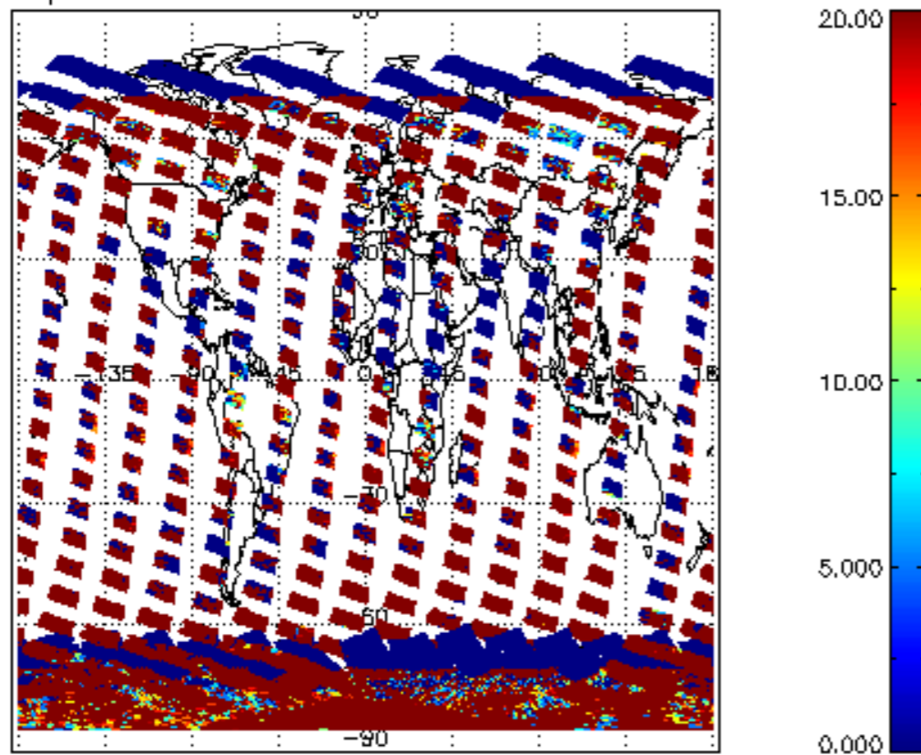
cLopt_depth for 25JAN2011 00:00:00 to 26JAN2011 00:00:00
