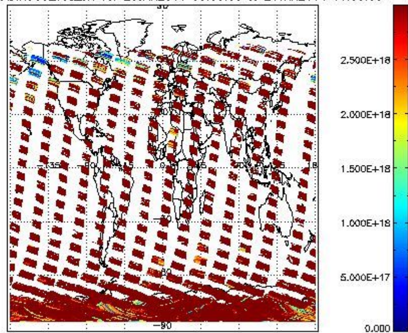
SCIDL2P_NADIR3CO_vcd_err for 25JAN2011 00:00:00 to 26JAN2011 00:00:00
