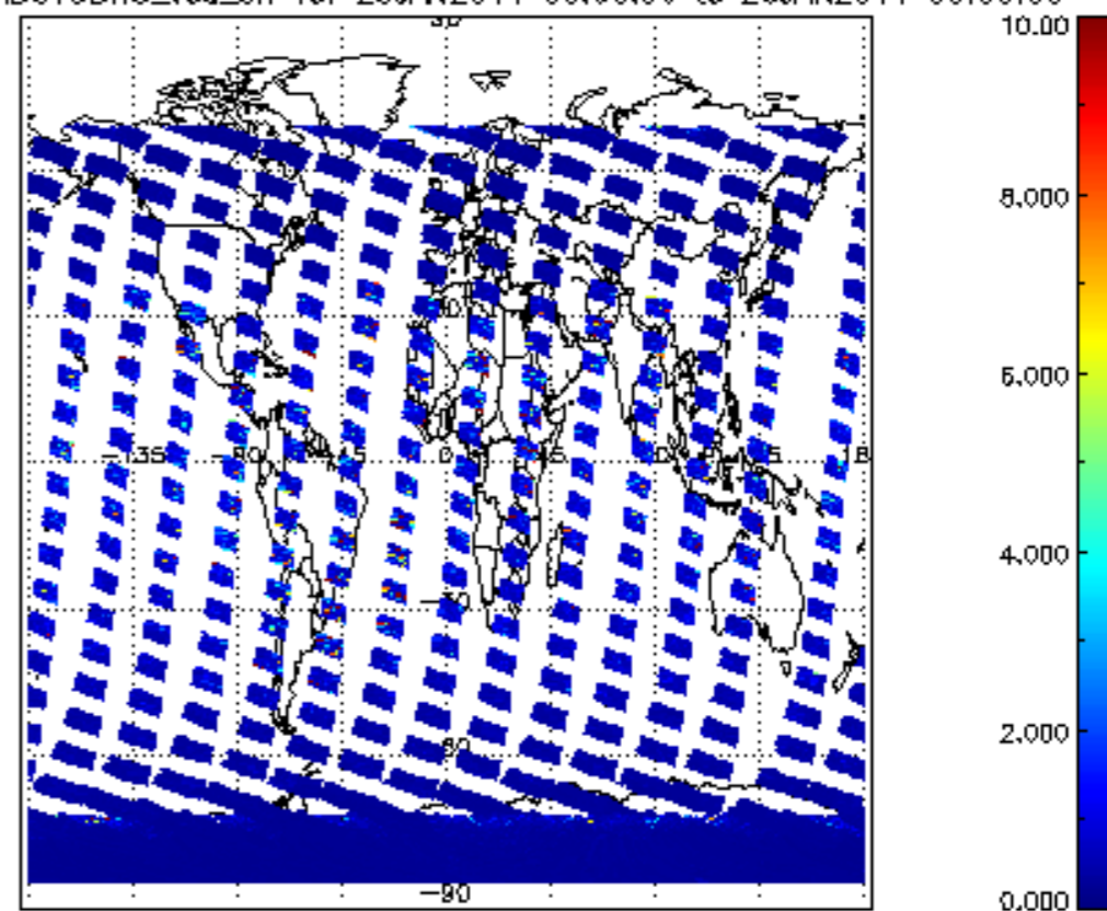
SCIOL2P_NADUV3BRO_vcd_err for 25JAN2011 00:00:00 to 26JAN2011 00:00:00
