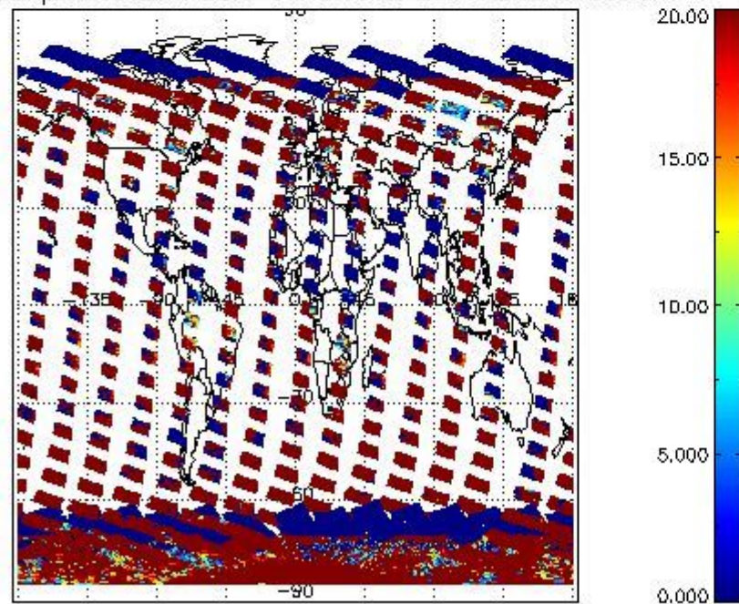
cLopt_depth for 25JAN2011 00:00:00 to 26JAN2011 00:00:00
