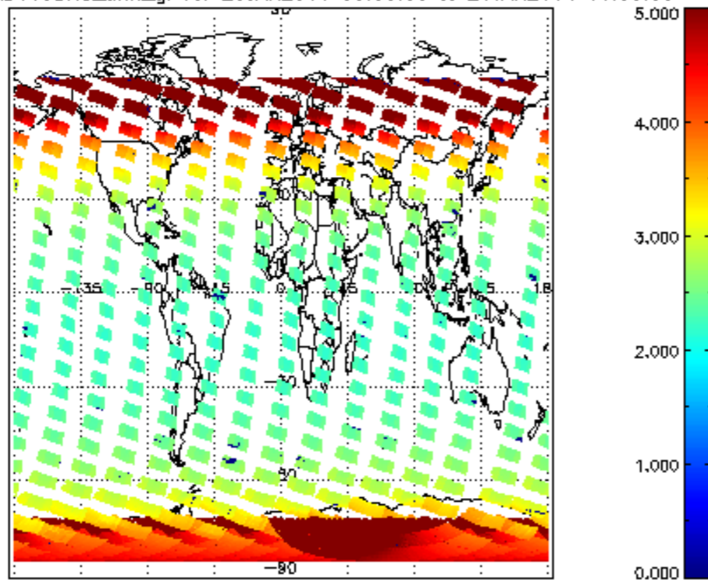
SCIOL2P_NADUV3BRO_amf_gr for 25JAN2011 00:00:00 to 26JAN2011 00:00:00
