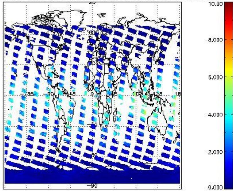
SCIOL2P_NADUV8H20_vcd for 25JAN2011 00:00:00 to 26JAN2011 00:00:00
