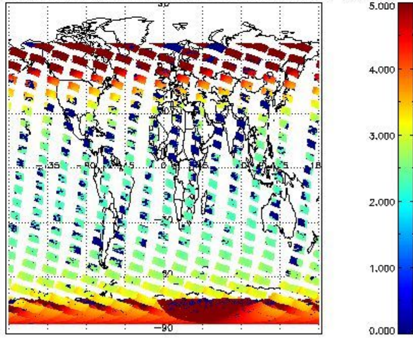
SCIOL2P_NADUV1NO2_amf_cl for 25JAN2011 00:00:00 to 26JAN2011 00:00:00
