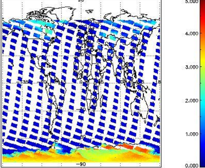
SCIOL2P_NADUV5SO2_amf_gr for 25JAN2011 00:00:00 to 26JAN2011 00:00:00
