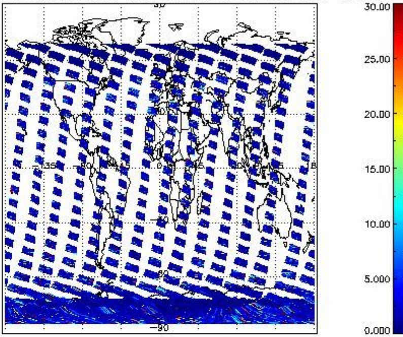
SCIOL2P_NADUV5SO2_vcd_err for 25JAN2011 00:00:00 to 26JAN2011 00:00:00
