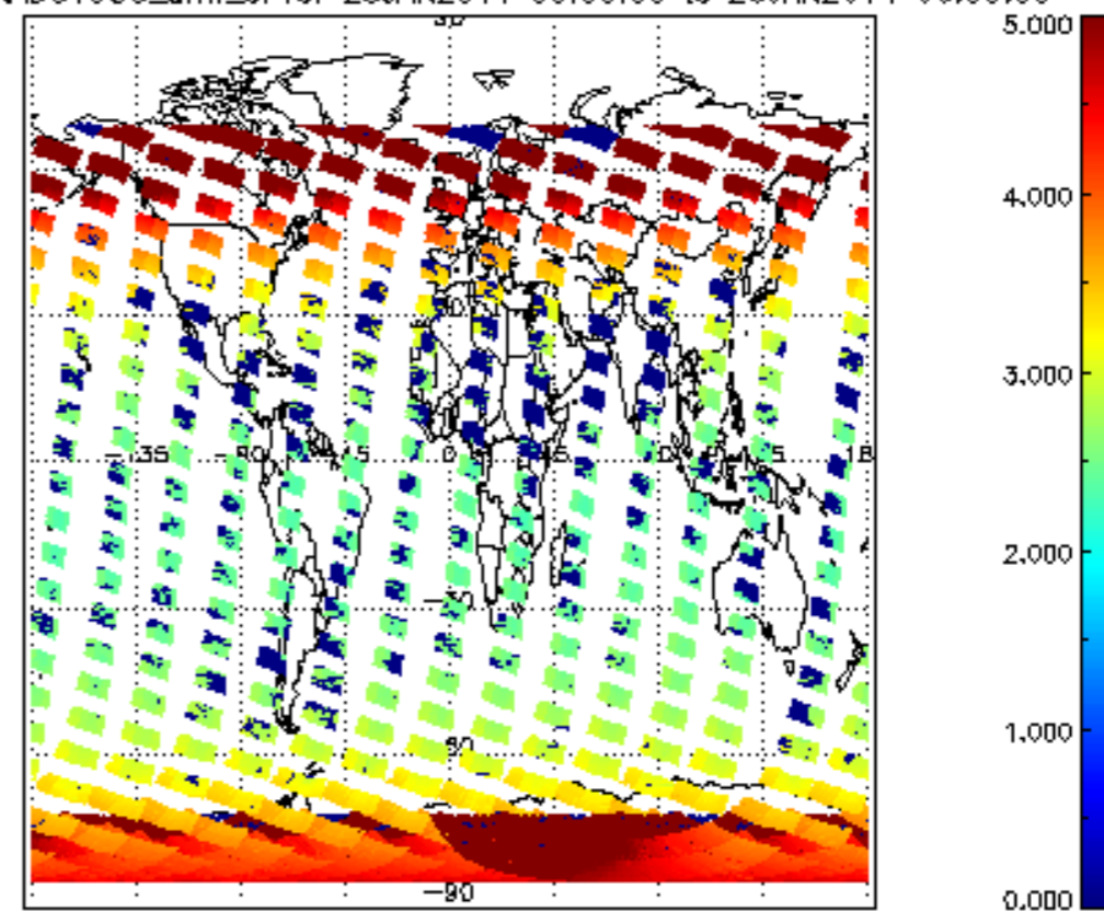
SCIOL2P_NADUV003_amf_cl for 25JAN2011 00:00:00 to 26JAN2011 00:00:00
