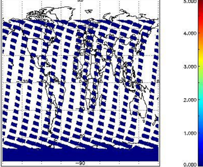
SCIOL2P_NADUV5SO2_amf_cl for 25JAN2011 00:00:00 to 26JAN2011 00:00:00
