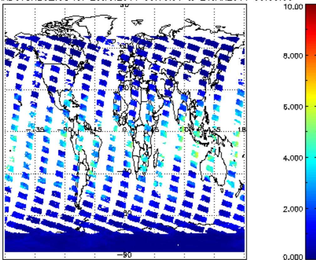
SCIOL2P_NADUV8H20_vcd for 25JAN2011 00:00:00 to 26JAN2011 00:00:00
