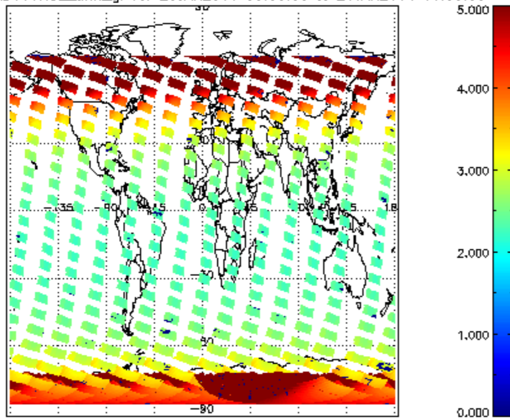
SCIOL2P_NADUV1NO2_amf_gr for 25JAN2011 00:00:00 to 26JAN2011 00:00:00
