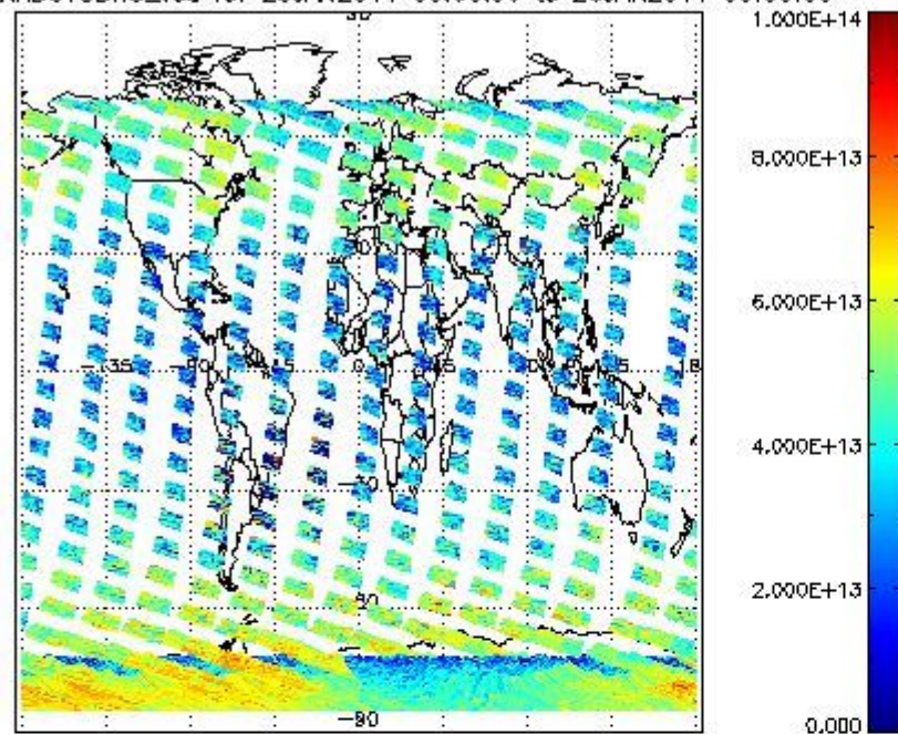
SCIOL2P_NADUV3BRO_vcd for 25JAN2011 00:00:00 to 26JAN2011 00:00:00
