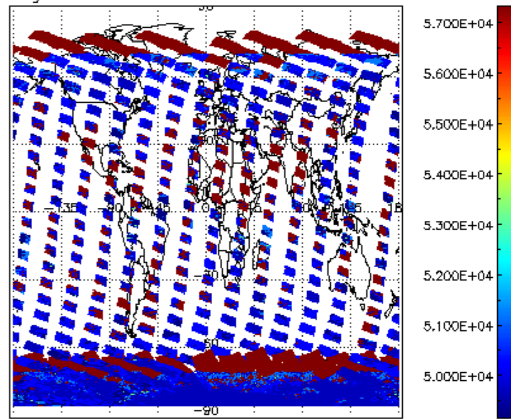
cloud_flags for 25JAN2011 00:00:00 to 26JAN2011 00:00:00
