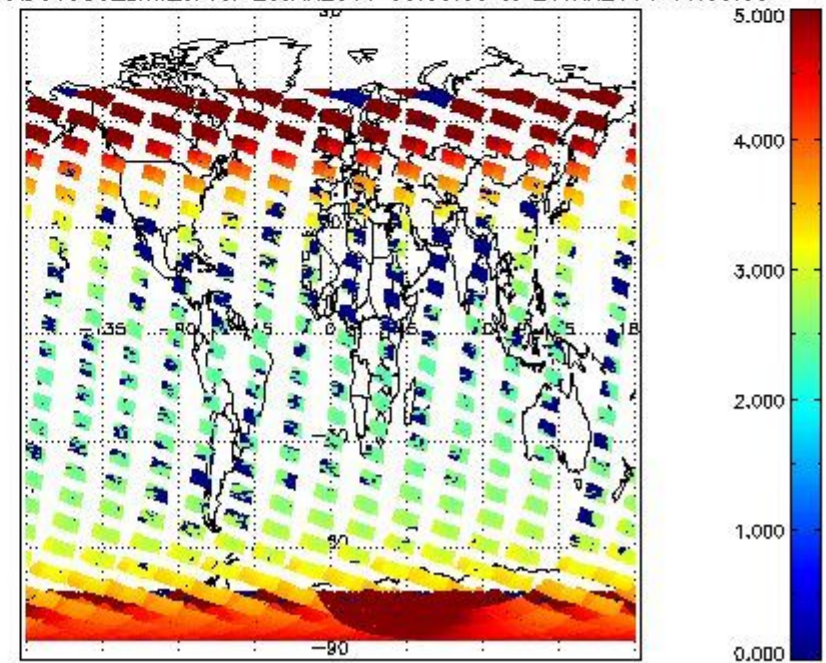
SCIOL2P_NADUV003_amf_cl for 25JAN2011 00:00:00 to 26JAN2011 00:00:00
