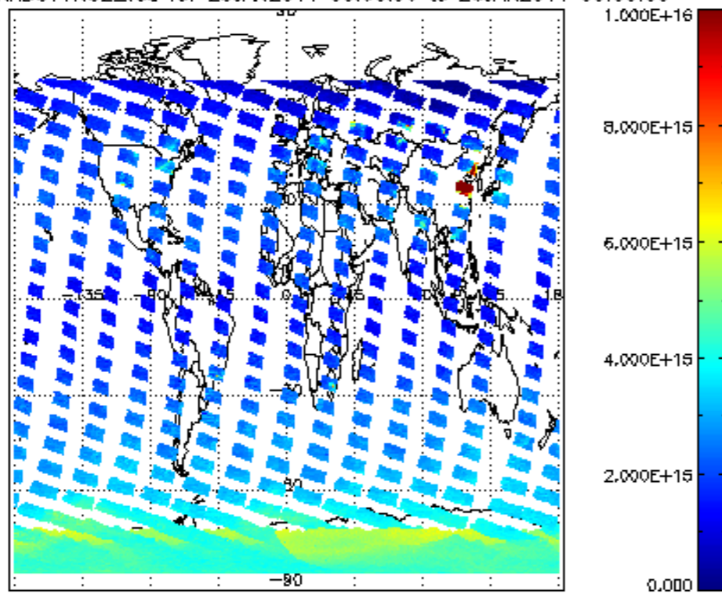
SCIOL2P_NADUV1NO2_vcd for 25JAN2011 00:00:00 to 26JAN2011 00:00:00
