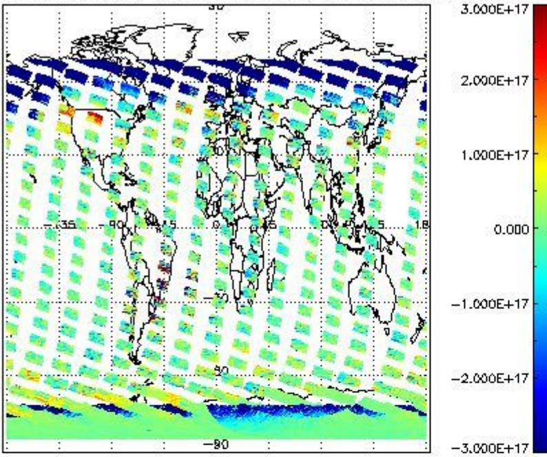
SCIOL2P_NADUV5SO2_vcd for 25JAN2011 00:00:00 to 26JAN2011 00:00:00
