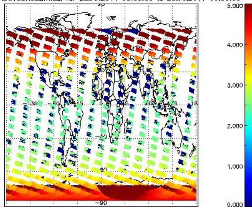
SCIOL2P_NADUV3BRO_amf_cl for 25JAN2011 00:00:00 to 26JAN2011 00:00:00
