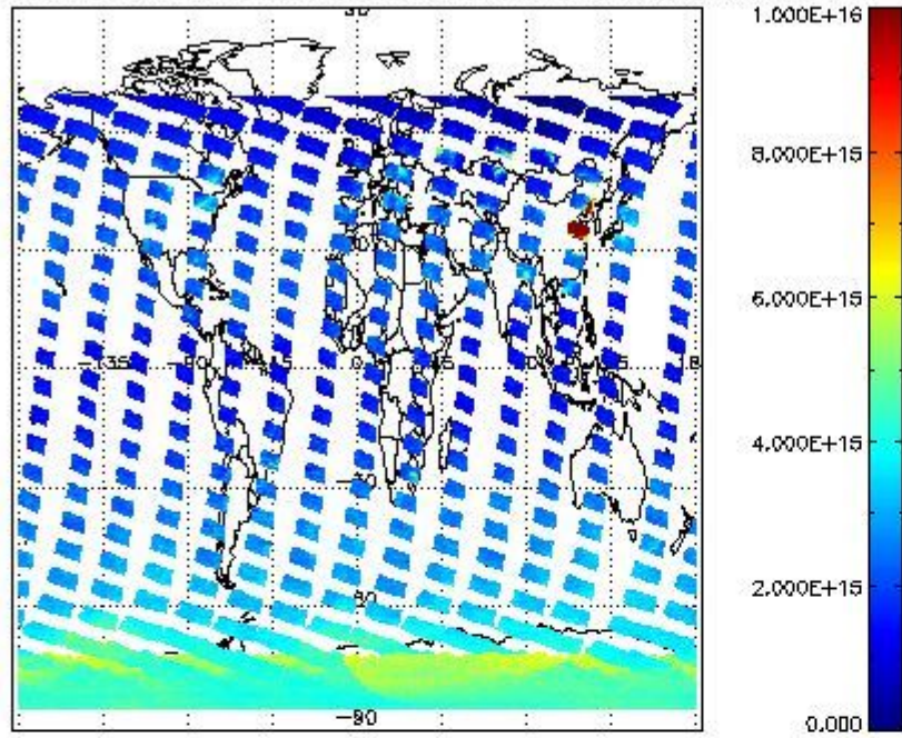
SCIOL2P_NADUV1NO2_vcd for 25JAN2011 00:00:00 to 26JAN2011 00:00:00
