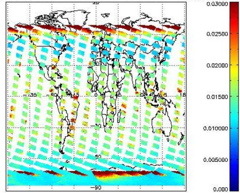
SCIOL2P_NADUV003_vcd_err for 25JAN2011 00:00:00 to 26JAN2011 00:00:00
