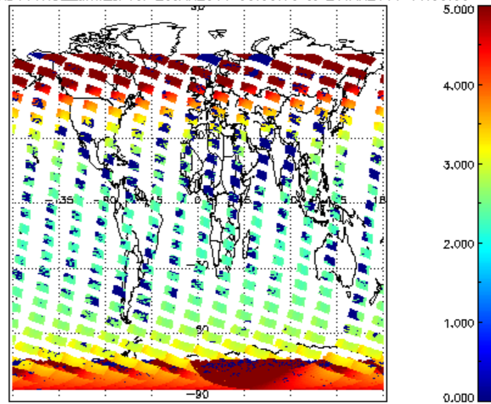
SCIOL2P_NADUV1NO2_amf_cl for 25JAN2011 00:00:00 to 26JAN2011 00:00:00
