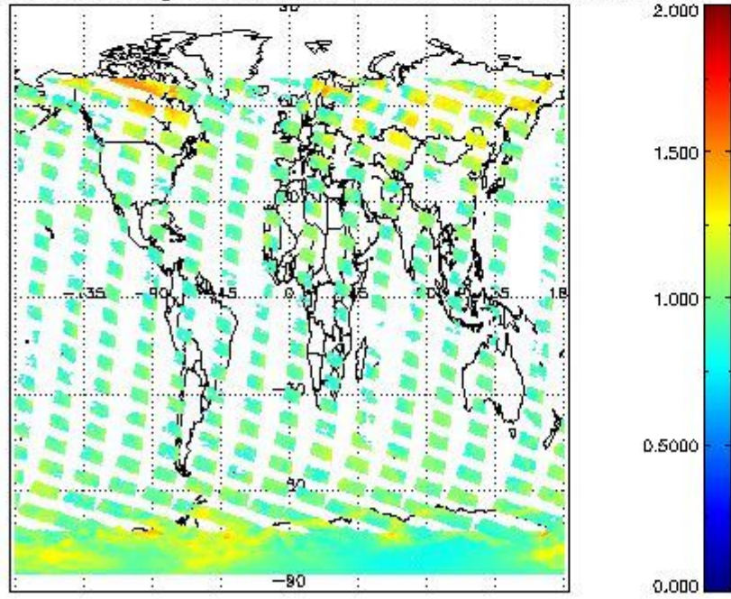
SCIOL2P_NADUV8H20_amf_gr for 25JAN2011 00:00:00 to 26JAN2011 00:00:00
