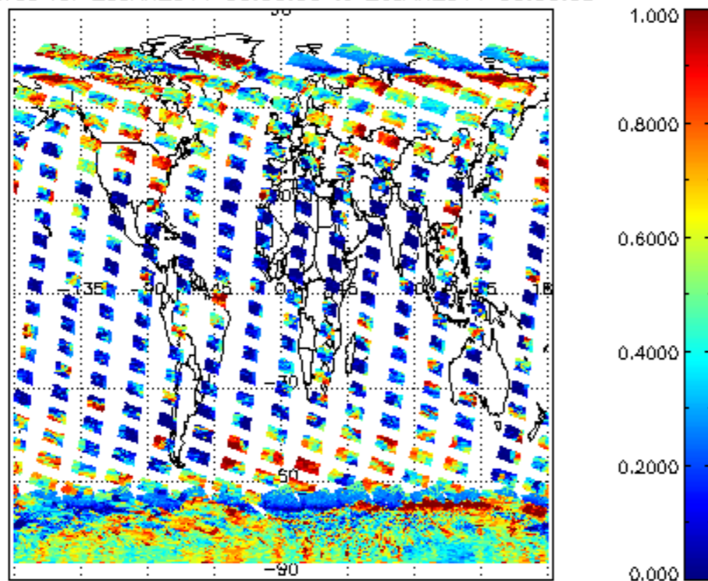
cL_frac for 25JAN2011 00:00:00 to 26JAN2011 00:00:00
