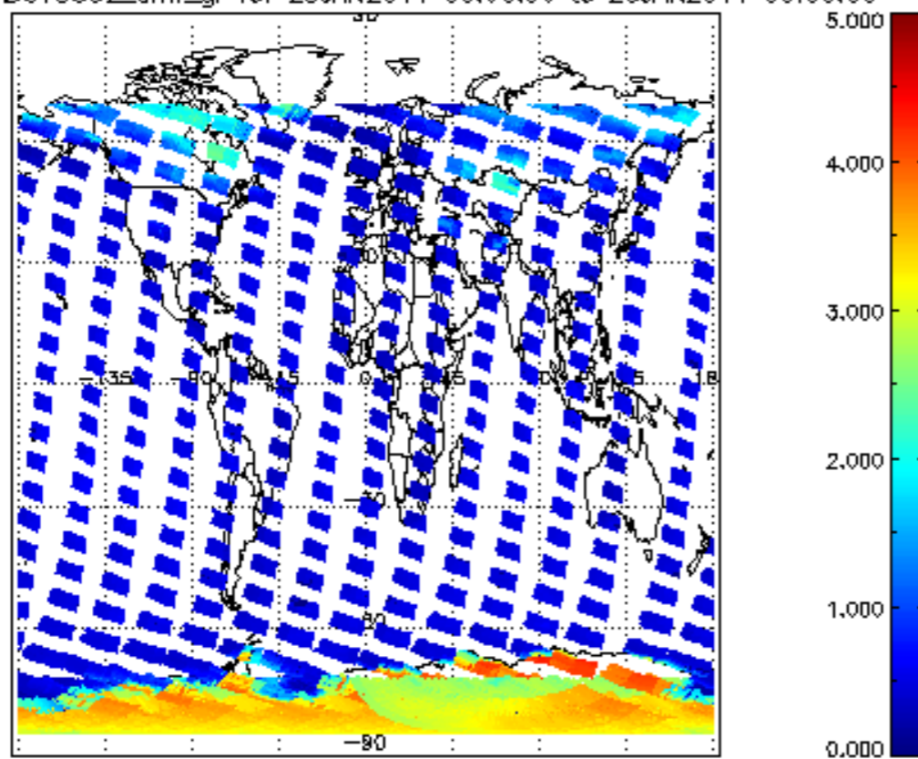
SCIOL2P_NADUV5S02_amf_gr for 25JAN2011 00:00:00 to 26JAN2011 00:00:00
