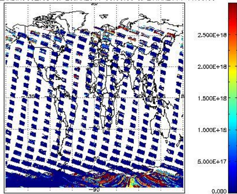
SCIDL2P_NADIR3CO_vcd for 25JAN2011 00:00:00 to 26JAN2011 00:00:00
