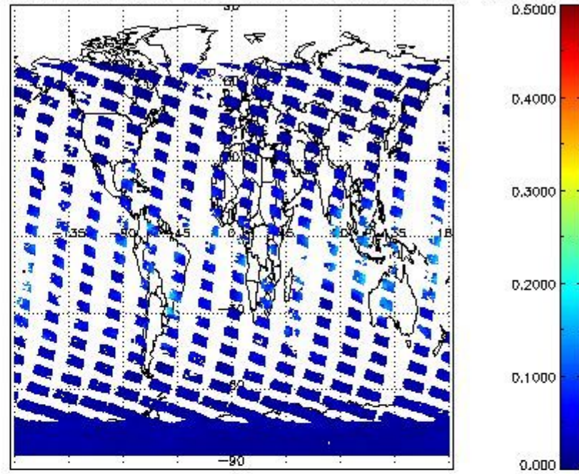
SCIOL2P_NADUV8H20_vcd_err for 25JAN2011 00:00:00 to 26JAN2011 00:00:00
