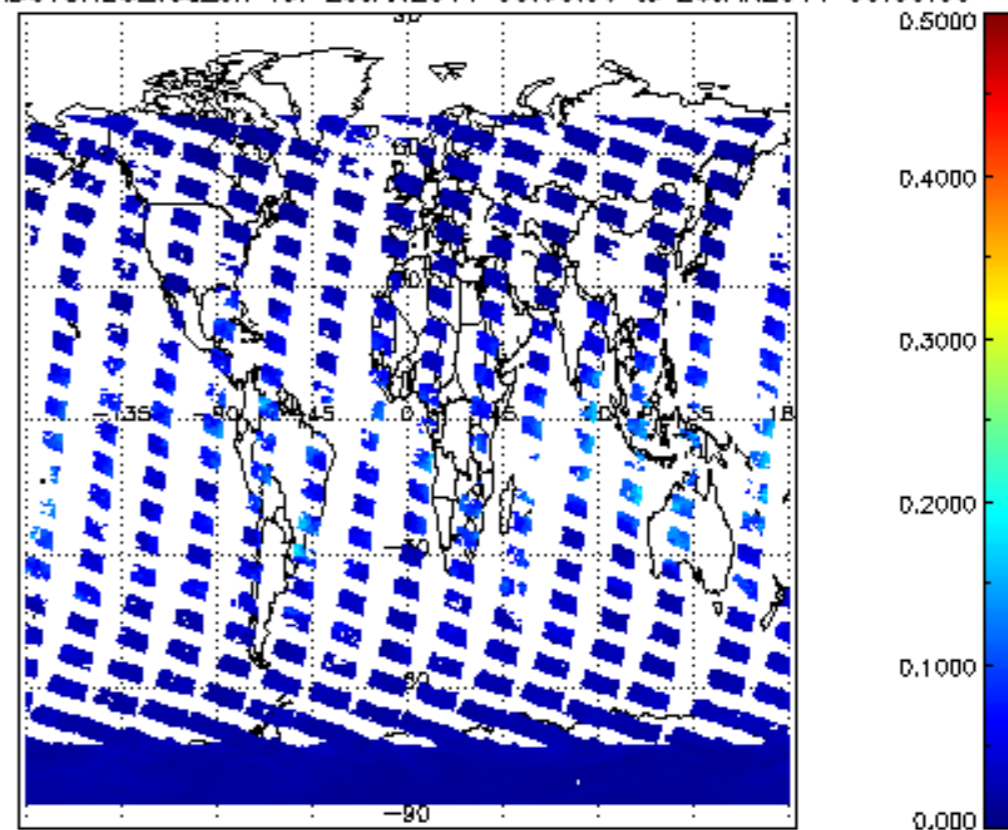
SCIOL2P_NADUV8H20_vcd_err for 25JAN2011 00:00:00 to 26JAN2011 00:00:00
