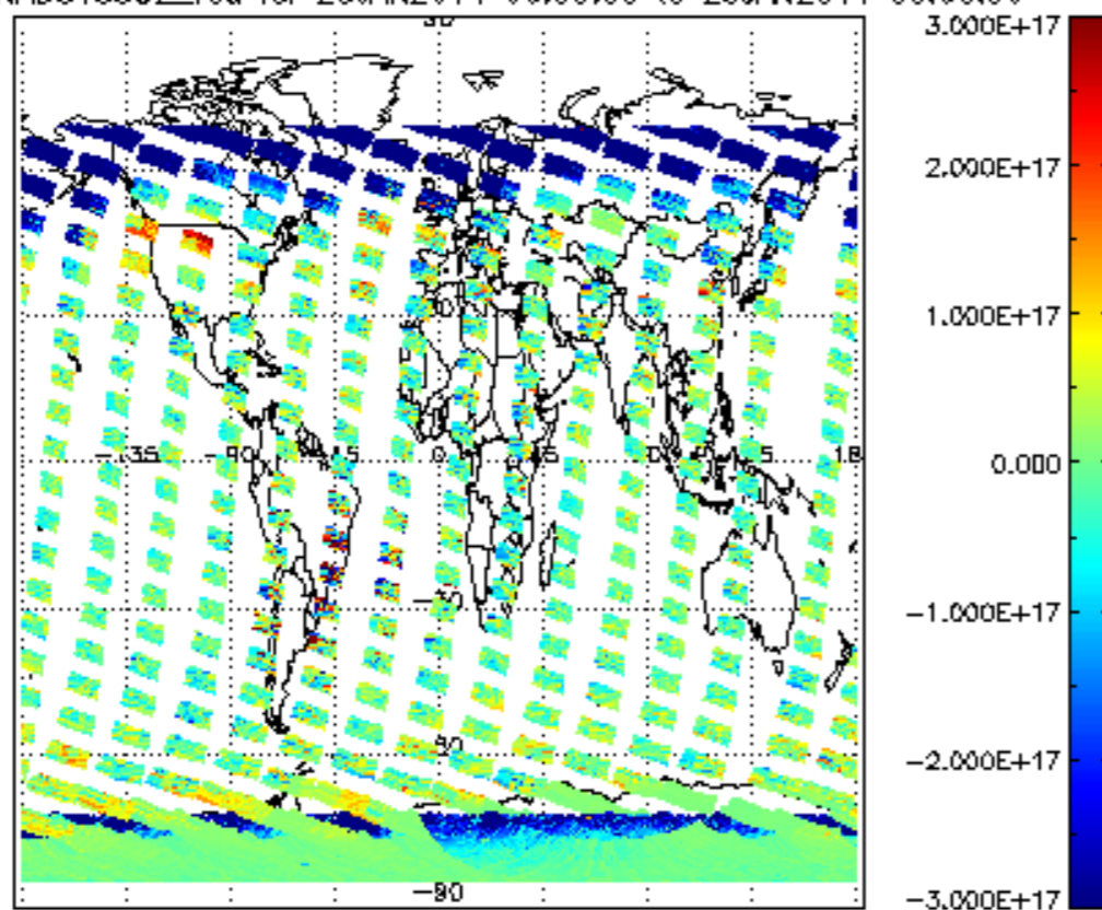
SCIOL2P_NADUV5S02_vcd for 25JAN2011 00:00:00 to 26JAN2011 00:00:00
