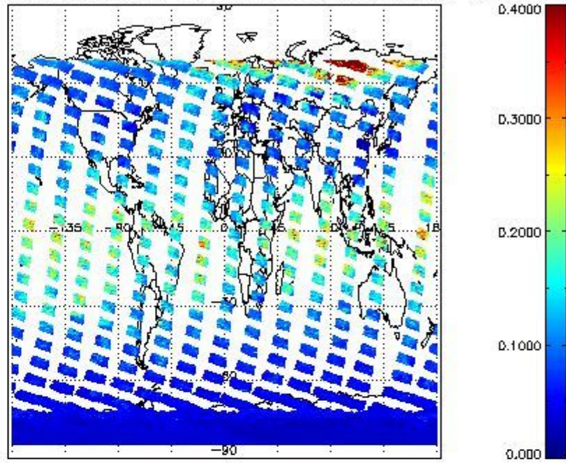
SCIOL2P_NADUV1NO2_vcd_err for 25JAN2011 00:00:00 to 26JAN2011 00:00:00
