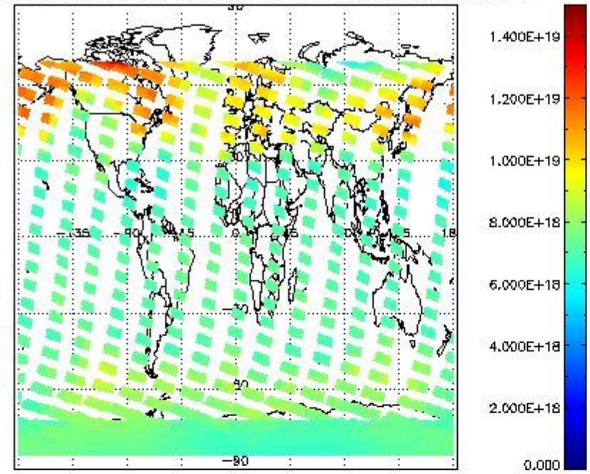
SCIOL2P_NADUV003_vcd for 25JAN2011 00:00:00 to 26JAN2011 00:00:00
