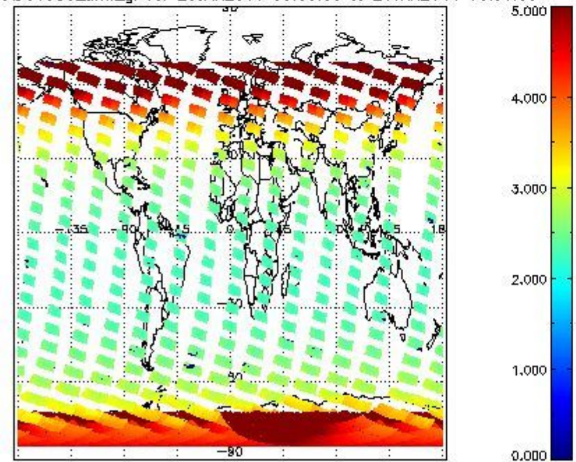
SCIOL2P_NADUV003_amf_gr for 25JAN2011 00:00:00 to 26JAN2011 00:00:00
