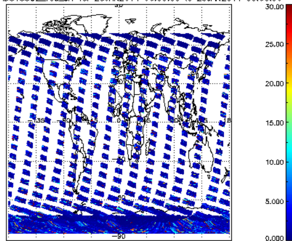
SCIOL2P_NADUV5S02_vcd_err for 25JAN2011 00:00:00 to 26JAN2011 00:00:00
