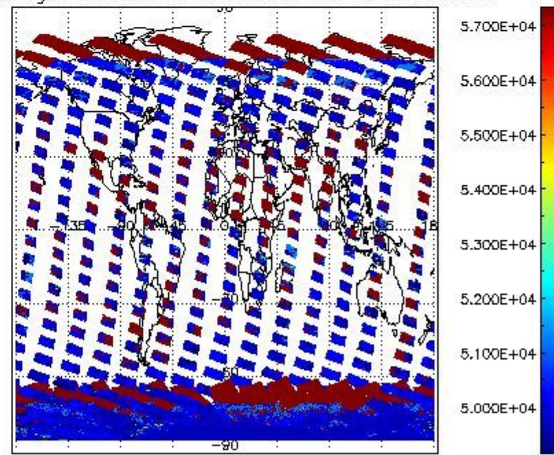
cloud_flags for 25JAN2011 00:00:00 to 26JAN2011 00:00:00
