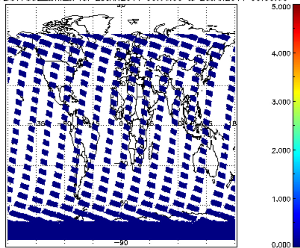
SCIOL2P_NADUV7S02_amf_sl for 25JAN2011 00:00:00 to 26JAN2011 00:00:00
