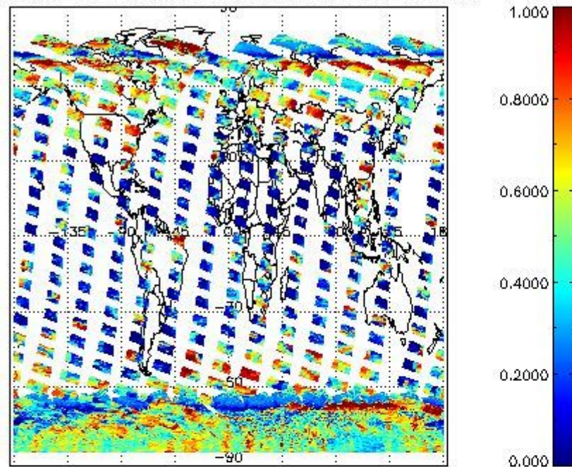
cL_frac for 25JAN2011 00:00:00 to 26JAN2011 00:00:00
