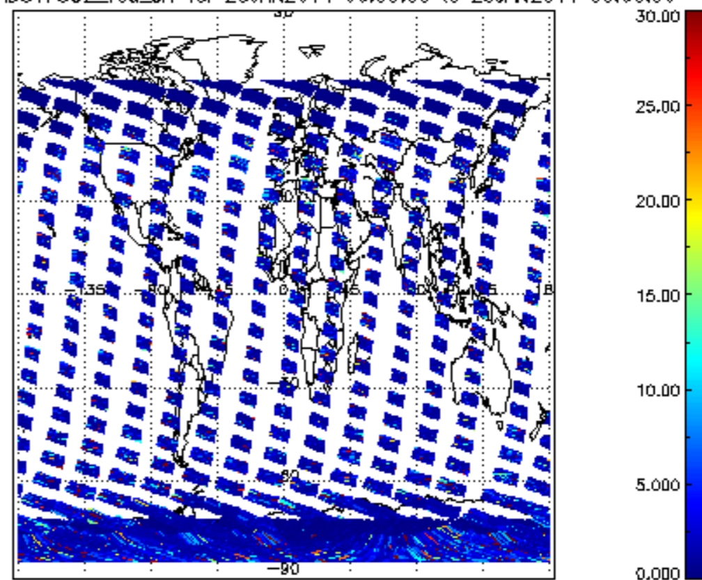
SCIOL2P_NADUV7S02_vcd_err for 25JAN2011 00:00:00 to 26JAN2011 00:00:00
