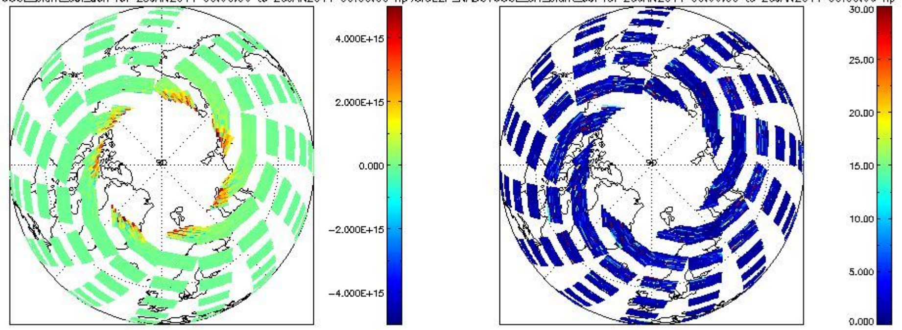
SCIOI2P_NADUV60CL_slant_col_den for 25JAN2011 00:00:00 to 26JAN2011 00:00:00 np; SCIOI2P_NADUV60CL_err_slant_col for 25JAN2011 00:00:00 to 26JAN2011 00:00:00 np
