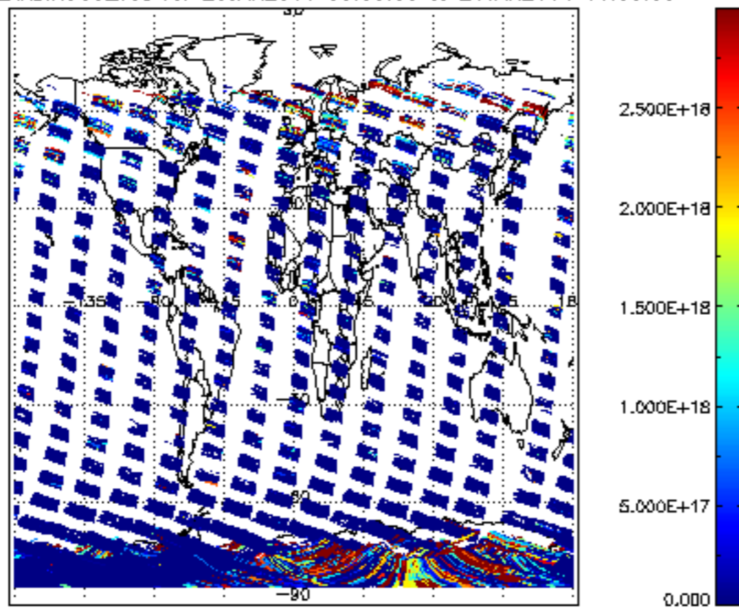
SCIOL2P_NADIR3CO_vcd for 25JAN2011 00:00:00 to 26JAN2011 00:00:00
