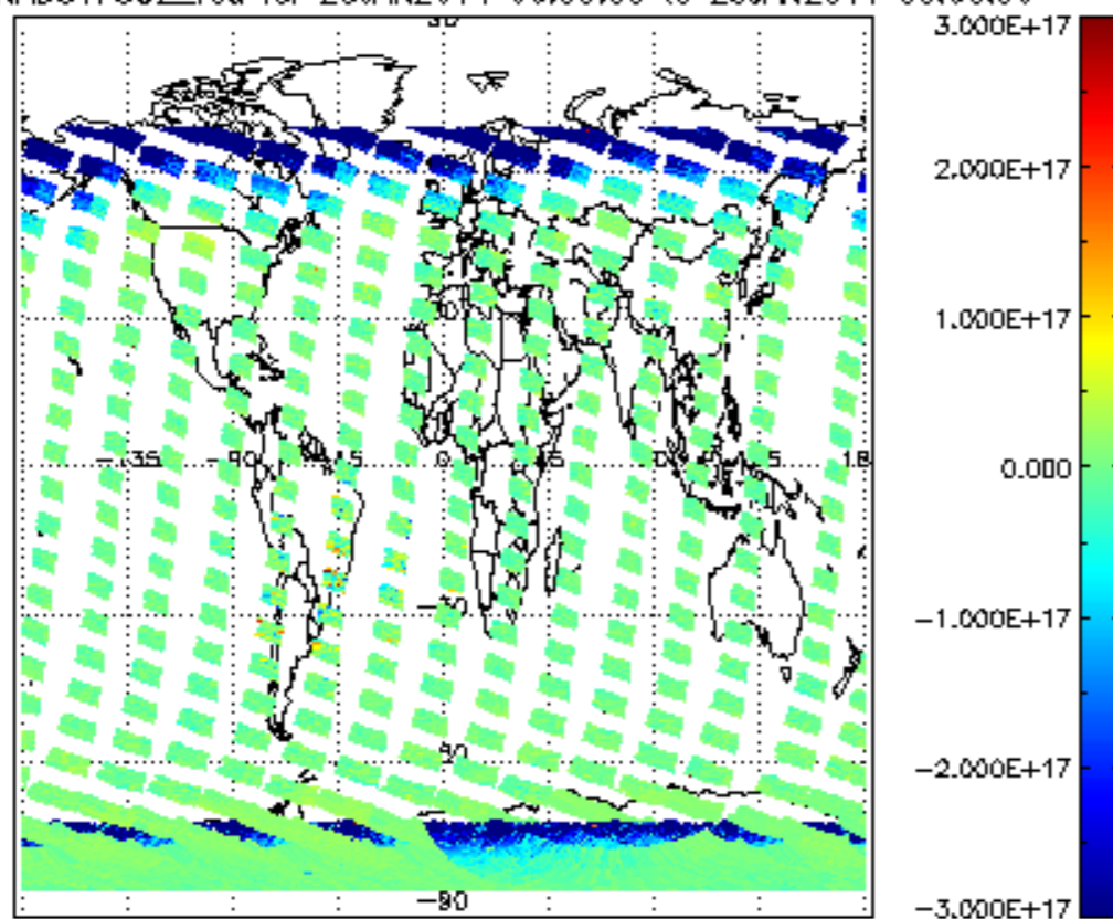
SCIOL2P_NADUV7S02_vcd for 25JAN2011 00:00:00 to 26JAN2011 00:00:00
