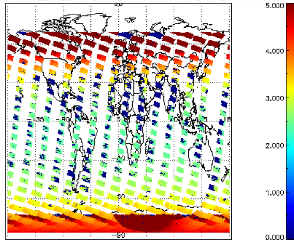
SCIOL2P_NADUV3BRO_amf_cl for 25JAN2011 00:00:00 to 26JAN2011 00:00:00
