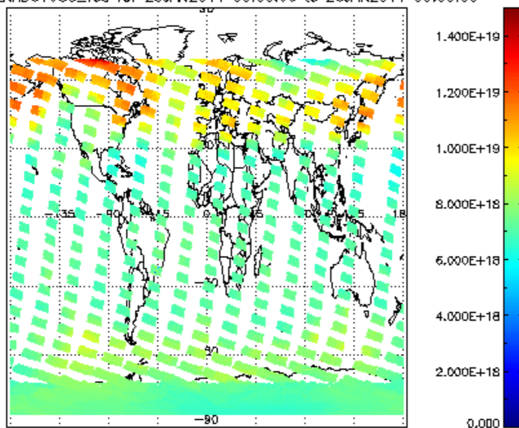
SCIOL2P_NADUV003_vcd for 25JAN2011 00:00:00 to 26JAN2011 00:00:00
