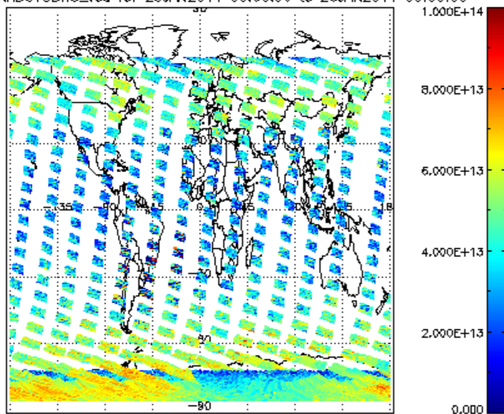
SCIOL2P_NADUV3BRO_vcd for 25JAN2011 00:00:00 to 26JAN2011 00:00:00
