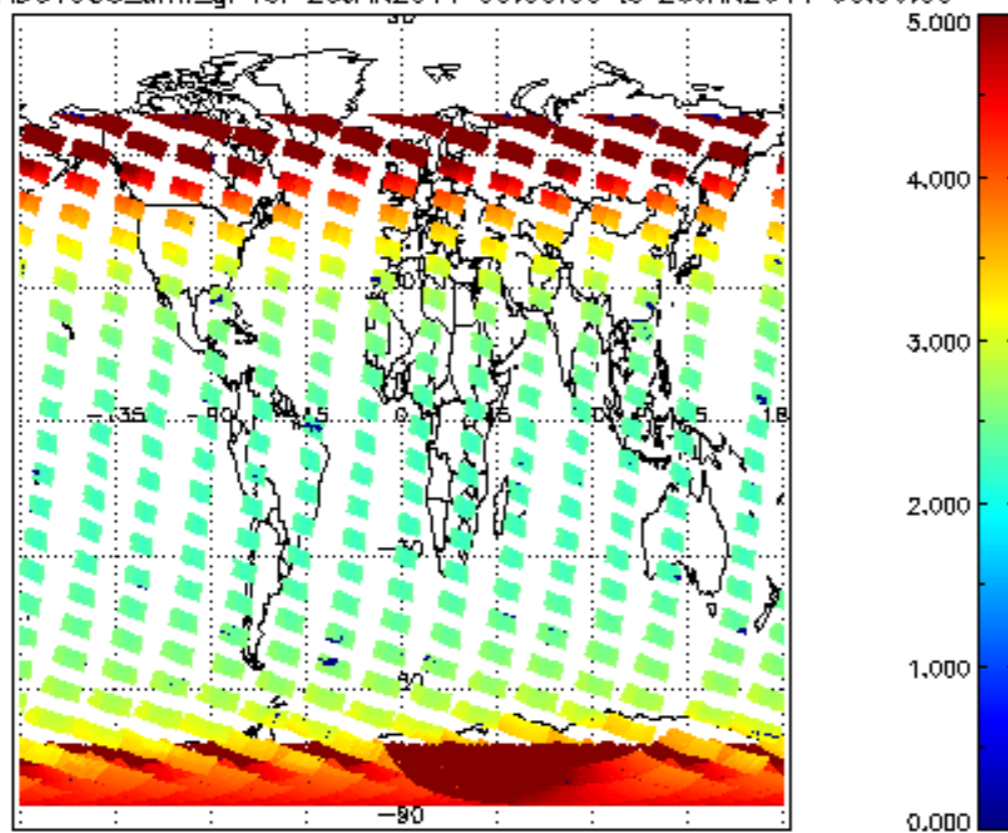
SCIOL2P_NADUV003_amf_gr for 25JAN2011 00:00:00 to 26JAN2011 00:00:00
