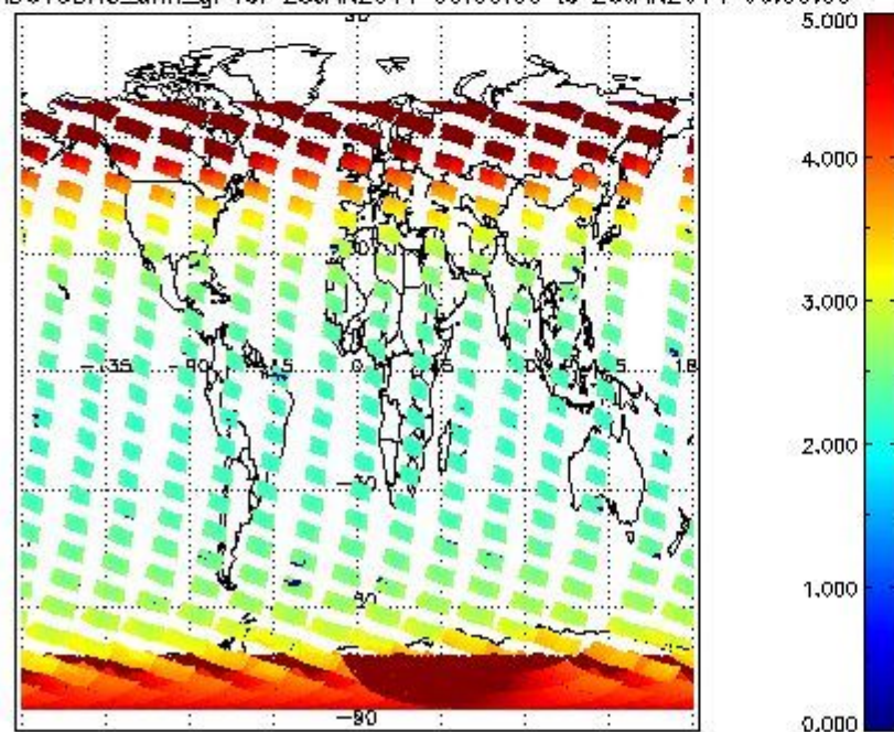
SCIOL2P_NADUV3BRO_amf_gr for 25JAN2011 00:00:00 to 26JAN2011 00:00:00
