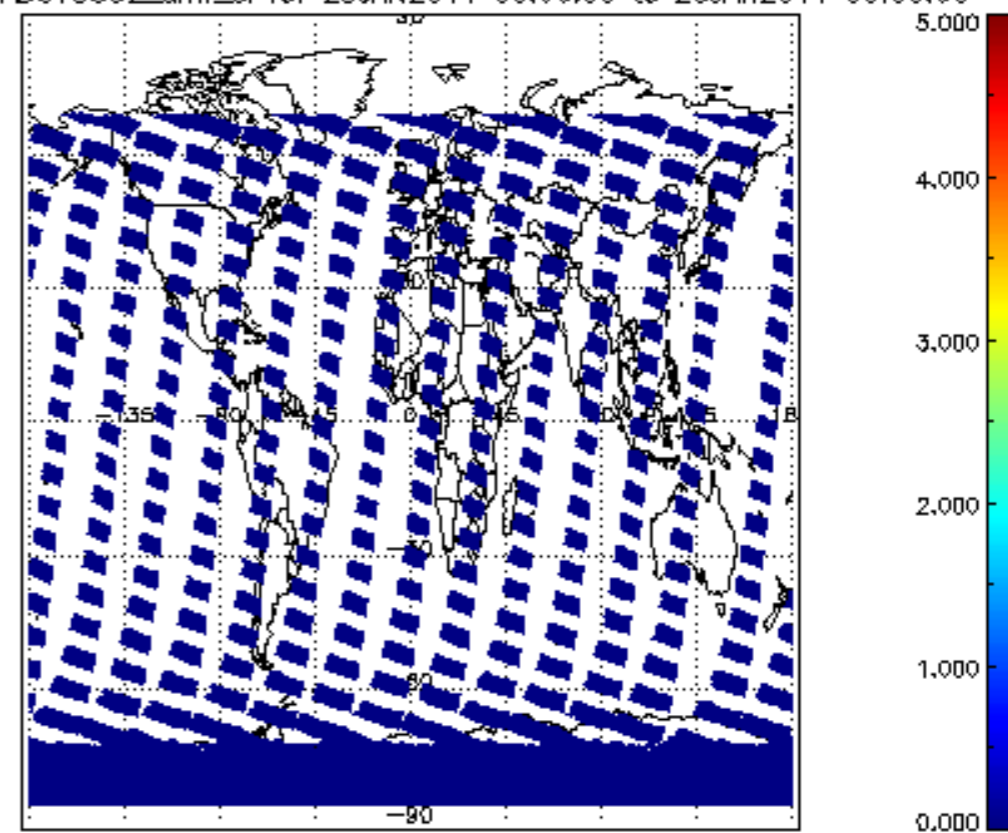
SCIOL2P_NADUV5S02_amf_cl for 25JAN2011 00:00:00 to 26JAN2011 00:00:00
