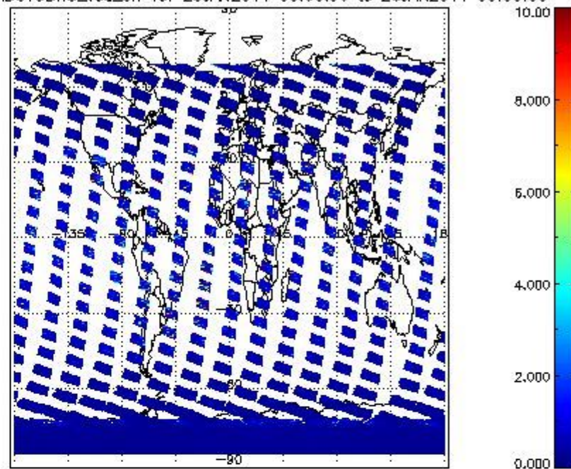
SCIOL2P_NADUV3BRO_vcd_err for 25JAN2011 00:00:00 to 26JAN2011 00:00:00
