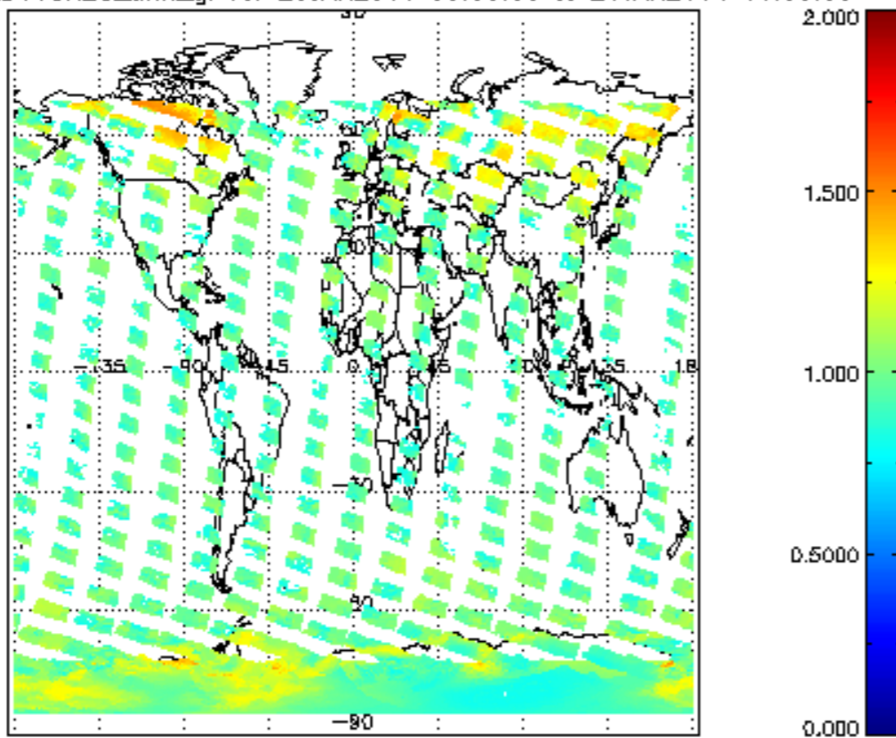
SCIOL2P_NADUV8H20_amf_gr for 25JAN2011 00:00:00 to 26JAN2011 00:00:00
