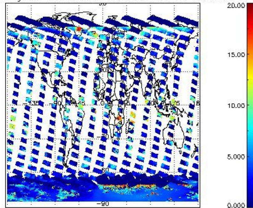
cL_top_height for 25JAN2011 00:00:00 to 26JAN2011 00:00:00
