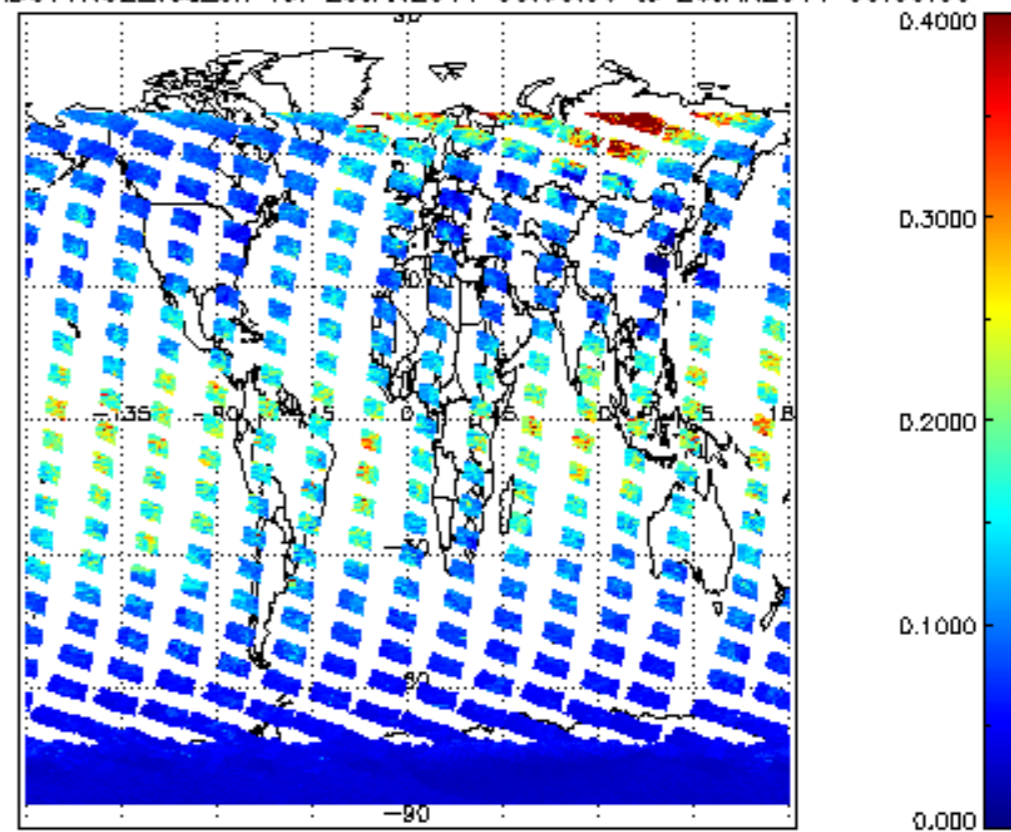
SCIOL2P_NADUV1NO2_vcd_err for 25JAN2011 00:00:00 to 26JAN2011 00:00:00
