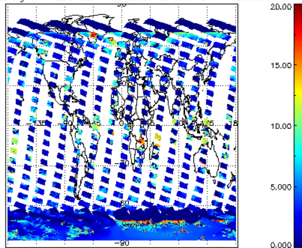
cL_top_height for 25JAN2011 00:00:00 to 26JAN2011 00:00:00
