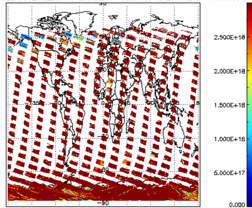
SCIOL2P_NADIR3CO_vcd_err for 25JAN2011 00:00:00 to 26JAN2011 00:00:00
