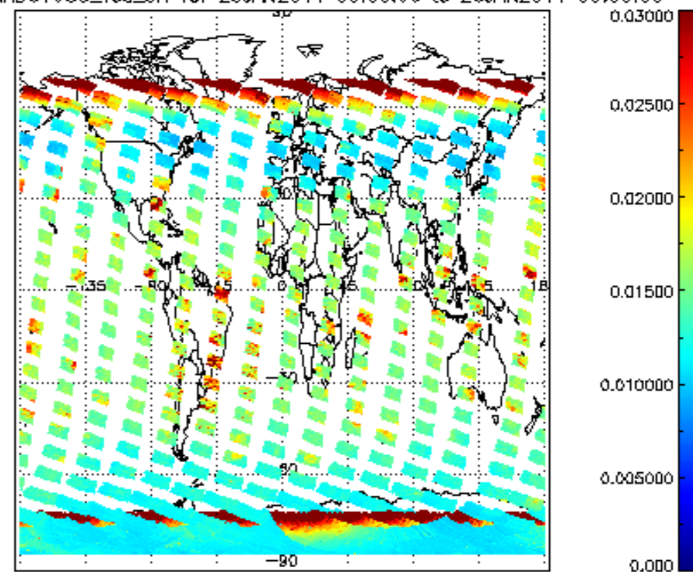
SCIOL2P_NADUV003_vcd_err for 25JAN2011 00:00:00 to 26JAN2011 00:00:00
