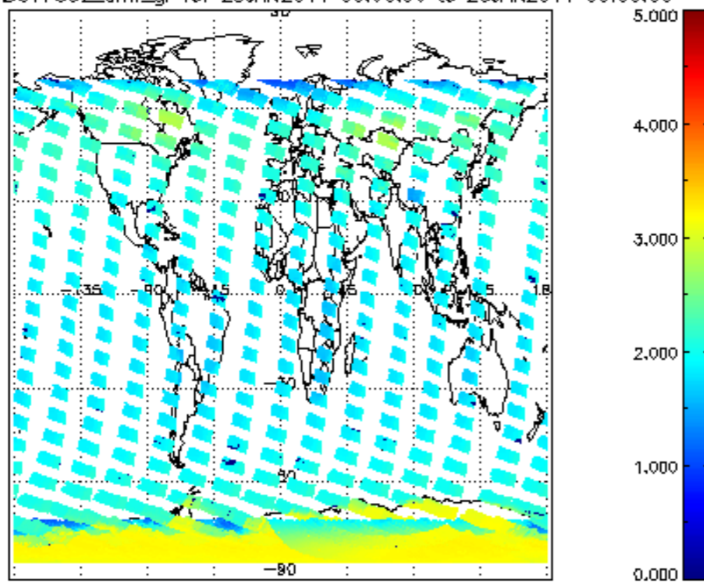
SCIOL2P_NADUV7S02_amf_gr for 25JAN2011 00:00:00 to 26JAN2011 00:00:00
