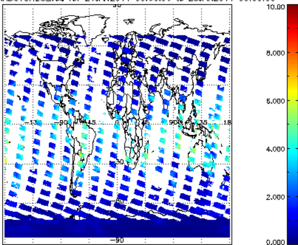
SCIOL2P_NADUV8H20_vcd for 24JAN2011 00:00:00 to 25JAN2011 00:00:00
