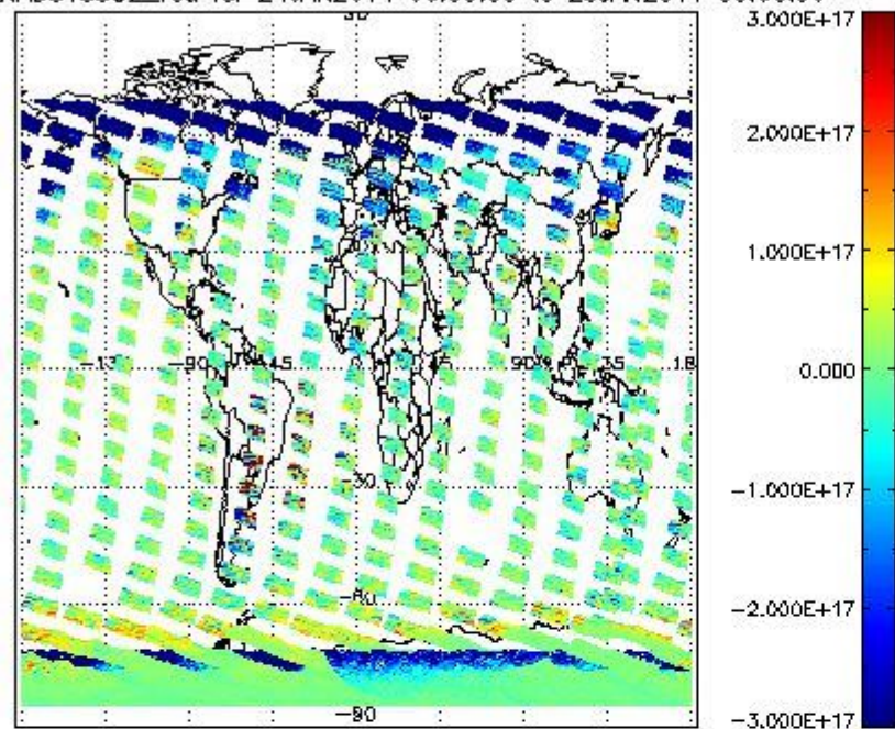
SCIOL2P_NADUV5SO2_vcd for 24JAN2011 00:00:00 to 25JAN2011 00:00:00
