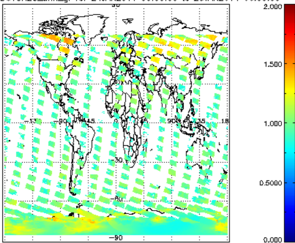
SCIOL2P_NADUV8H20_amf_gr for 24JAN2011 00:00:00 to 25JAN2011 00:00:00
