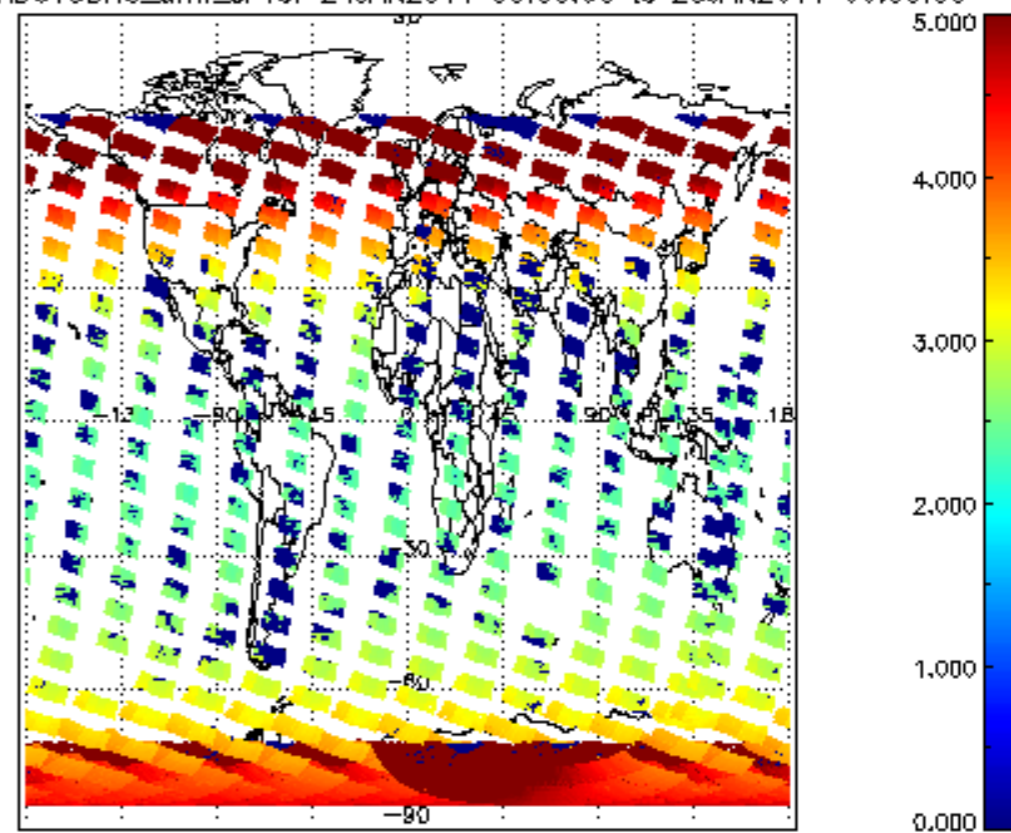
SCIOL2P_NADUV3BRO_amf_cl for 24JAN2011 00:00:00 to 25JAN2011 00:00:00
