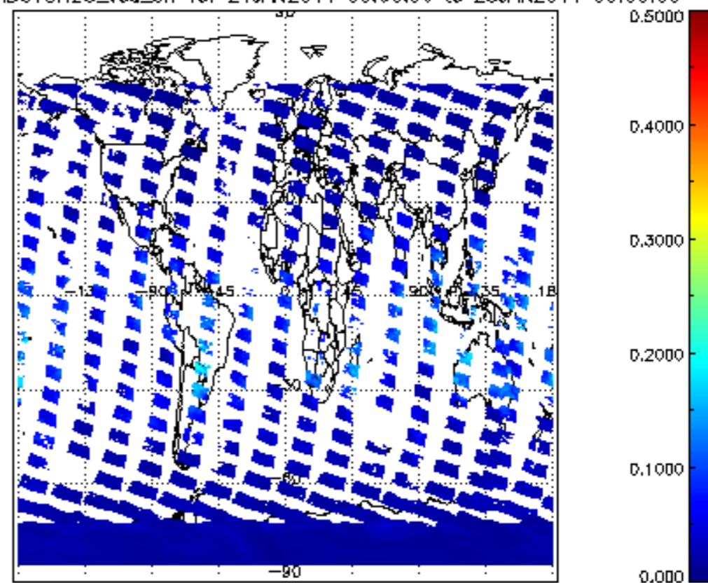
SCIOL2P_NADUV8H20_vcd_err for 24JAN2011 00:00:00 to 25JAN2011 00:00:00
