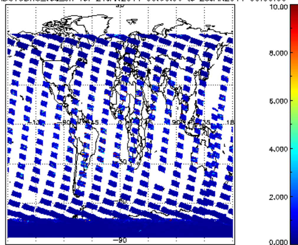
SCIOL2P_NADUV3BRO_vcd_err for 24JAN2011 00:00:00 to 25JAN2011 00:00:00
