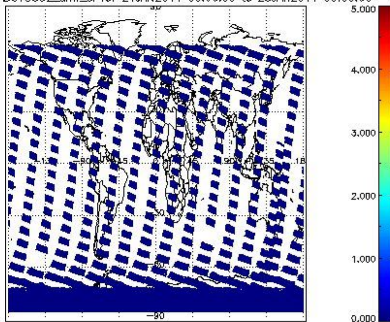
SCIOL2P_NADUV5SO2_amf_cl for 24JAN2011 00:00:00 to 25JAN2011 00:00:00
