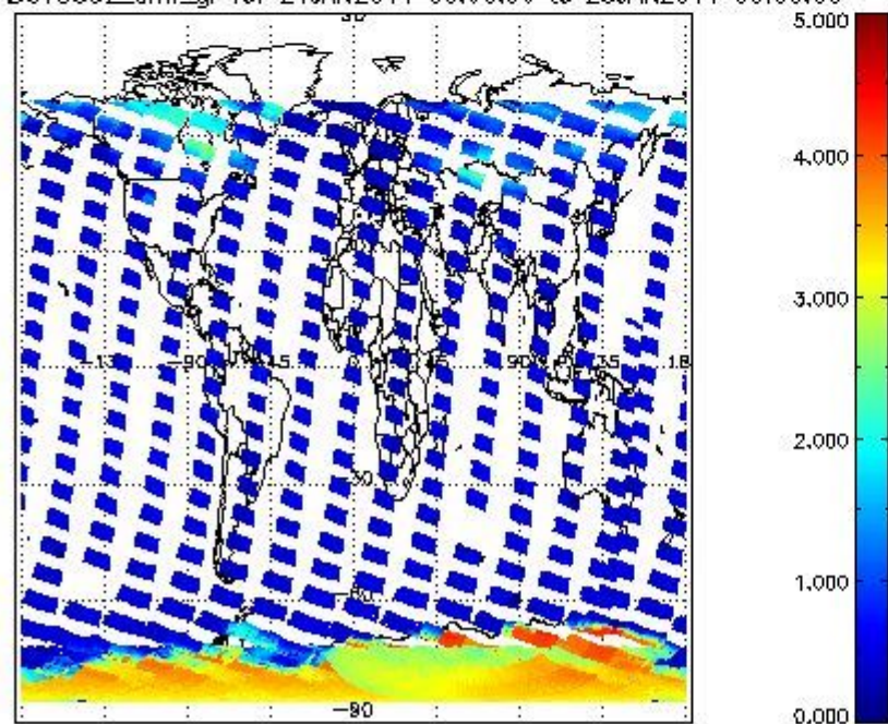
SCIOL2P_NADUV5SO2_amf_gr for 24JAN2011 00:00:00 to 25JAN2011 00:00:00
