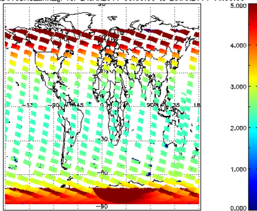
SCIOL2P_NADUV3BRO_amf_gr for 24JAN2011 00:00:00 to 25JAN2011 00:00:00
