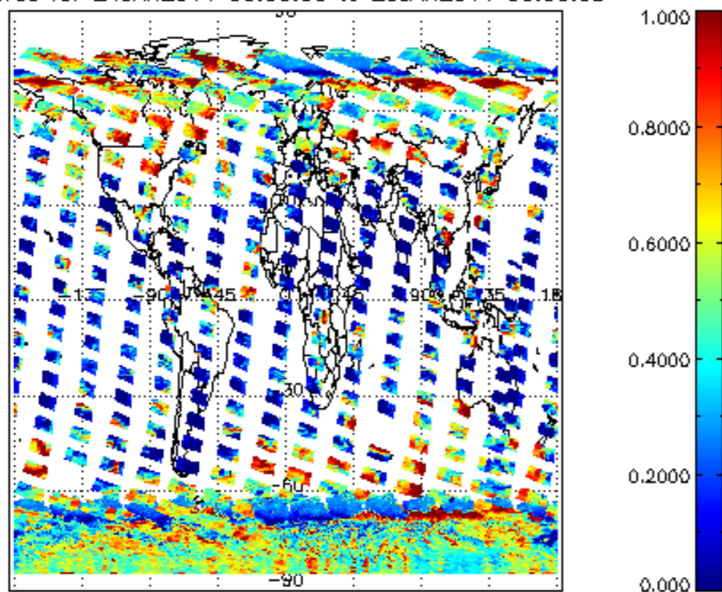
cL_frac for 24JAN2011 00:00:00 to 25JAN2011 00:00:00
