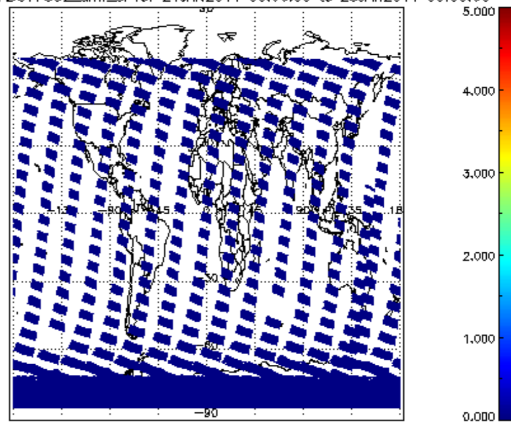
SCIOL2P_NADUV7S02_amf_sl for 24JAN2011 00:00:00 to 25JAN2011 00:00:00
