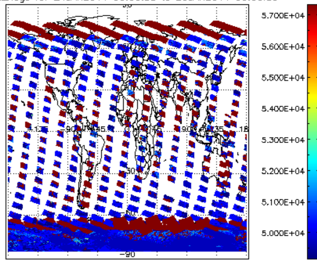
cloud_flags for 24JAN2011 00:00:00 to 25JAN2011 00:00:00
