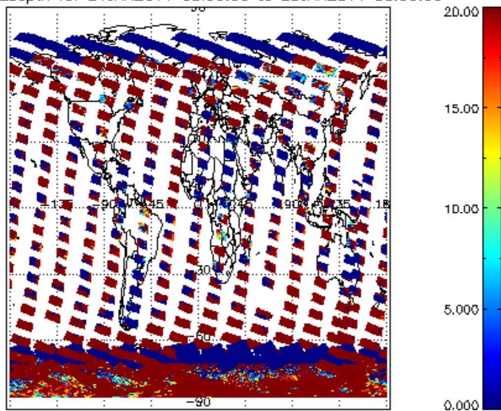
cL_opt_depth for 24JAN2011 00:00:00 to 25JAN2011 00:00:00
