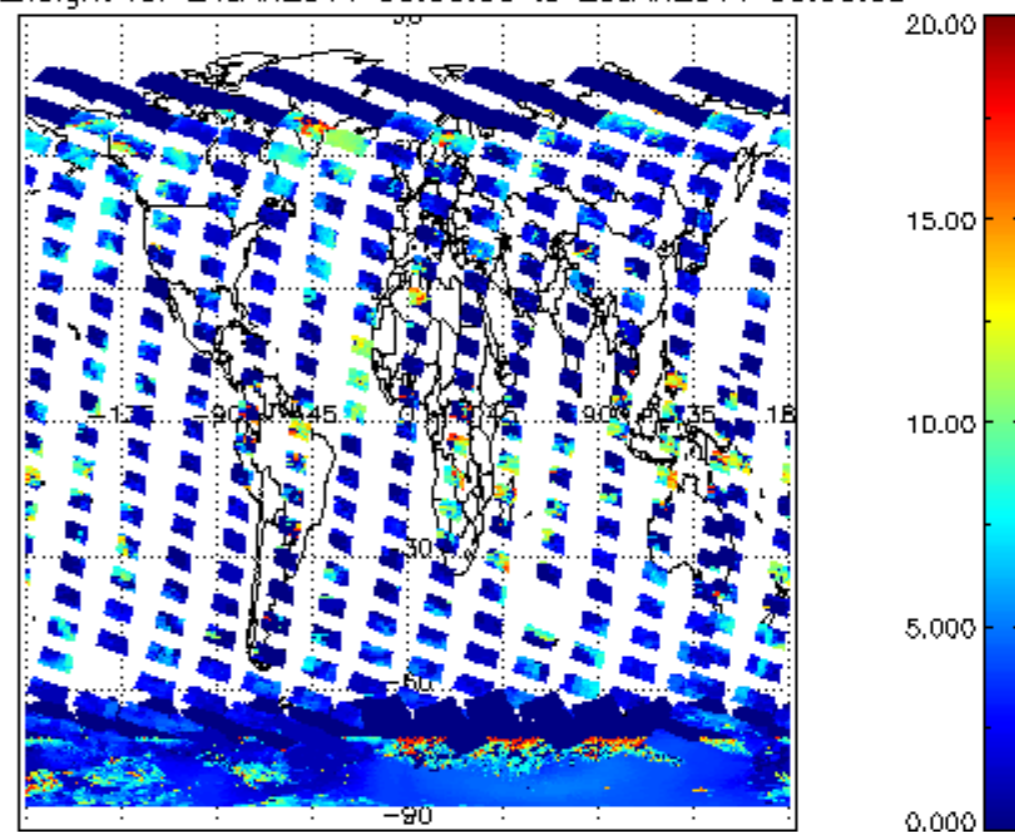
cL_top_height for 24JAN2011 00:00:00 to 25JAN2011 00:00:00
