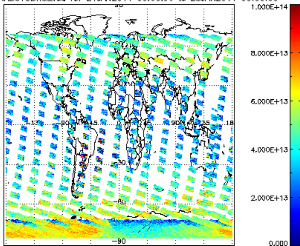
SCIOL2P_NADUV3BRO_vcd for 24JAN2011 00:00:00 to 25JAN2011 00:00:00
