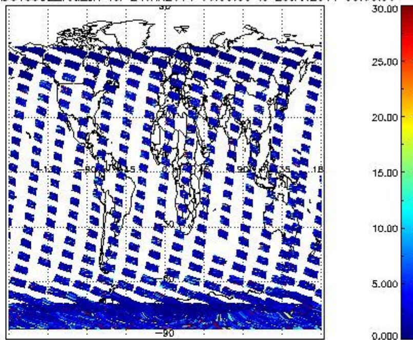
SCIOL2P_NADUV5SO2_vcd_err for 24JAN2011 00:00:00 to 25JAN2011 00:00:00
