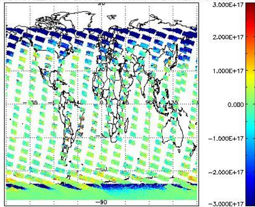
SCIOL2P_NADUV5S02_vcd for 23JAN2011 00:00:00 to 24JAN2011 00:00:00
