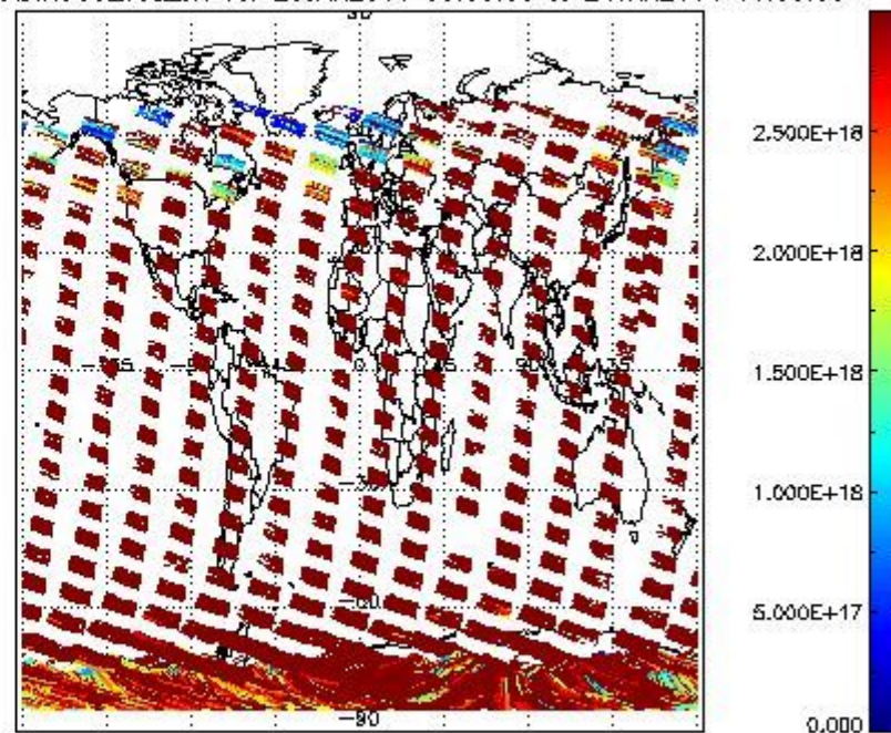
SCIDL2P_NADIR3CO_vcd_err for 23JAN2011 00:00:00 to 24JAN2011 00:00:00
