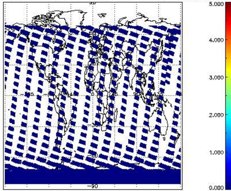
SCIOL2P_NADUV5S02_amf_cl for 23JAN2011 00:00:00 to 24JAN2011 00:00:00
