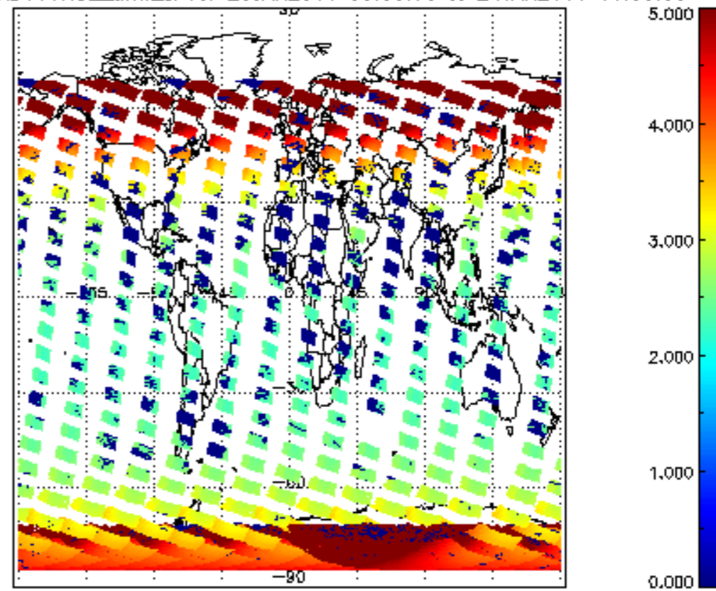
SCIOL2P_NADUV1NO2_amf_cl for 23JAN2011 00:00:00 to 24JAN2011 00:00:00
