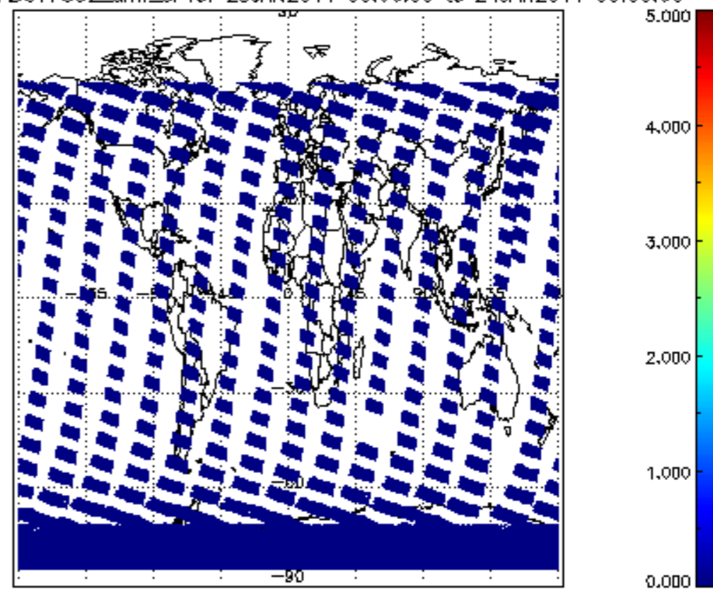
SCIOL2P_NADUV7S02_amf_sl for 23JAN2011 00:00:00 to 24JAN2011 00:00:00
