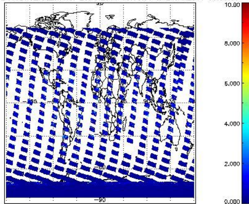
SCIOL2P_NADUV3BRO_vcd_err for 23JAN2011 00:00:00 to 24JAN2011 00:00:00
