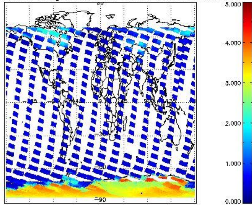
SCIOL2P_NADUV5S02_amf_gr for 23JAN2011 00:00:00 to 24JAN2011 00:00:00
