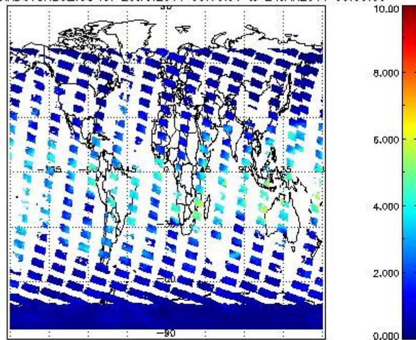
SCIOL2P_NADUV8H20_vcd for 23JAN2011 00:00:00 to 24JAN2011 00:00:00
