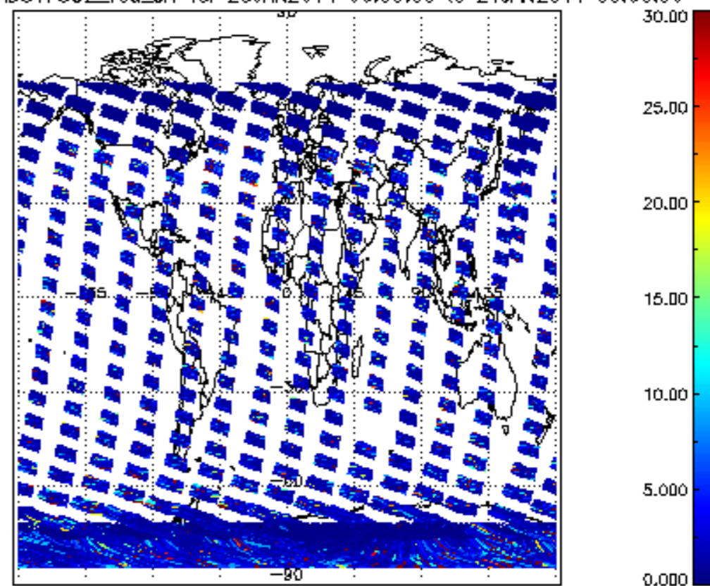
SCIOL2P_NADUV7S02_vcd_err for 23JAN2011 00:00:00 to 24JAN2011 00:00:00
