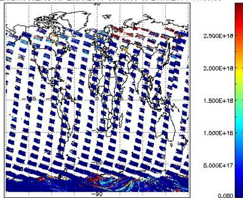
SCIDL2P_NADIR3CO_vcd for 23JAN2011 00:00:00 to 24JAN2011 00:00:00
