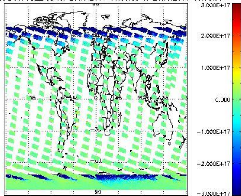
SCIOL2P_NADUV7S02_vcd for 23JAN2011 00:00:00 to 24JAN2011 00:00:00
