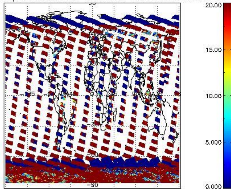
cLopt_depth for 23JAN2011 00:00:00 to 24JAN2011 00:00:00
