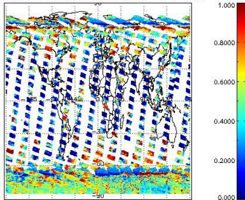
cL_frac for 23JAN2011 00:00:00 to 24JAN2011 00:00:00
