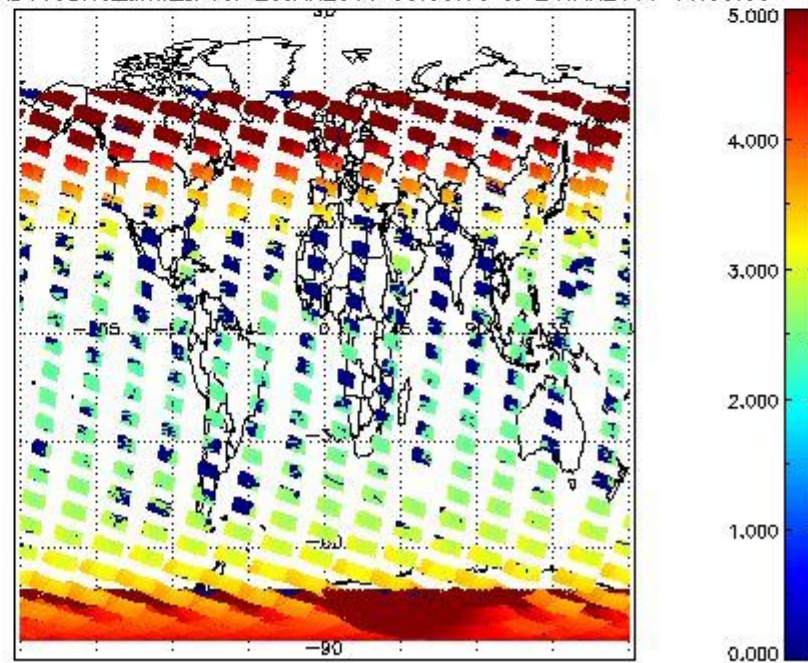
SCIOL2P_NADUV3BRO_amf_cl for 23JAN2011 00:00:00 to 24JAN2011 00:00:00
