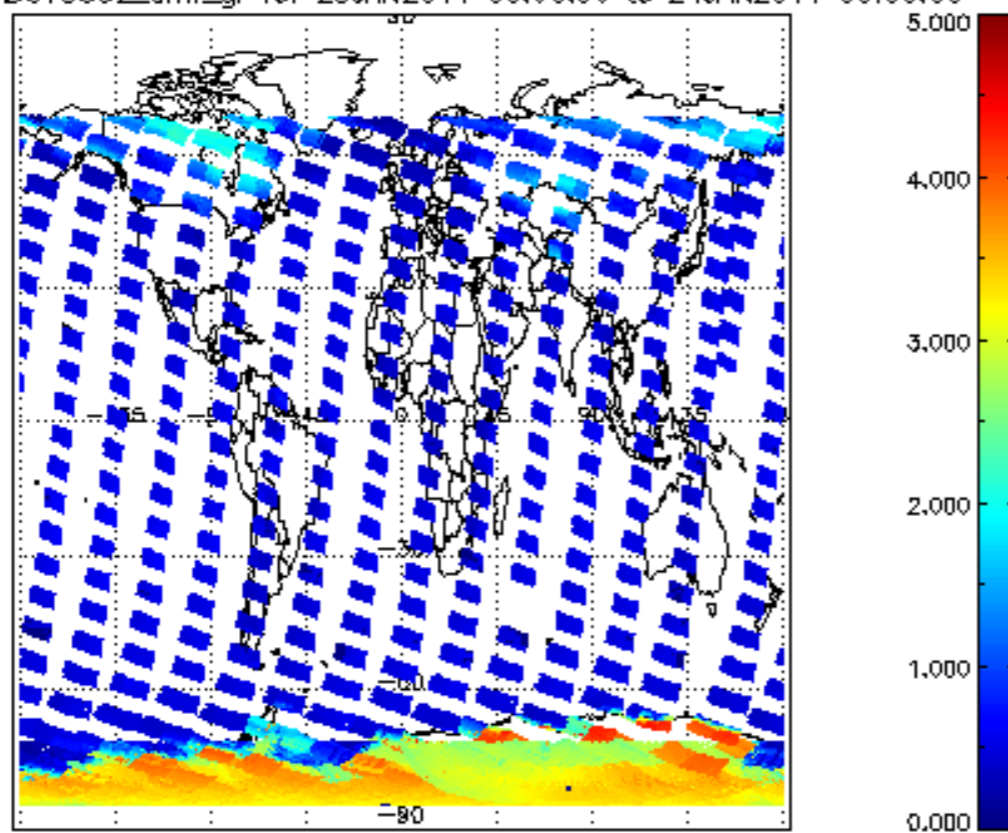
SCIOL2P_NADUV5S02_amf_gr for 23JAN2011 00:00:00 to 24JAN2011 00:00:00
