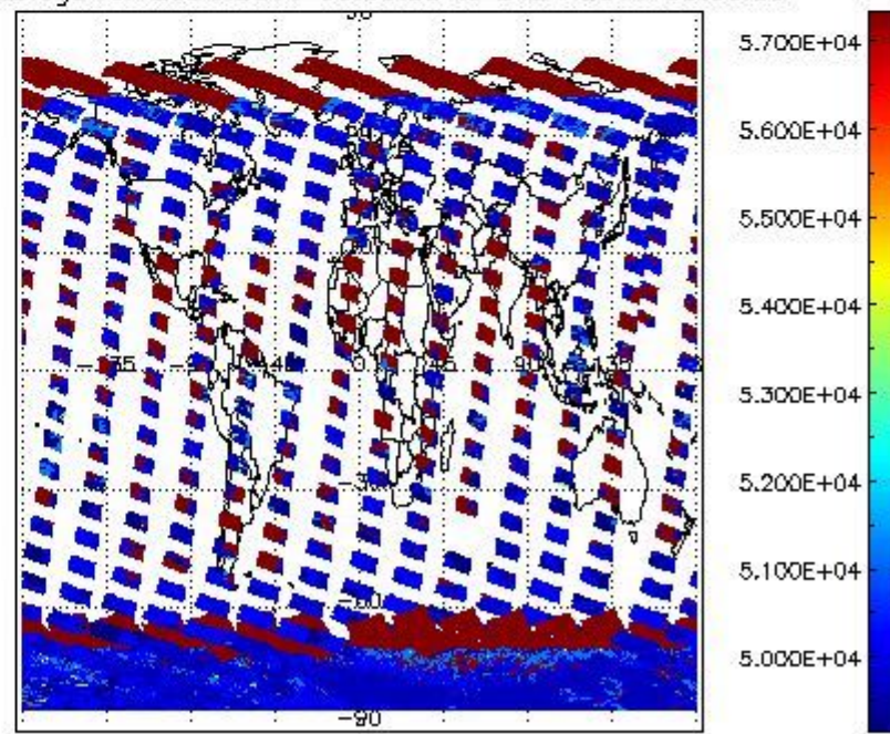
cloud_flags for 23JAN2011 00:00:00 to 24JAN2011 00:00:00
