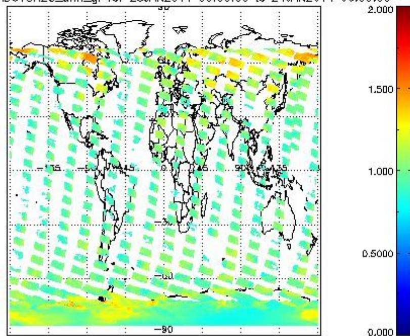
SCIOL2P_NADUV8H20_amf_gr for 23JAN2011 00:00:00 to 24JAN2011 00:00:00
