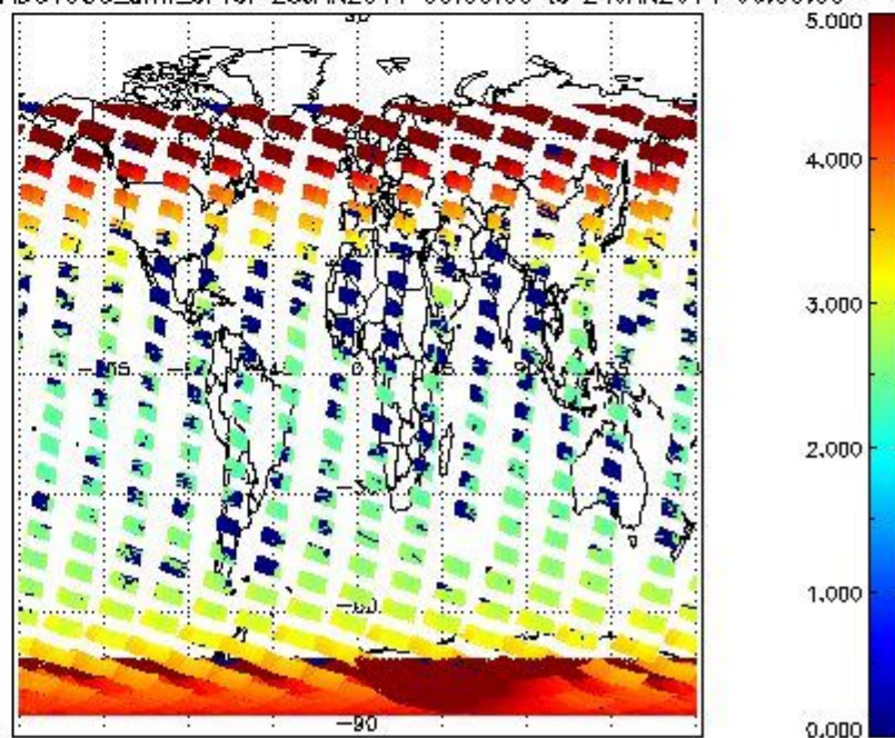
SCIOL2P_NADUV003_amf_cl for 23JAN2011 00:00:00 to 24JAN2011 00:00:00
