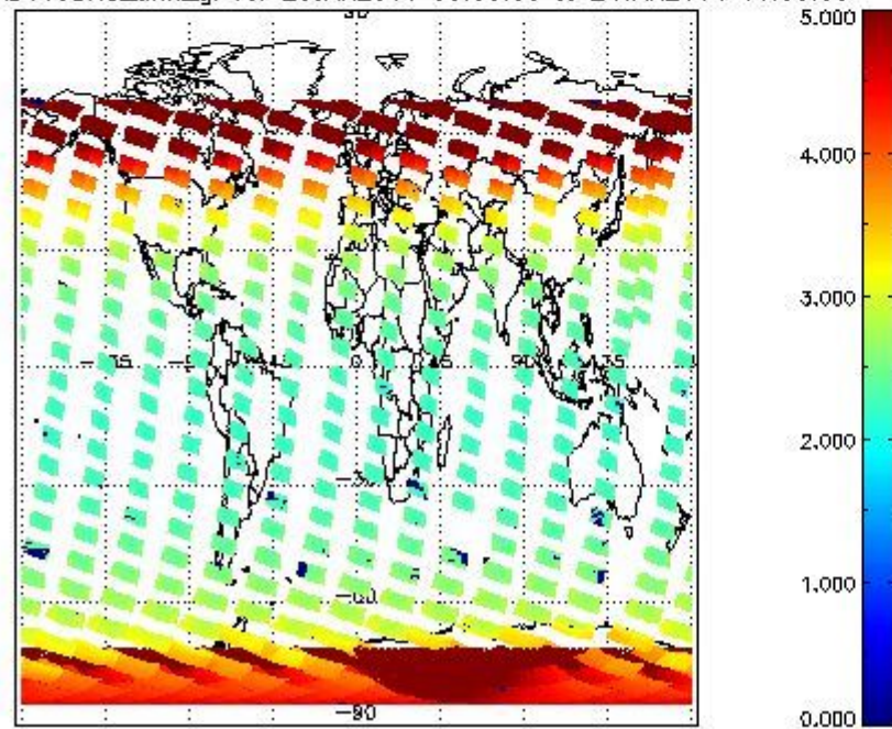
SCIOL2P_NADUV3BRO_amf_gr for 23JAN2011 00:00:00 to 24JAN2011 00:00:00
