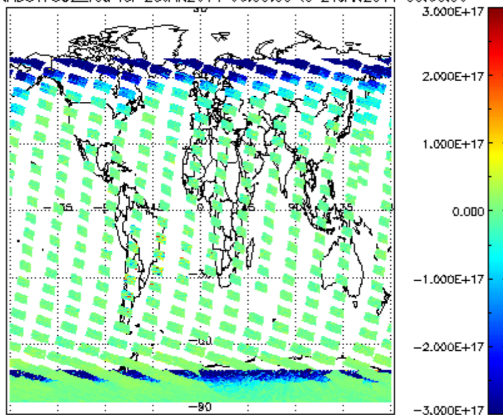
SCIOL2P_NADUV7S02_vcd for 23JAN2011 00:00:00 to 24JAN2011 00:00:00
