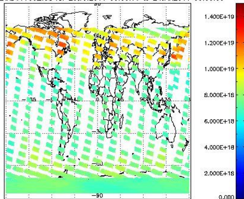
SCIOL2P_NADUV003_vcd for 23JAN2011 00:00:00 to 24JAN2011 00:00:00
