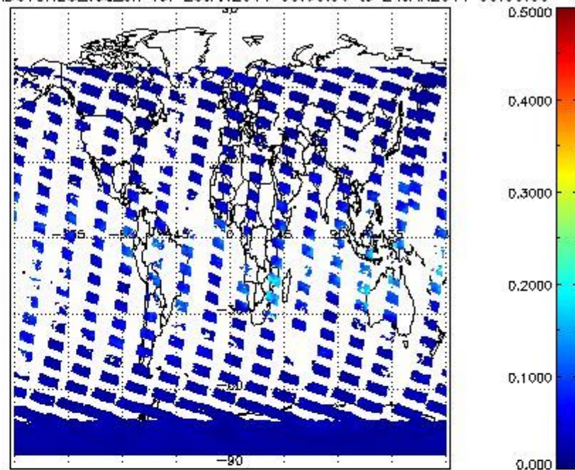
SCIOL2P_NADUV8H20_vcd_err for 23JAN2011 00:00:00 to 24JAN2011 00:00:00
