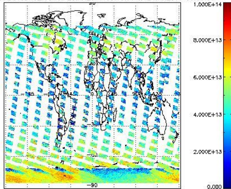
SCIOL2P_NADUV3BRO_vcd for 23JAN2011 00:00:00 to 24JAN2011 00:00:00
