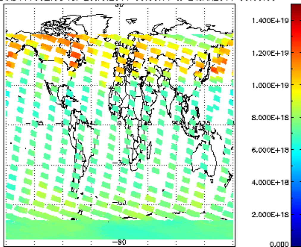
SCIOL2P_NADUV003_vcd for 23JAN2011 00:00:00 to 24JAN2011 00:00:00
