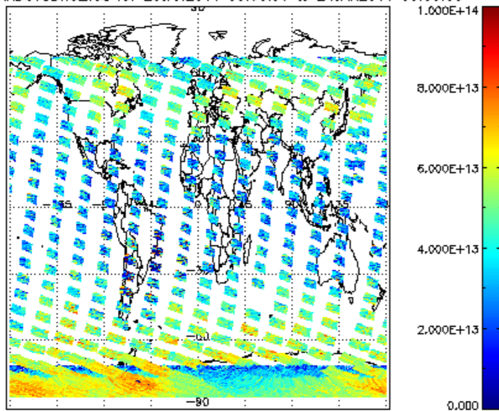
SCIOL2P_NADUV3BRO_vcd for 23JAN2011 00:00:00 to 24JAN2011 00:00:00
