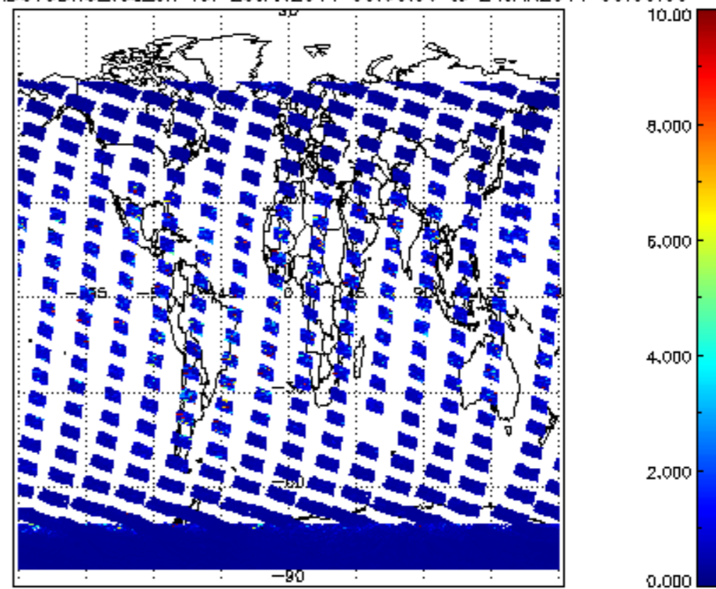
SCIOL2P_NADUV3BRO_vcd_err for 23JAN2011 00:00:00 to 24JAN2011 00:00:00
