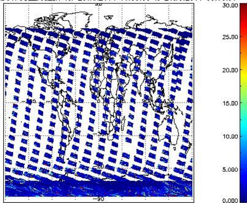
SCIOL2P_NADUV7S02_vcd_err for 23JAN2011 00:00:00 to 24JAN2011 00:00:00
