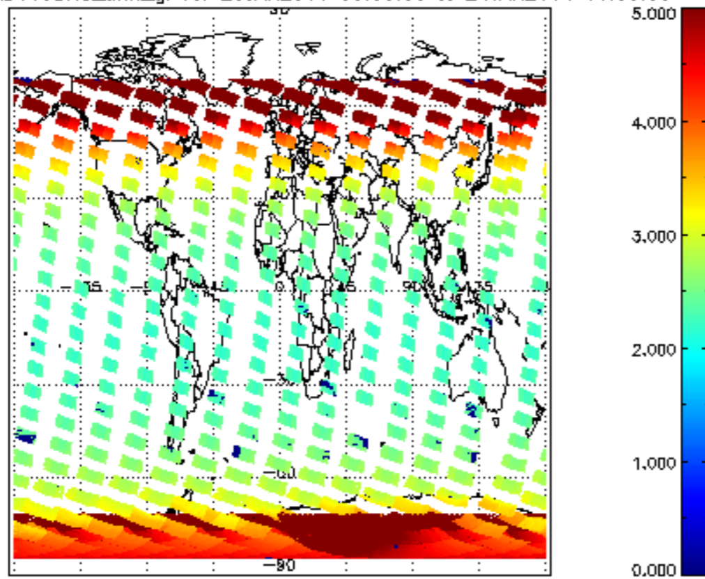
SCIOL2P_NADUV3BRO_amf_gr for 23JAN2011 00:00:00 to 24JAN2011 00:00:00
