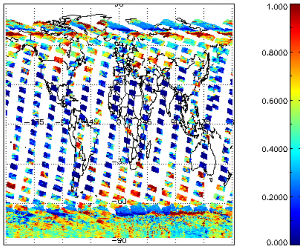
cL_frac for 23JAN2011 00:00:00 to 24JAN2011 00:00:00
