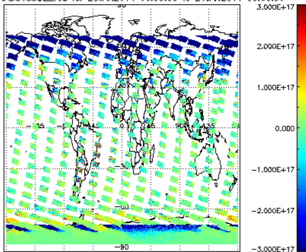
SCIOL2P_NADUV5S02_vcd for 23JAN2011 00:00:00 to 24JAN2011 00:00:00
