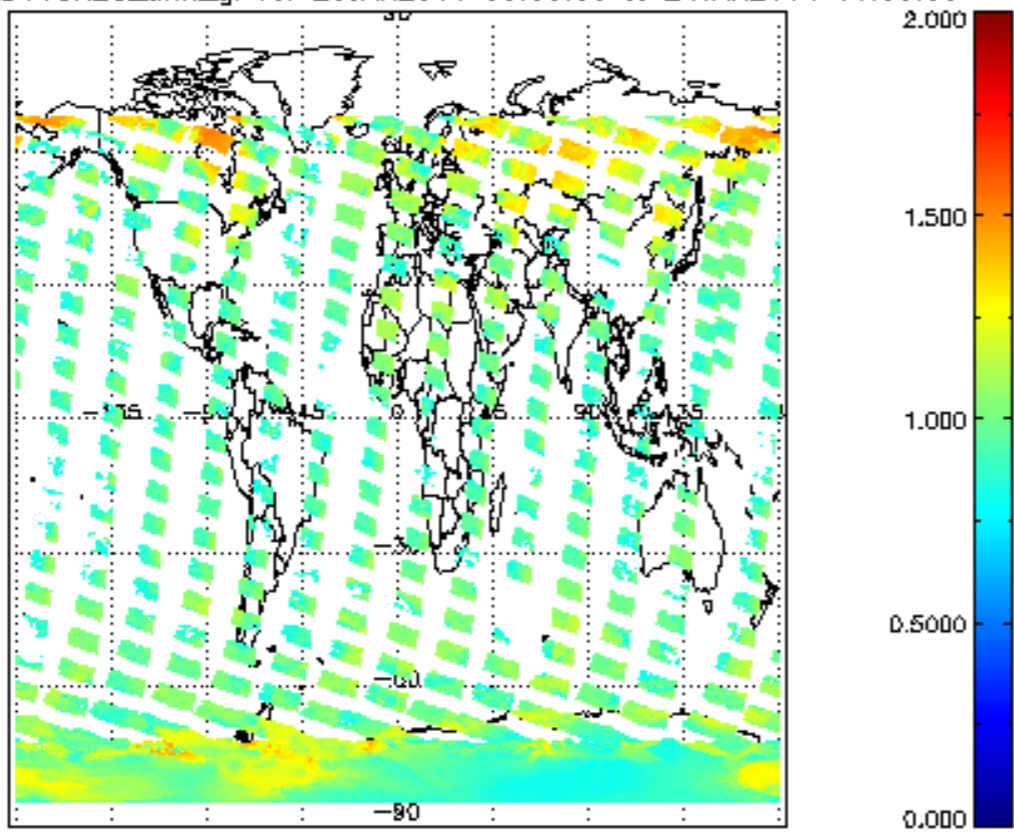
SCIOL2P_NADUVBH20_amf_gr for 23JAN2011 00:00:00 to 24JAN2011 00:00:00
