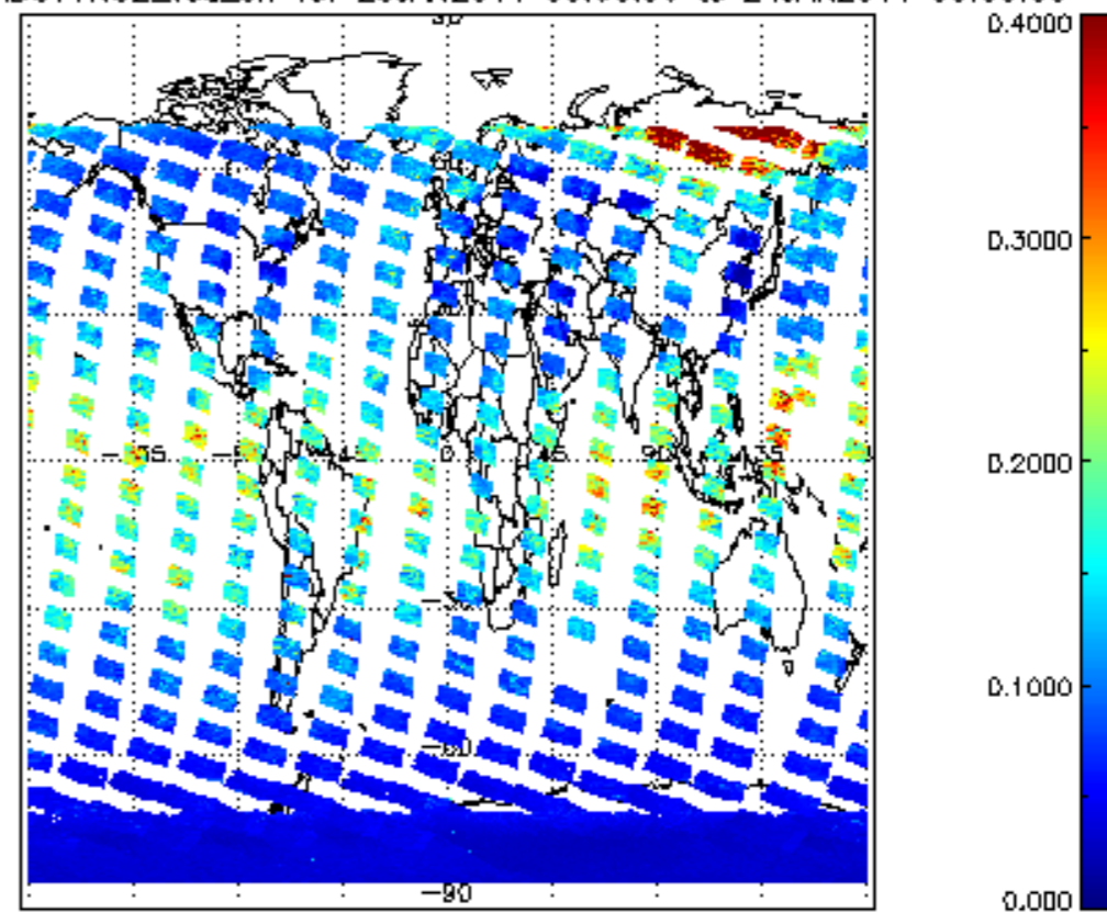
SCIOL2P_NADUV1NO2_vcd_err for 23JAN2011 00:00:00 to 24JAN2011 00:00:00
