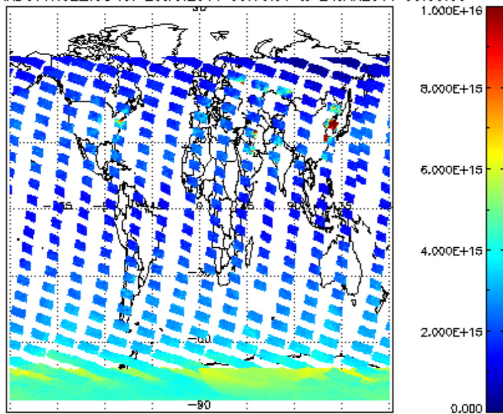
SCIOL2P_NADUV1NO2_vcd for 23JAN2011 00:00:00 to 24JAN2011 00:00:00
