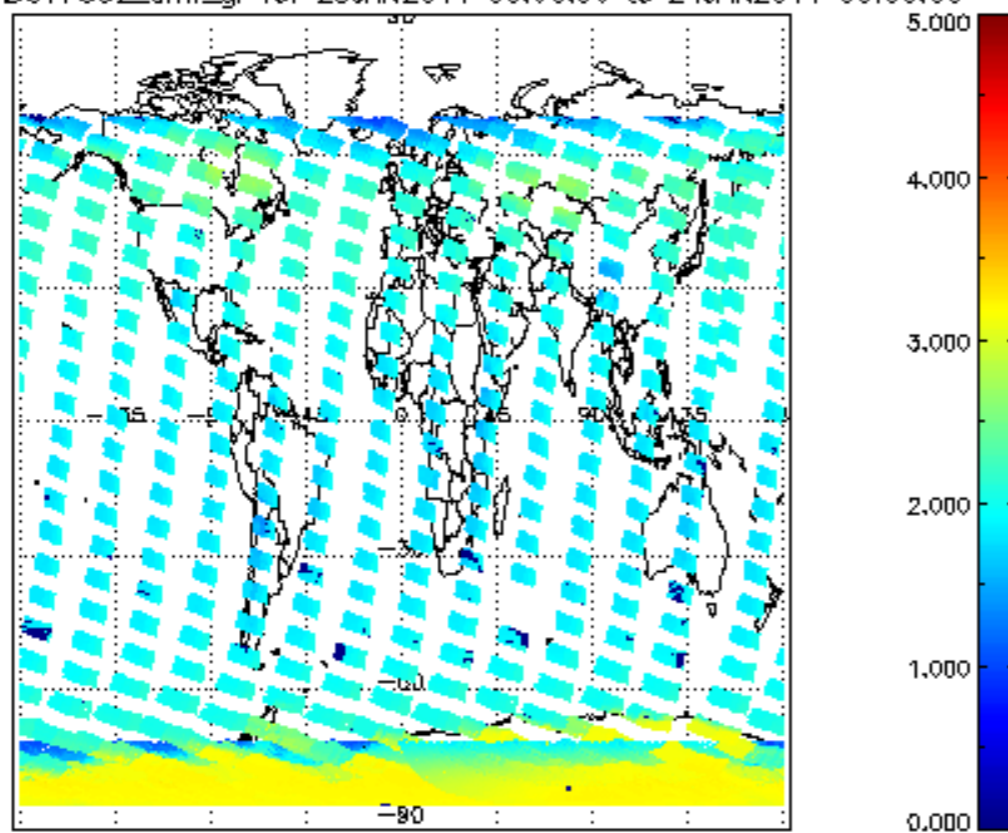
SCIOL2P_NADUV7S02_amf_gr for 23JAN2011 00:00:00 to 24JAN2011 00:00:00
