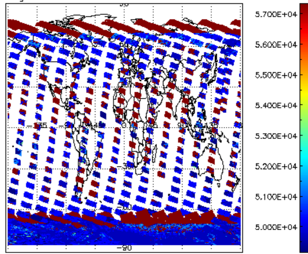
cloud_flags for 23JAN2011 00:00:00 to 24JAN2011 00:00:00
