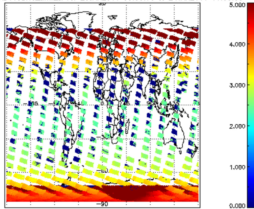
SCIOL2P_NADUV3BRO_amf_cl for 23JAN2011 00:00:00 to 24JAN2011 00:00:00
