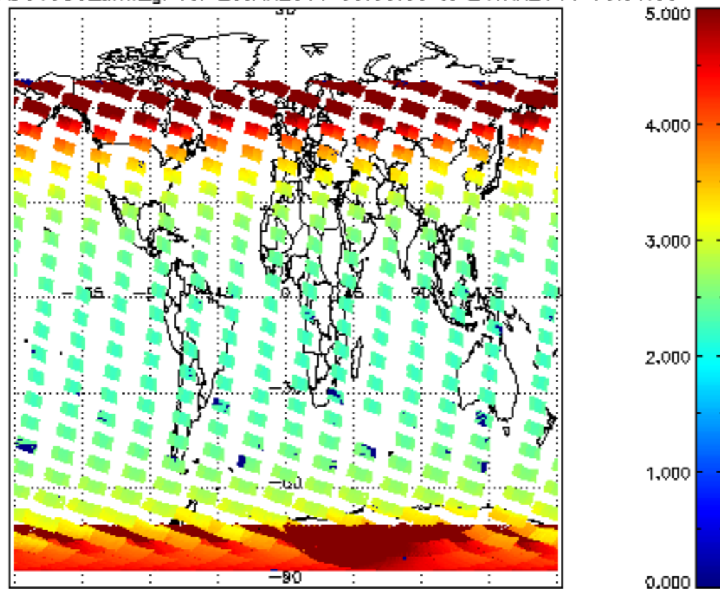
SCIOL2P_NADUV003_amf_gr for 23JAN2011 00:00:00 to 24JAN2011 00:00:00
