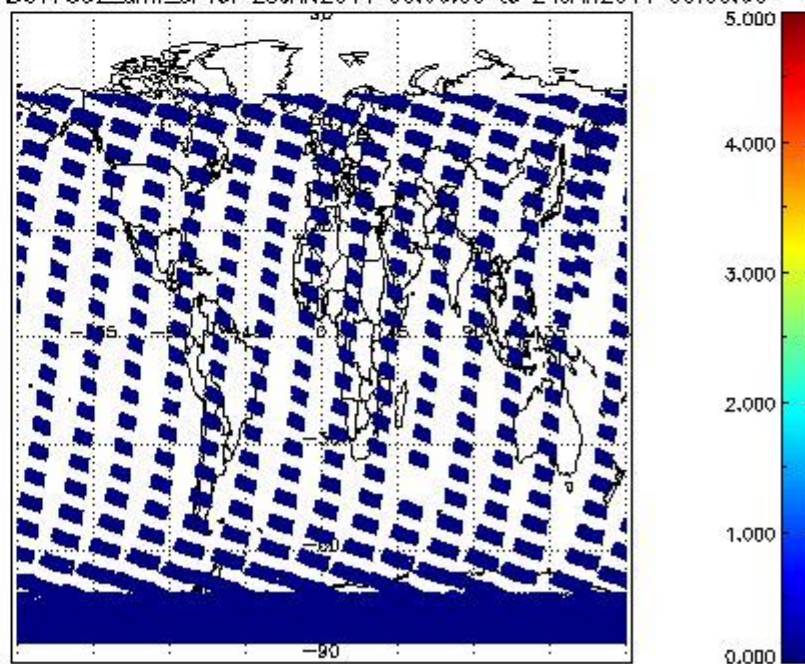
SCIOL2P_NADUV7S02_amf_cl for 23JAN2011 00:00:00 to 24JAN2011 00:00:00
