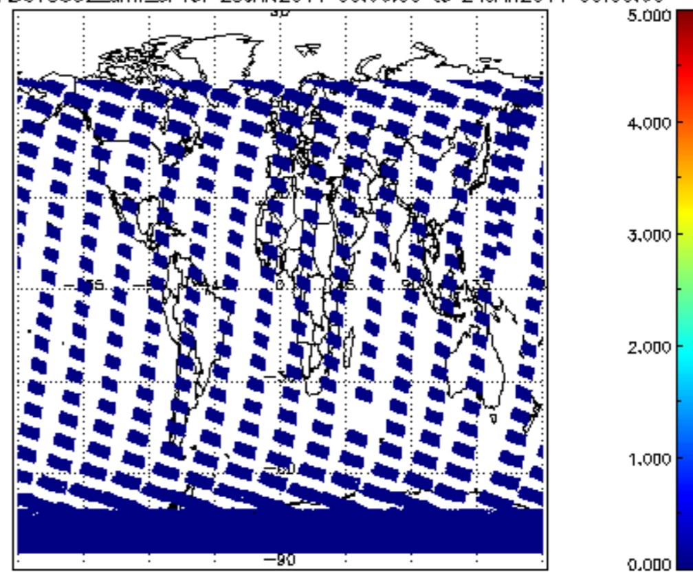
SCIOL2P_NADUV5S02_amf_cl for 23JAN2011 00:00:00 to 24JAN2011 00:00:00
