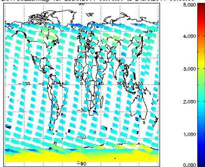
SCIOL2P_NADUV7S02_amf_gr for 23JAN2011 00:00:00 to 24JAN2011 00:00:00
