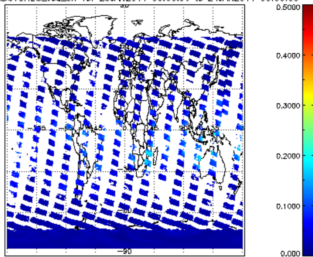
SCIOL2P_NADUVBH20_vcd_err for 23JAN2011 00:00:00 to 24JAN2011 00:00:00
