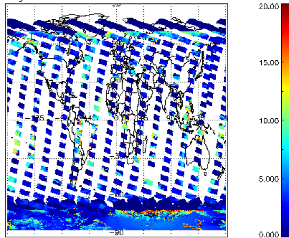
cL_top_height for 23JAN2011 00:00:00 to 24JAN2011 00:00:00
