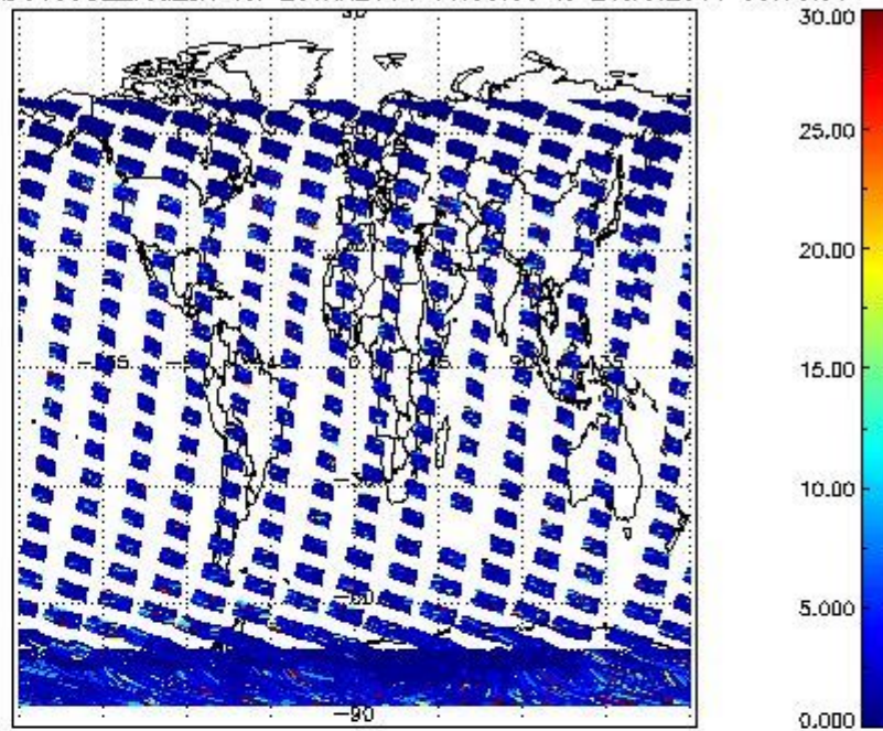
SCIOL2P_NADUV5S02_vcd_err for 23JAN2011 00:00:00 to 24JAN2011 00:00:00
