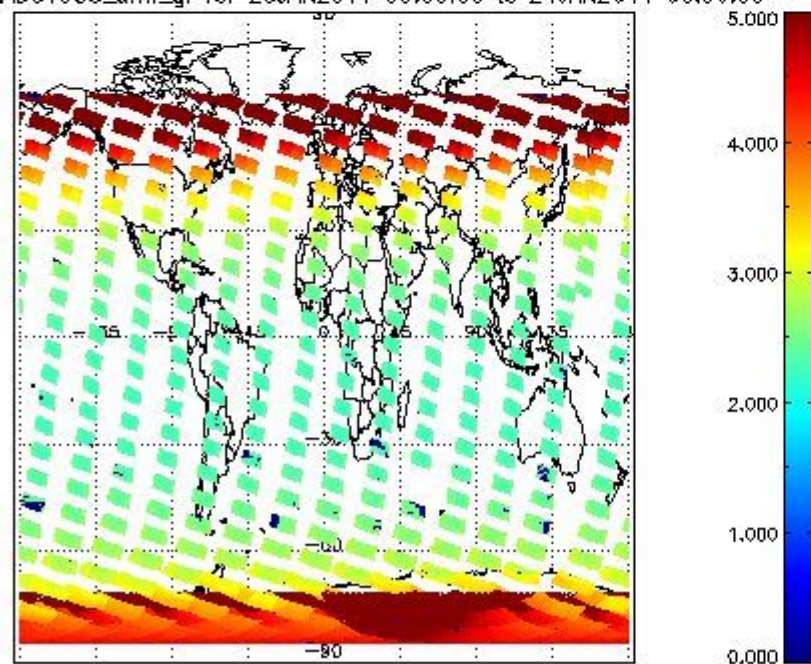
SCIOL2P_NADUV003_amf_gr for 23JAN2011 00:00:00 to 24JAN2011 00:00:00
