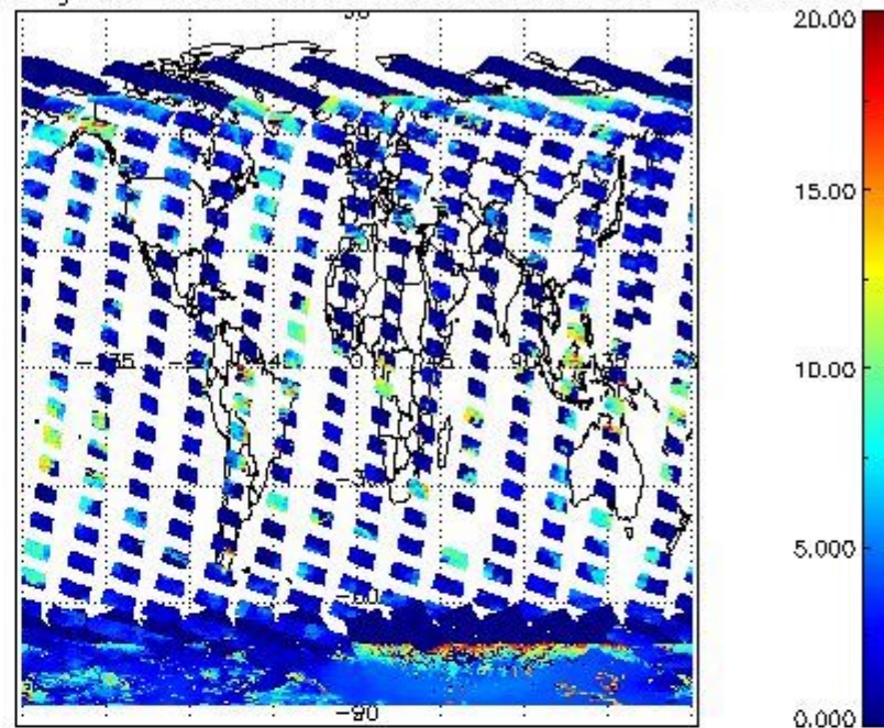
cL_top_height for 23JAN2011 00:00:00 to 24JAN2011 00:00:00
