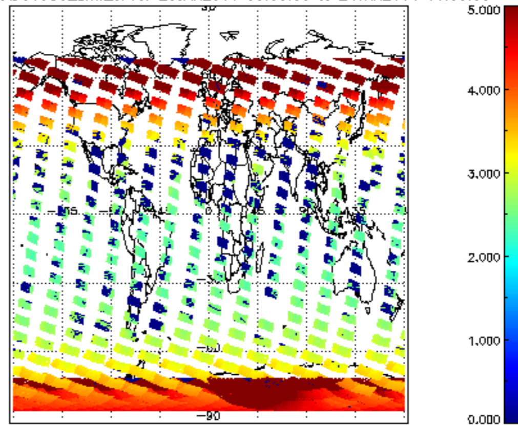
SCIOL2P_NADUV003_amf_cl for 23JAN2011 00:00:00 to 24JAN2011 00:00:00
