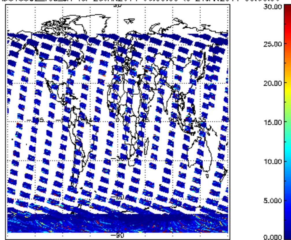
SCIOL2P_NADUV5S02_vcd_err for 23JAN2011 00:00:00 to 24JAN2011 00:00:00
