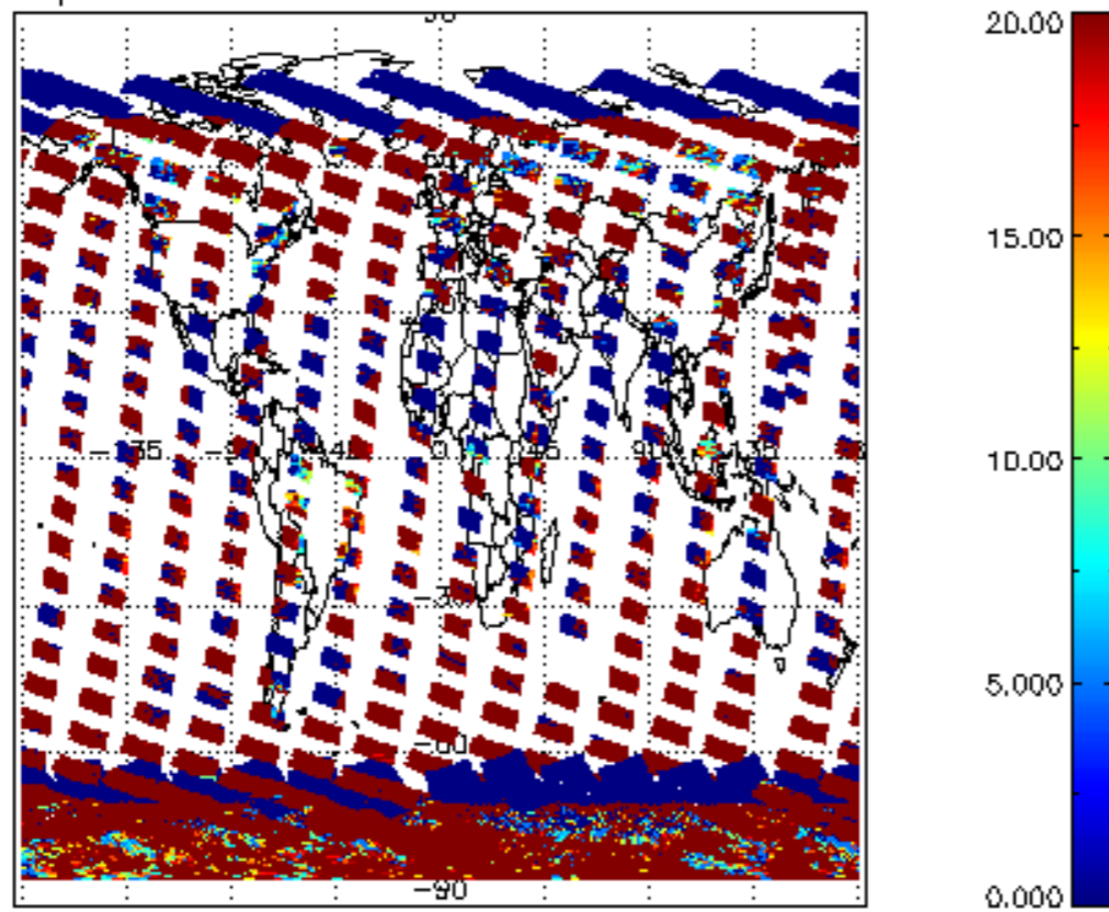
cLopt_depth for 23JAN2011 00:00:00 to 24JAN2011 00:00:00
