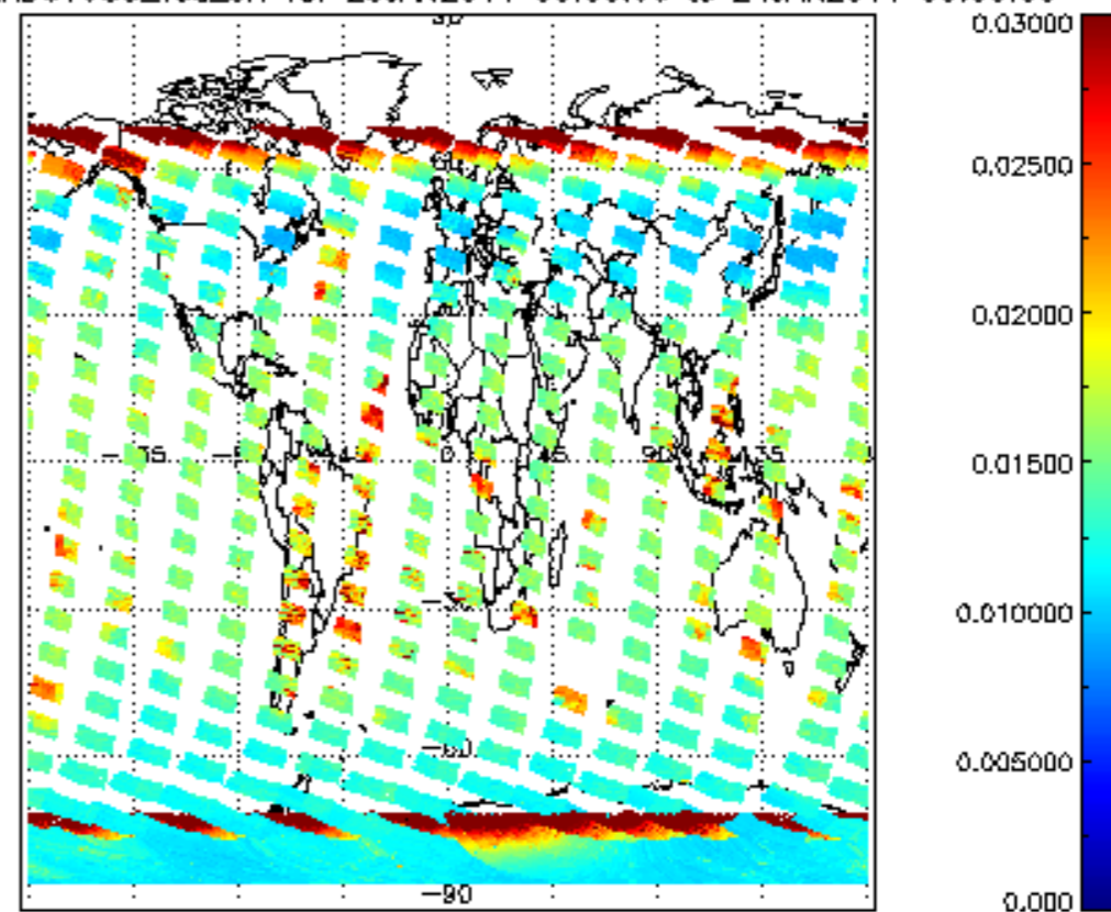
SCIOL2P_NADUV003_vcd_err for 23JAN2011 00:00:00 to 24JAN2011 00:00:00
