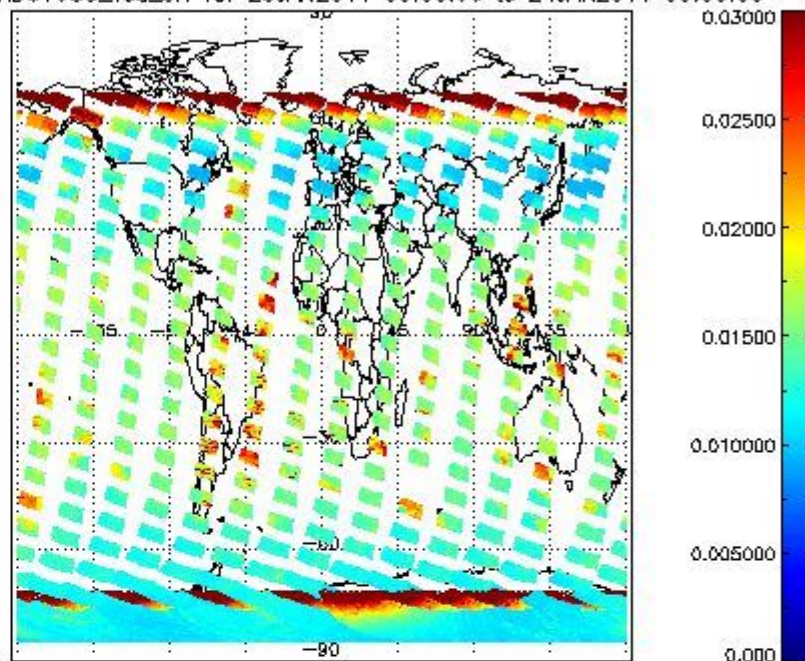
SCIOL2P_NADUV003_vcd_err for 23JAN2011 00:00:00 to 24JAN2011 00:00:00
