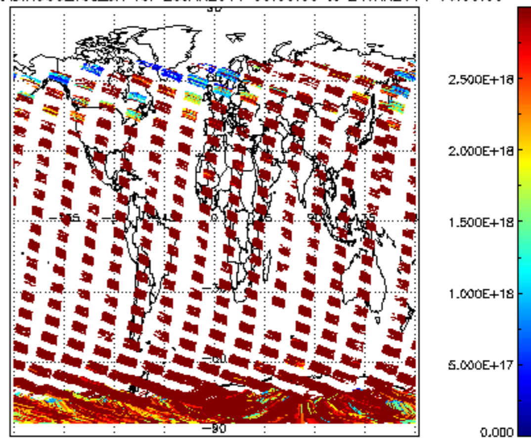
SCIOL2P_NADIR3CO_vcd_err for 23JAN2011 00:00:00 to 24JAN2011 00:00:00
