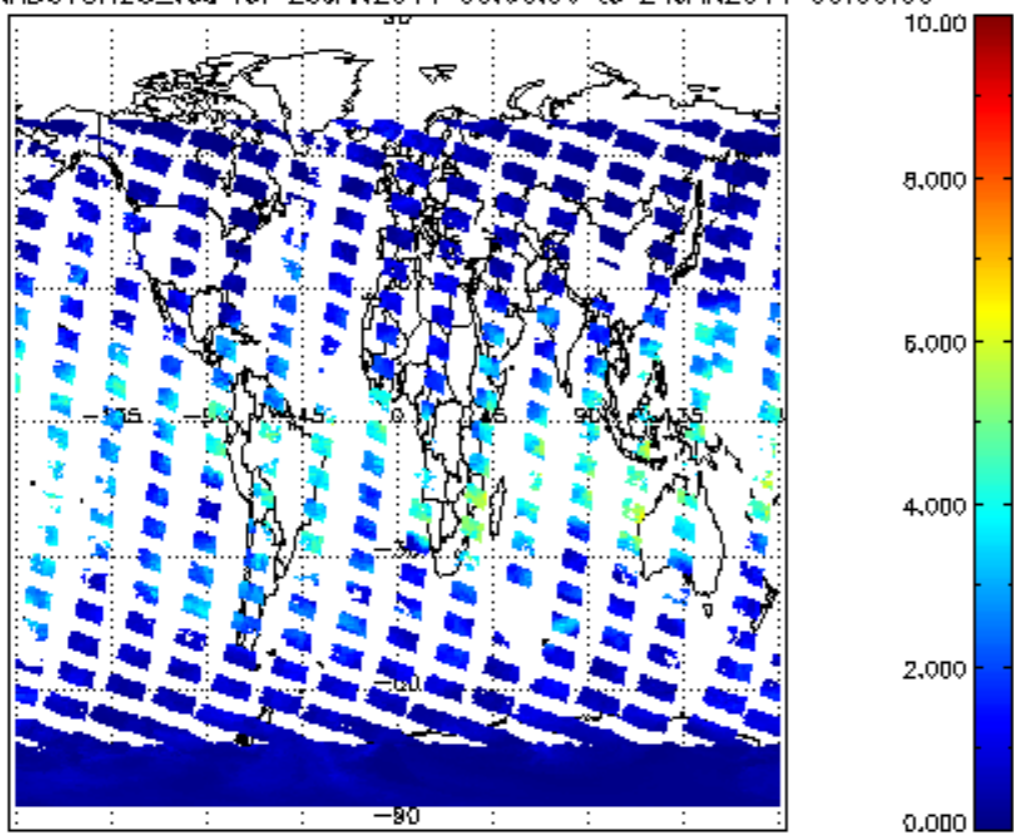
SCIOL2P_NADUVBH20_vcd for 23JAN2011 00:00:00 to 24JAN2011 00:00:00
