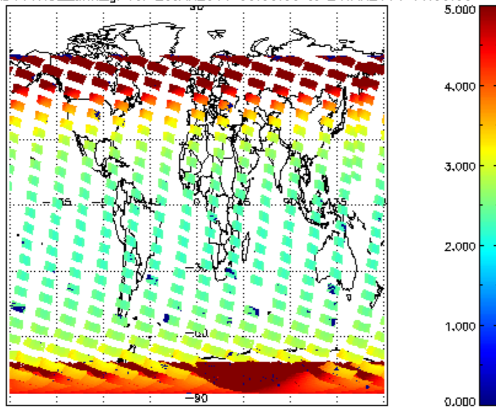
SCIOL2P_NADUV1NO2_amf_gr for 23JAN2011 00:00:00 to 24JAN2011 00:00:00
