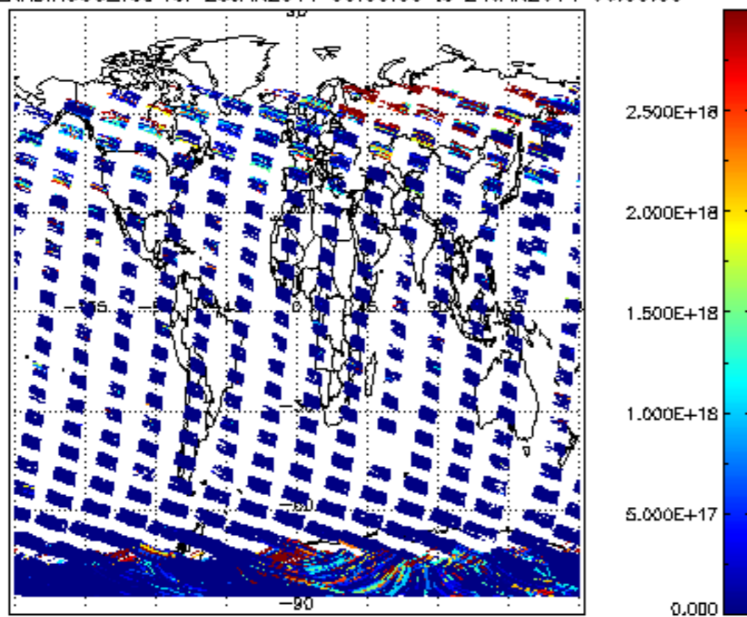
SCIOL2P_NADIR3CO_vcd for 23JAN2011 00:00:00 to 24JAN2011 00:00:00
