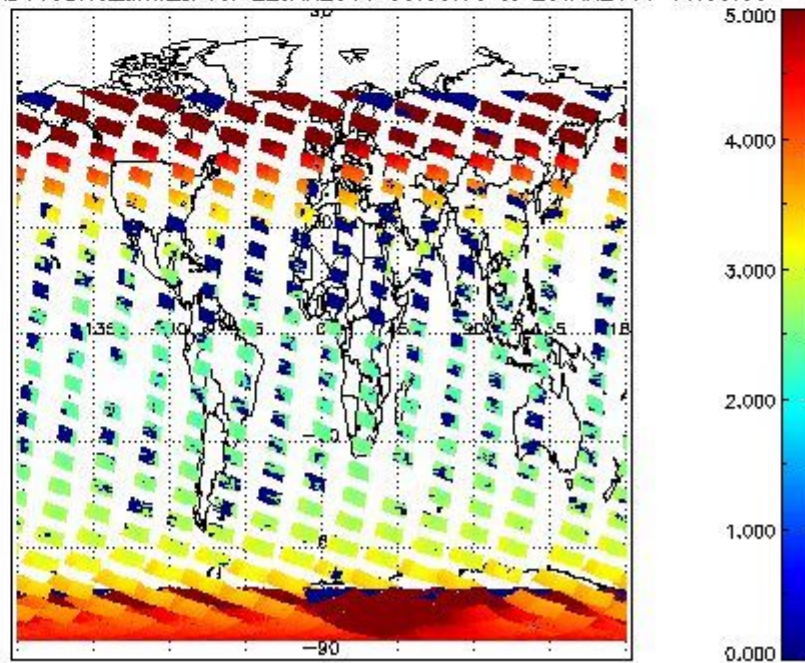
SCIOL2P_NADUV3BRO_amf_cl for 22JAN2011 00:00:00 to 23JAN2011 00:00:00
