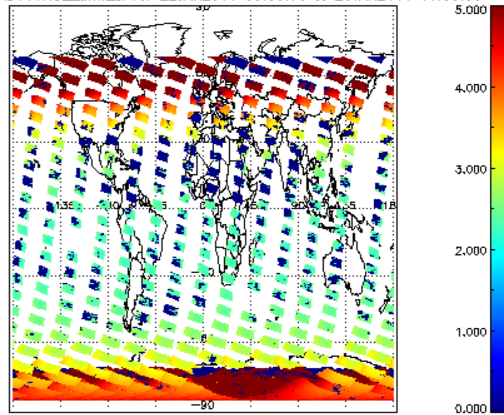
SCIOL2P_NADUV1NO2_amf_cl for 22JAN2011 00:00:00 to 23JAN2011 00:00:00
