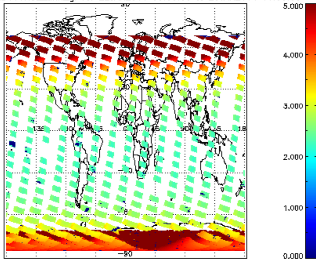
SCIOL2P_NADUV1NO2_amf_gr for 22JAN2011 00:00:00 to 23JAN2011 00:00:00
