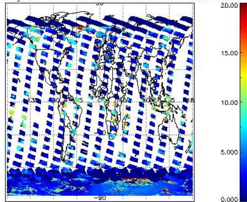
cL_top_height for 22JAN2011 00:00:00 to 23JAN2011 00:00:00
