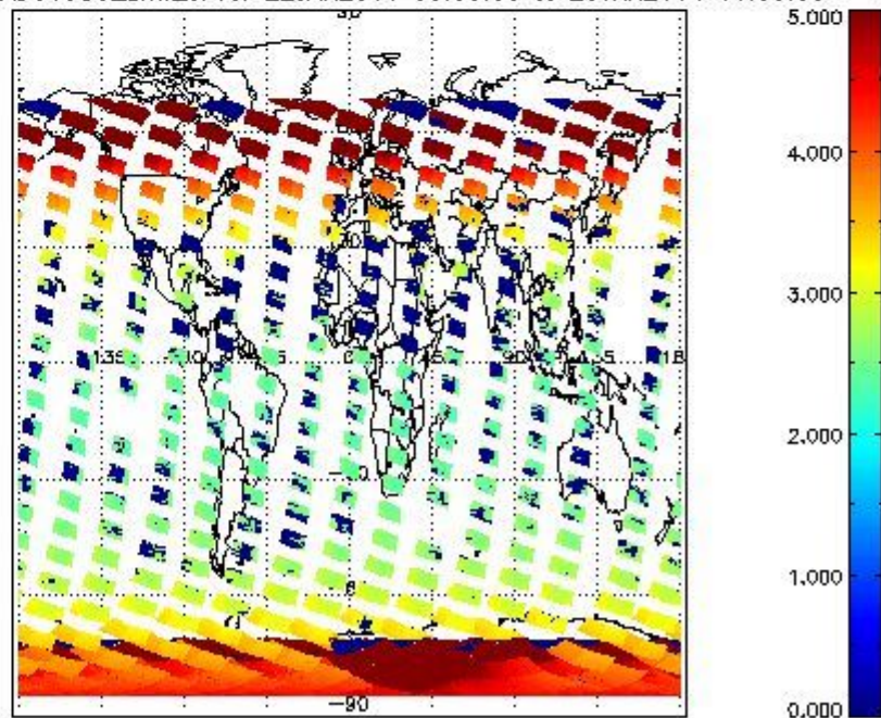
SCIOL2P_NADUV003_amf_cl for 22JAN2011 00:00:00 to 23JAN2011 00:00:00
