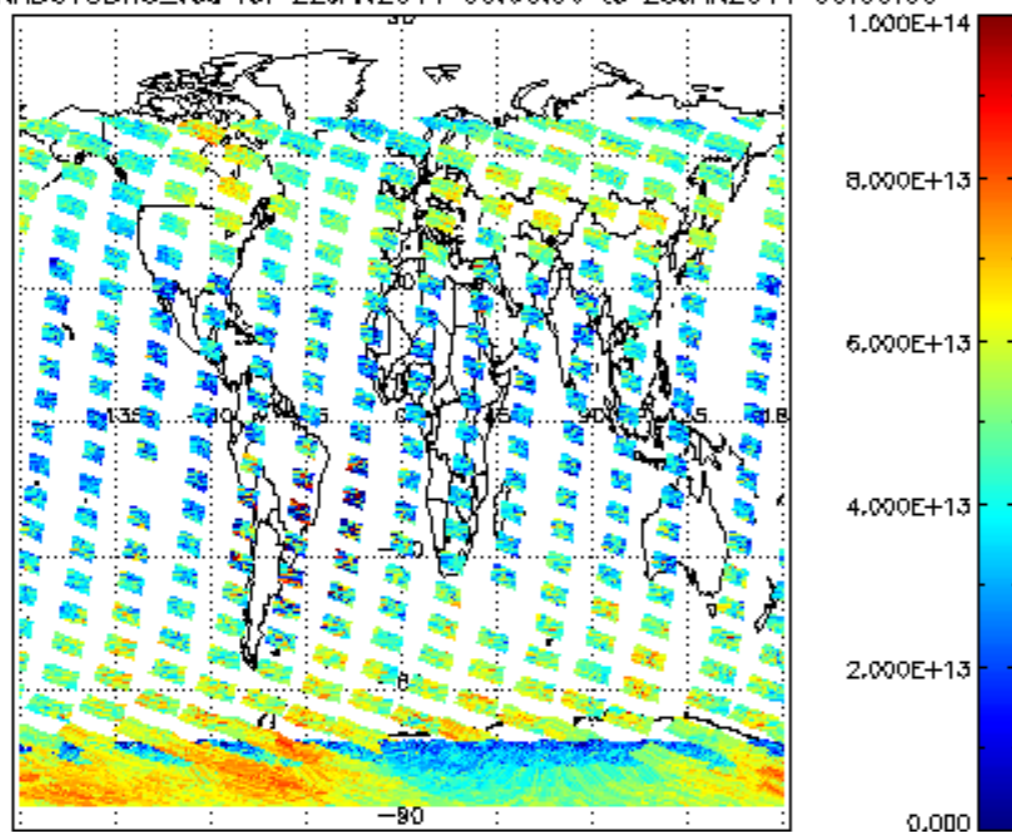
SCIOL2P_NADUV3BRO_vcd for 22JAN2011 00:00:00 to 23JAN2011 00:00:00
