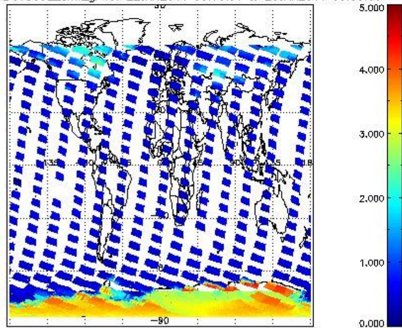
SCIOL2P_NADUV5SO2_amf_gr for 22JAN2011 00:00:00 to 23JAN2011 00:00:00
