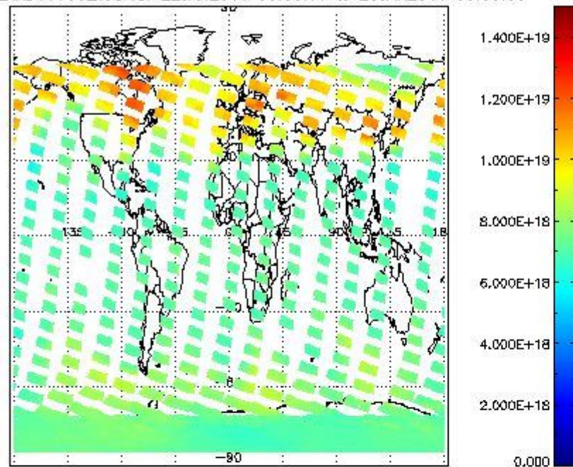
SCIOL2P_NADUV003_vcd for 22JAN2011 00:00:00 to 23JAN2011 00:00:00
