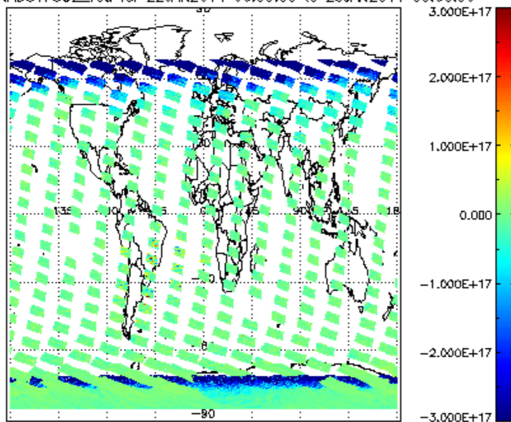
SCIOL2P_NADUV7S02_vcd for 22JAN2011 00:00:00 to 23JAN2011 00:00:00
