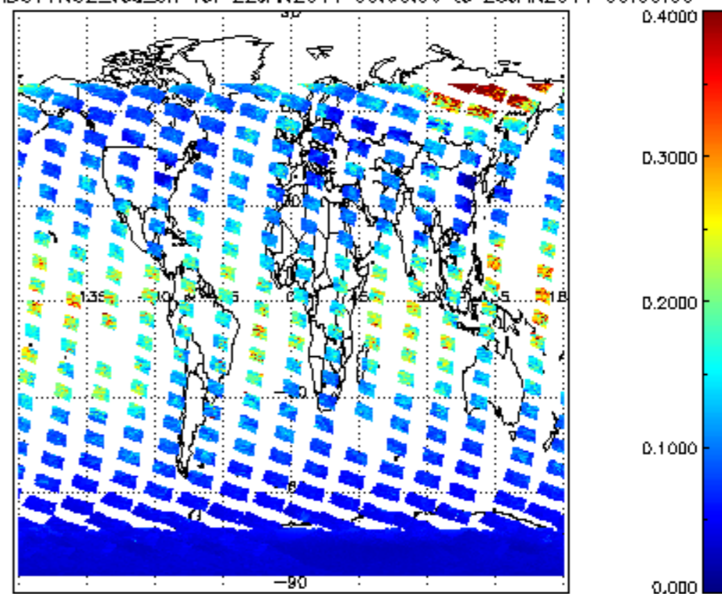
SCIOL2P_NADUV1NO2_vcd_err for 22JAN2011 00:00:00 to 23JAN2011 00:00:00
