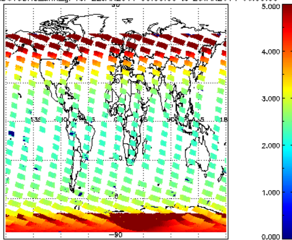
SCIOL2P_NADUV3BRO_amf_gr for 22JAN2011 00:00:00 to 23JAN2011 00:00:00
