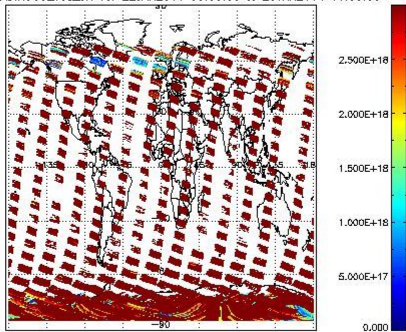
SCIDL2P_NADIR3CO_vcd_err for 22JAN2011 00:00:00 to 23JAN2011 00:00:00
