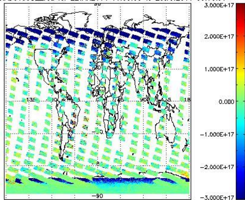
SCIOL2P_NADUV5SO2_vcd for 22JAN2011 00:00:00 to 23JAN2011 00:00:00
