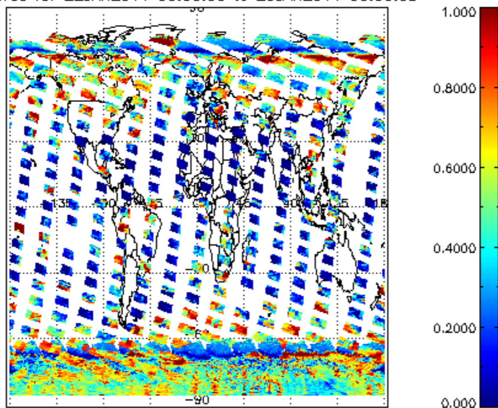
cL_frac for 22JAN2011 00:00:00 to 23JAN2011 00:00:00
