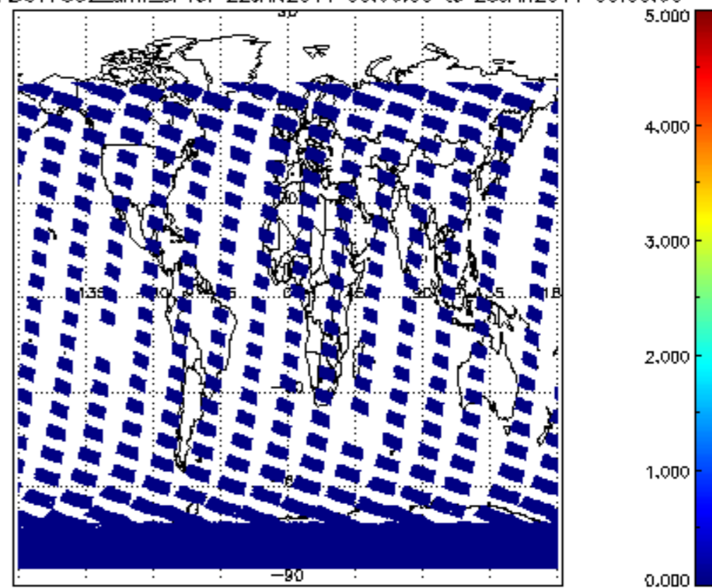
SCIOL2P_NADUV7S02_amf_sl for 22JAN2011 00:00:00 to 23JAN2011 00:00:00
