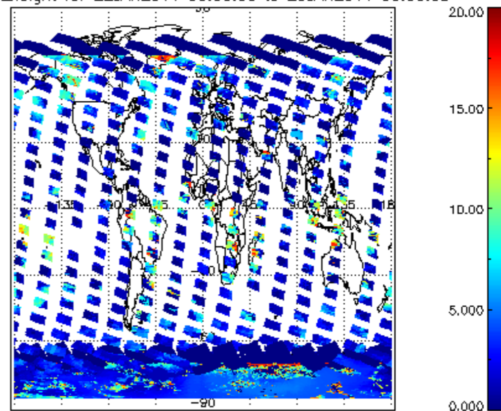
cL_top_height for 22JAN2011 00:00:00 to 23JAN2011 00:00:00
