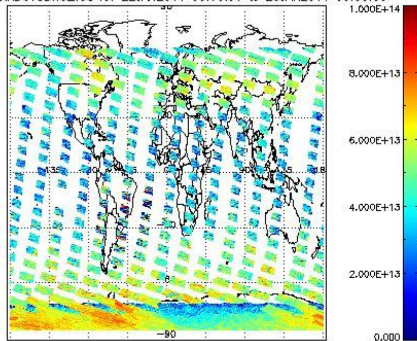
SCIOL2P_NADUV3BRO_vcd for 22JAN2011 00:00:00 to 23JAN2011 00:00:00
