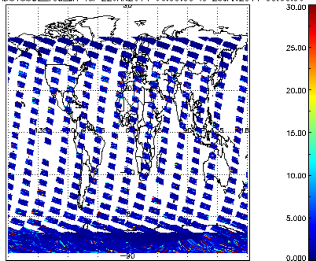
SCIOL2P_NADUV5S02_vcd_err for 22JAN2011 00:00:00 to 23JAN2011 00:00:00
