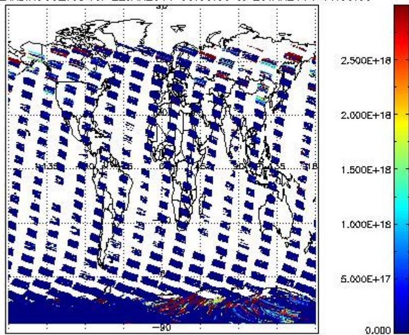
SCIDL2P_NADIR3CO_vcd for 22JAN2011 00:00:00 to 23JAN2011 00:00:00
