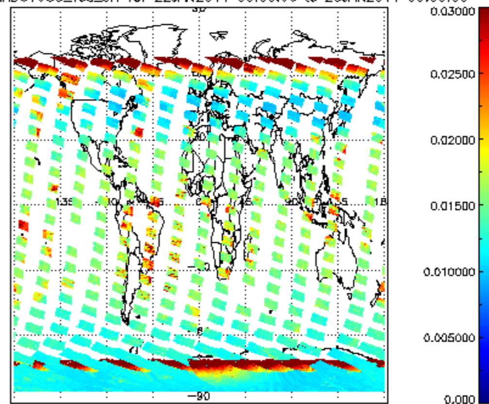
SCIOL2P_NADUV003_vcd_err for 22JAN2011 00:00:00 to 23JAN2011 00:00:00
