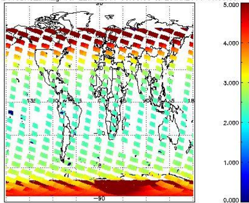
SCIOL2P_NADUV3BRO_amf_gr for 22JAN2011 00:00:00 to 23JAN2011 00:00:00
