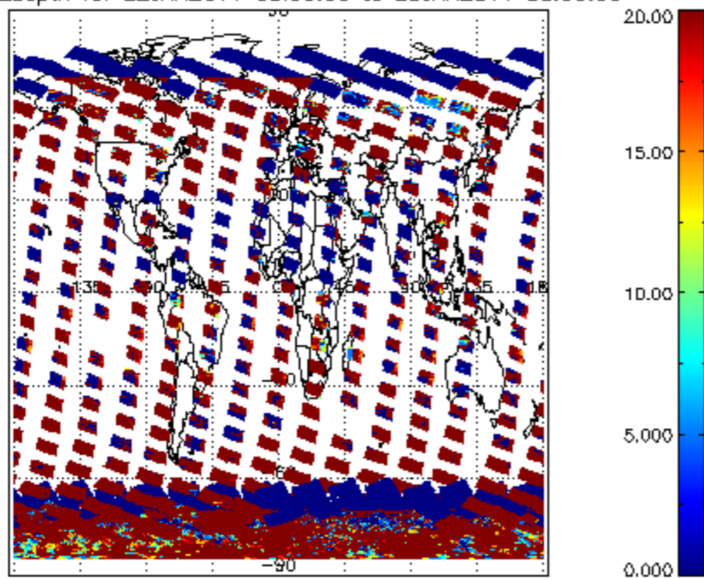
cLopt_depth for 22JAN2011 00:00:00 to 23JAN2011 00:00:00
