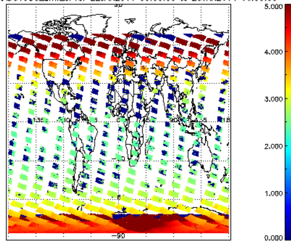
SCIOL2P_NADUV003_amf_cl for 22JAN2011 00:00:00 to 23JAN2011 00:00:00
