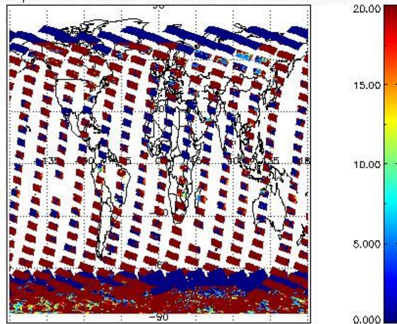
cLopt_depth for 22JAN2011 00:00:00 to 23JAN2011 00:00:00
