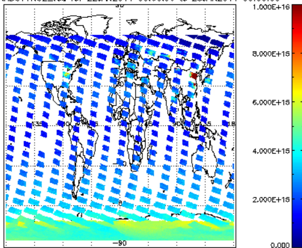
SCIOL2P_NADUV1NO2_vcd for 22JAN2011 00:00:00 to 23JAN2011 00:00:00
