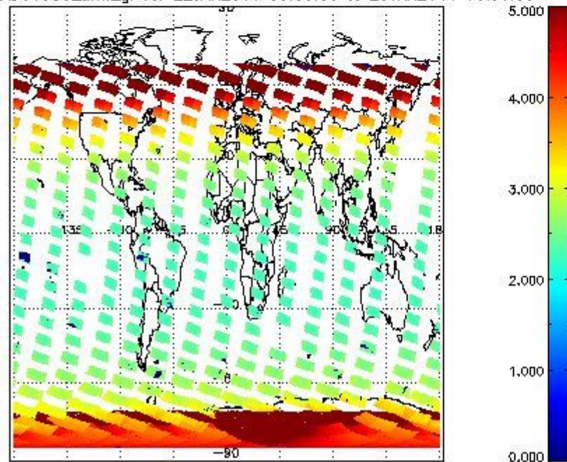
SCIOL2P_NADUV003_amf_gr for 22JAN2011 00:00:00 to 23JAN2011 00:00:00
