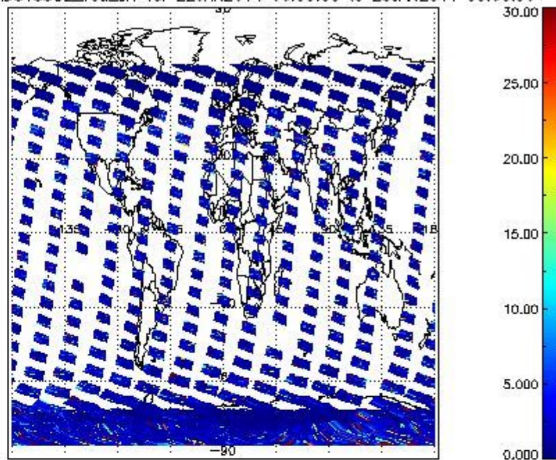
SCIOL2P_NADUV5SO2_vcd_err for 22JAN2011 00:00:00 to 23JAN2011 00:00:00
