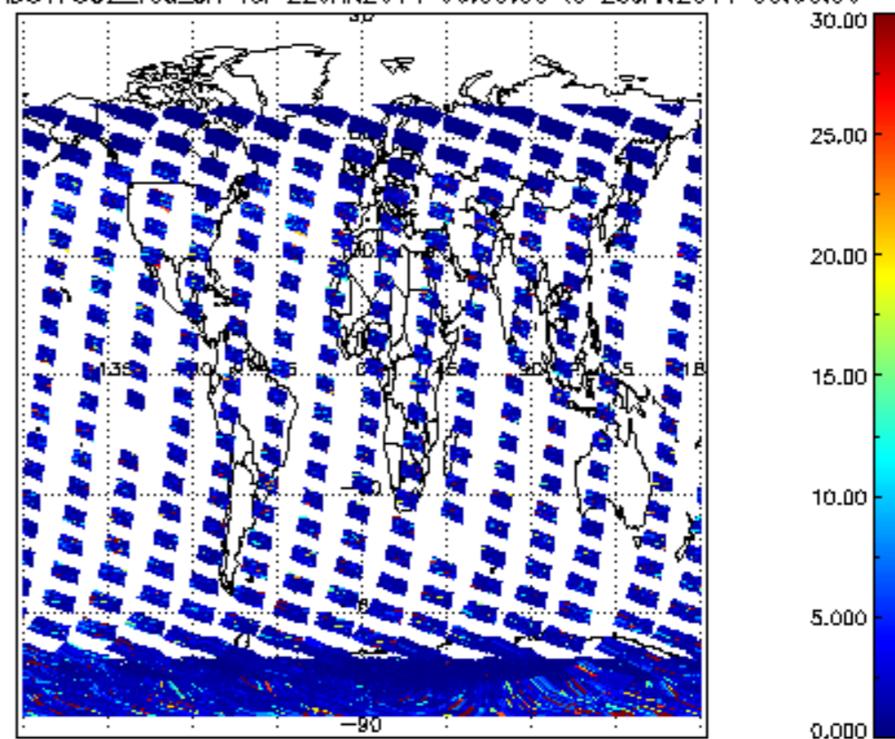
SCIOL2P_NADUV7S02_vcd_err for 22JAN2011 00:00:00 to 23JAN2011 00:00:00
