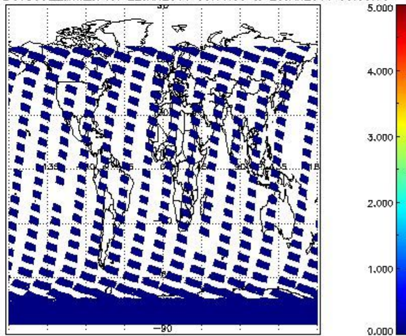
SCIOL2P_NADUV5SO2_amf_cl for 22JAN2011 00:00:00 to 23JAN2011 00:00:00
