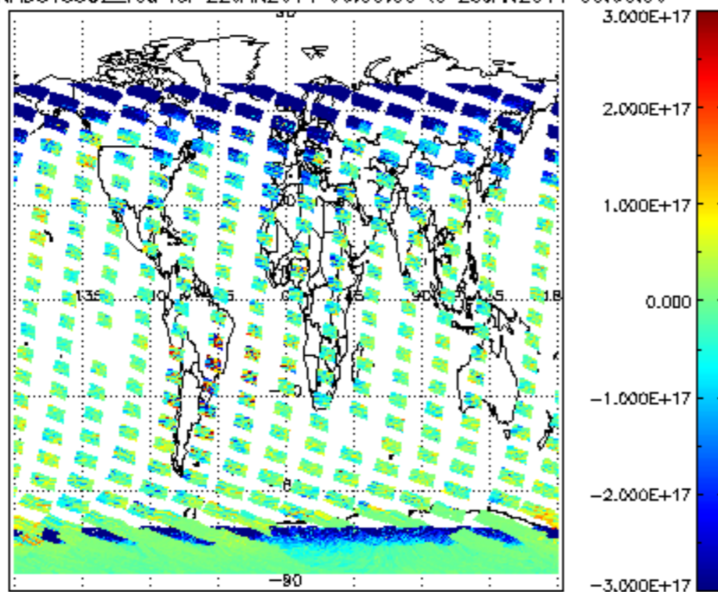
SCIOL2P_NADUV5S02_vcd for 22JAN2011 00:00:00 to 23JAN2011 00:00:00
