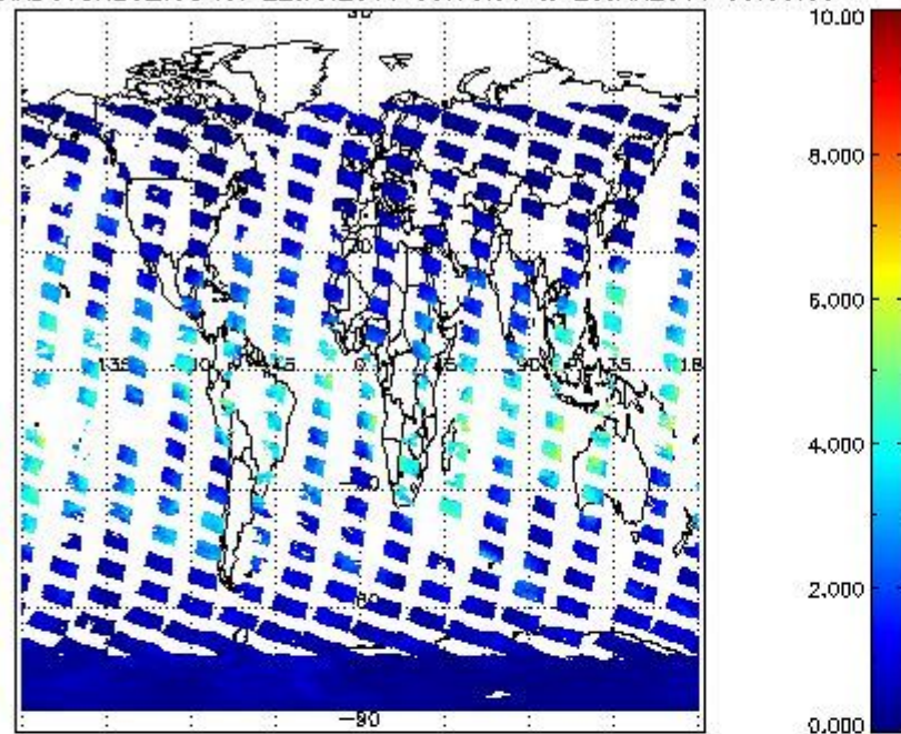
SCIOL2P_NADUV8H20_vcd for 22JAN2011 00:00:00 to 23JAN2011 00:00:00
