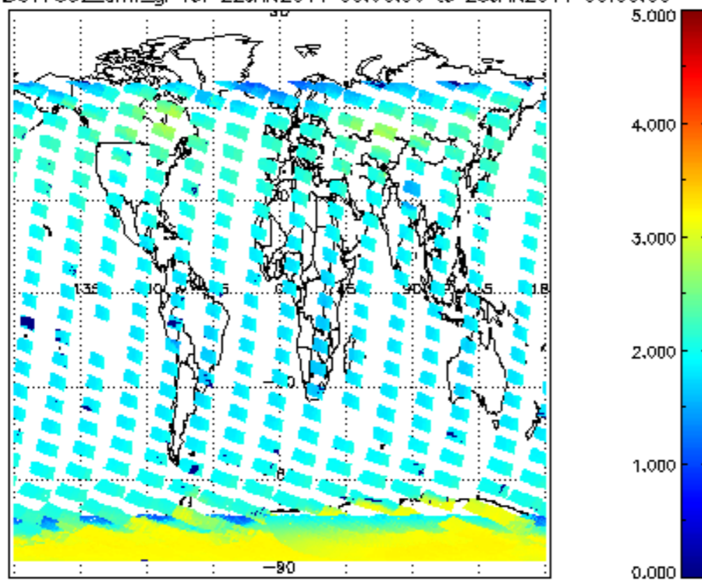
SCIOL2P_NADUV7S02_amf_gr for 22JAN2011 00:00:00 to 23JAN2011 00:00:00
