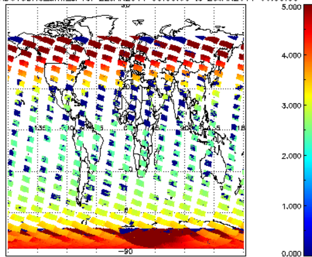
SCIOL2P_NADUV3BRO_amf_cl for 22JAN2011 00:00:00 to 23JAN2011 00:00:00
