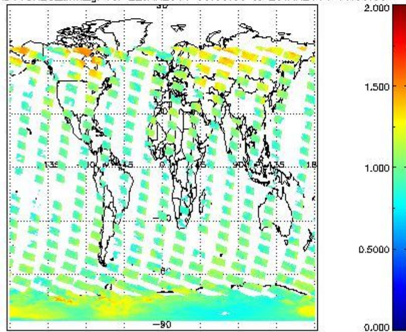
SCIOL2P_NADUV8H20_amf_gr for 22JAN2011 00:00:00 to 23JAN2011 00:00:00
