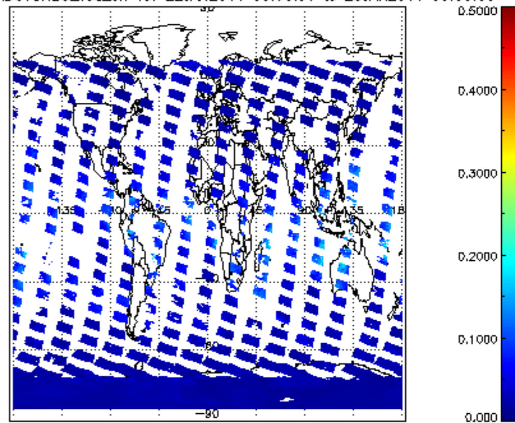
SCIOL2P_NADUVBH20_vcd_err for 22JAN2011 00:00:00 to 23JAN2011 00:00:00
