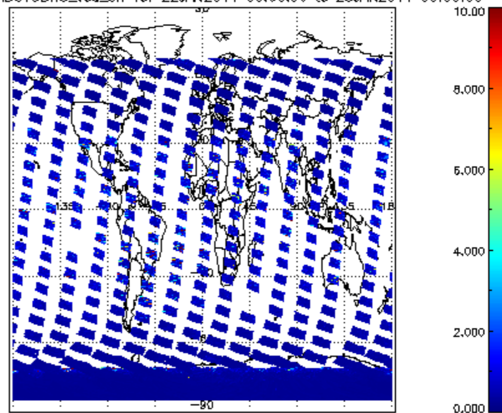
SCIOL2P_NADUV3BRO_vcd_err for 22JAN2011 00:00:00 to 23JAN2011 00:00:00
