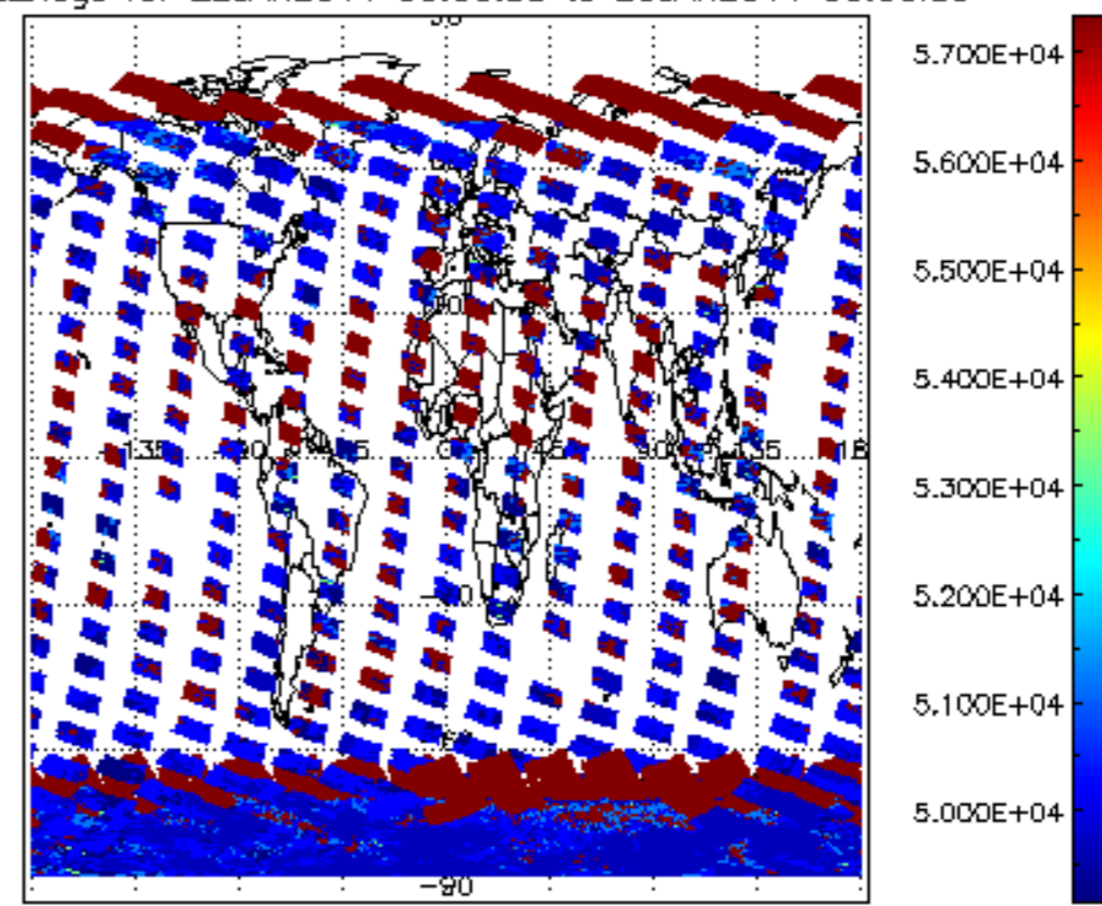
cloud_flags for 22JAN2011 00:00:00 to 23JAN2011 00:00:00
