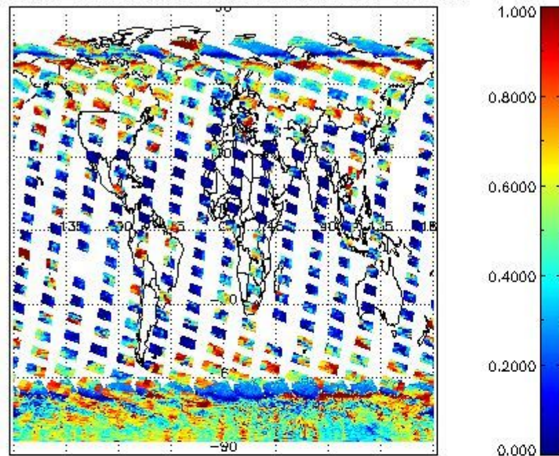
cL_frac for 22JAN2011 00:00:00 to 23JAN2011 00:00:00
