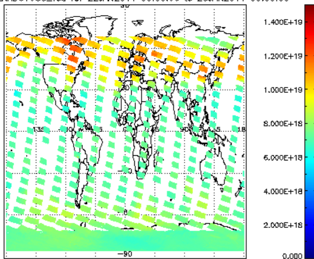
SCIOL2P_NADUV003_vcd for 22JAN2011 00:00:00 to 23JAN2011 00:00:00
