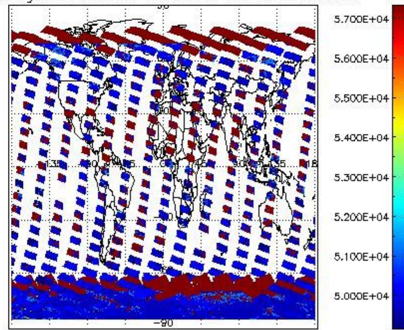
cloud_flags for 22JAN2011 00:00:00 to 23JAN2011 00:00:00
