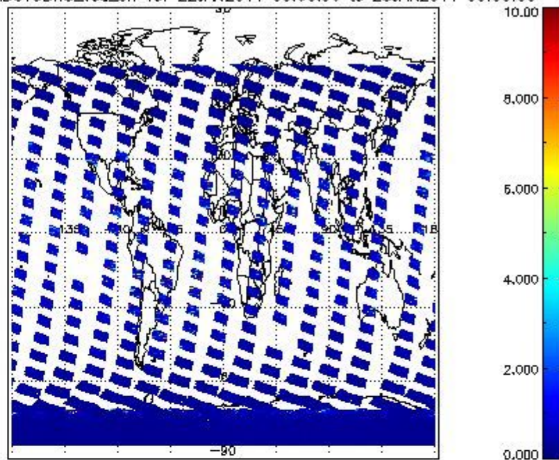
SCIOL2P_NADUV3BRO_vcd_err for 22JAN2011 00:00:00 to 23JAN2011 00:00:00
