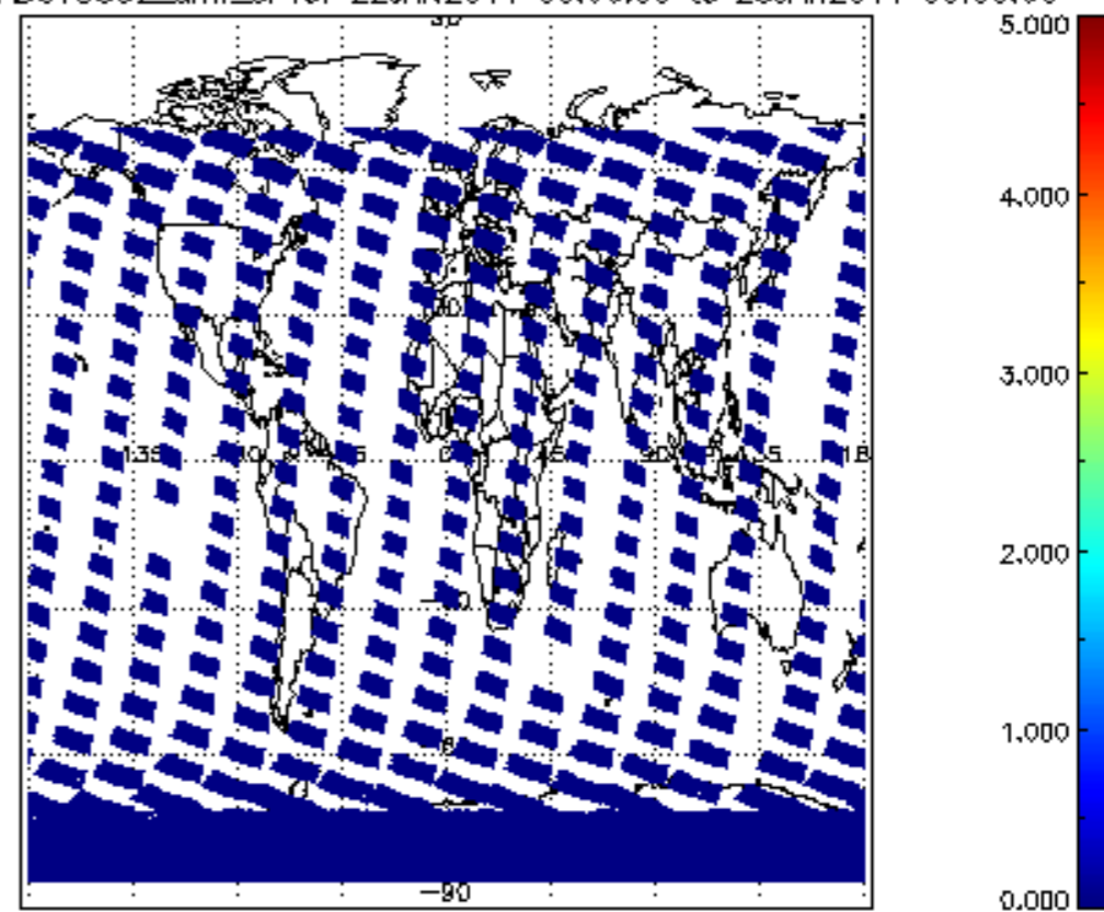
SCIOL2P_NADUV5S02_amf_cl for 22JAN2011 00:00:00 to 23JAN2011 00:00:00
