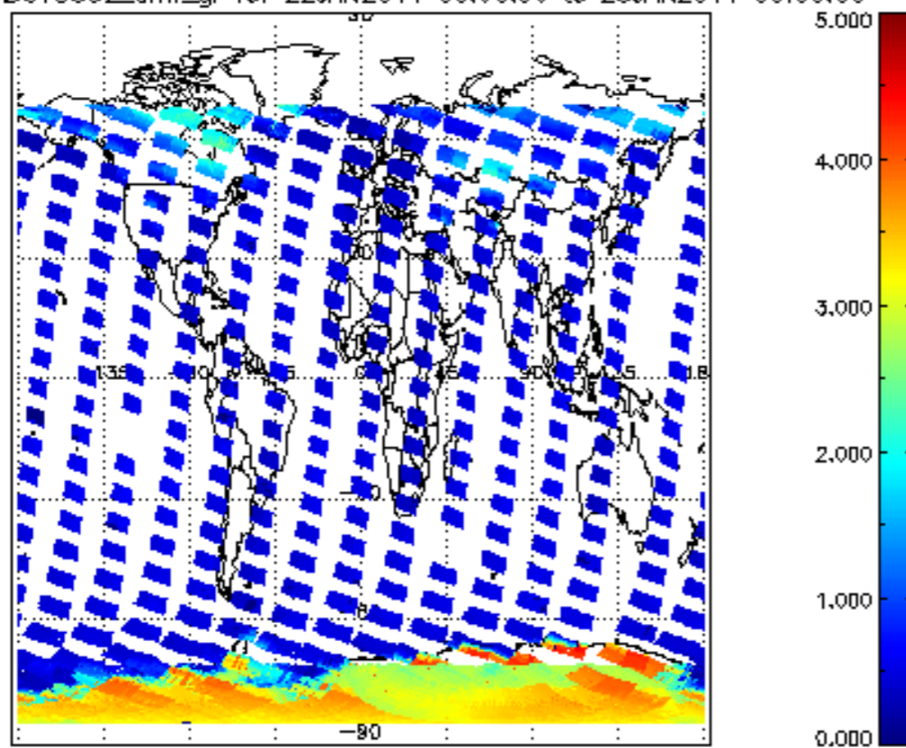
SCIOL2P_NADUV5S02_amf_gr for 22JAN2011 00:00:00 to 23JAN2011 00:00:00
