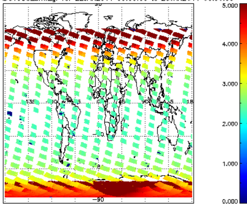
SCIOL2P_NADUV003_amf_gr for 22JAN2011 00:00:00 to 23JAN2011 00:00:00
