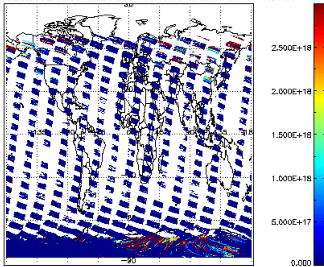
SCIOL2P_NADIR3CO_vcd for 22JAN2011 00:00:00 to 23JAN2011 00:00:00
