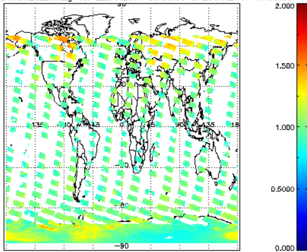
SCIOL2P_NADUVBH20_amf_gr for 22JAN2011 00:00:00 to 23JAN2011 00:00:00
