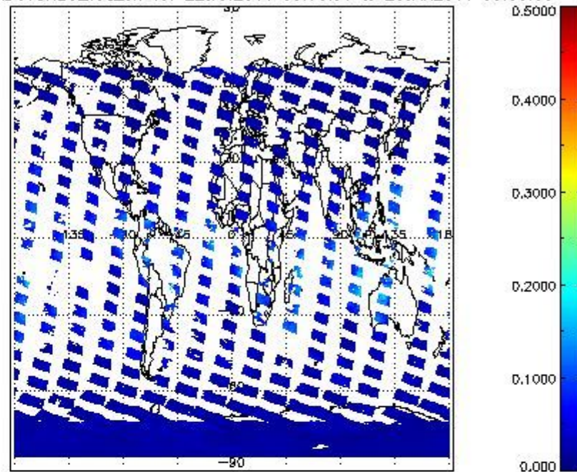
SCIOL2P_NADUV8H20_vcd_err for 22JAN2011 00:00:00 to 23JAN2011 00:00:00
