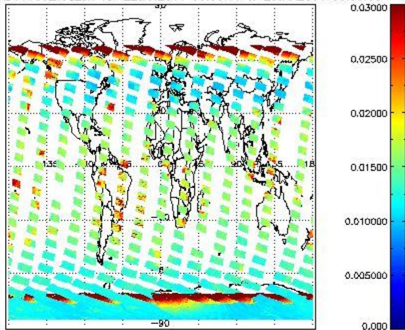
SCIOL2P_NADUV003_vcd_err for 22JAN2011 00:00:00 to 23JAN2011 00:00:00
