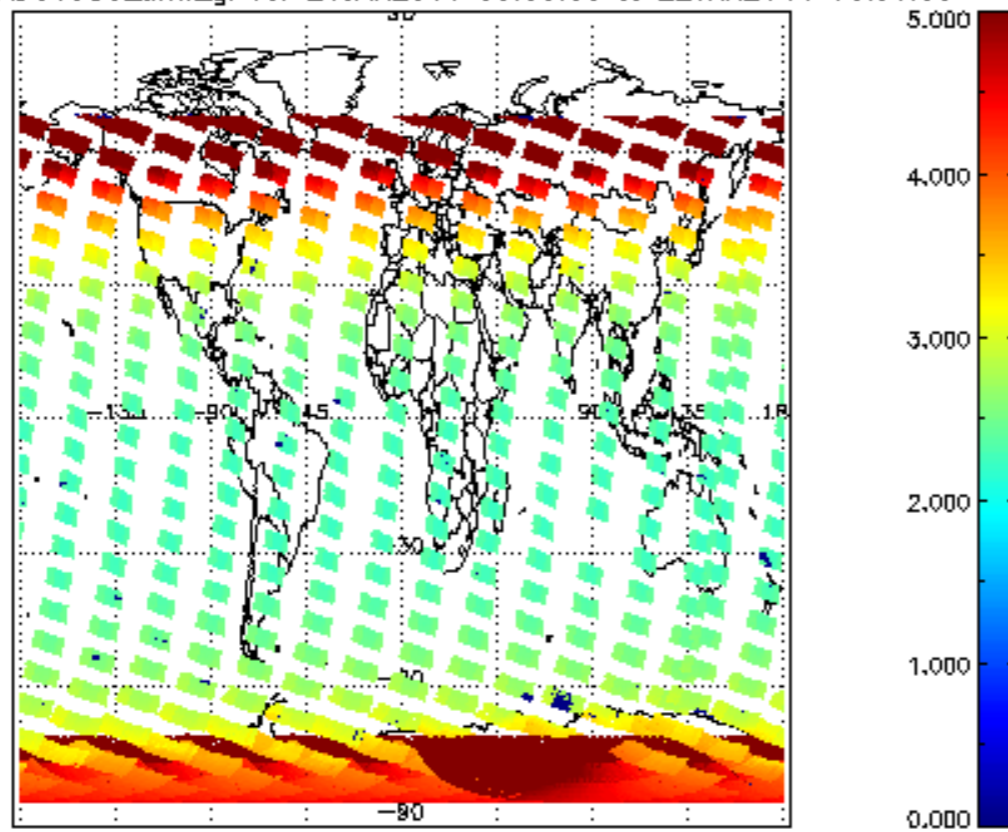
SCIOL2P_NADUV003_amf_gr for 21JAN2011 00:00:00 to 22JAN2011 00:00:00
