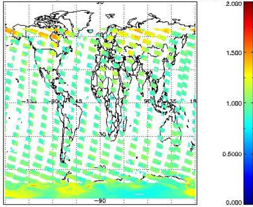
SCIOL2P_NADUV8H20_amf_gr for 21JAN2011 00:00:00 to 22JAN2011 00:00:00
