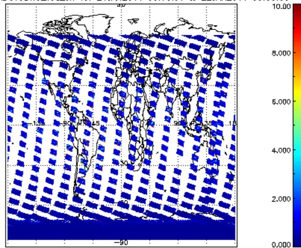
SCIOL2P_NADUV3BRO_vcd_err for 21JAN2011 00:00:00 to 22JAN2011 00:00:00
