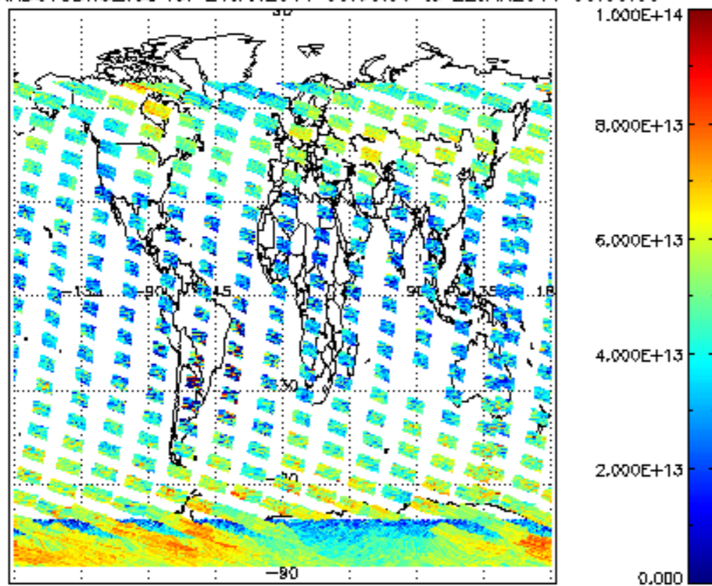
SCIOL2P_NADUV3BRO_vcd for 21JAN2011 00:00:00 to 22JAN2011 00:00:00
