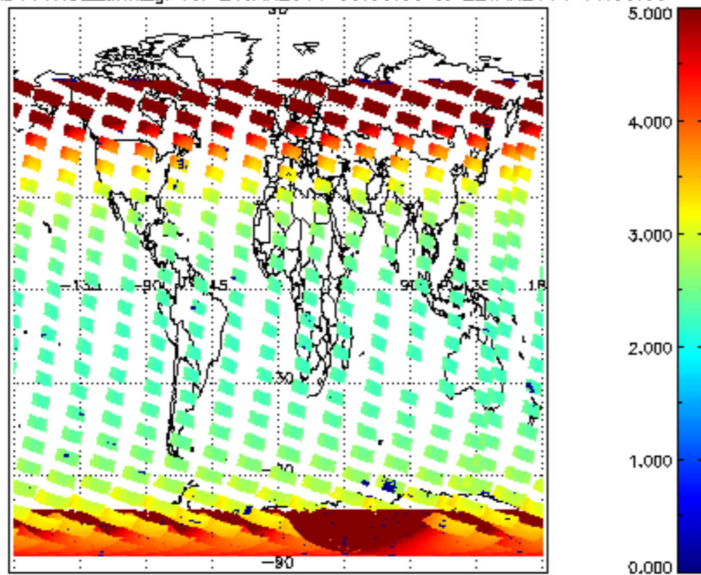
SCIOL2P_NADUV1NO2_amf_gr for 21JAN2011 00:00:00 to 22JAN2011 00:00:00
