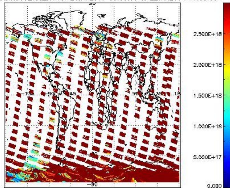
SCIDL2P_NADIR3CO_vcd_err for 21JAN2011 00:00:00 to 22JAN2011 00:00:00
