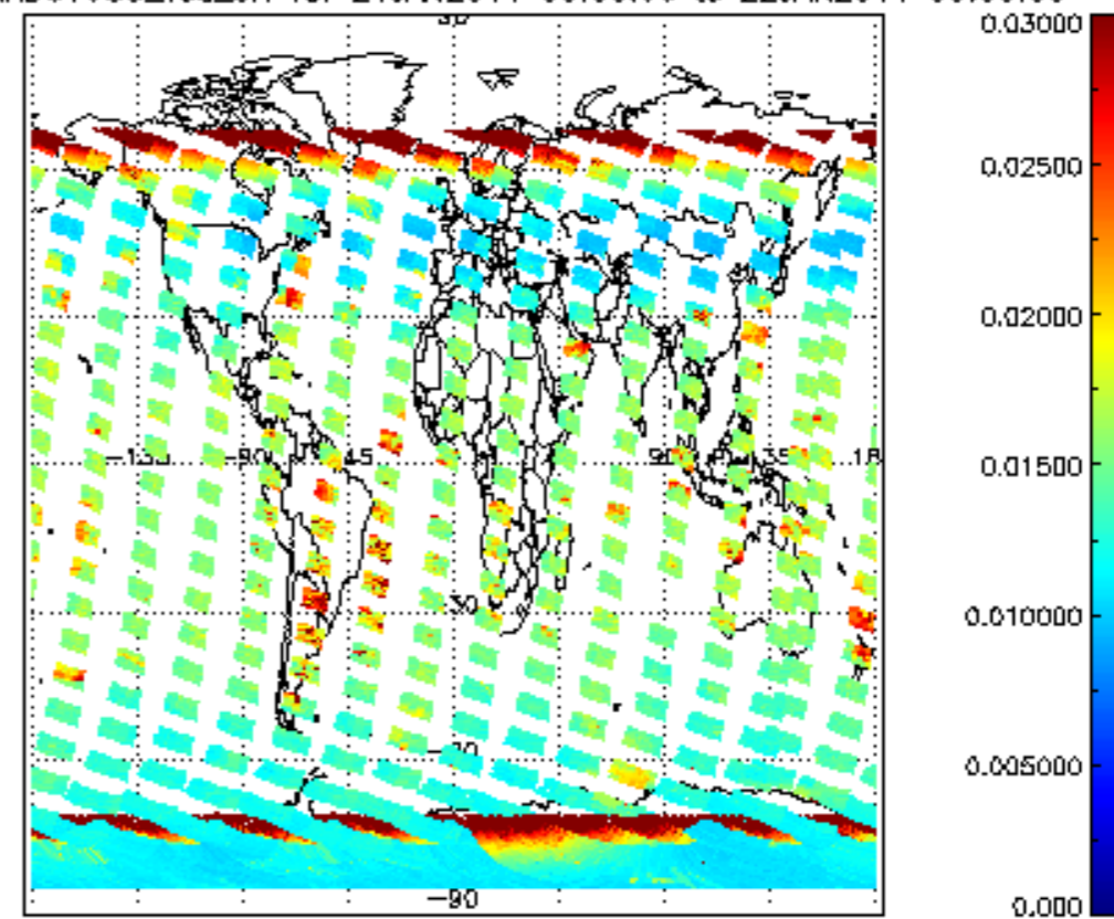
SCIOL2P_NADUV003_vcd_err for 21JAN2011 00:00:00 to 22JAN2011 00:00:00
