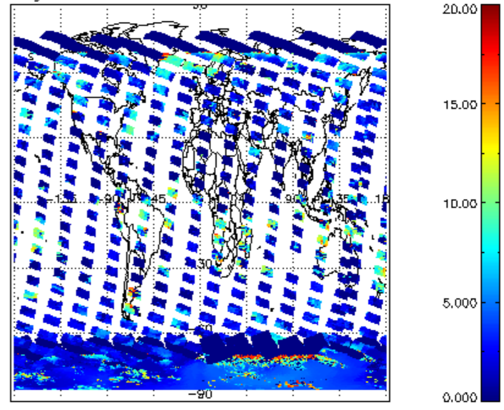
cL_top_height for 21JAN2011 00:00:00 to 22JAN2011 00:00:00
