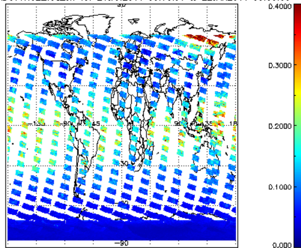
SCIOL2P_NADUV1NO2_vcd_err for 21JAN2011 00:00:00 to 22JAN2011 00:00:00
