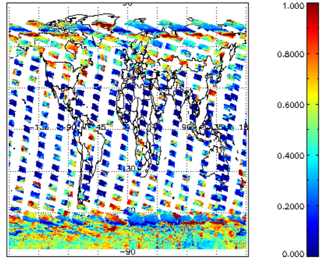
cL_frac for 21JAN2011 00:00:00 to 22JAN2011 00:00:00
