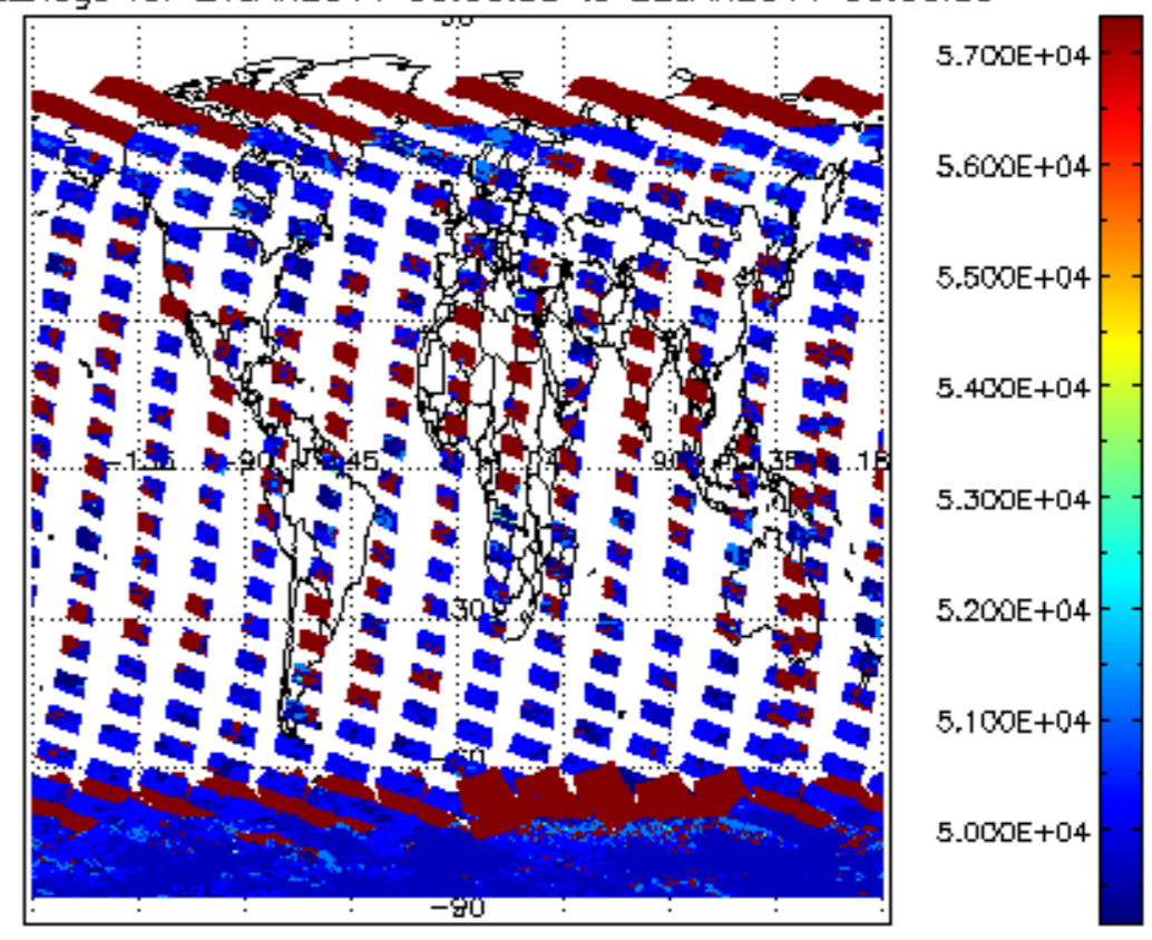
cloud_flags for 21JAN2011 00:00:00 to 22JAN2011 00:00:00
