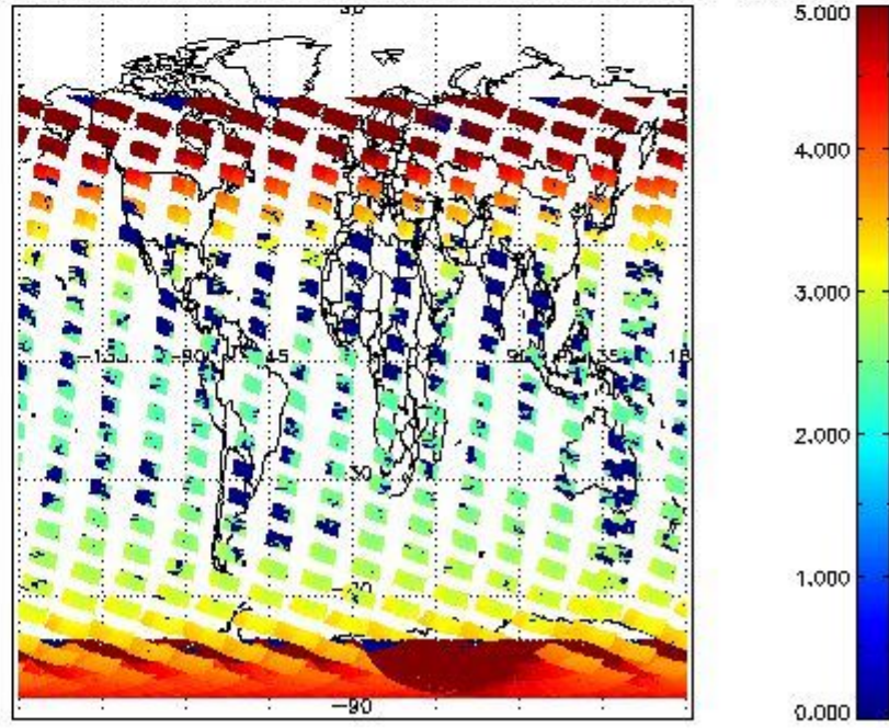
SCIOL2P_NADUV3BRO_amf_cl for 21JAN2011 00:00:00 to 22JAN2011 00:00:00
