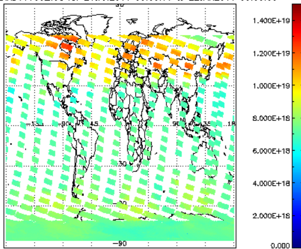
SCIOL2P_NADUV003_vcd for 21JAN2011 00:00:00 to 22JAN2011 00:00:00
