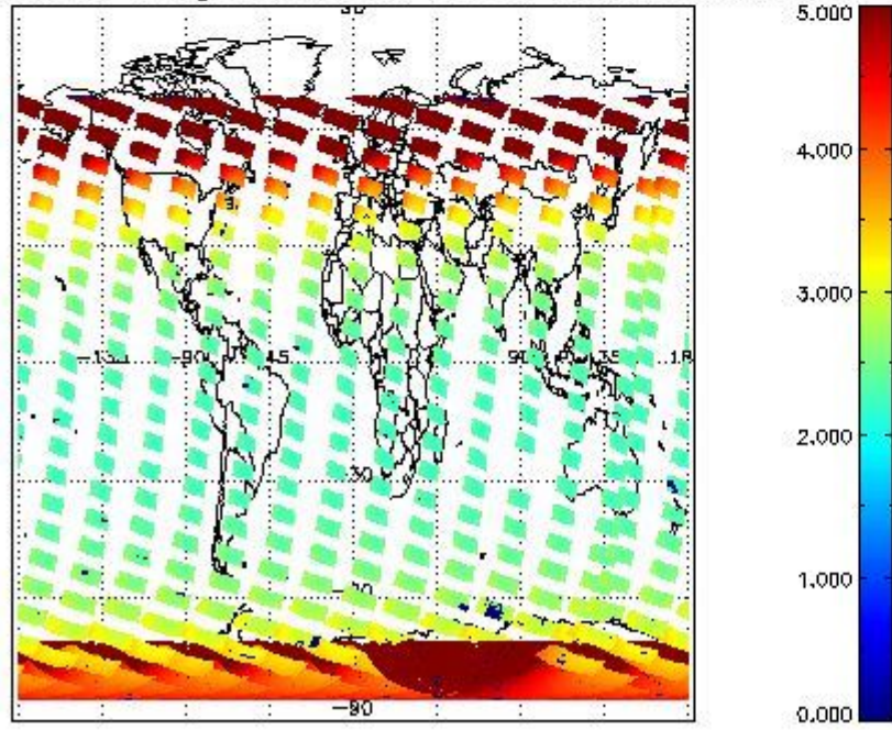
SCIOL2P_NADUV1NO2_amf_gr for 21JAN2011 00:00:00 to 22JAN2011 00:00:00
