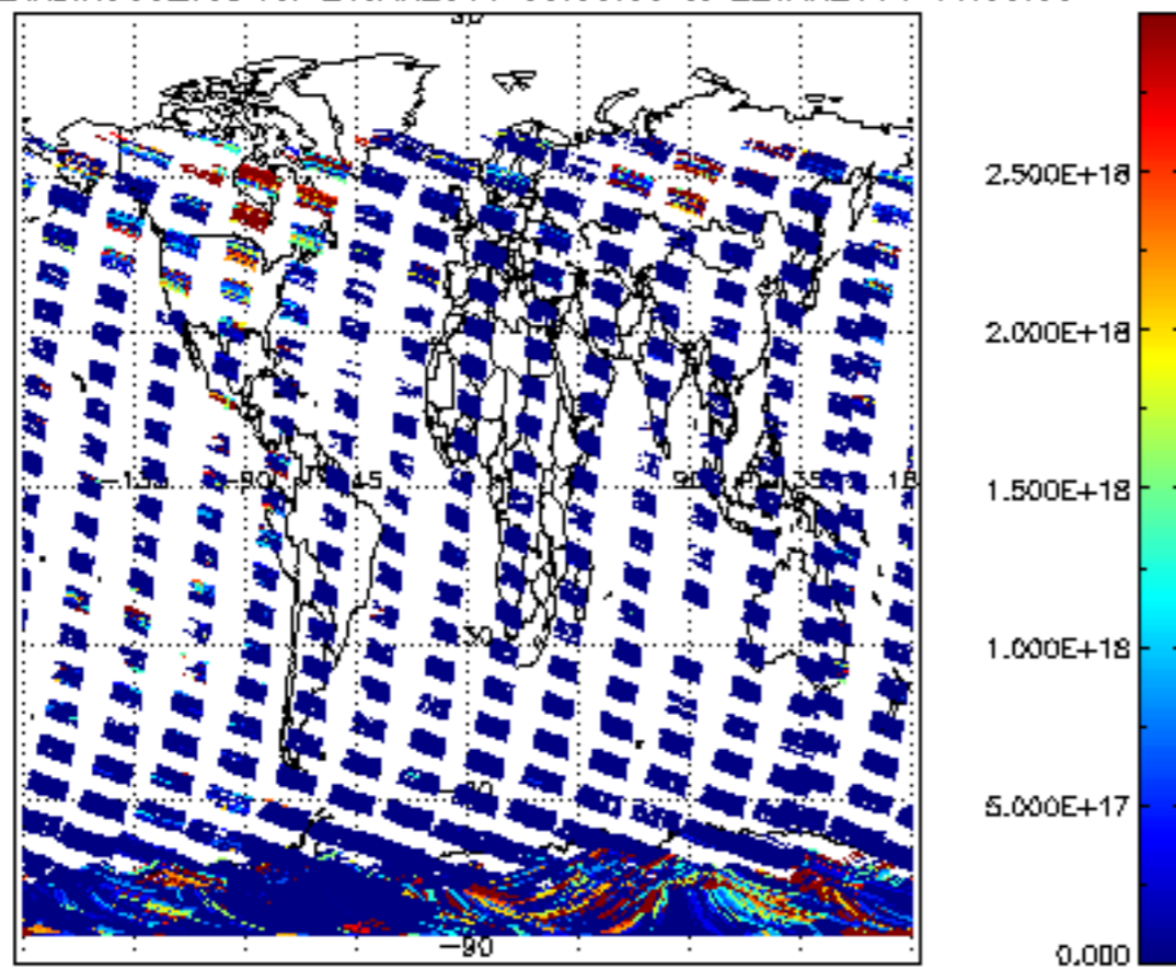
SCIOL2P_NADIR3CO_vcd for 21JAN2011 00:00:00 to 22JAN2011 00:00:00
