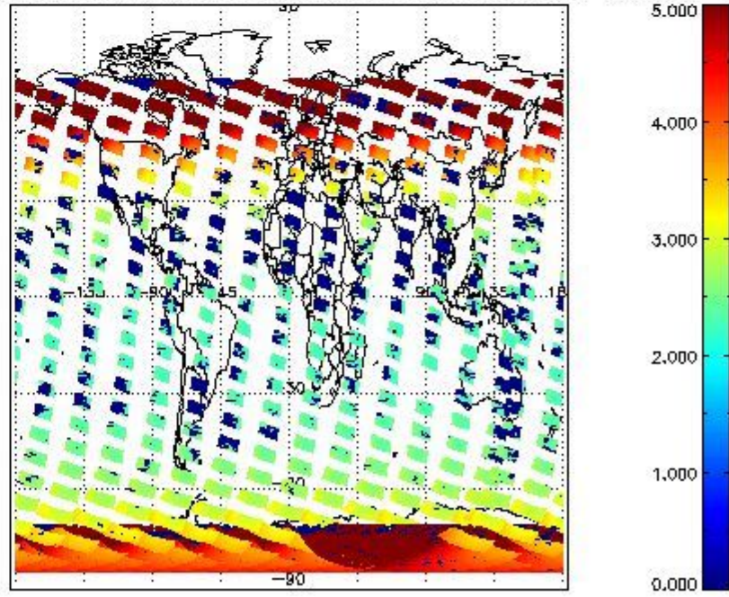
SCIOL2P_NADUV1NO2_amf_cl for 21JAN2011 00:00:00 to 22JAN2011 00:00:00
