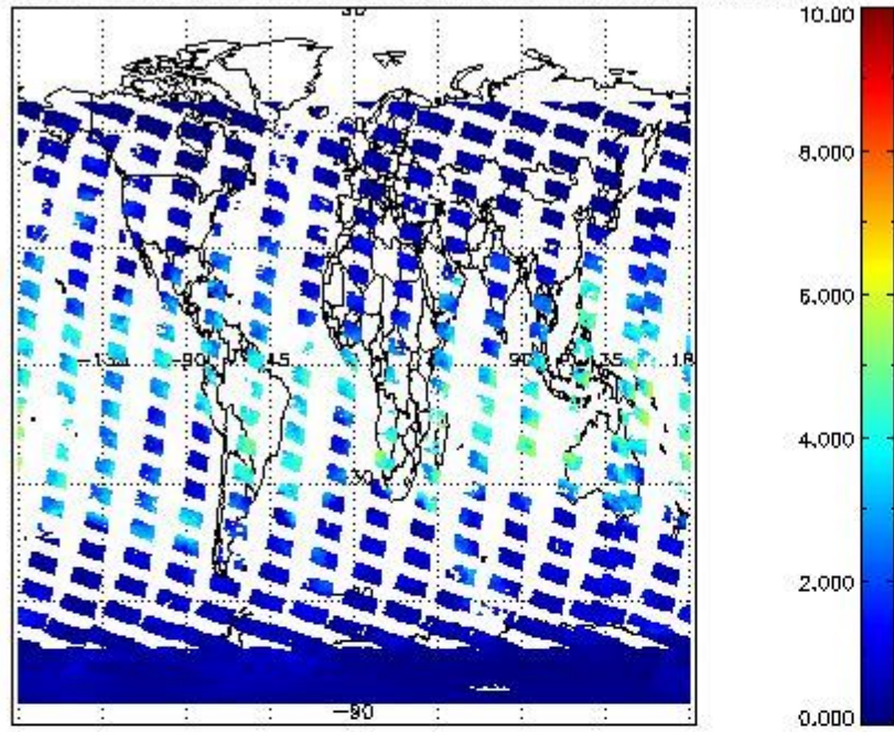
SCIOL2P_NADUV8H20_vcd for 21JAN2011 00:00:00 to 22JAN2011 00:00:00
