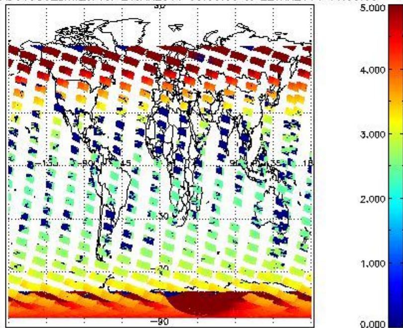
SCIOL2P_NADUV003_amf_cl for 21JAN2011 00:00:00 to 22JAN2011 00:00:00
