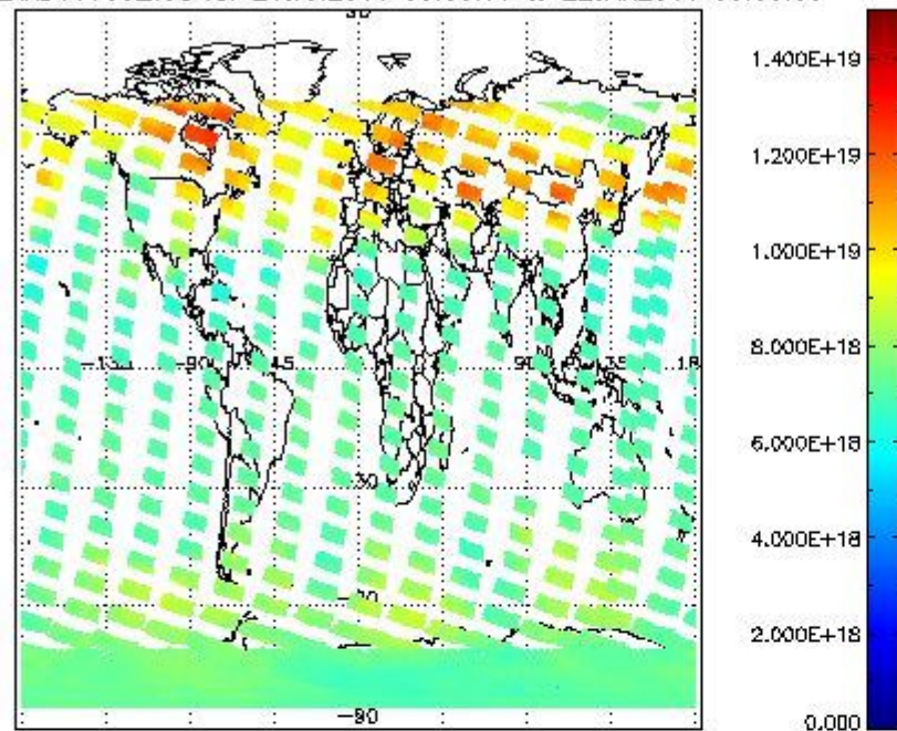
SCIOL2P_NADUV003_vcd for 21JAN2011 00:00:00 to 22JAN2011 00:00:00
