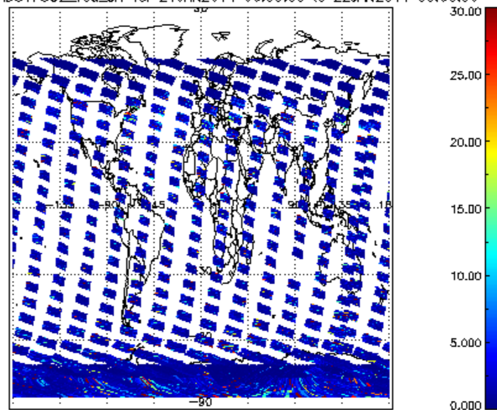
SCIOL2P_NADUV7S02_vcd_err for 21JAN2011 00:00:00 to 22JAN2011 00:00:00
