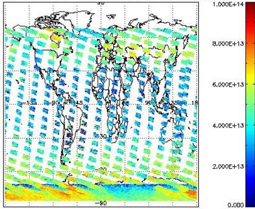
SCIOL2P_NADUV3BRO_vcd for 21JAN2011 00:00:00 to 22JAN2011 00:00:00
