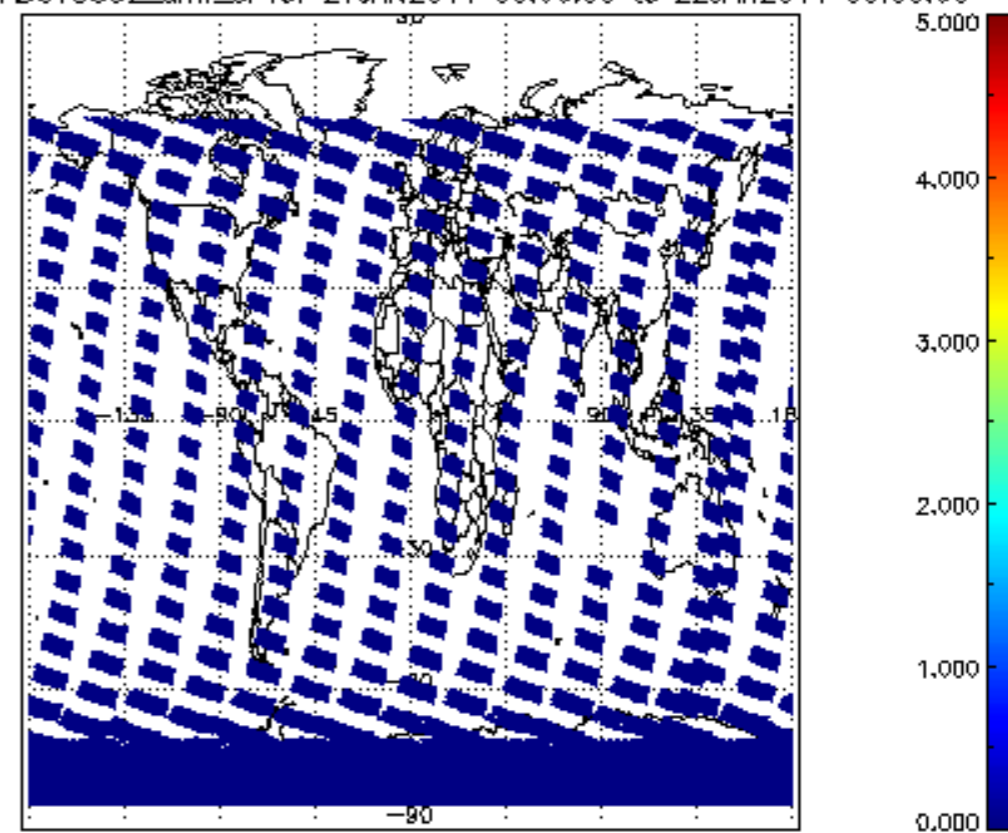
SCIOL2P_NADUV5S02_amf_cl for 21JAN2011 00:00:00 to 22JAN2011 00:00:00
