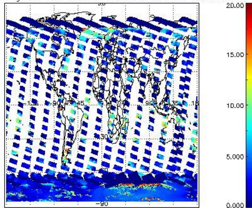
cL_top_height for 21JAN2011 00:00:00 to 22JAN2011 00:00:00
