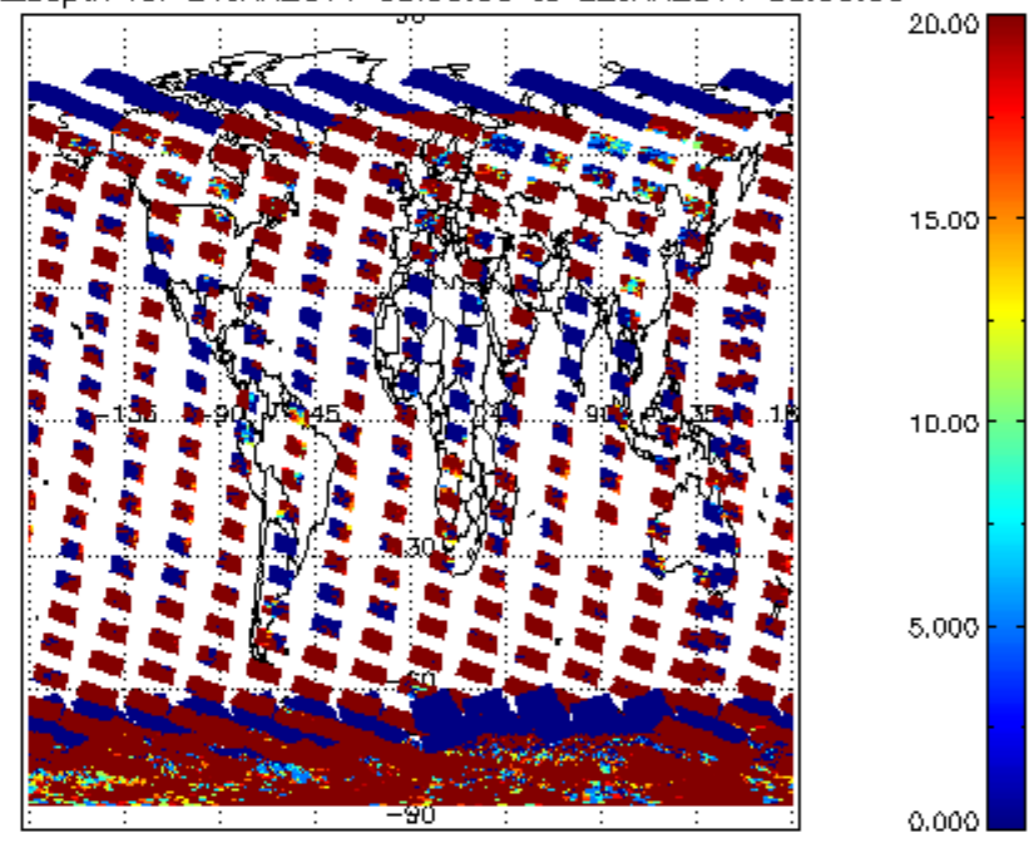
cLopt_depth for 21JAN2011 00:00:00 to 22JAN2011 00:00:00
