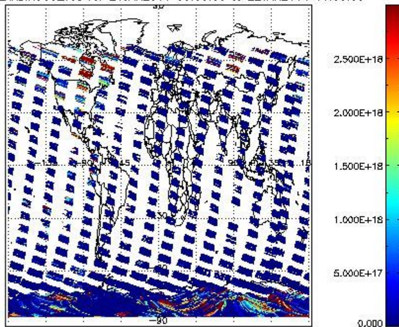
SCIDL2P_NADIR3CO_vcd for 21JAN2011 00:00:00 to 22JAN2011 00:00:00
