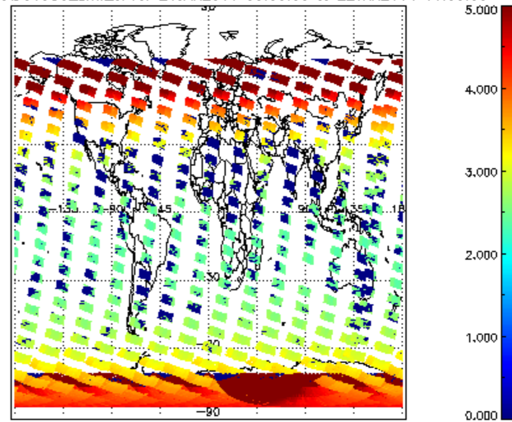
SCIOL2P_NADUV003_amf_cl for 21JAN2011 00:00:00 to 22JAN2011 00:00:00
