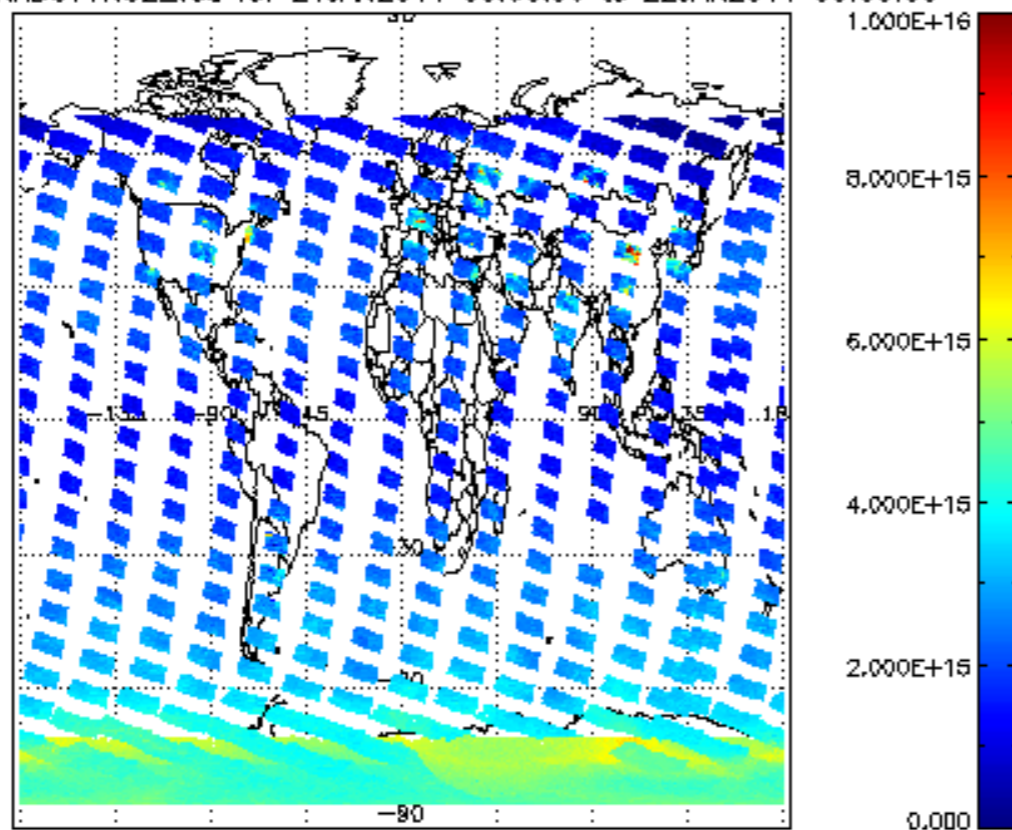
SCIOL2P_NADUV1NO2_vcd for 21JAN2011 00:00:00 to 22JAN2011 00:00:00
