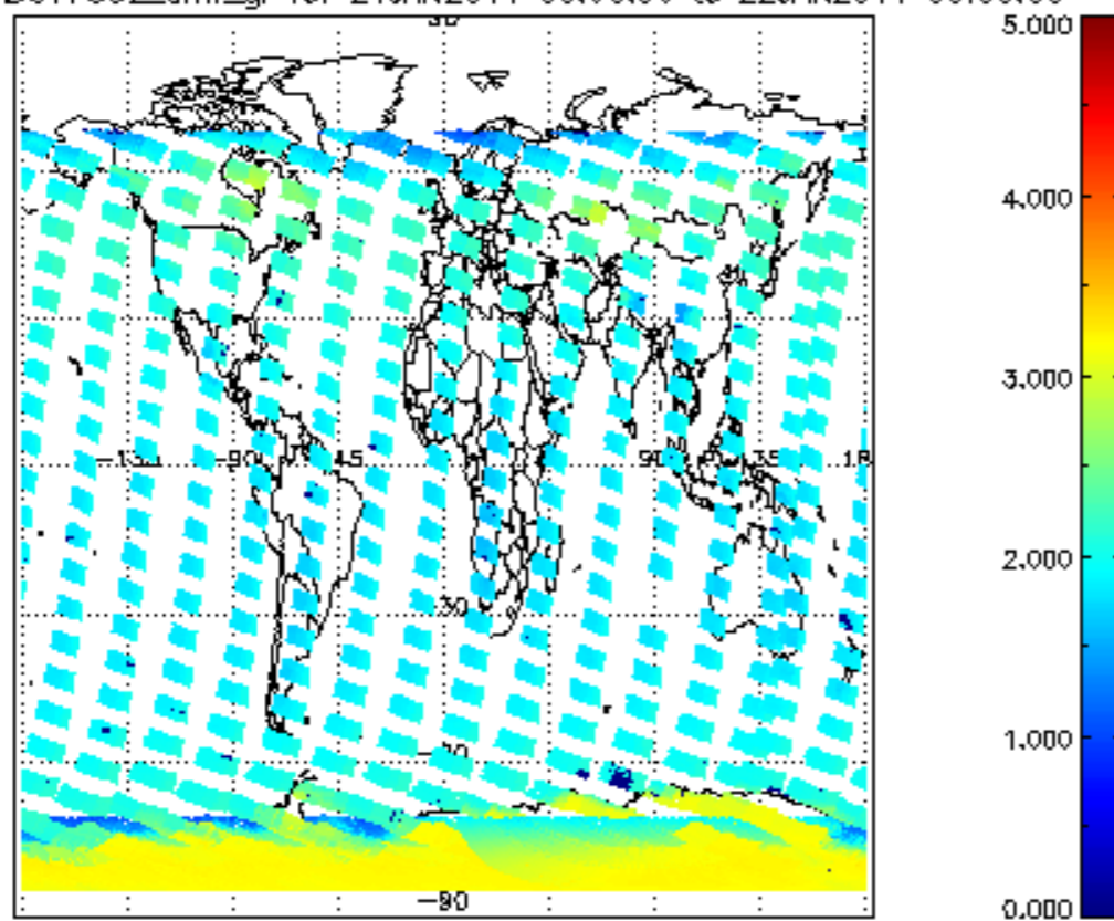
SCIOL2P_NADUV7S02_amf_gr for 21JAN2011 00:00:00 to 22JAN2011 00:00:00
