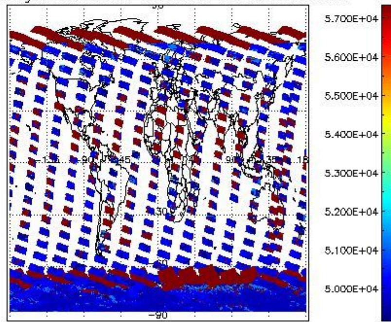
cloud_flags for 21JAN2011 00:00:00 to 22JAN2011 00:00:00
