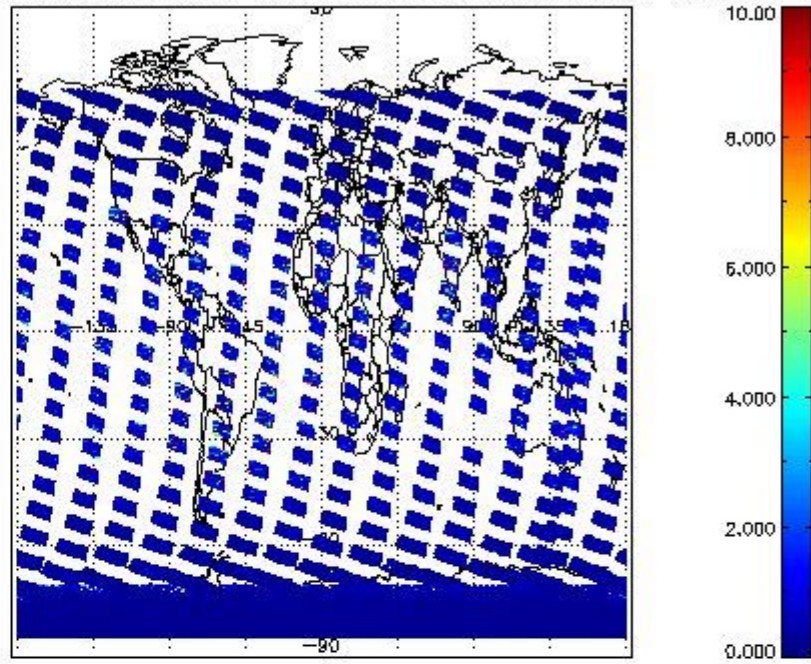
SCIOL2P_NADUV3BRO_vcd_err for 21JAN2011 00:00:00 to 22JAN2011 00:00:00
