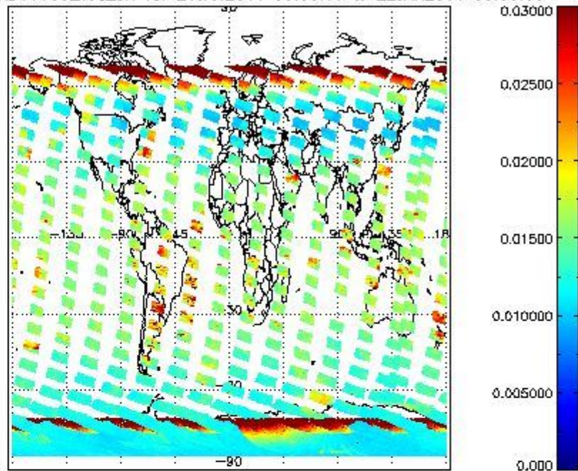
SCIOL2P_NADUV003_vcd_err for 21JAN2011 00:00:00 to 22JAN2011 00:00:00
