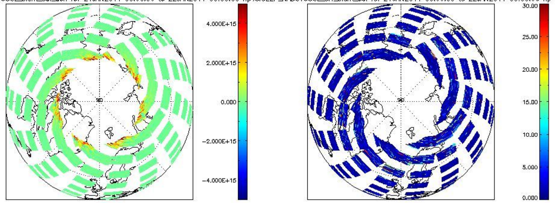
SCIOI2P_NADUV60CL_slant_col_den for 21JAN2011 00:00:00 to 22JAN2011 00:00:00 np; SCIOI2P_NADUV60CL_err_slant_col for 21JAN2011 00:00:00 to 22JAN2011 00:00:00 np
