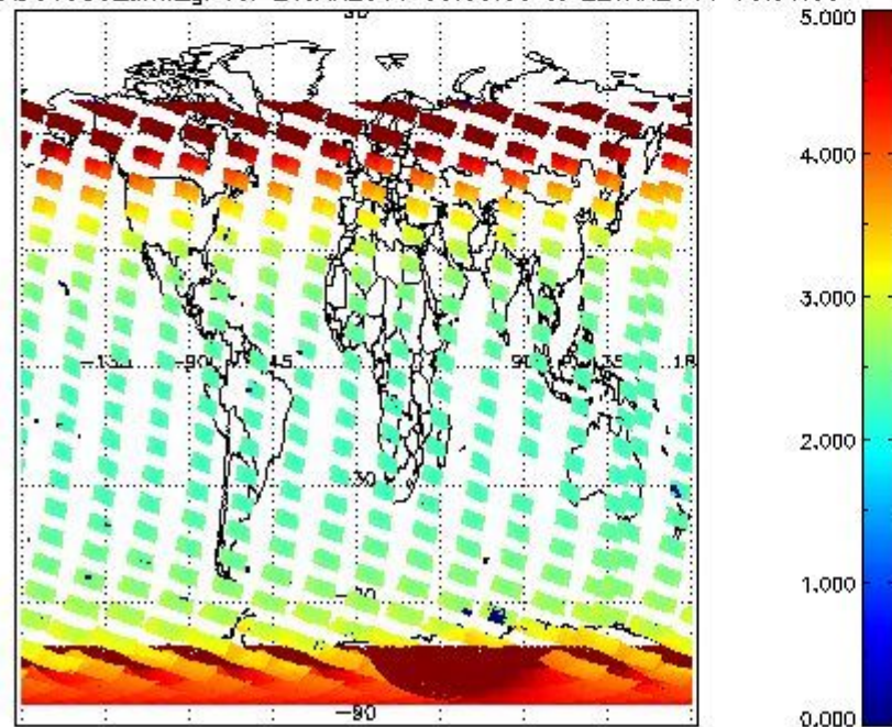
SCIOL2P_NADUV003_amf_gr for 21JAN2011 00:00:00 to 22JAN2011 00:00:00
