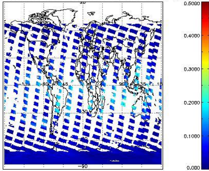
SCIOL2P_NADUV8H20_vcd_err for 21JAN2011 00:00:00 to 22JAN2011 00:00:00
