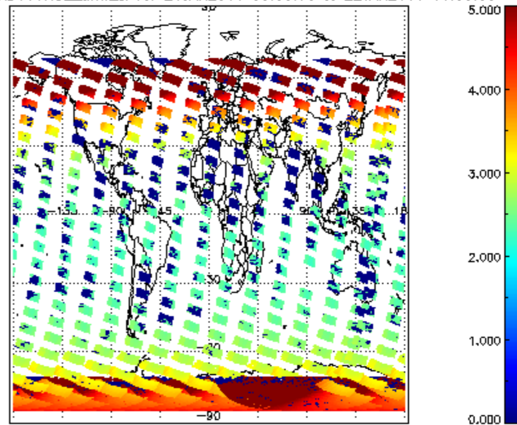
SCIOL2P_NADUV1NO2_amf_cl for 21JAN2011 00:00:00 to 22JAN2011 00:00:00
