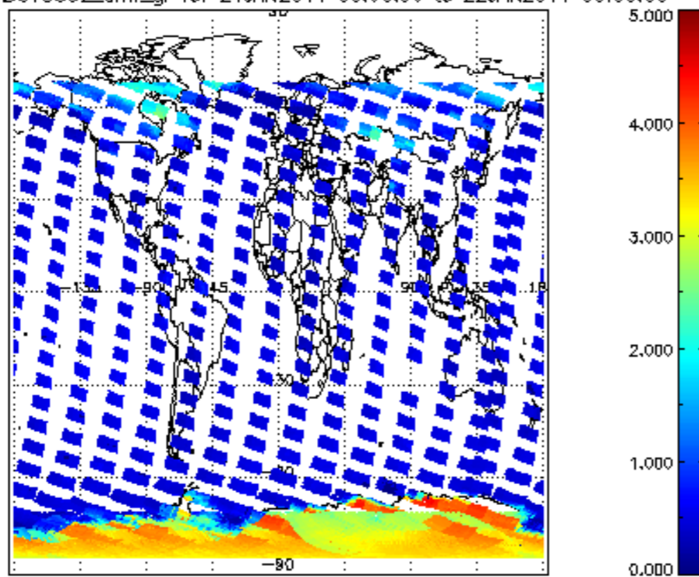
SCIOL2P_NADUV5S02_amf_gr for 21JAN2011 00:00:00 to 22JAN2011 00:00:00
