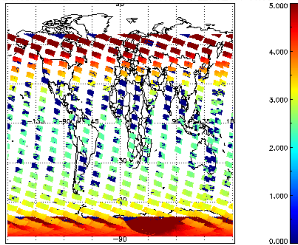
SCIOL2P_NADUV3BRO_amf_cl for 21JAN2011 00:00:00 to 22JAN2011 00:00:00
