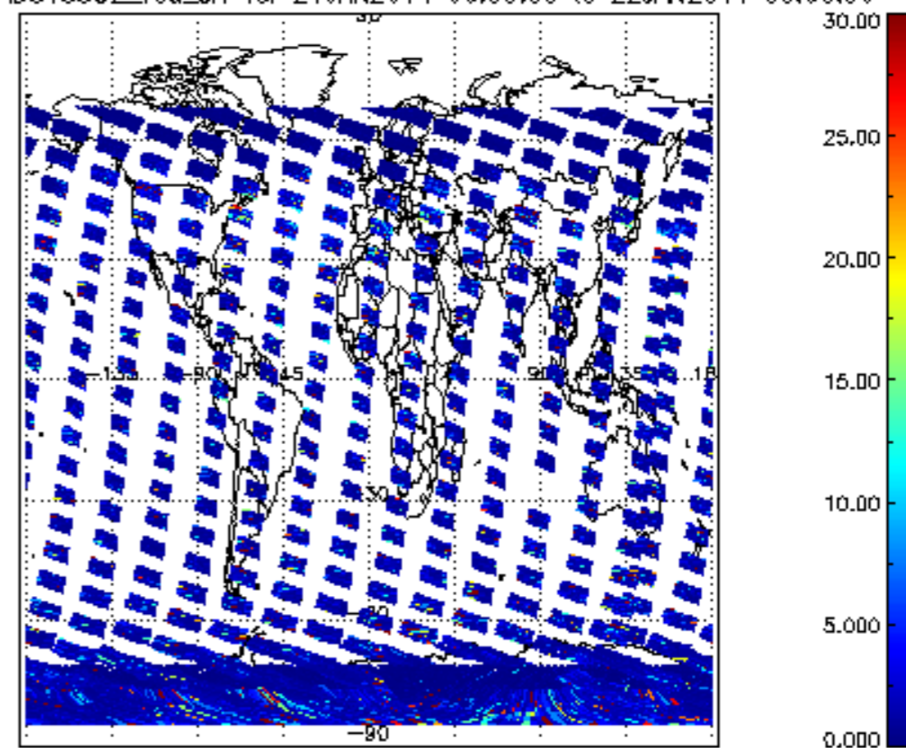
SCIOL2P_NADUV5S02_vcd_err for 21JAN2011 00:00:00 to 22JAN2011 00:00:00
