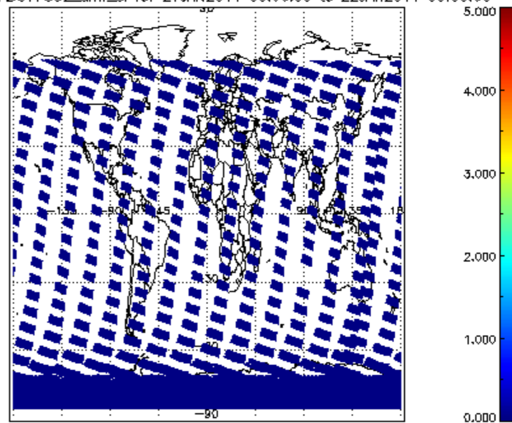
SCIOL2P_NADUV7S02_amf_cl for 21JAN2011 00:00:00 to 22JAN2011 00:00:00
