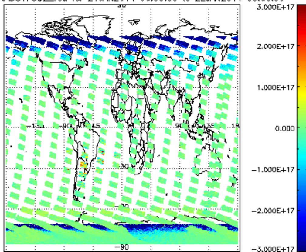
SCIOL2P_NADUV7S02_vcd for 21JAN2011 00:00:00 to 22JAN2011 00:00:00
