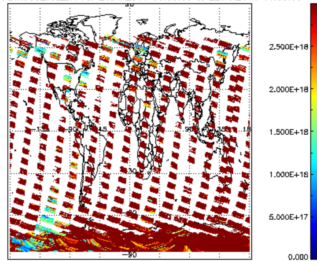
SCIOL2P_NADIR3CO_vcd_err for 21JAN2011 00:00:00 to 22JAN2011 00:00:00
