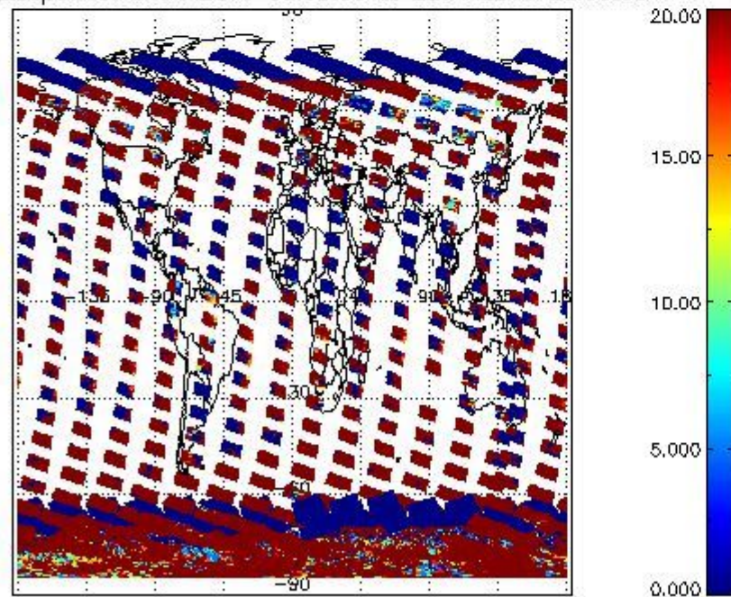
cLopt_depth for 21JAN2011 00:00:00 to 22JAN2011 00:00:00
