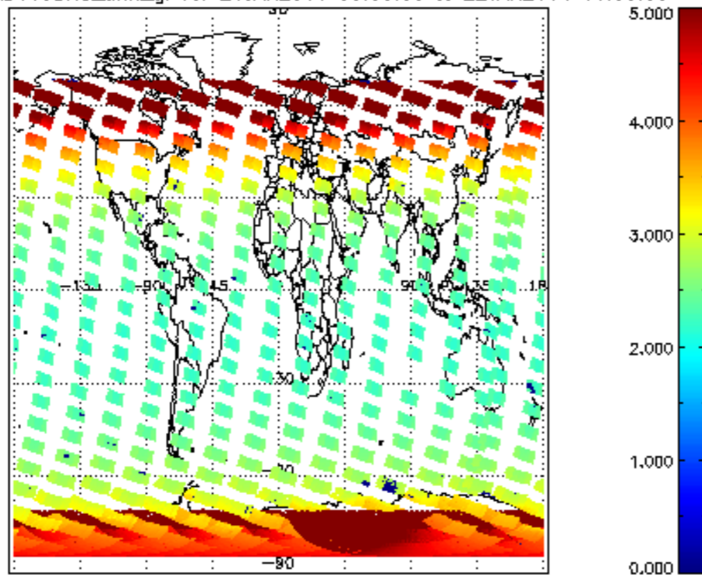
SCIOL2P_NADUV3BRO_amf_gr for 21JAN2011 00:00:00 to 22JAN2011 00:00:00
