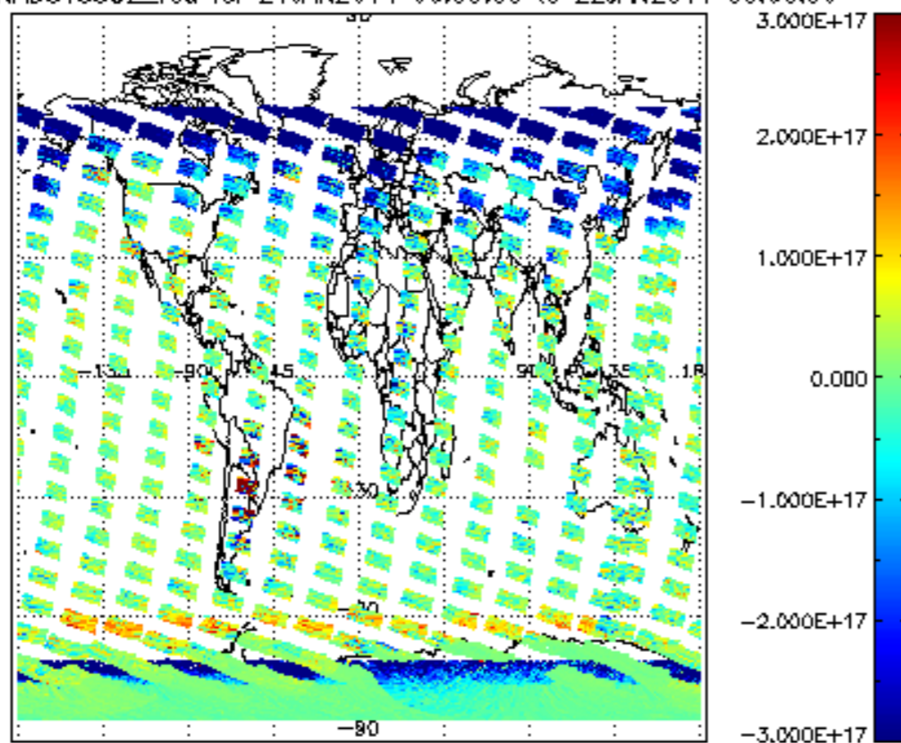
SCIOL2P_NADUV5S02_vcd for 21JAN2011 00:00:00 to 22JAN2011 00:00:00
