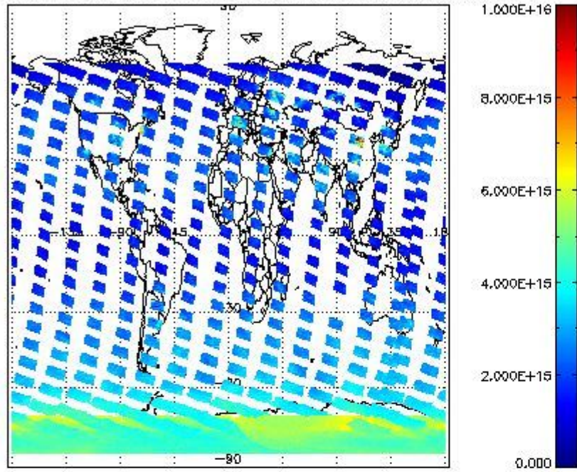
SCIOL2P_NADUV1NO2_vcd for 21JAN2011 00:00:00 to 22JAN2011 00:00:00
