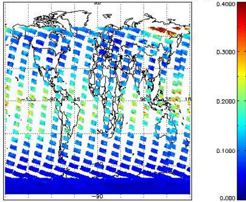
SCIOL2P_NADUV1NO2_vcd_err for 21JAN2011 00:00:00 to 22JAN2011 00:00:00
