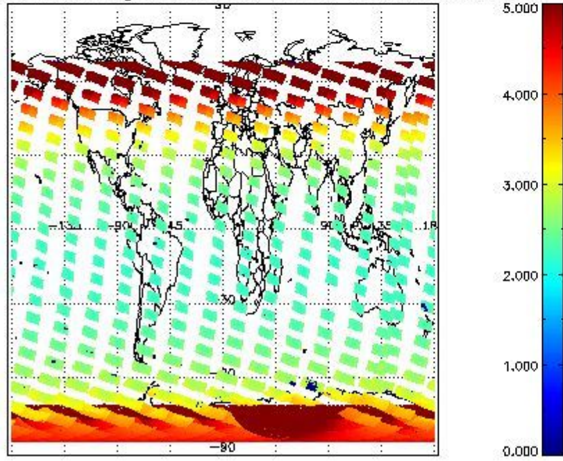
SCIOL2P_NADUV3BRO_amf_gr for 21JAN2011 00:00:00 to 22JAN2011 00:00:00
