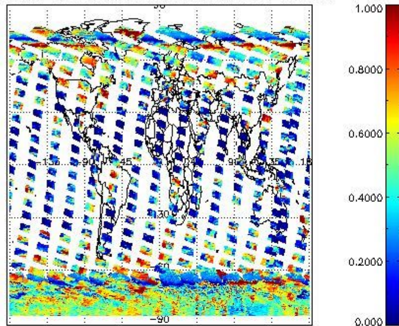
cL_frac for 21JAN2011 00:00:00 to 22JAN2011 00:00:00
