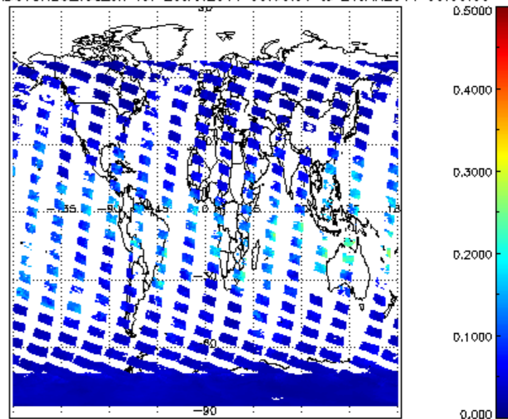
SCIOL2P_NADUV8H20_vcd_err for 20JAN2011 00:00:00 to 21JAN2011 00:00:00
