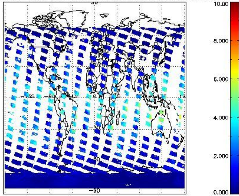
SCIOL2P_NADUV8H20_vcd for 20JAN2011 00:00:00 to 21JAN2011 00:00:00
