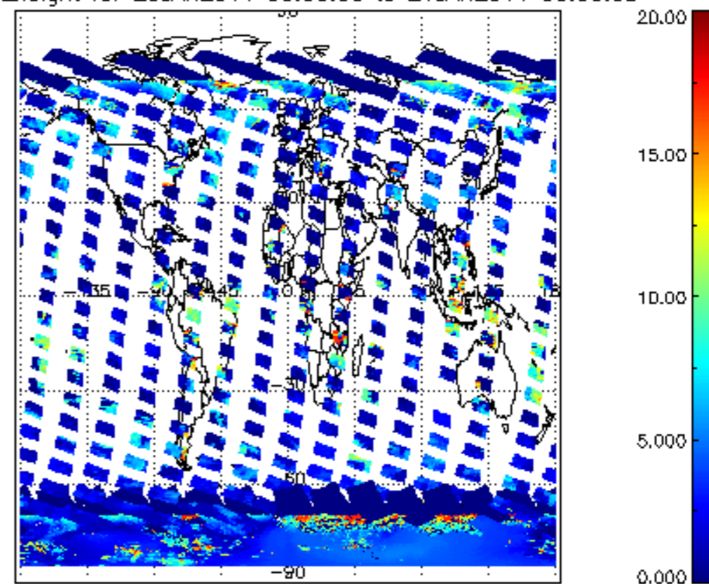
cL_top_height for 20JAN2011 00:00:00 to 21JAN2011 00:00:00
