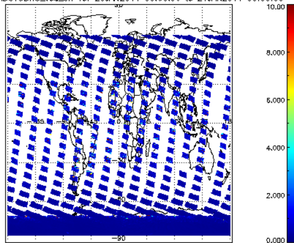
SCIOL2P_NADUV3BRO_vcd_err for 20JAN2011 00:00:00 to 21JAN2011 00:00:00
