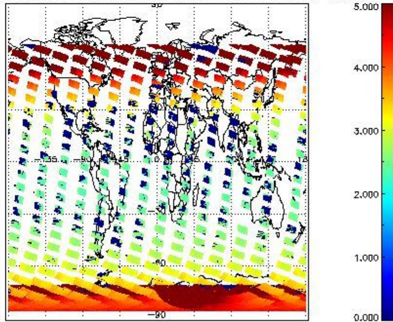
SCIOL2P_NADUV3BRO_amf_cl for 20JAN2011 00:00:00 to 21JAN2011 00:00:00
