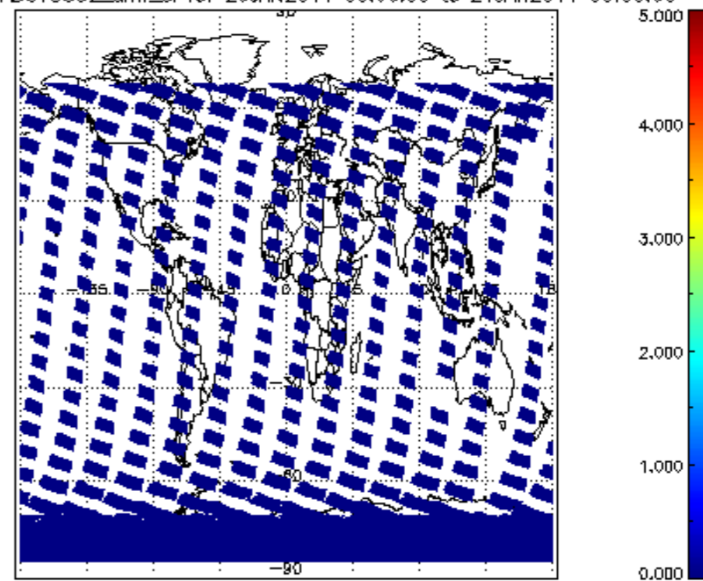
SCIOL2P_NADUV5S02_amf_sl for 20JAN2011 00:00:00 to 21JAN2011 00:00:00
