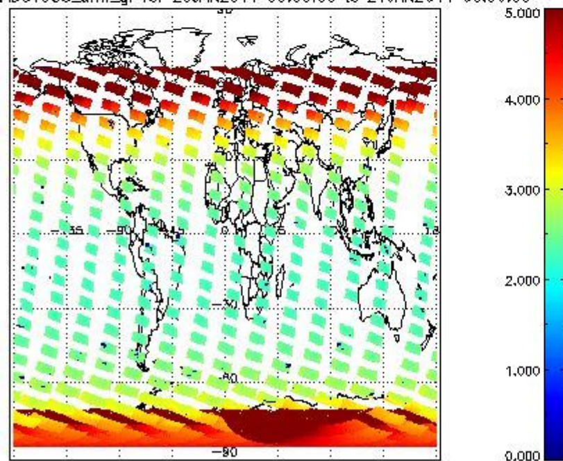
SCIOL2P_NADUV003_amf_gr for 20JAN2011 00:00:00 to 21JAN2011 00:00:00
