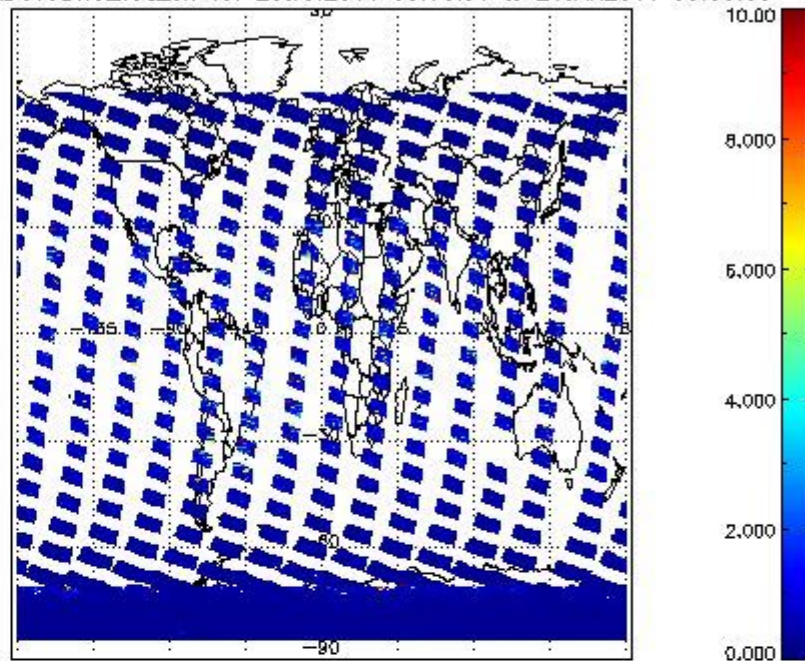
SCIOL2P_NADUV3BRO_vcd_err for 20JAN2011 00:00:00 to 21JAN2011 00:00:00
