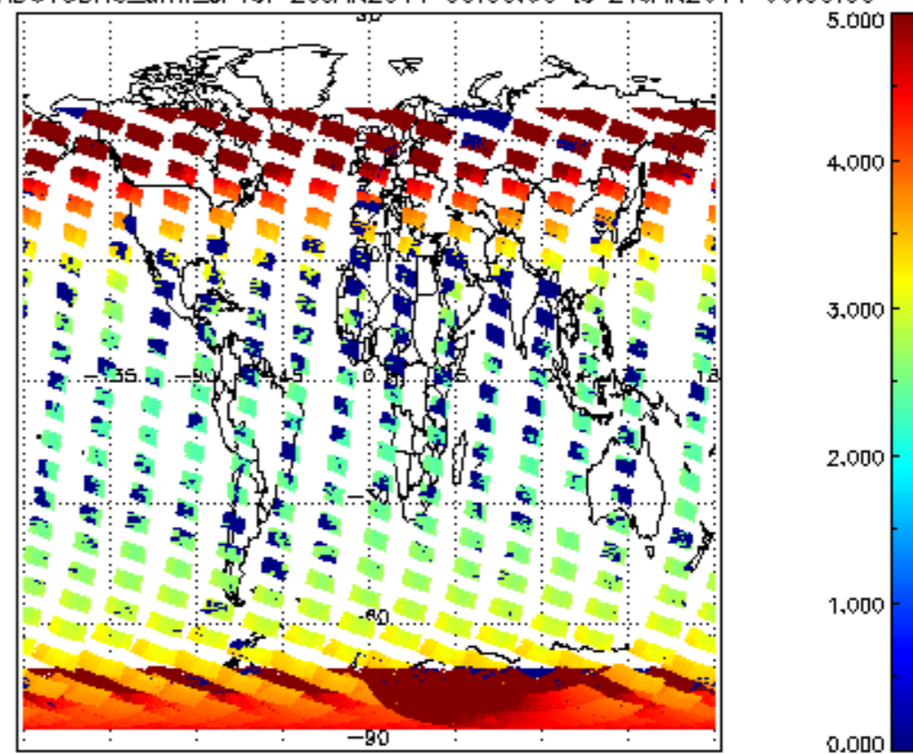
SCIOL2P_NADUV3BRO_amf_cl for 20JAN2011 00:00:00 to 21JAN2011 00:00:00
