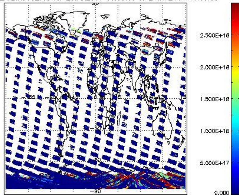
SCIDL2P_NADIR3CO_vcd for 20JAN2011 00:00:00 to 21JAN2011 00:00:00
