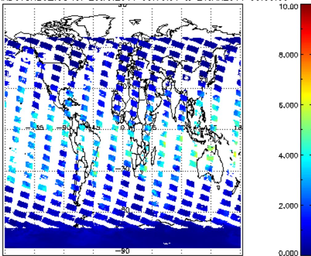
SCIOL2P_NADUV8H20_vcd for 20JAN2011 00:00:00 to 21JAN2011 00:00:00
