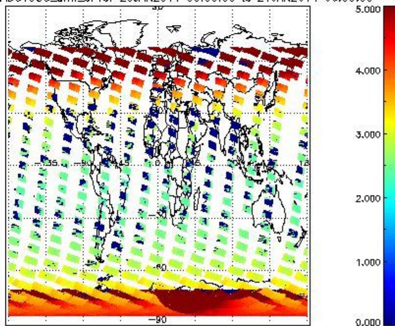
SCIOL2P_NADUV003_amf_cl for 20JAN2011 00:00:00 to 21JAN2011 00:00:00
