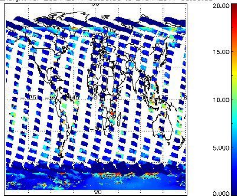
cL_top_height for 20JAN2011 00:00:00 to 21JAN2011 00:00:00
