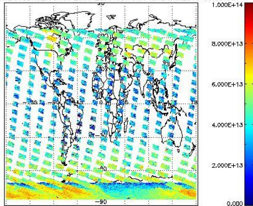
SCIOL2P_NADUV3BRO_vcd for 20JAN2011 00:00:00 to 21JAN2011 00:00:00
