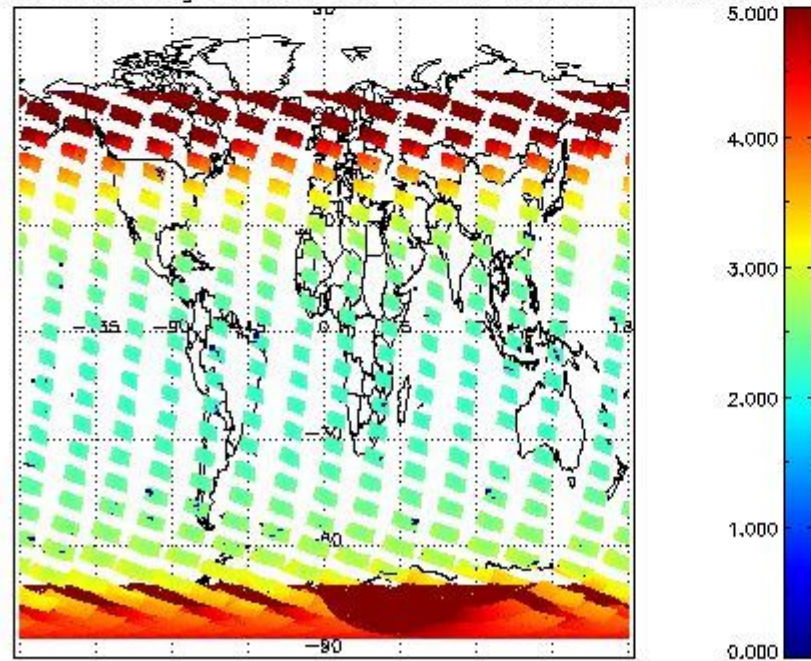
SCIOL2P_NADUV3BRO_amf_gr for 20JAN2011 00:00:00 to 21JAN2011 00:00:00
