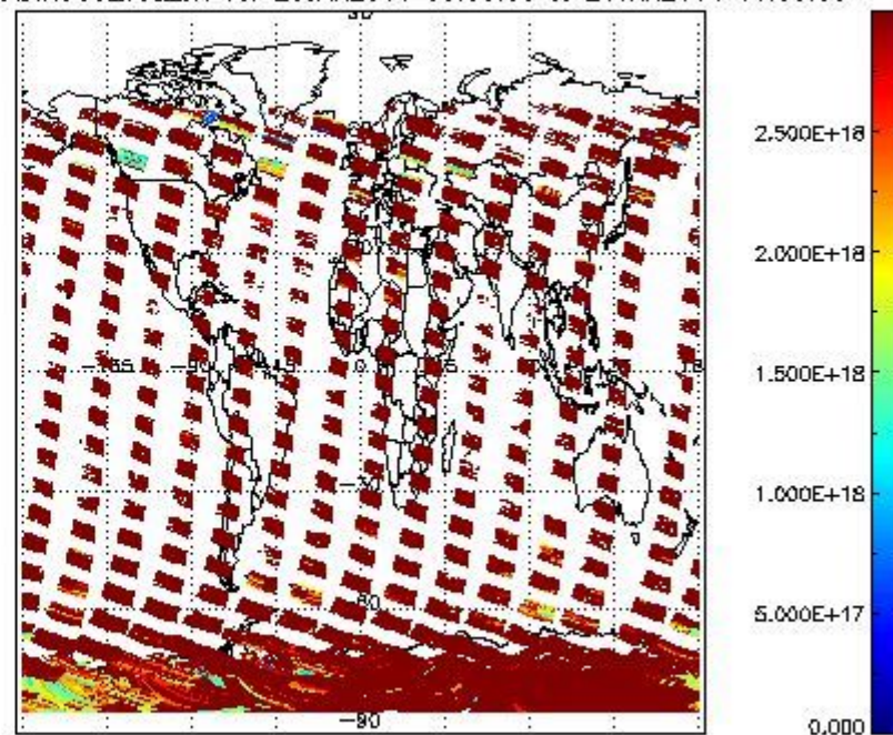
SCIDL2P_NADIR3CO_vcd_err for 20JAN2011 00:00:00 to 21JAN2011 00:00:00
