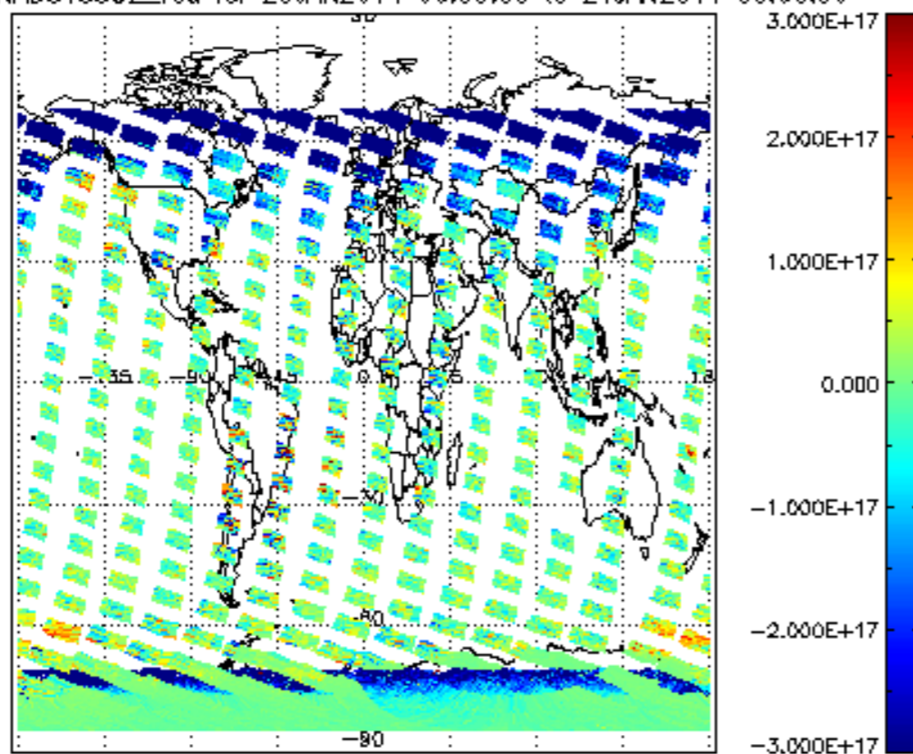
SCIOL2P_NADUV5S02_vcd for 20JAN2011 00:00:00 to 21JAN2011 00:00:00
