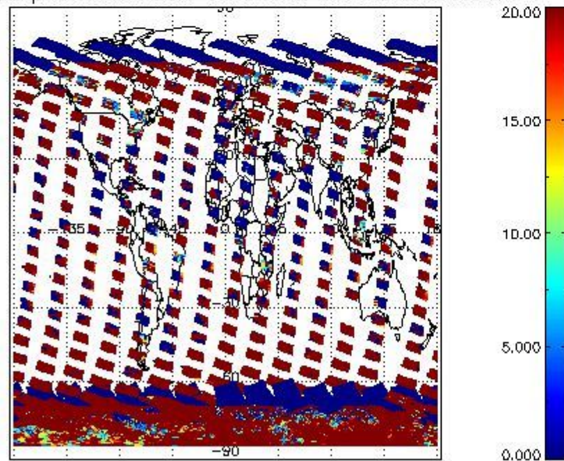
cLopt_depth for 20JAN2011 00:00:00 to 21JAN2011 00:00:00
