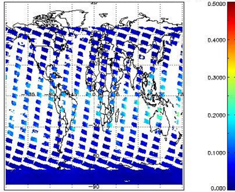
SCIOL2P_NADUV8H20_vcd_err for 20JAN2011 00:00:00 to 21JAN2011 00:00:00
