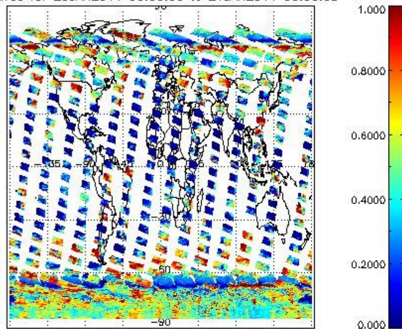
cL_frac for 20JAN2011 00:00:00 to 21JAN2011 00:00:00
