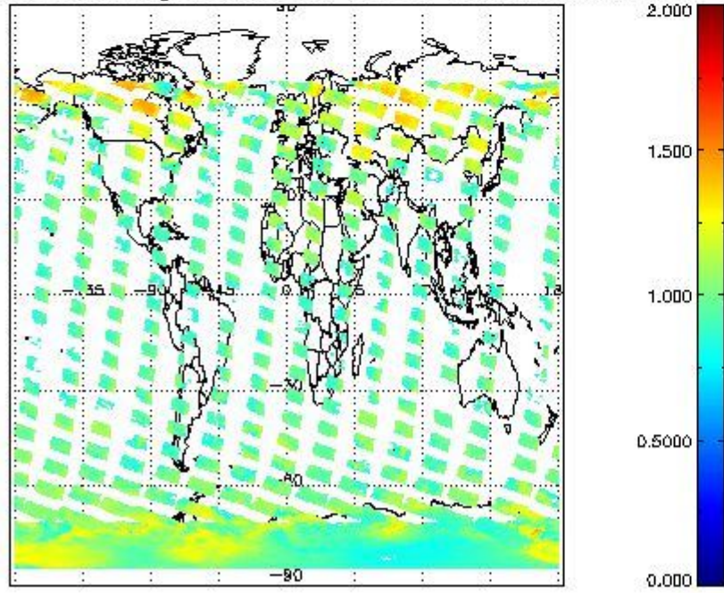
SCIOL2P_NADUV8H20_amf_gr for 20JAN2011 00:00:00 to 21JAN2011 00:00:00
