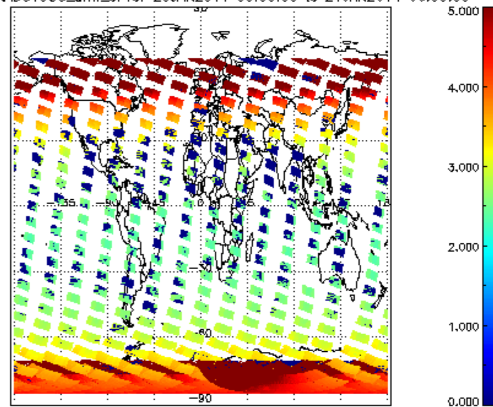
SCIOL2P_NADUV003_amf_cl for 20JAN2011 00:00:00 to 21JAN2011 00:00:00
