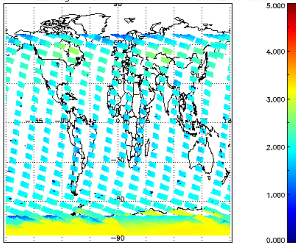
SCIOL2P_NADUV7S02_amf_gr for 20JAN2011 00:00:00 to 21JAN2011 00:00:00
