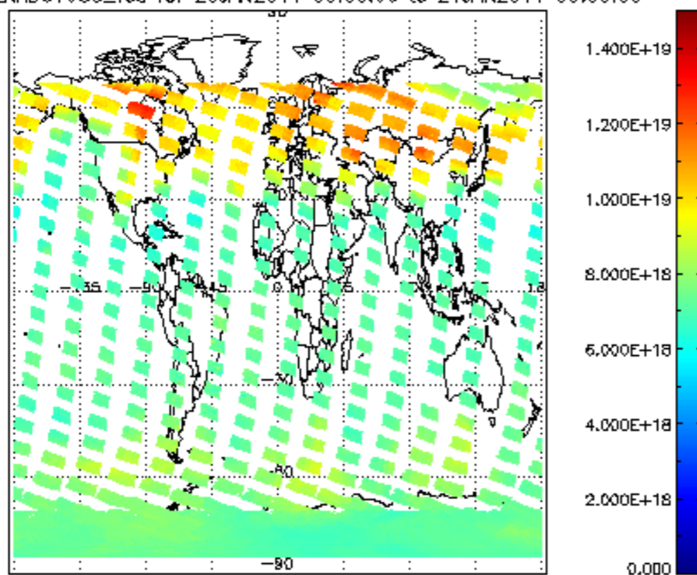
SCIOL2P_NADUV003_vcd for 20JAN2011 00:00:00 to 21JAN2011 00:00:00
