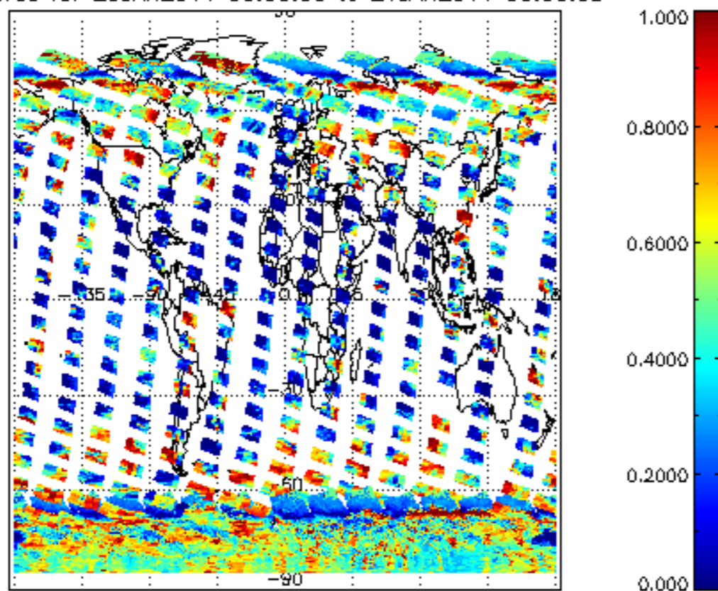
cL_frac for 20JAN2011 00:00:00 to 21JAN2011 00:00:00
