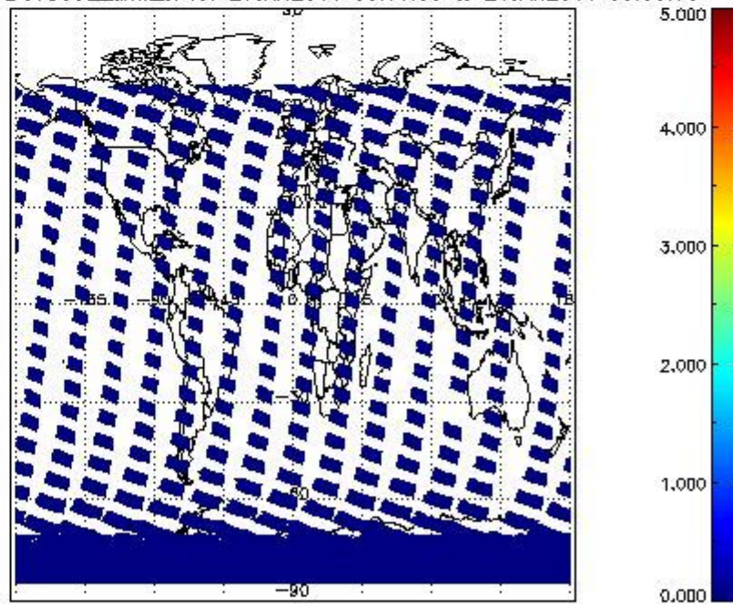
SCIOL2P_NADUV5SO2_amf_cl for 20JAN2011 00:00:00 to 21JAN2011 00:00:00
