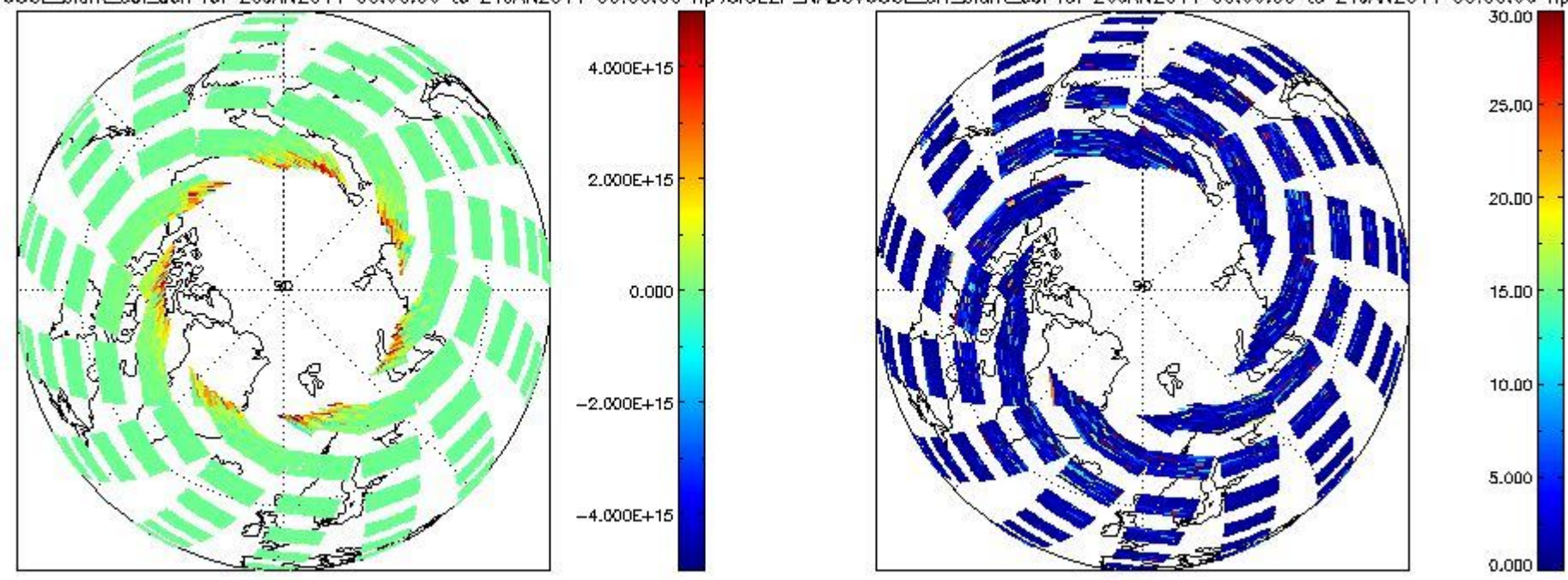
SCIOI2P_NADUV60CL_slant_col_den for 20JAN2011 00:00:00 to 21JAN2011 00:00:00 np; SCIOI2P_NADUV60CL_err_slant_col for 20JAN2011 00:00:00 to 21JAN2011 00:00:00 np
