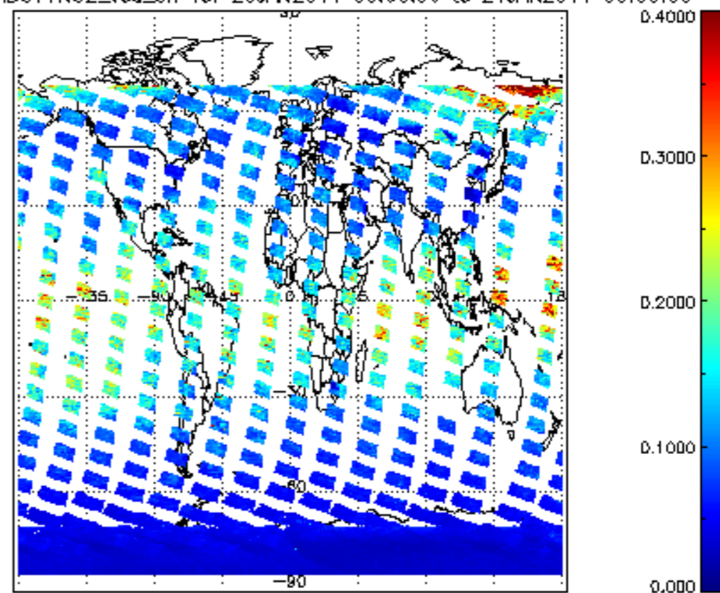
SCIOL2P_NADUV1NO2_vcd_err for 20JAN2011 00:00:00 to 21JAN2011 00:00:00
