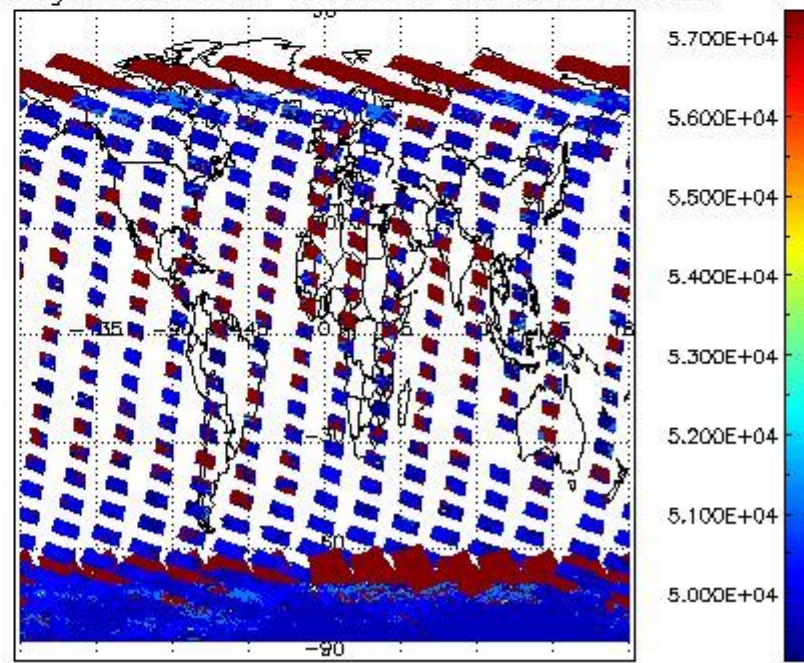
cloud_flags for 20JAN2011 00:00:00 to 21JAN2011 00:00:00
