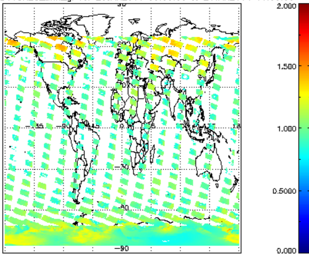
SCIOL2P_NADUV8H20_amf_gr for 20JAN2011 00:00:00 to 21JAN2011 00:00:00
