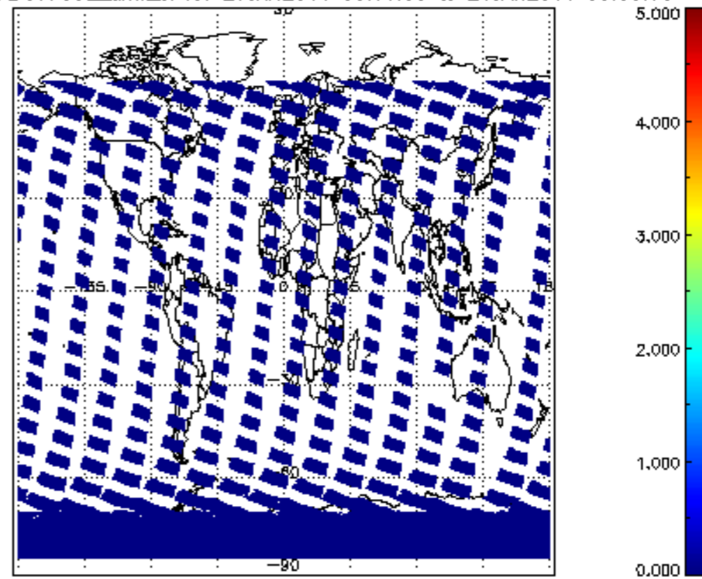
SCIOL2P_NADUV7S02_amf_sl for 20JAN2011 00:00:00 to 21JAN2011 00:00:00
