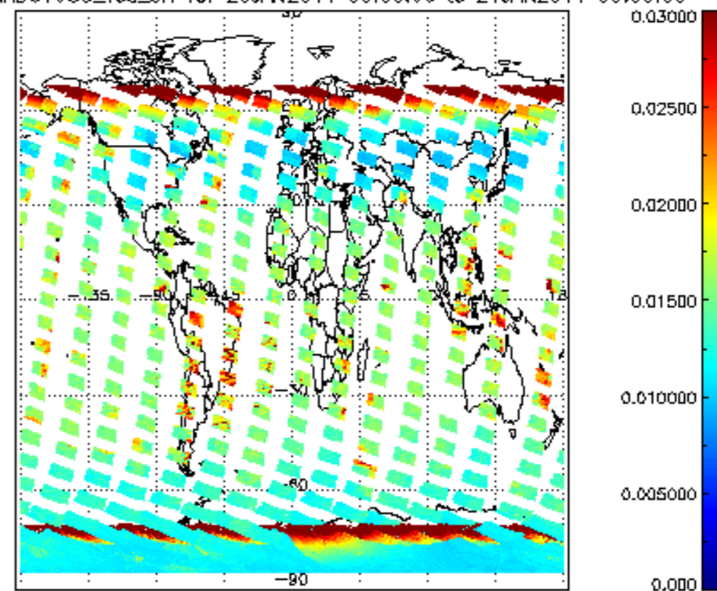
SCIOL2P_NADUV003_vcd_err for 20JAN2011 00:00:00 to 21JAN2011 00:00:00
