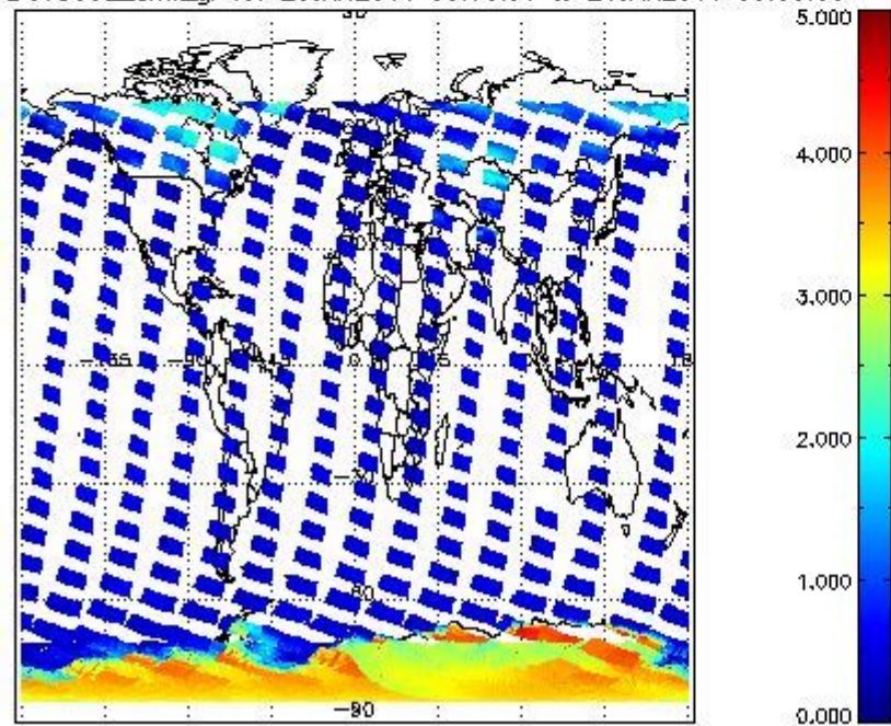
SCIOL2P_NADUV5SO2_amf_gr for 20JAN2011 00:00:00 to 21JAN2011 00:00:00
