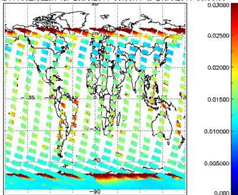
SCIOL2P_NADUV003_vcd_err for 20JAN2011 00:00:00 to 21JAN2011 00:00:00
