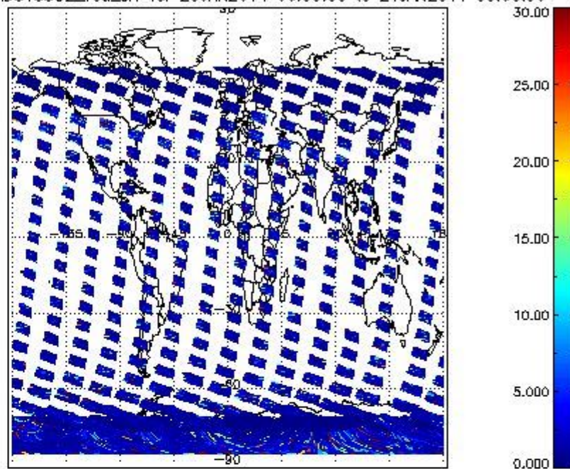
SCIOL2P_NADUV5SO2_vcd_err for 20JAN2011 00:00:00 to 21JAN2011 00:00:00
