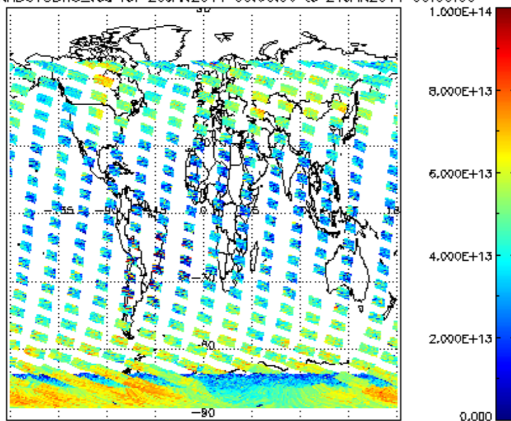
SCIOL2P_NADUV3BRO_vcd for 20JAN2011 00:00:00 to 21JAN2011 00:00:00
