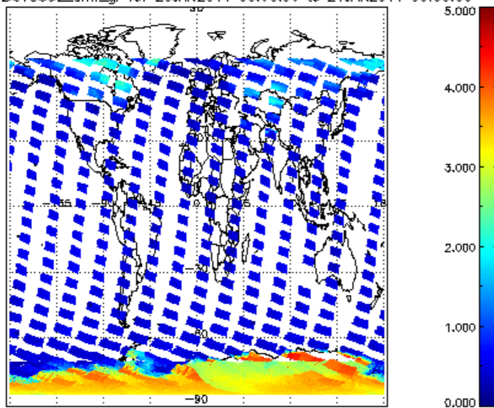
SCIOL2P_NADUV5S02_amf_gr for 20JAN2011 00:00:00 to 21JAN2011 00:00:00
