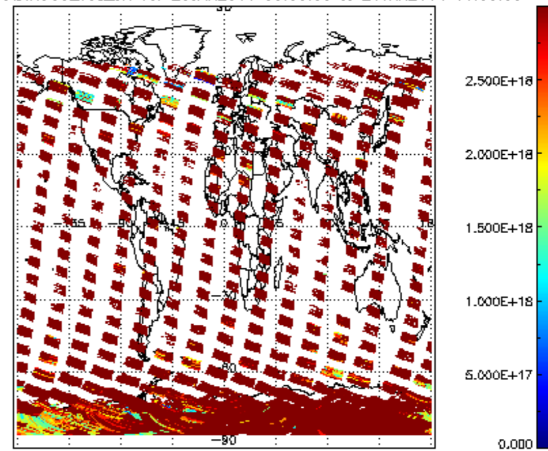
SCIOL2P_NADIR3CO_vcd_err for 20JAN2011 00:00:00 to 21JAN2011 00:00:00
