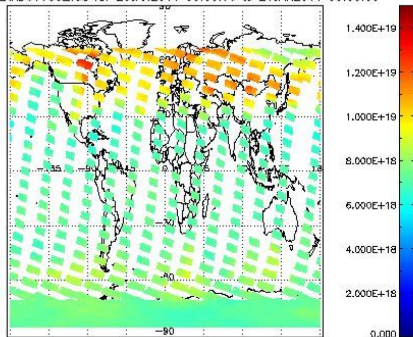
SCIOL2P_NADUV003_vcd for 20JAN2011 00:00:00 to 21JAN2011 00:00:00
