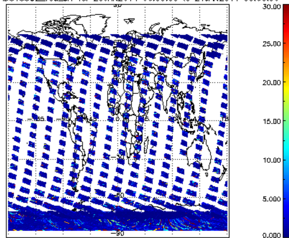
SCIOL2P_NADUV5S02_vcd_err for 20JAN2011 00:00:00 to 21JAN2011 00:00:00
