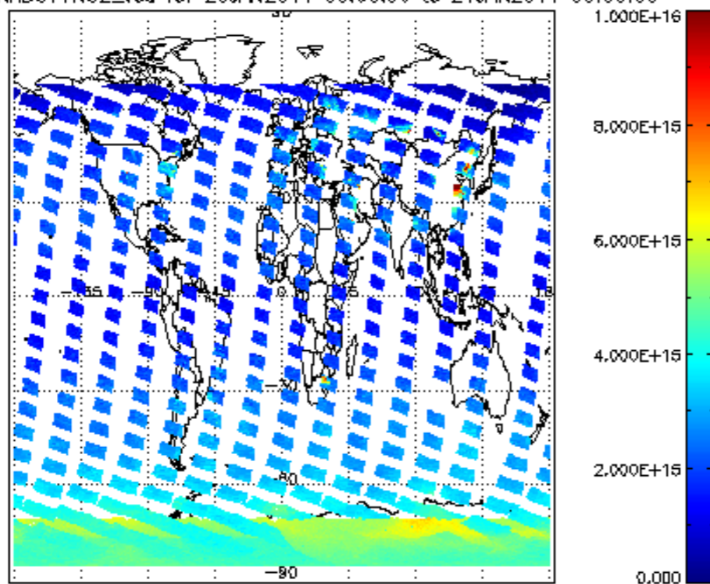
SCIOL2P_NADUV1NO2_vcd for 20JAN2011 00:00:00 to 21JAN2011 00:00:00
