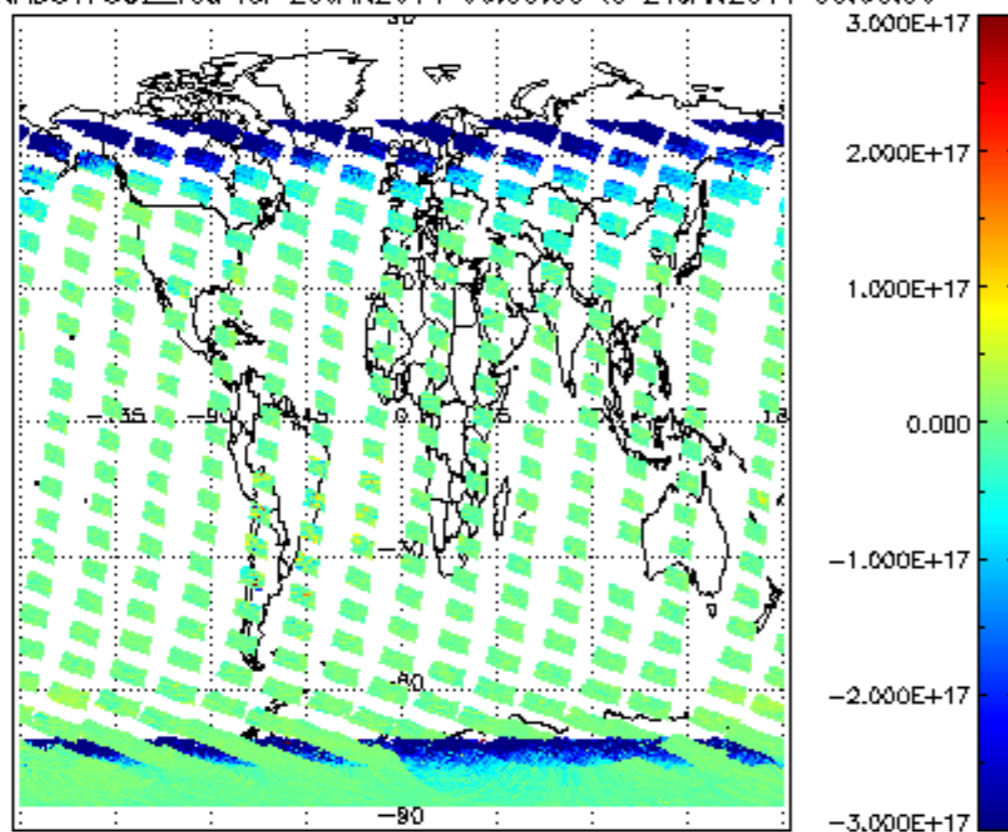
SCIOL2P_NADUV7S02_vcd for 20JAN2011 00:00:00 to 21JAN2011 00:00:00
