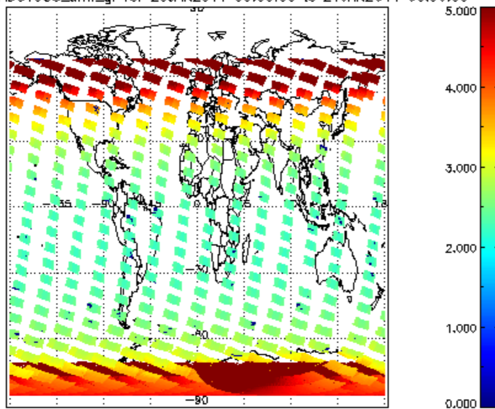
SCIOL2P_NADUV003_amf_gr for 20JAN2011 00:00:00 to 21JAN2011 00:00:00
