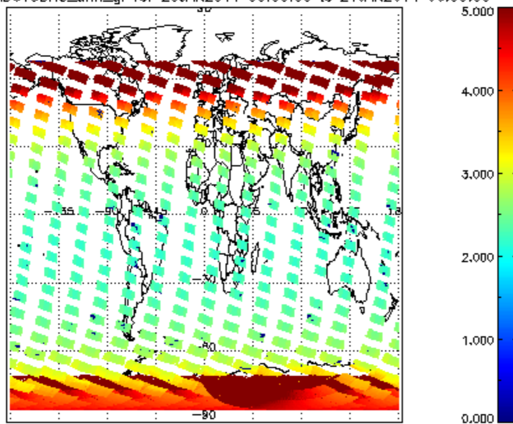
SCIOL2P_NADUV3BRO_amf_gr for 20JAN2011 00:00:00 to 21JAN2011 00:00:00
