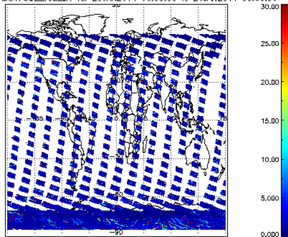
SCIOL2P_NADUV7S02_vcd_err for 20JAN2011 00:00:00 to 21JAN2011 00:00:00
