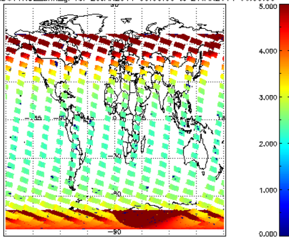
SCIOL2P_NADUV1NO2_amf_gr for 20JAN2011 00:00:00 to 21JAN2011 00:00:00
