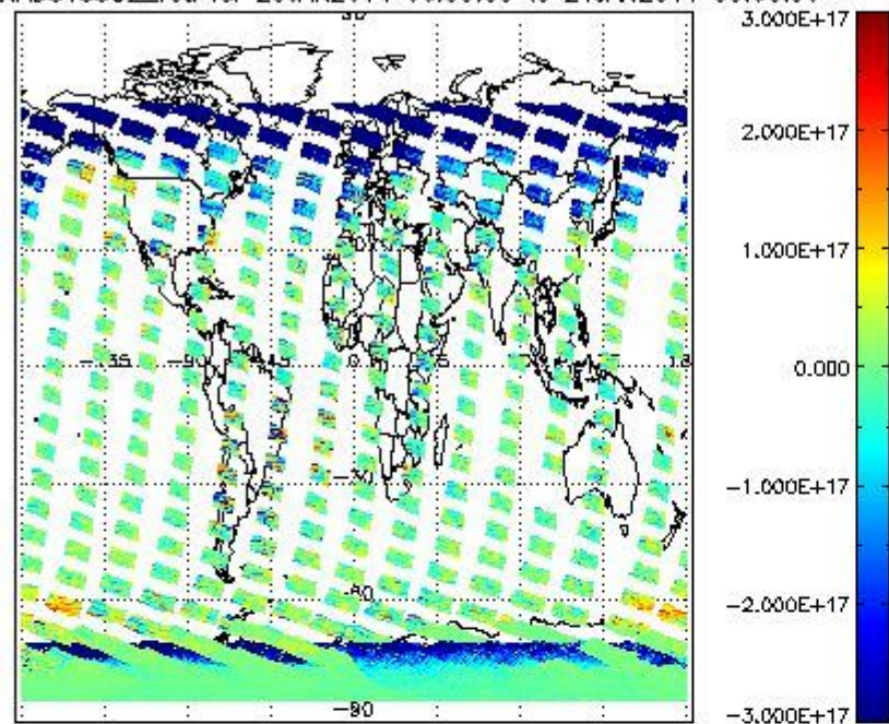
SCIOL2P_NADUV5SO2_vcd for 20JAN2011 00:00:00 to 21JAN2011 00:00:00
