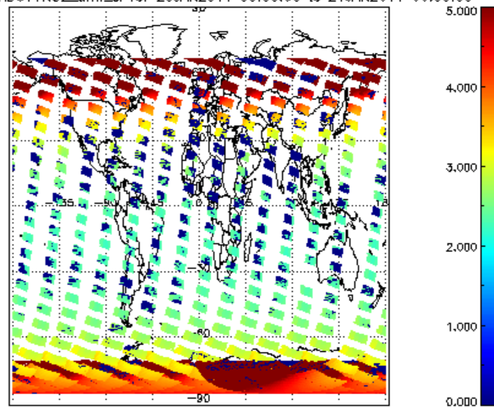
SCIOL2P_NADUV1NO2_amf_cl for 20JAN2011 00:00:00 to 21JAN2011 00:00:00
