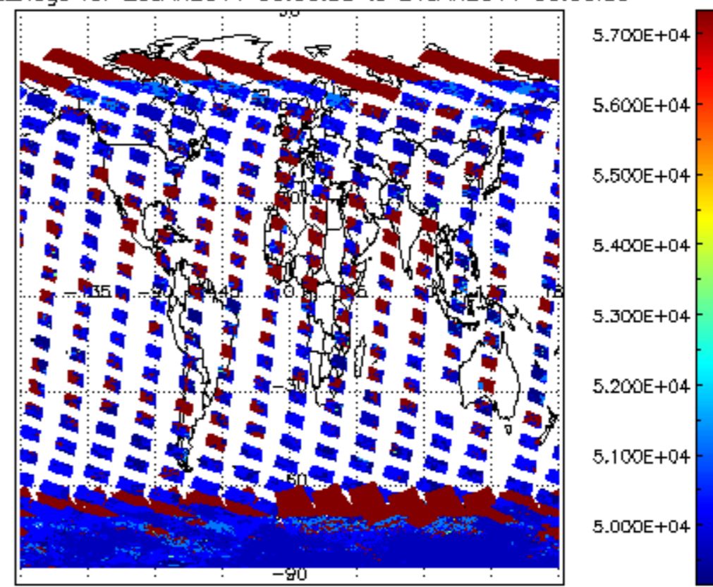
cloud_flags for 20JAN2011 00:00:00 to 21JAN2011 00:00:00
