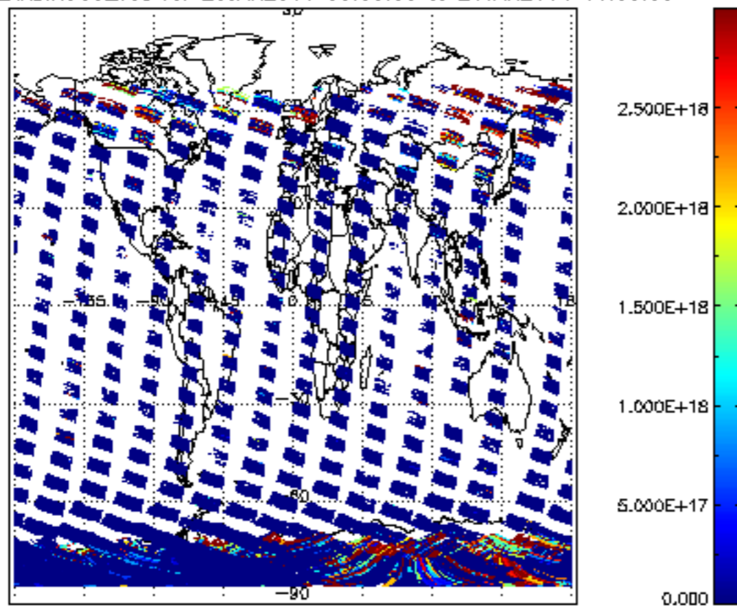
SCIOL2P_NADIR3CO_vcd for 20JAN2011 00:00:00 to 21JAN2011 00:00:00
