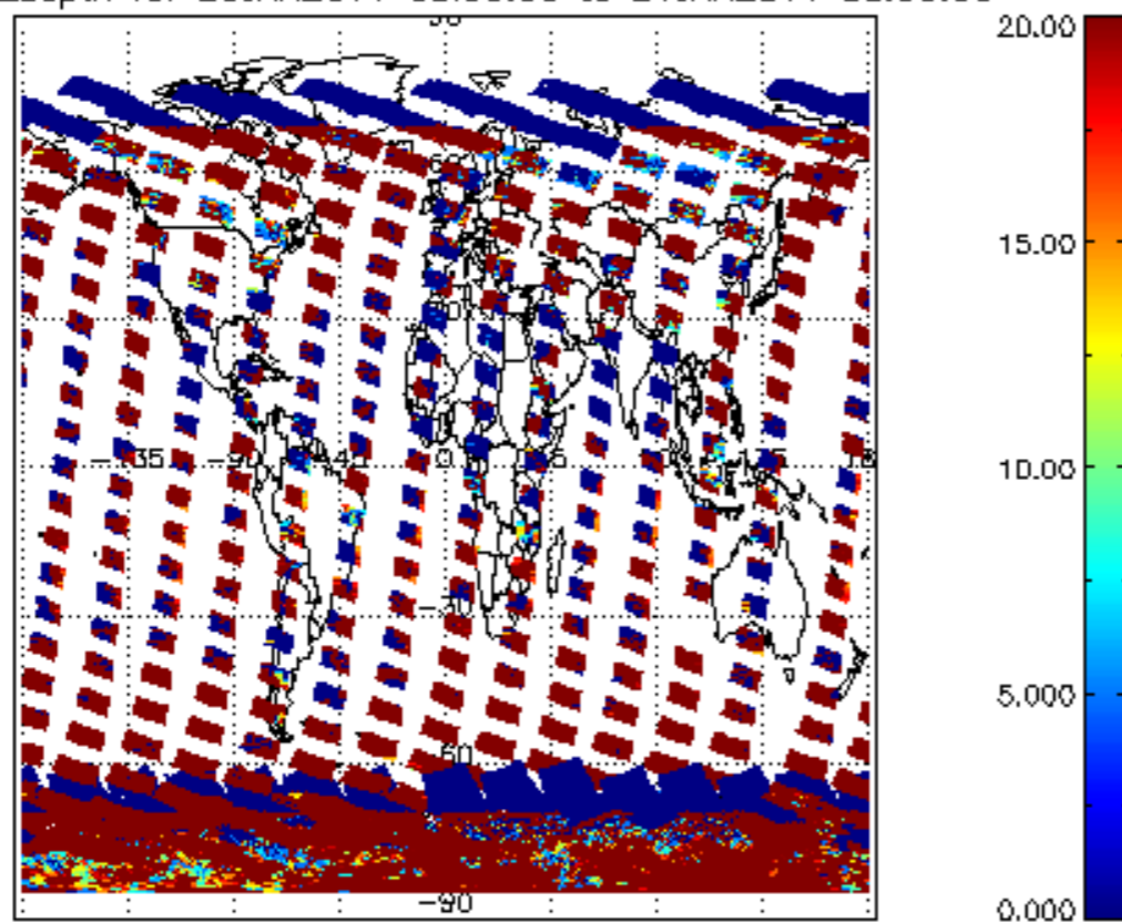
cLopt_depth for 20JAN2011 00:00:00 to 21JAN2011 00:00:00
