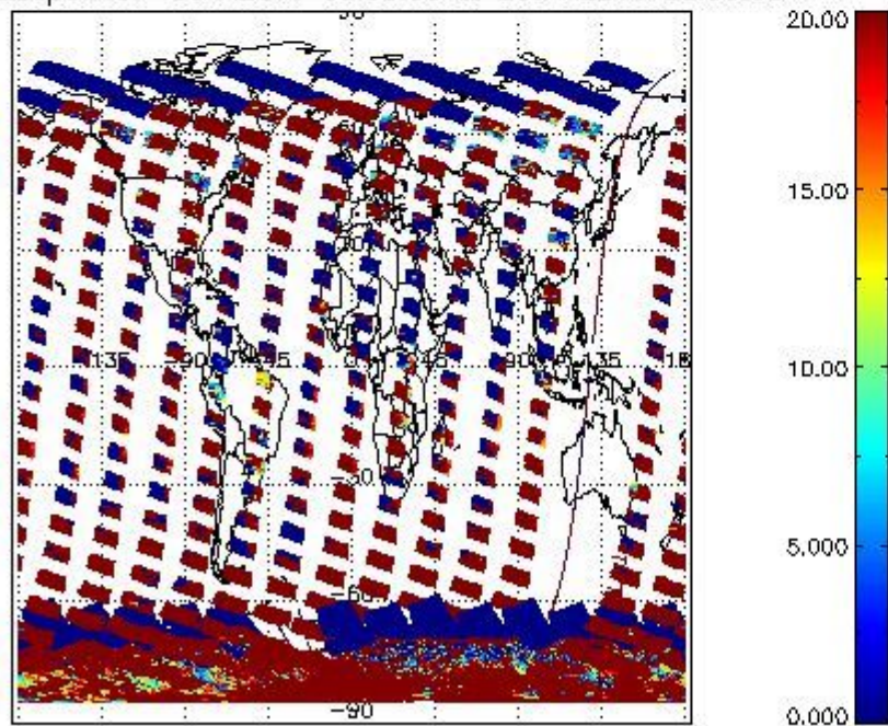
cLopt_depth for 19JAN2011 00:00:00 to 20JAN2011 00:00:00
