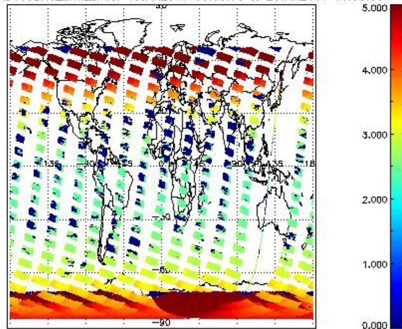
SCIOL2P_NADUV3BRO_amf_cl for 19JAN2011 00:00:00 to 20JAN2011 00:00:00
