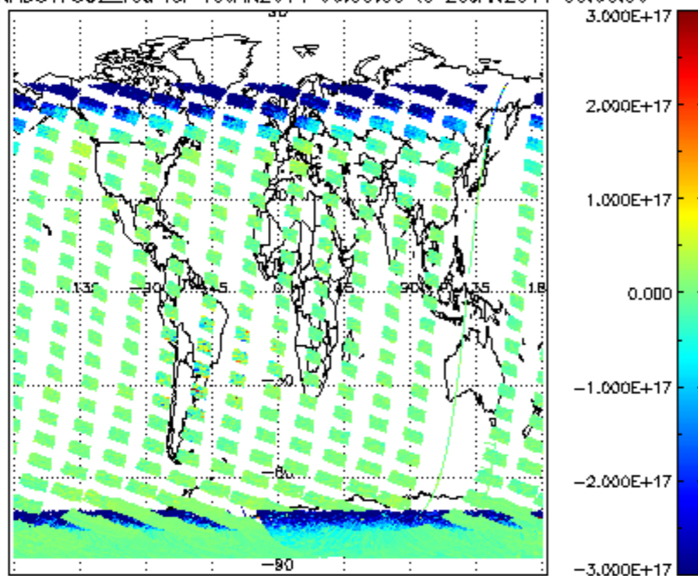
SCIOL2P_NADUV7S02_vcd for 19JAN2011 00:00:00 to 20JAN2011 00:00:00
