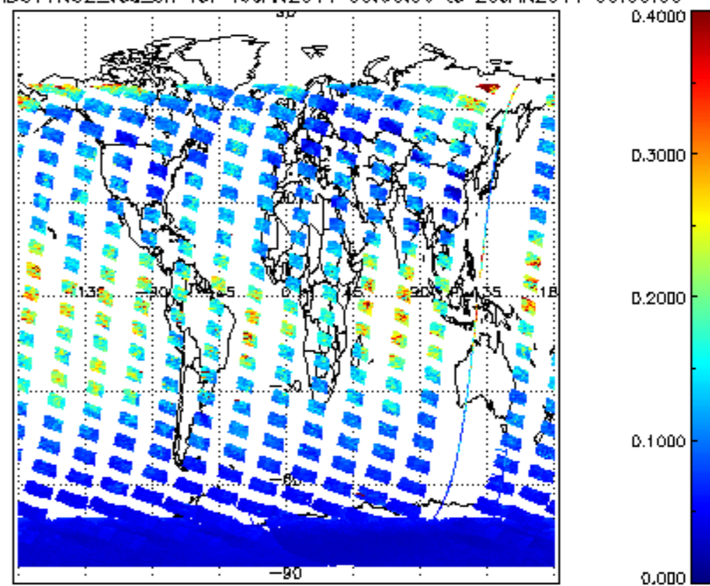
SCIOL2P_NADUV1NO2_vcd_err for 19JAN2011 00:00:00 to 20JAN2011 00:00:00
