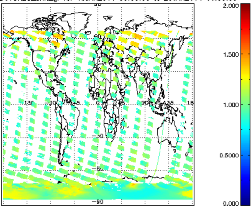
SCIOL2P_NADUV8H20_amf_gr for 19JAN2011 00:00:00 to 20JAN2011 00:00:00
