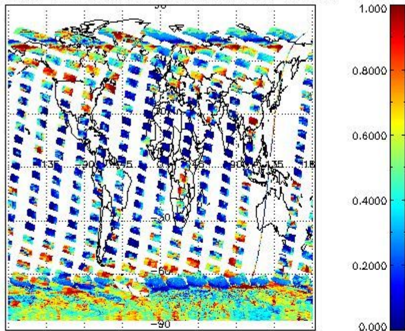
cL_frac for 19JAN2011 00:00:00 to 20JAN2011 00:00:00
