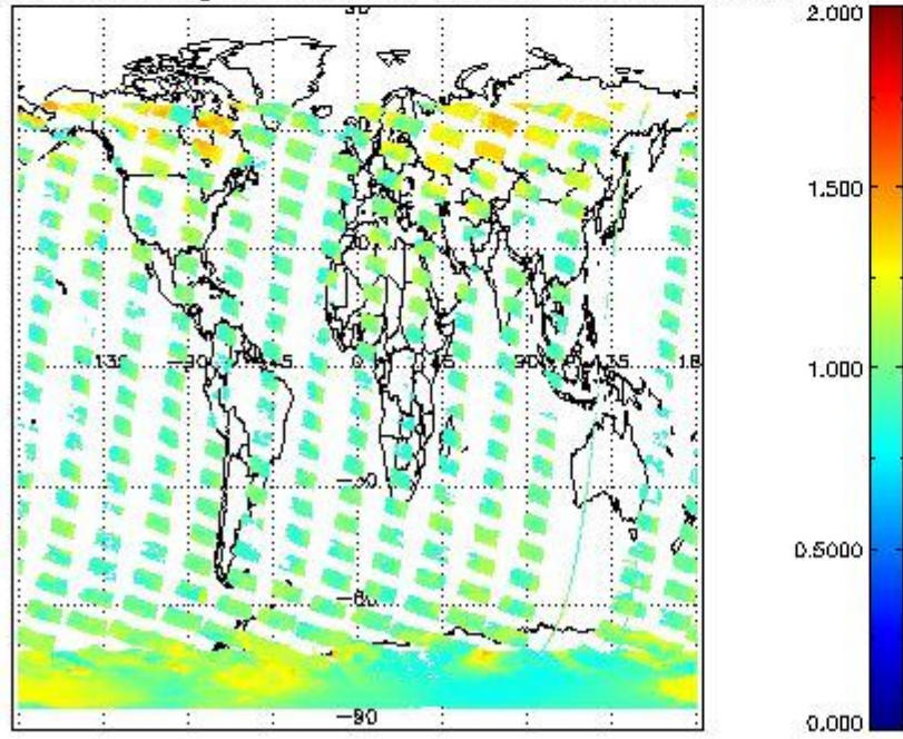
SCIOL2P_NADUV8H20_amf_gr for 19JAN2011 00:00:00 to 20JAN2011 00:00:00
