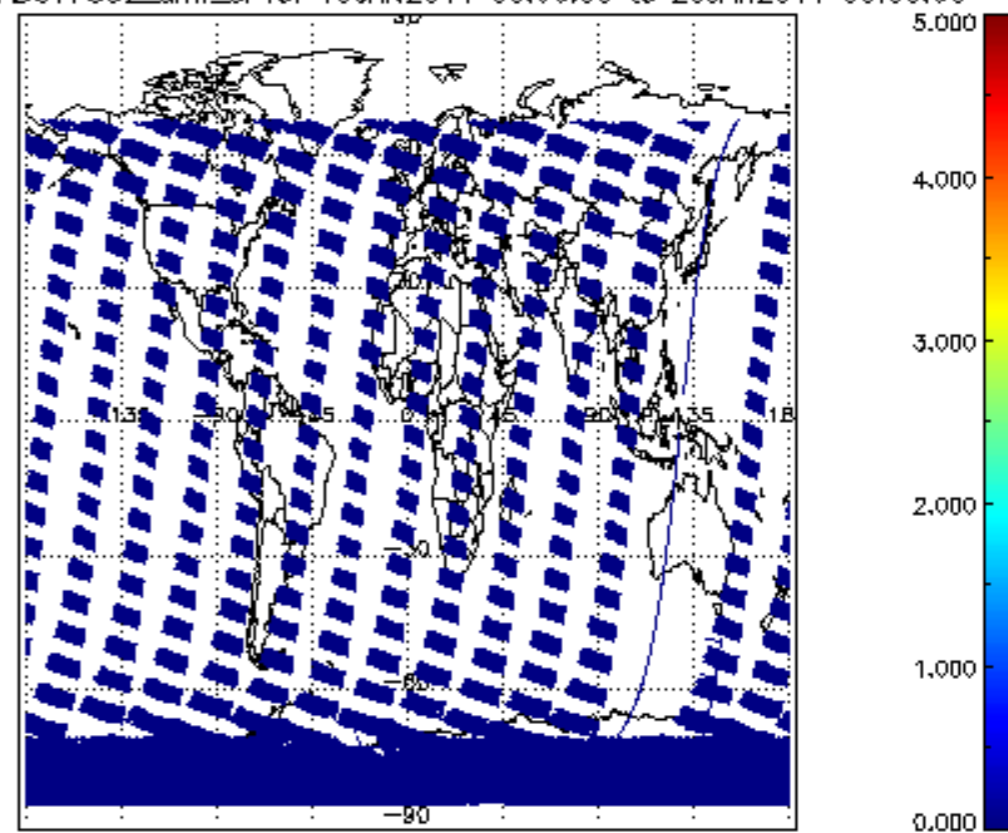
SCIOL2P_NADUV7S02_amf_sl for 19JAN2011 00:00:00 to 20JAN2011 00:00:00
