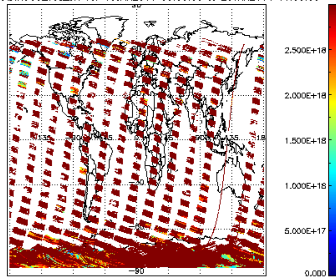
SCIOL2P_NADIR3CO_vcd_err for 19JAN2011 00:00:00 to 20JAN2011 00:00:00
