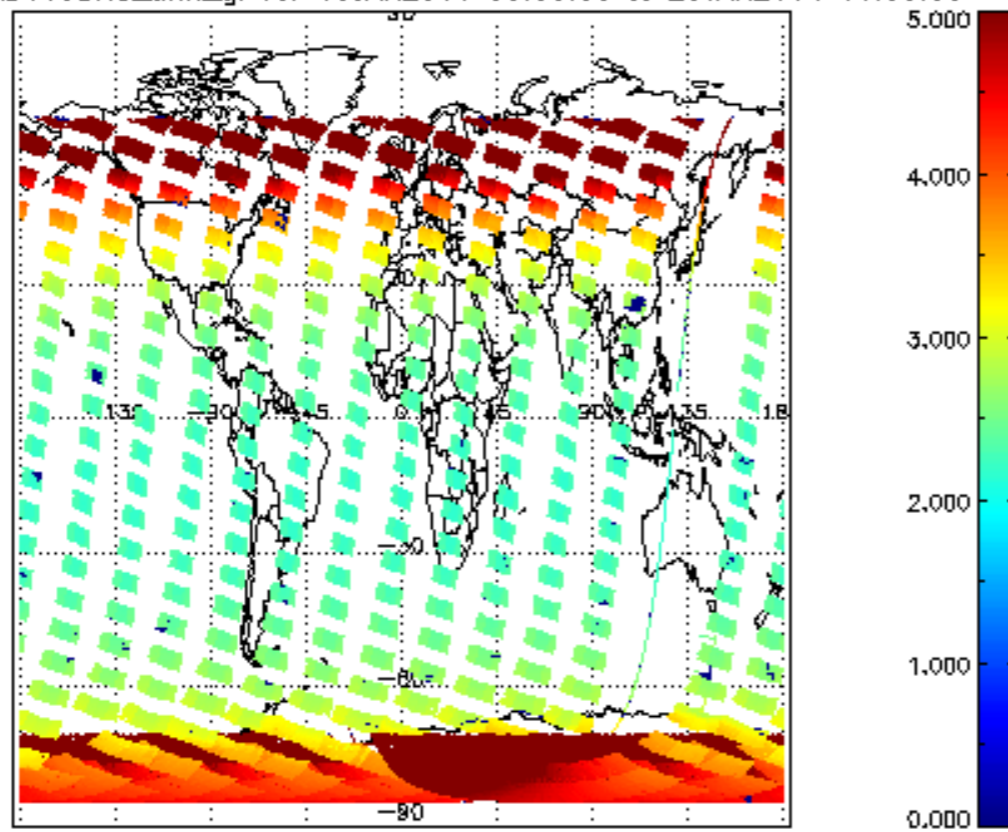
SCIOL2P_NADUV3BRO_amf_gr for 19JAN2011 00:00:00 to 20JAN2011 00:00:00
