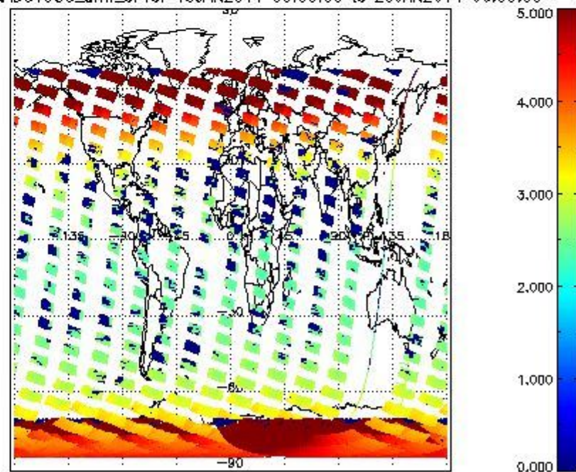
SCIOL2P_NADUV003_amf_cl for 19JAN2011 00:00:00 to 20JAN2011 00:00:00
