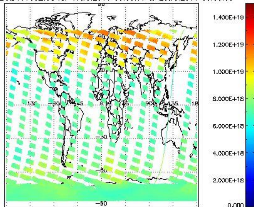
SCIOL2P_NADUV003_vcd for 19JAN2011 00:00:00 to 20JAN2011 00:00:00
