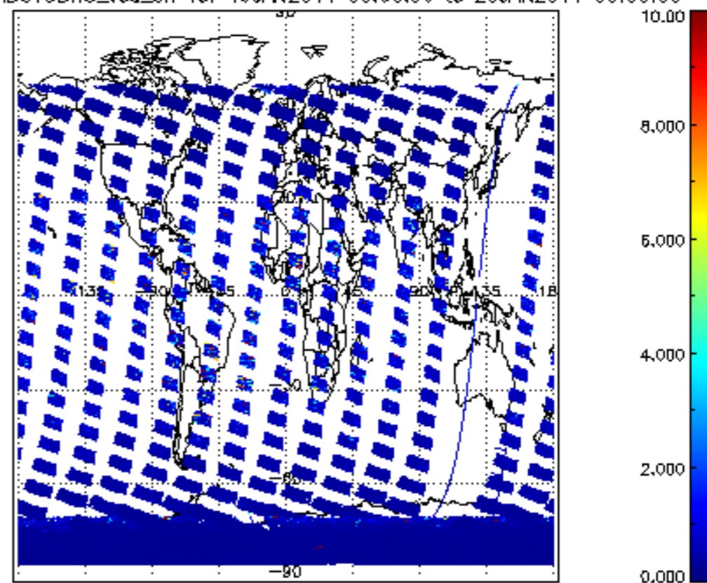
SCIOL2P_NADUV3BRO_vcd_err for 19JAN2011 00:00:00 to 20JAN2011 00:00:00
