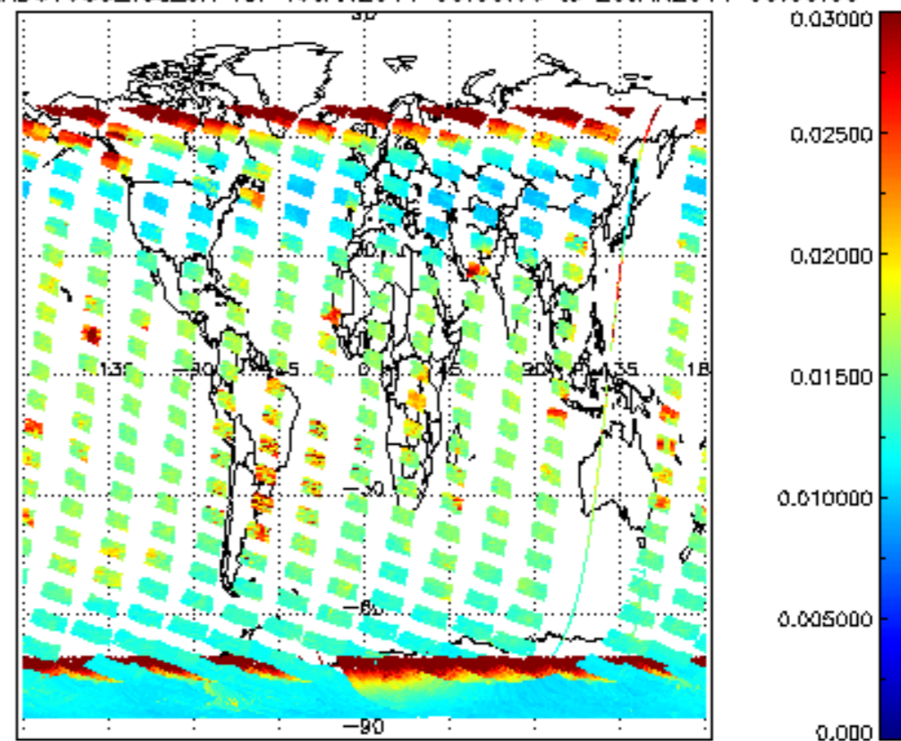
SCIOL2P_NADUV003_vcd_err for 19JAN2011 00:00:00 to 20JAN2011 00:00:00
