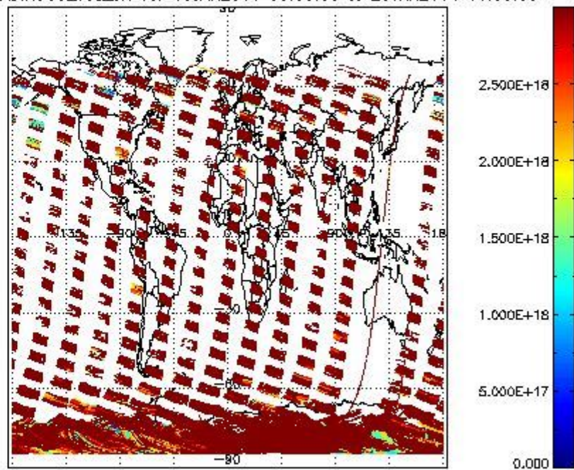
SCIDL2P_NADIR3CO_vcd_err for 19JAN2011 00:00:00 to 20JAN2011 00:00:00
