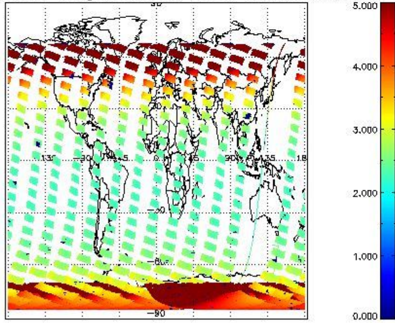
SCIOL2P_NADUV1NO2_amf_gr for 19JAN2011 00:00:00 to 20JAN2011 00:00:00
