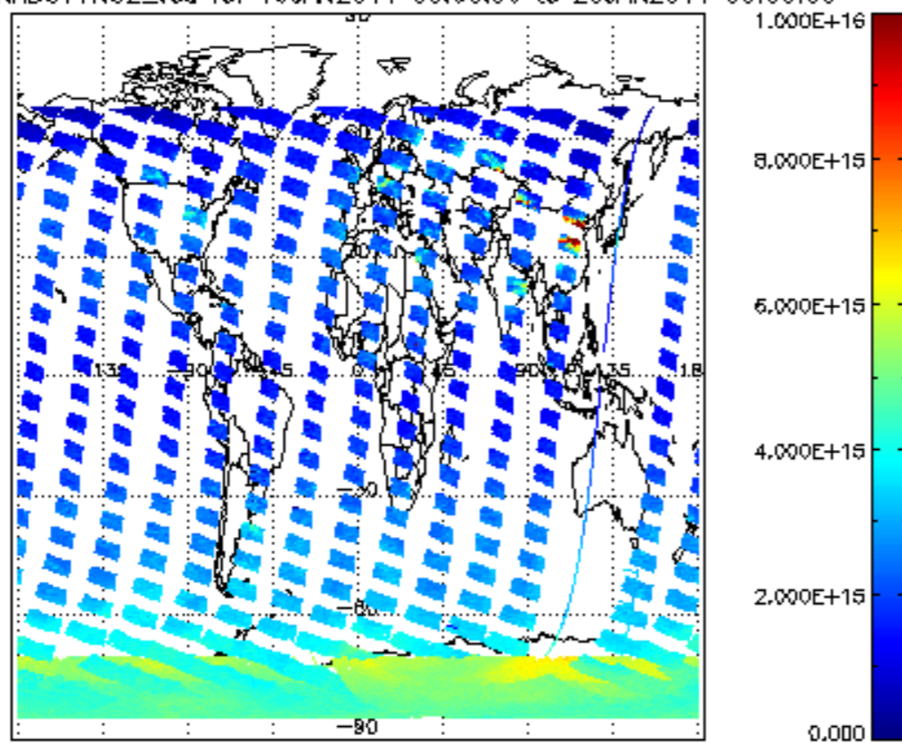
SCIOL2P_NADUV1NO2_vcd for 19JAN2011 00:00:00 to 20JAN2011 00:00:00
