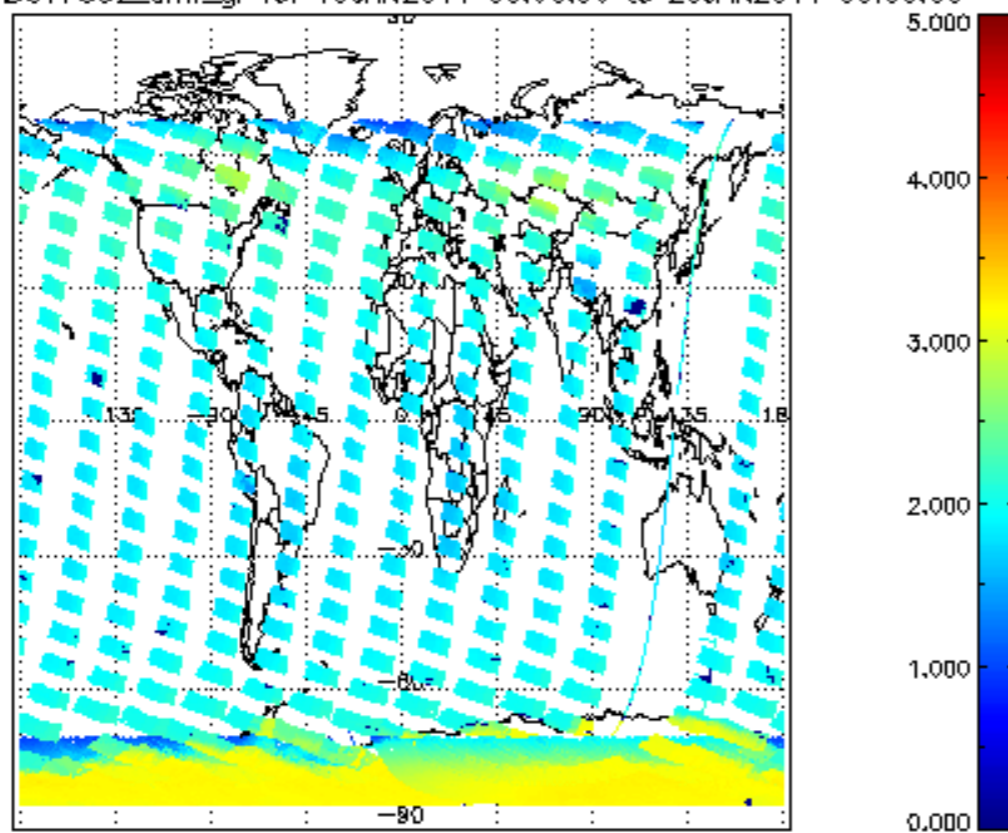
SCIOL2P_NADUV7S02_amf_gr for 19JAN2011 00:00:00 to 20JAN2011 00:00:00
