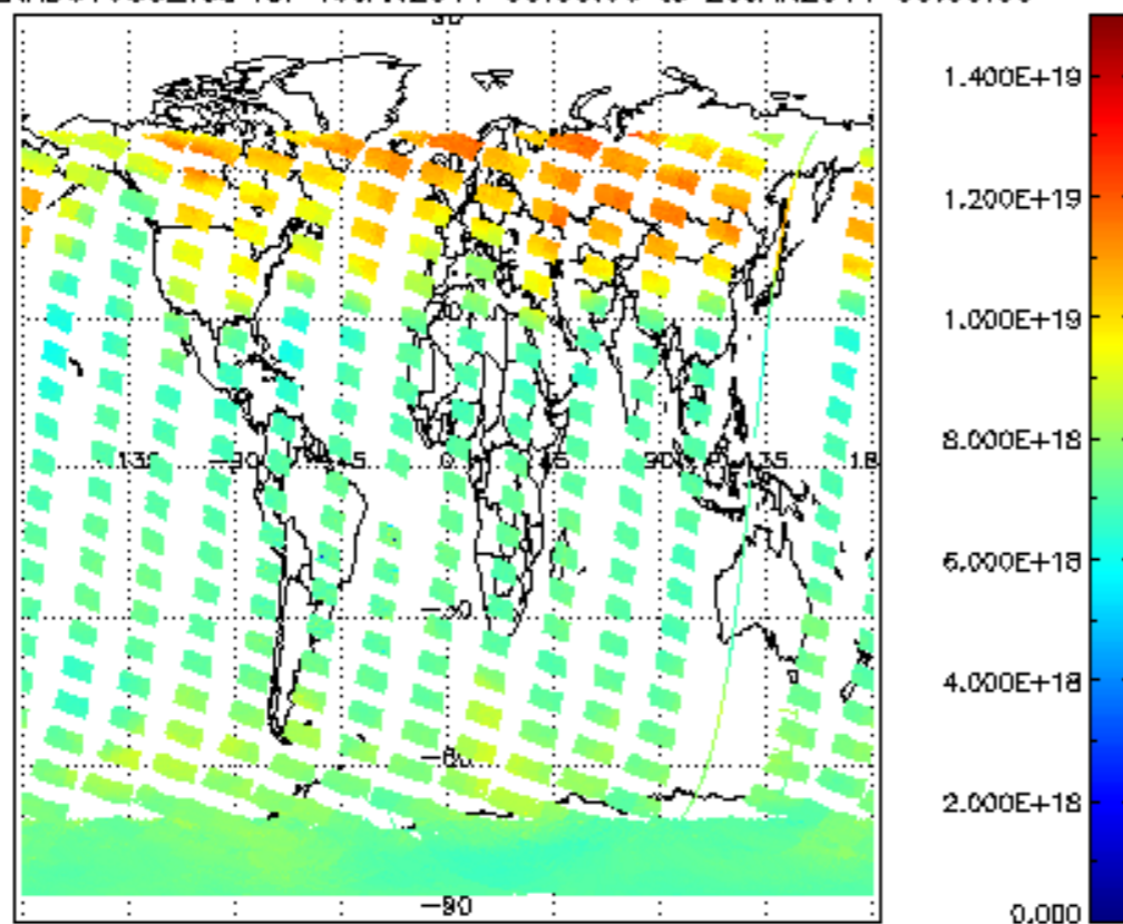
SCIOL2P_NADUV003_vcd for 19JAN2011 00:00:00 to 20JAN2011 00:00:00
