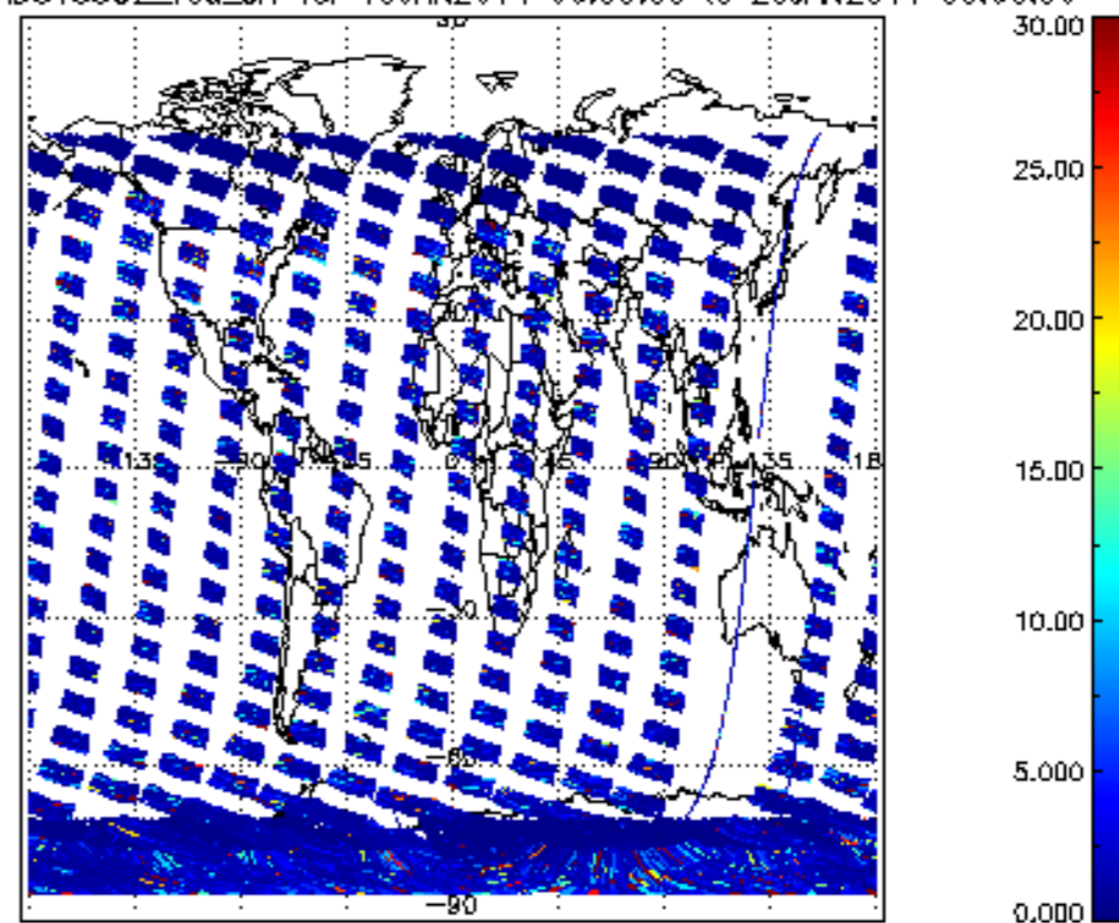
SCIOL2P_NADUV5S02_vcd_err for 19JAN2011 00:00:00 to 20JAN2011 00:00:00
