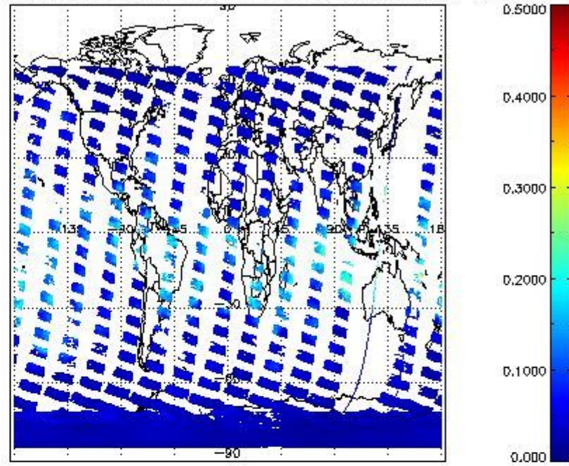
SCIOL2P_NADUV8H20_vcd_err for 19JAN2011 00:00:00 to 20JAN2011 00:00:00
