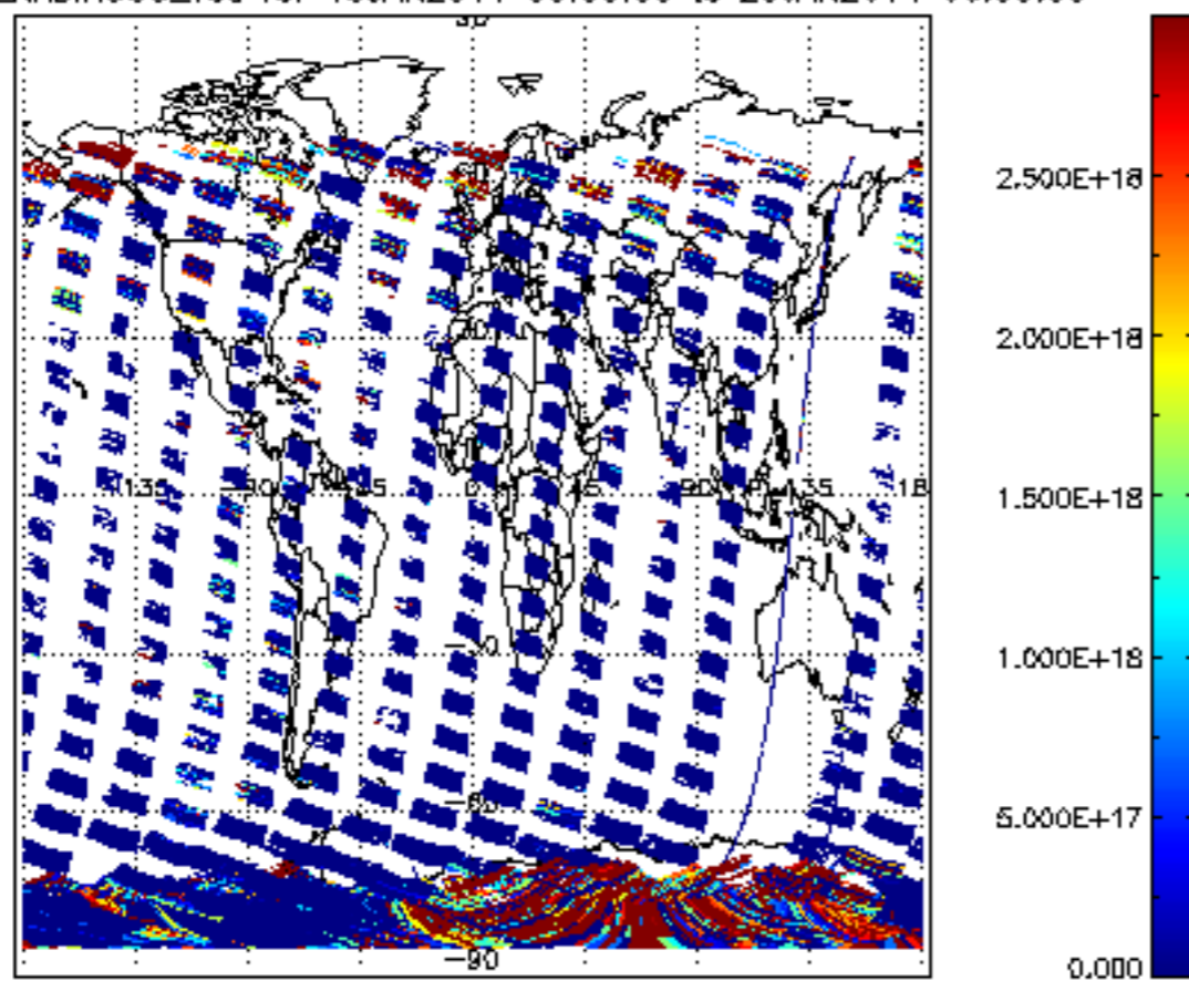
SCIOL2P_NADIR3CO_vcd for 19JAN2011 00:00:00 to 20JAN2011 00:00:00
