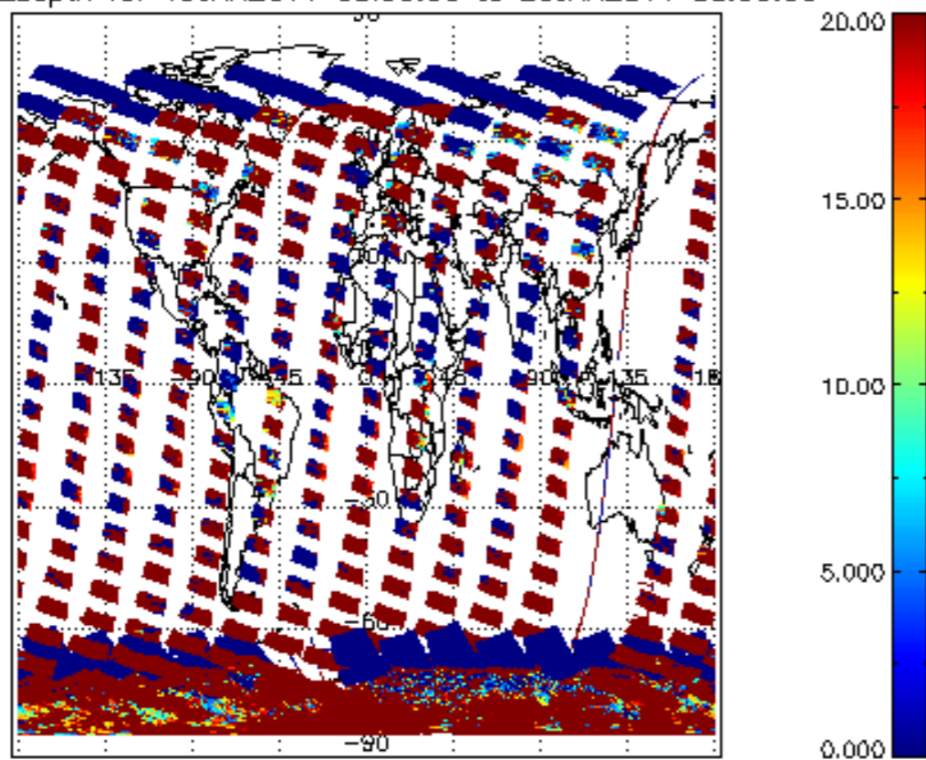
cLopt_depth for 19JAN2011 00:00:00 to 20JAN2011 00:00:00
