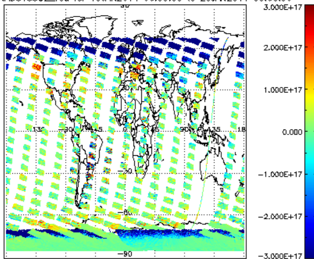
SCIOL2P_NADUV5S02_vcd for 19JAN2011 00:00:00 to 20JAN2011 00:00:00
