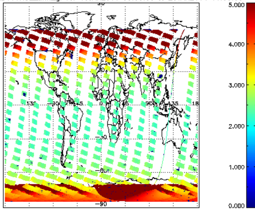
SCIOL2P_NADUV1NO2_amf_gr for 19JAN2011 00:00:00 to 20JAN2011 00:00:00
