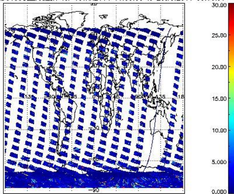
SCIOL2P_NADUV5SO2_vcd_err for 19JAN2011 00:00:00 to 20JAN2011 00:00:00
