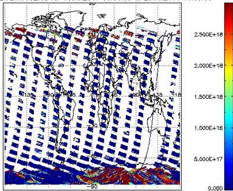
SCIDL2P_NADIR3CO_vcd for 19JAN2011 00:00:00 to 20JAN2011 00:00:00
