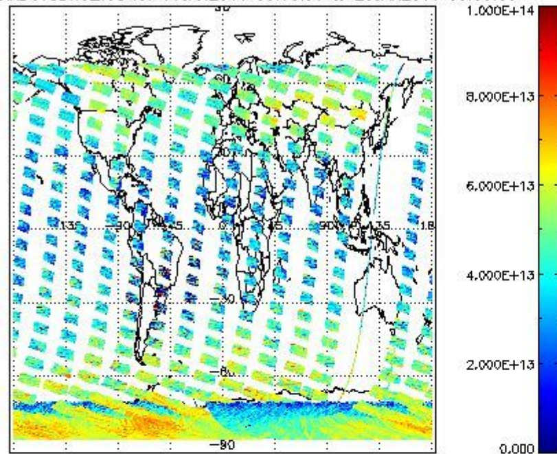
SCIOL2P_NADUV3BRO_vcd for 19JAN2011 00:00:00 to 20JAN2011 00:00:00
