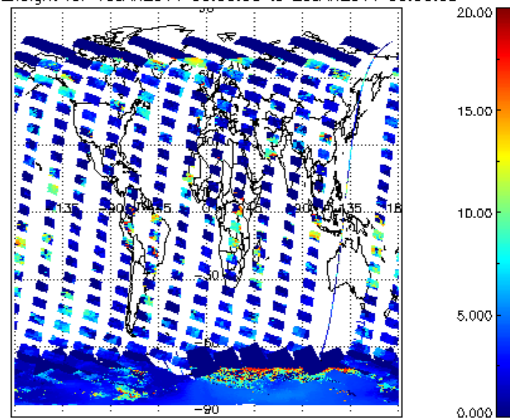
cL_top_height for 19JAN2011 00:00:00 to 20JAN2011 00:00:00
