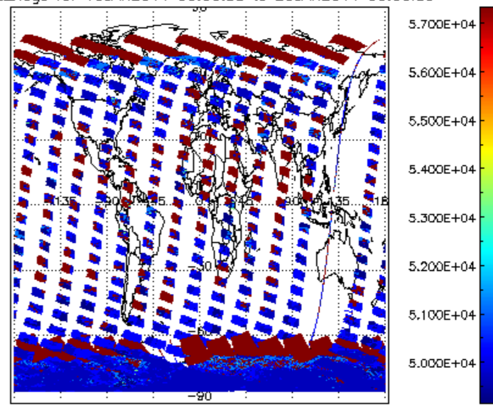
cloud_flags for 19JAN2011 00:00:00 to 20JAN2011 00:00:00
