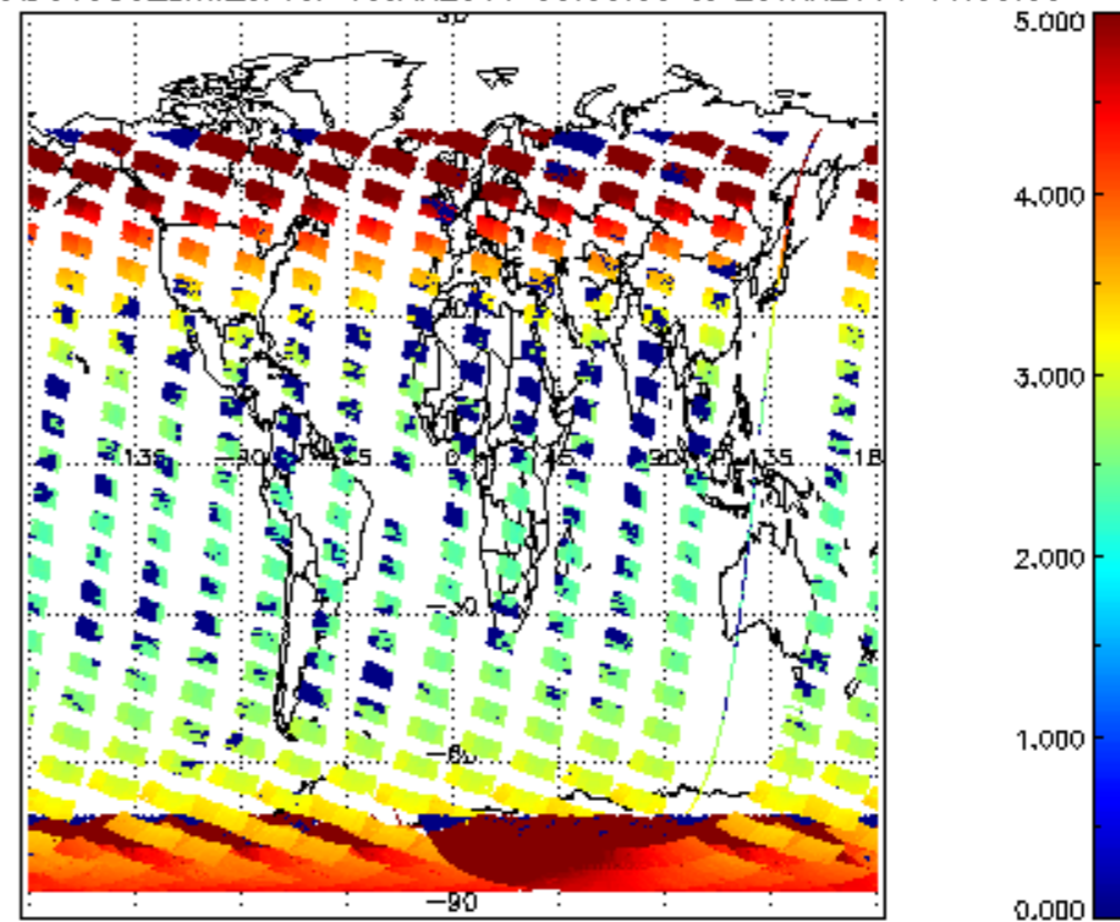
SCIOL2P_NADUV003_amf_cl for 19JAN2011 00:00:00 to 20JAN2011 00:00:00
