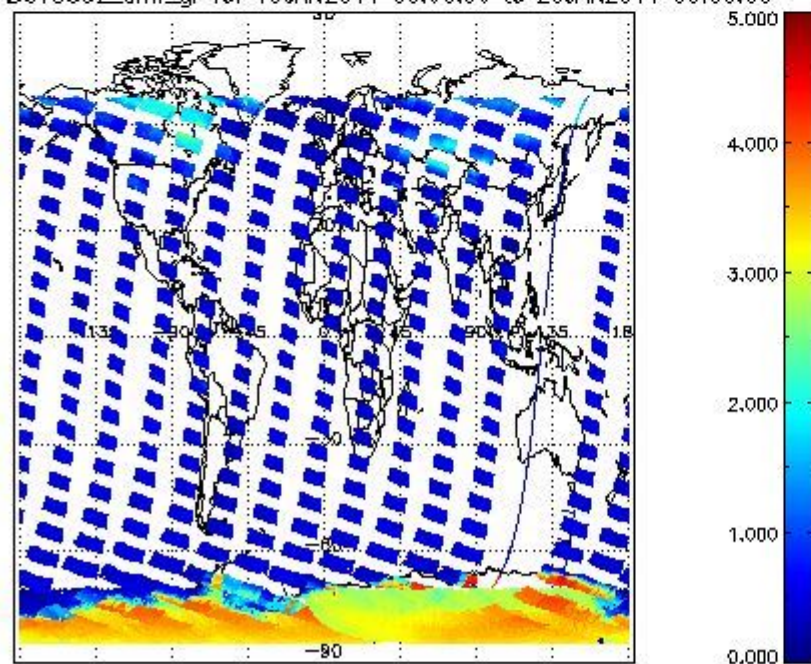
SCIOL2P_NADUV5SO2_amf_gr for 19JAN2011 00:00:00 to 20JAN2011 00:00:00
