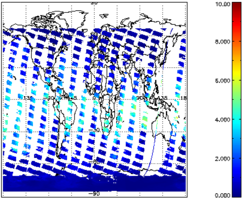
SCIOL2P_NADUV8H20_vcd for 19JAN2011 00:00:00 to 20JAN2011 00:00:00
