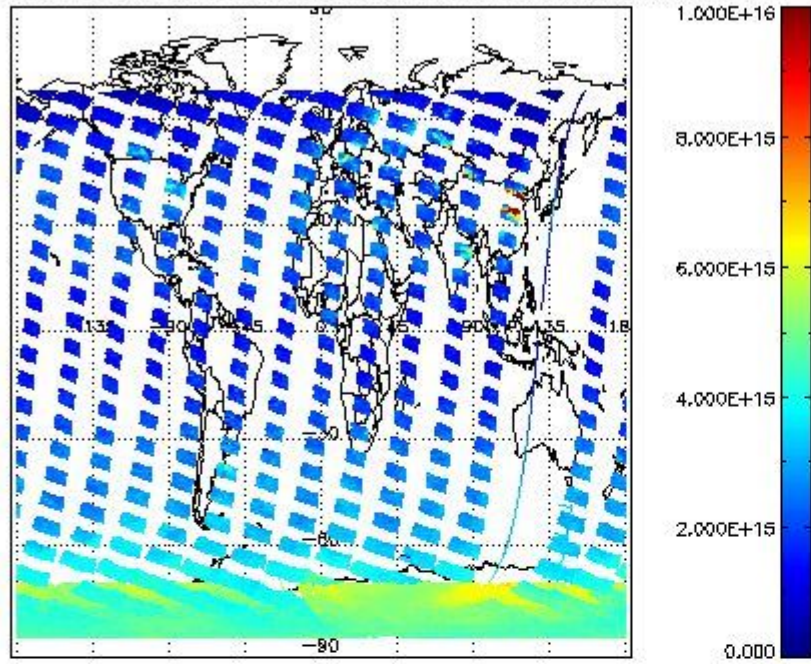
SCIOL2P_NADUV1NO2_vcd for 19JAN2011 00:00:00 to 20JAN2011 00:00:00
