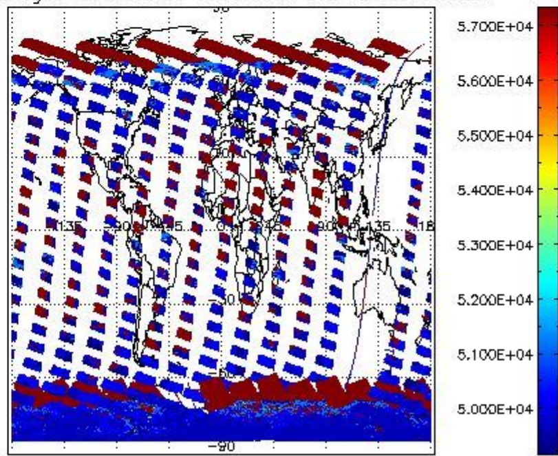
cloud_flags for 19JAN2011 00:00:00 to 20JAN2011 00:00:00
