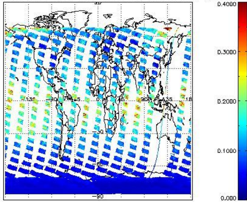
SCIOL2P_NADUV1NO2_vcd_err for 19JAN2011 00:00:00 to 20JAN2011 00:00:00
