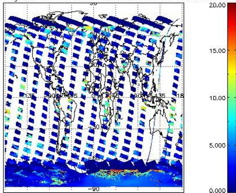
cL_top_height for 19JAN2011 00:00:00 to 20JAN2011 00:00:00
