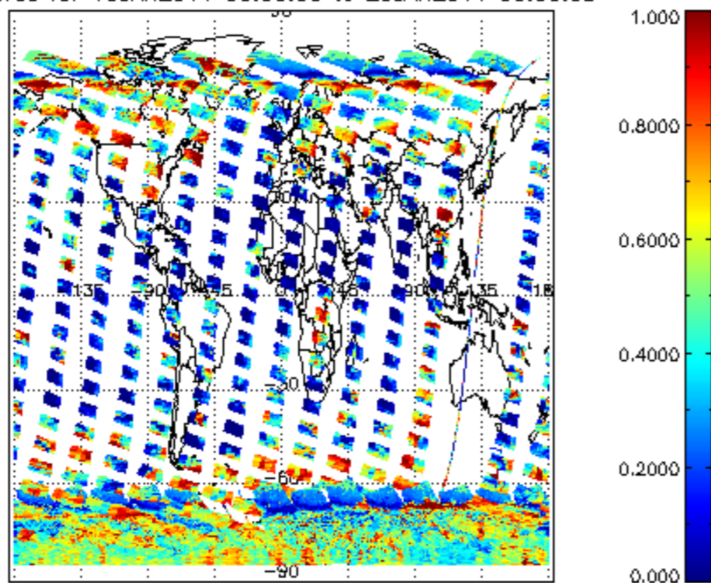
cL_frac for 19JAN2011 00:00:00 to 20JAN2011 00:00:00
