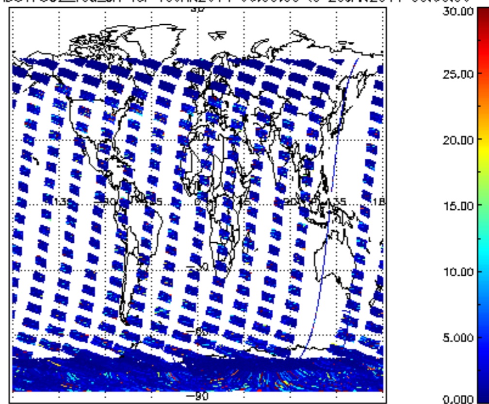
SCIOL2P_NADUV7S02_vcd_err for 19JAN2011 00:00:00 to 20JAN2011 00:00:00
