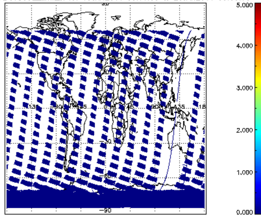
SCIOL2P_NADUV5S02_amf_cl for 19JAN2011 00:00:00 to 20JAN2011 00:00:00
