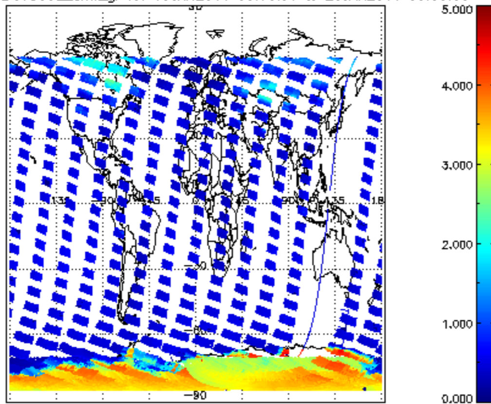
SCIOL2P_NADUV5S02_amf_gr for 19JAN2011 00:00:00 to 20JAN2011 00:00:00
