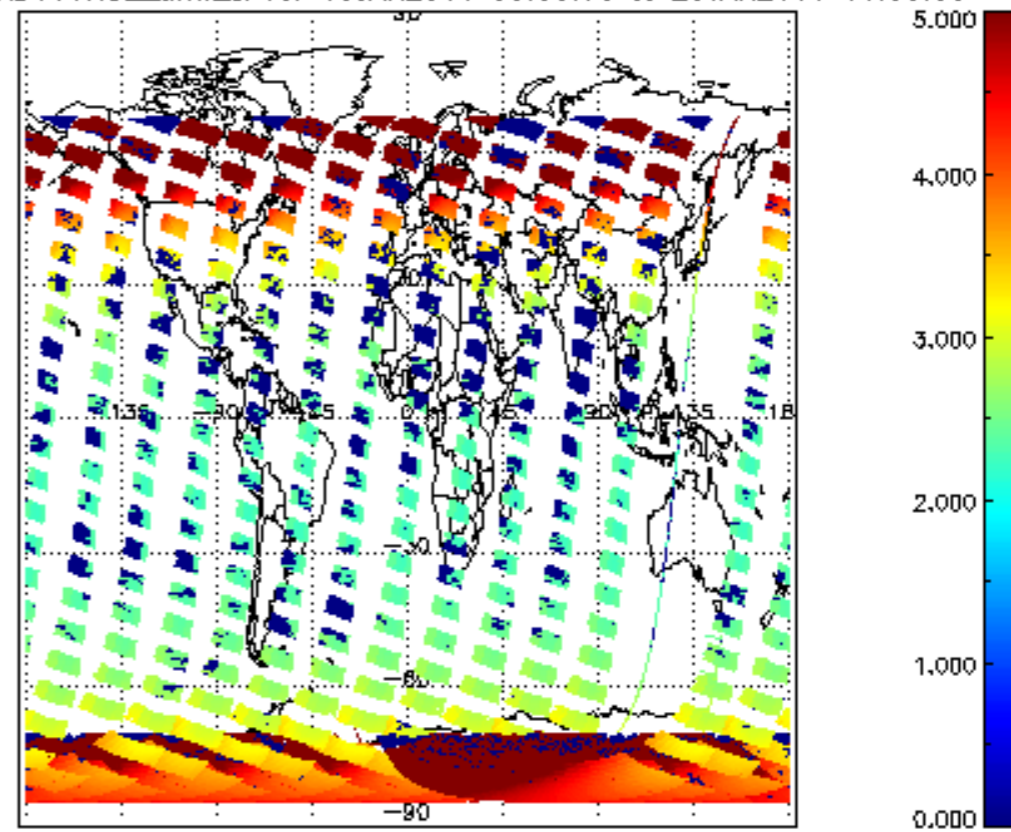
SCIOL2P_NADUV1NO2_amf_cl for 19JAN2011 00:00:00 to 20JAN2011 00:00:00
