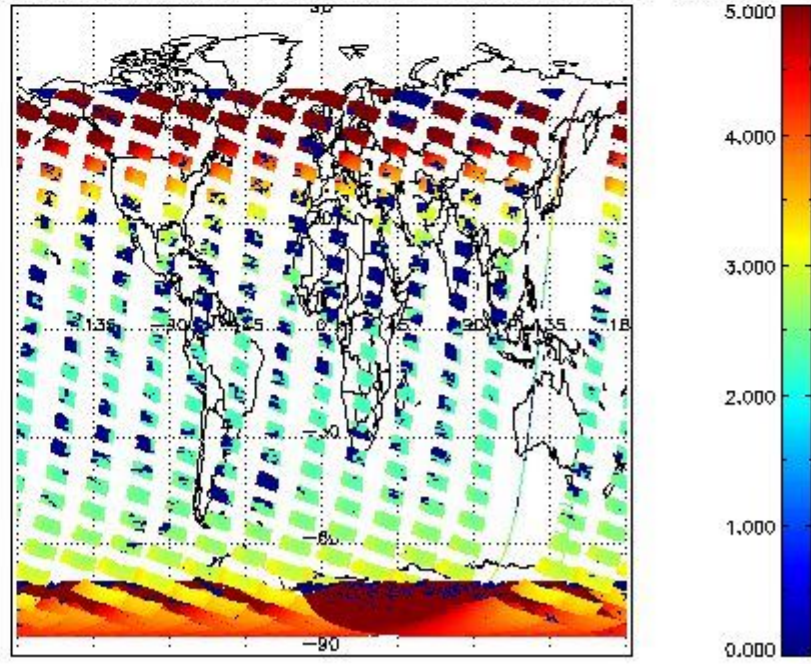
SCIOL2P_NADUV1NO2_amf_cl for 19JAN2011 00:00:00 to 20JAN2011 00:00:00
