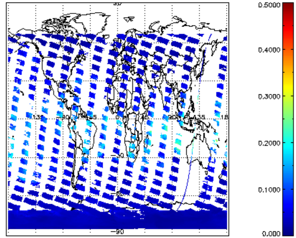
SCIOL2P_NADUV8H20_vcd_err for 19JAN2011 00:00:00 to 20JAN2011 00:00:00
