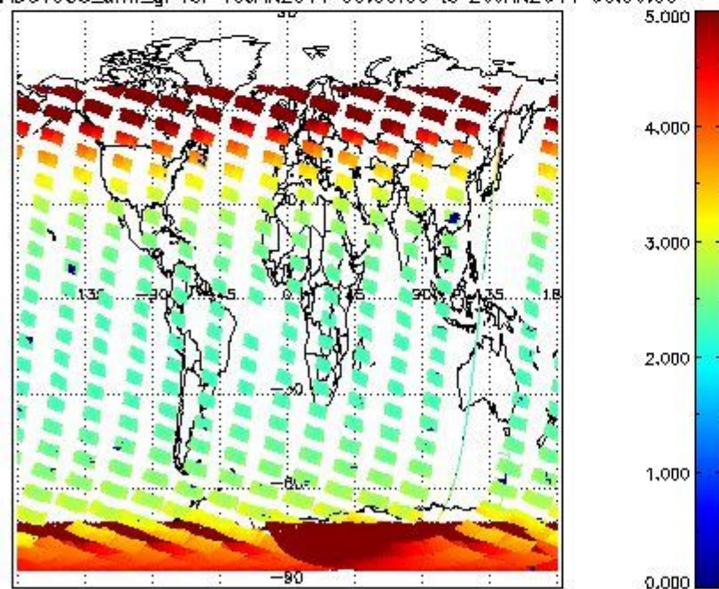
SCIOL2P_NADUV003_amf_gr for 19JAN2011 00:00:00 to 20JAN2011 00:00:00
