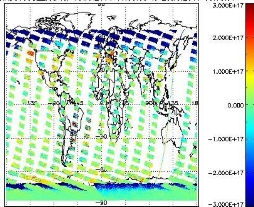
SCIOL2P_NADUV5SO2_vcd for 19JAN2011 00:00:00 to 20JAN2011 00:00:00
