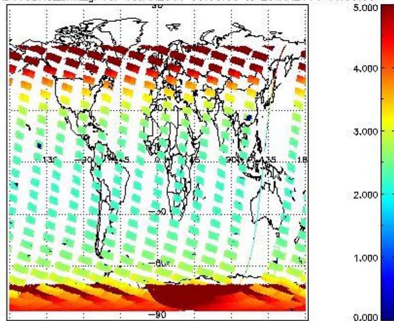
SCIOL2P_NADUV3BRO_amf_gr for 19JAN2011 00:00:00 to 20JAN2011 00:00:00
