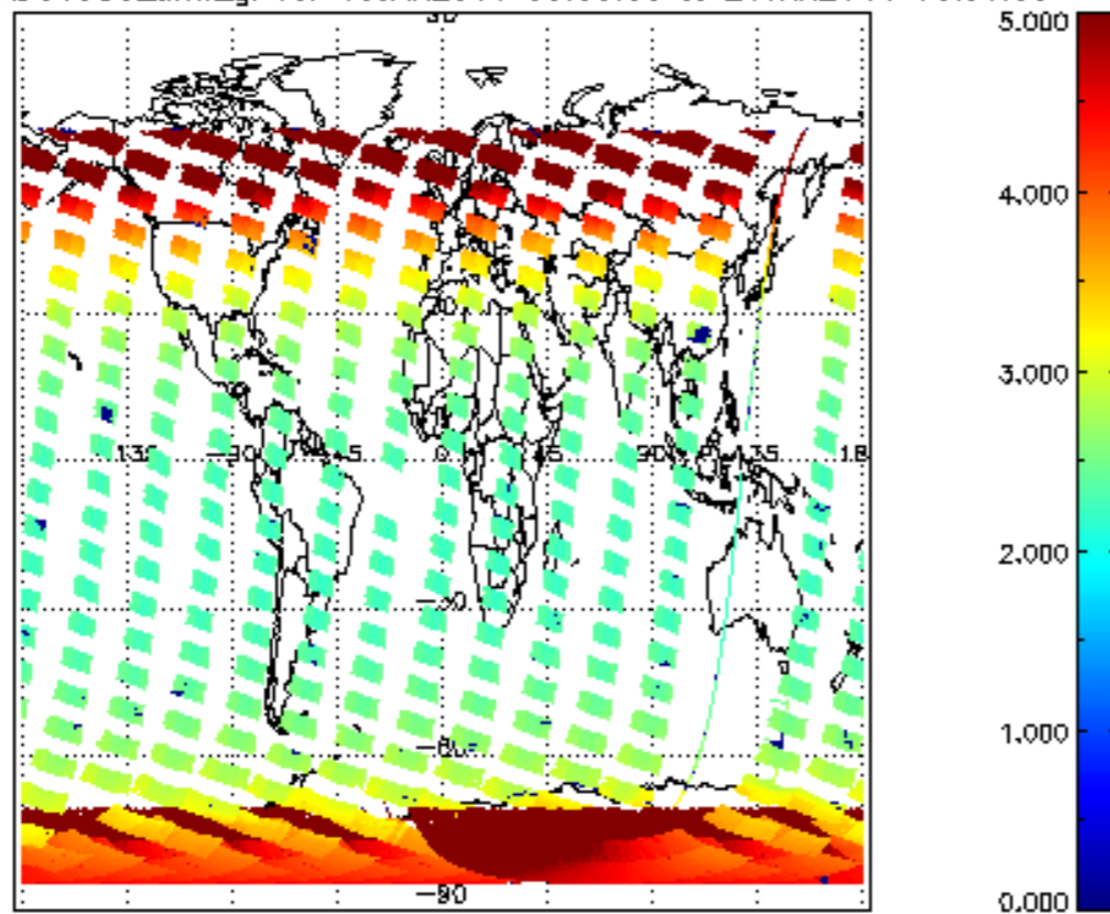
SCIOL2P_NADUV003_amf_gr for 19JAN2011 00:00:00 to 20JAN2011 00:00:00
