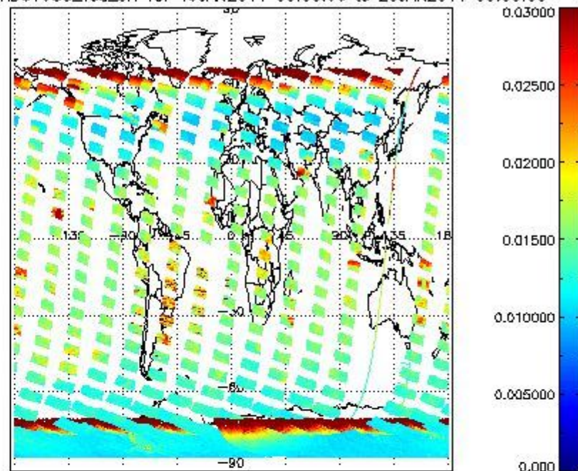
SCIOL2P_NADUV003_vcd_err for 19JAN2011 00:00:00 to 20JAN2011 00:00:00
