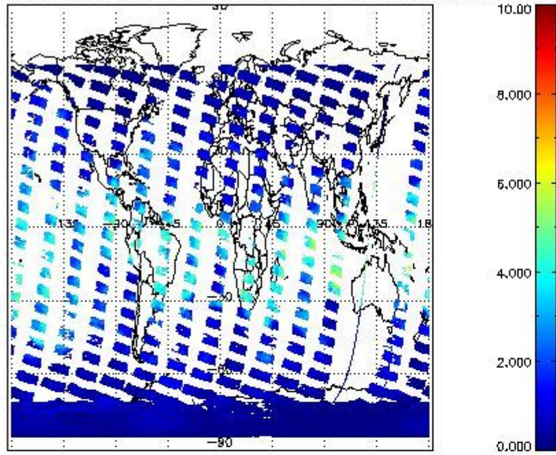
SCIOL2P_NADUV8H20_vcd for 19JAN2011 00:00:00 to 20JAN2011 00:00:00
