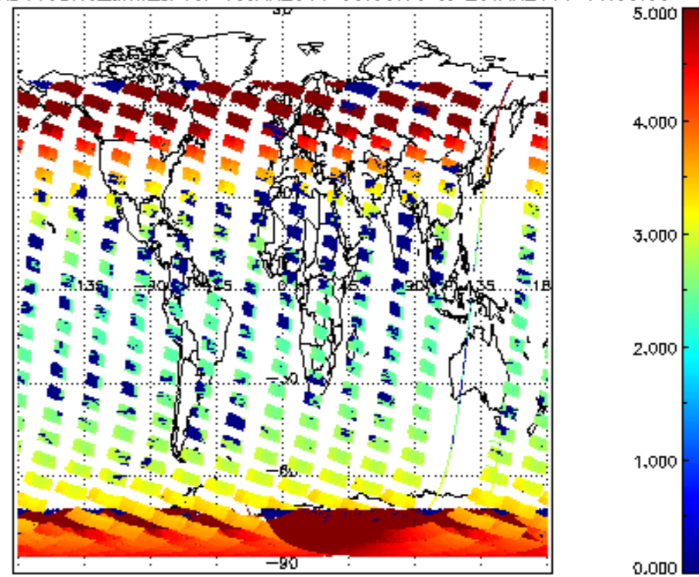
SCIOL2P_NADUV3BRO_amf_cl for 19JAN2011 00:00:00 to 20JAN2011 00:00:00
