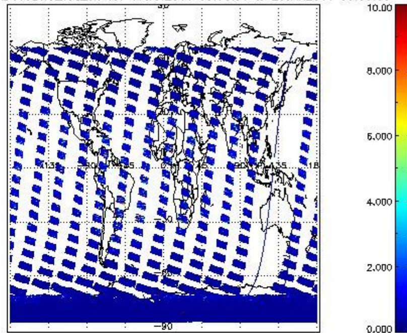
SCIOL2P_NADUV3BRO_vcd_err for 19JAN2011 00:00:00 to 20JAN2011 00:00:00
