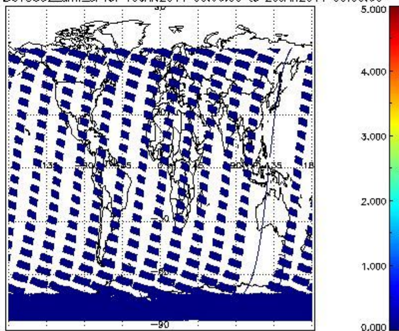
SCIOL2P_NADUV5SO2_amf_cl for 19JAN2011 00:00:00 to 20JAN2011 00:00:00
