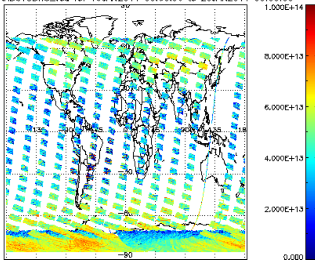
SCIOL2P_NADUV3BRO_vcd for 19JAN2011 00:00:00 to 20JAN2011 00:00:00
