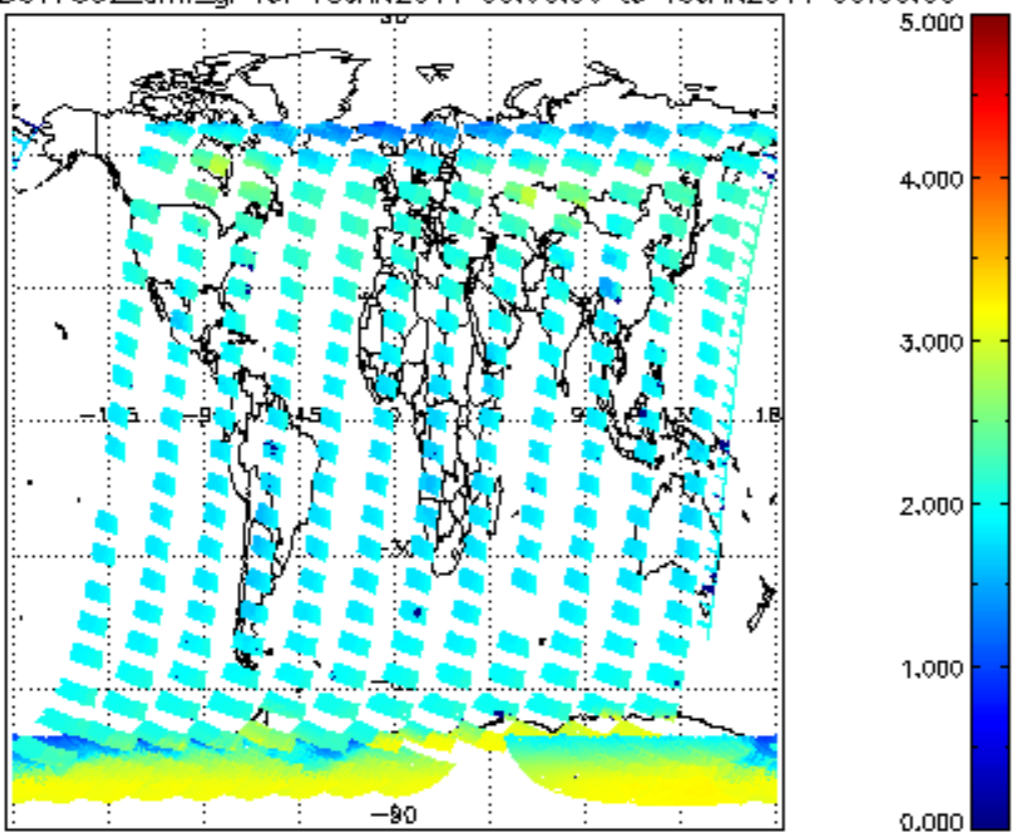
SCIOL2P_NADUV7S02_amf_gr for 18JAN2011 00:00:00 to 19JAN2011 00:00:00
