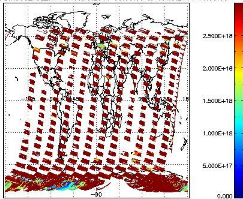
SCIDL2P_NADIR3CO_vcd_err for 18JAN2011 00:00:00 to 19JAN2011 00:00:00
