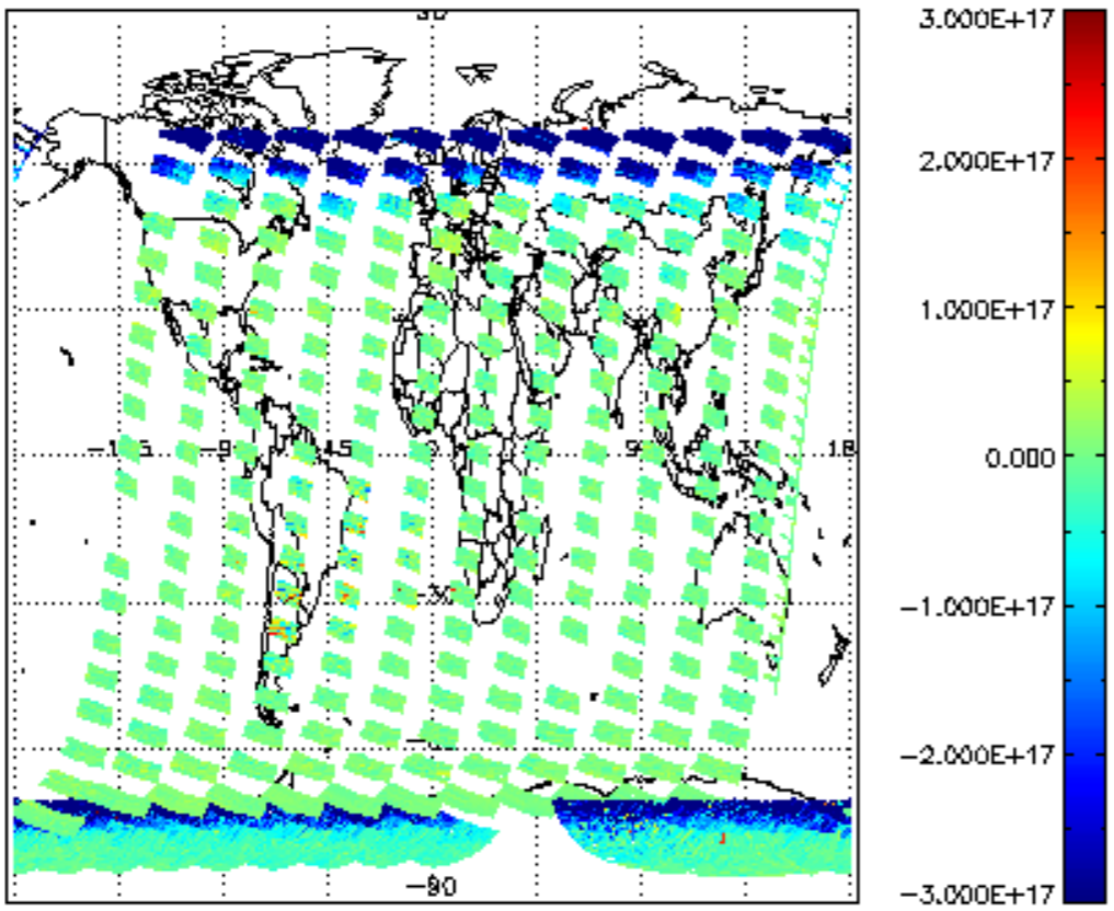
SCIOL2P_NADUV7S02_vcd for 18JAN2011 00:00:00 to 19JAN2011 00:00:00
