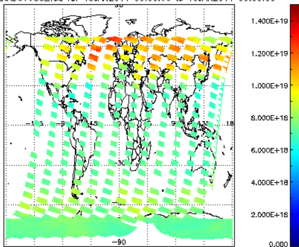
SCIOL2P_NADUV003_vcd for 18JAN2011 00:00:00 to 19JAN2011 00:00:00
