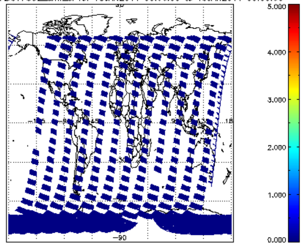
SCIOL2P_NADUV7S02_amf_cl for 18JAN2011 00:00:00 to 19JAN2011 00:00:00
