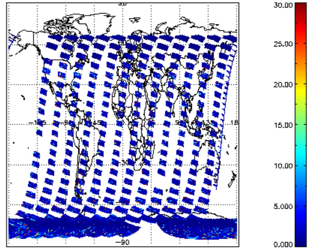
SCIOL2P_NADUV7S02_vcd_err for 18JAN2011 00:00:00 to 19JAN2011 00:00:00
