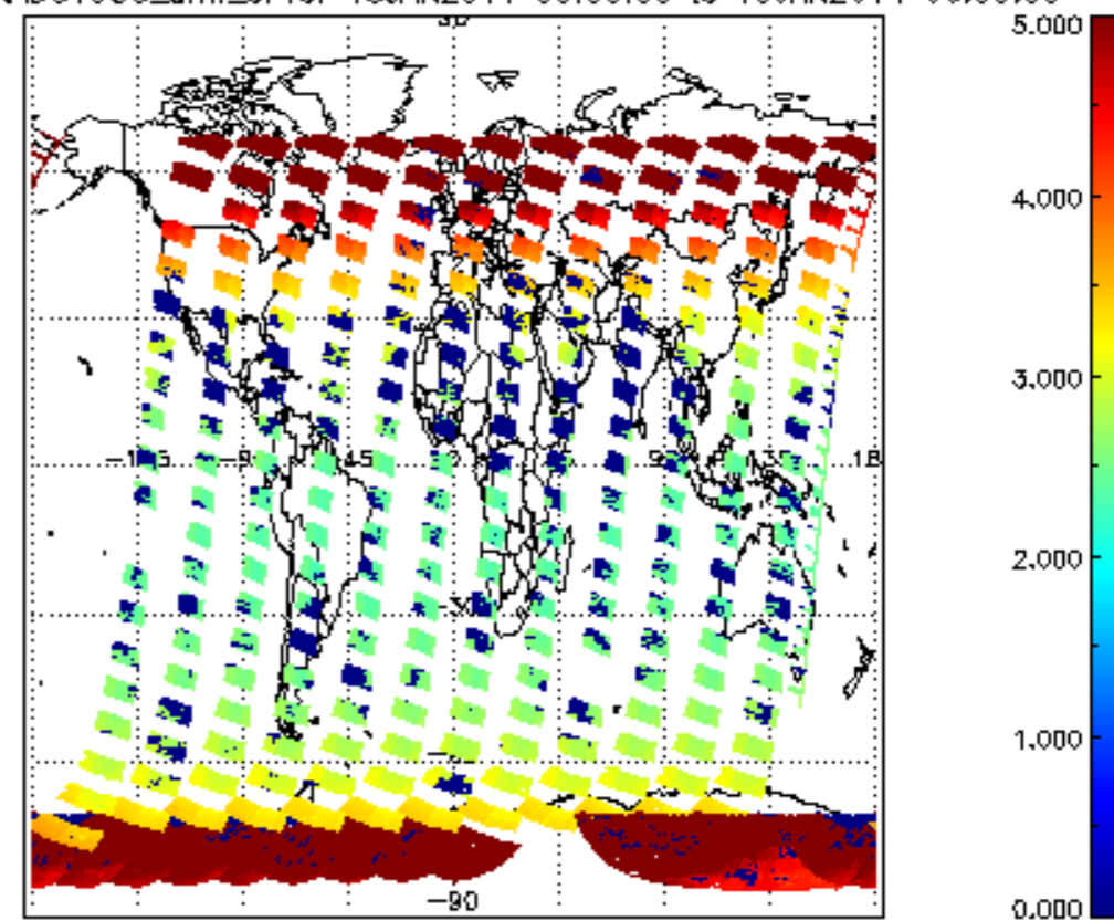
SCIOL2P_NADUV003_amf_cl for 18JAN2011 00:00:00 to 19JAN2011 00:00:00
