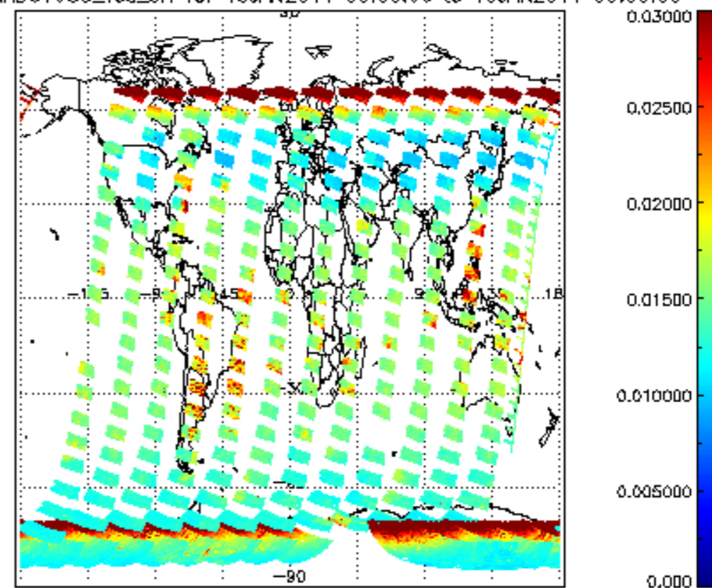
SCIOL2P_NADUV003_vcd_err for 18JAN2011 00:00:00 to 19JAN2011 00:00:00
