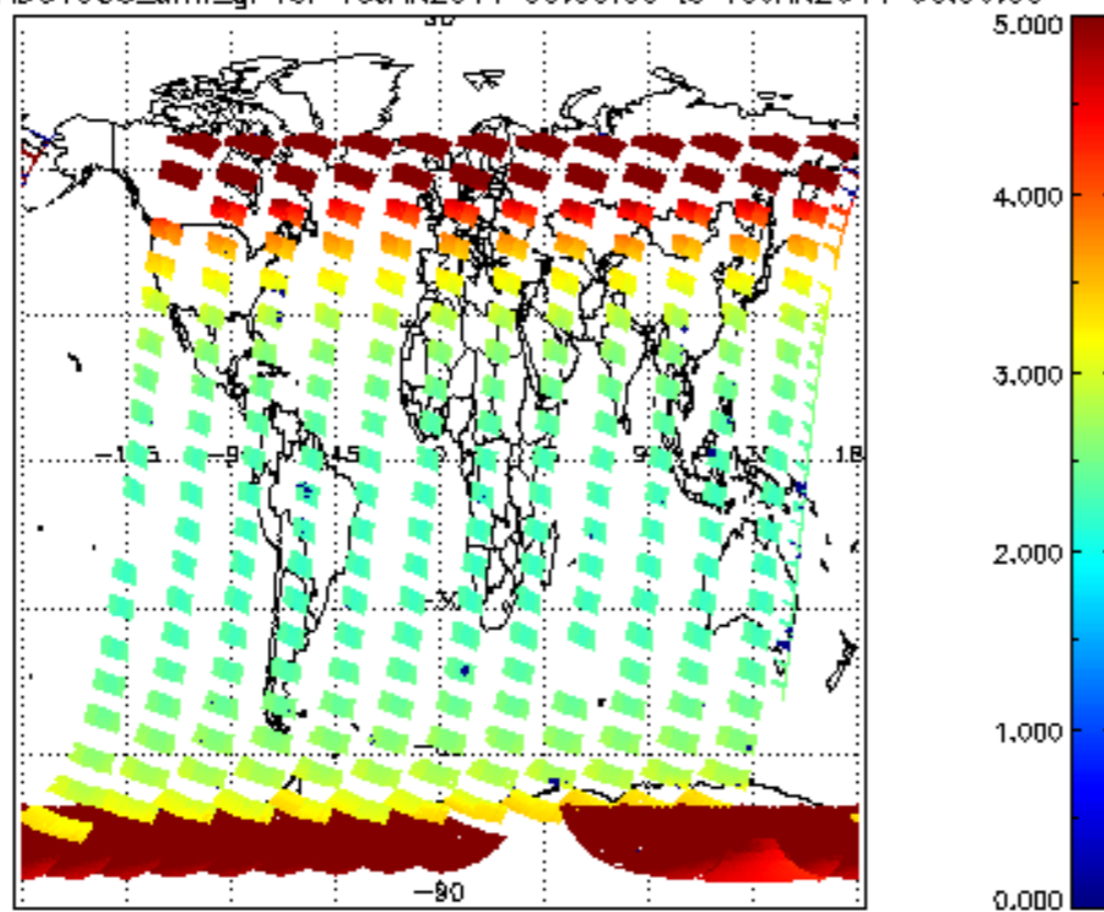
SCIOL2P_NADUV003_amf_gr for 18JAN2011 00:00:00 to 19JAN2011 00:00:00
