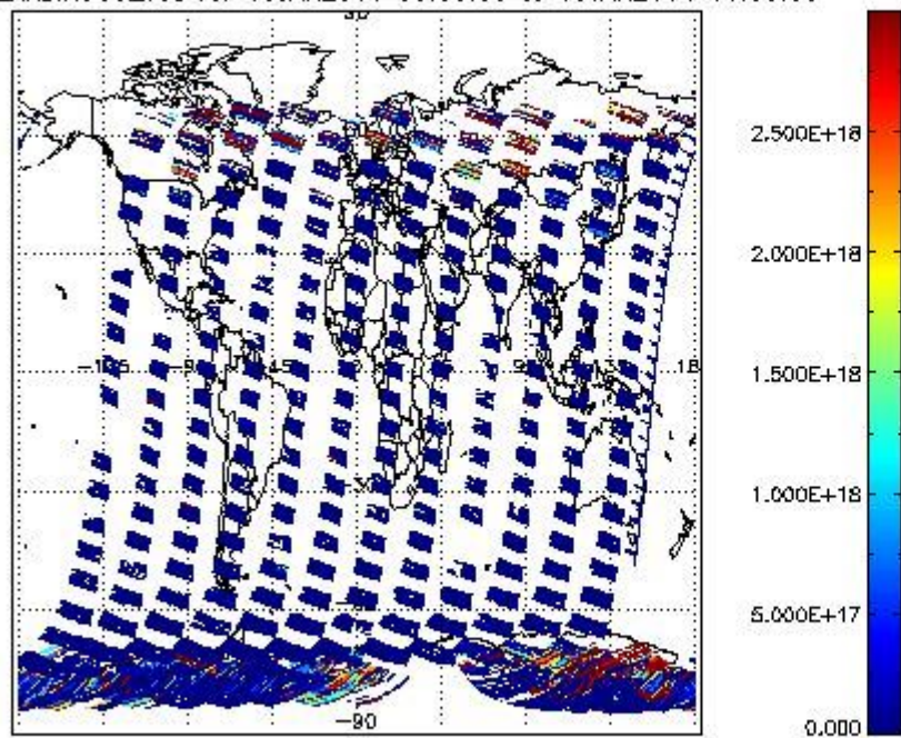
SCIDL2P_NADIR3CO_vcd for 18JAN2011 00:00:00 to 19JAN2011 00:00:00
