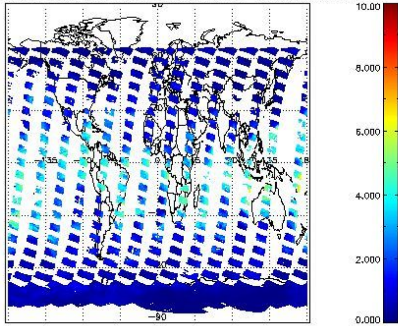
SCIOL2P_NADUV8H20_vcd for 17JAN2011 00:00:00 to 18JAN2011 00:00:00
