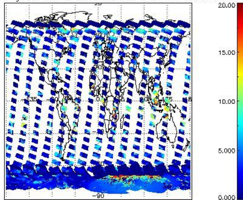
cL_top_height for 17JAN2011 00:00:00 to 18JAN2011 00:00:00
