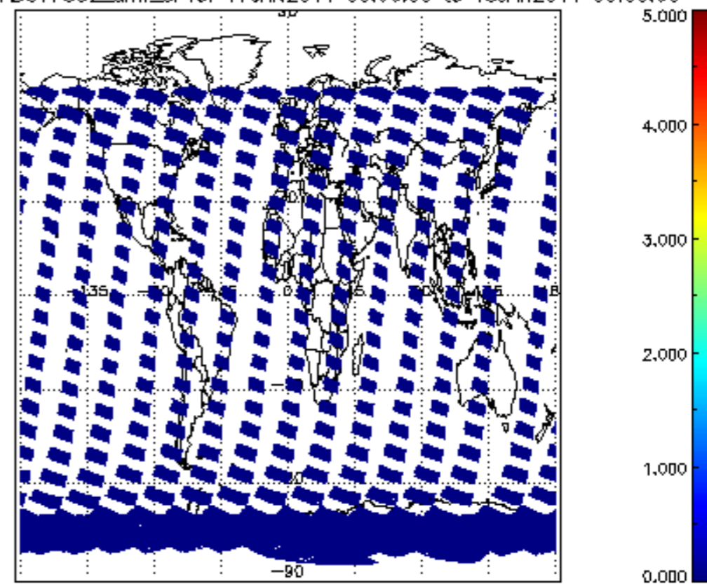
SCIOL2P_NADUV7S02_amf_sl for 17JAN2011 00:00:00 to 18JAN2011 00:00:00
