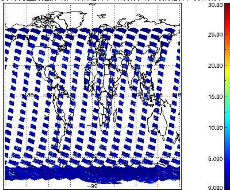
SCIOL2P_NADUV5SO2_vcd_err for 17JAN2011 00:00:00 to 18JAN2011 00:00:00
