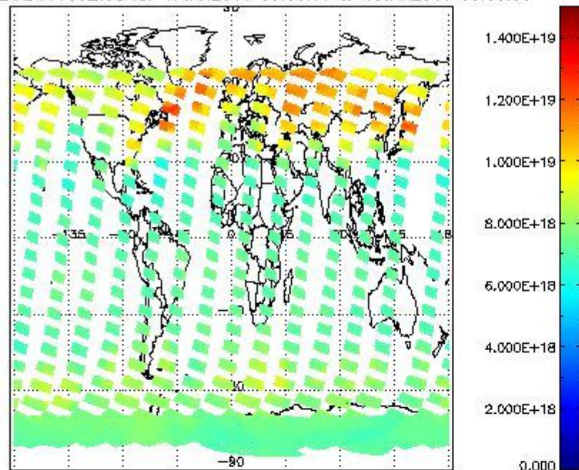
SCIOL2P_NADUV003_vcd for 17JAN2011 00:00:00 to 18JAN2011 00:00:00
