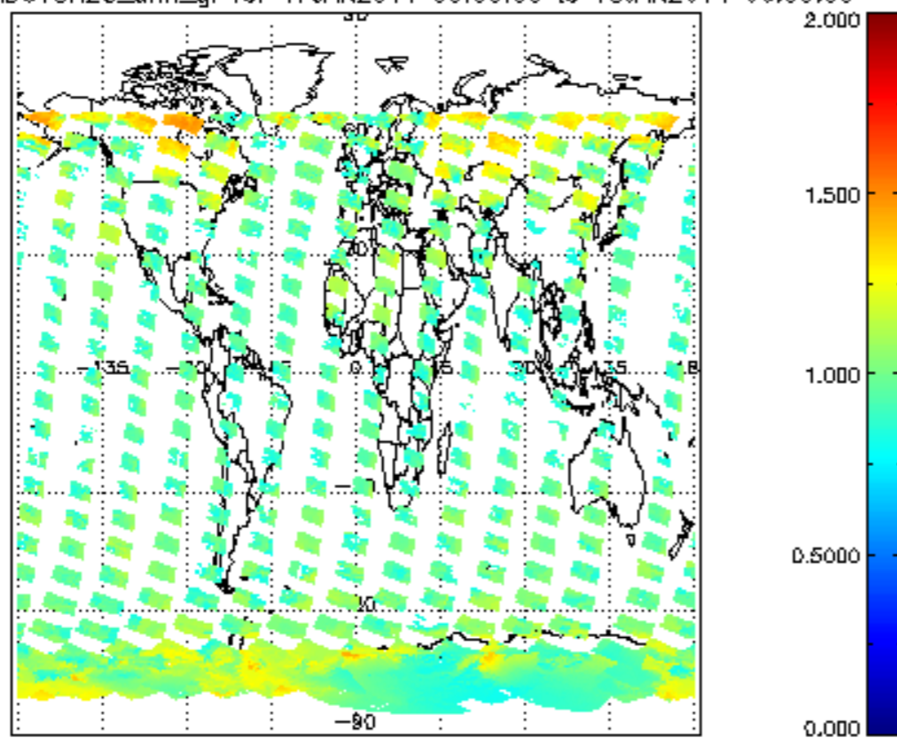
SCIOL2P_NADUV8H20_amf_gr for 17JAN2011 00:00:00 to 18JAN2011 00:00:00
