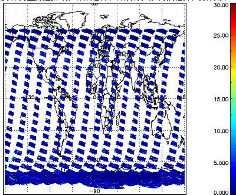
SCIOL2P_NADUV7S02_vcd_err for 17JAN2011 00:00:00 to 18JAN2011 00:00:00
