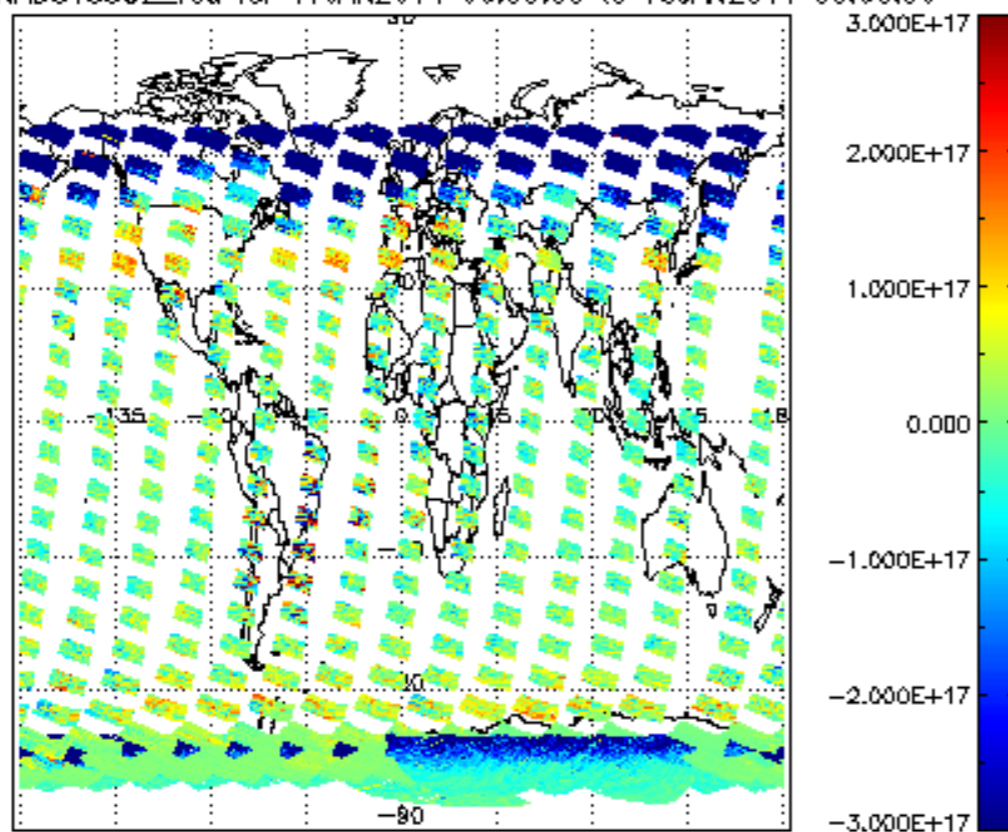
SCIOL2P_NADUV5S02_vcd for 17JAN2011 00:00:00 to 18JAN2011 00:00:00
