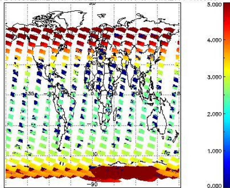
SCIOL2P_NADUV003_amf_cl for 17JAN2011 00:00:00 to 18JAN2011 00:00:00
