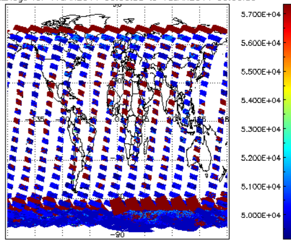
cloud_flags for 17JAN2011 00:00:00 to 18JAN2011 00:00:00
