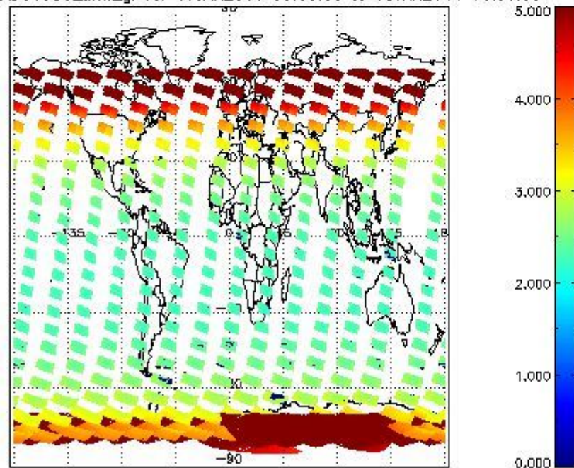
SCIOL2P_NADUV003_amf_gr for 17JAN2011 00:00:00 to 18JAN2011 00:00:00
