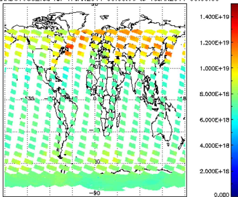
SCIOL2P_NADUV003_vcd for 17JAN2011 00:00:00 to 18JAN2011 00:00:00
