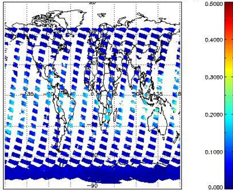
SCIOL2P_NADUV8H20_vcd_err for 17JAN2011 00:00:00 to 18JAN2011 00:00:00
