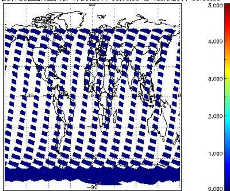
SCIOL2P_NADUV7S02_amf_cl for 17JAN2011 00:00:00 to 18JAN2011 00:00:00
