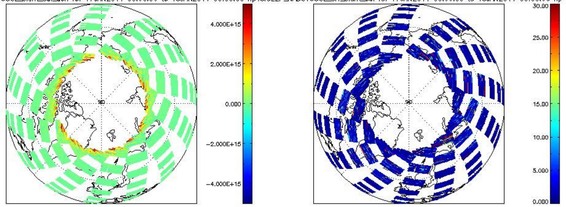
SCIOI2P_NADUV6OCL_slant_col_den for 17JAN2011 00:00:00 to 18JAN2011 00:00:00 np; SCIOI2P_NADUV6OCL_err_slant_col for 17JAN2011 00:00:00 to 18JAN2011 00:00:00 np
