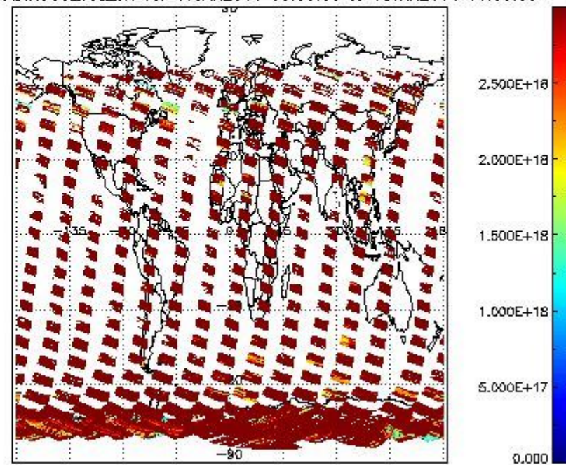
SCIDL2P_NADIR3CO_vcd_err for 17JAN2011 00:00:00 to 18JAN2011 00:00:00
