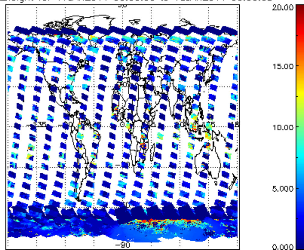
cL_top_height for 17JAN2011 00:00:00 to 18JAN2011 00:00:00
