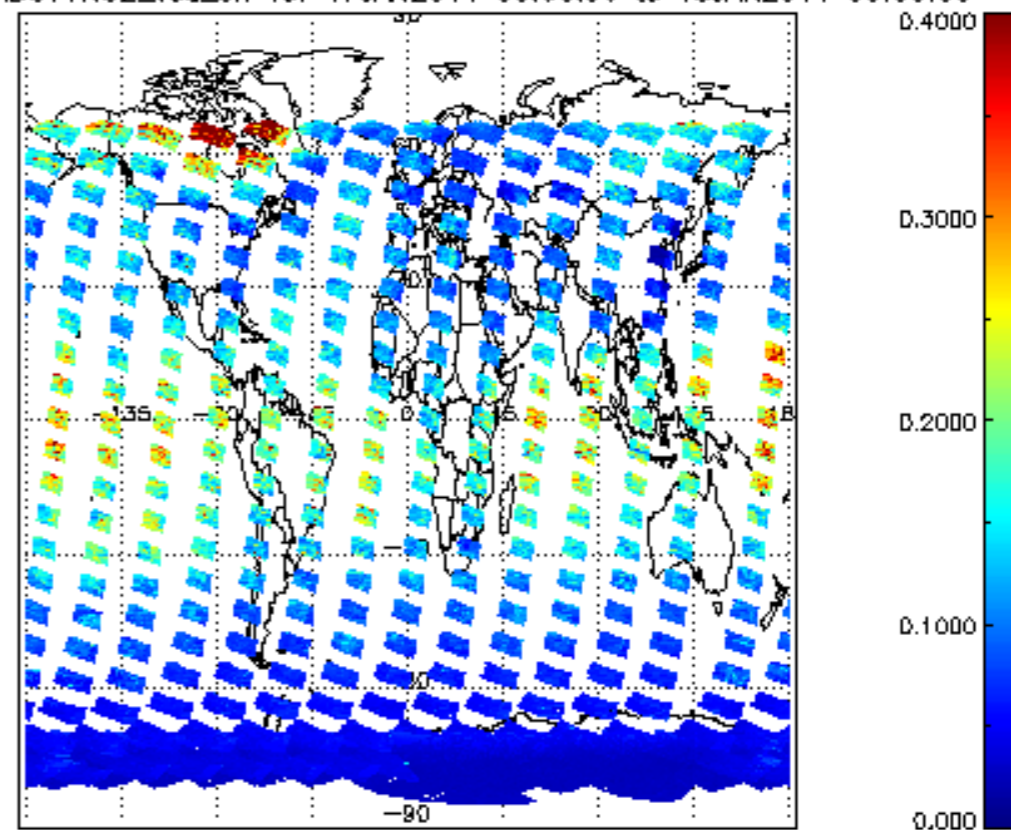
SCIOL2P_NADUV1NO2_vcd_err for 17JAN2011 00:00:00 to 18JAN2011 00:00:00
