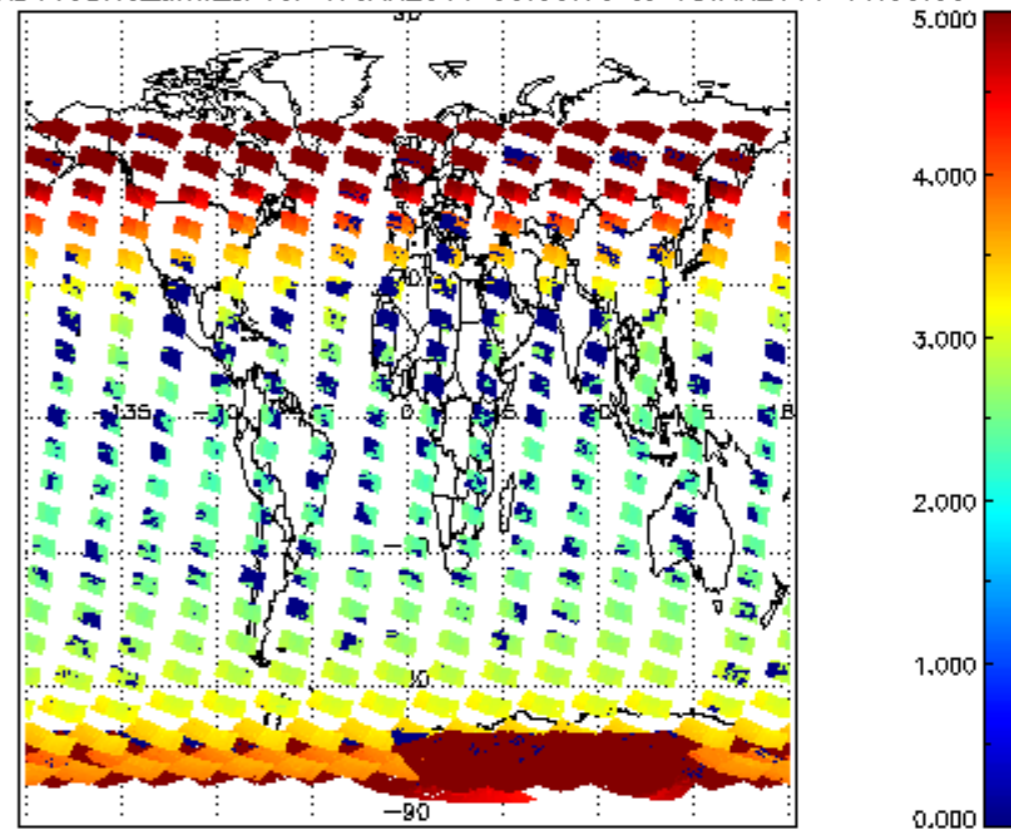
SCIOL2P_NADUV3BRO_amf_cl for 17JAN2011 00:00:00 to 18JAN2011 00:00:00
