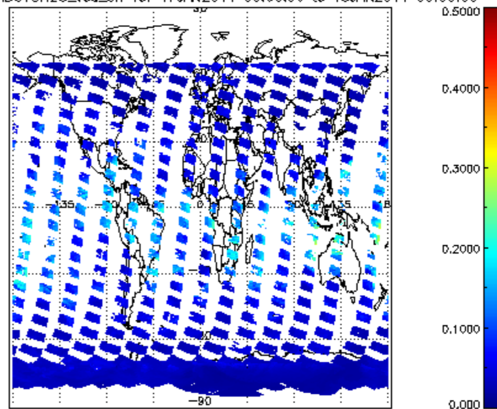
SCIOL2P_NADUV8H20_vcd_err for 17JAN2011 00:00:00 to 18JAN2011 00:00:00
