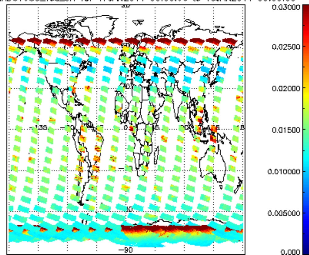
SCIOL2P_NADUV003_vcd_err for 17JAN2011 00:00:00 to 18JAN2011 00:00:00
