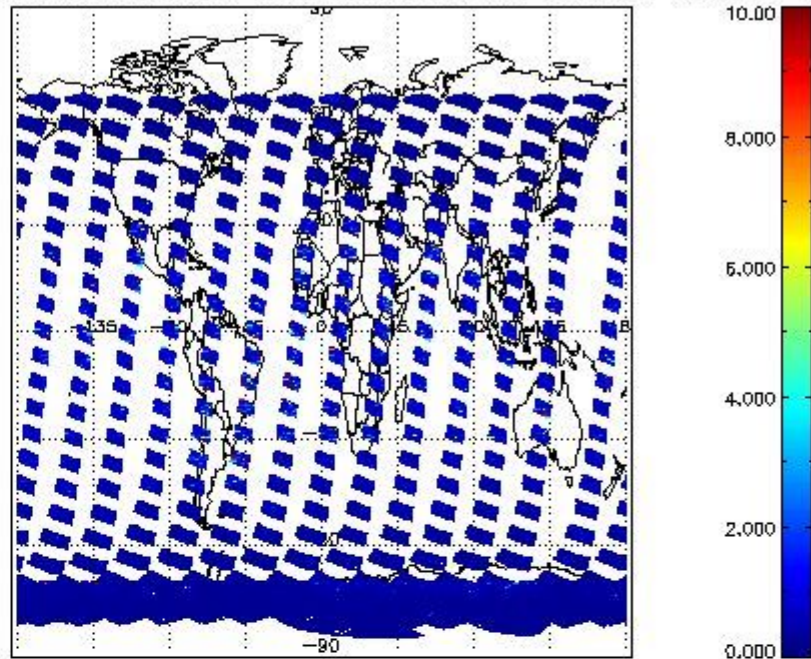
SCIOL2P_NADUV3BRO_vcd_err for 17JAN2011 00:00:00 to 18JAN2011 00:00:00
