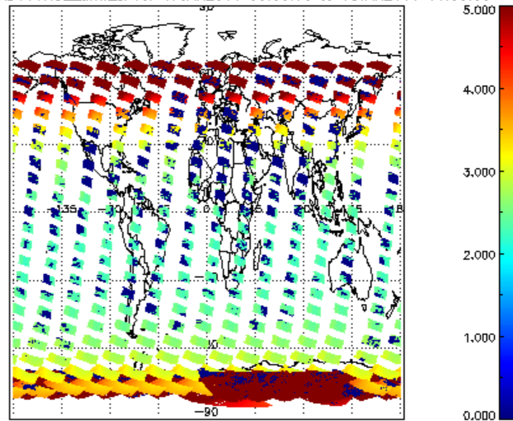
SCIOL2P_NADUV1NO2_amf_cl for 17JAN2011 00:00:00 to 18JAN2011 00:00:00
