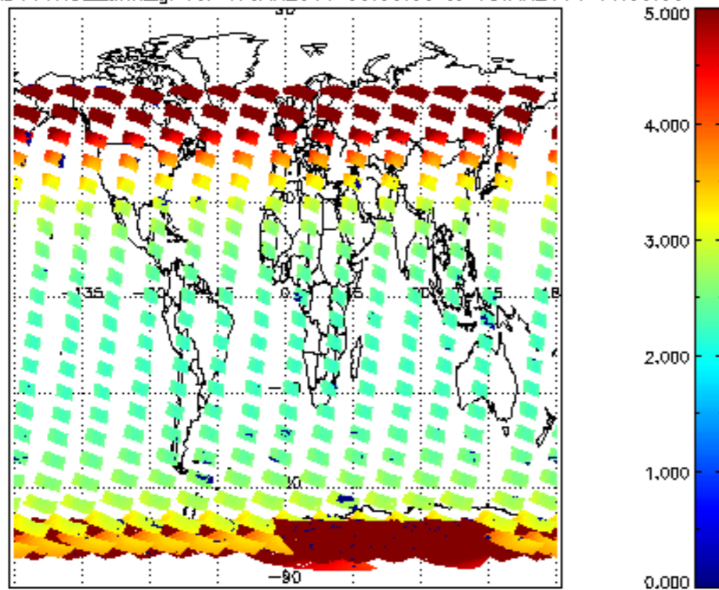
SCIOL2P_NADUV1NO2_amf_gr for 17JAN2011 00:00:00 to 18JAN2011 00:00:00
