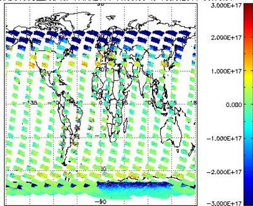
SCIOL2P_NADUV5SO2_vcd for 17JAN2011 00:00:00 to 18JAN2011 00:00:00
