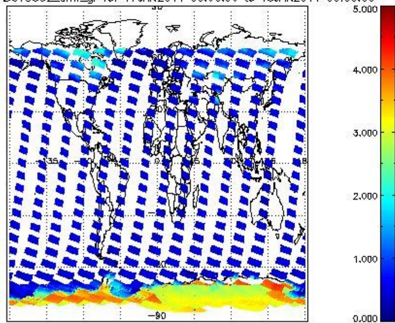
SCIOL2P_NADUV5SO2_amf_gr for 17JAN2011 00:00:00 to 18JAN2011 00:00:00
