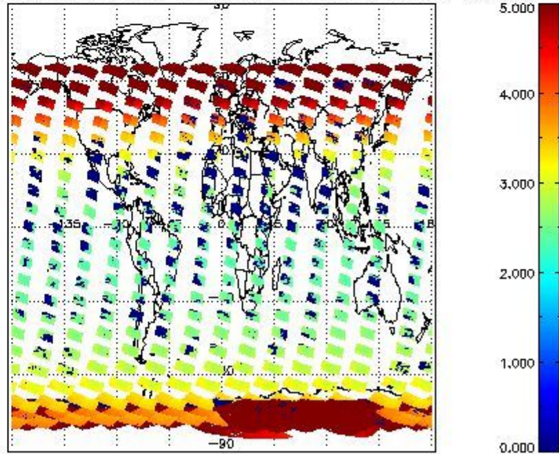
SCIOL2P_NADUV3BRO_amf_cl for 17JAN2011 00:00:00 to 18JAN2011 00:00:00
