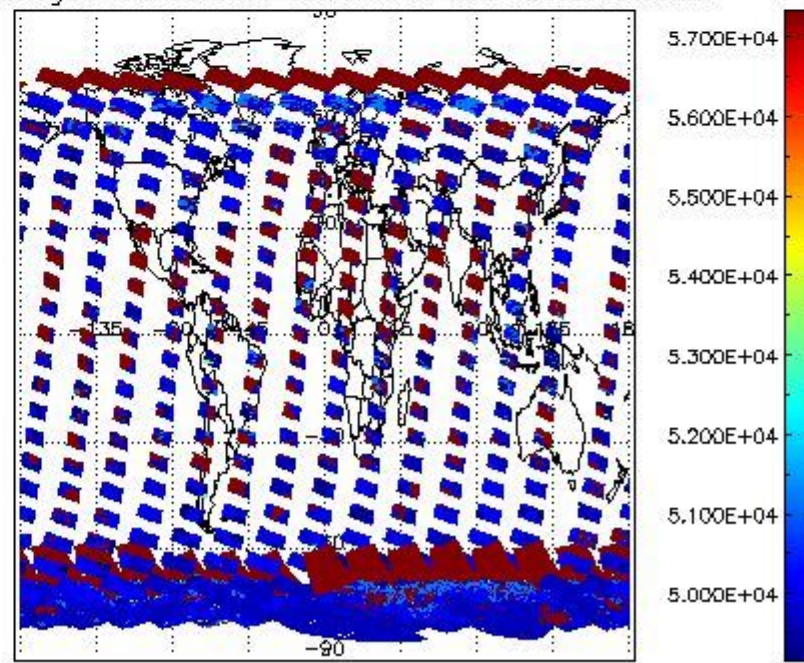
cloud_flags for 17JAN2011 00:00:00 to 18JAN2011 00:00:00
