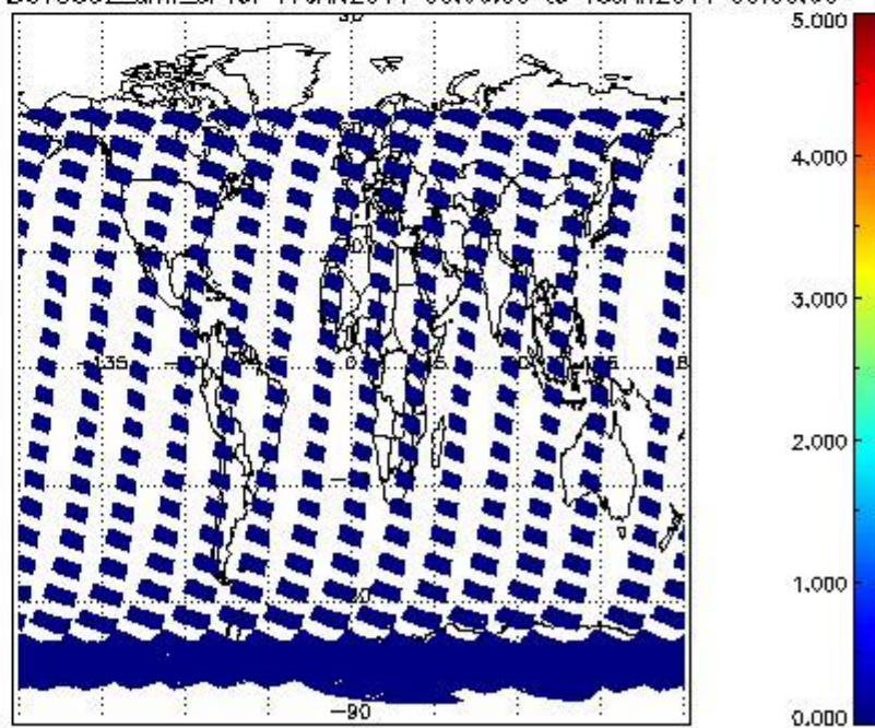
SCIOL2P_NADUV5SO2_amf_cl for 17JAN2011 00:00:00 to 18JAN2011 00:00:00
