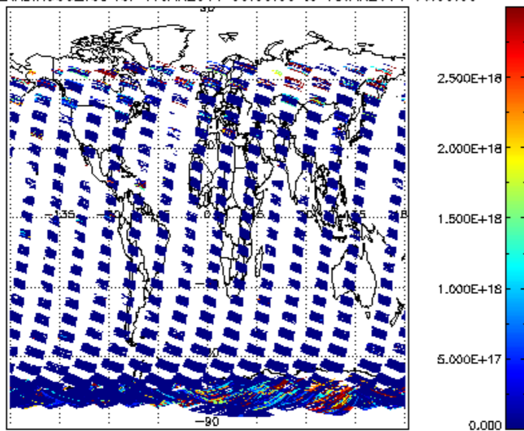
SCIOL2P_NADIR3CO_vcd for 17JAN2011 00:00:00 to 18JAN2011 00:00:00
