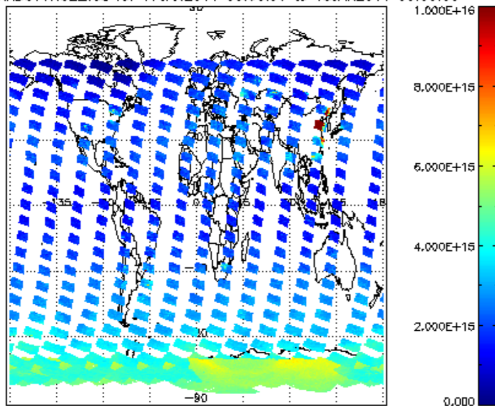
SCIOL2P_NADUV1NO2_vcd for 17JAN2011 00:00:00 to 18JAN2011 00:00:00
