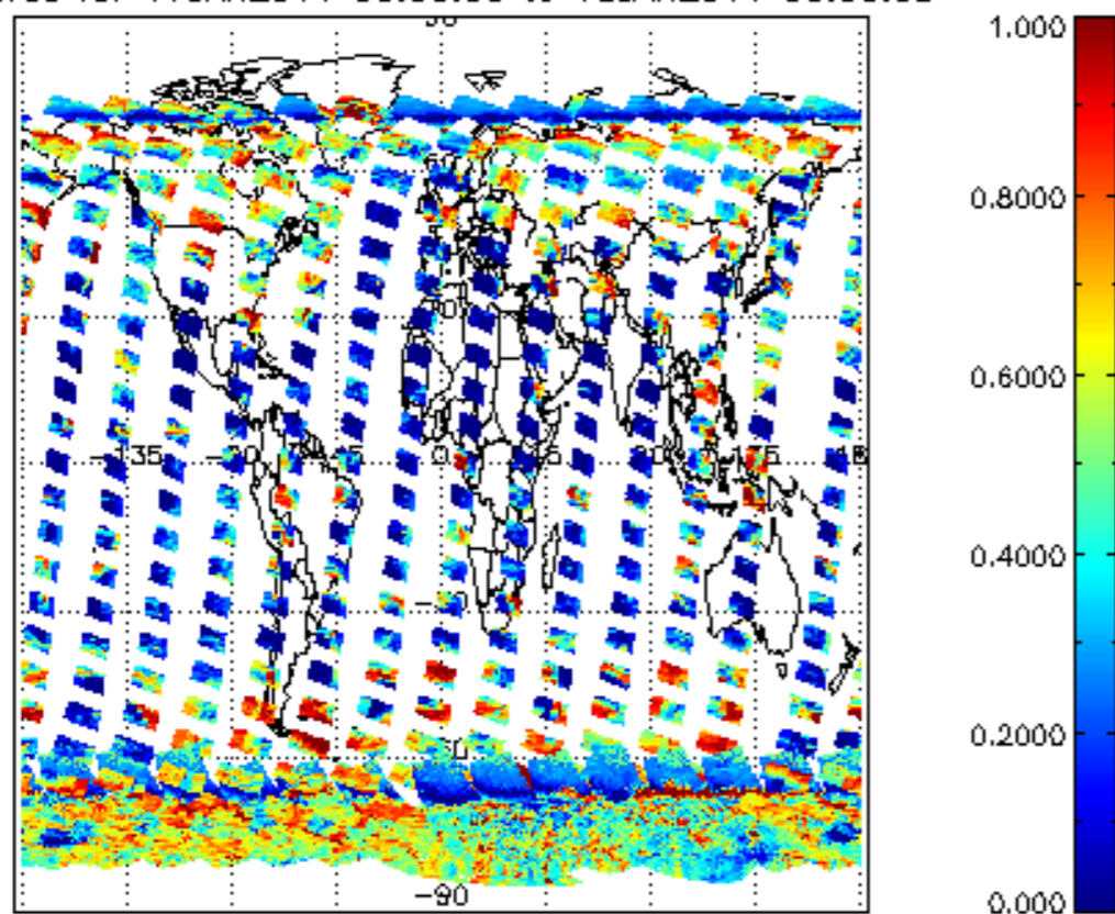
cL_frac for 17JAN2011 00:00:00 to 18JAN2011 00:00:00
