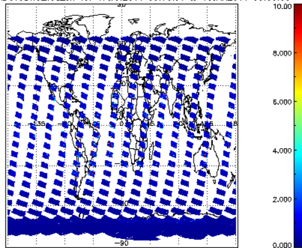
SCIOL2P_NADUV3BRO_vcd_err for 17JAN2011 00:00:00 to 18JAN2011 00:00:00
