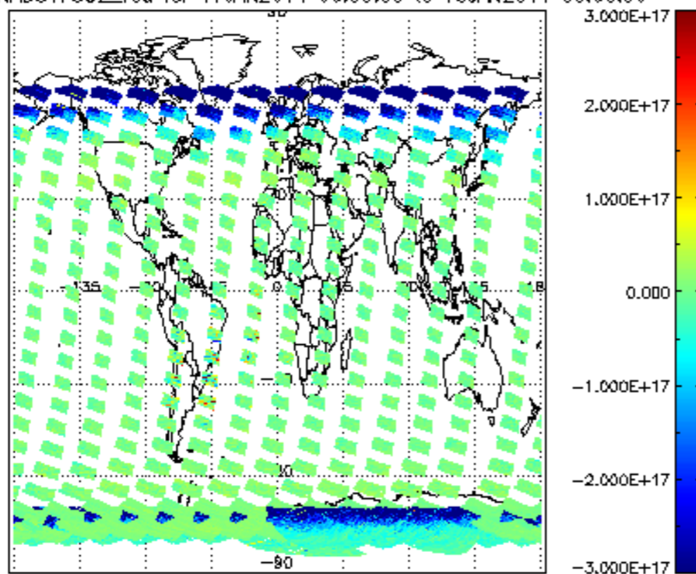
SCIOL2P_NADUV7S02_vcd for 17JAN2011 00:00:00 to 18JAN2011 00:00:00
