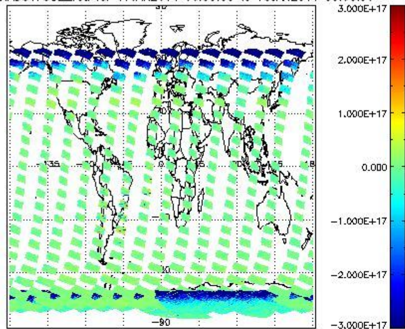
SCIOL2P_NADUV7S02_vcd for 17JAN2011 00:00:00 to 18JAN2011 00:00:00
