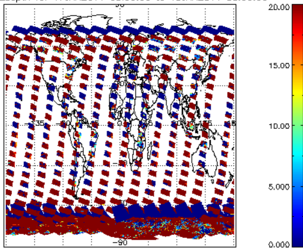
cLopt_depth for 17JAN2011 00:00:00 to 18JAN2011 00:00:00
