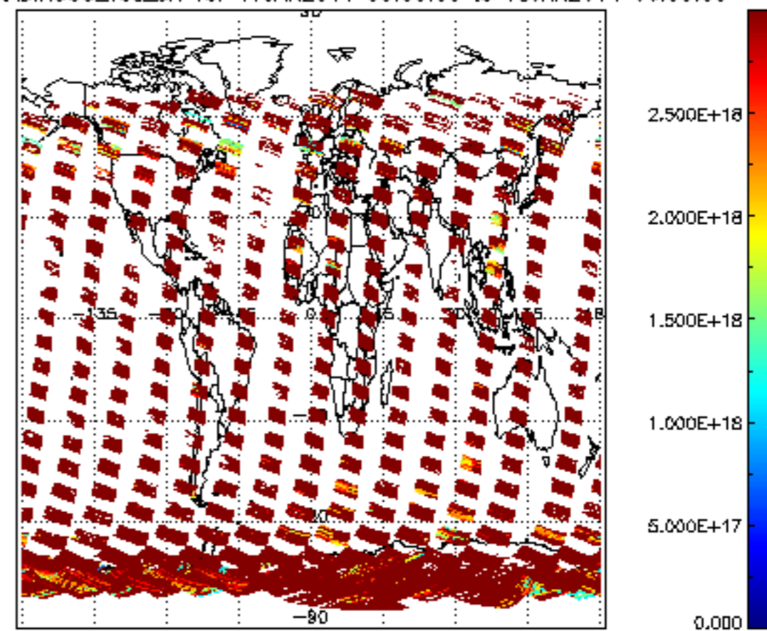
SCIOL2P_NADIR3CO_vcd_err for 17JAN2011 00:00:00 to 18JAN2011 00:00:00
