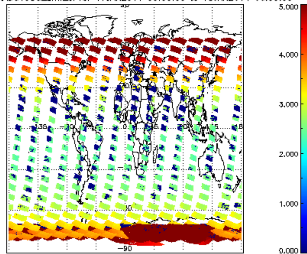
SCIOL2P_NADUV003_amf_cl for 17JAN2011 00:00:00 to 18JAN2011 00:00:00
