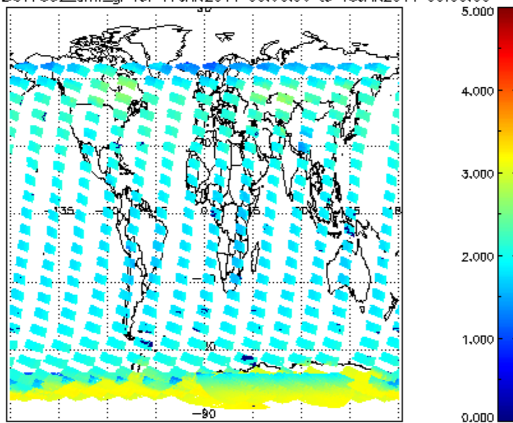
SCIOL2P_NADUV7S02_amf_gr for 17JAN2011 00:00:00 to 18JAN2011 00:00:00
