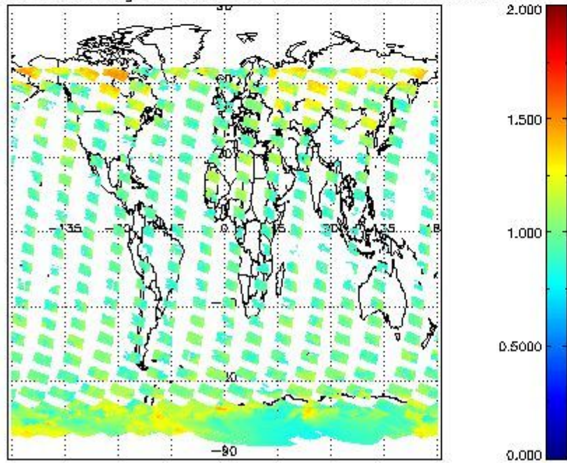
SCIOL2P_NADUV8H20_amf_gr for 17JAN2011 00:00:00 to 18JAN2011 00:00:00
