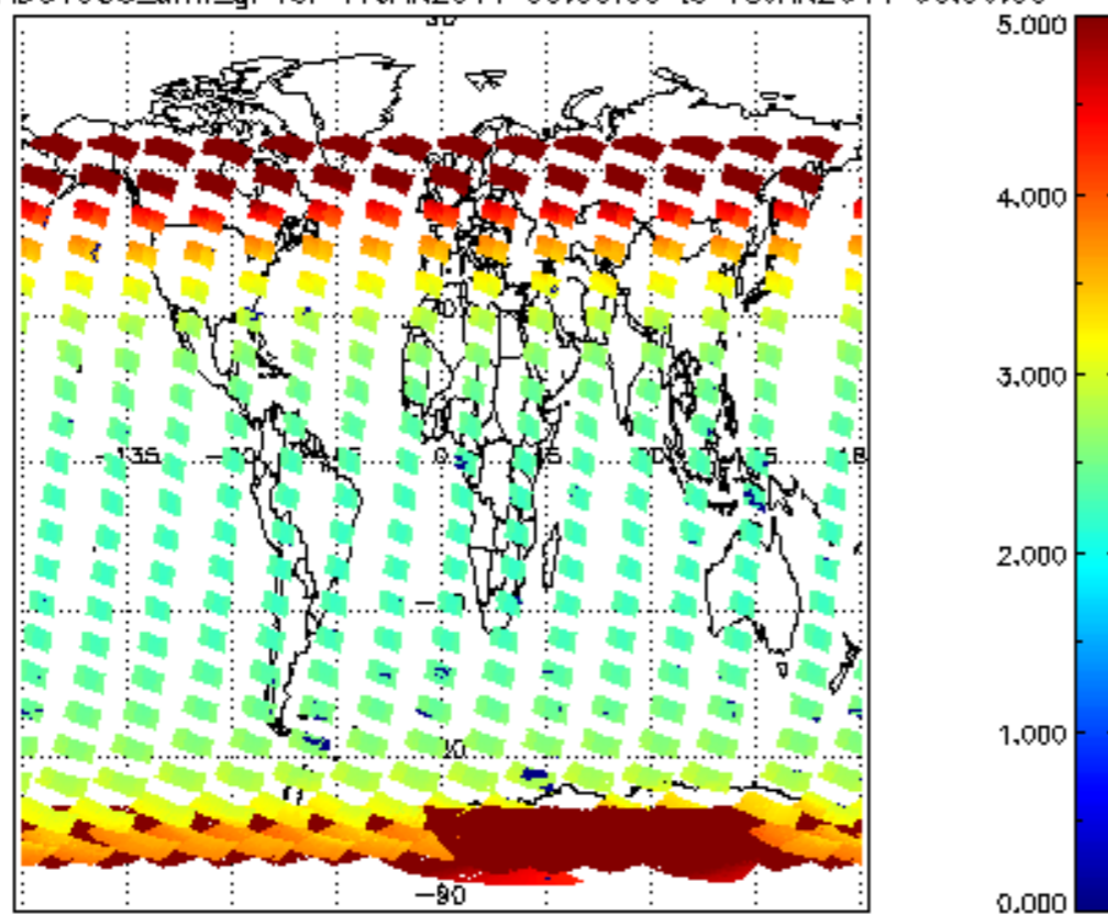
SCIOL2P_NADUV003_amf_gr for 17JAN2011 00:00:00 to 18JAN2011 00:00:00
