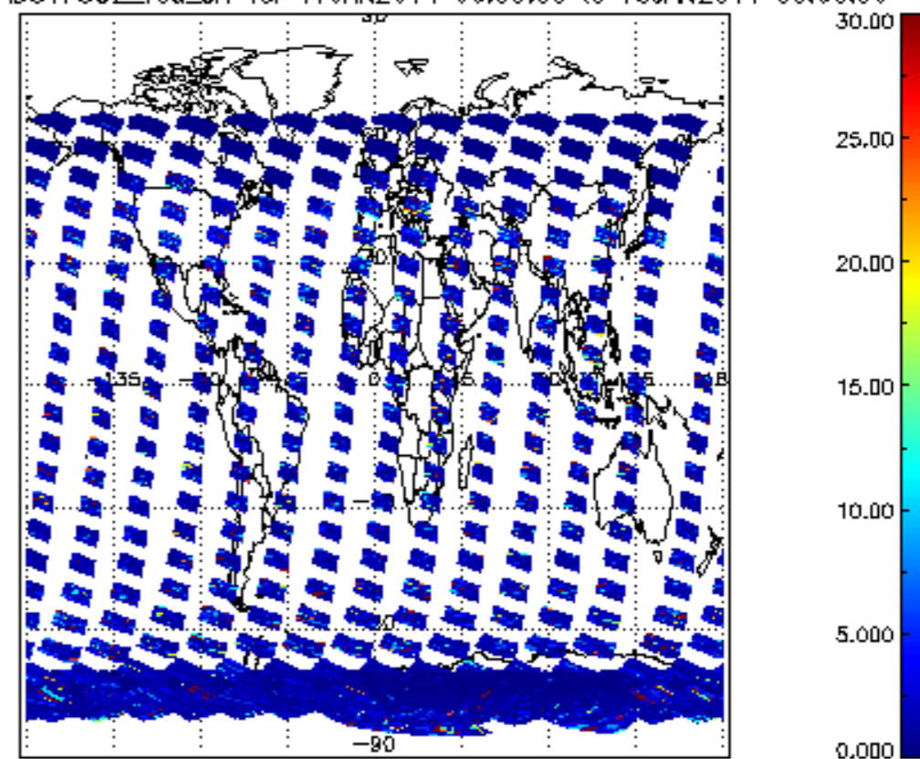
SCIOL2P_NADUV7S02_vcd_err for 17JAN2011 00:00:00 to 18JAN2011 00:00:00
