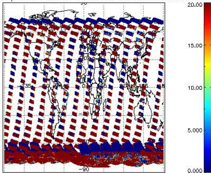
cLopt_depth for 17JAN2011 00:00:00 to 18JAN2011 00:00:00
