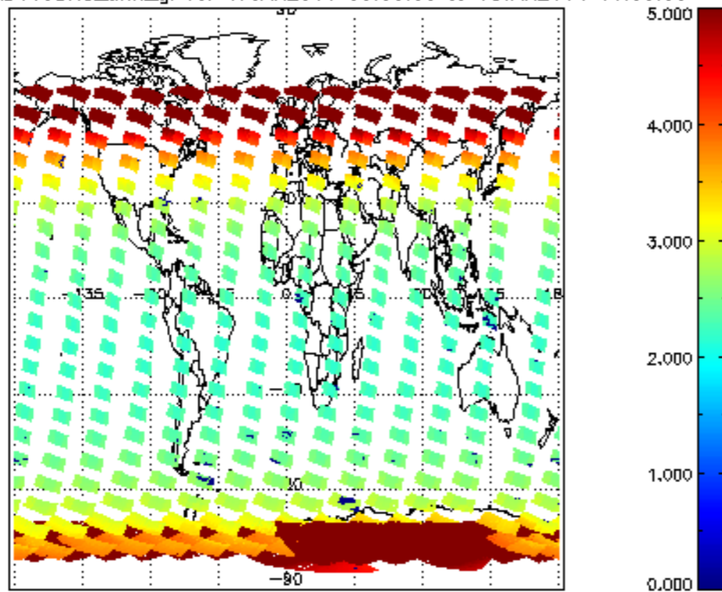
SCIOL2P_NADUV3BRO_amf_gr for 17JAN2011 00:00:00 to 18JAN2011 00:00:00
