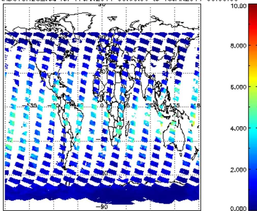
SCIOL2P_NADUV8H20_vcd for 17JAN2011 00:00:00 to 18JAN2011 00:00:00
