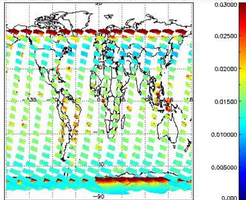
SCIOL2P_NADUV003_vcd_err for 17JAN2011 00:00:00 to 18JAN2011 00:00:00
