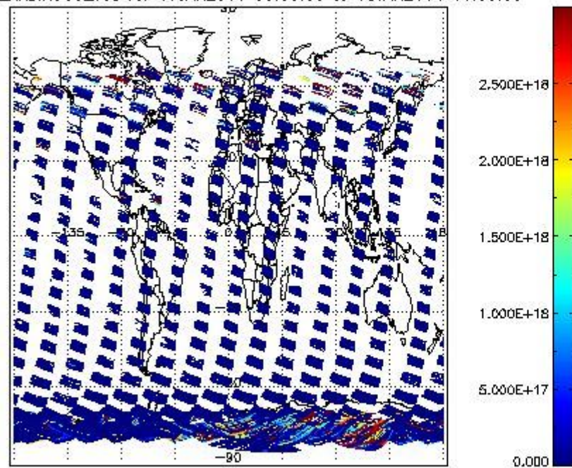
SCIDL2P_NADIR3CO_vcd for 17JAN2011 00:00:00 to 18JAN2011 00:00:00
