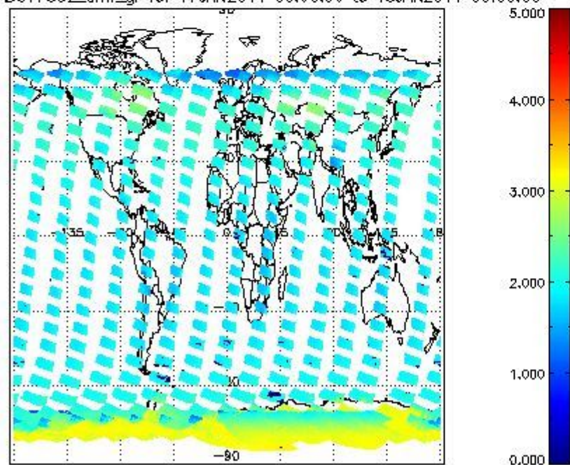
SCIOL2P_NADUV7S02_amf_gr for 17JAN2011 00:00:00 to 18JAN2011 00:00:00
