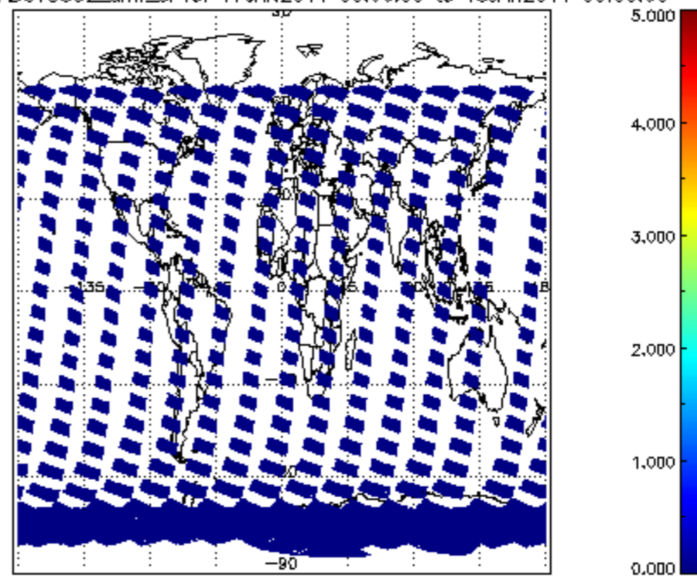
SCIOL2P_NADUV5S02_amf_cl for 17JAN2011 00:00:00 to 18JAN2011 00:00:00
