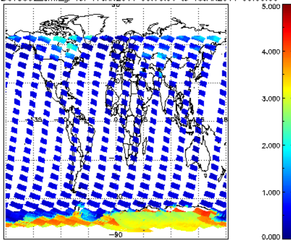
SCIOL2P_NADUV5S02_amf_gr for 17JAN2011 00:00:00 to 18JAN2011 00:00:00
