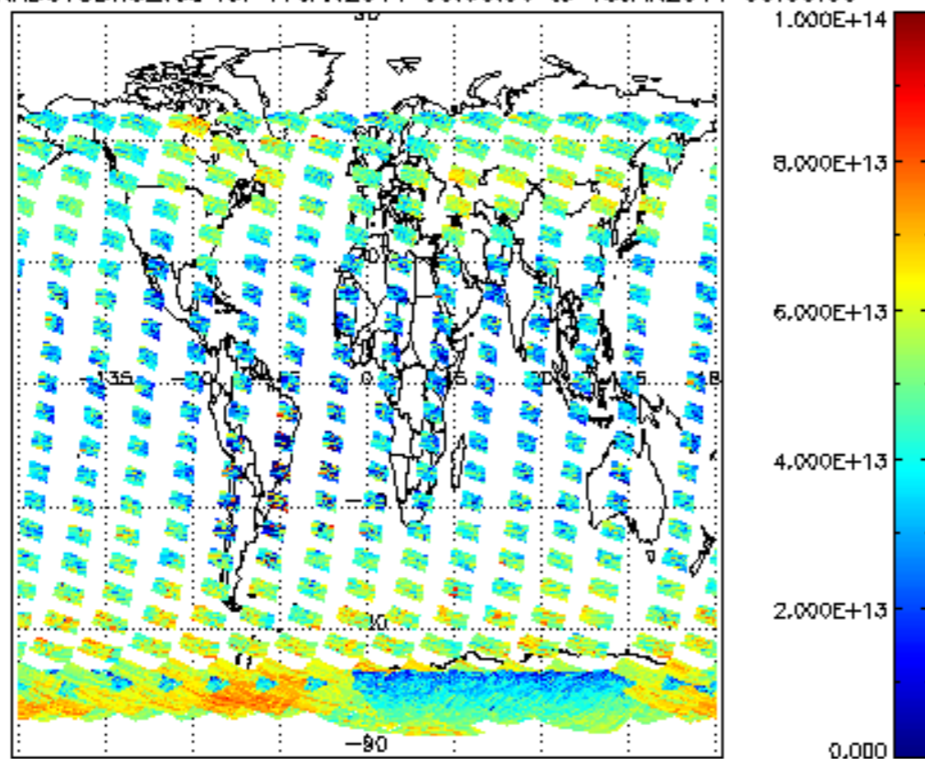
SCIOL2P_NADUV3BRO_vcd for 17JAN2011 00:00:00 to 18JAN2011 00:00:00
