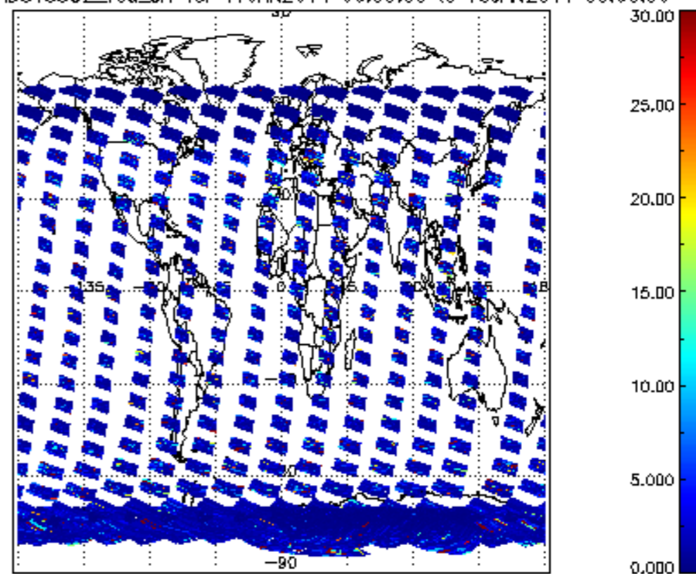
SCIOL2P_NADUV5S02_vcd_err for 17JAN2011 00:00:00 to 18JAN2011 00:00:00
