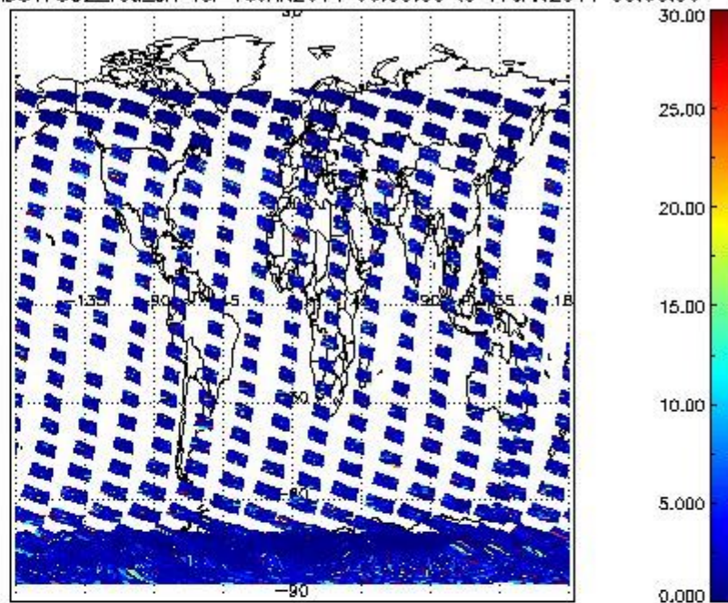
SCIOL2P_NADUV7S02_vcd_err for 16JAN2011 00:00:00 to 17JAN2011 00:00:00
