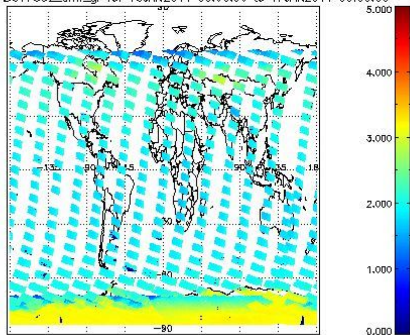
SCIOL2P_NADUV7S02_amf_gr for 16JAN2011 00:00:00 to 17JAN2011 00:00:00
