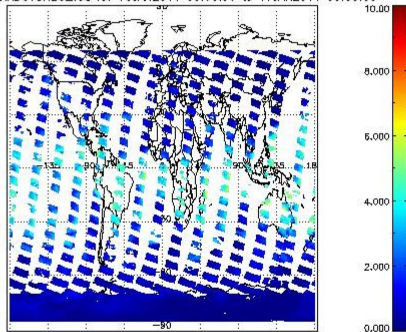
SCIOL2P_NADUV8H20_vcd for 16JAN2011 00:00:00 to 17JAN2011 00:00:00
