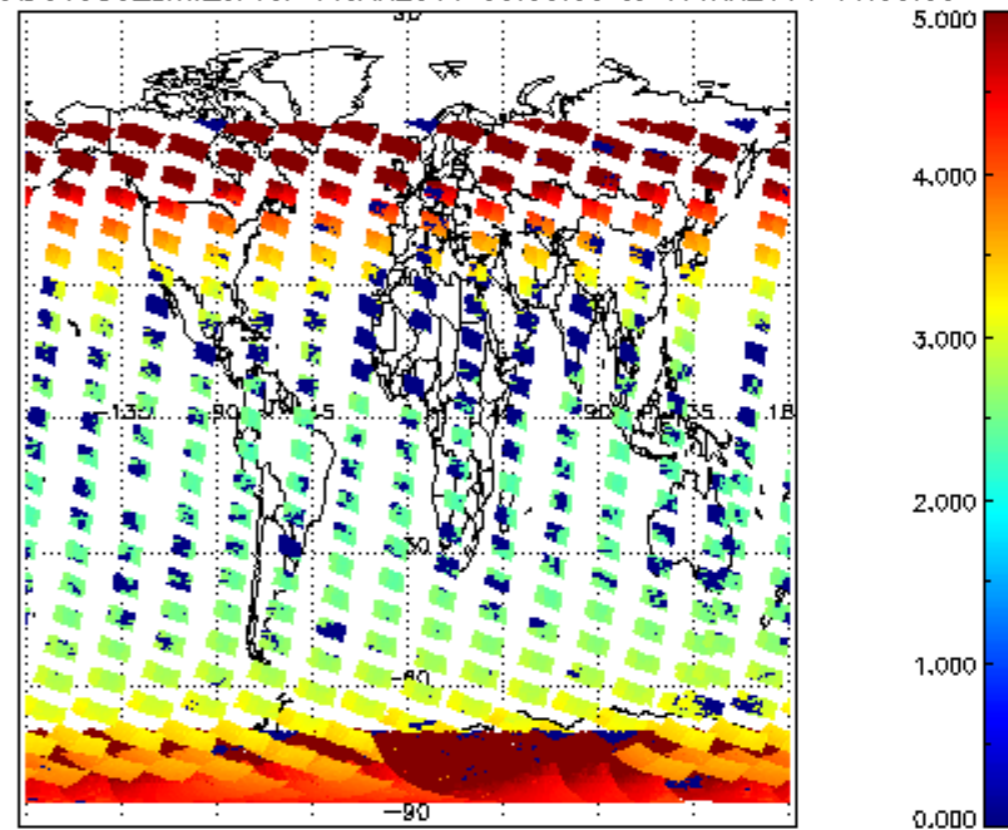
SCIOL2P_NADUV003_amf_cl for 16JAN2011 00:00:00 to 17JAN2011 00:00:00
