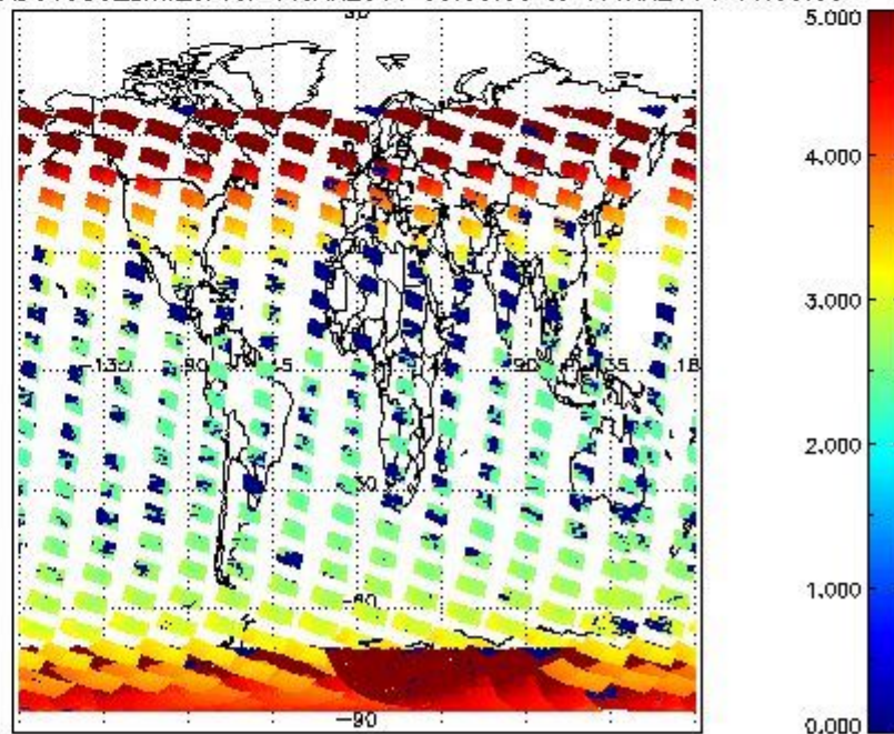
SCIOL2P_NADUV003_amf_cl for 16JAN2011 00:00:00 to 17JAN2011 00:00:00
