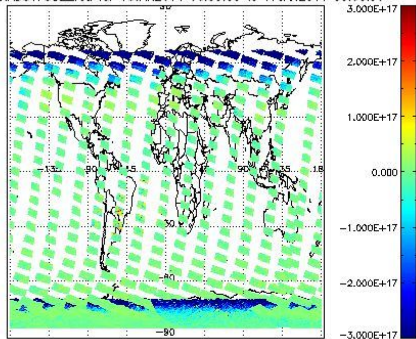
SCIOL2P_NADUV7S02_vcd for 16JAN2011 00:00:00 to 17JAN2011 00:00:00
