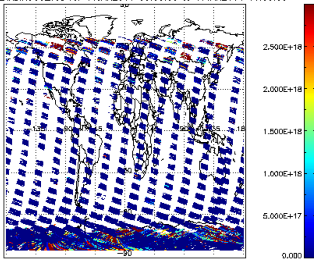
SCIOL2P_NADIR3CO_vcd for 16JAN2011 00:00:00 to 17JAN2011 00:00:00
