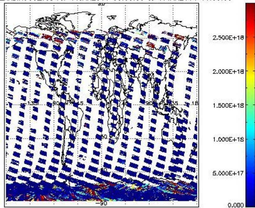
SCIDL2P_NADIR3CO_vcd for 16JAN2011 00:00:00 to 17JAN2011 00:00:00
