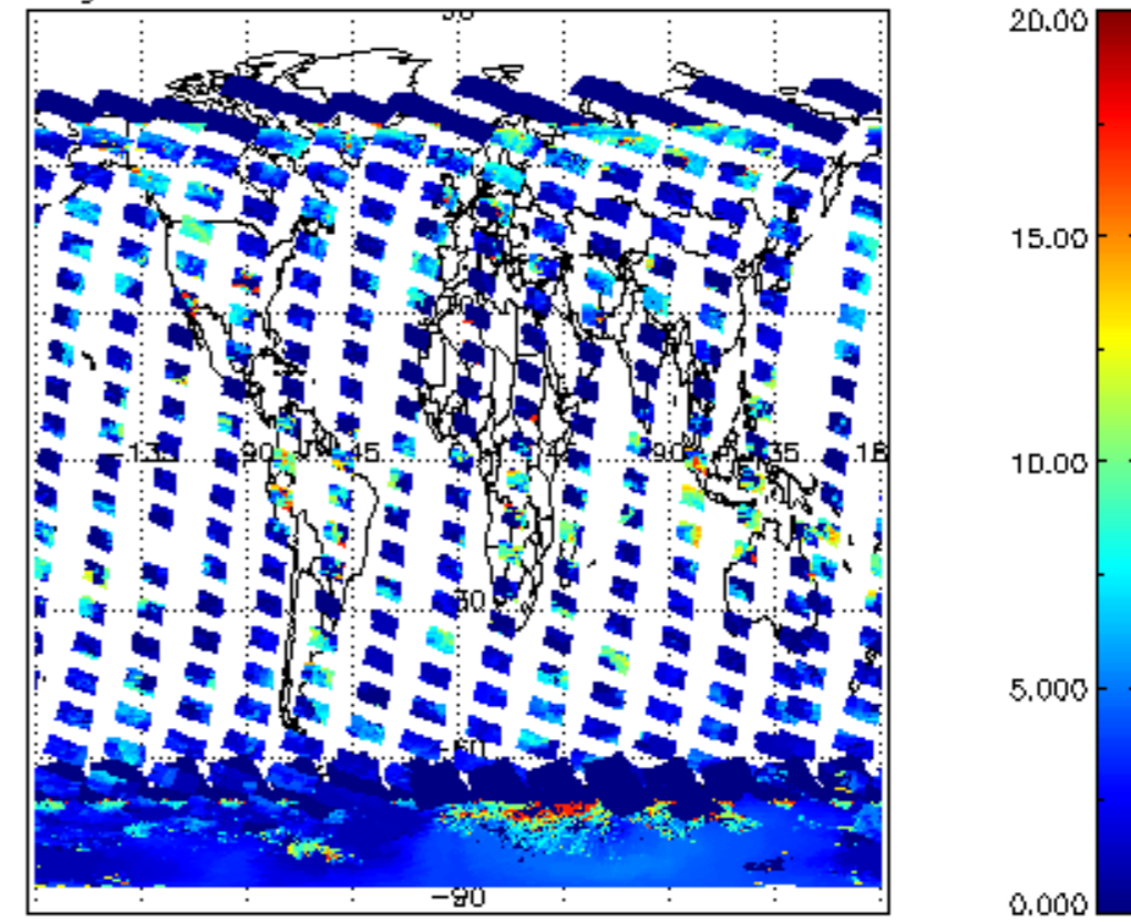
cL_top_height for 16JAN2011 00:00:00 to 17JAN2011 00:00:00
