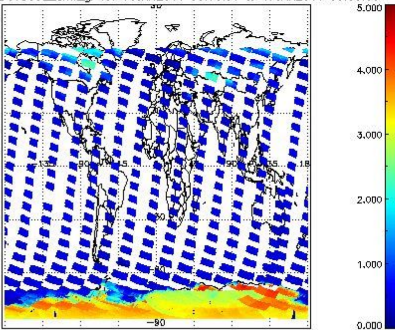
SCIOL2P_NADUV5S02_amf_gr for 16JAN2011 00:00:00 to 17JAN2011 00:00:00
