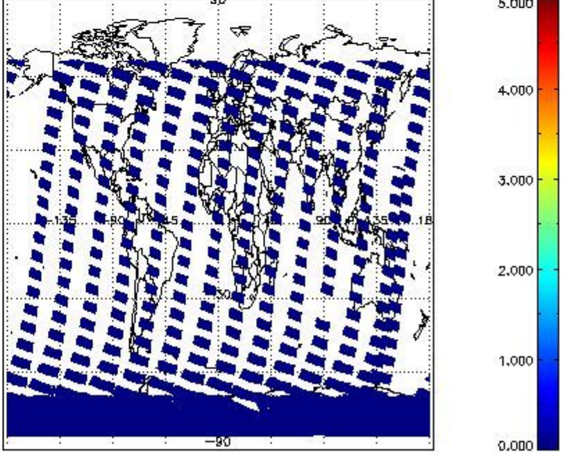
SCIOL2P_NADUV5SO2_amf_cl for 13JAN2011 00:00:00 to 14JAN2011 00:00:00
