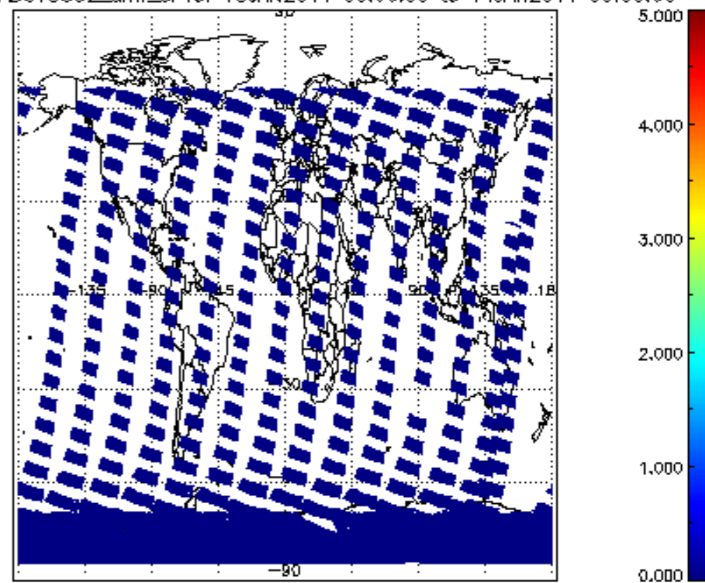
SCIOL2P_NADUV5S02_amf_sl for 13JAN2011 00:00:00 to 14JAN2011 00:00:00
