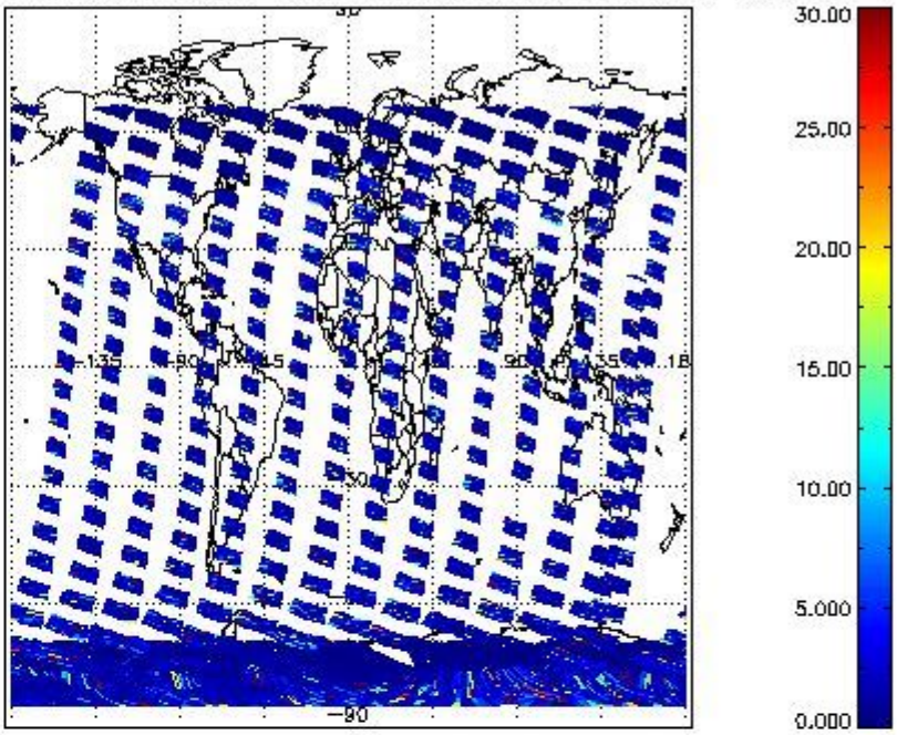
SCIOL2P_NADUV5SO2_vcd_err for 13JAN2011 00:00:00 to 14JAN2011 00:00:00
