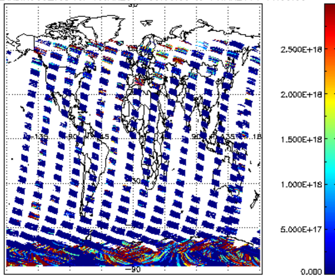
SCIOL2P_NADIR3CO_vcd for 13JAN2011 00:00:00 to 14JAN2011 00:00:00
