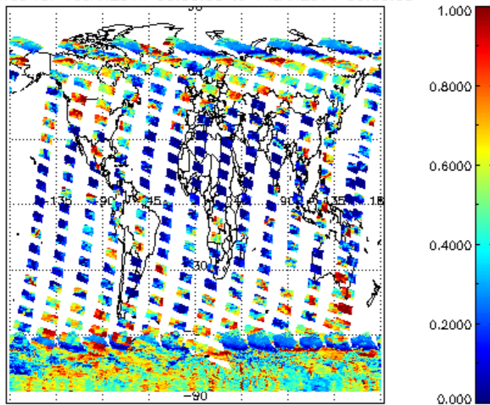
cL_frac for 13JAN2011 00:00:00 to 14JAN2011 00:00:00
