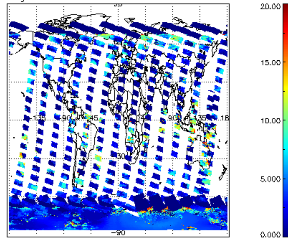
cL_top_height for 13JAN2011 00:00:00 to 14JAN2011 00:00:00
