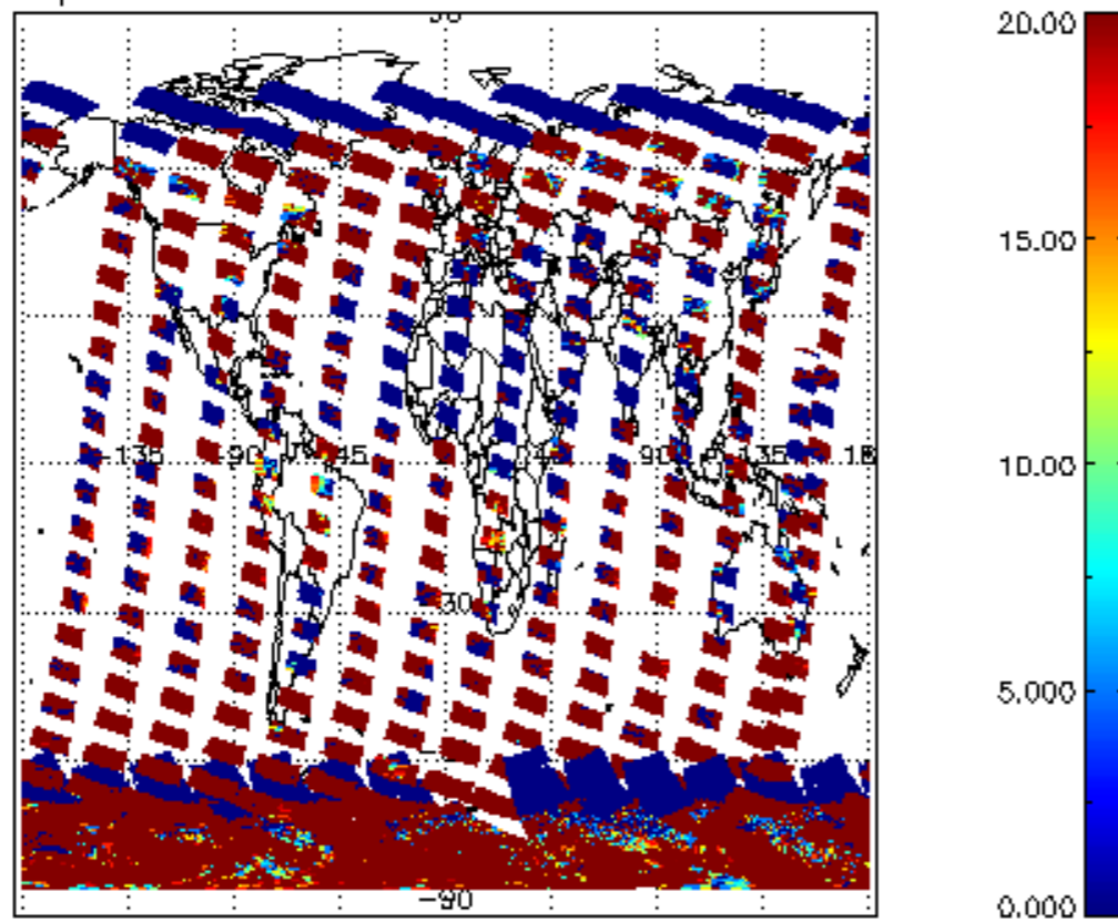
cLopt_depth for 13JAN2011 00:00:00 to 14JAN2011 00:00:00
