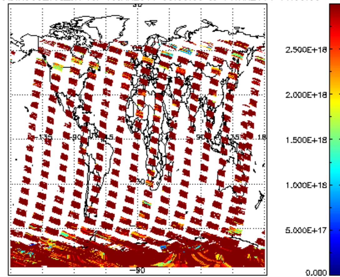
SCIOL2P_NADIR3CO_vcd_err for 13JAN2011 00:00:00 to 14JAN2011 00:00:00
