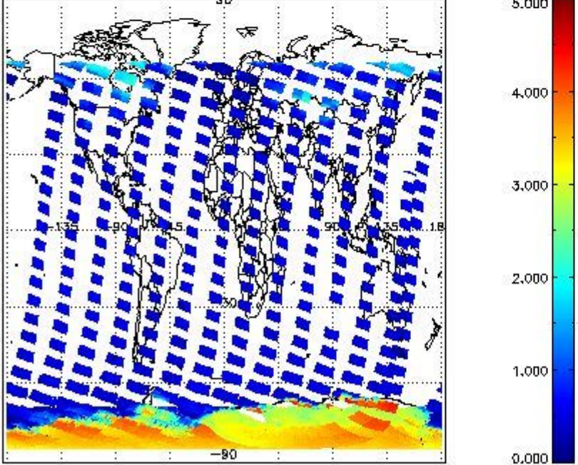
SCIOL2P_NADUV5SO2_amf_gr for 13JAN2011 00:00:00 to 14JAN2011 00:00:00
