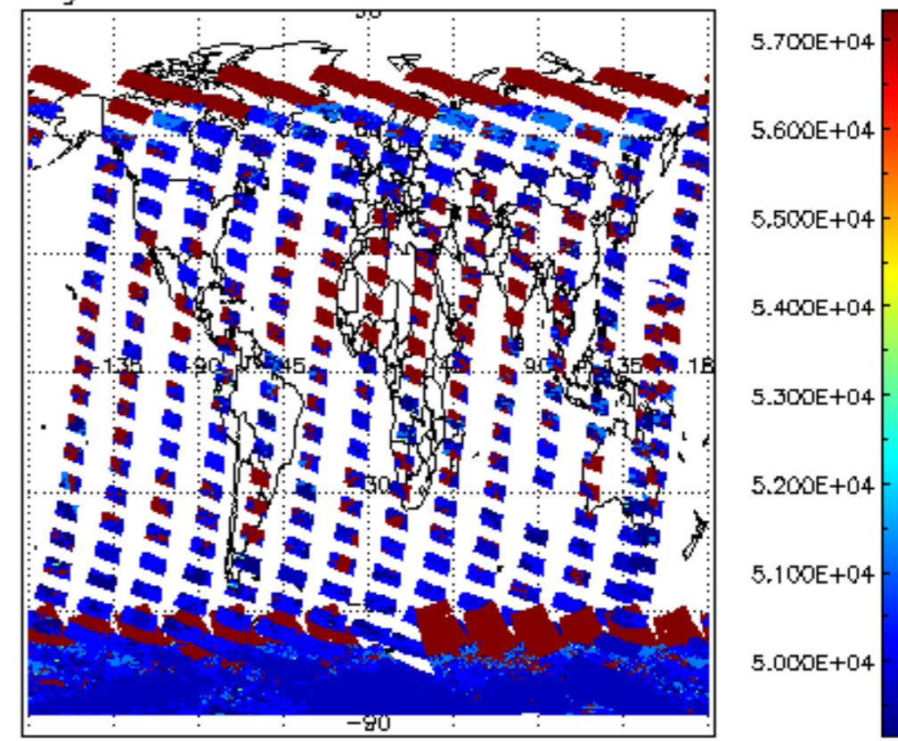
cloud_flags for 13JAN2011 00:00:00 to 14JAN2011 00:00:00
