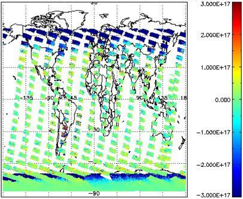
SCIOL2P_NADUV5SO2_vcd for 13JAN2011 00:00:00 to 14JAN2011 00:00:00
