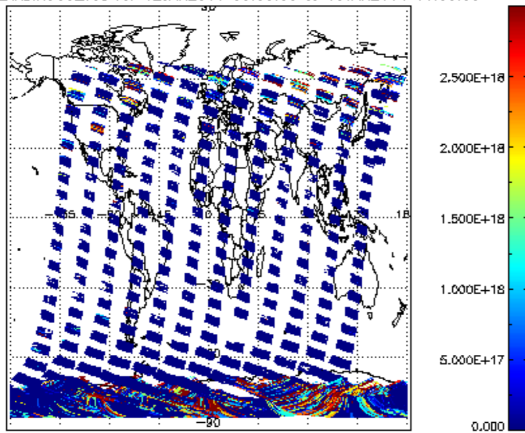
SCIOL2P_NADIR3CO_vcd for 12JAN2011 00:00:00 to 13JAN2011 00:00:00
