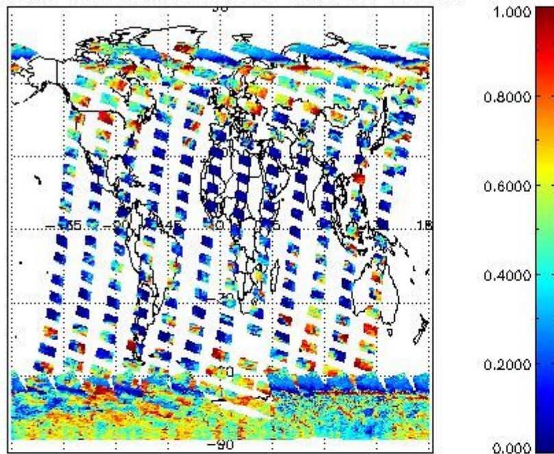
cL_frac for 12JAN2011 00:00:00 to 13JAN2011 00:00:00
