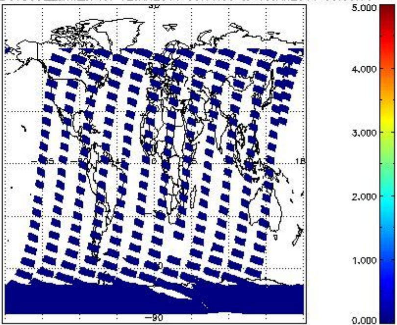
SCIOL2P_NADUV5SO2_amf_cl for 12JAN2011 00:00:00 to 13JAN2011 00:00:00
