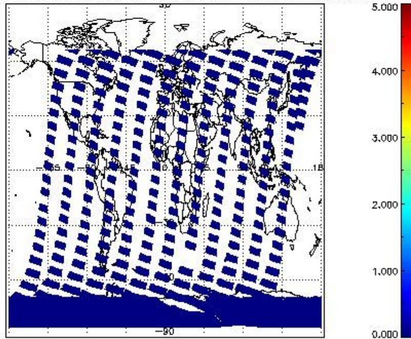
SCIOL2P_NADUV7S02_amf_cl for 12JAN2011 00:00:00 to 13JAN2011 00:00:00
