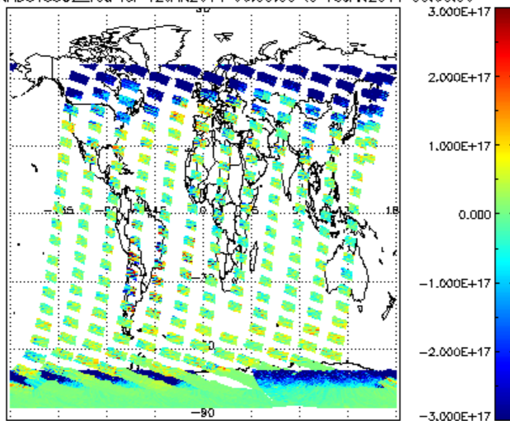
SCIOL2P_NADUV5S02_vcd for 12JAN2011 00:00:00 to 13JAN2011 00:00:00
