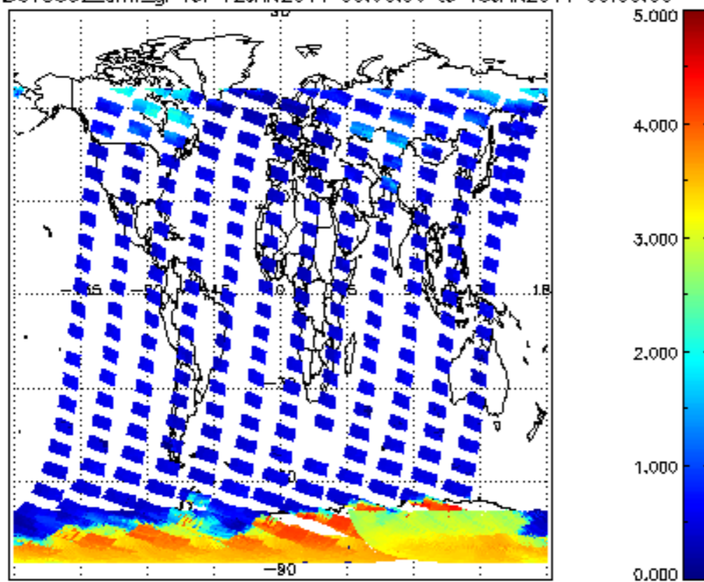
SCIOL2P_NADUV5S02_amf_gr for 12JAN2011 00:00:00 to 13JAN2011 00:00:00
