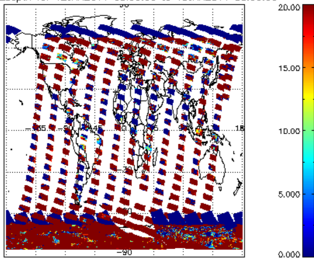
cLopt_depth for 12JAN2011 00:00:00 to 13JAN2011 00:00:00
