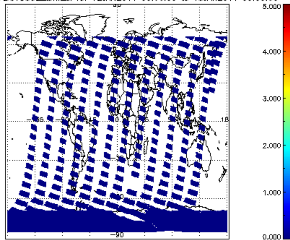
SCIOL2P_NADUV5S02_amf_cl for 12JAN2011 00:00:00 to 13JAN2011 00:00:00
