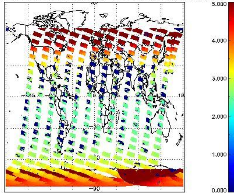
SCIOL2P_NADUV003_amf_cl for 12JAN2011 00:00:00 to 13JAN2011 00:00:00
