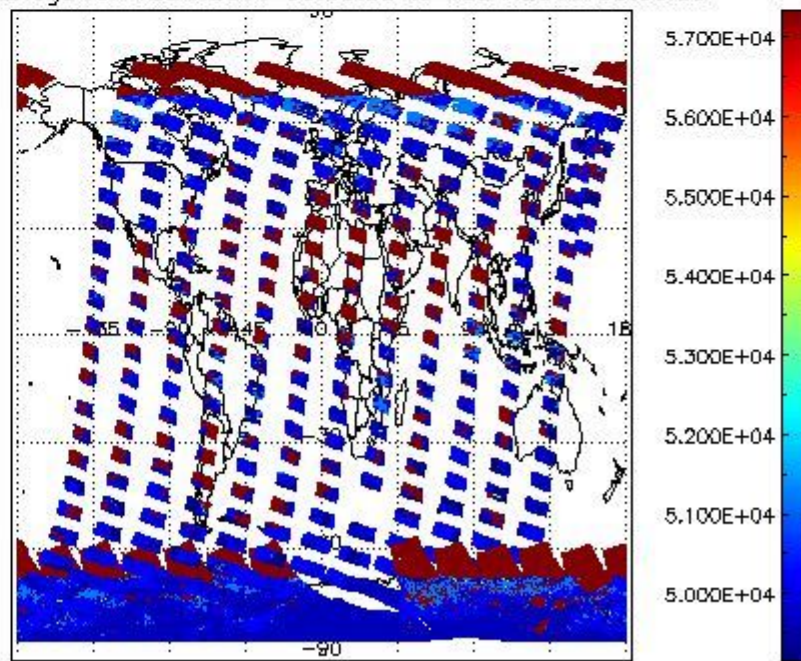
cloud_flags for 12JAN2011 00:00:00 to 13JAN2011 00:00:00
