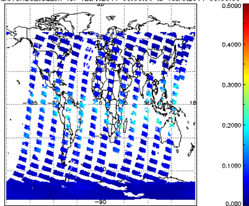
SCIOL2P_NADUVBH20_vcd_err for 12JAN2011 00:00:00 to 13JAN2011 00:00:00
