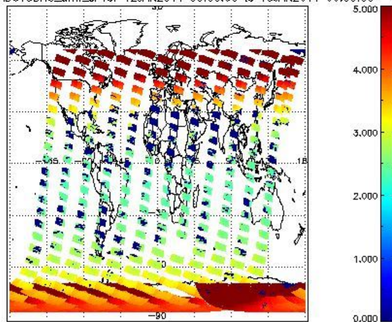
SCIOL2P_NADUV3BRO_amf_cl for 12JAN2011 00:00:00 to 13JAN2011 00:00:00
