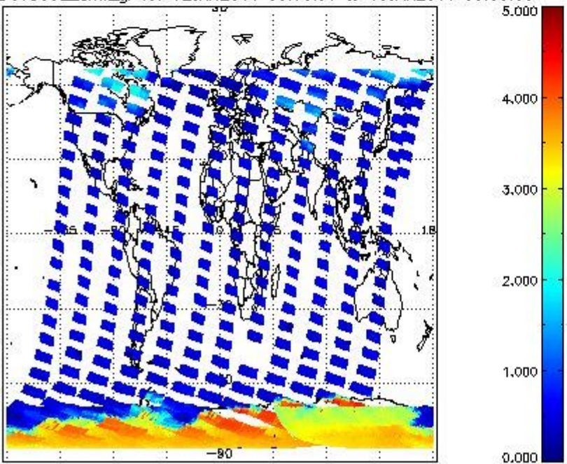
SCIOL2P_NADUV5SO2_amf_gr for 12JAN2011 00:00:00 to 13JAN2011 00:00:00
