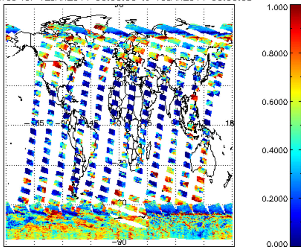
cL_frac for 12JAN2011 00:00:00 to 13JAN2011 00:00:00
