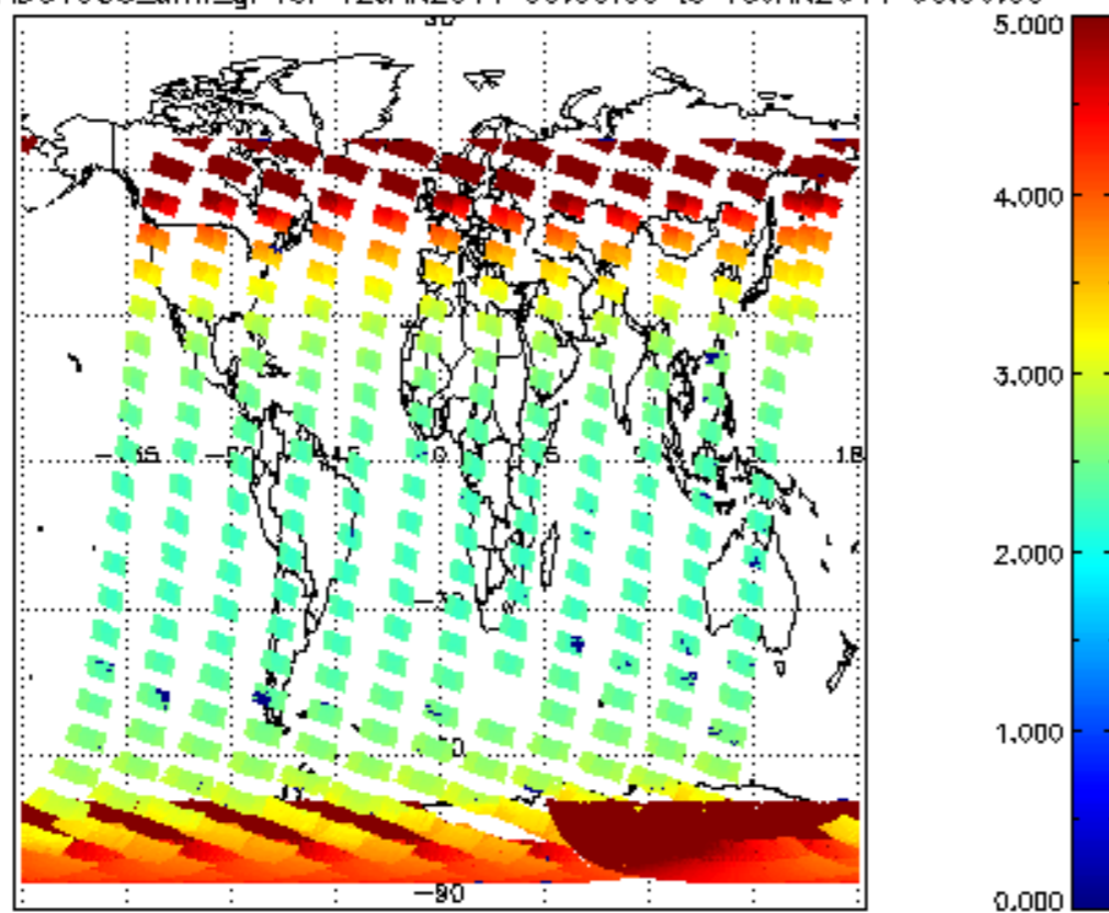
SCIOL2P_NADUV003_amf_gr for 12JAN2011 00:00:00 to 13JAN2011 00:00:00
