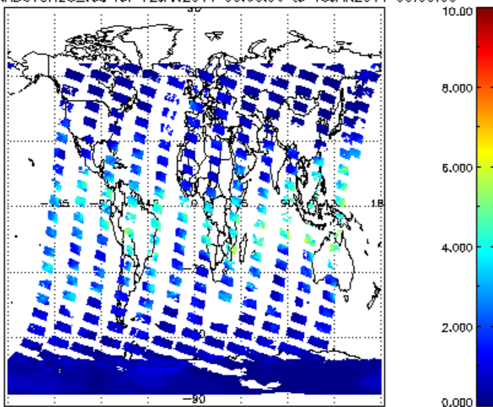
SCIOL2P_NADUVBH20_vcd for 12JAN2011 00:00:00 to 13JAN2011 00:00:00
