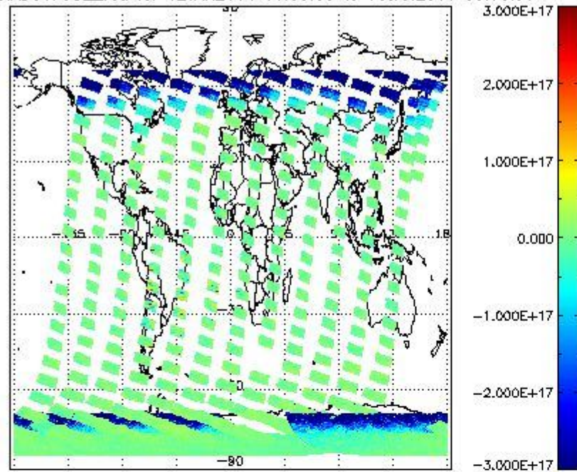
SCIOL2P_NADUV7S02_vcd for 12JAN2011 00:00:00 to 13JAN2011 00:00:00
