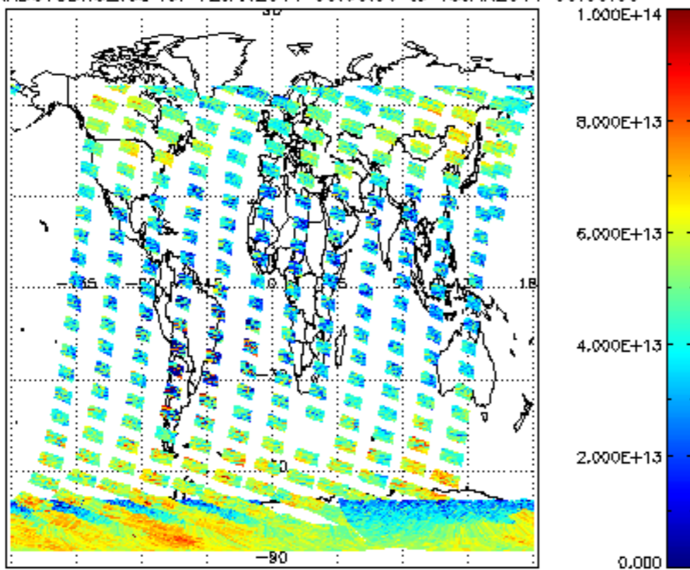
SCIOL2P_NADUV3BRO_vcd for 12JAN2011 00:00:00 to 13JAN2011 00:00:00
