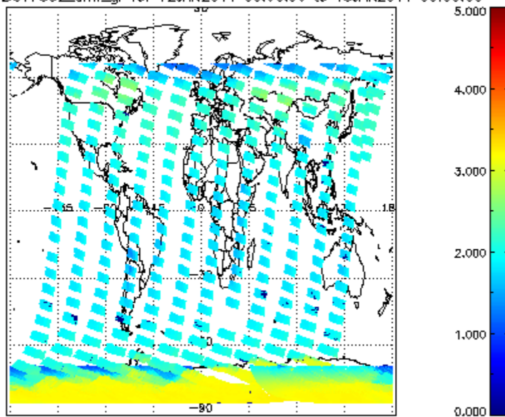
SCIOL2P_NADUV7S02_amf_gr for 12JAN2011 00:00:00 to 13JAN2011 00:00:00
