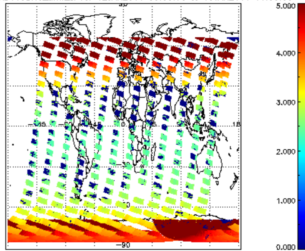
SCIOL2P_NADUV3BRO_amf_cl for 12JAN2011 00:00:00 to 13JAN2011 00:00:00
