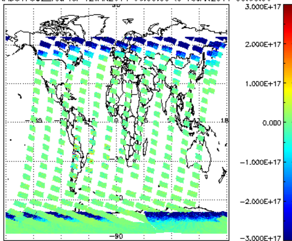
SCIOL2P_NADUV7S02_vcd for 12JAN2011 00:00:00 to 13JAN2011 00:00:00
