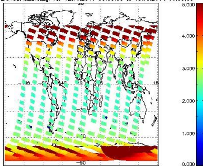
SCIOL2P_NADUV3BRO_amf_gr for 12JAN2011 00:00:00 to 13JAN2011 00:00:00
