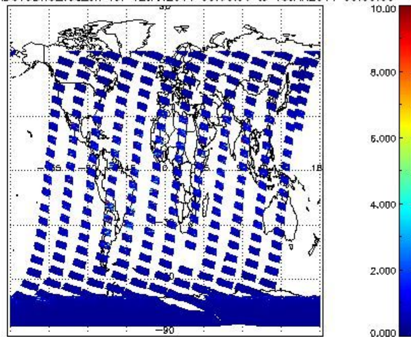
SCIOL2P_NADUV3BRO_vcd_err for 12JAN2011 00:00:00 to 13JAN2011 00:00:00
