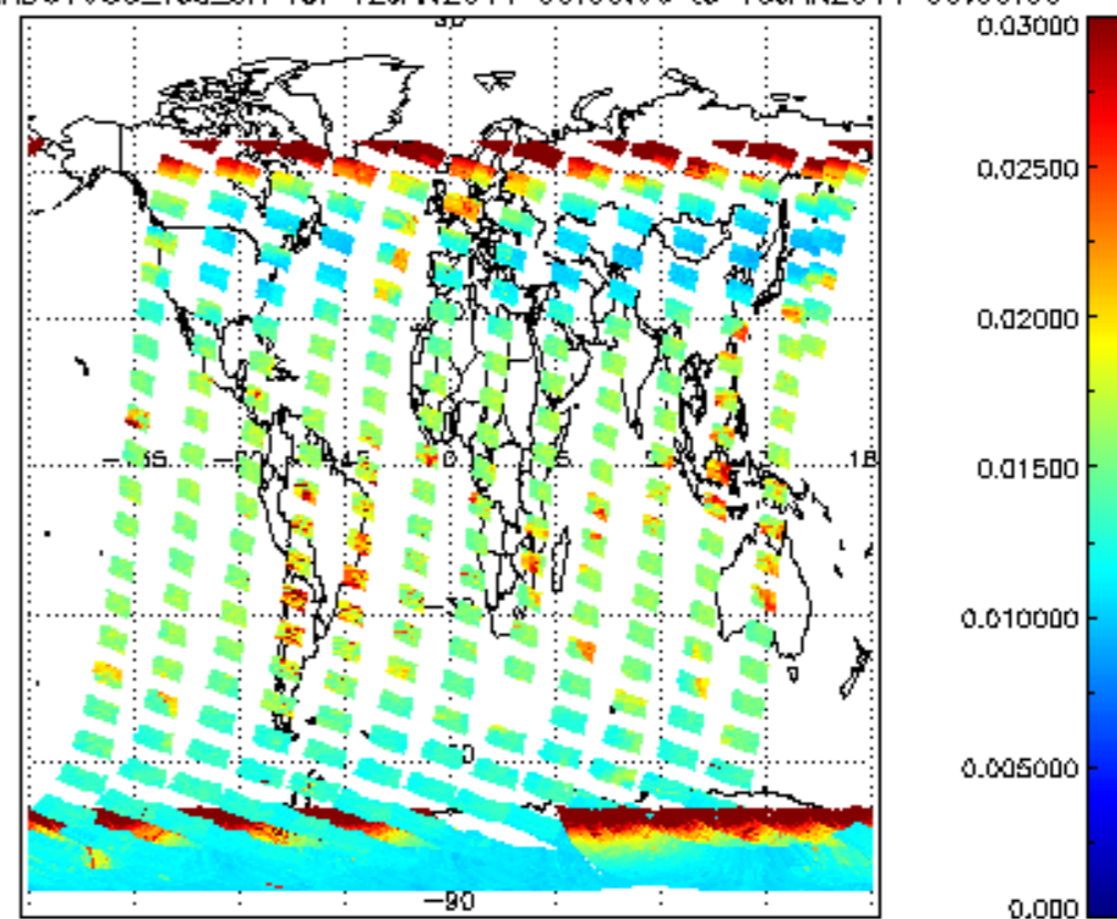
SCIOL2P_NADUV003_vcd_err for 12JAN2011 00:00:00 to 13JAN2011 00:00:00
