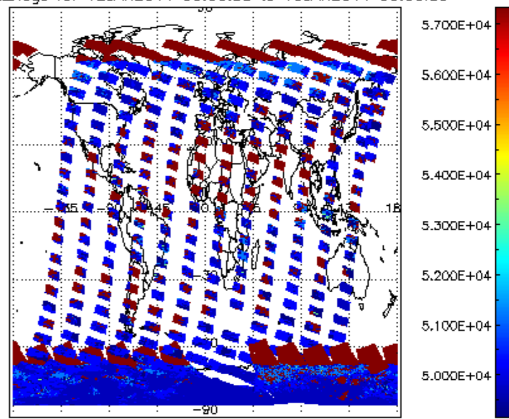
cloud_flags for 12JAN2011 00:00:00 to 13JAN2011 00:00:00
