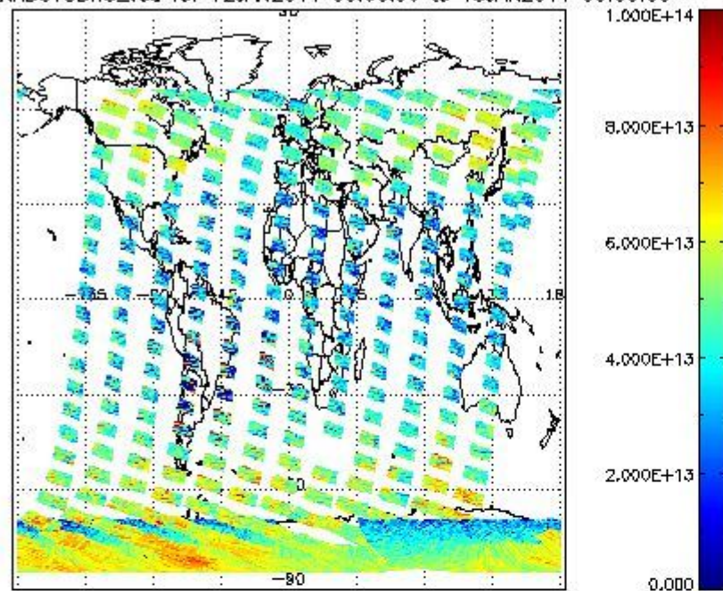
SCIOL2P_NADUV3BRO_vcd for 12JAN2011 00:00:00 to 13JAN2011 00:00:00
