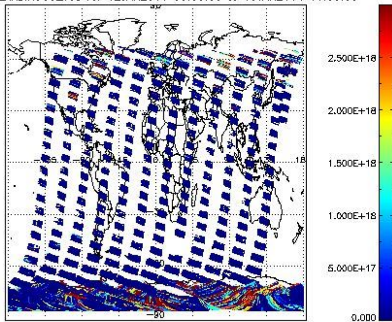
SCIDL2P_NADIR3CO_vcd for 12JAN2011 00:00:00 to 13JAN2011 00:00:00
