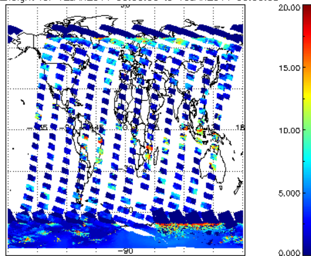
cL_top_height for 12JAN2011 00:00:00 to 13JAN2011 00:00:00
