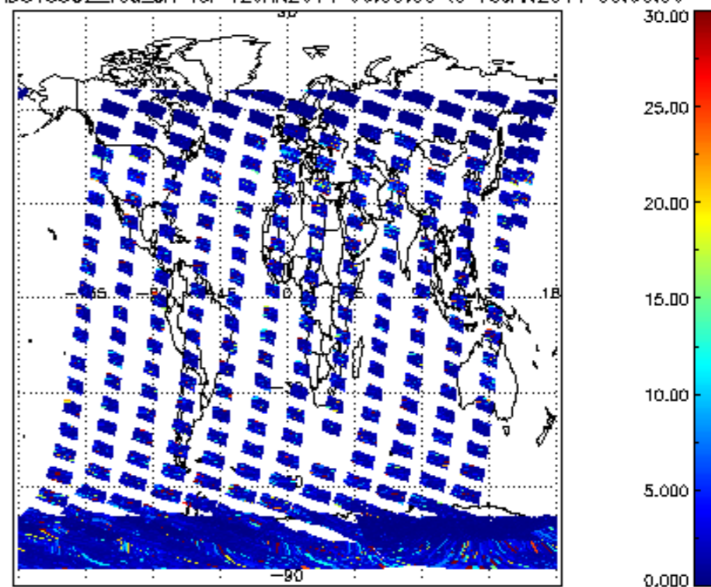
SCIOL2P_NADUV5S02_vcd_err for 12JAN2011 00:00:00 to 13JAN2011 00:00:00
