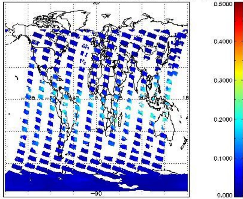
SCIOL2P_NADUV8H20_vcd_err for 12JAN2011 00:00:00 to 13JAN2011 00:00:00
