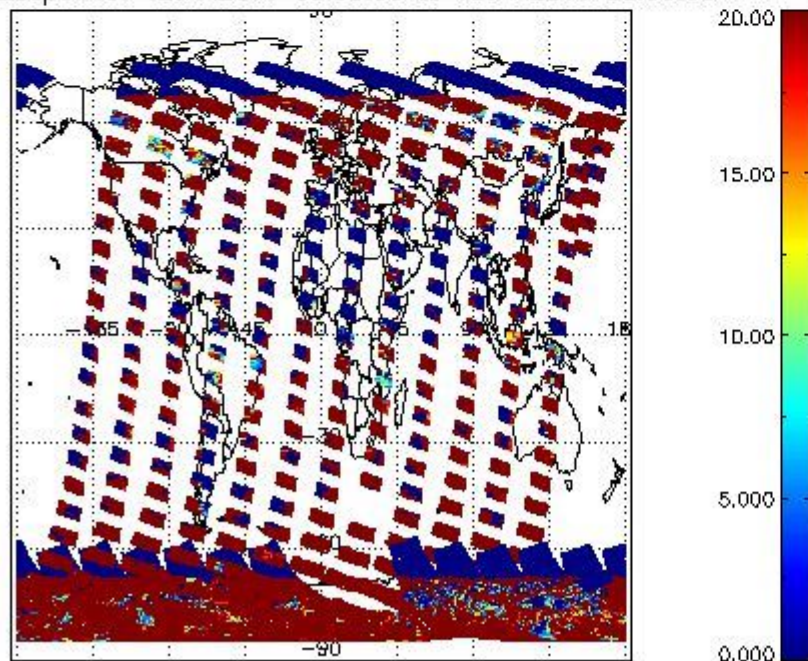
cLopt_depth for 12JAN2011 00:00:00 to 13JAN2011 00:00:00
