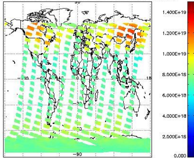
SCIOL2P_NADUV003_vcd for 12JAN2011 00:00:00 to 13JAN2011 00:00:00
