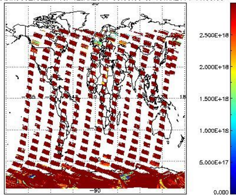
SCIDL2P_NADIR3CO_vcd_err for 12JAN2011 00:00:00 to 13JAN2011 00:00:00
