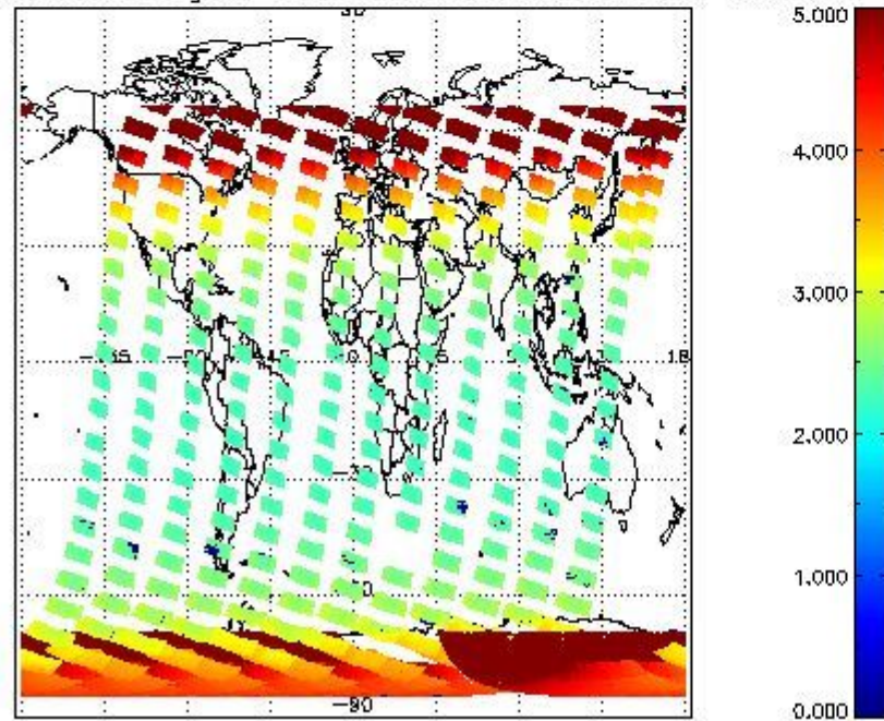
SCIOL2P_NADUV003_amf_gr for 12JAN2011 00:00:00 to 13JAN2011 00:00:00
