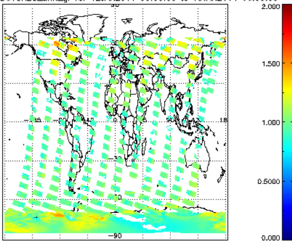
SCIOL2P_NADUVBH20_amf_gr for 12JAN2011 00:00:00 to 13JAN2011 00:00:00
