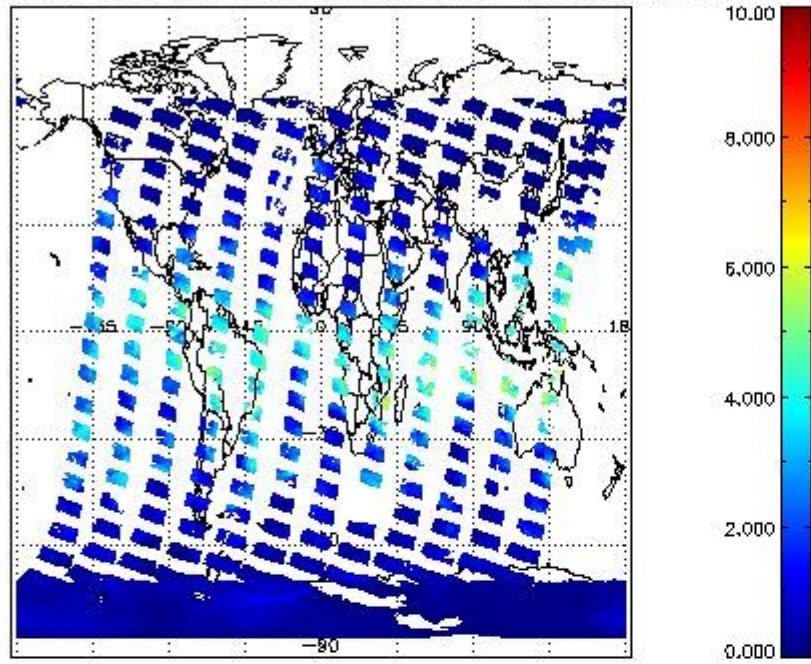
SCIOL2P_NADUV8H20_vcd for 12JAN2011 00:00:00 to 13JAN2011 00:00:00
