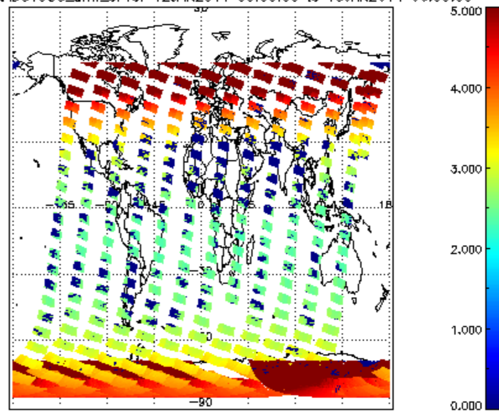
SCIOL2P_NADUV003_amf_cl for 12JAN2011 00:00:00 to 13JAN2011 00:00:00
