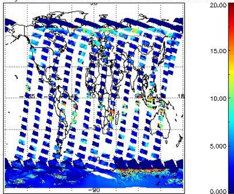
cL_top_height for 12JAN2011 00:00:00 to 13JAN2011 00:00:00
