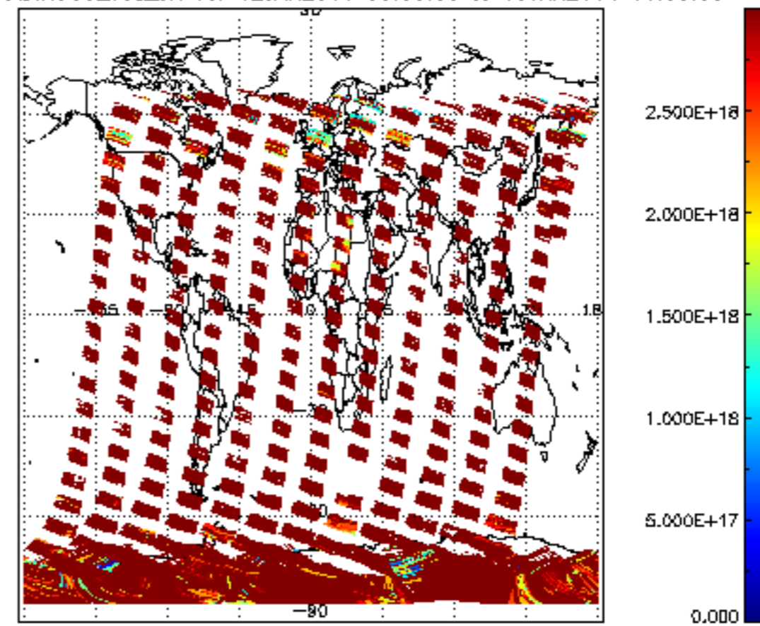
SCIOL2P_NADIR3CO_vcd_err for 12JAN2011 00:00:00 to 13JAN2011 00:00:00
