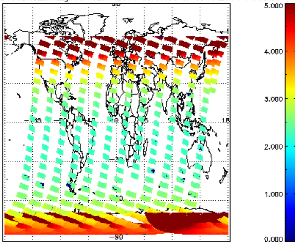
SCIOL2P_NADUV3BRO_amf_gr for 12JAN2011 00:00:00 to 13JAN2011 00:00:00
