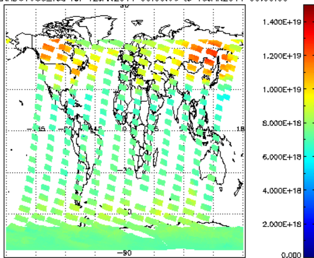
SCIOL2P_NADUV003_vcd for 12JAN2011 00:00:00 to 13JAN2011 00:00:00
