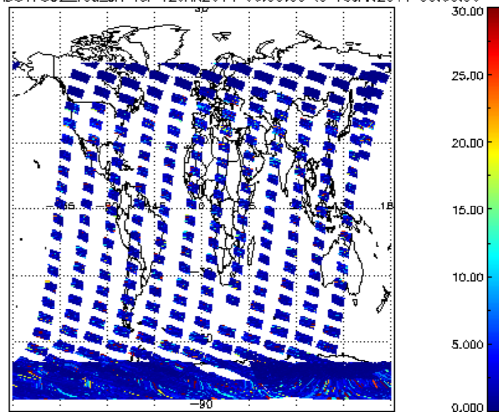
SCIOL2P_NADUV7S02_vcd_err for 12JAN2011 00:00:00 to 13JAN2011 00:00:00
