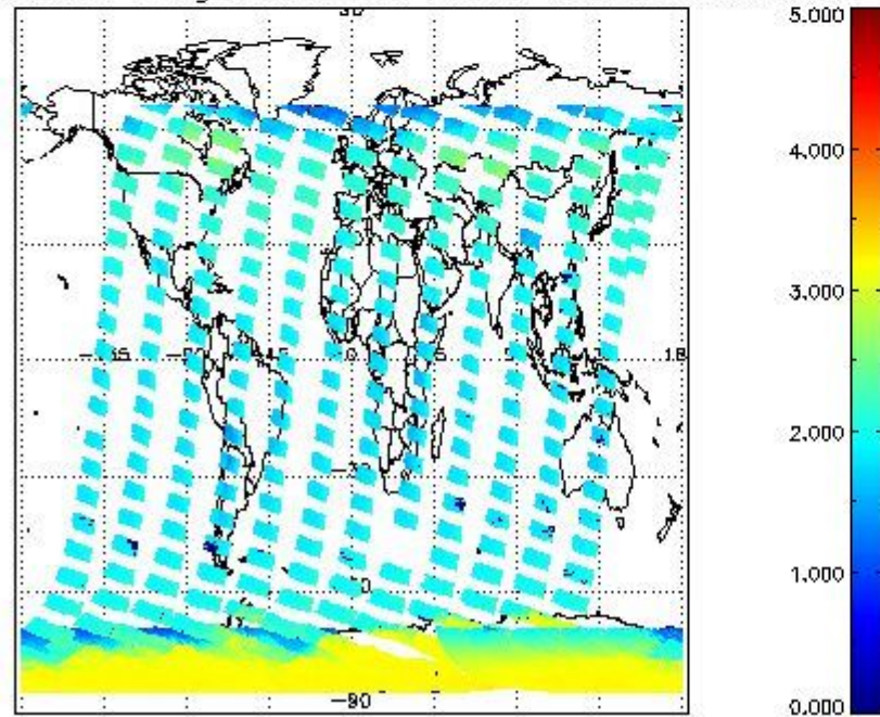
SCIOL2P_NADUV7S02_amf_gr for 12JAN2011 00:00:00 to 13JAN2011 00:00:00
