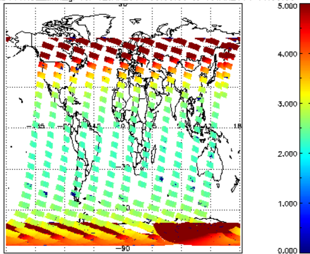
SCIOL2P_NADUV1NO2_amf_gr for 12JAN2011 00:00:00 to 13JAN2011 00:00:00
