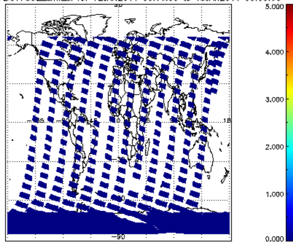
SCIOL2P_NADUV7S02_amf_sl for 12JAN2011 00:00:00 to 13JAN2011 00:00:00
