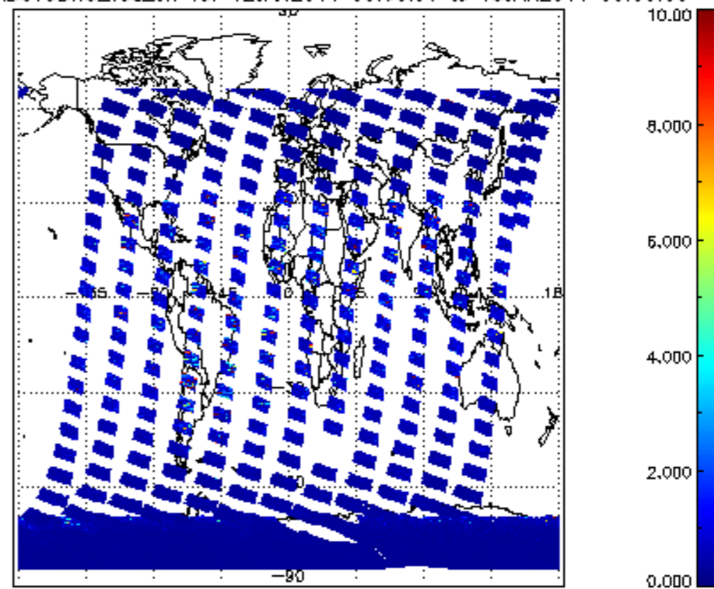
SCIOL2P_NADUV3BRO_vcd_err for 12JAN2011 00:00:00 to 13JAN2011 00:00:00
