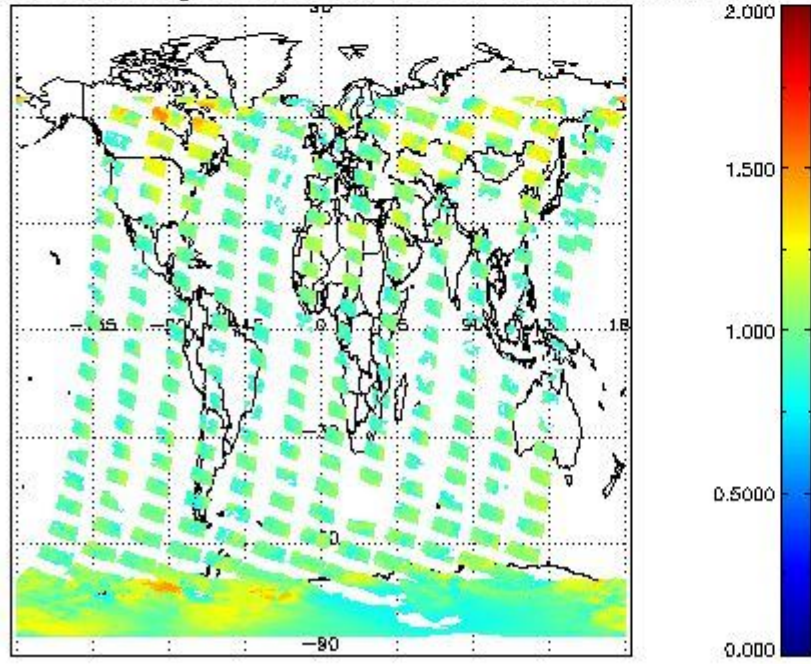
SCIOL2P_NADUV8H20_amf_gr for 12JAN2011 00:00:00 to 13JAN2011 00:00:00
