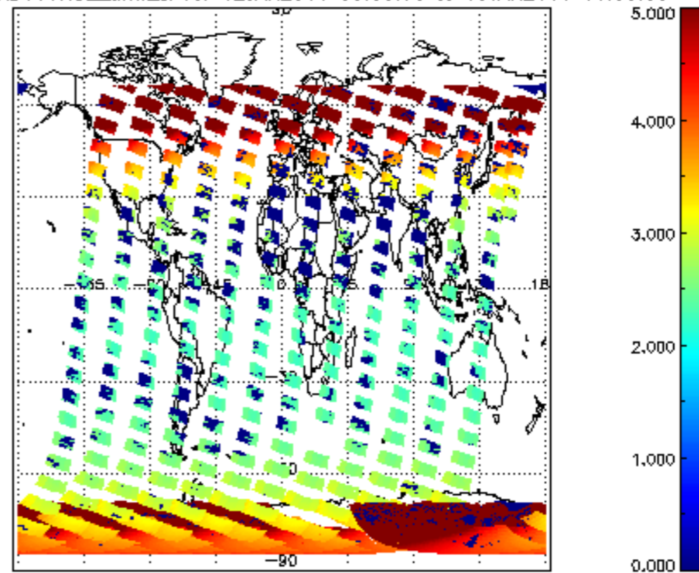
SCIOL2P_NADUV1NO2_amf_cl for 12JAN2011 00:00:00 to 13JAN2011 00:00:00
