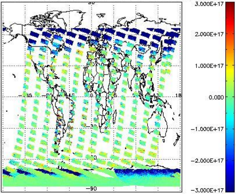
SCIOL2P_NADUV5SO2_vcd for 12JAN2011 00:00:00 to 13JAN2011 00:00:00
