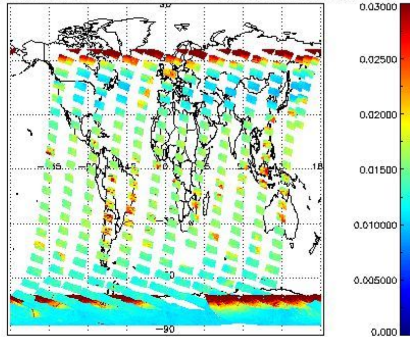
SCIOL2P_NADUV003_vcd_err for 12JAN2011 00:00:00 to 13JAN2011 00:00:00
