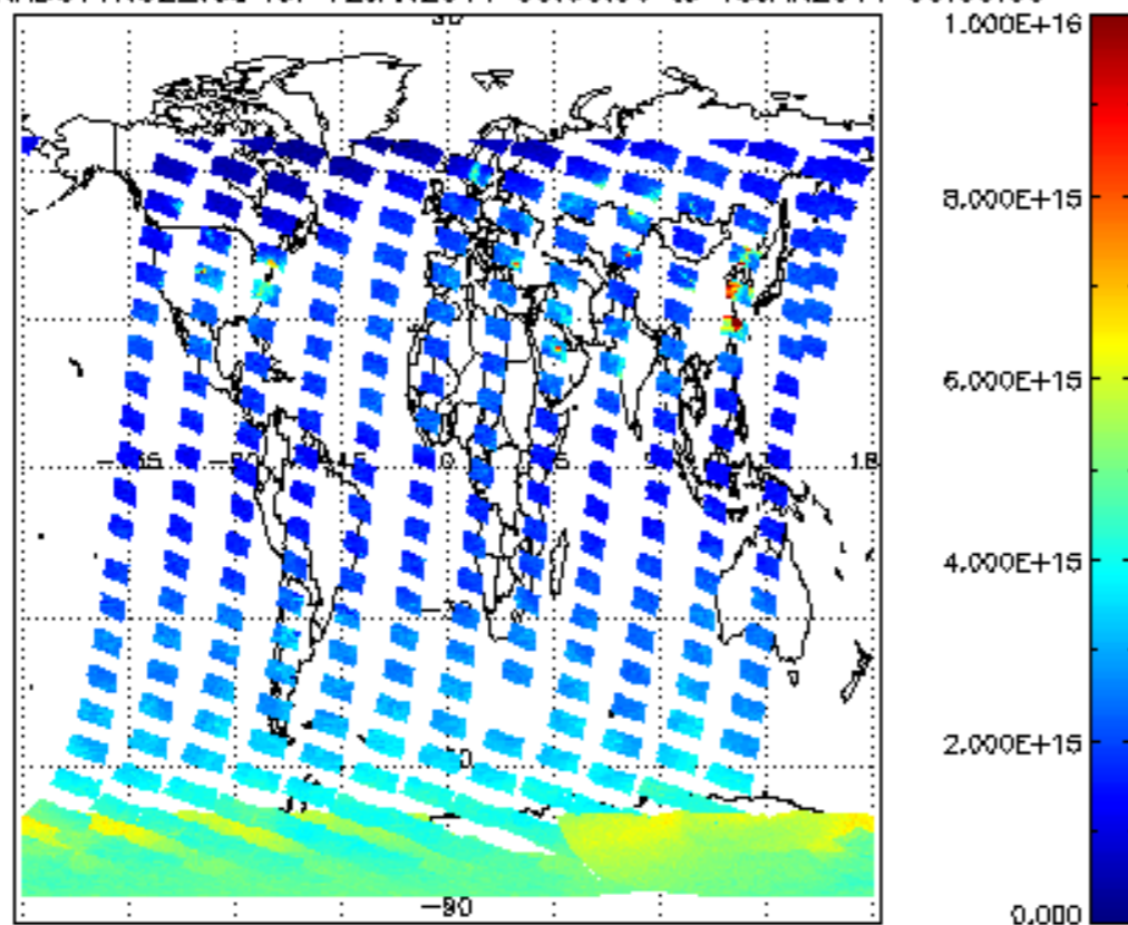
SCIOL2P_NADUV1NO2_vcd for 12JAN2011 00:00:00 to 13JAN2011 00:00:00
