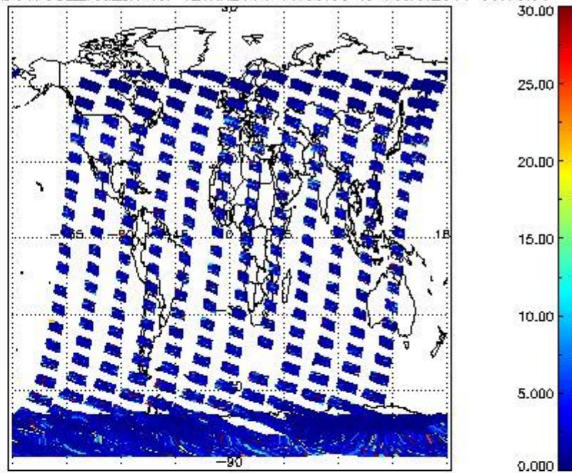
SCIOL2P_NADUV7S02_vcd_err for 12JAN2011 00:00:00 to 13JAN2011 00:00:00
