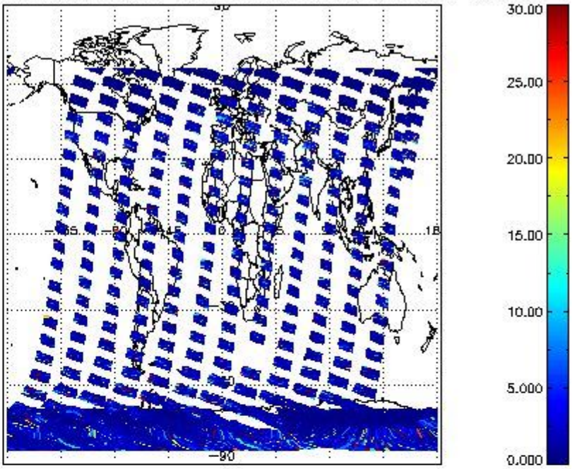
SCIOL2P_NADUV5SO2_vcd_err for 12JAN2011 00:00:00 to 13JAN2011 00:00:00
