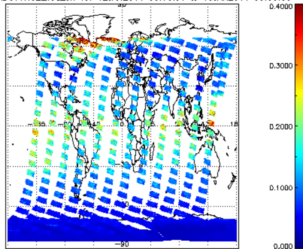
SCIOL2P_NADUV1NO2_vcd_err for 12JAN2011 00:00:00 to 13JAN2011 00:00:00
