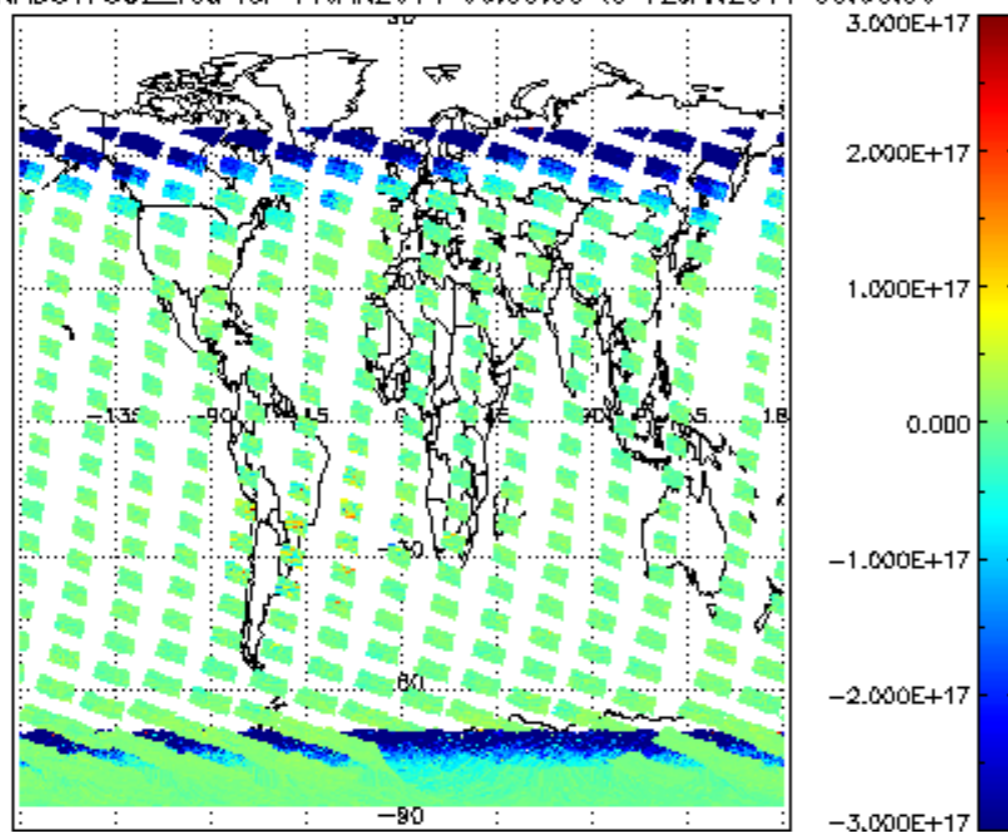
SCIOL2P_NADUV7S02_vcd for 11JAN2011 00:00:00 to 12JAN2011 00:00:00
