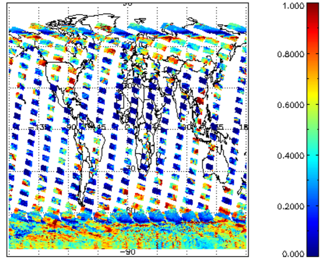
cL_frac for 11JAN2011 00:00:00 to 12JAN2011 00:00:00
