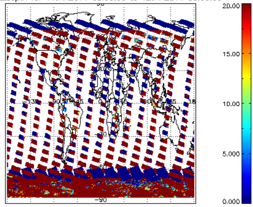
cLopt_depth for 11JAN2011 00:00:00 to 12JAN2011 00:00:00
