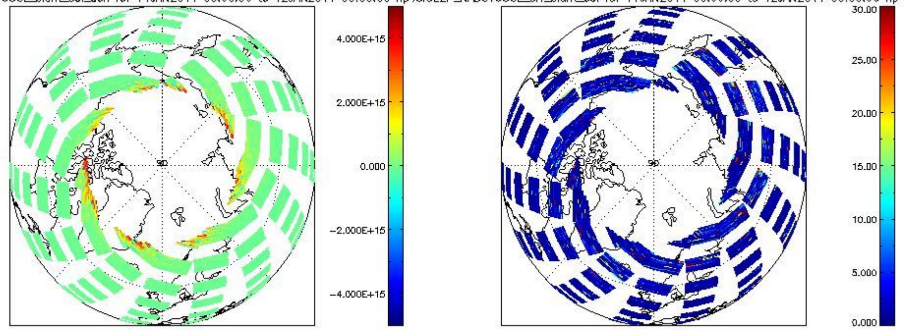
SCIOI2P_NADUV6OCL_slant_col_den for 11JAN2011 00:00:00 to 12JAN2011 00:00:00 np; SCIOI2P_NADUV6OCL_err_slant_col for 11JAN2011 00:00:00 to 12JAN2011 00:00:00 np
