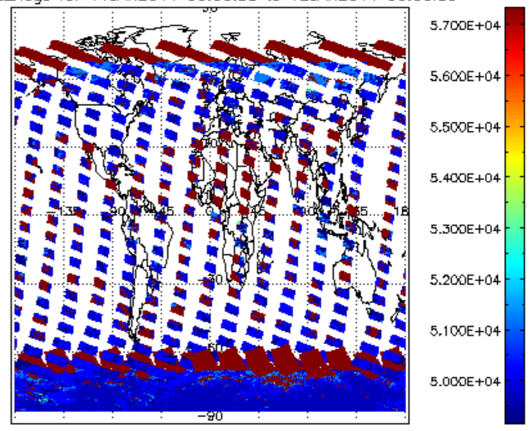
cloud_flags for 11JAN2011 00:00:00 to 12JAN2011 00:00:00
