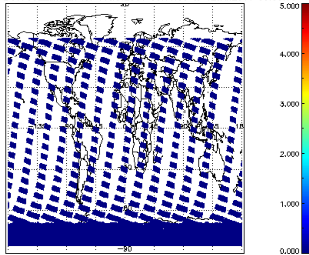
SCIOL2P_NADUV7S02_amf_cl for 11JAN2011 00:00:00 to 12JAN2011 00:00:00
