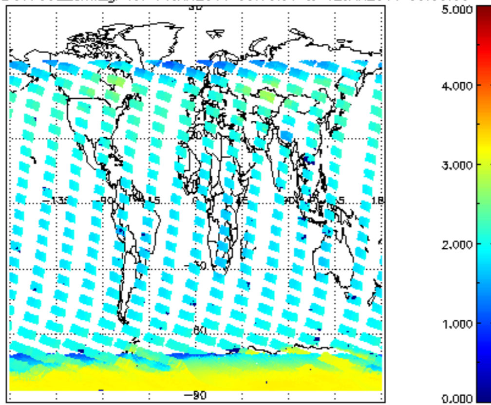
SCIOL2P_NADUV7S02_amf_gr for 11JAN2011 00:00:00 to 12JAN2011 00:00:00
