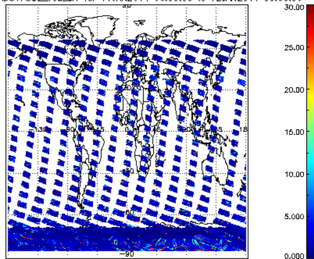
SCIOL2P_NADUV7S02_vcd_err for 11JAN2011 00:00:00 to 12JAN2011 00:00:00
