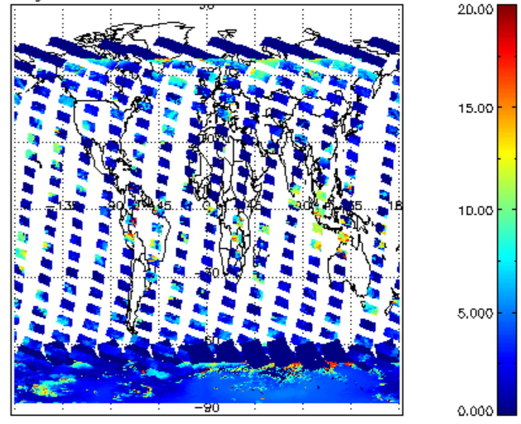
cL_top_height for 11JAN2011 00:00:00 to 12JAN2011 00:00:00
