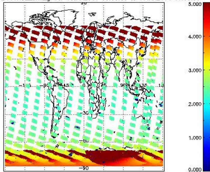
SCIOL2P_NADUV1NO2_amf_gr for 10JAN2011 00:00:00 to 11JAN2011 00:00:00
