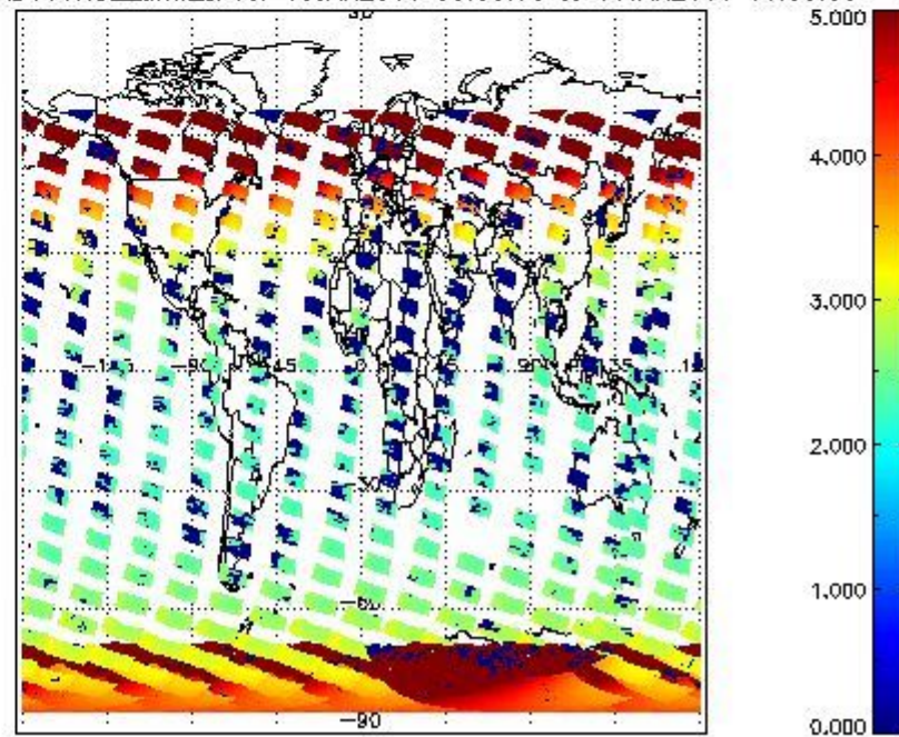
SCIOL2P_NADUV1NO2_amf_cl for 10JAN2011 00:00:00 to 11JAN2011 00:00:00
