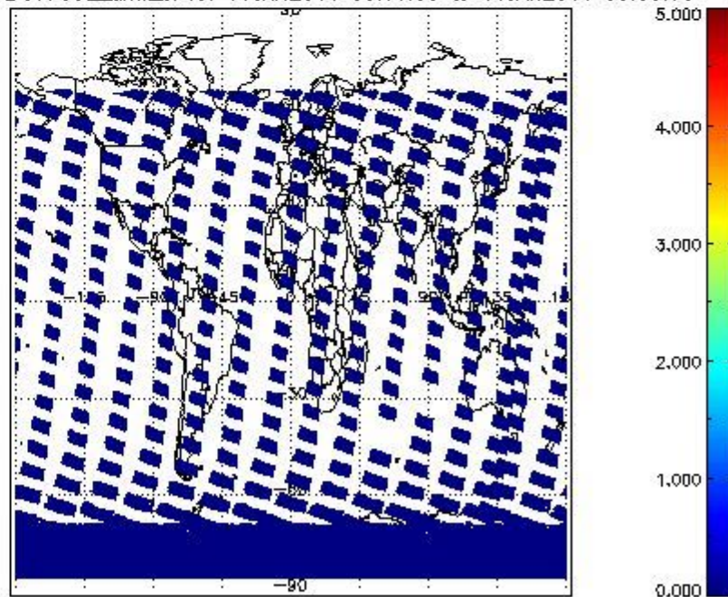
SCIOL2P_NADUV7S02_amf_cl for 10JAN2011 00:00:00 to 11JAN2011 00:00:00
