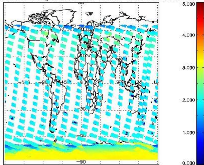
SCIOL2P_NADUV7S02_amf_gr for 10JAN2011 00:00:00 to 11JAN2011 00:00:00
