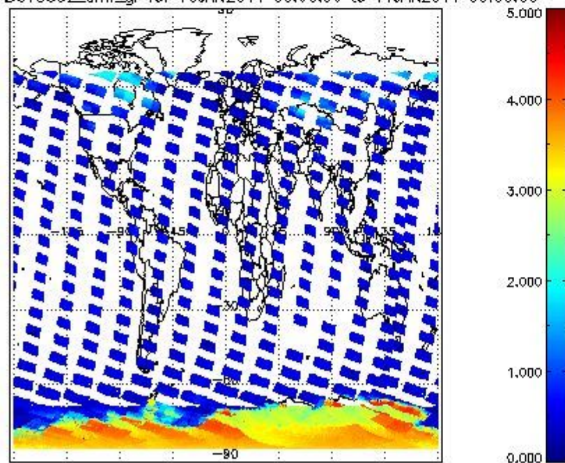
SCIOL2P_NADUV5SO2_amf_gr for 10JAN2011 00:00:00 to 11JAN2011 00:00:00
