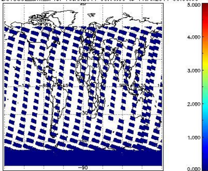
SCIOL2P_NADUV5SO2_amf_cl for 10JAN2011 00:00:00 to 11JAN2011 00:00:00
