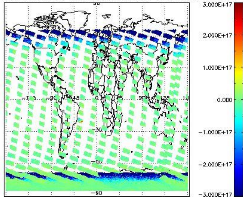
SCIOL2P_NADUV7S02_vcd for 10JAN2011 00:00:00 to 11JAN2011 00:00:00
