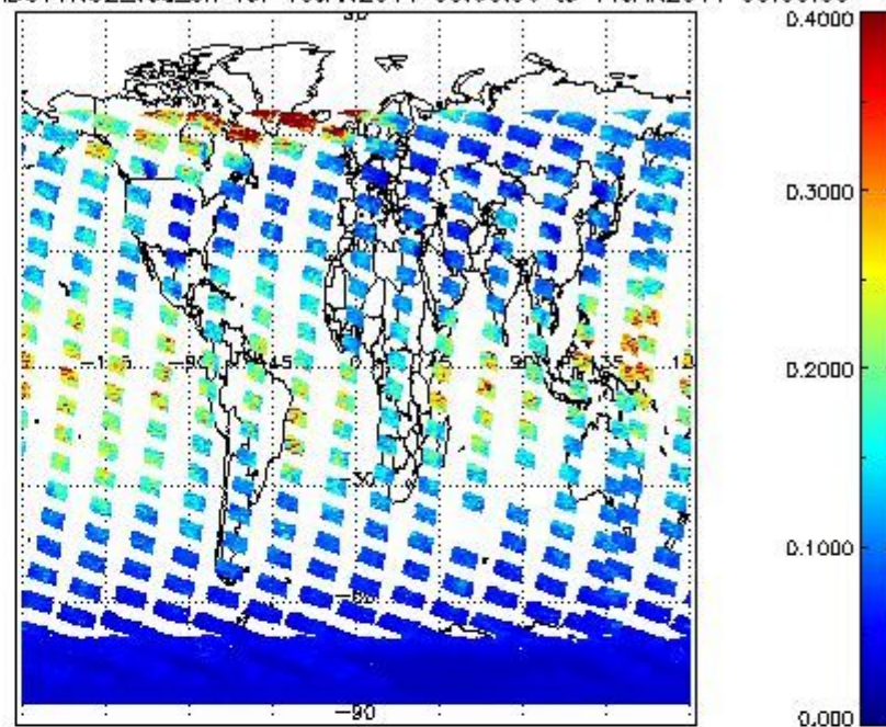
SCIOL2P_NADUV1NO2_vcd_err for 10JAN2011 00:00:00 to 11JAN2011 00:00:00
