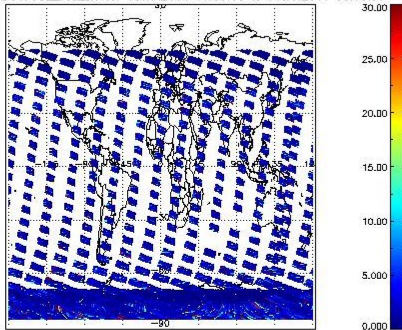
SCIOL2P_NADUV7S02_vcd_err for 10JAN2011 00:00:00 to 11JAN2011 00:00:00
