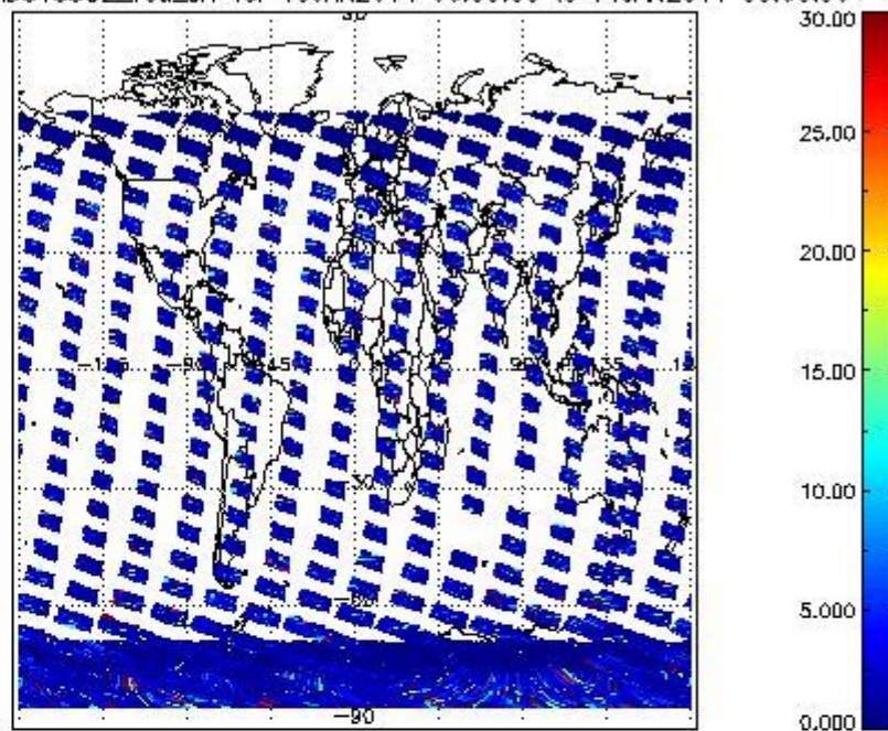
SCIOL2P_NADUV5SO2_vcd_err for 10JAN2011 00:00:00 to 11JAN2011 00:00:00
