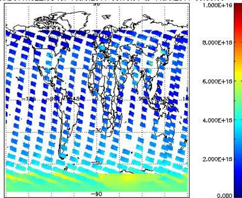
SCIOL2P_NADUV1NO2_vcd for 10JAN2011 00:00:00 to 11JAN2011 00:00:00
