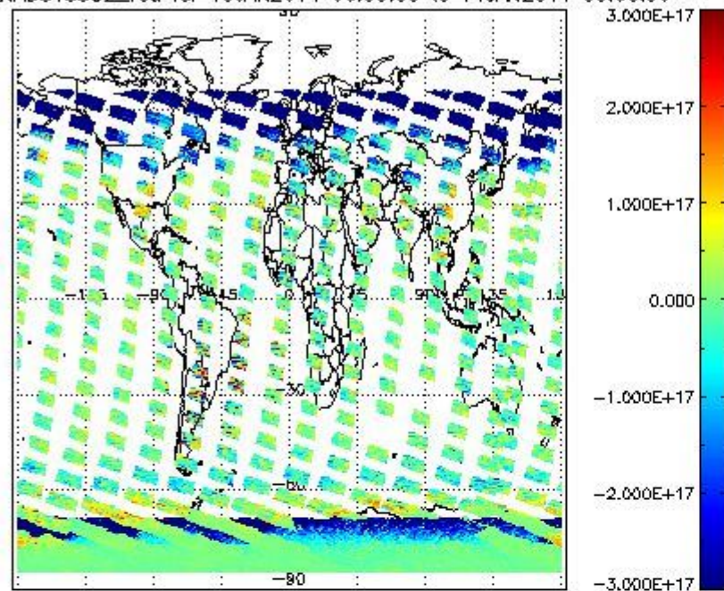
SCIOL2P_NADUV5SO2_vcd for 10JAN2011 00:00:00 to 11JAN2011 00:00:00
