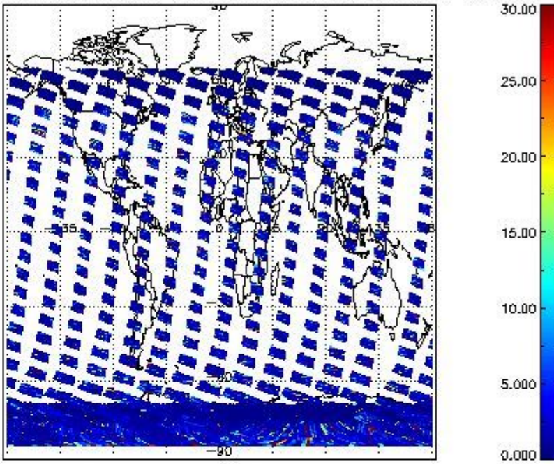
SCIOL2P_NADUV5SO2_vcd_err for 09JAN2011 00:00:00 to 10JAN2011 00:00:00
