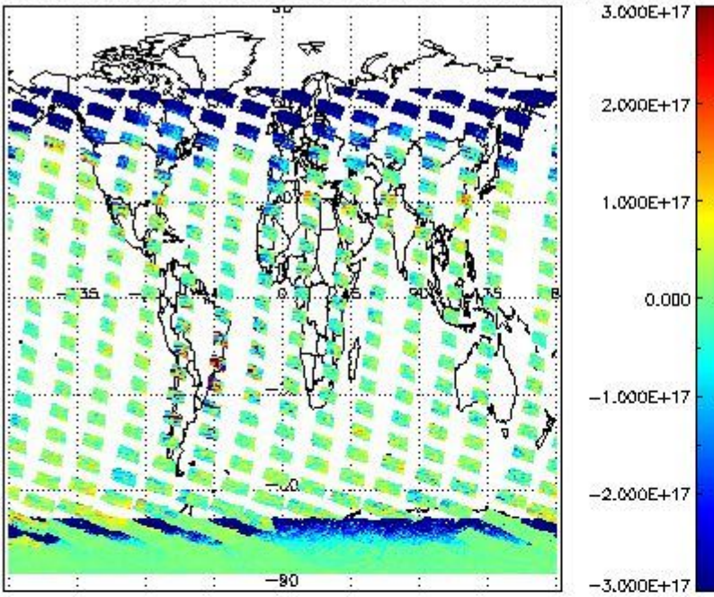
SCIOL2P_NADUV5SO2_vcd for 09JAN2011 00:00:00 to 10JAN2011 00:00:00
