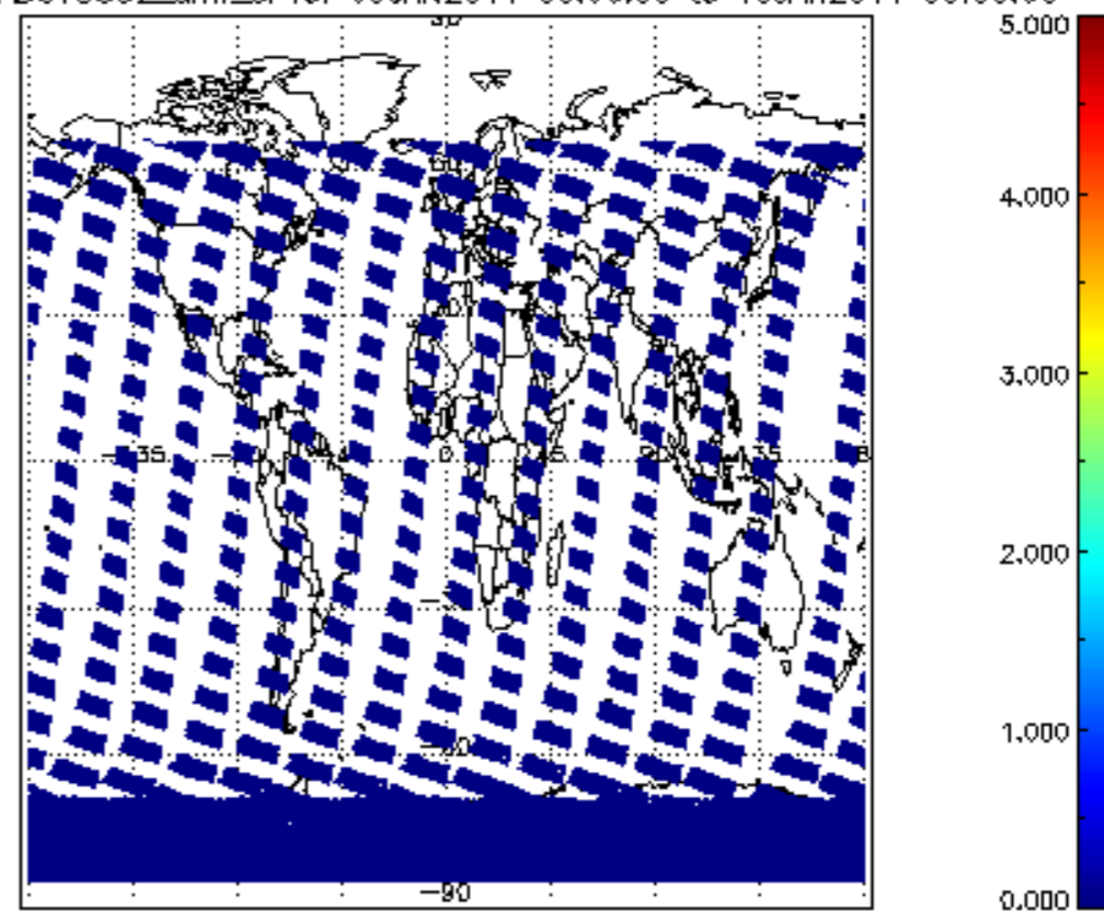
SCIOL2P_NADUV5S02_amf_sl for 09JAN2011 00:00:00 to 10JAN2011 00:00:00
