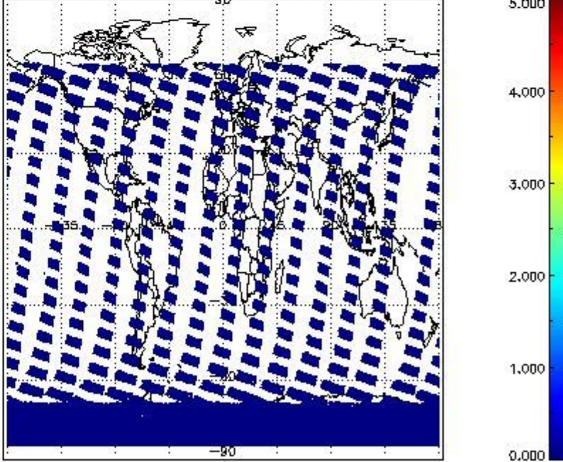
SCIOL2P_NADUV5SO2_amf_cl for 09JAN2011 00:00:00 to 10JAN2011 00:00:00
