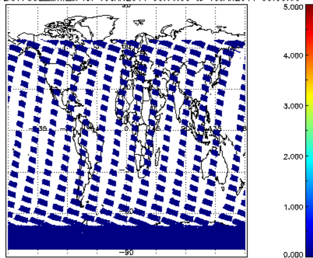
SCIOL2P_NADUV7S02_amf_cl for 09JAN2011 00:00:00 to 10JAN2011 00:00:00
