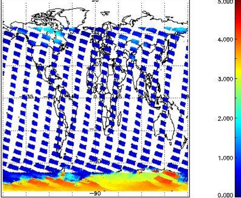
SCIOL2P_NADUV5SO2_amf_gr for 09JAN2011 00:00:00 to 10JAN2011 00:00:00
