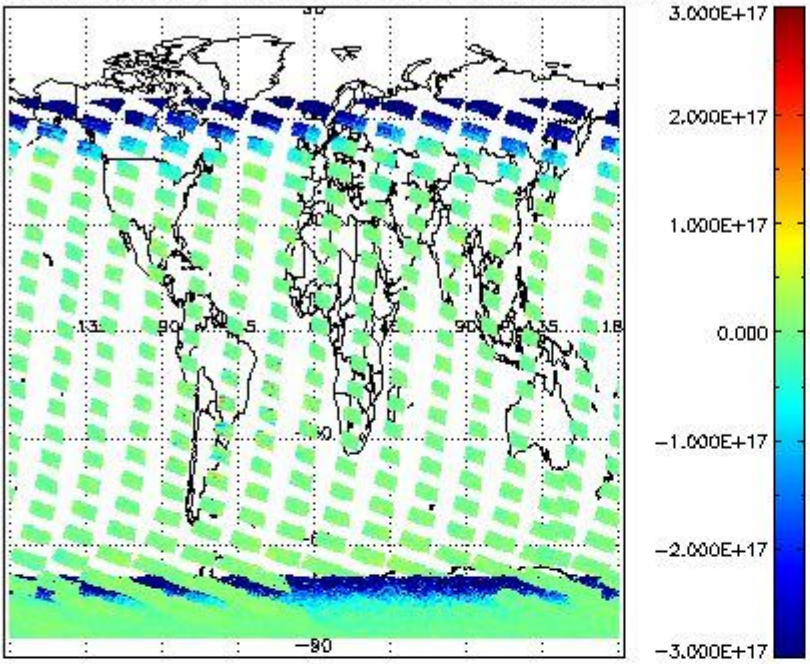
SCIOL2P_NADUV7S02_vcd for 08JAN2011 00:00:00 to 09JAN2011 00:00:00
