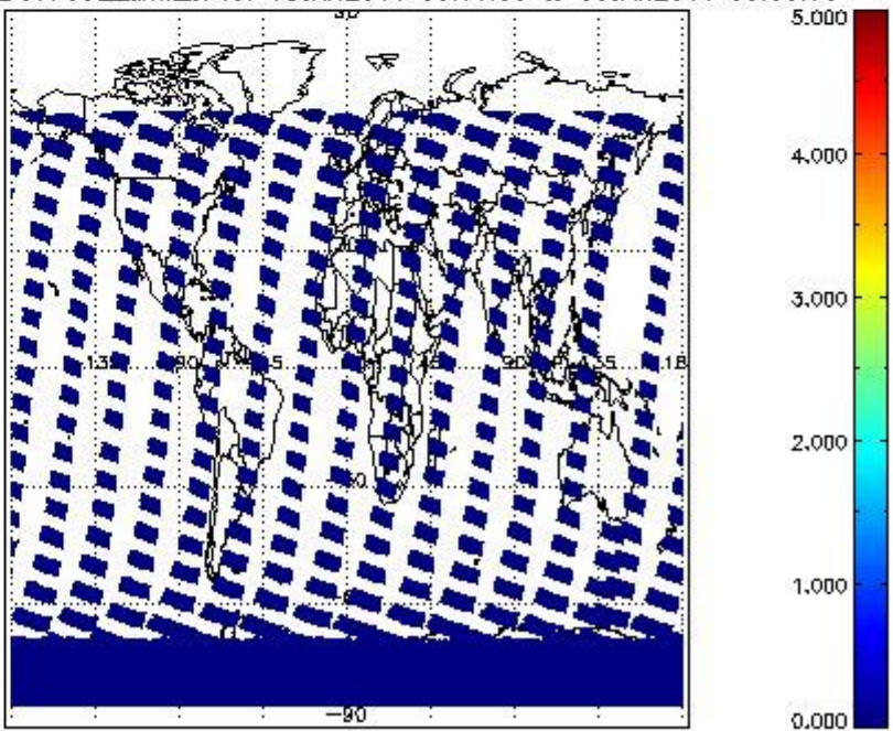
SCIOL2P_NADUV7S02_amf_cl for 08JAN2011 00:00:00 to 09JAN2011 00:00:00
