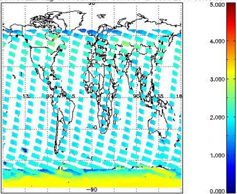
SCIOL2P_NADUV7S02_amf_gr for 08JAN2011 00:00:00 to 09JAN2011 00:00:00
