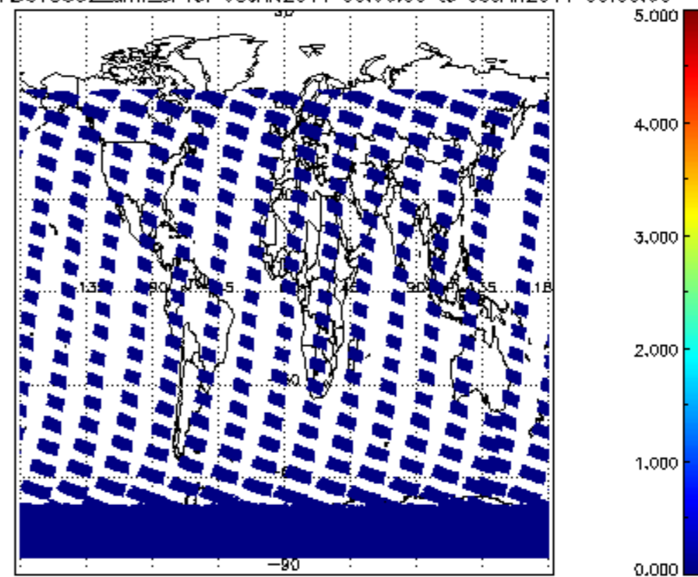
SCIOL2P_NADUV5S02_amf_sl for 08JAN2011 00:00:00 to 09JAN2011 00:00:00
