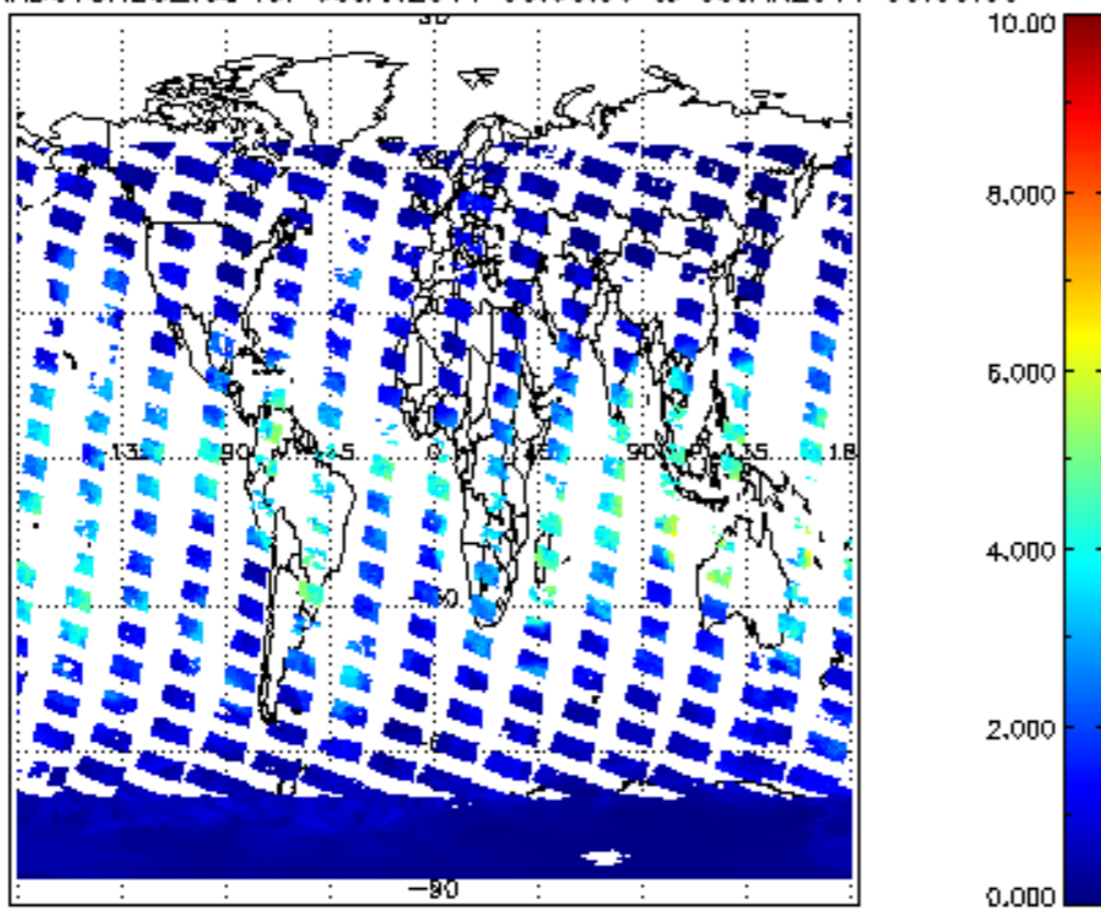
SCIOL2P_NADUV8H20_vcd for 08JAN2011 00:00:00 to 09JAN2011 00:00:00
