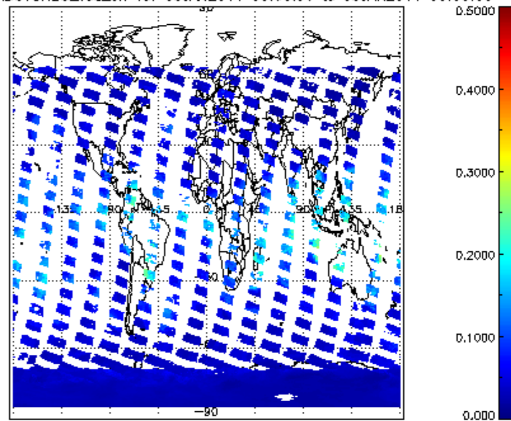
SCIOL2P_NADUV8H20_vcd_err for 08JAN2011 00:00:00 to 09JAN2011 00:00:00
