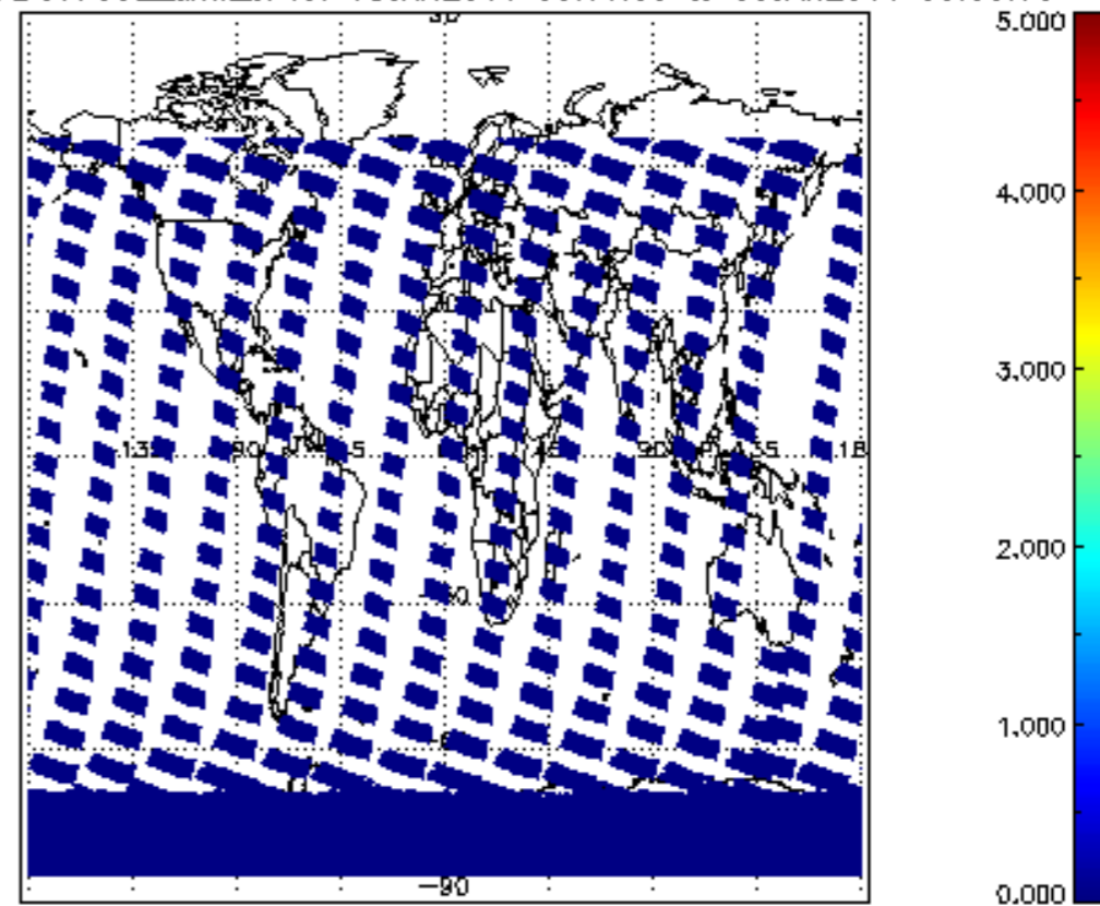
SCIOL2P_NADUV7S02_amf_sl for 08JAN2011 00:00:00 to 09JAN2011 00:00:00
