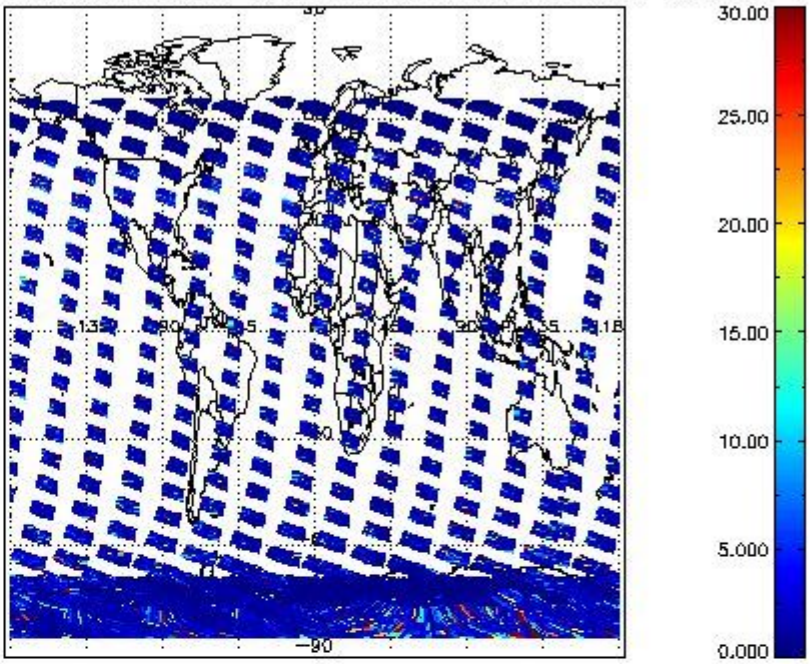
SCIOL2P_NADUV7S02_vcd_err for 08JAN2011 00:00:00 to 09JAN2011 00:00:00
