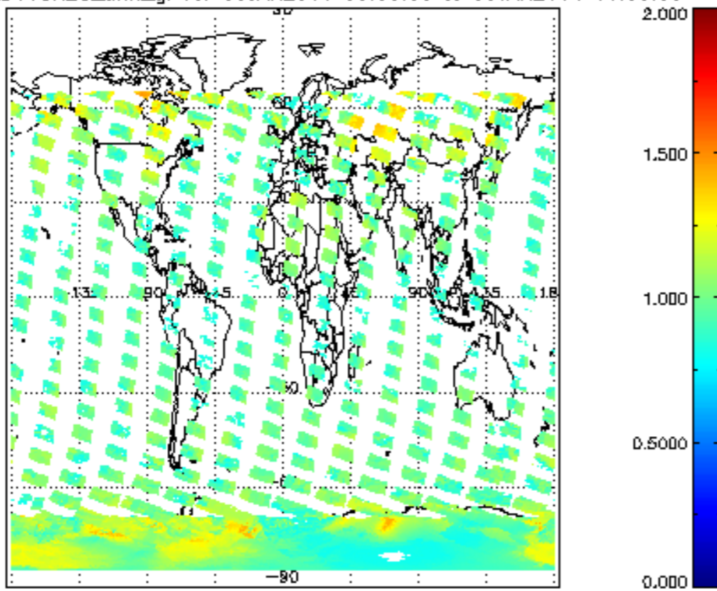
SCIOL2P_NADUV8H20_amf_gr for 08JAN2011 00:00:00 to 09JAN2011 00:00:00
