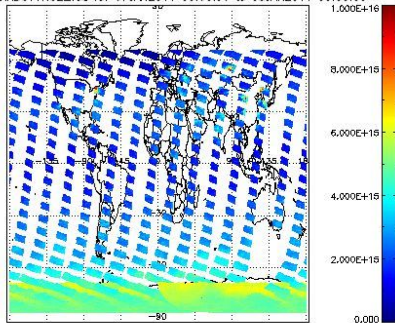
SCIOL2P_NADUV1N02_vcd for 07JAN2011 00:00:00 to 08JAN2011 00:00:00
