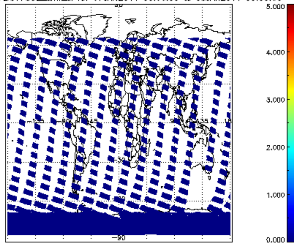
SCIOL2P_NADUV7S02_amf_sl for 07JAN2011 00:00:00 to 08JAN2011 00:00:00
