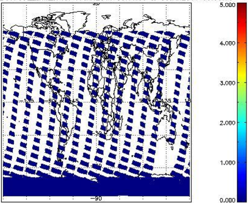
SCIOL2P_NADUV7S02_amf_cl for 07JAN2011 00:00:00 to 08JAN2011 00:00:00
