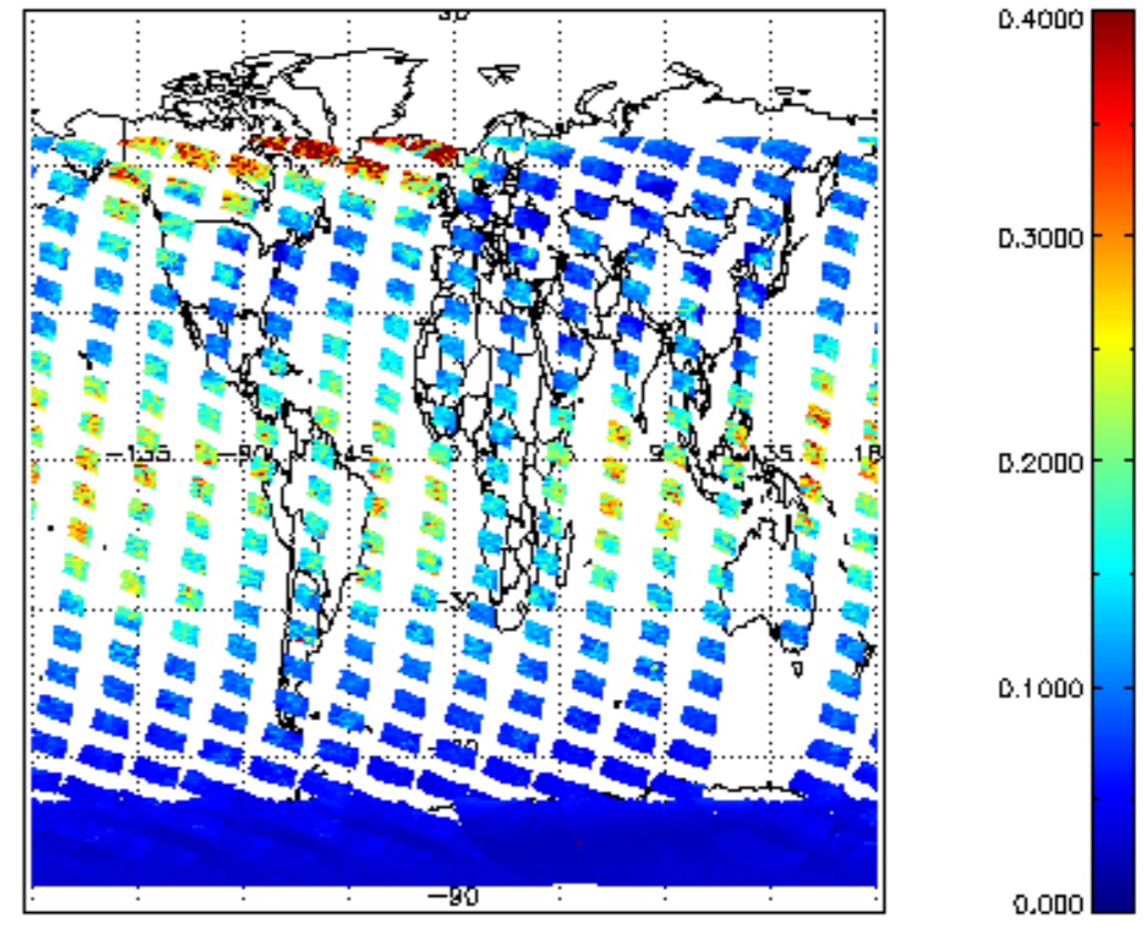
SCIOL2P_NADUV1NO2_vcd_err for 07JAN2011 00:00:00 to 08JAN2011 00:00:00
