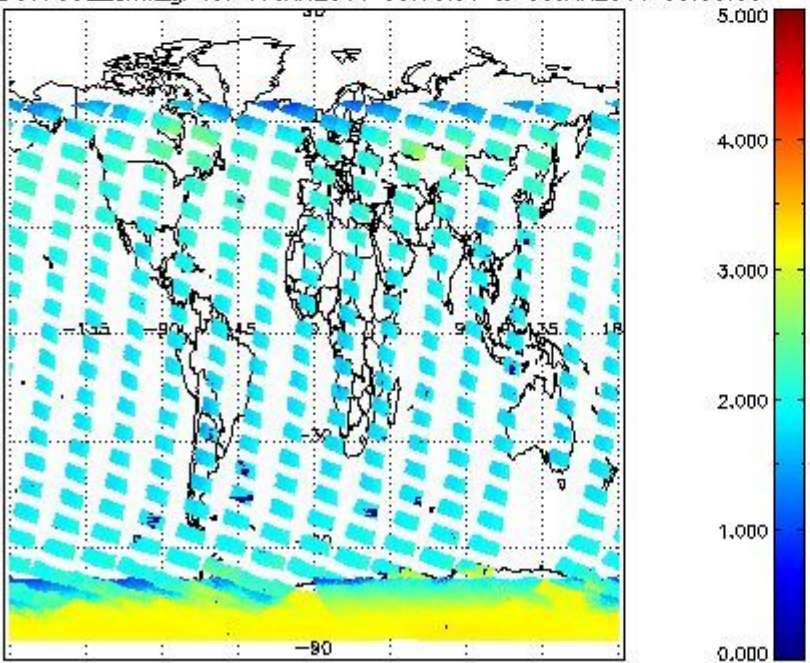
SCIOL2P_NADUV7S02_amf_gr for 07JAN2011 00:00:00 to 08JAN2011 00:00:00
