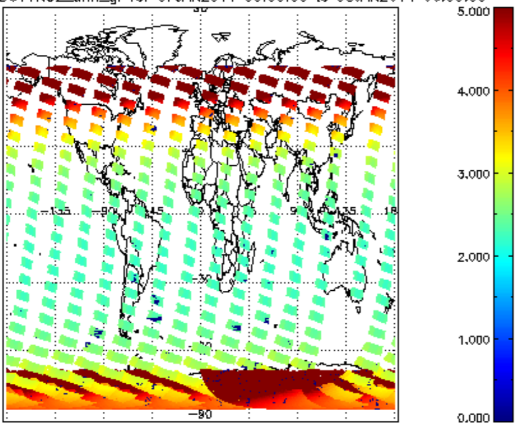
SCIOL2P_NADUV1NO2_amf_gr for 07JAN2011 00:00:00 to 08JAN2011 00:00:00
