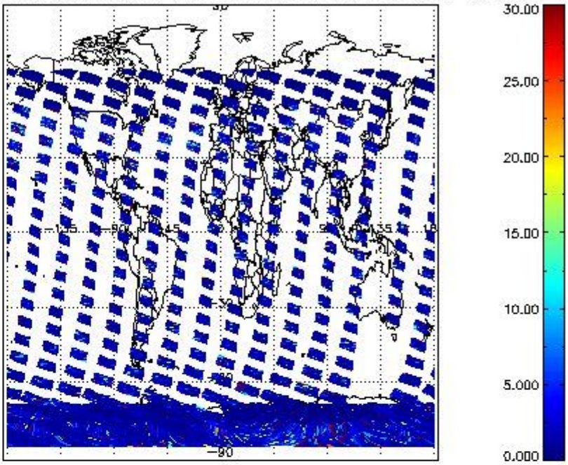
SCIOL2P_NADUV7S02_vcd_err for 07JAN2011 00:00:00 to 08JAN2011 00:00:00
