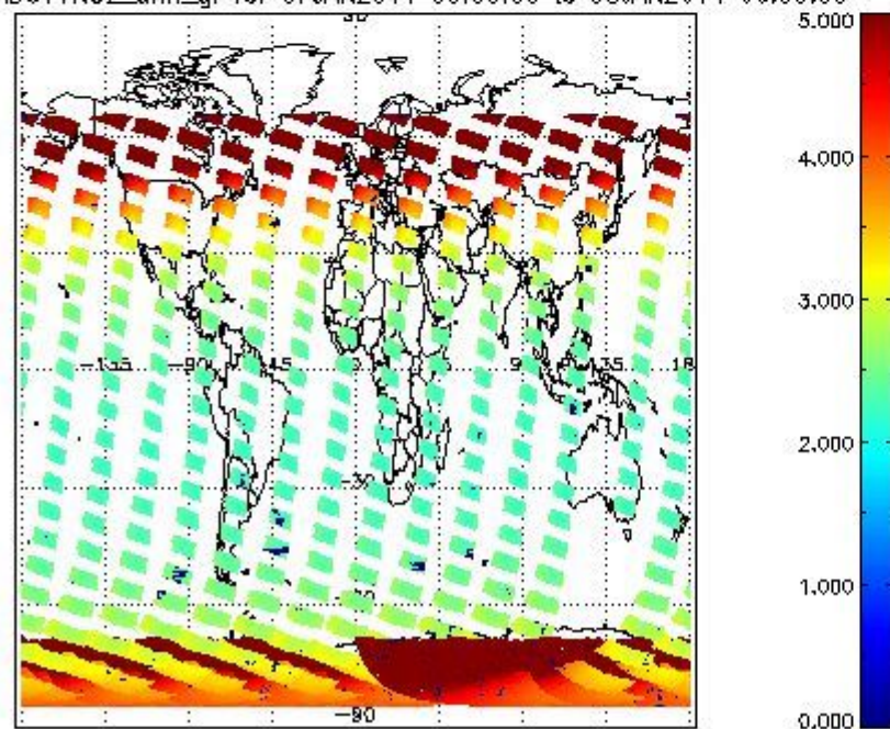
SCIOL2P_NADUV1N02_amf_gr for 07JAN2011 00:00:00 to 08JAN2011 00:00:00
