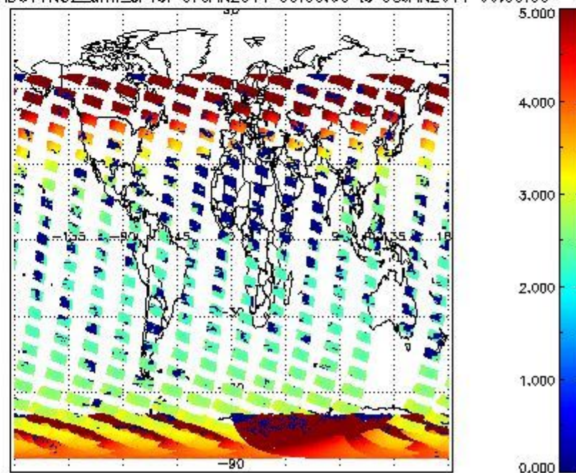
SCIOL2P_NADUV1N02_amf_cl for 07JAN2011 00:00:00 to 08JAN2011 00:00:00
