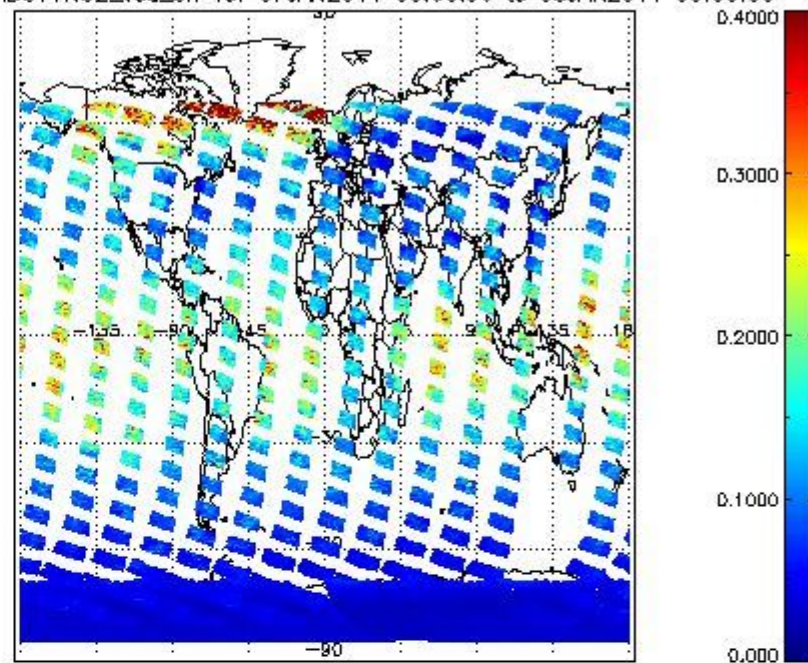
SCIOL2P_NADUV1N02_vcd_err for 07JAN2011 00:00:00 to 08JAN2011 00:00:00
