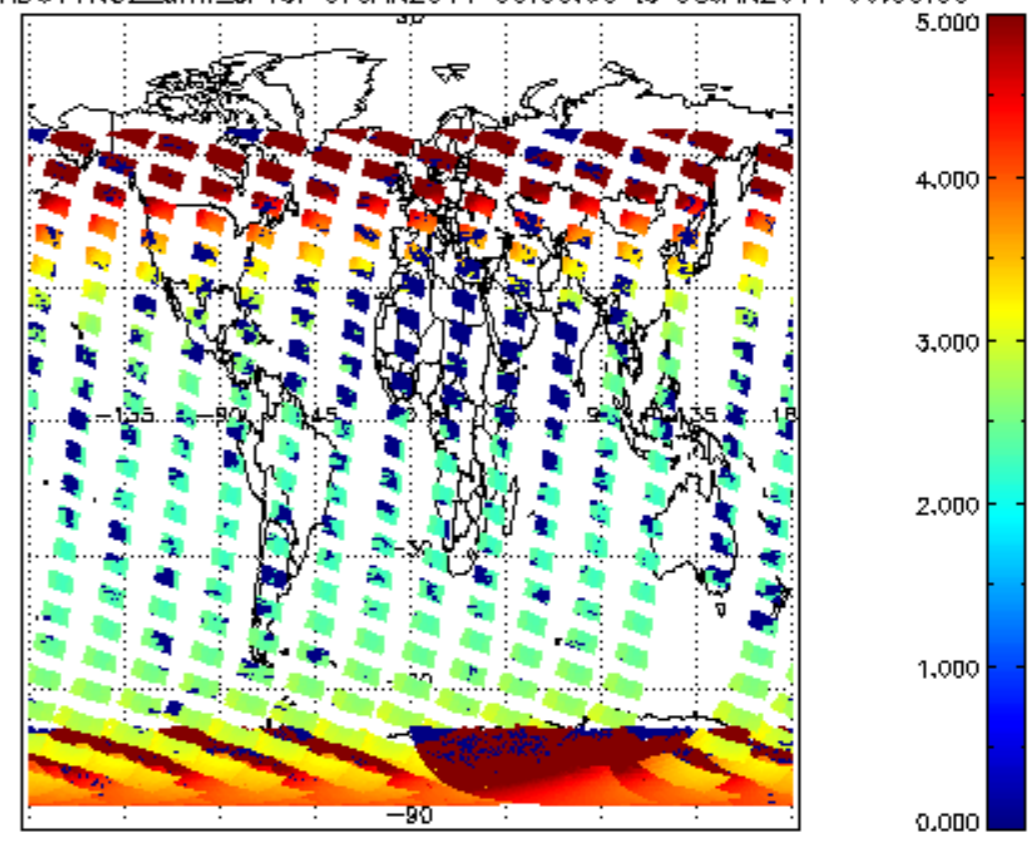
SCIOL2P_NADUV1NO2_amf_cl for 07JAN2011 00:00:00 to 08JAN2011 00:00:00
