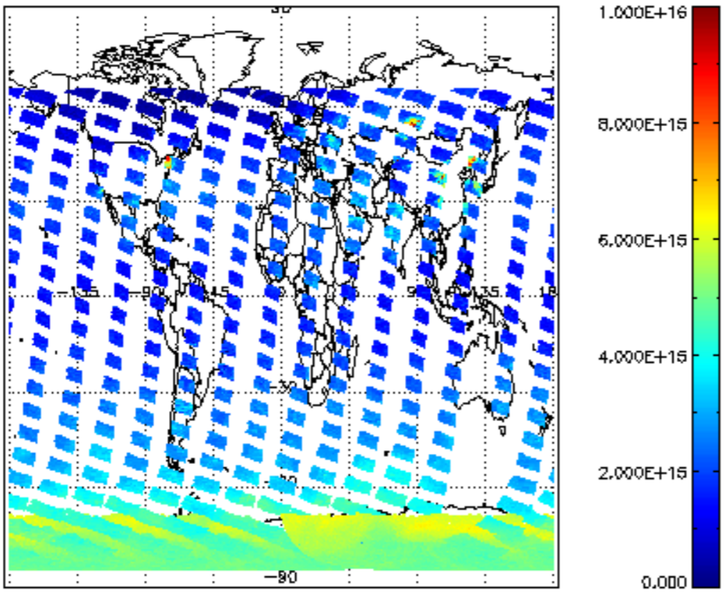
SCIOL2P_NADUV1NO2_vcd for 07JAN2011 00:00:00 to 08JAN2011 00:00:00
