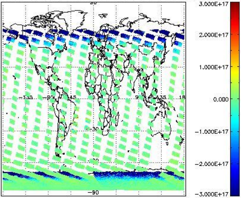
SCIOL2P_NADUV7S02_vcd for 07JAN2011 00:00:00 to 08JAN2011 00:00:00
