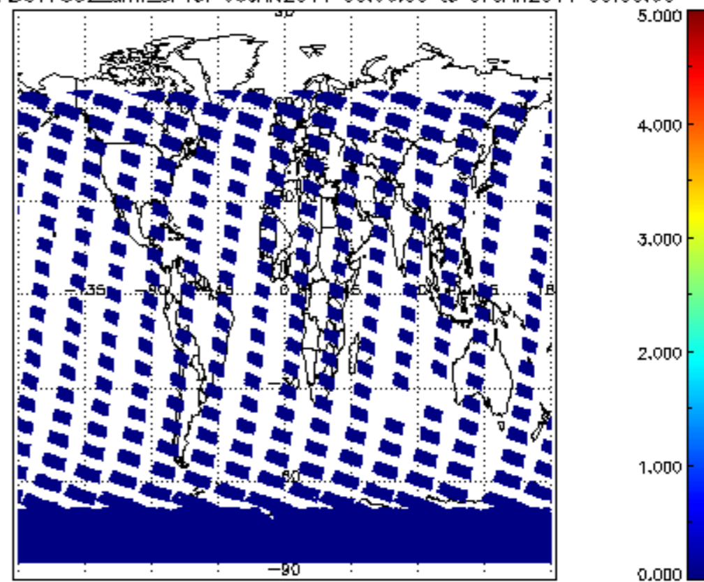
SCIOL2P_NADUV7S02_amf_sl for 06JAN2011 00:00:00 to 07JAN2011 00:00:00
