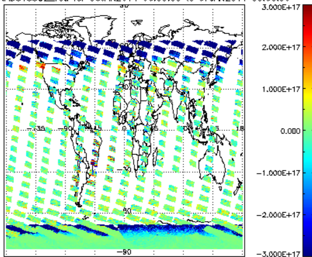
SCIOL2P_NADUV5SO2_vcd for 06JAN2011 00:00:00 to 07JAN2011 00:00:00
