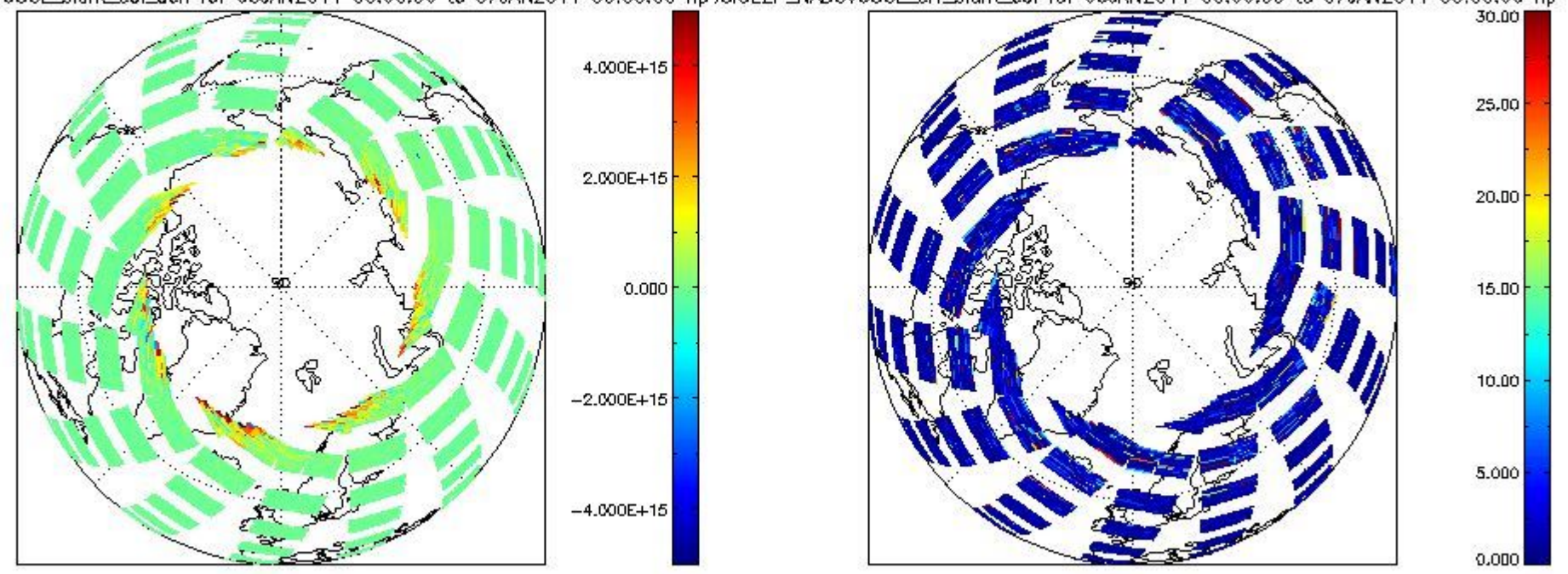
SCIOI2P_NADUV60CLslant_col_den for 06JAN2011 00:00:00 to 07JAN2011 00:00:00 np; SCIOI2P_NADUV60CLarr_slant_col for 06JAN2011 00:00:00 to 07JAN2011 00:00:00 np
