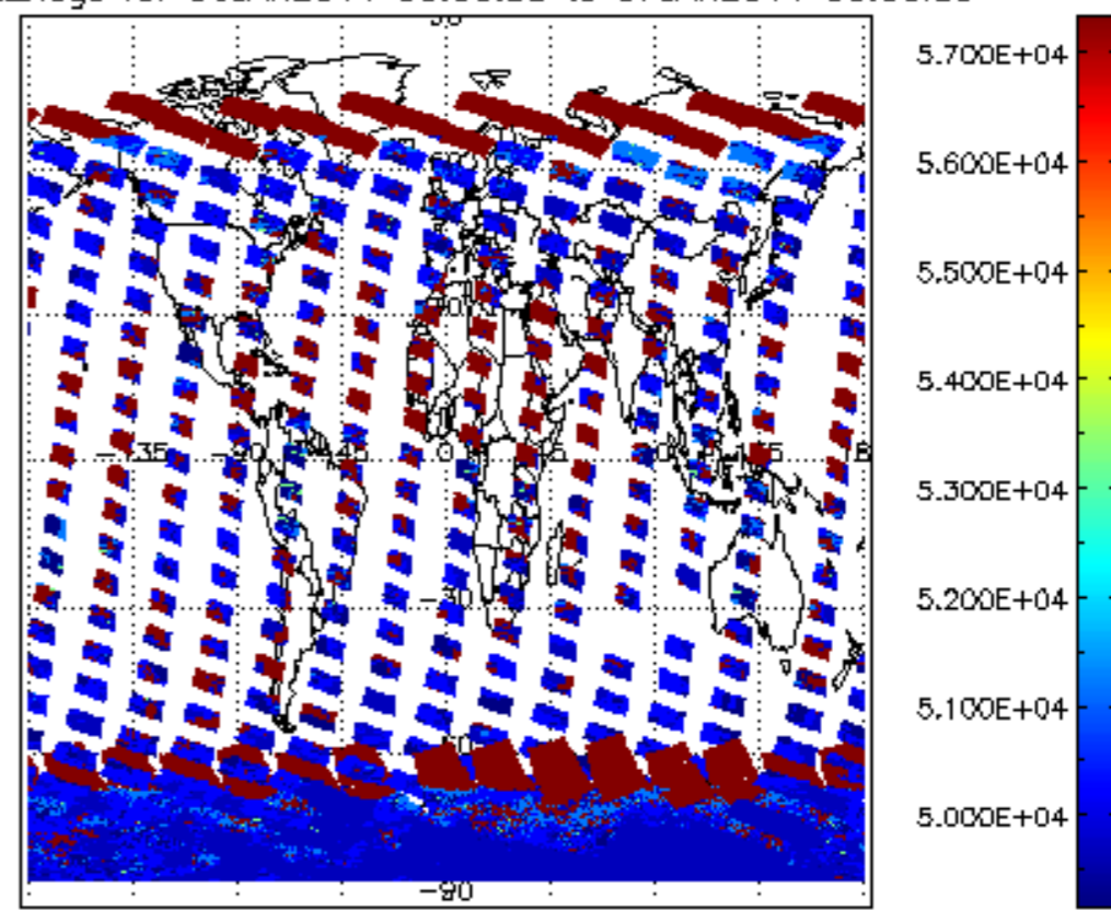
cloud_flags for 06JAN2011 00:00:00 to 07JAN2011 00:00:00
