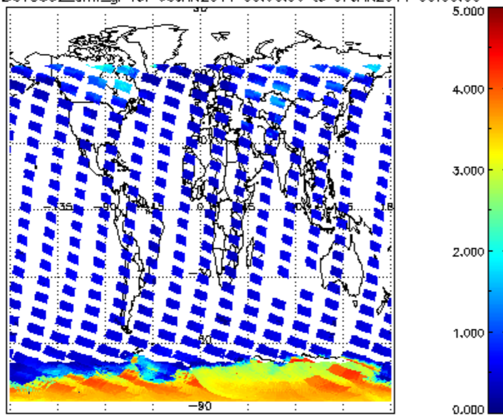
SCIOL2P_NADUV5SO2_amf_gr for 06JAN2011 00:00:00 to 07JAN2011 00:00:00
