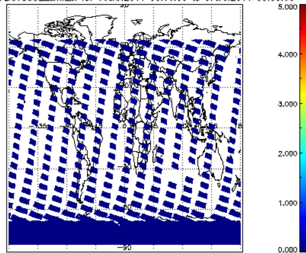
SCIOL2P_NADUV5SO2_amf_sl for 06JAN2011 00:00:00 to 07JAN2011 00:00:00
