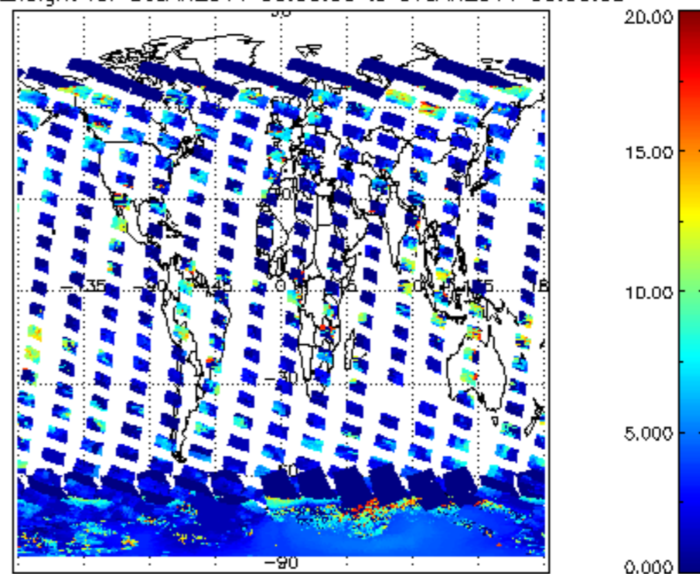
cL_top_height for 06JAN2011 00:00:00 to 07JAN2011 00:00:00
