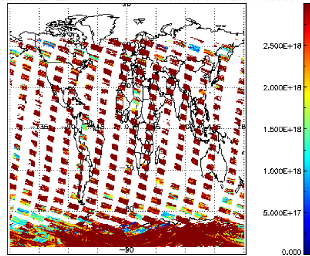
SCIOL2P_NADIR3CO_vcd_err for 06JAN2011 00:00:00 to 07JAN2011 00:00:00
