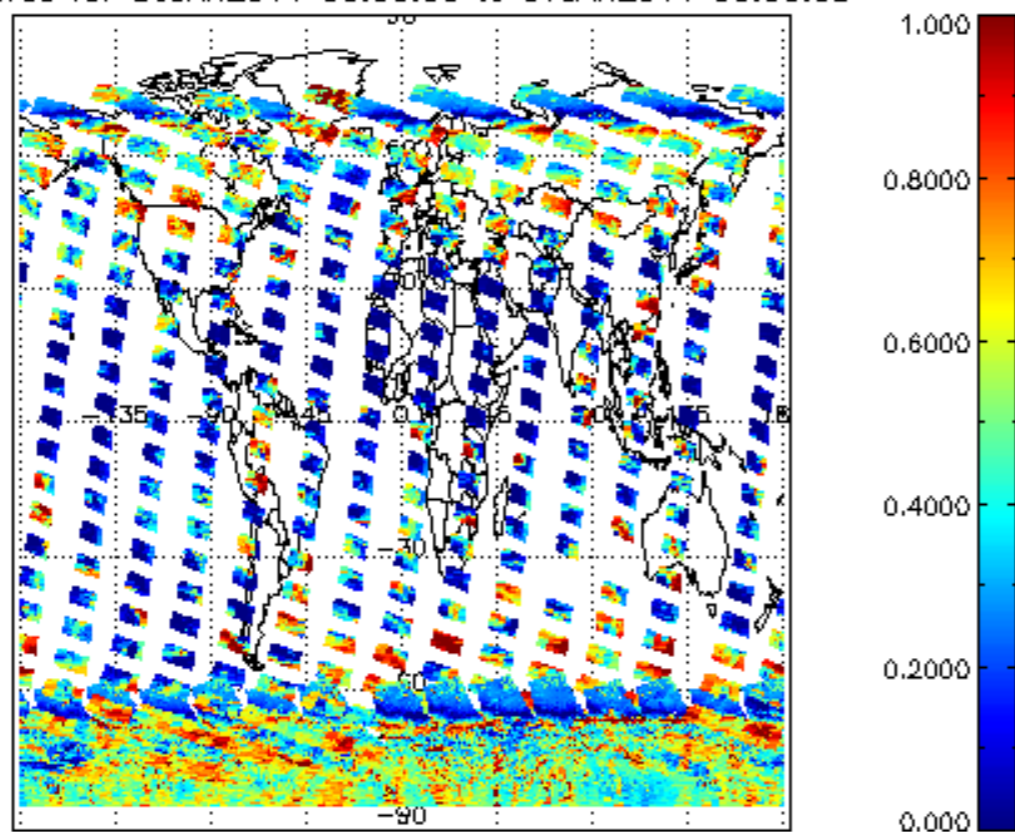
cL_frac for 06JAN2011 00:00:00 to 07JAN2011 00:00:00
