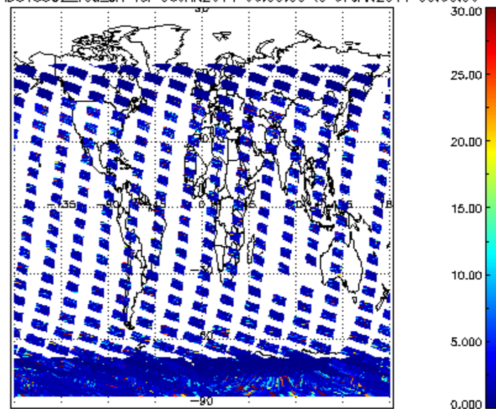
SCIOL2P_NADUV5SO2_vcd_err for 06JAN2011 00:00:00 to 07JAN2011 00:00:00
