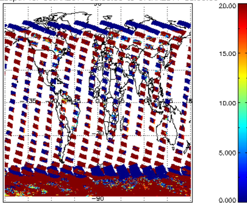
cLopt_depth for 06JAN2011 00:00:00 to 07JAN2011 00:00:00
