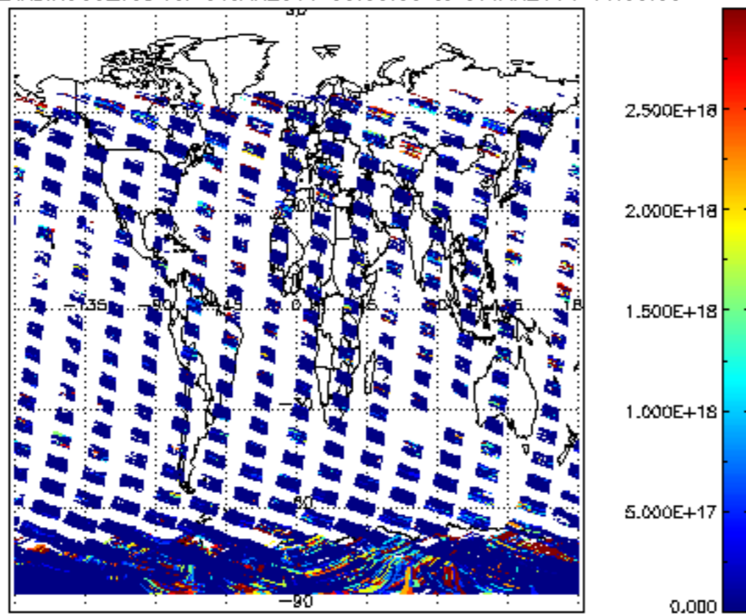
SCIOL2P_NADIR3CO_vcd for 06JAN2011 00:00:00 to 07JAN2011 00:00:00
