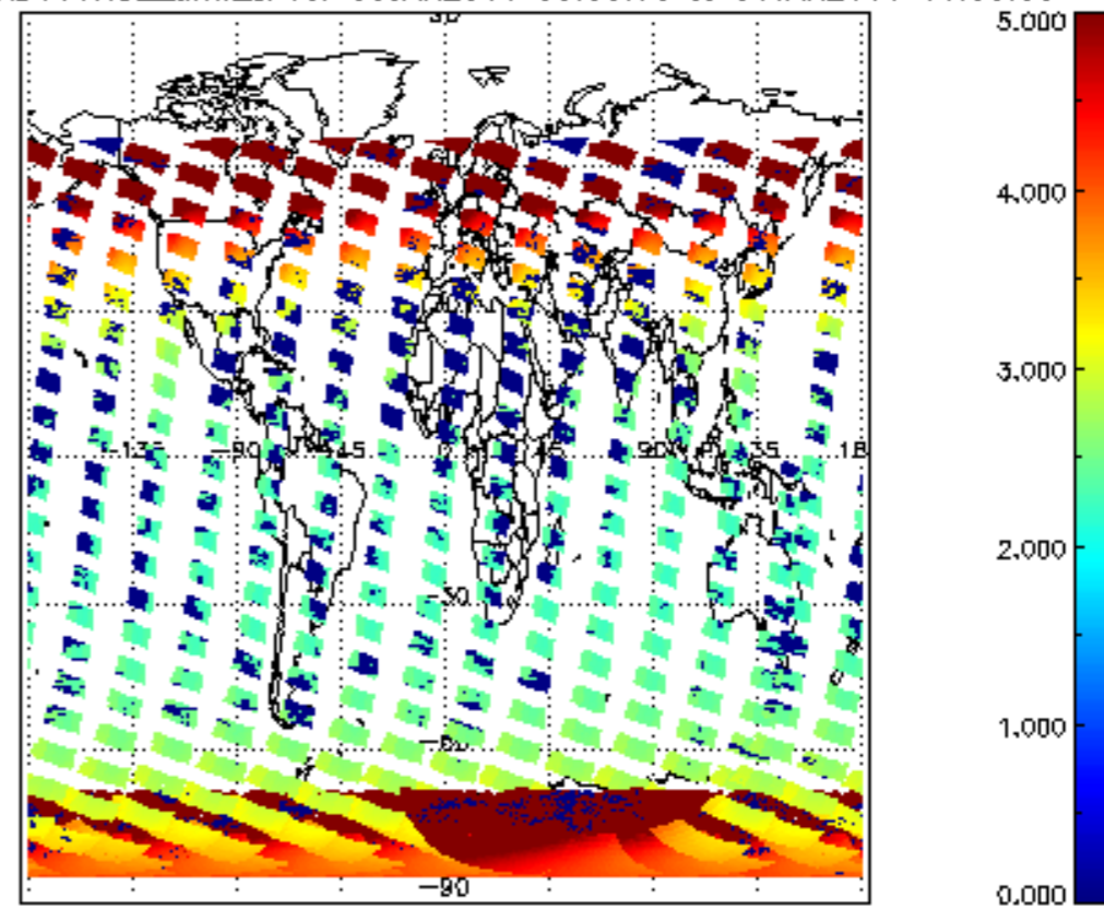
SCIOL2P_NADUV1NO2_amf_cl for 05JAN2011 00:00:00 to 06JAN2011 00:00:00
