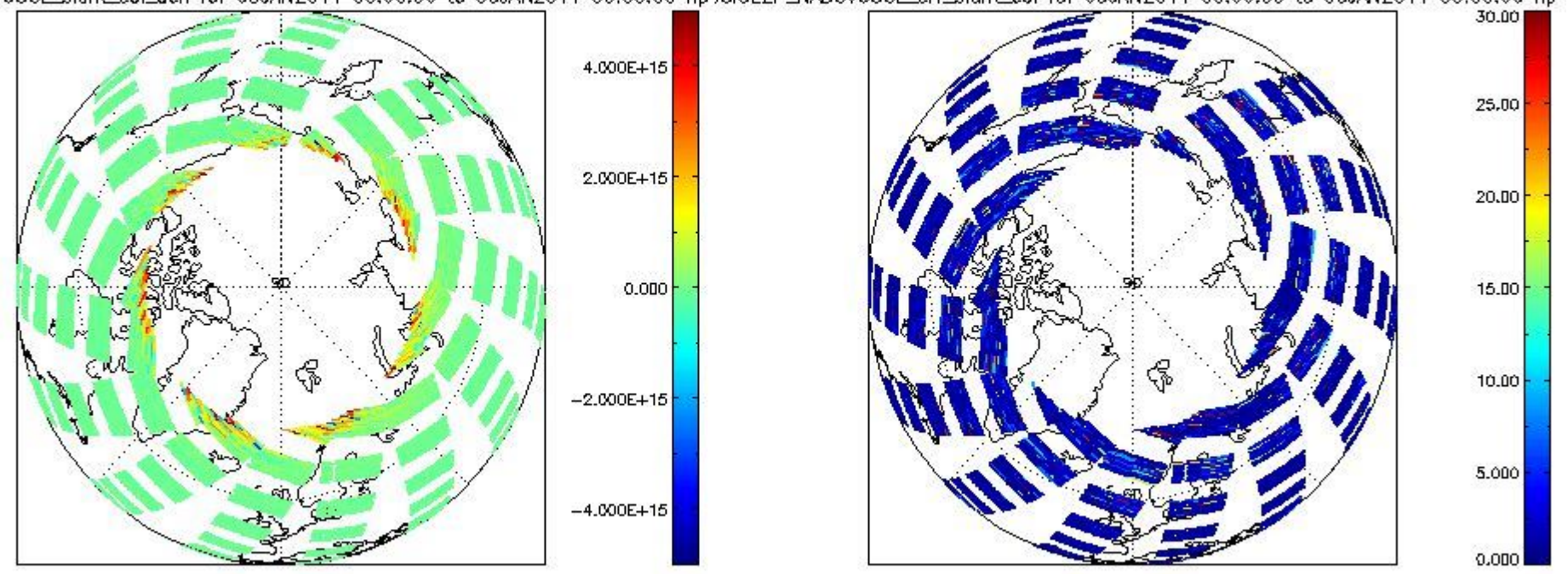
SCIO2P_NADUV60CL_slant_col_den for 05JAN2011 00:00:00 to 06JAN2011 00:00:00 np; SCIO2P_NADUV60CL_err_slant_col for 05JAN2011 00:00:00 to 06JAN2011 00:00:00 np
