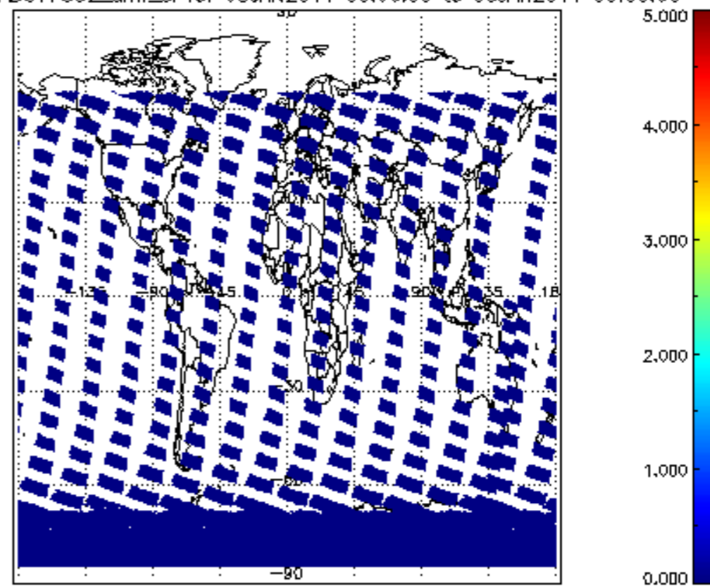
SCIOL2P_NADUV7S02_amf_sl for 05JAN2011 00:00:00 to 06JAN2011 00:00:00
