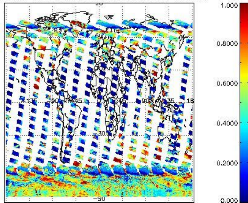
cL_frac for 05JAN2011 00:00:00 to 06JAN2011 00:00:00
