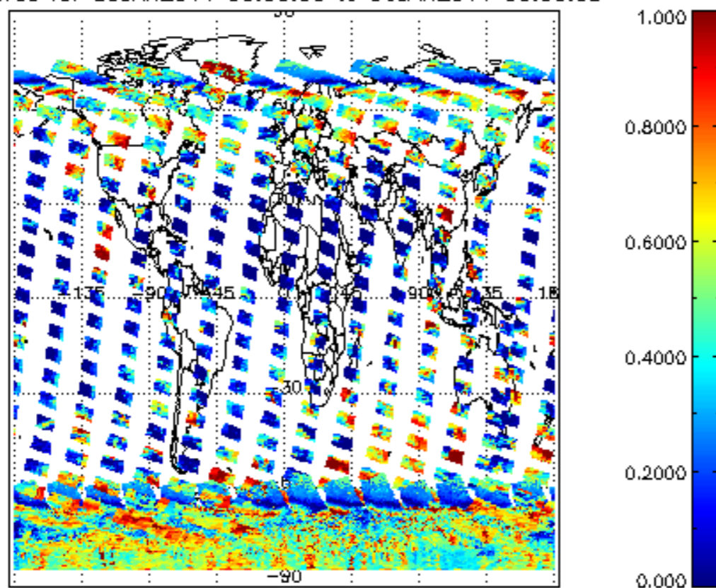
cL_frac for 05JAN2011 00:00:00 to 06JAN2011 00:00:00
