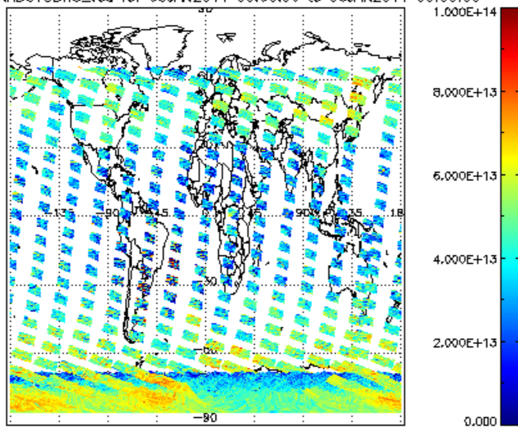
SCIOL2P_NADUV3BRO_vcd for 05JAN2011 00:00:00 to 06JAN2011 00:00:00
