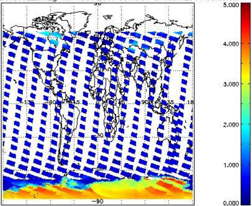
SCIOL2P_NADUV5SO2_amf_gr for 05JAN2011 00:00:00 to 06JAN2011 00:00:00
