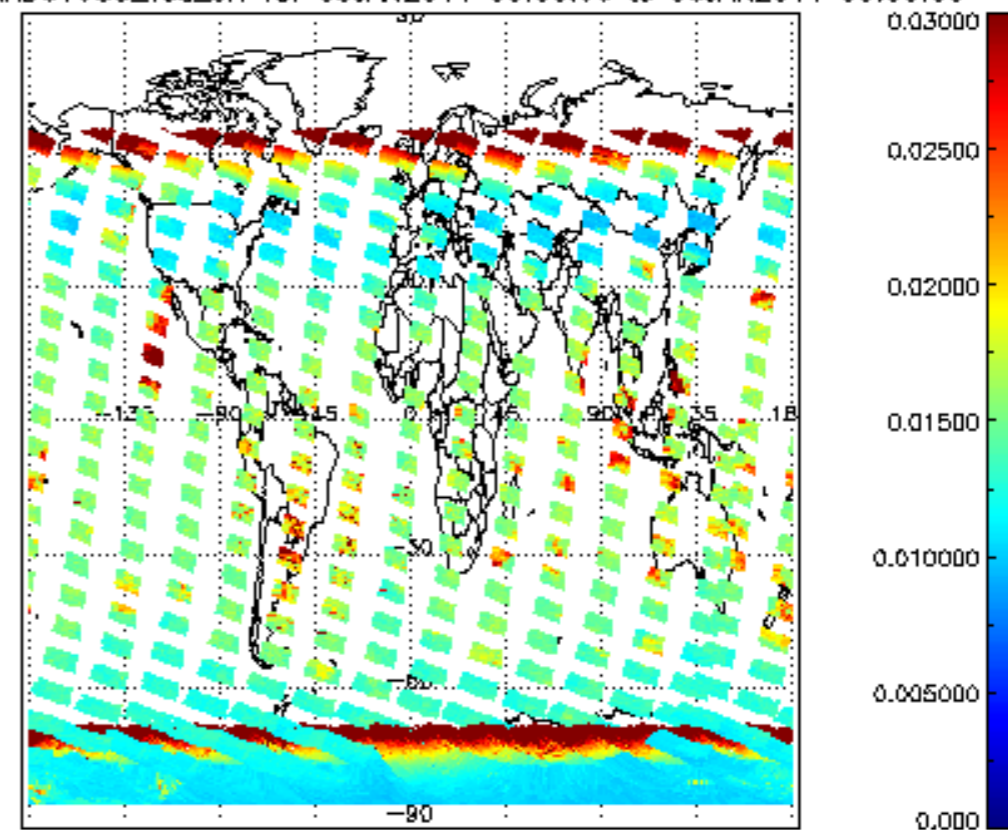
SCIOL2P_NADUV003_vcd_err for 05JAN2011 00:00:00 to 06JAN2011 00:00:00
