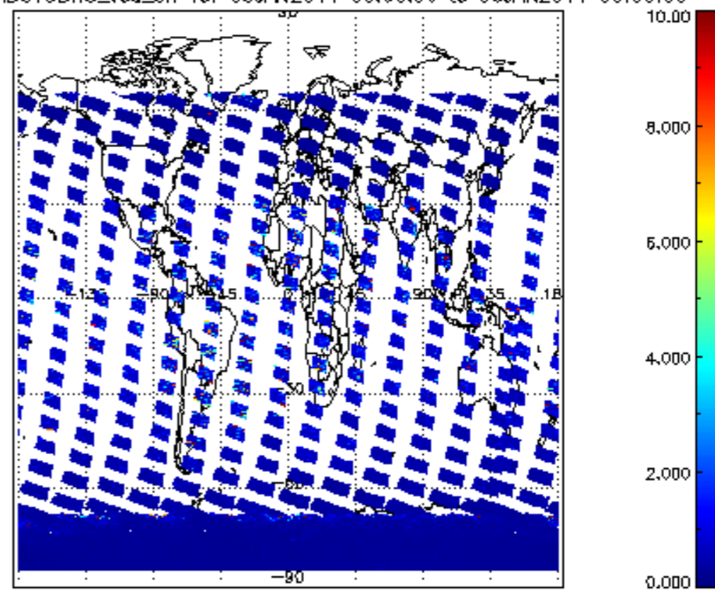
SCIOL2P_NADUV3BRO_vcd_err for 05JAN2011 00:00:00 to 06JAN2011 00:00:00
