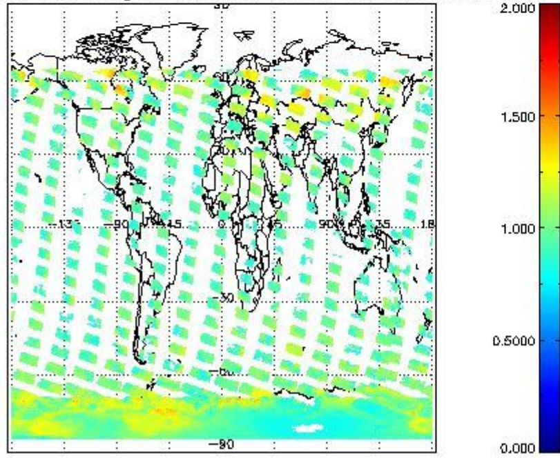
SCIOL2P_NADUV8H20_amf_gr for 05JAN2011 00:00:00 to 06JAN2011 00:00:00
