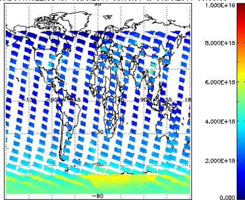
SCIOL2P_NADUV1NO2_vcd for 05JAN2011 00:00:00 to 06JAN2011 00:00:00
