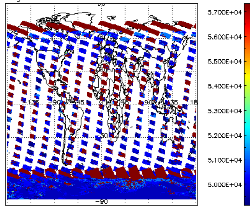
cloud_flags for 05JAN2011 00:00:00 to 06JAN2011 00:00:00
