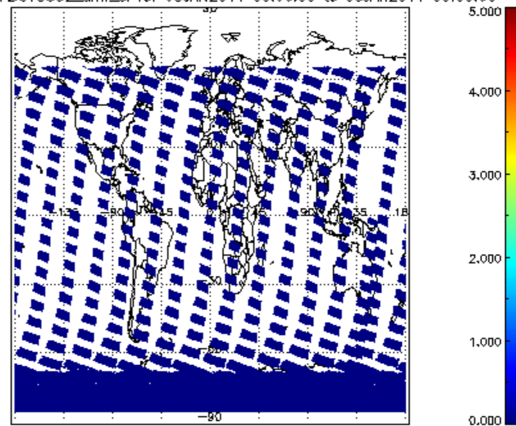
SCIOL2P_NADUV5S02_amf_sl for 05JAN2011 00:00:00 to 06JAN2011 00:00:00
