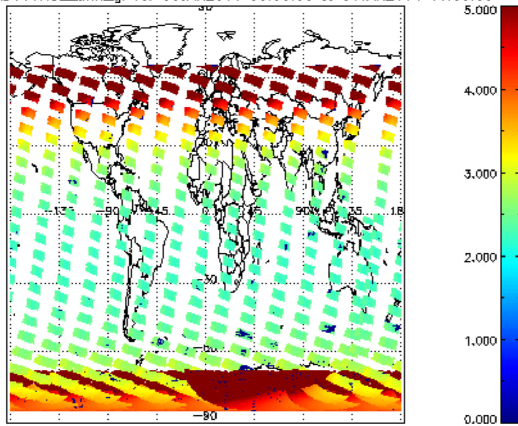
SCIOL2P_NADUV1NO2_amf_gr for 05JAN2011 00:00:00 to 06JAN2011 00:00:00
