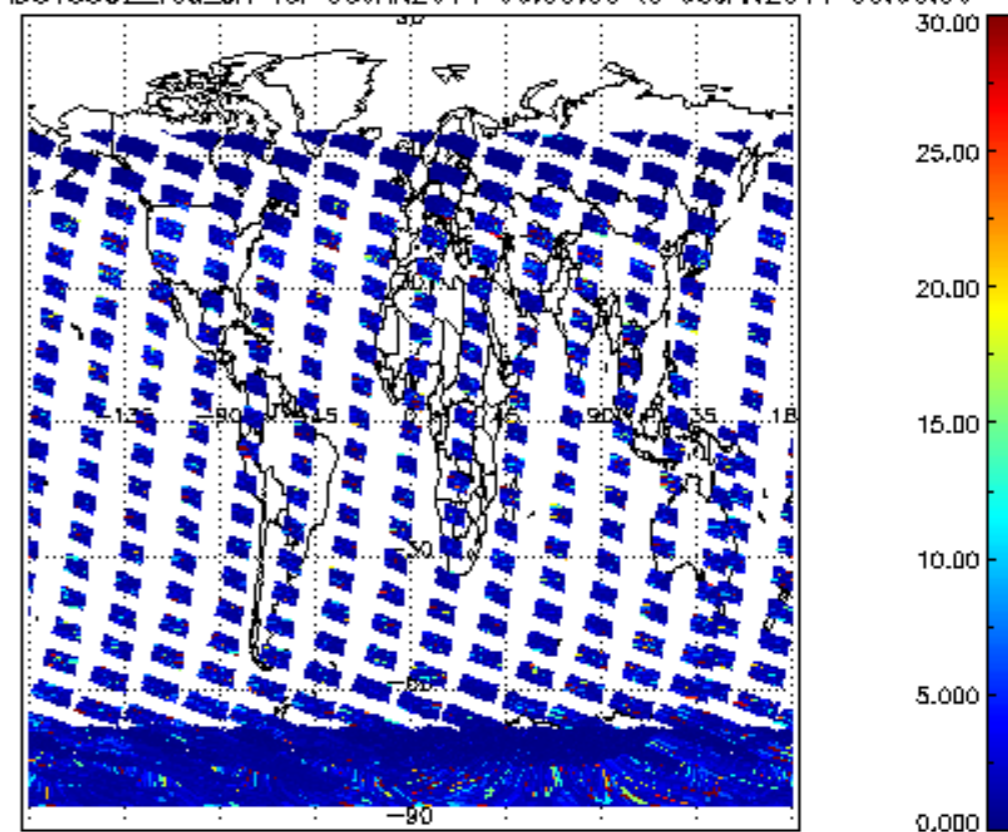
SCIOL2P_NADUV5S02_vcd_err for 05JAN2011 00:00:00 to 06JAN2011 00:00:00
