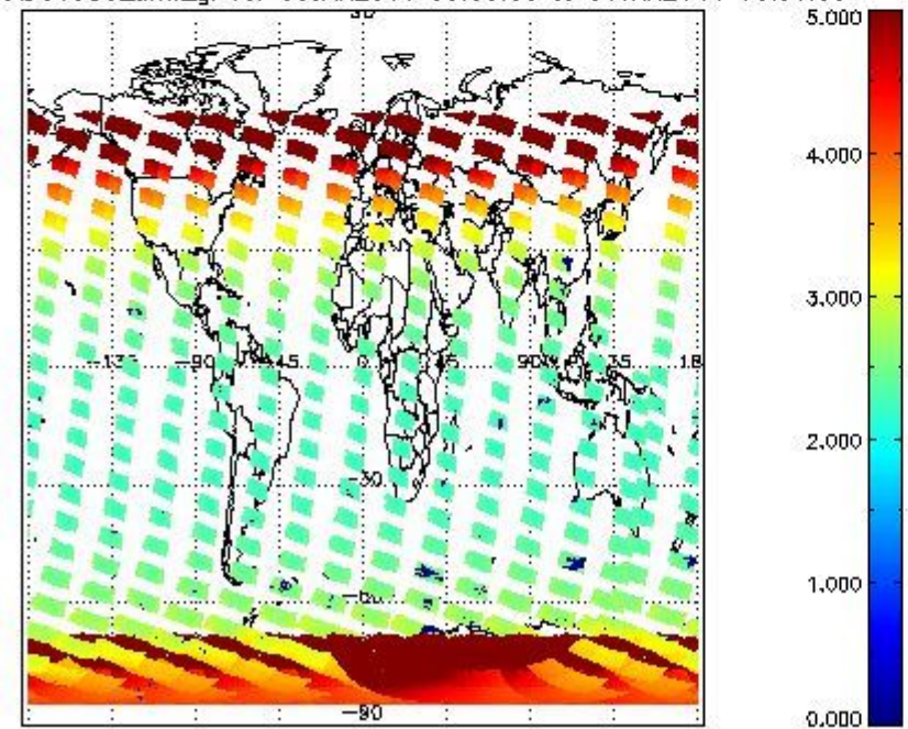
SCIOL2P_NADUV003_amf_gr for 05JAN2011 00:00:00 to 06JAN2011 00:00:00
