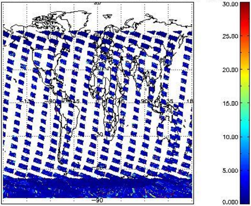
SCIOL2P_NADUV5SO2_vcd_err for 05JAN2011 00:00:00 to 06JAN2011 00:00:00
