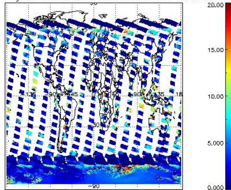
cL_top_height for 05JAN2011 00:00:00 to 06JAN2011 00:00:00
