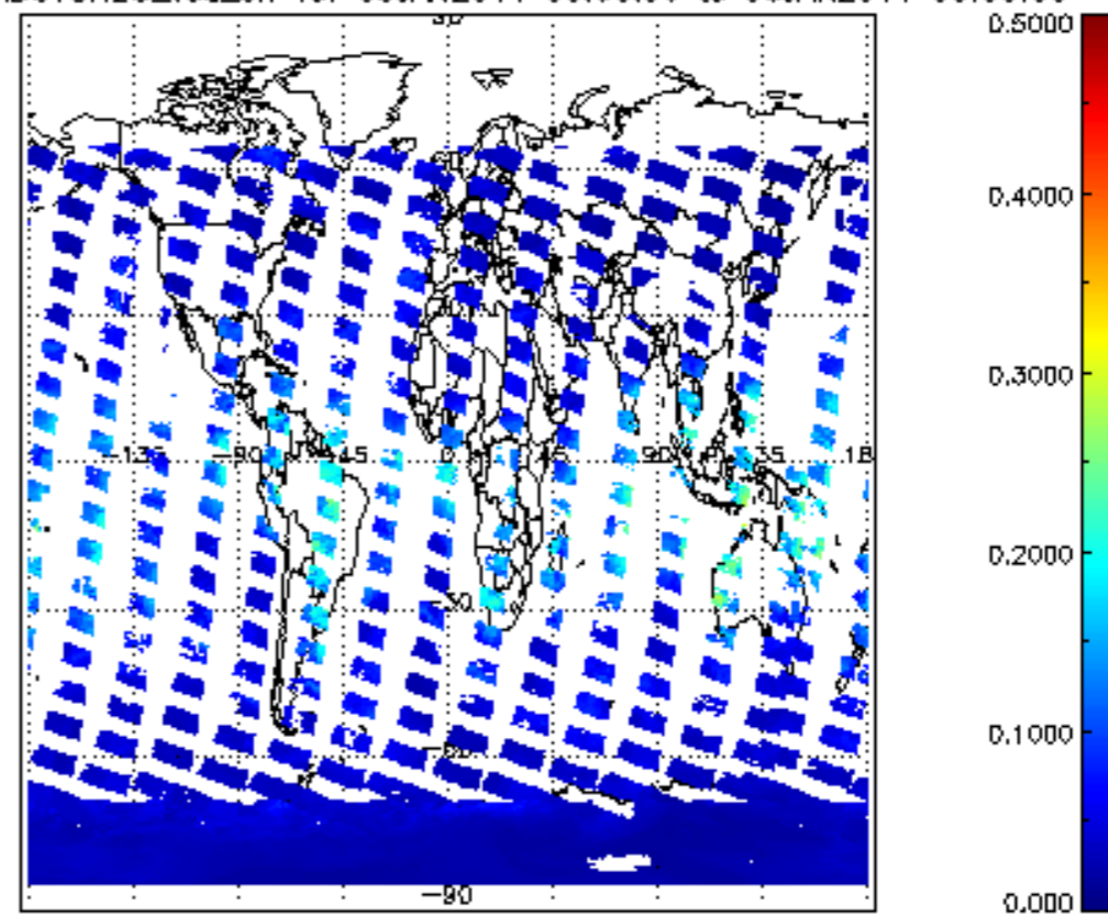
SCIOL2P_NADUV8H20_vcd_err for 05JAN2011 00:00:00 to 06JAN2011 00:00:00
