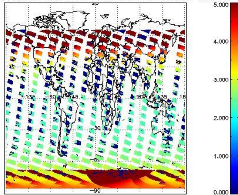
SCIOL2P_NADUV1NO2_amf_cl for 05JAN2011 00:00:00 to 06JAN2011 00:00:00
