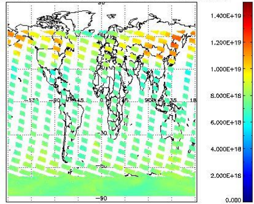
SCIOL2P_NADUV003_vcd for 05JAN2011 00:00:00 to 06JAN2011 00:00:00
