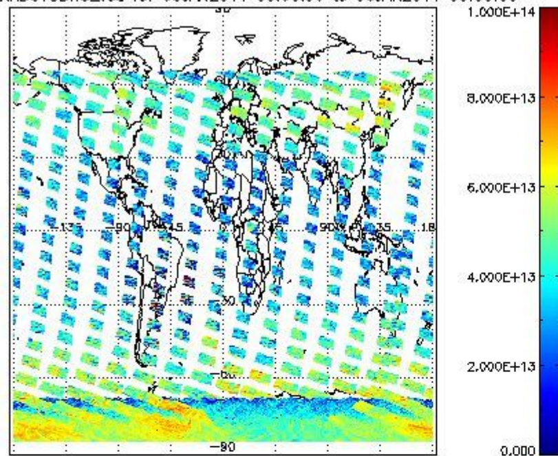
SCIOL2P_NADUV3BRO_vcd for 05JAN2011 00:00:00 to 06JAN2011 00:00:00
