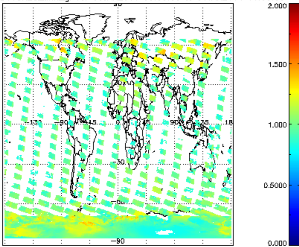
SCIOL2P_NADUV8H20_amf_gr for 05JAN2011 00:00:00 to 06JAN2011 00:00:00
