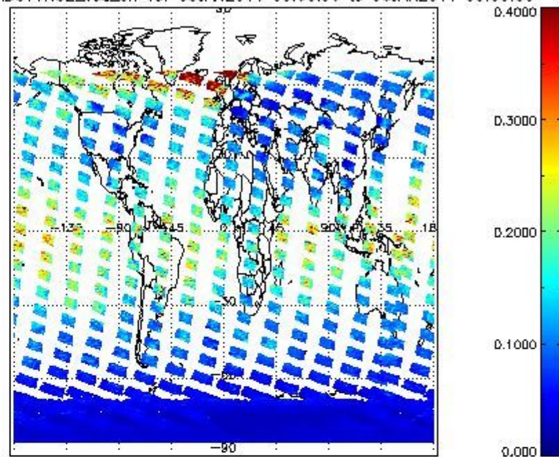
SCIOL2P_NADUV1NO2_vcd_err for 05JAN2011 00:00:00 to 06JAN2011 00:00:00
