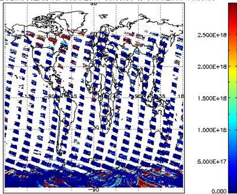
SCIDL2P_NADIR3CO_vcd for 05JAN2011 00:00:00 to 06JAN2011 00:00:00
