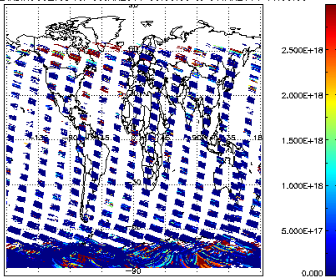
SCIOL2P_NADIR3CO_vcd for 05JAN2011 00:00:00 to 06JAN2011 00:00:00
