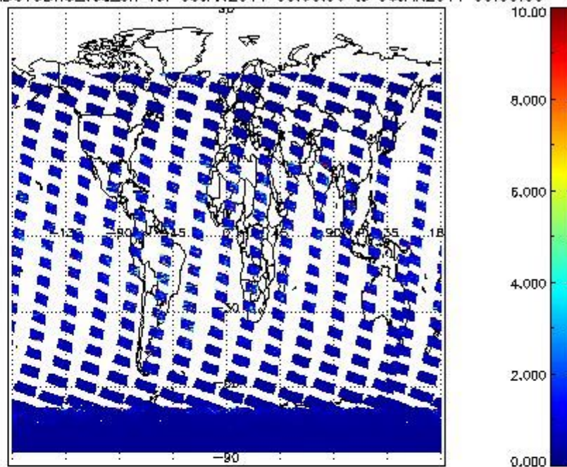
SCIOL2P_NADUV3BRO_vcd_err for 05JAN2011 00:00:00 to 06JAN2011 00:00:00
