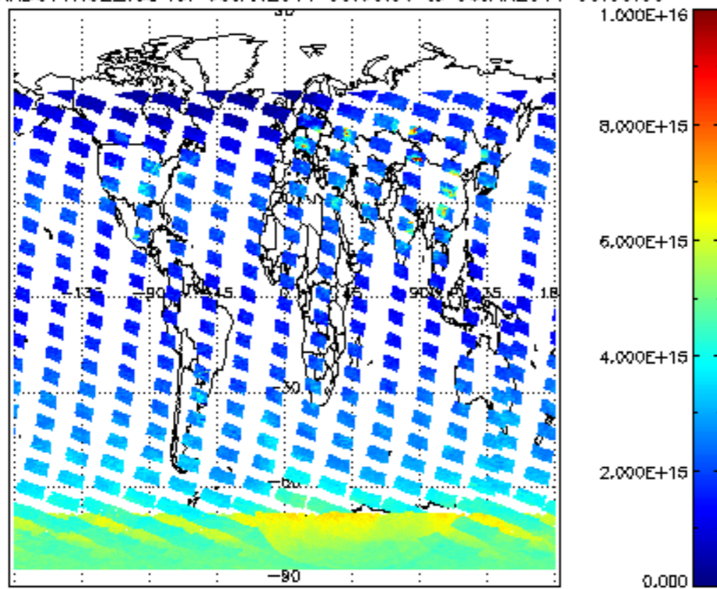
SCIOL2P_NADUV1NO2_vcd for 05JAN2011 00:00:00 to 06JAN2011 00:00:00
