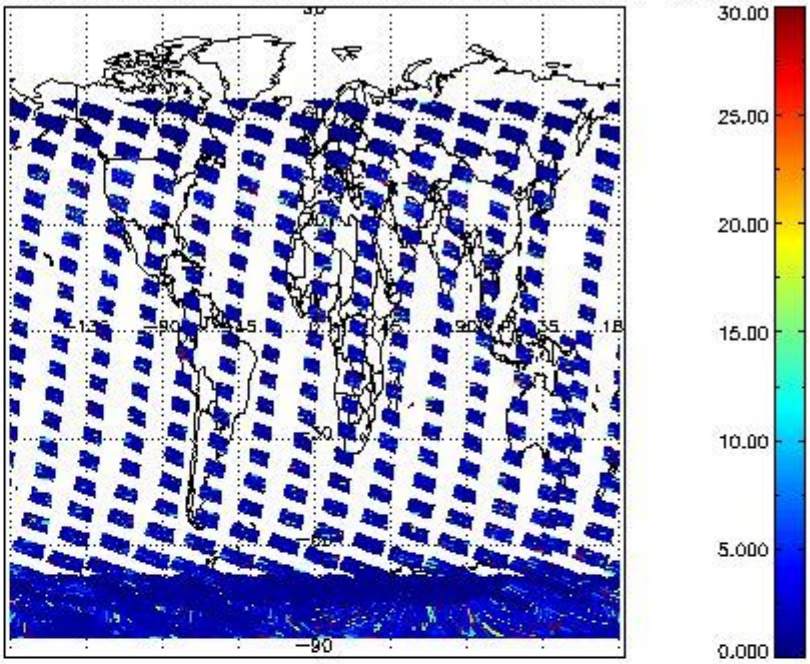
SCIOL2P_NADUV7S02_vcd_err for 05JAN2011 00:00:00 to 06JAN2011 00:00:00
