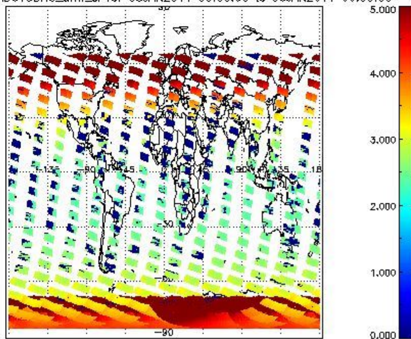
SCIOL2P_NADUV3BRO_amf_cl for 05JAN2011 00:00:00 to 06JAN2011 00:00:00
