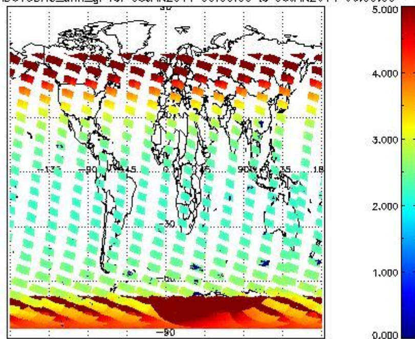
SCIOL2P_NADUV3BRO_amf_gr for 05JAN2011 00:00:00 to 06JAN2011 00:00:00
