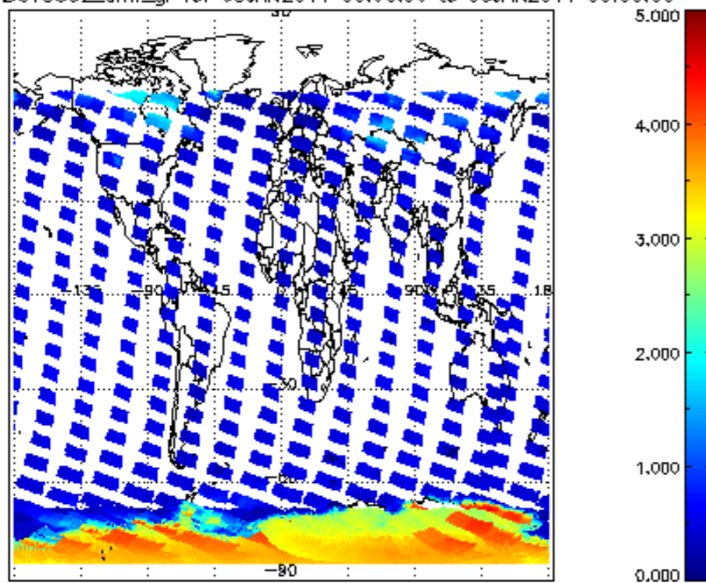
SCIOL2P_NADUV5S02_amf_gr for 05JAN2011 00:00:00 to 06JAN2011 00:00:00
