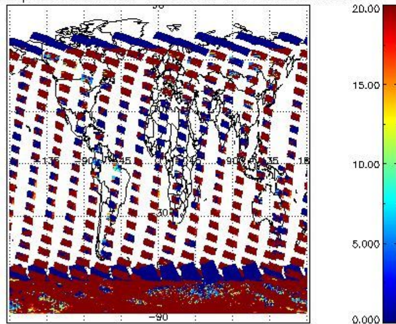
cLopt_depth for 05JAN2011 00:00:00 to 06JAN2011 00:00:00
