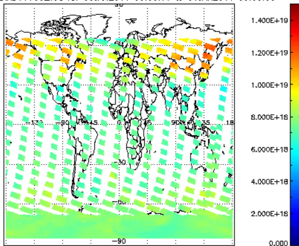
SCIOL2P_NADUV003_vcd for 05JAN2011 00:00:00 to 06JAN2011 00:00:00
