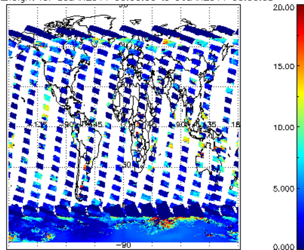
cL_top_height for 05JAN2011 00:00:00 to 06JAN2011 00:00:00
