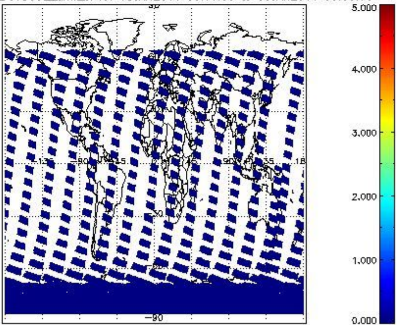
SCIOL2P_NADUV5SO2_amf_cl for 05JAN2011 00:00:00 to 06JAN2011 00:00:00
