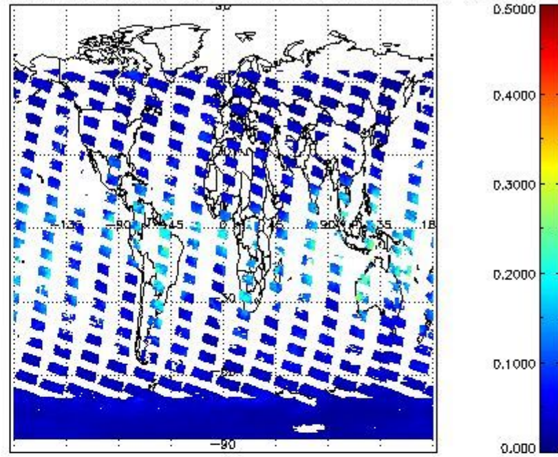
SCIOL2P_NADUV8H20_vcd_err for 05JAN2011 00:00:00 to 06JAN2011 00:00:00
