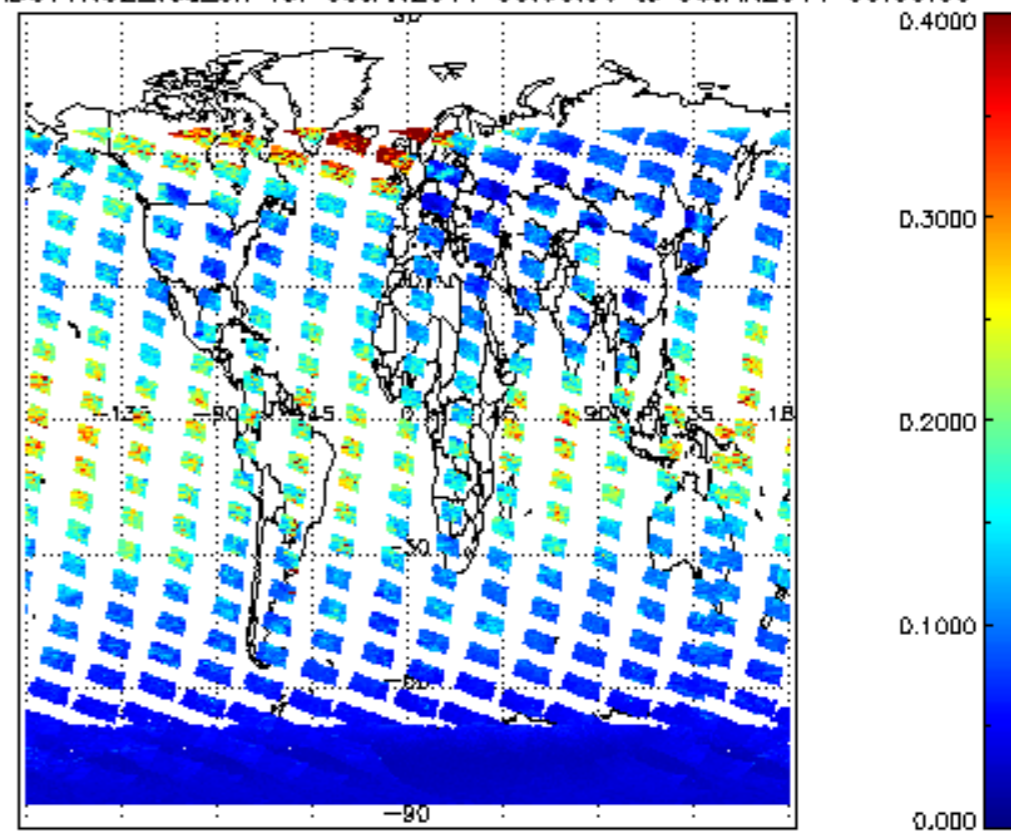
SCIOL2P_NADUV1NO2_vcd_err for 05JAN2011 00:00:00 to 06JAN2011 00:00:00
