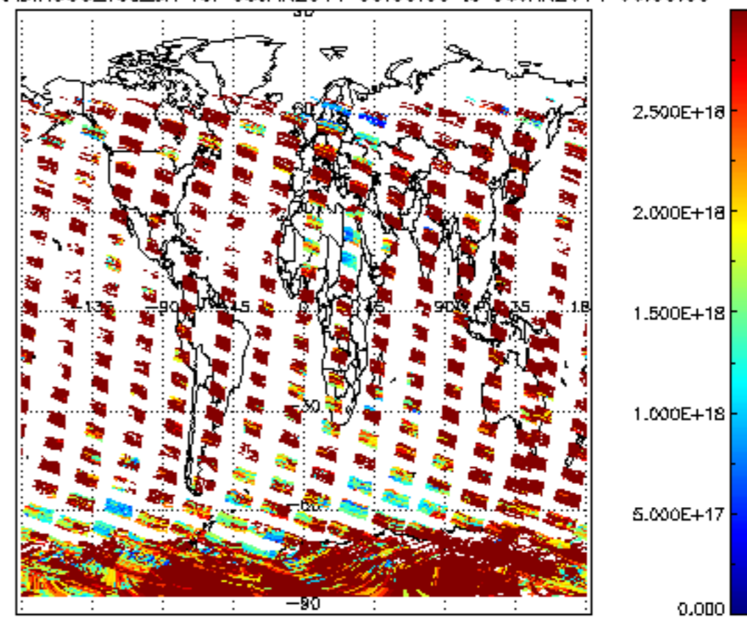
SCIOL2P_NADIR3CO_vcd_err for 05JAN2011 00:00:00 to 06JAN2011 00:00:00
