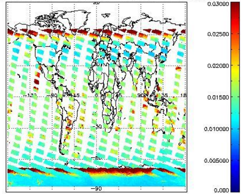
SCIOL2P_NADUV003_vcd_err for 05JAN2011 00:00:00 to 06JAN2011 00:00:00
