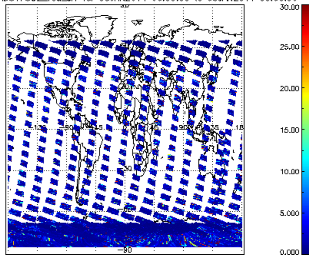
SCIOL2P_NADUV7S02_vcd_err for 05JAN2011 00:00:00 to 06JAN2011 00:00:00
