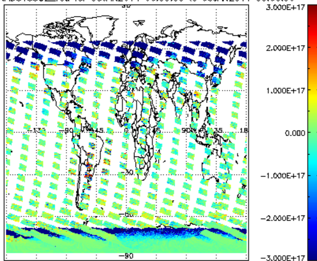
SCIOL2P_NADUV5S02_vcd for 05JAN2011 00:00:00 to 06JAN2011 00:00:00
