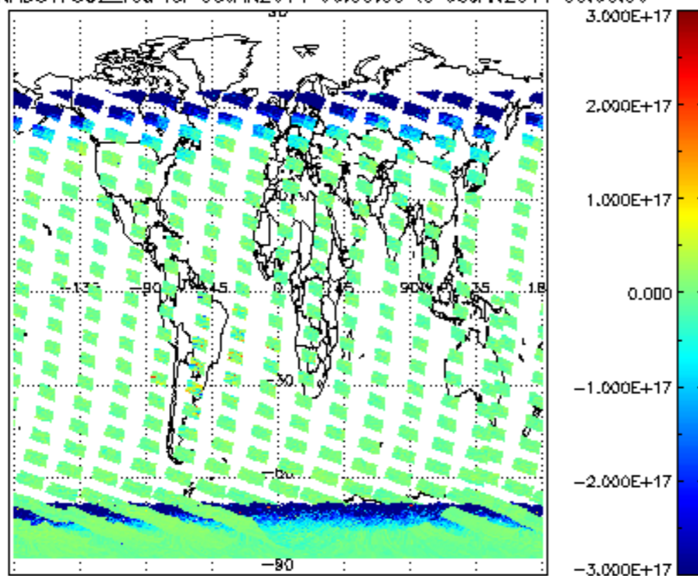
SCIOL2P_NADUV7S02_vcd for 05JAN2011 00:00:00 to 06JAN2011 00:00:00
