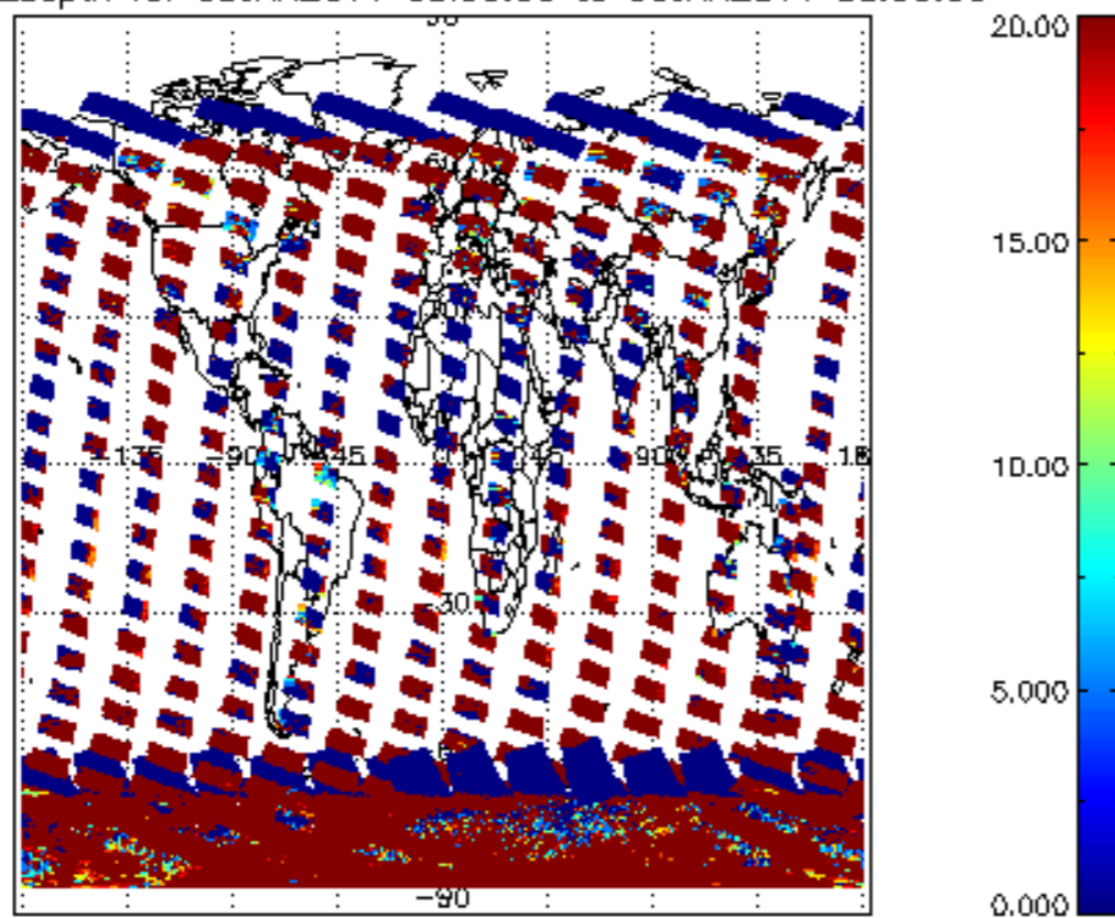
cLopt_depth for 05JAN2011 00:00:00 to 06JAN2011 00:00:00
