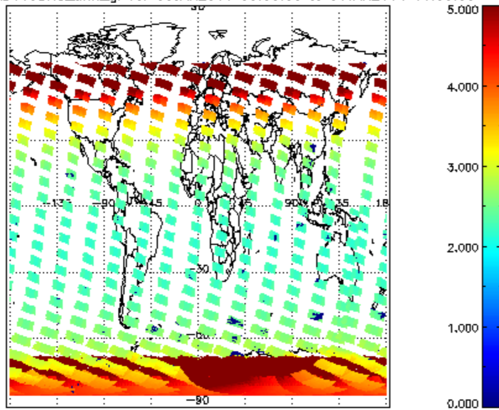
SCIOL2P_NADUV3BRO_amf_gr for 05JAN2011 00:00:00 to 06JAN2011 00:00:00
