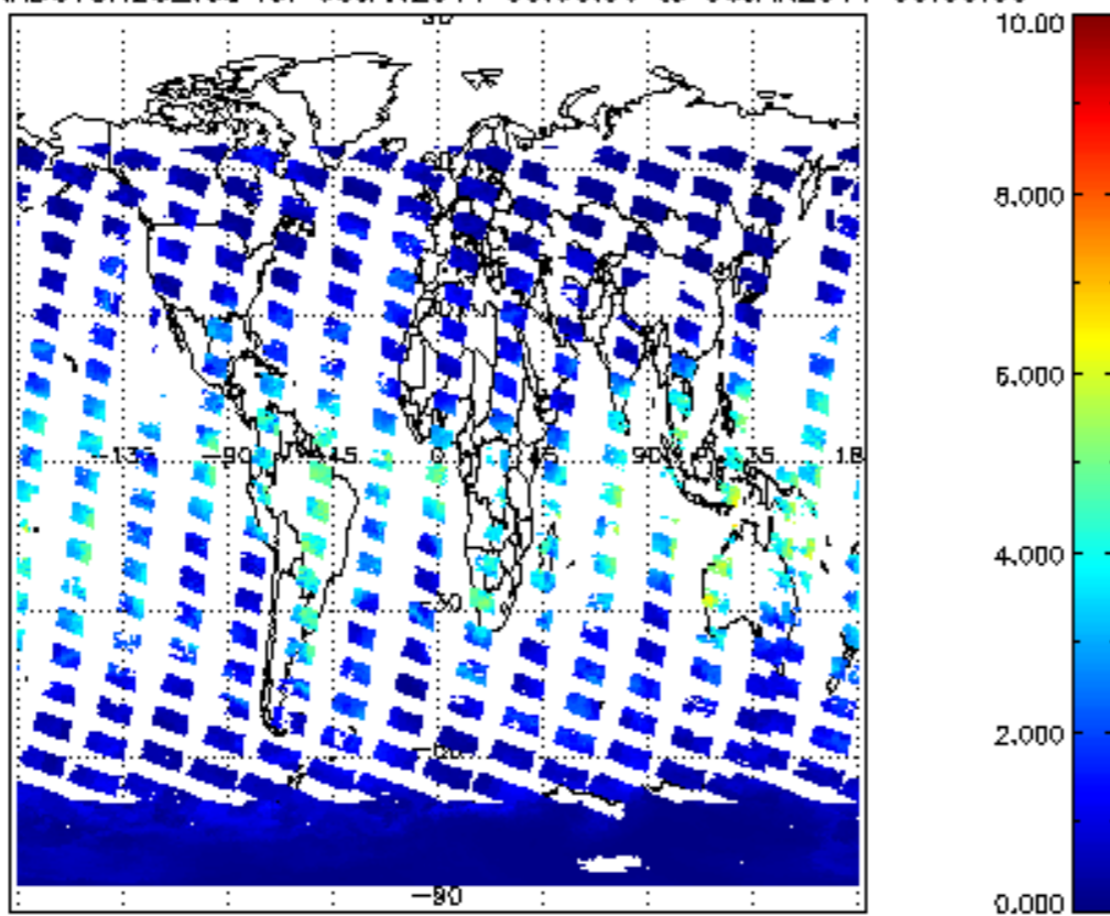
SCIOL2P_NADUV8H20_vcd for 05JAN2011 00:00:00 to 06JAN2011 00:00:00
