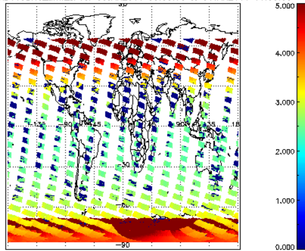
SCIOL2P_NADUV3BRO_amf_cl for 05JAN2011 00:00:00 to 06JAN2011 00:00:00
