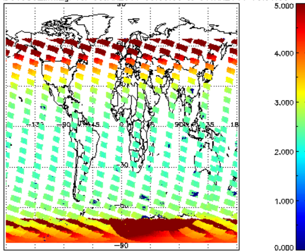
SCIOL2P_NADUV003_amf_gr for 05JAN2011 00:00:00 to 06JAN2011 00:00:00
