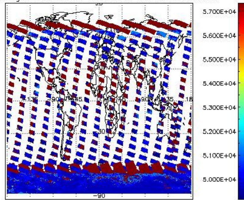
cloud_flags for 05JAN2011 00:00:00 to 06JAN2011 00:00:00
