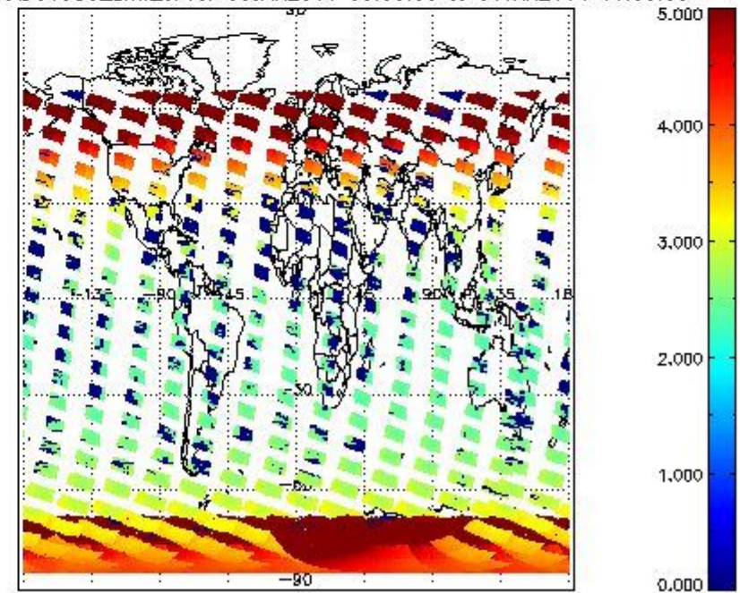
SCIOL2P_NADUV003_amf_cl for 05JAN2011 00:00:00 to 06JAN2011 00:00:00
