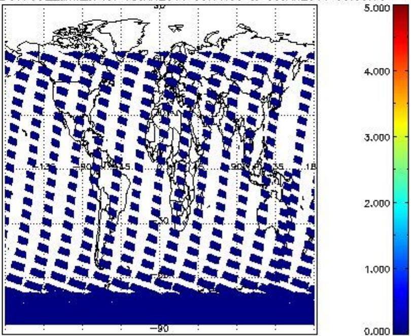
SCIOL2P_NADUV7S02_amf_cl for 05JAN2011 00:00:00 to 06JAN2011 00:00:00
