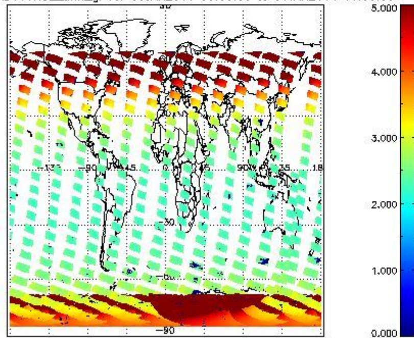
SCIOL2P_NADUV1NO2_amf_gr for 05JAN2011 00:00:00 to 06JAN2011 00:00:00
