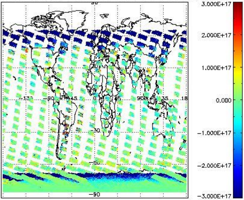
SCIOL2P_NADUV5SO2_vcd for 05JAN2011 00:00:00 to 06JAN2011 00:00:00
