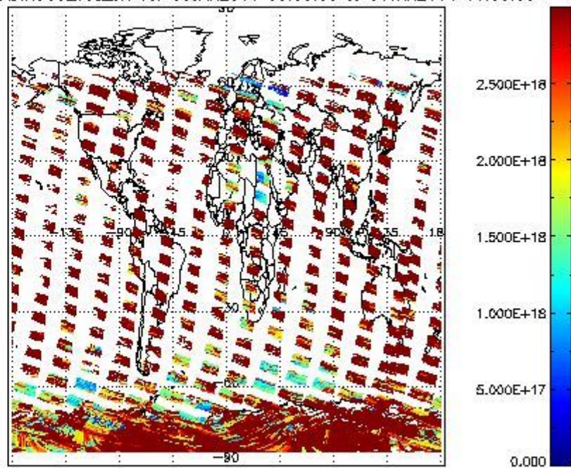
SCIDL2P_NADIR3CO_vcd_err for 05JAN2011 00:00:00 to 06JAN2011 00:00:00
