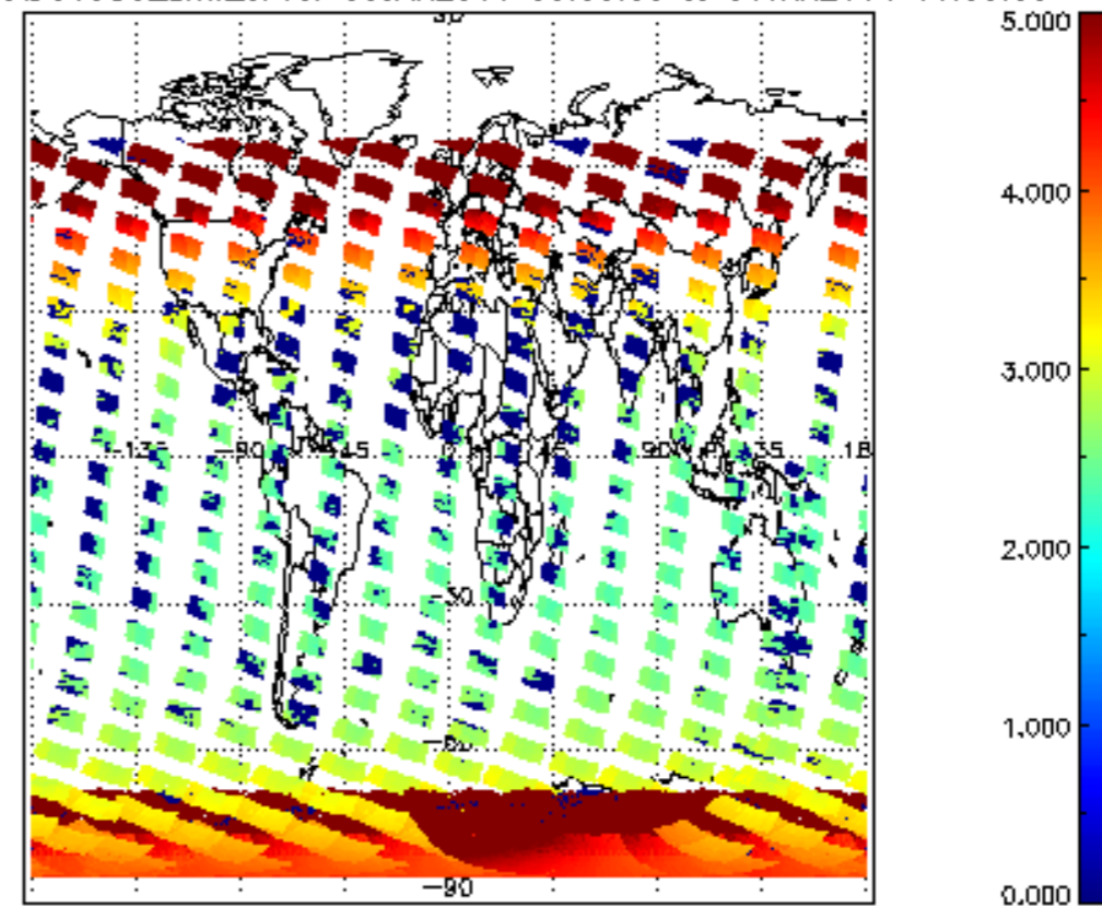
SCIOL2P_NADUV003_amf_cl for 05JAN2011 00:00:00 to 06JAN2011 00:00:00
