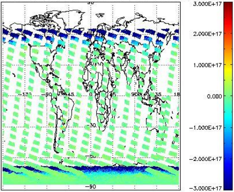
SCIOL2P_NADUV7S02_vcd for 05JAN2011 00:00:00 to 06JAN2011 00:00:00
