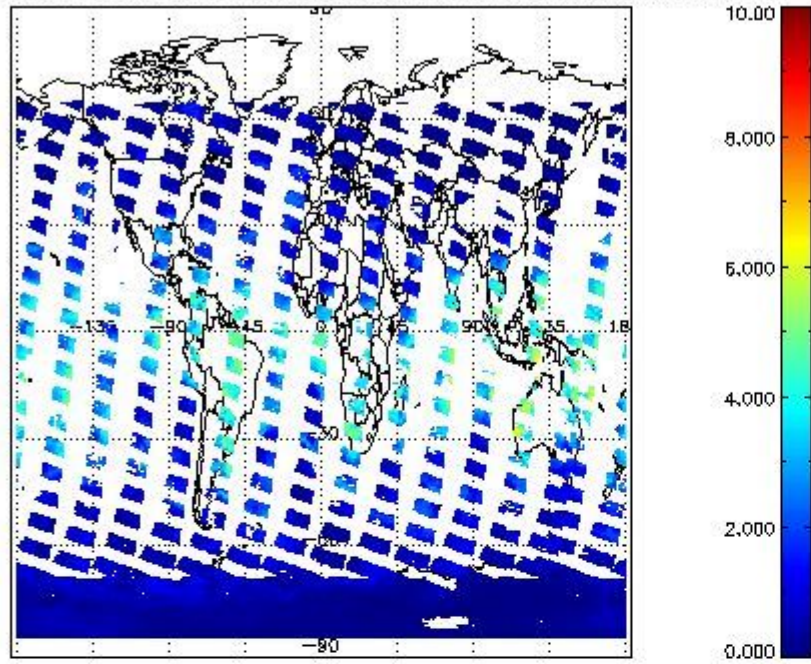
SCIOL2P_NADUV8H20_vcd for 05JAN2011 00:00:00 to 06JAN2011 00:00:00
