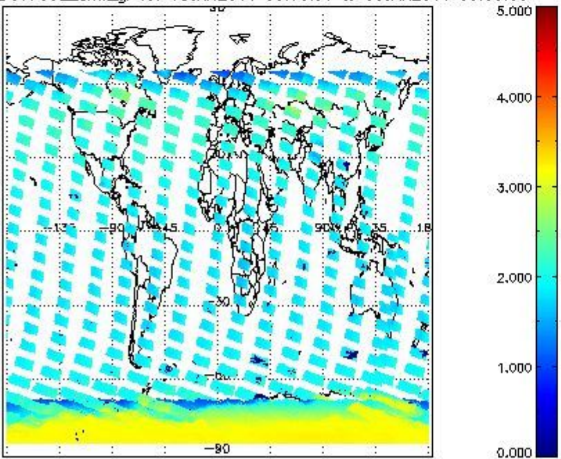
SCIOL2P_NADUV7S02_amf_gr for 05JAN2011 00:00:00 to 06JAN2011 00:00:00
