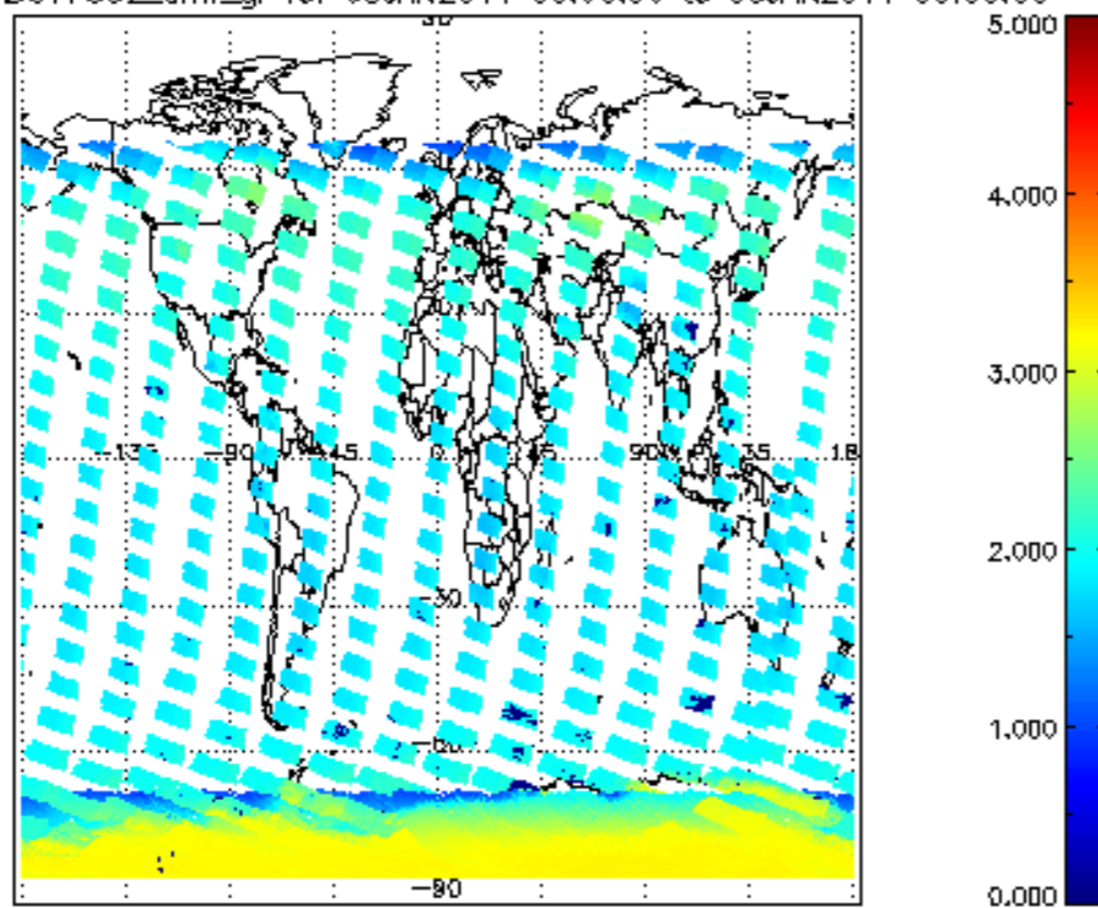
SCIOL2P_NADUV7S02_amf_gr for 05JAN2011 00:00:00 to 06JAN2011 00:00:00
