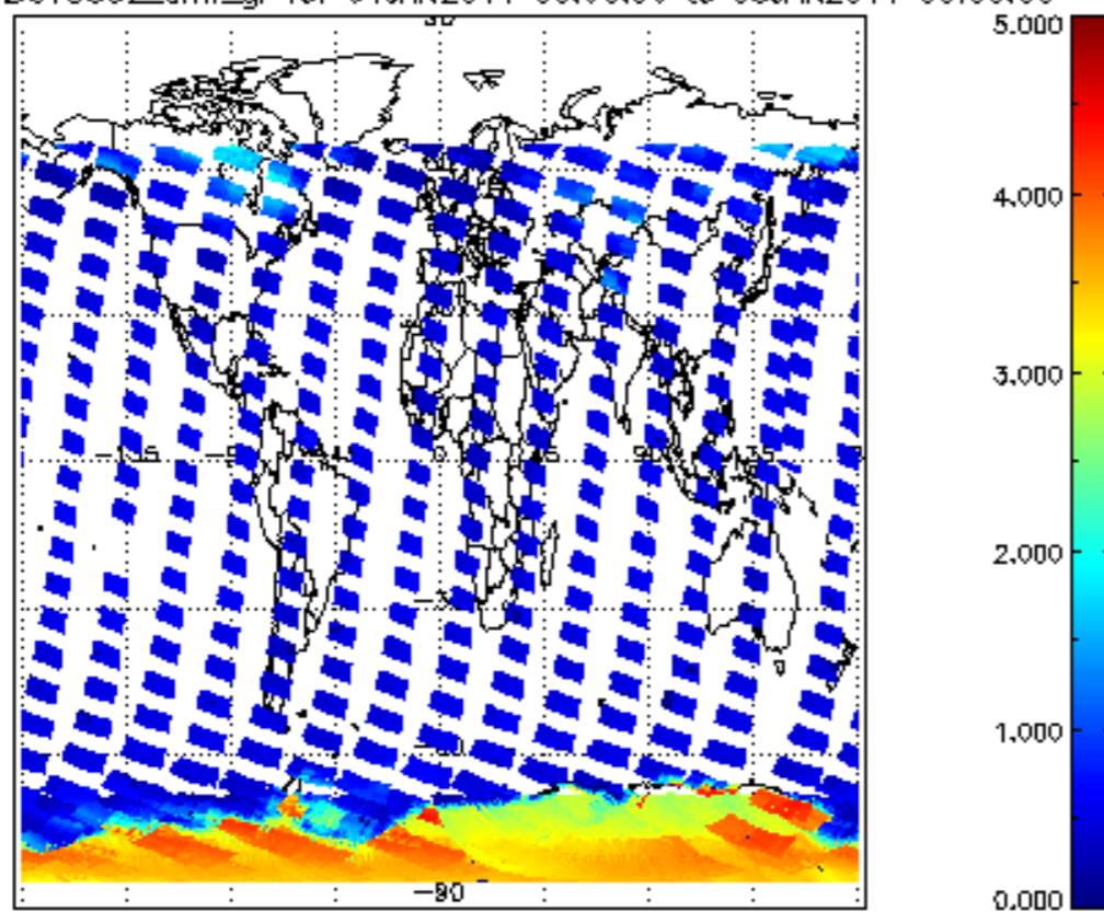
SCIOL2P_NADUV5S02_amf_gr for 04JAN2011 00:00:00 to 05JAN2011 00:00:00
