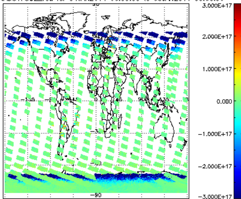
SCIOL2P_NADUV7S02_vcd for 04JAN2011 00:00:00 to 05JAN2011 00:00:00
