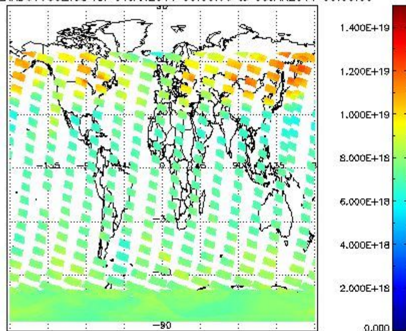
SCIOL2P_NADUV003_vcd for 04JAN2011 00:00:00 to 05JAN2011 00:00:00
