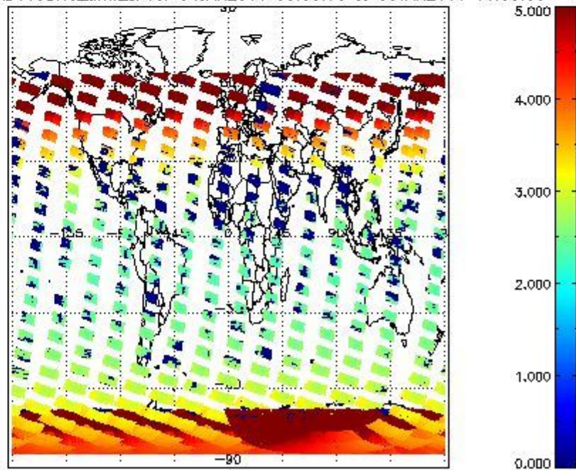
SCIOL2P_NADUV3BRO_amf_cl for 04JAN2011 00:00:00 to 05JAN2011 00:00:00
