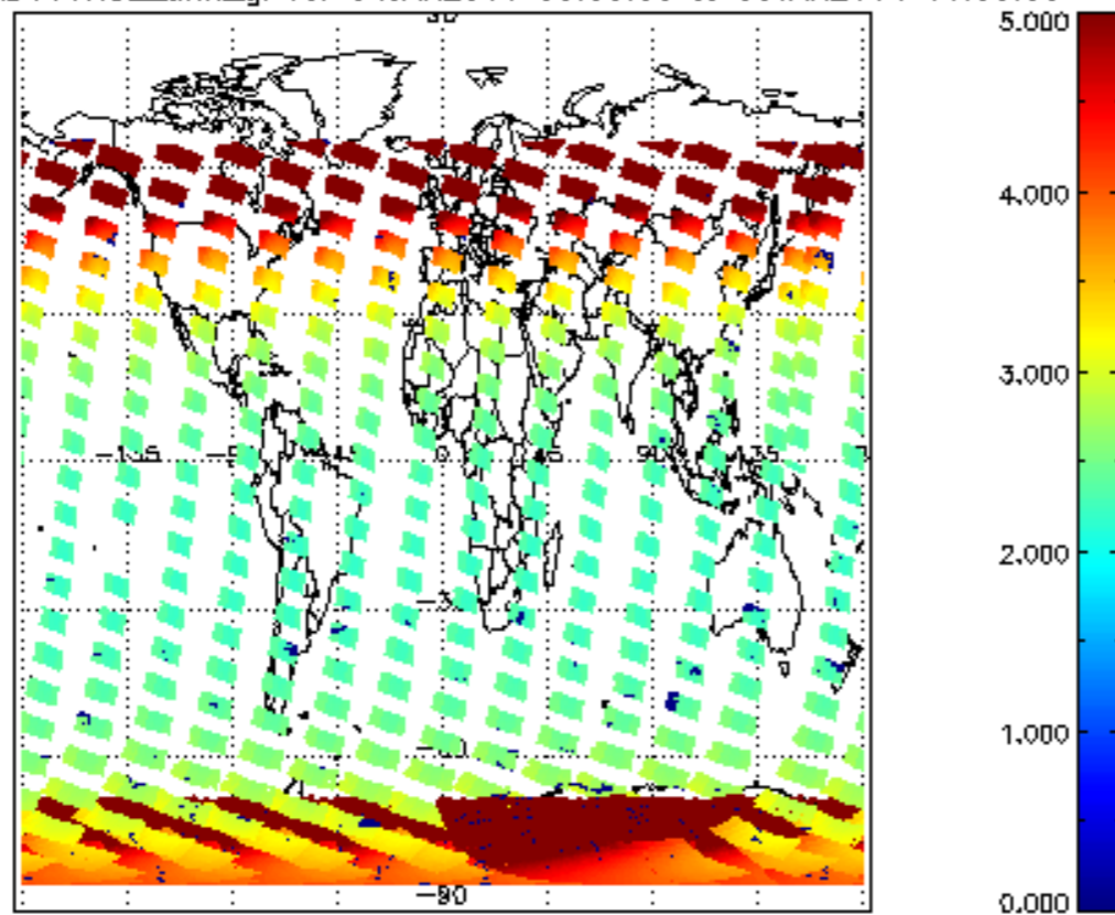
SCIOL2P_NADUV1NO2_amf_gr for 04JAN2011 00:00:00 to 05JAN2011 00:00:00
