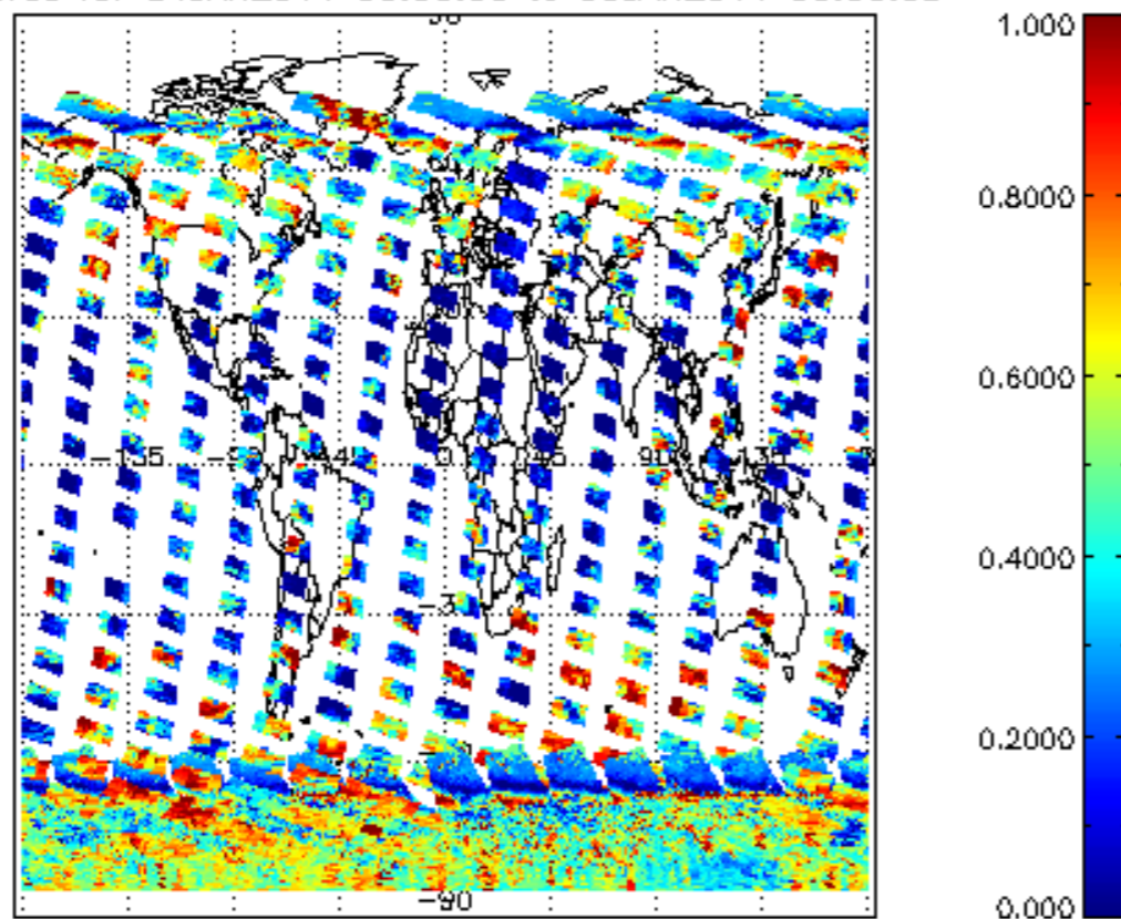
cL_frac for 04JAN2011 00:00:00 to 05JAN2011 00:00:00
