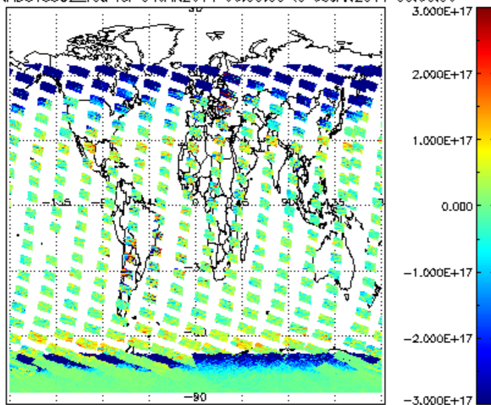
SCIOL2P_NADUV5S02_vcd for 04JAN2011 00:00:00 to 05JAN2011 00:00:00
