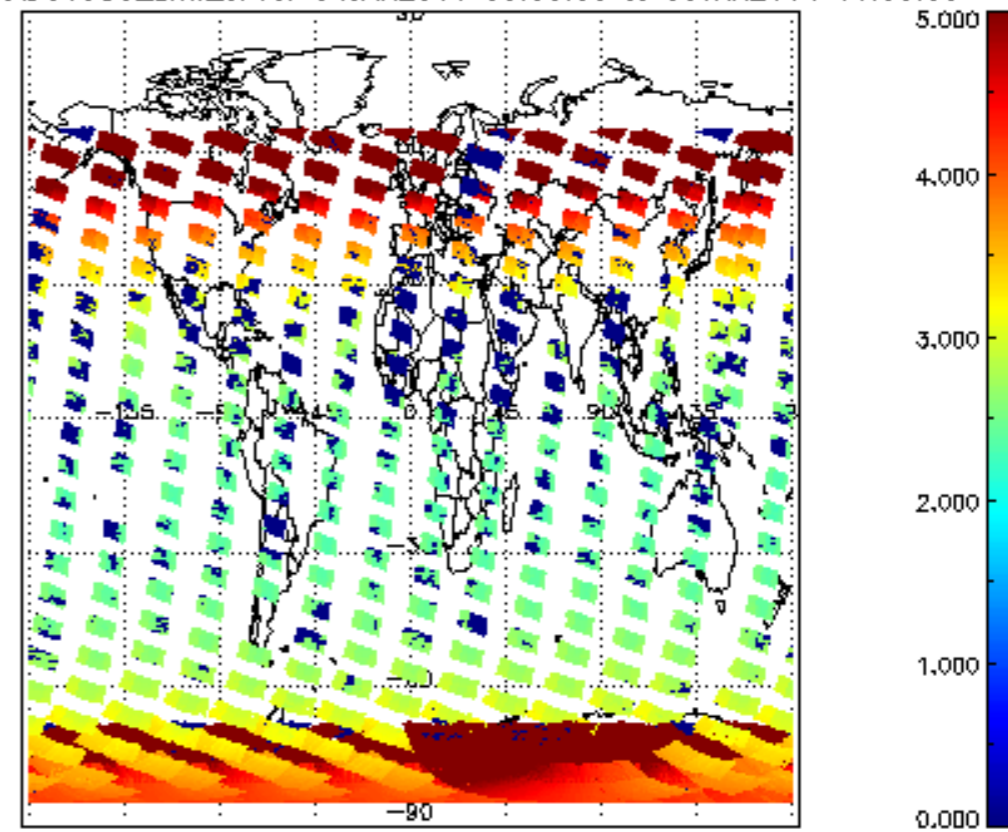
SCIOL2P_NADUV003_amf_cl for 04JAN2011 00:00:00 to 05JAN2011 00:00:00
