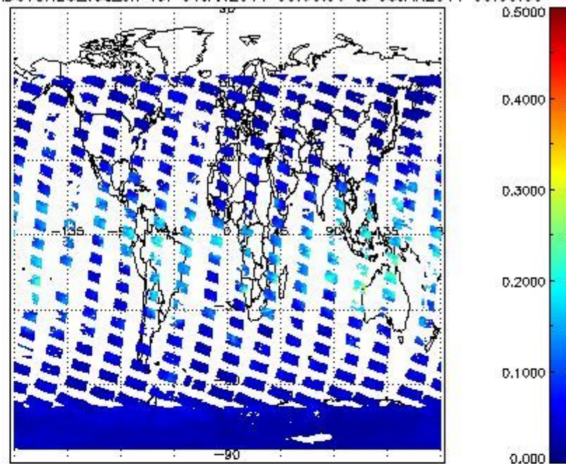
SCIOL2P_NADUV8H20_vcd_err for 04JAN2011 00:00:00 to 05JAN2011 00:00:00
