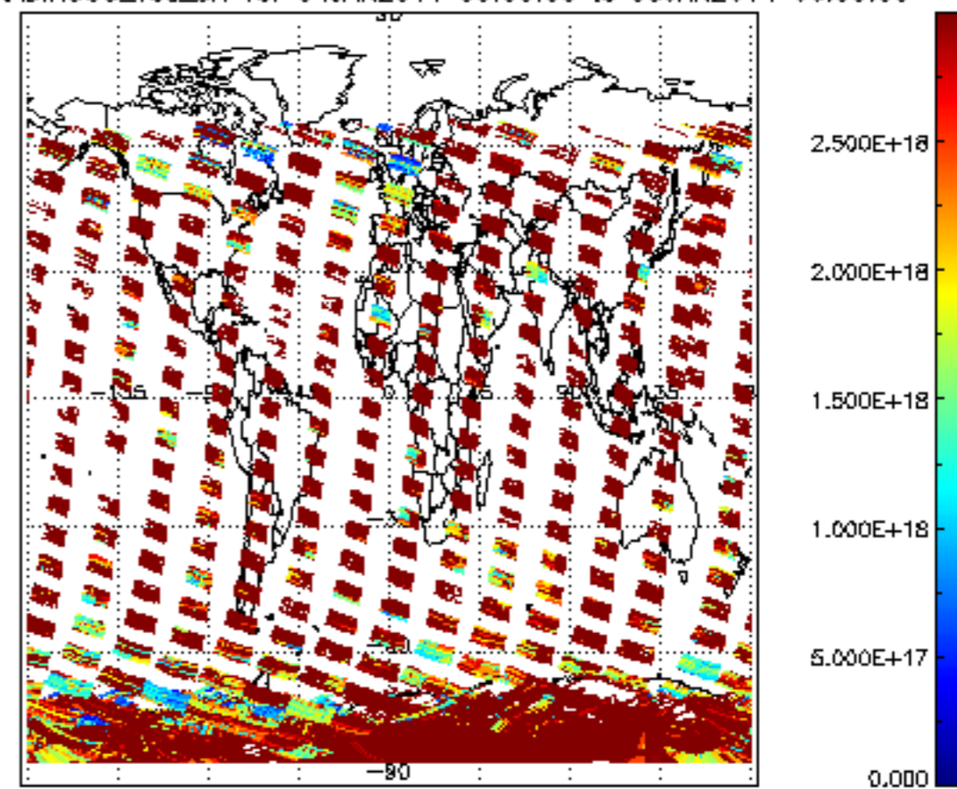
SCIOL2P_NADIR3CO_vcd_err for 04JAN2011 00:00:00 to 05JAN2011 00:00:00
