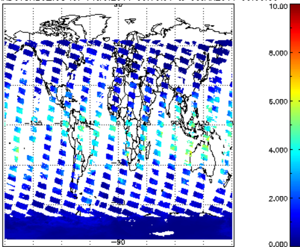
SCIOL2P_NADUVBH20_vcd for 04JAN2011 00:00:00 to 05JAN2011 00:00:00
