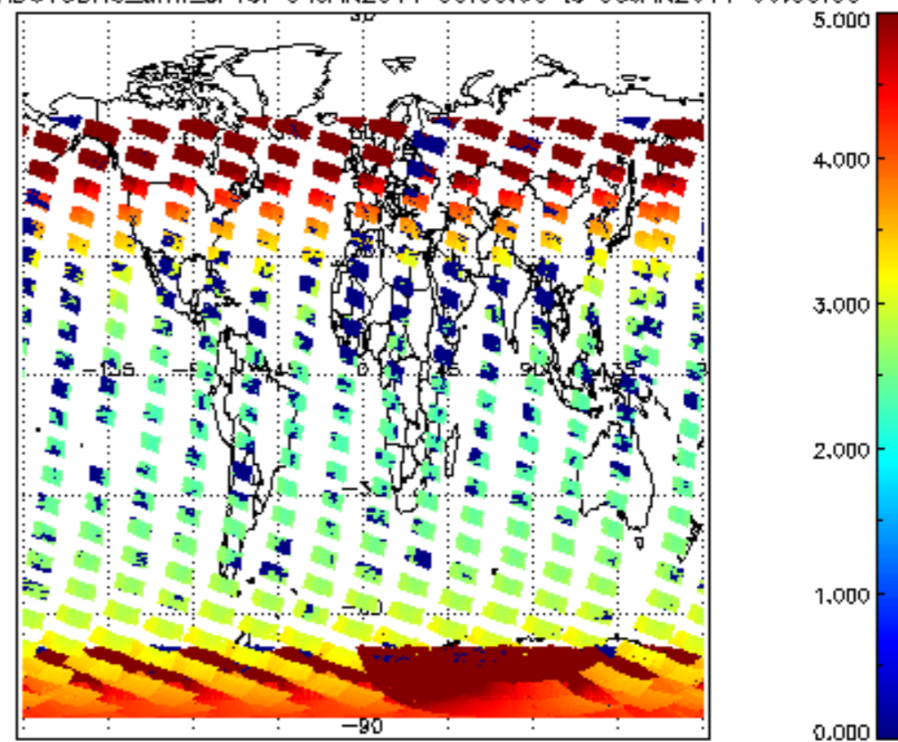
SCIOL2P_NADUV3BRO_amf_cl for 04JAN2011 00:00:00 to 05JAN2011 00:00:00
