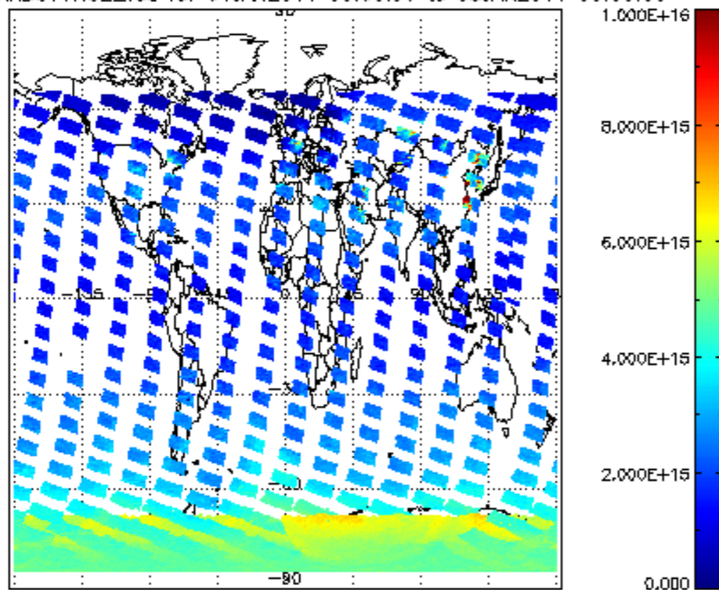
SCIOL2P_NADUV1NO2_vcd for 04JAN2011 00:00:00 to 05JAN2011 00:00:00
