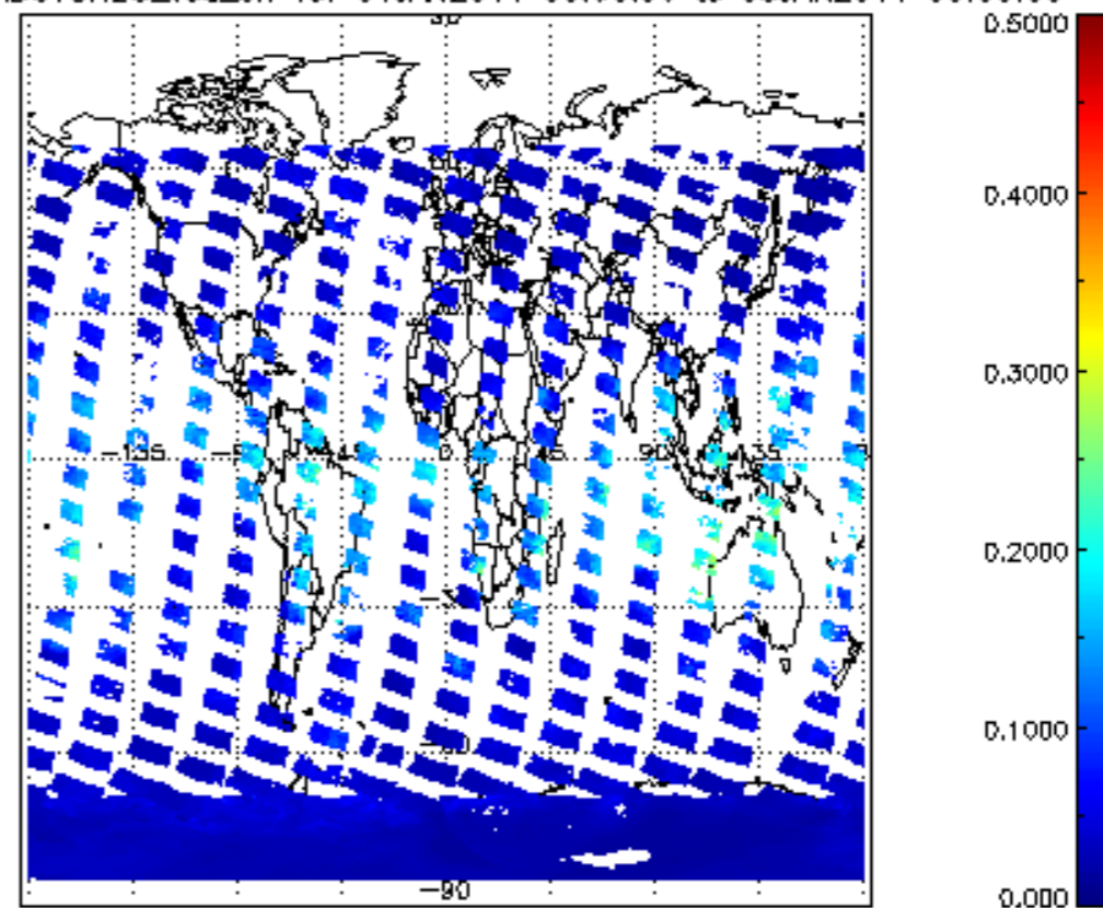
SCIOL2P_NADUVBH20_vcd_err for 04JAN2011 00:00:00 to 05JAN2011 00:00:00
