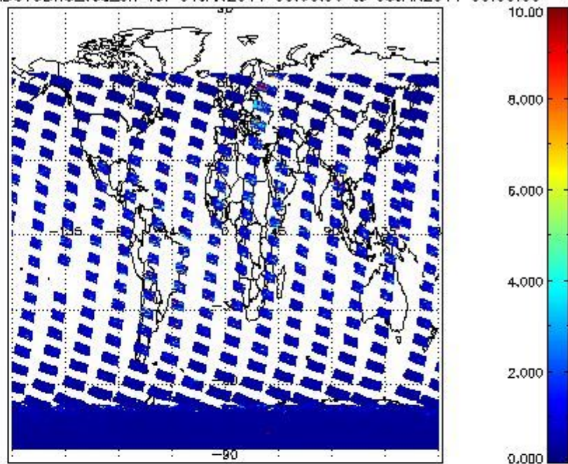
SCIOL2P_NADUV3BRO_vcd_err for 04JAN2011 00:00:00 to 05JAN2011 00:00:00
