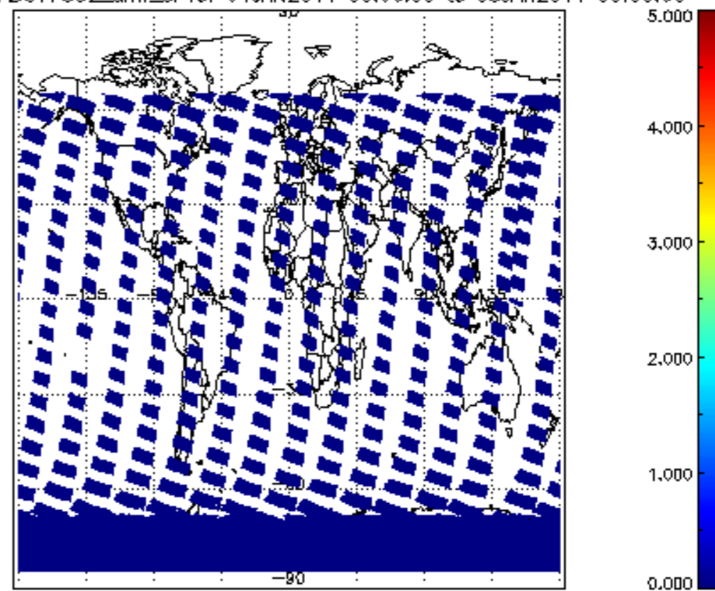
SCIOL2P_NADUV7S02_amf_cl for 04JAN2011 00:00:00 to 05JAN2011 00:00:00
