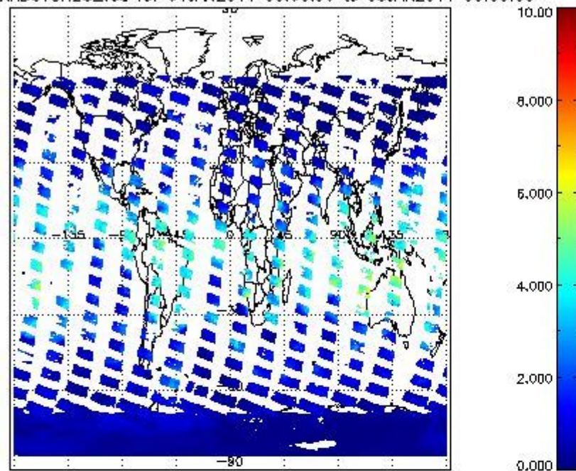
SCIOL2P_NADUV8H20_vcd for 04JAN2011 00:00:00 to 05JAN2011 00:00:00
