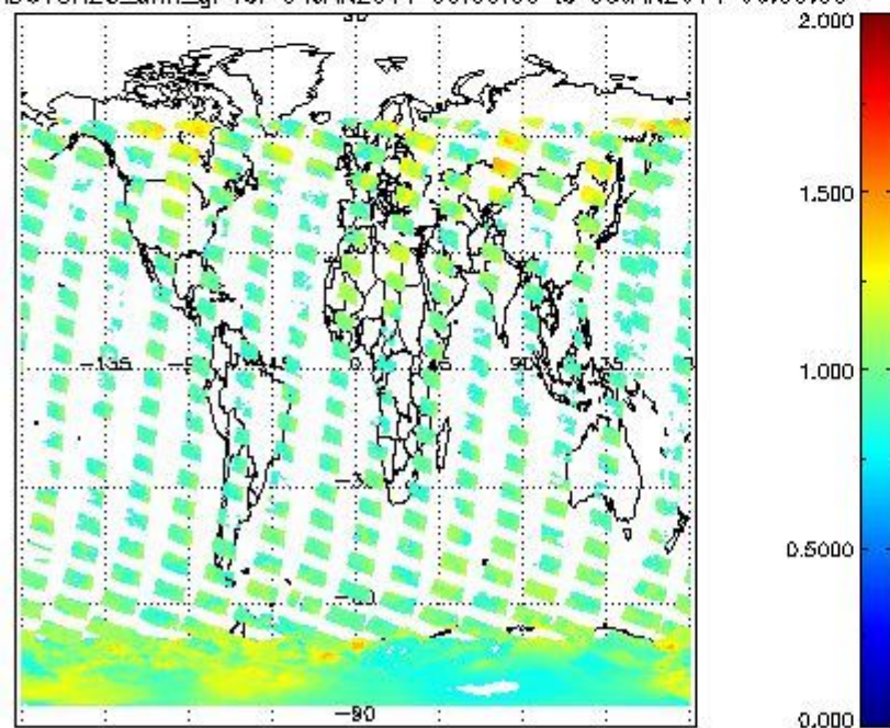
SCIOL2P_NADUV8H20_amf_gr for 04JAN2011 00:00:00 to 05JAN2011 00:00:00
