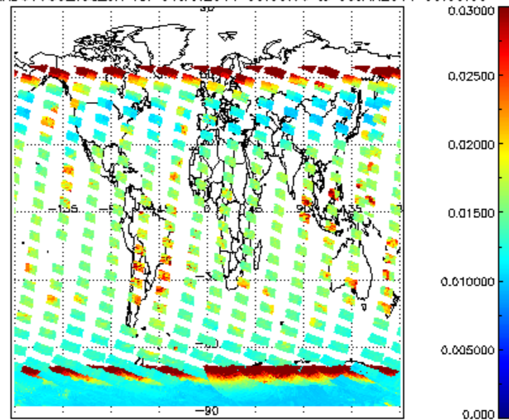
SCIOL2P_NADUV003_vcd_err for 04JAN2011 00:00:00 to 05JAN2011 00:00:00
