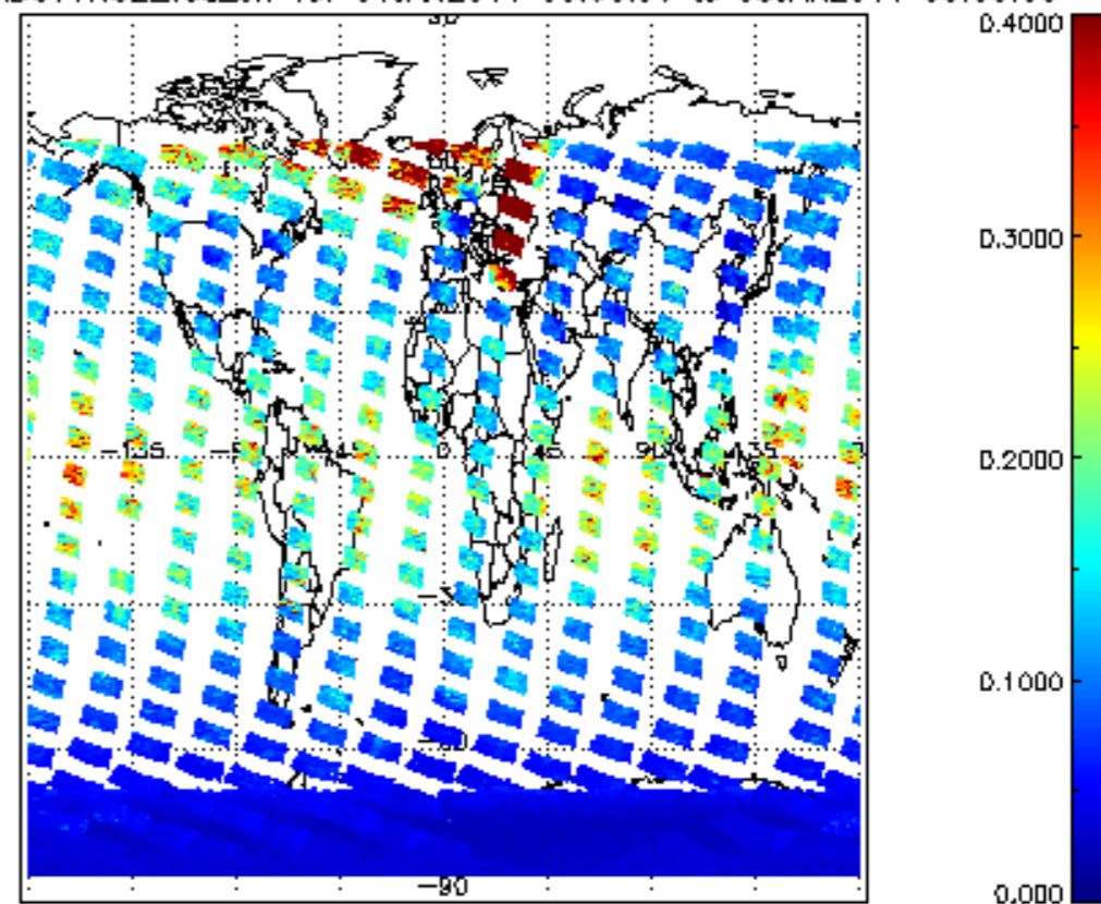
SCIOL2P_NADUV1NO2_vcd_err for 04JAN2011 00:00:00 to 05JAN2011 00:00:00
