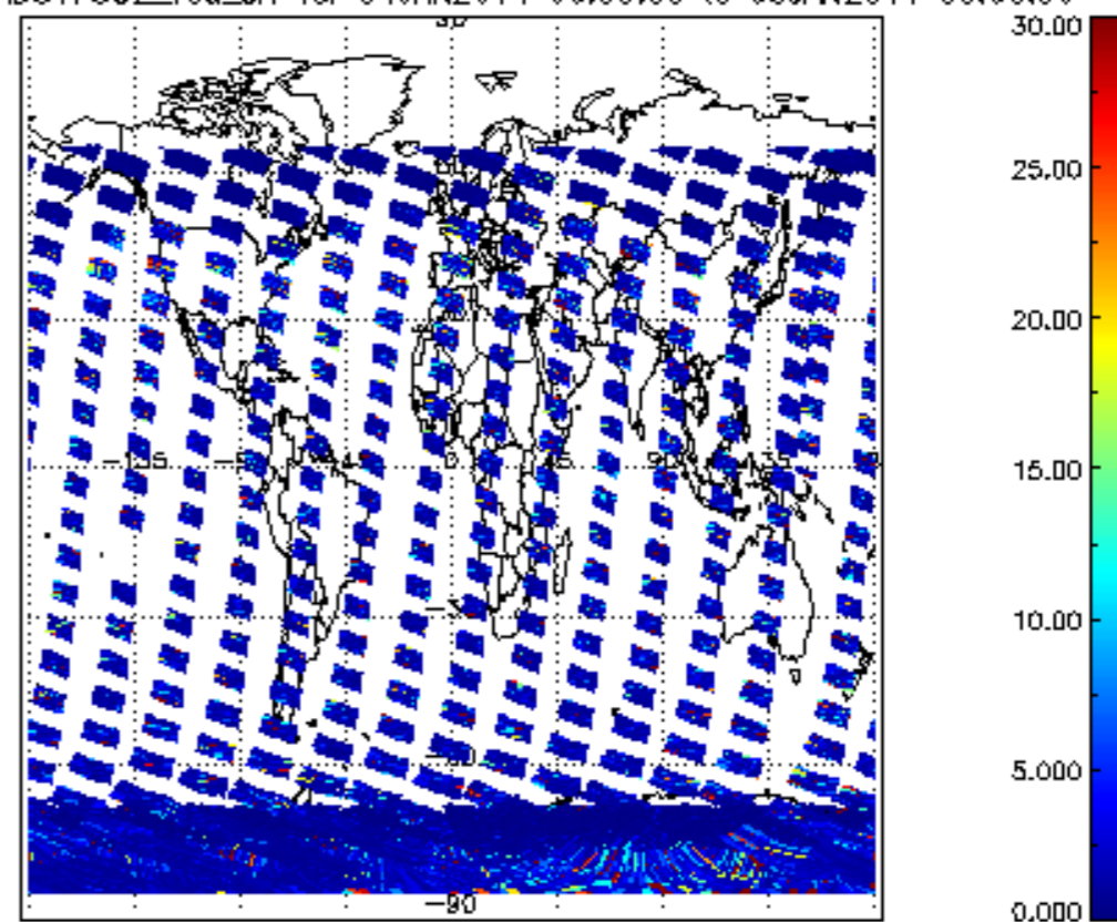
SCIOL2P_NADUV7S02_vcd_err for 04JAN2011 00:00:00 to 05JAN2011 00:00:00
