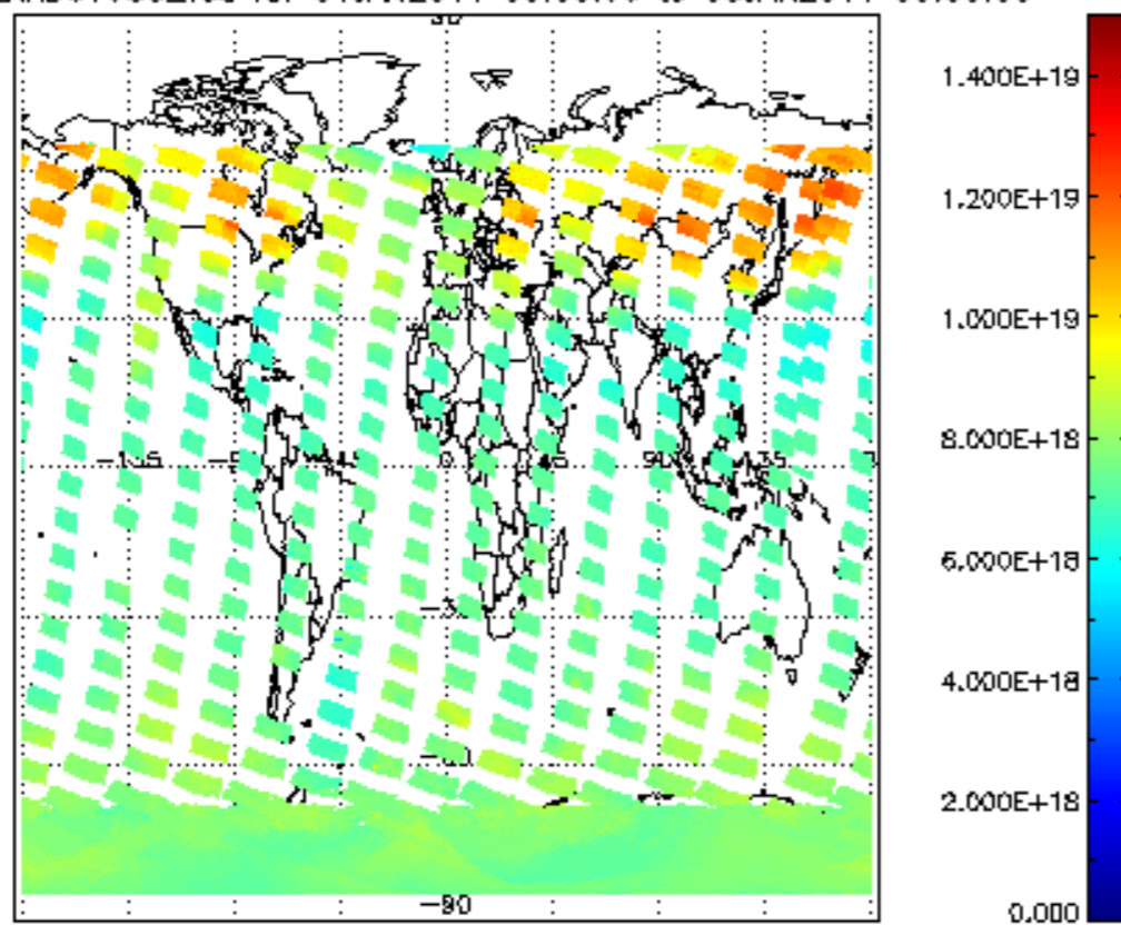
SCIOL2P_NADUV003_vcd for 04JAN2011 00:00:00 to 05JAN2011 00:00:00
