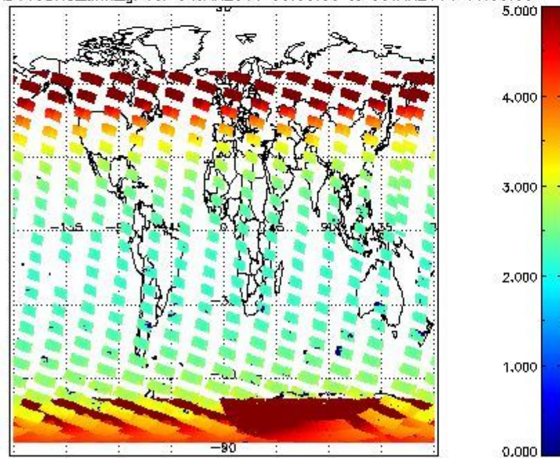
SCIOL2P_NADUV3BRO_amf_gr for 04JAN2011 00:00:00 to 05JAN2011 00:00:00
