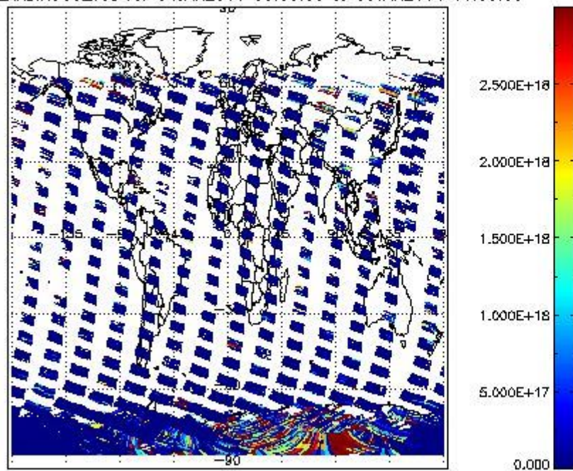
SCIDL2P_NADIR3CO_vcd for 04JAN2011 00:00:00 to 05JAN2011 00:00:00
