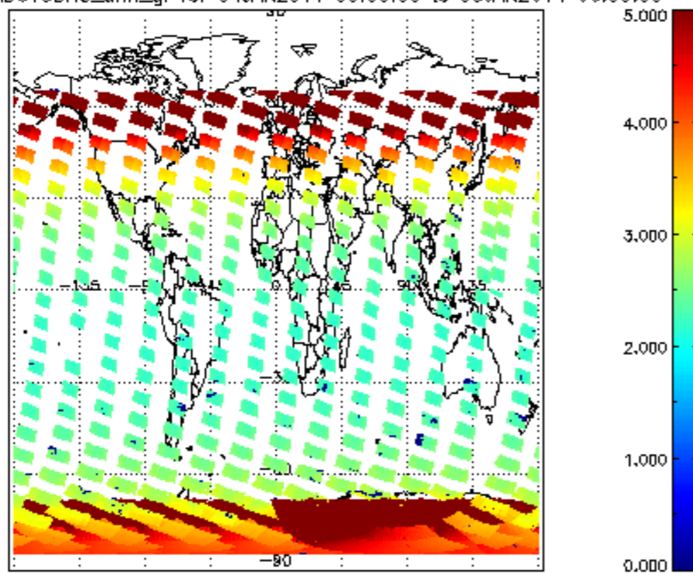
SCIOL2P_NADUV3BRO_amf_gr for 04JAN2011 00:00:00 to 05JAN2011 00:00:00
