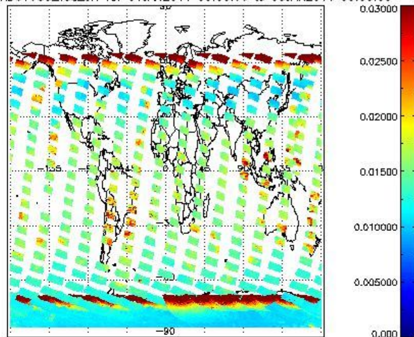
SCIOL2P_NADUV003_vcd_err for 04JAN2011 00:00:00 to 05JAN2011 00:00:00
