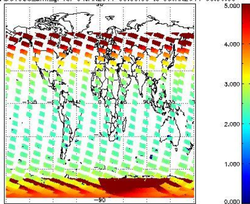
SCIOL2P_NADUV003_amf_gr for 04JAN2011 00:00:00 to 05JAN2011 00:00:00
