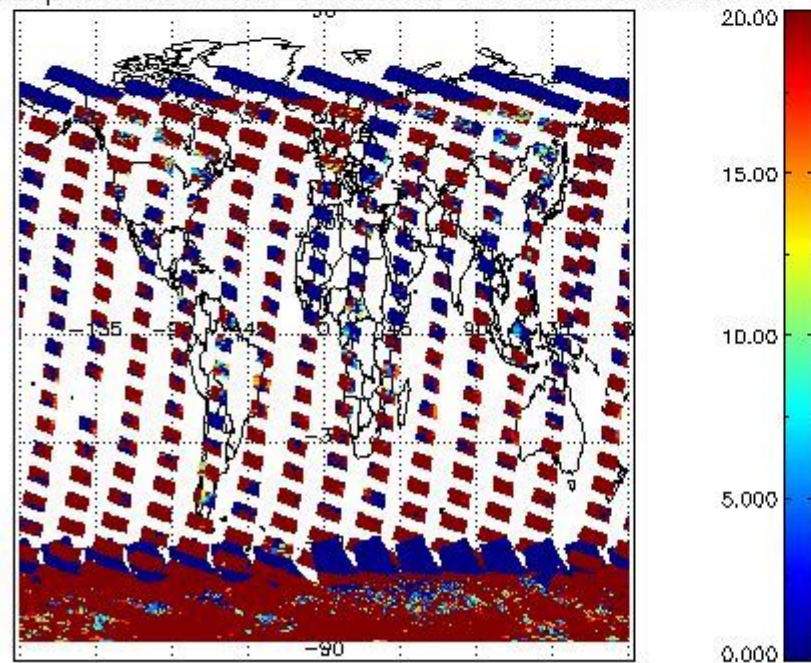
cLopt_depth for 04JAN2011 00:00:00 to 05JAN2011 00:00:00
