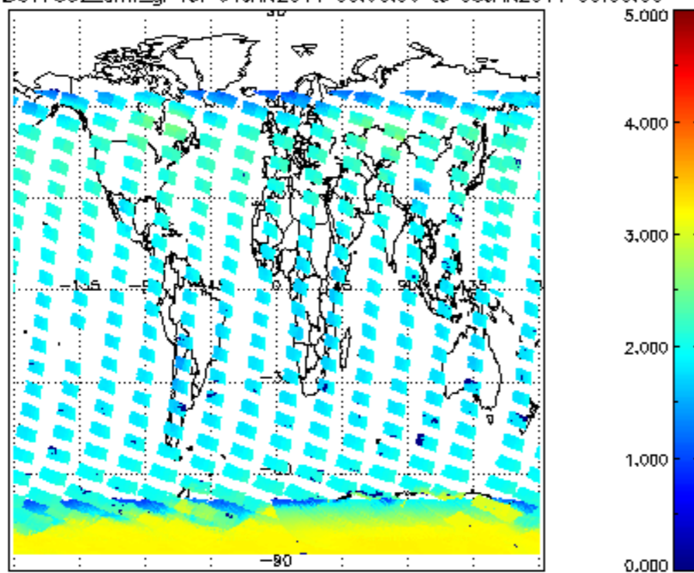
SCIOL2P_NADUV7S02_amf_gr for 04JAN2011 00:00:00 to 05JAN2011 00:00:00
