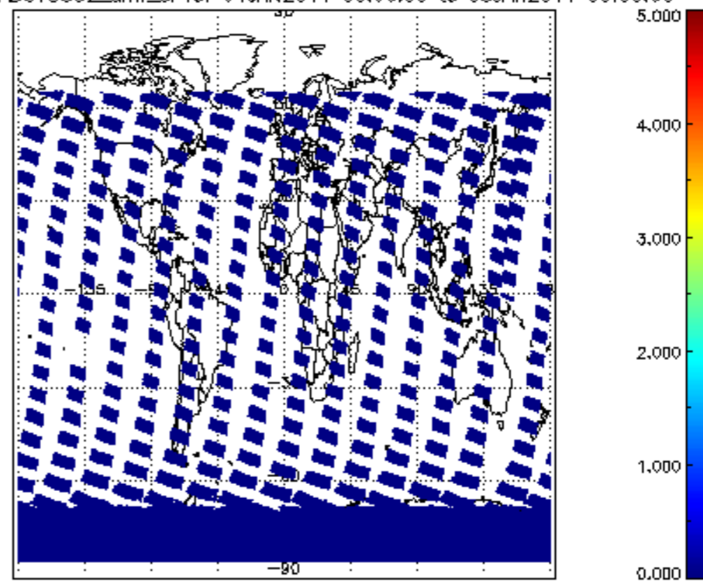
SCIOL2P_NADUV5S02_amf_sl for 04JAN2011 00:00:00 to 05JAN2011 00:00:00
