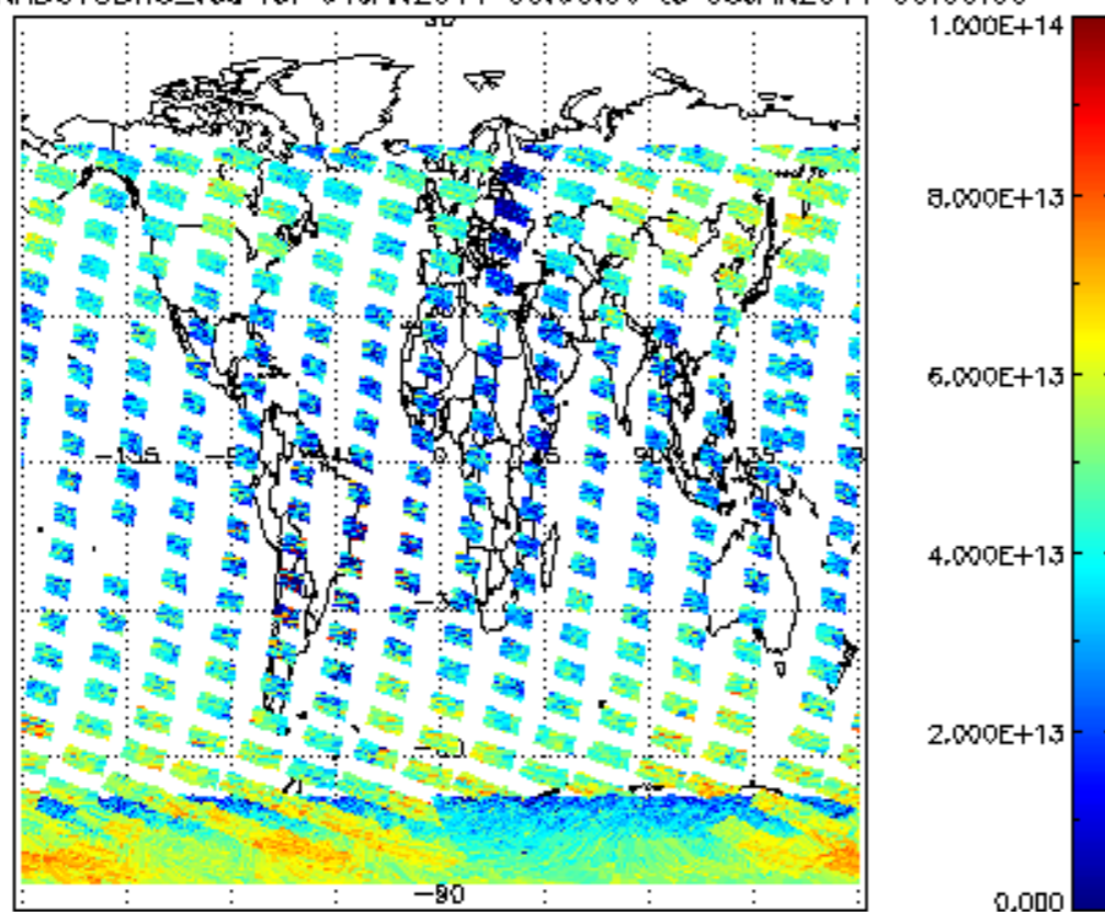
SCIOL2P_NADUV3BRO_vcd for 04JAN2011 00:00:00 to 05JAN2011 00:00:00
