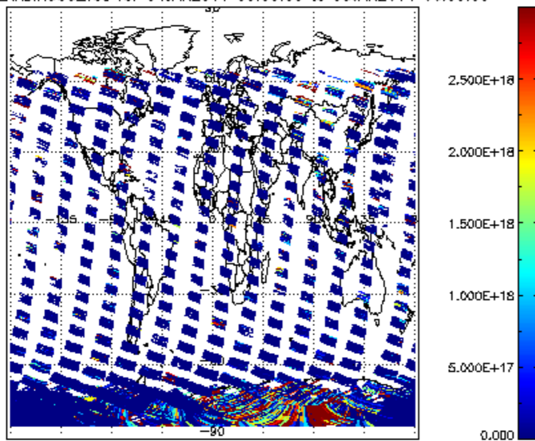
SCIOL2P_NADIR3CO_vcd for 04JAN2011 00:00:00 to 05JAN2011 00:00:00
