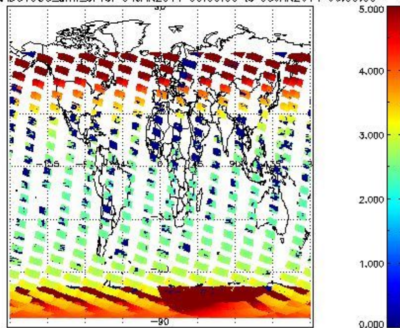
SCIOL2P_NADUV003_amf_cl for 04JAN2011 00:00:00 to 05JAN2011 00:00:00
