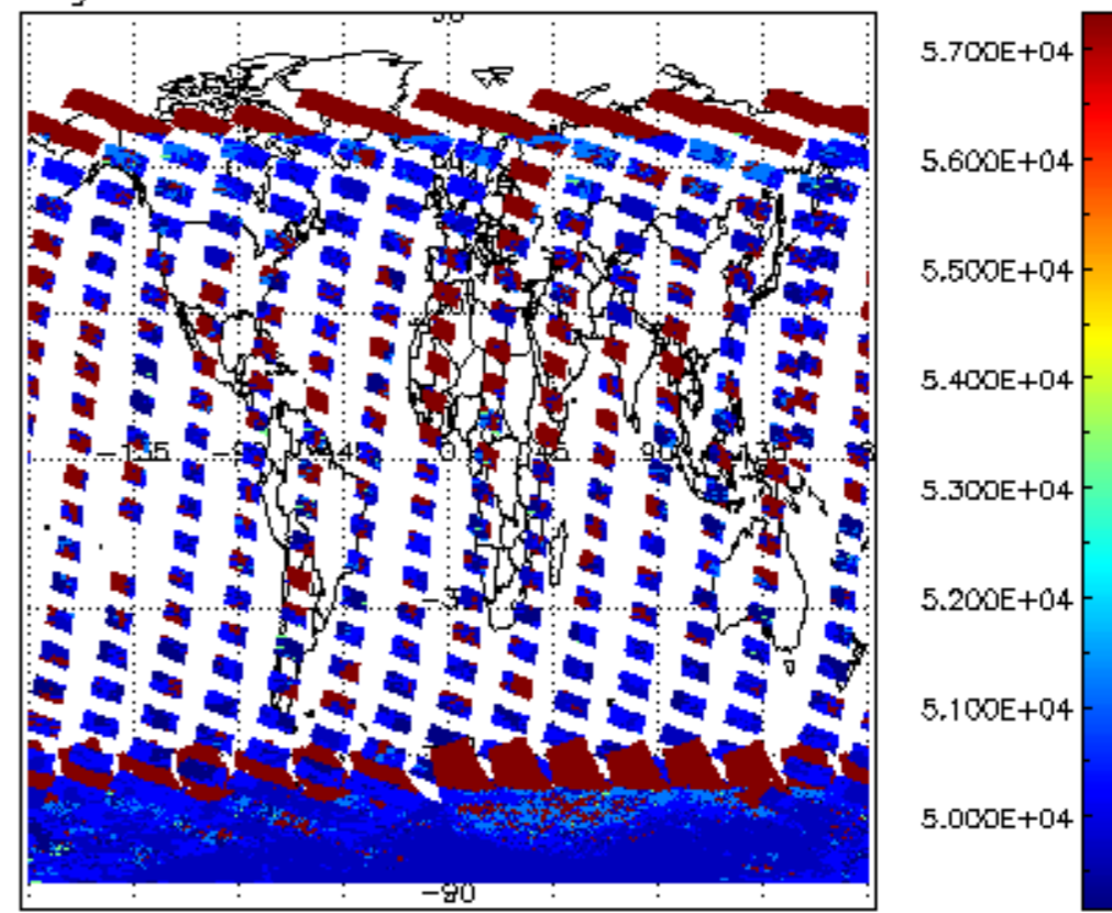
cloud_flags for 04JAN2011 00:00:00 to 05JAN2011 00:00:00
