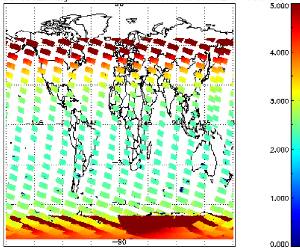
SCIOL2P_NADUV003_amf_gr for 04JAN2011 00:00:00 to 05JAN2011 00:00:00
