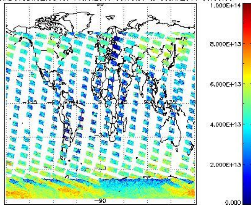
SCIOL2P_NADUV3BRO_vcd for 04JAN2011 00:00:00 to 05JAN2011 00:00:00
