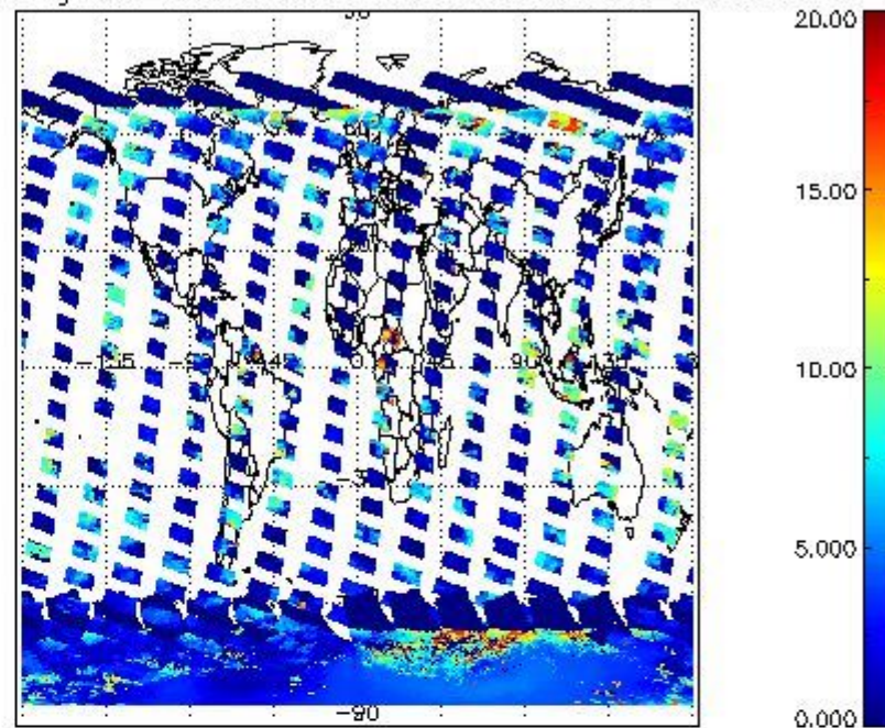
cL_top_height for 04JAN2011 00:00:00 to 05JAN2011 00:00:00
