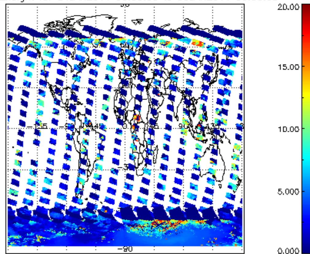
cL_top_height for 04JAN2011 00:00:00 to 05JAN2011 00:00:00
