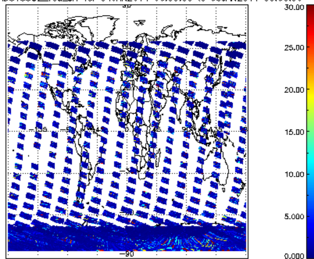
SCIOL2P_NADUV5S02_vcd_err for 04JAN2011 00:00:00 to 05JAN2011 00:00:00
