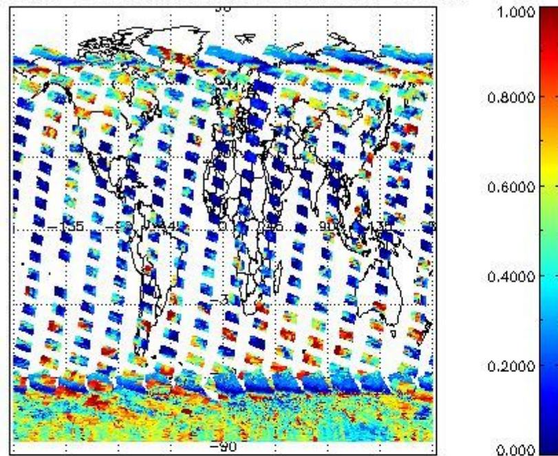
cL_frac for 04JAN2011 00:00:00 to 05JAN2011 00:00:00
