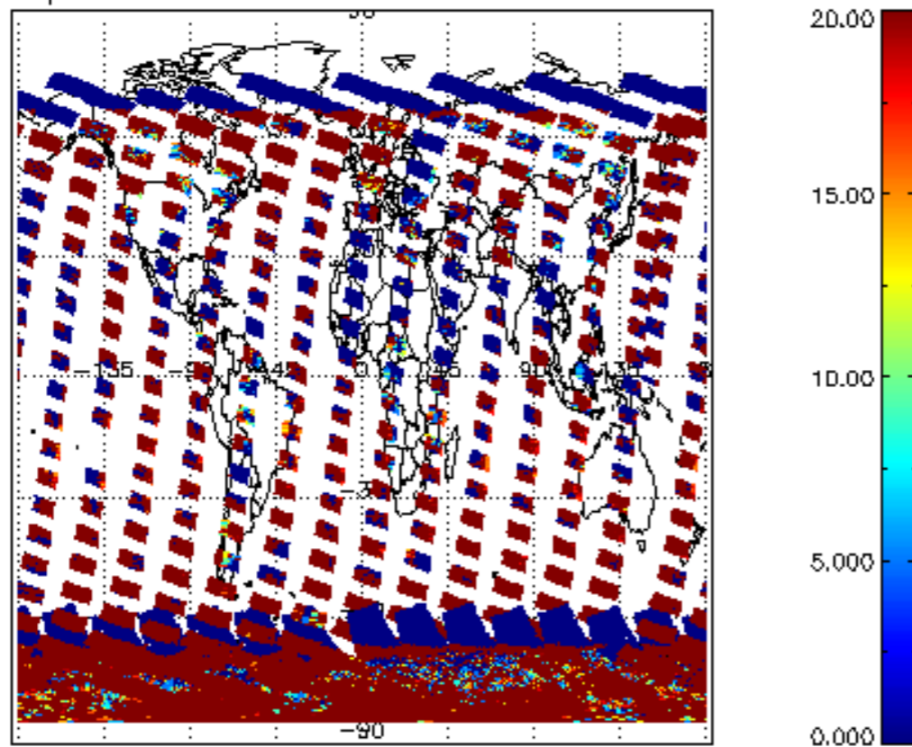
cLopt_depth for 04JAN2011 00:00:00 to 05JAN2011 00:00:00
