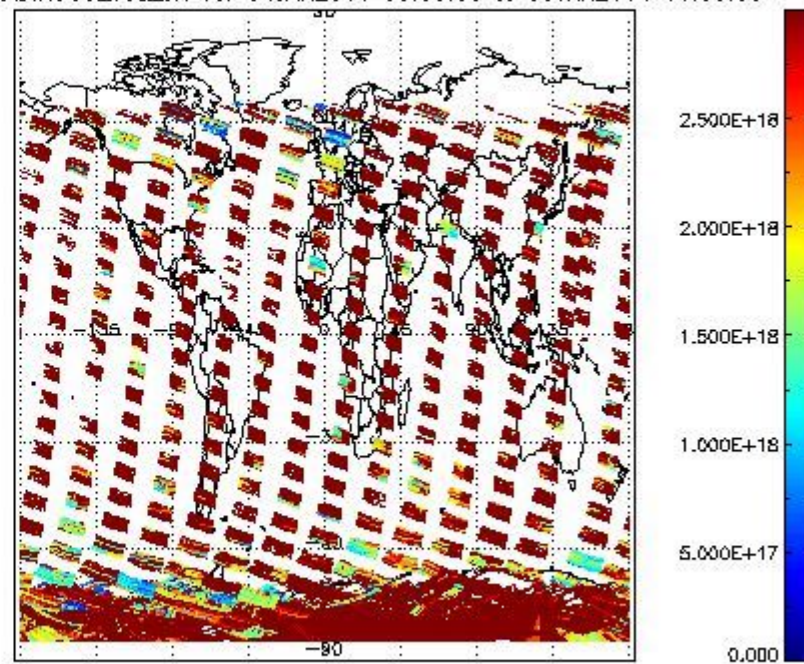
SCIDL2P_NADIR3CO_vcd_err for 04JAN2011 00:00:00 to 05JAN2011 00:00:00
