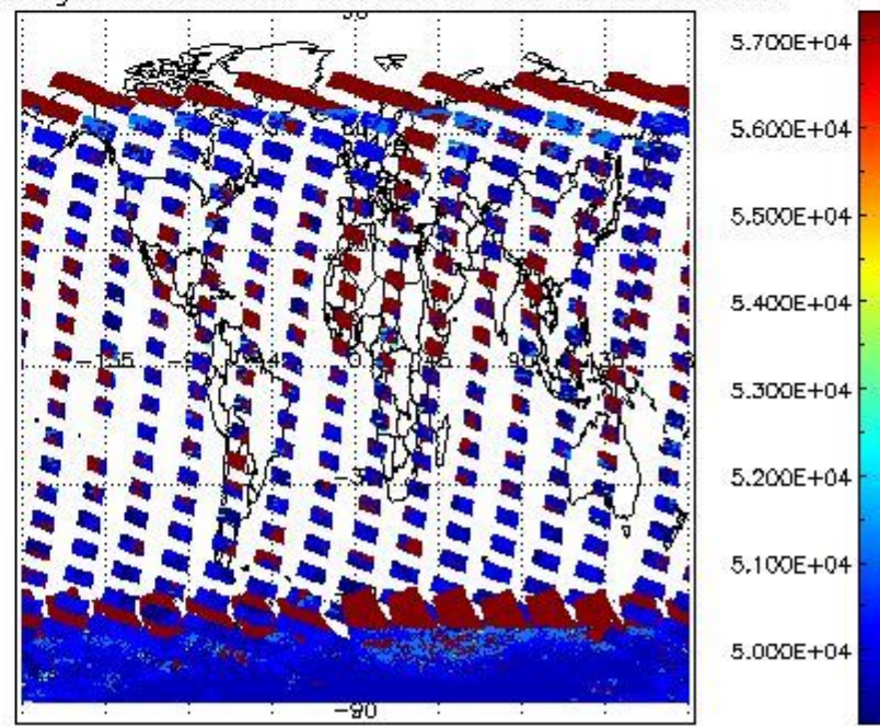
cloud_flags for 04JAN2011 00:00:00 to 05JAN2011 00:00:00
