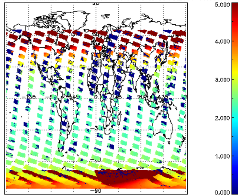
SCIOL2P_NADUV1NO2_amf_cl for 04JAN2011 00:00:00 to 05JAN2011 00:00:00
