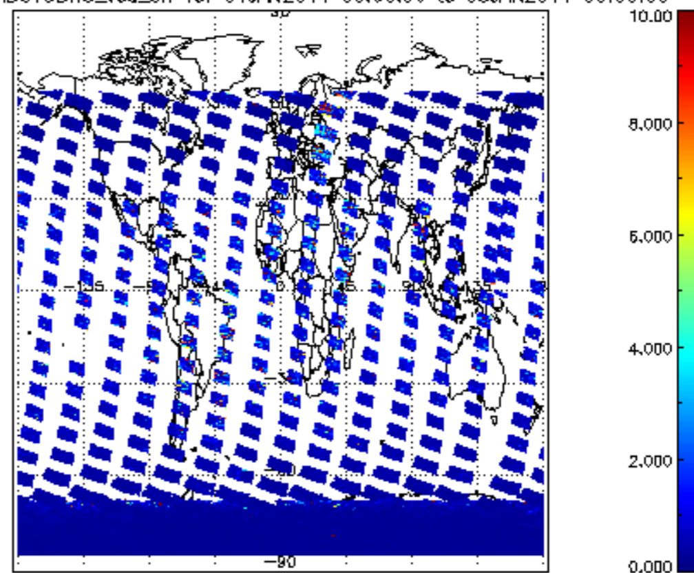
SCIOL2P_NADUV3BRO_vcd_err for 04JAN2011 00:00:00 to 05JAN2011 00:00:00
