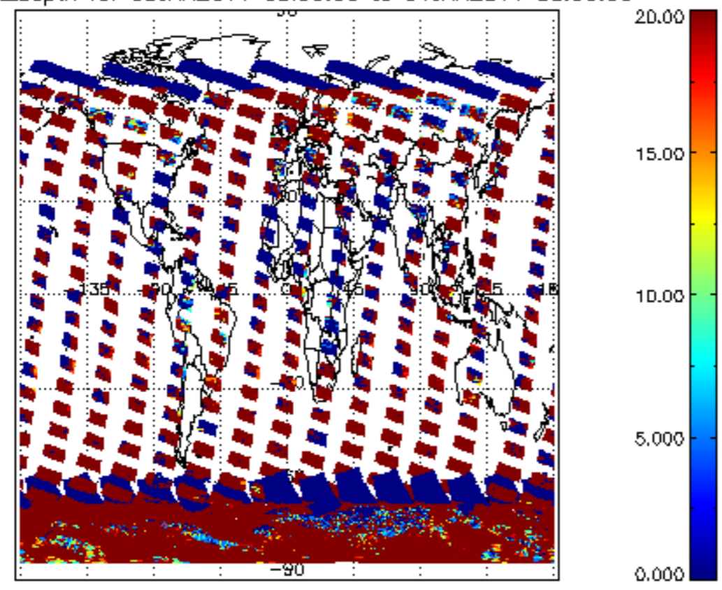
cLopt_depth for 03JAN2011 00:00:00 to 04JAN2011 00:00:00
