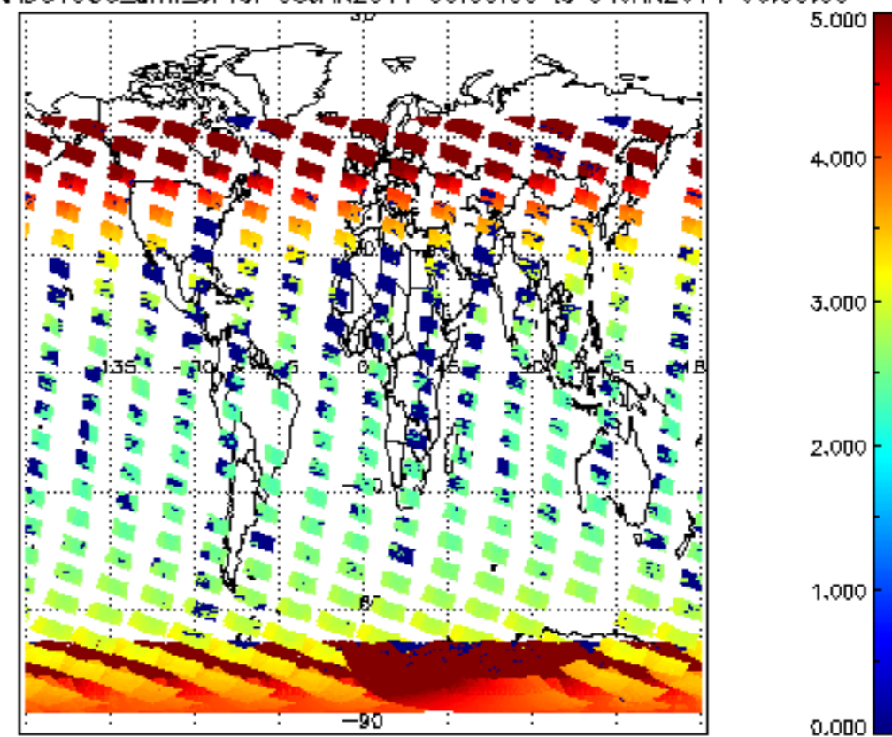
SCIOL2P_NADUV003_amf_cl for 03JAN2011 00:00:00 to 04JAN2011 00:00:00
