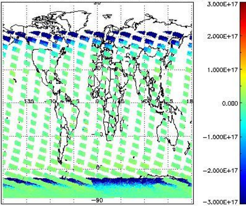
SCIOL2P_NADUV7S02_vcd for 03JAN2011 00:00:00 to 04JAN2011 00:00:00
