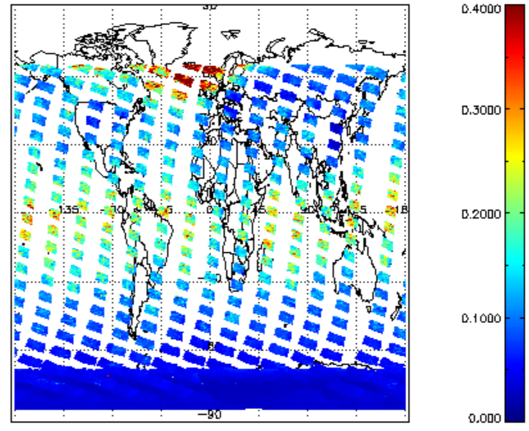
SCIOL2P_NADUV1NO2_vcd_err for 03JAN2011 00:00:00 to 04JAN2011 00:00:00
