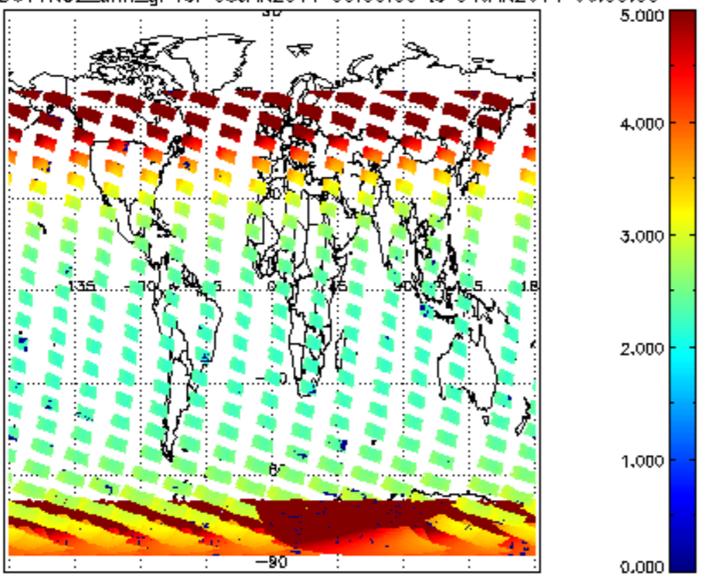
SCIOL2P_NADUV1NO2_amf_gr for 03JAN2011 00:00:00 to 04JAN2011 00:00:00
