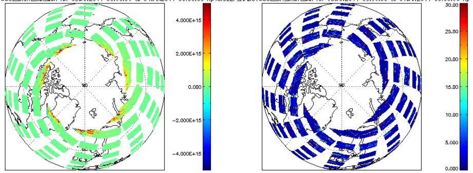
SCIOI2P_NADUV60CL_slant_col_den for 03JAN2011 00:00:00 to 04JAN2011 00:00:00 np; SCIOI2P_NADUV60CL_err_slant_col for 03JAN2011 00:00:00 to 04JAN2011 00:00:00 np
