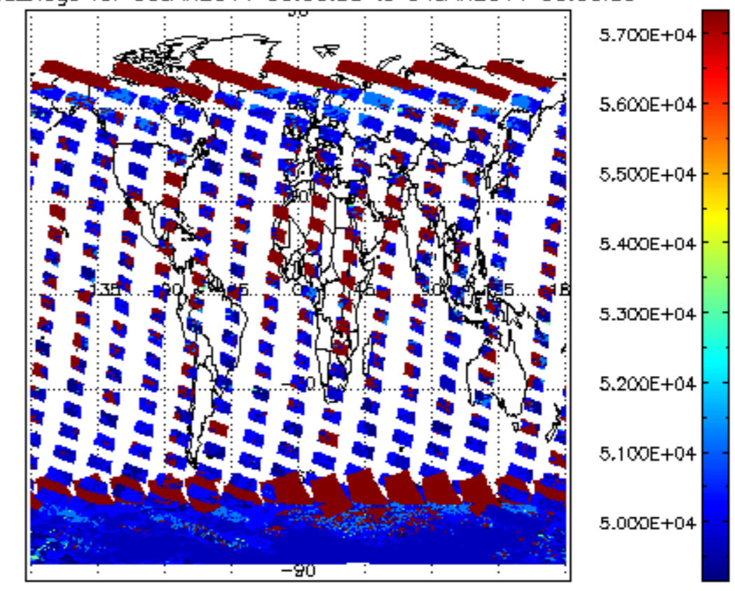
cloud_flags for 03JAN2011 00:00:00 to 04JAN2011 00:00:00
