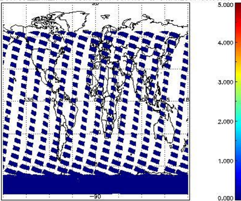
SCIOL2P_NADUV7S02_amf_cl for 03JAN2011 00:00:00 to 04JAN2011 00:00:00
