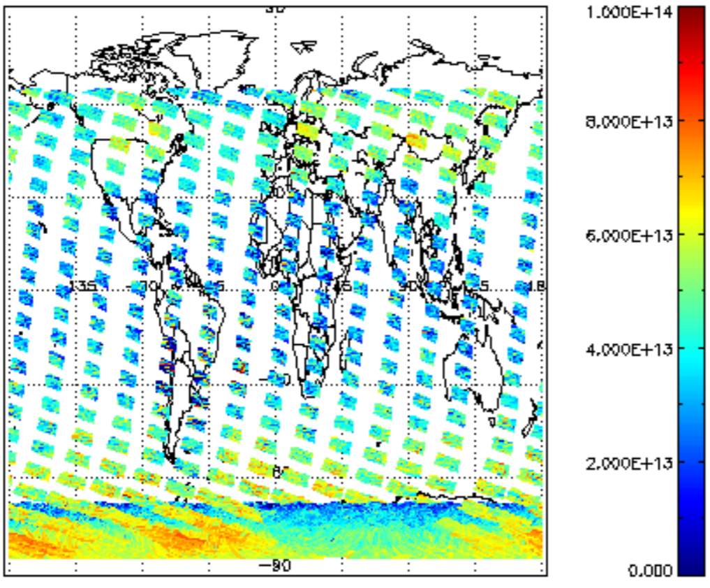
SCIOL2P_NADUV3BRO_vcd for 03JAN2011 00:00:00 to 04JAN2011 00:00:00
