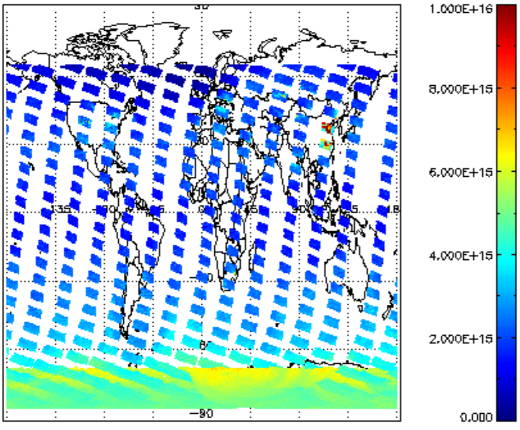
SCIOL2P_NADUV1NO2_vcd for 03JAN2011 00:00:00 to 04JAN2011 00:00:00
