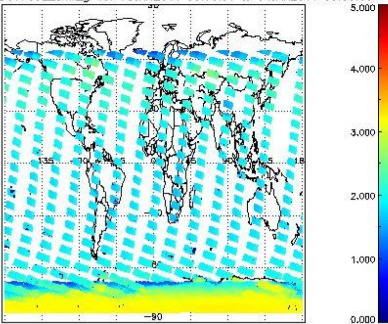
SCIOL2P_NADUV7S02_amf_gr for 03JAN2011 00:00:00 to 04JAN2011 00:00:00
