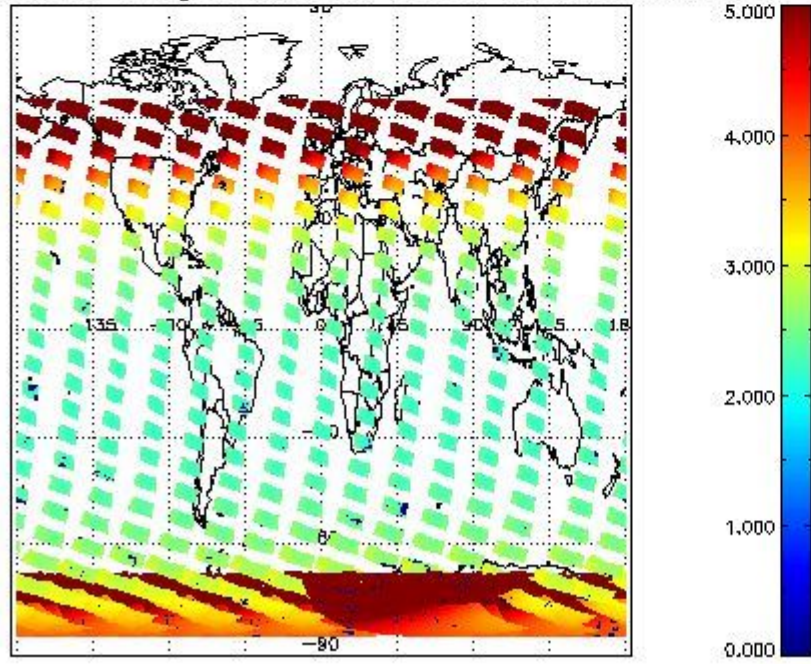
SCIOL2P_NADUV1NO2_amf_gr for 03JAN2011 00:00:00 to 04JAN2011 00:00:00
