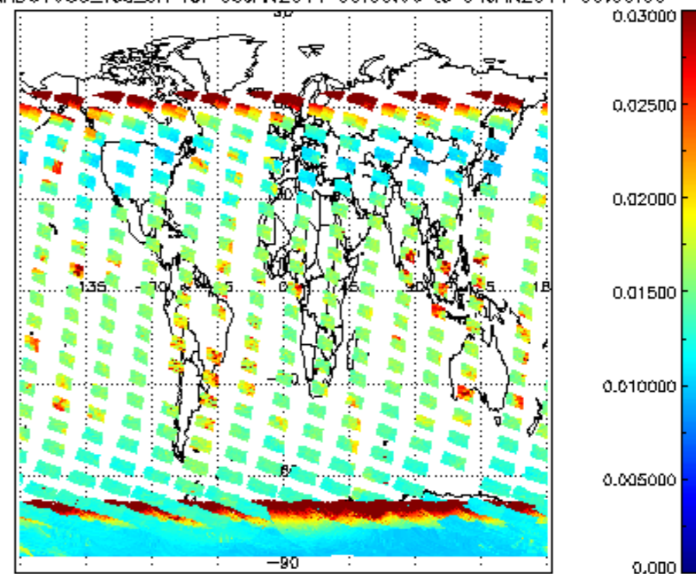
SCIOL2P_NADUV003_vcd_err for 03JAN2011 00:00:00 to 04JAN2011 00:00:00
