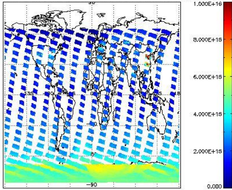
SCIOL2P_NADUV1NO2_vcd for 03JAN2011 00:00:00 to 04JAN2011 00:00:00
