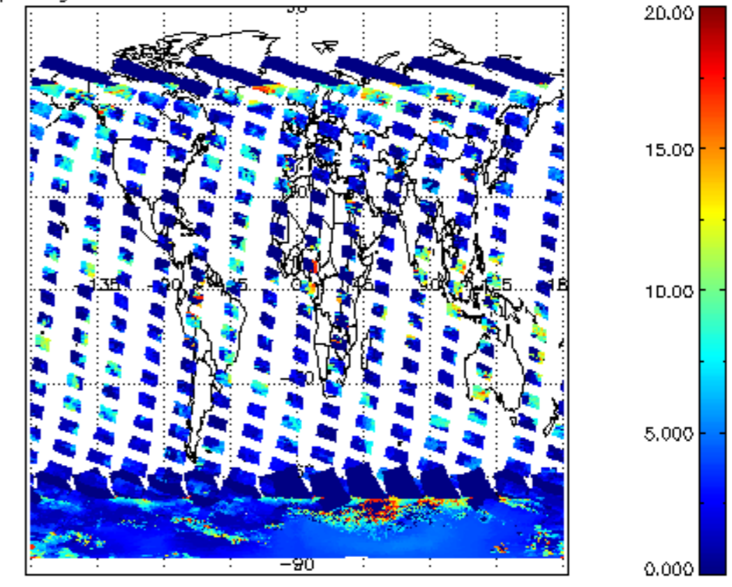
cL_top_height for 03JAN2011 00:00:00 to 04JAN2011 00:00:00
