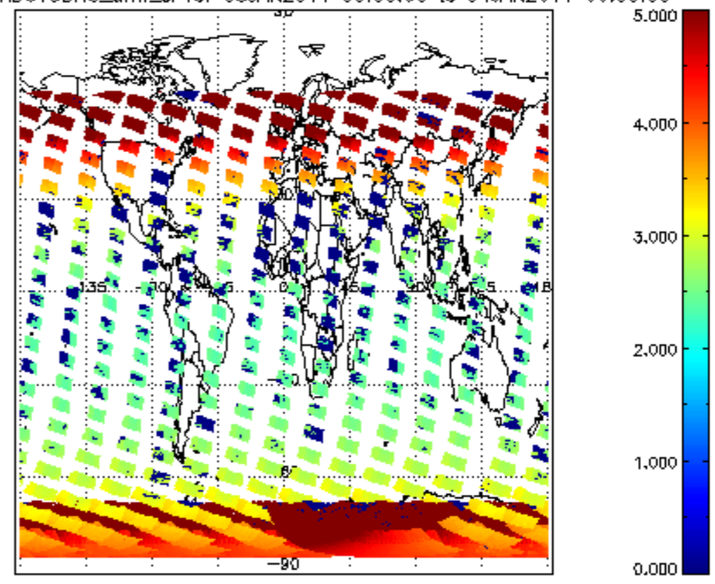
SCIOL2P_NADUV3BRO_amf_cl for 03JAN2011 00:00:00 to 04JAN2011 00:00:00
