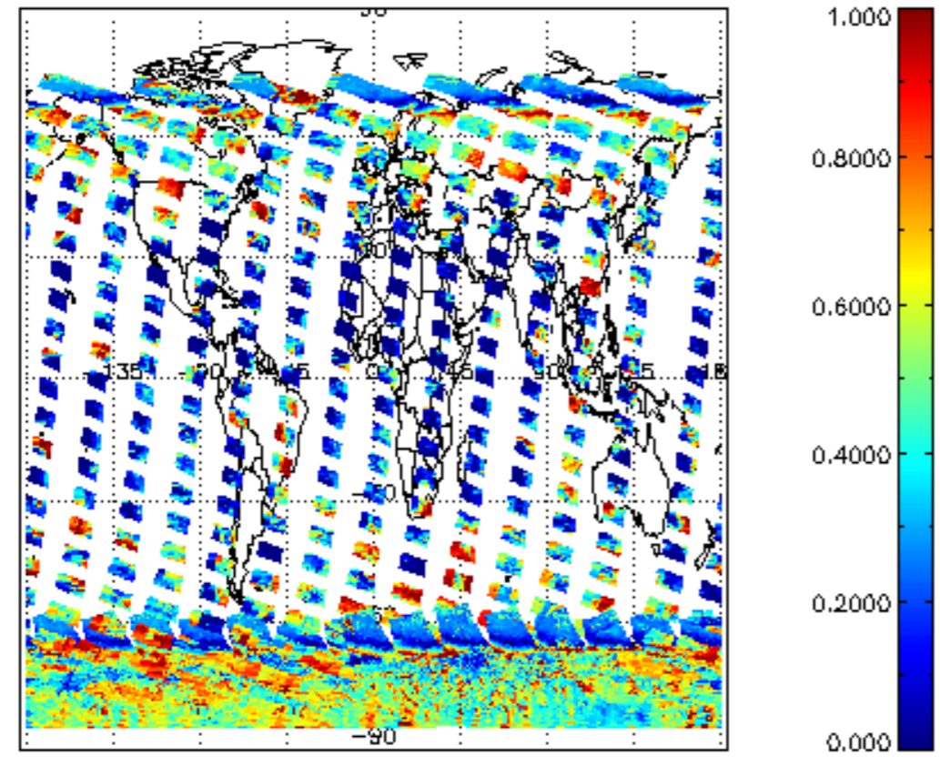
cL_frac for 03JAN2011 00:00:00 to 04JAN2011 00:00:00
