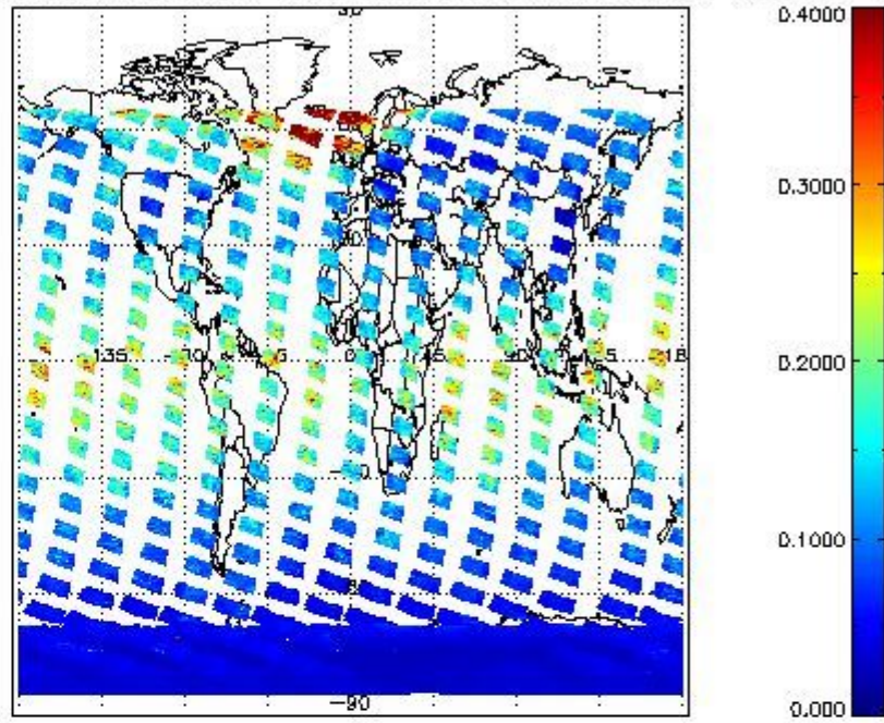
SCIOL2P_NADUV1NO2_vcd_err for 03JAN2011 00:00:00 to 04JAN2011 00:00:00
