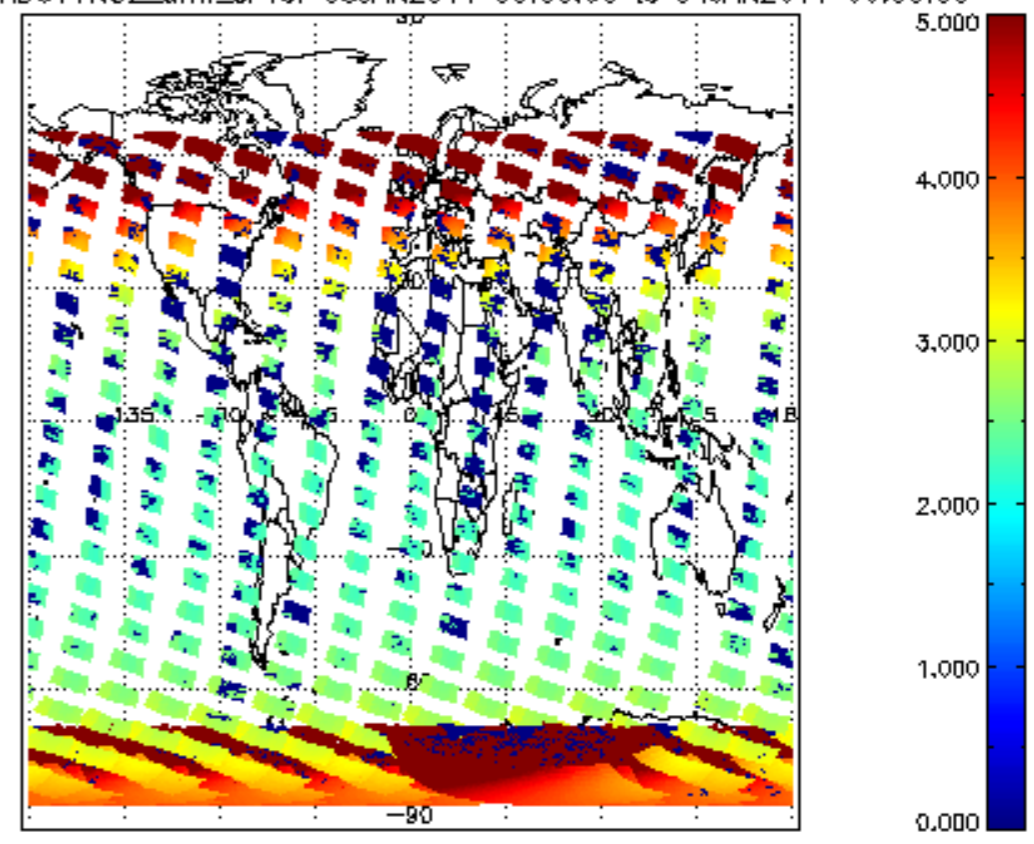
SCIOL2P_NADUV1NO2_amf_cl for 03JAN2011 00:00:00 to 04JAN2011 00:00:00
