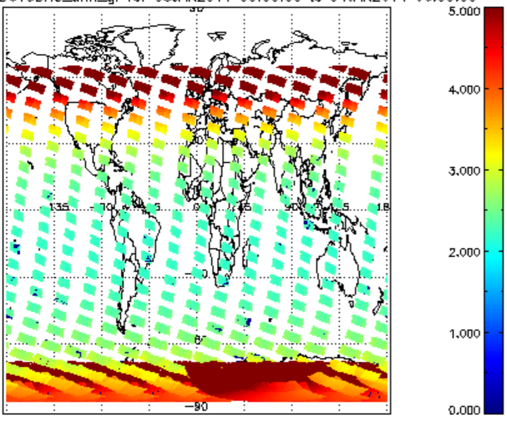
SCIOL2P_NADUV3BRO_amf_gr for 03JAN2011 00:00:00 to 04JAN2011 00:00:00
