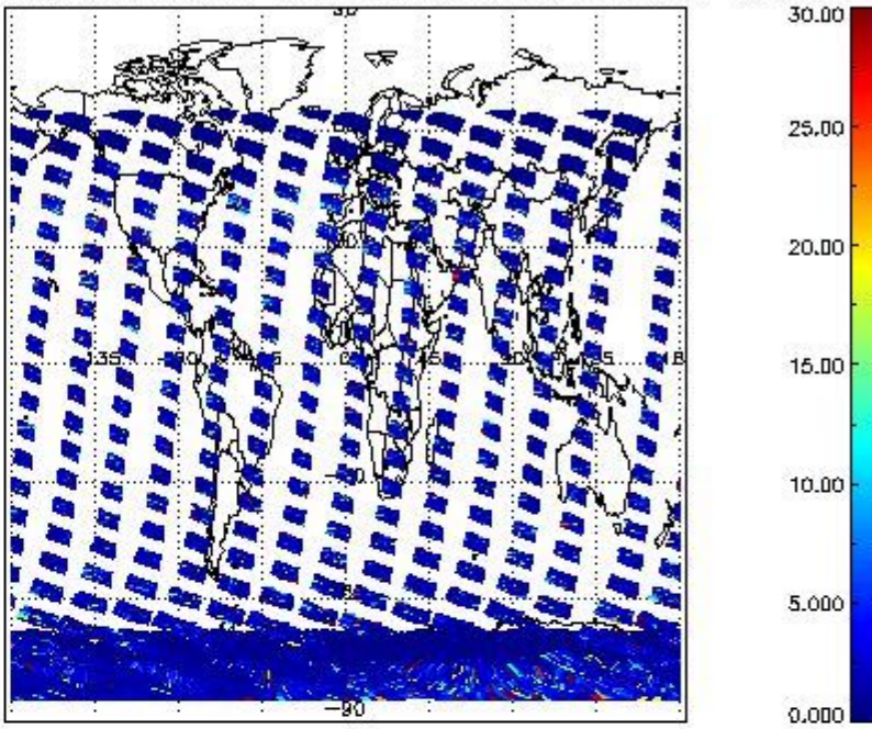
SCIOL2P_NADUV7S02_vcd_err for 03JAN2011 00:00:00 to 04JAN2011 00:00:00
