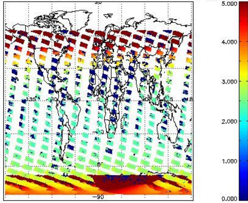
SCIOL2P_NADUV1NO2_amf_cl for 03JAN2011 00:00:00 to 04JAN2011 00:00:00
