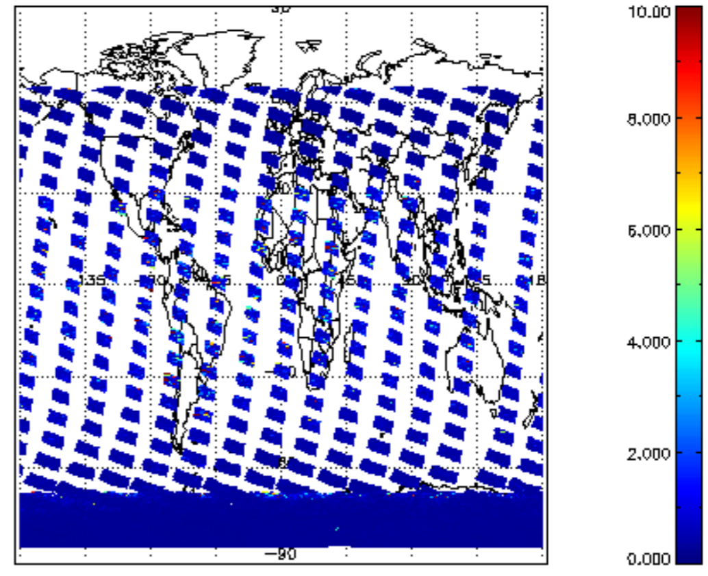
SCIOL2P_NADUV3BRO_vcd_err for 03JAN2011 00:00:00 to 04JAN2011 00:00:00
