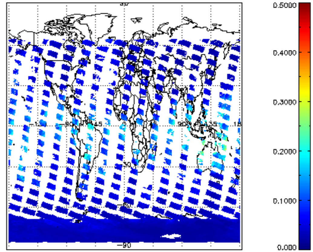
SCIOL2P_NADUV8H20_vcd_err for 02JAN2011 00:00:00 to 03JAN2011 00:00:00
