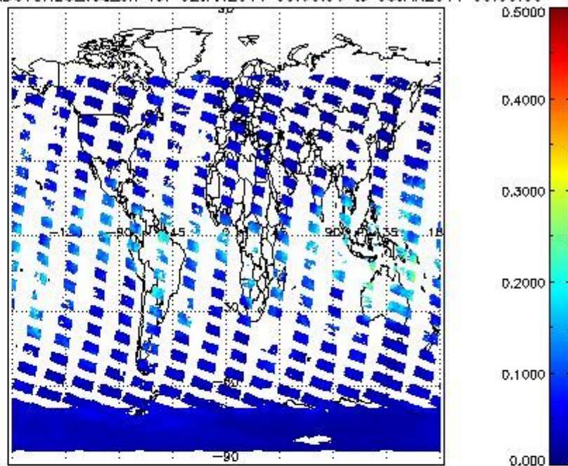
SCIOL2P_NADUV8H20_vcd_err for 02JAN2011 00:00:00 to 03JAN2011 00:00:00
