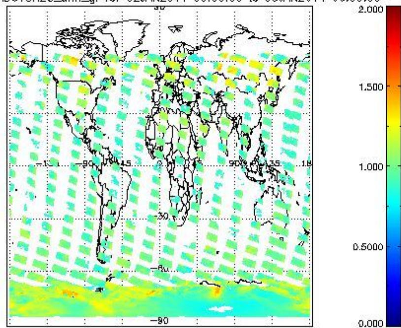
SCIOL2P_NADUV8H20_amf_gr for 02JAN2011 00:00:00 to 03JAN2011 00:00:00
