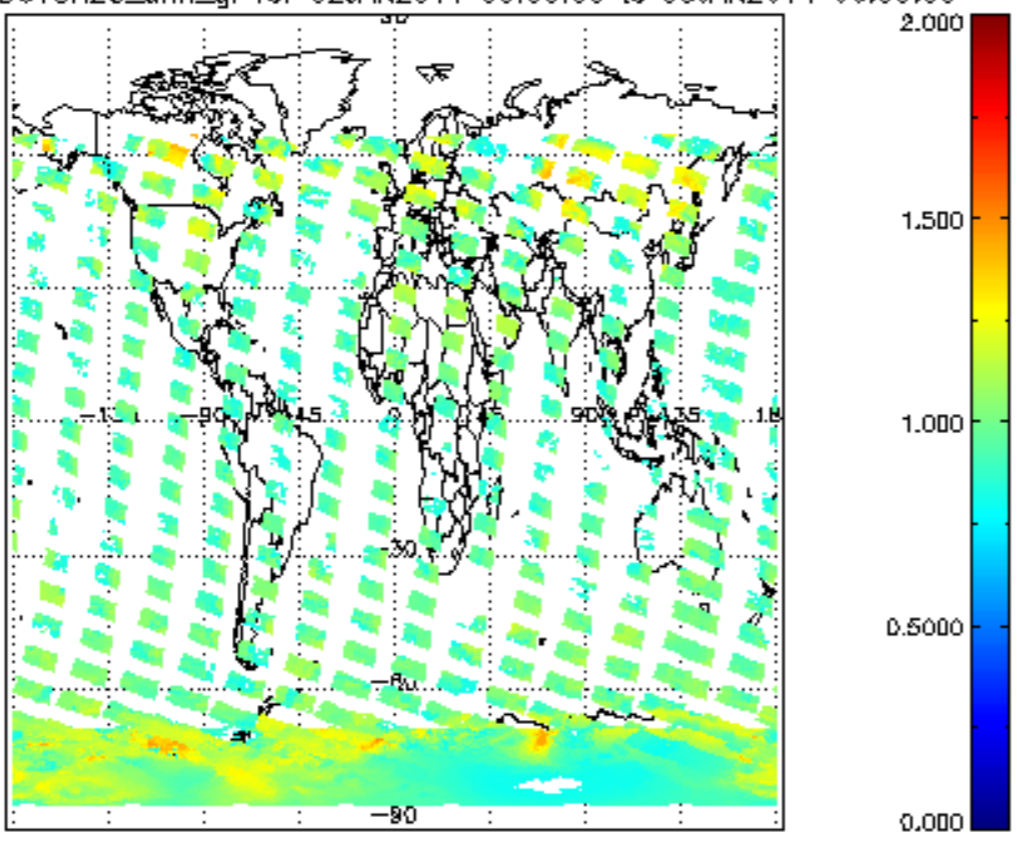
SCIOL2P_NADUV8H20_amf_gr for 02JAN2011 00:00:00 to 03JAN2011 00:00:00
