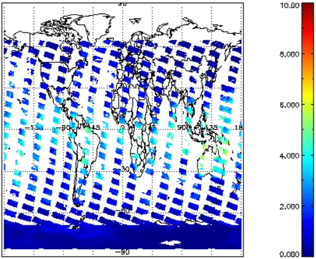
SCIOL2P_NADUV8H20_vcd for 02JAN2011 00:00:00 to 03JAN2011 00:00:00
