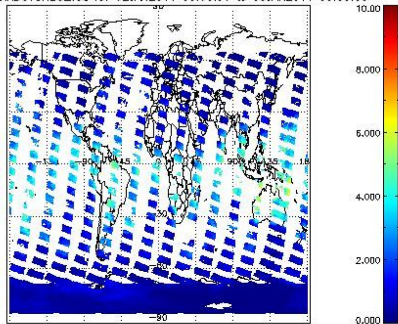
SCIOL2P_NADUV8H20_vcd for 02JAN2011 00:00:00 to 03JAN2011 00:00:00
