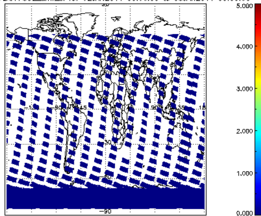
SCIOL2P_NADUV7S02_amf_cl for 02JAN2011 00:00:00 to 03JAN2011 00:00:00
