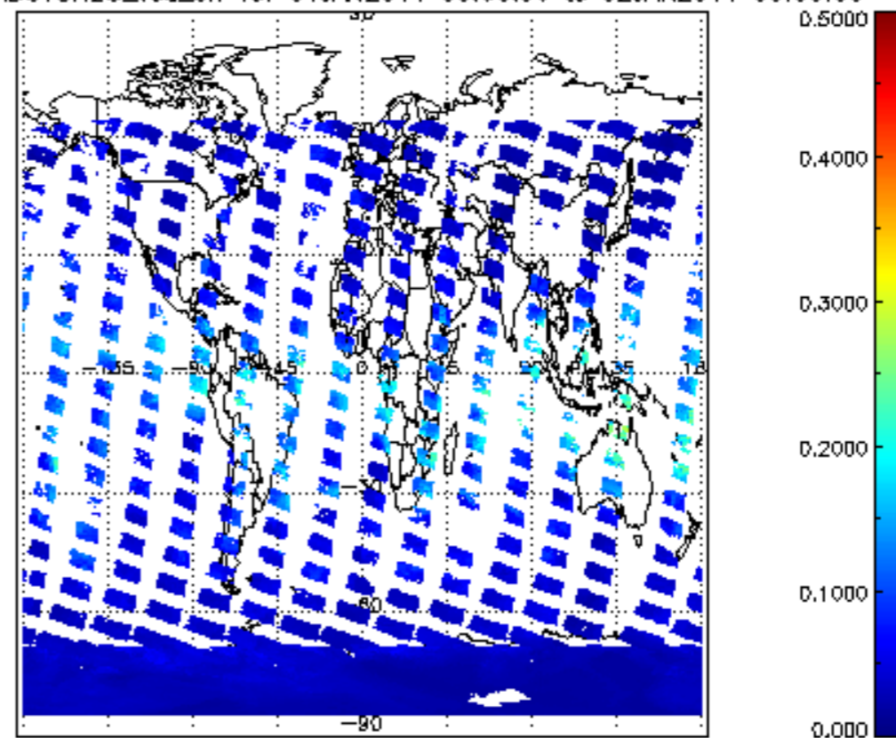
SCIOL2P_NADUV8H20_vcd_err for 01JAN2011 00:00:00 to 02JAN2011 00:00:00
