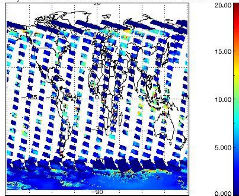
cL_top_height for 01JAN2011 00:00:00 to 02JAN2011 00:00:00
