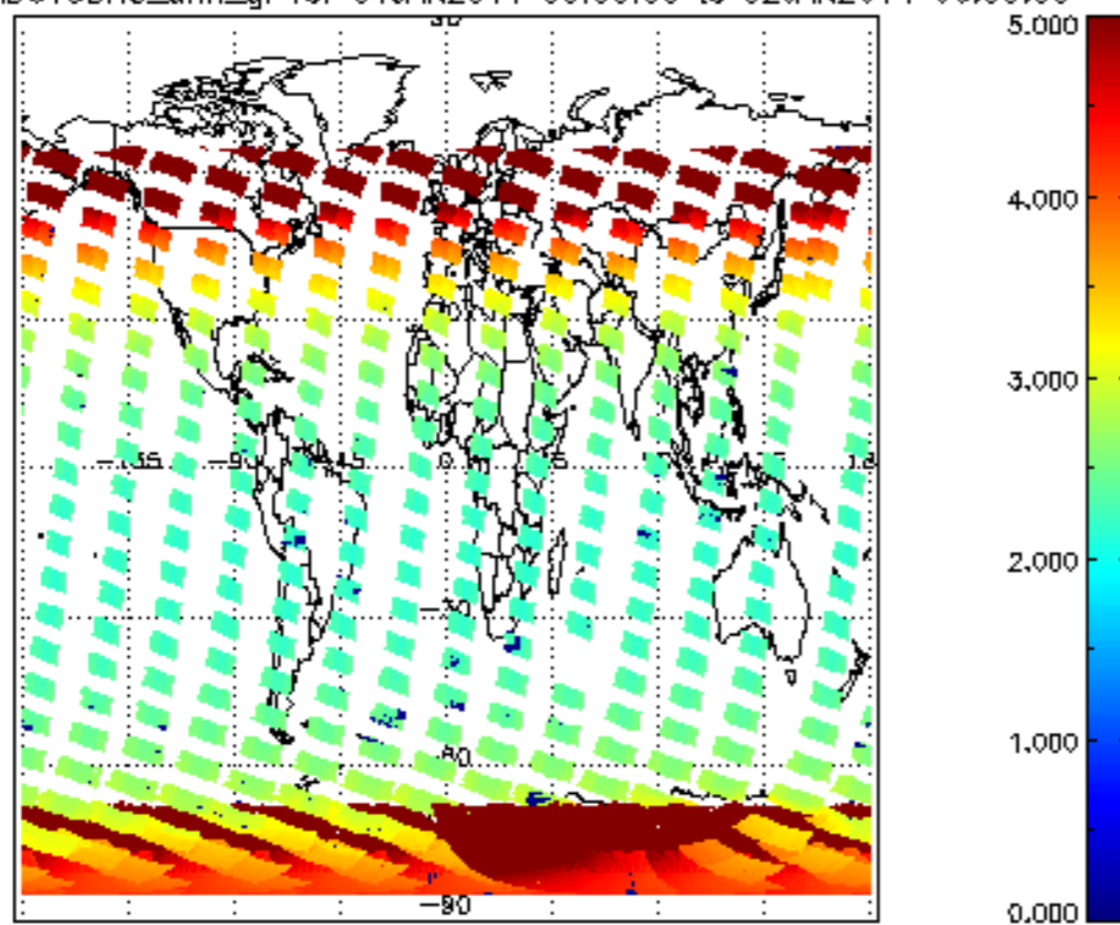
SCIOL2P_NADUV3BRO_amf_gr for 01JAN2011 00:00:00 to 02JAN2011 00:00:00
