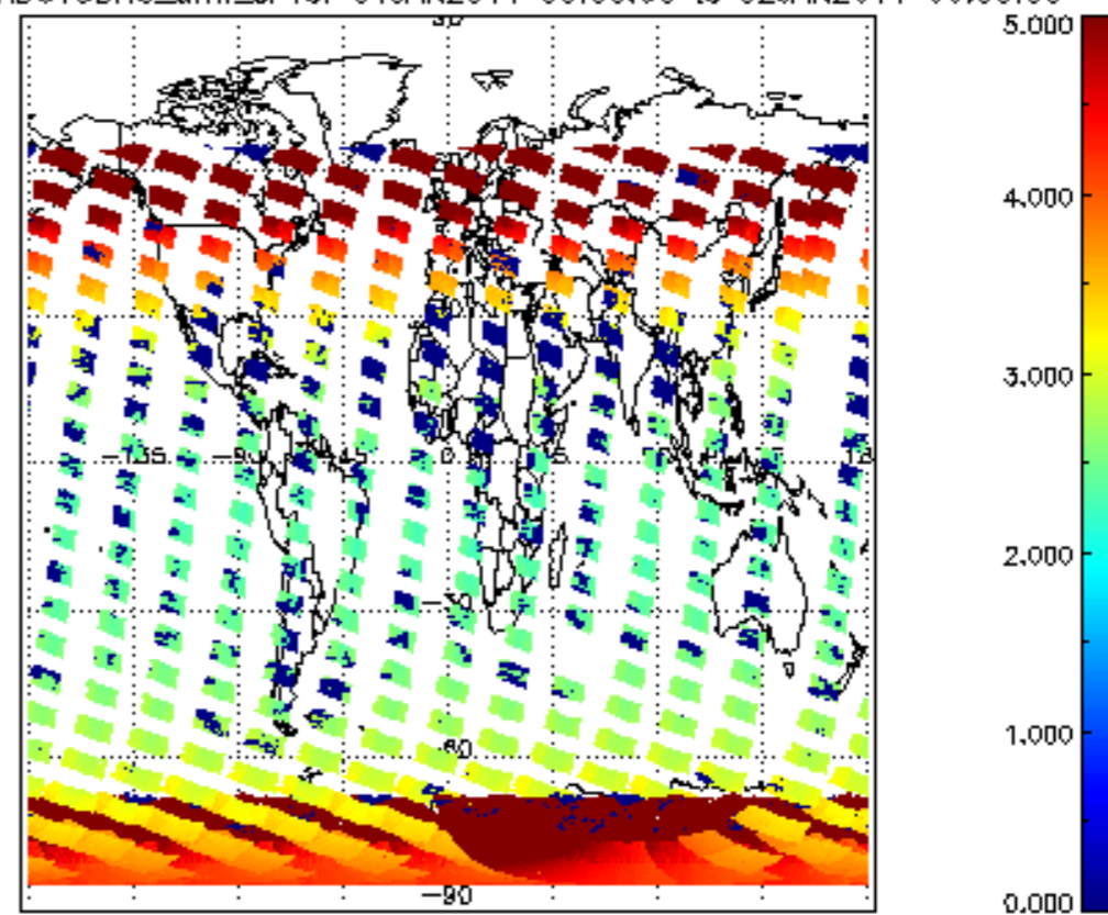
SCIOL2P_NADUV3BRO_amf_cl for 01JAN2011 00:00:00 to 02JAN2011 00:00:00
