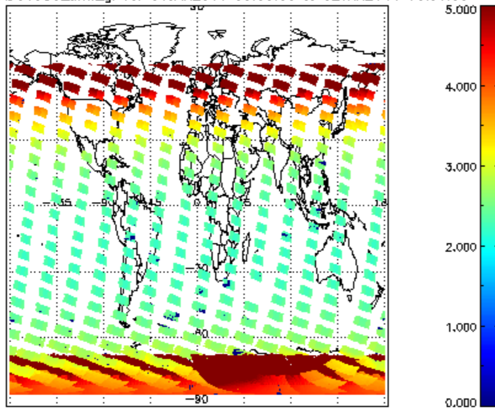
SCIOL2P_NADUV003_amf_gr for 01JAN2011 00:00:00 to 02JAN2011 00:00:00
