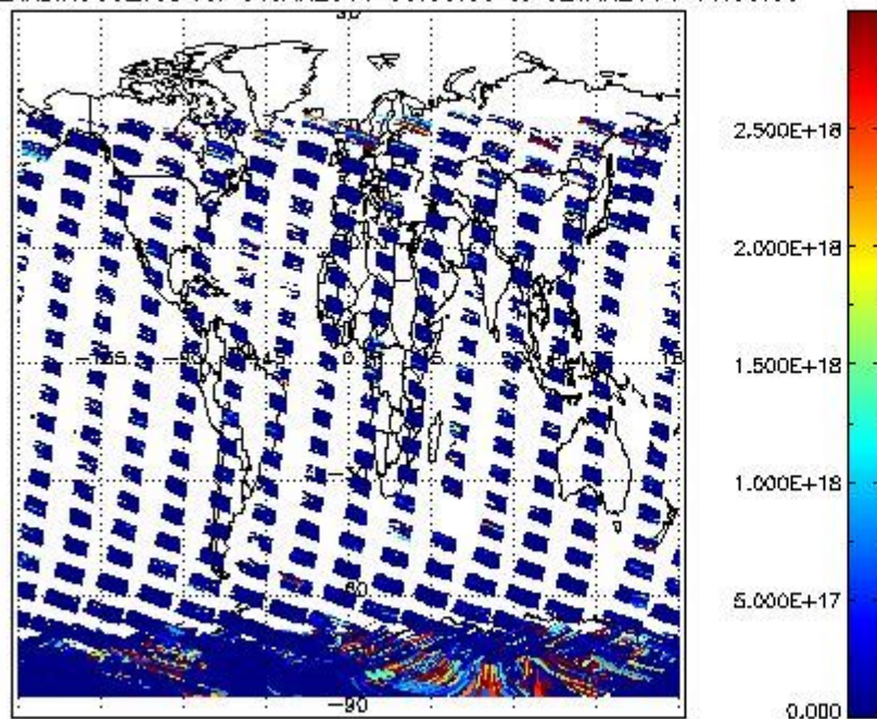
SCIDL2P_NADIR3CO_vcd for 01JAN2011 00:00:00 to 02JAN2011 00:00:00
