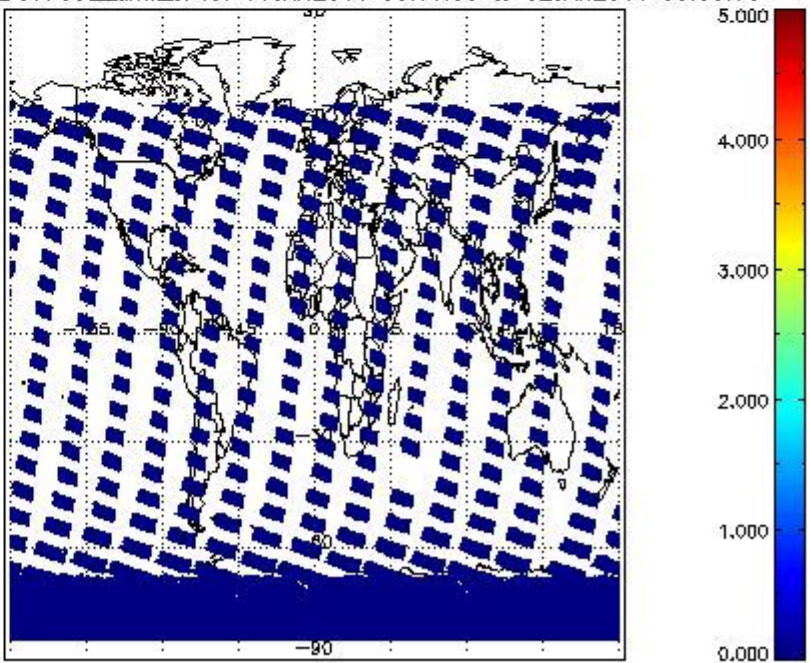
SCIOL2P_NADUV7S02_amf_cl for 01JAN2011 00:00:00 to 02JAN2011 00:00:00
