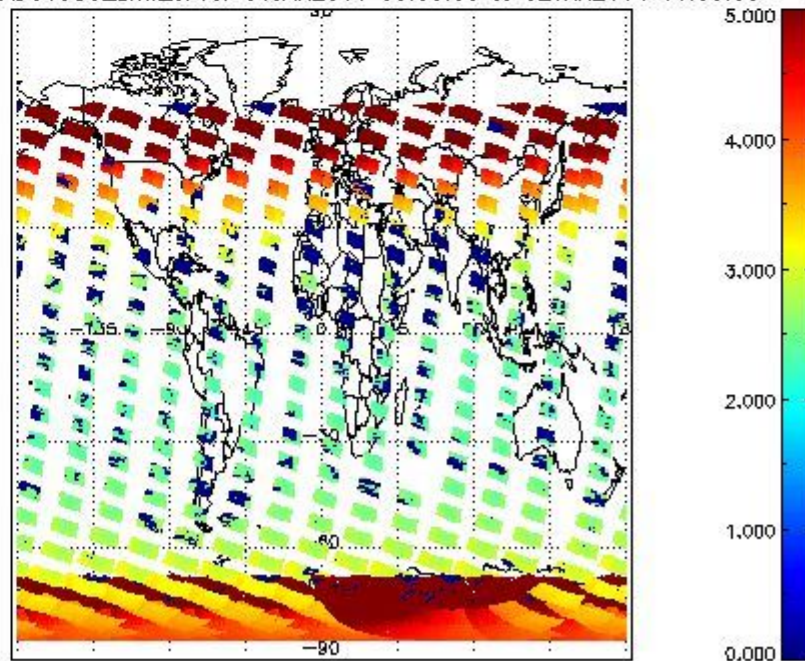
SCIOL2P_NADUV003_amf_cl for 01JAN2011 00:00:00 to 02JAN2011 00:00:00
