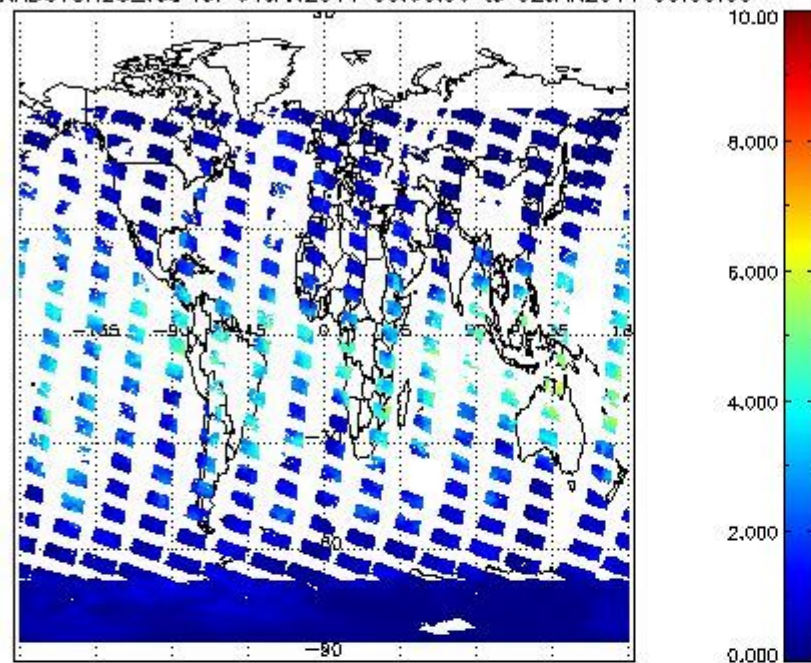
SCIOL2P_NADUV8H20_vcd for 01JAN2011 00:00:00 to 02JAN2011 00:00:00
