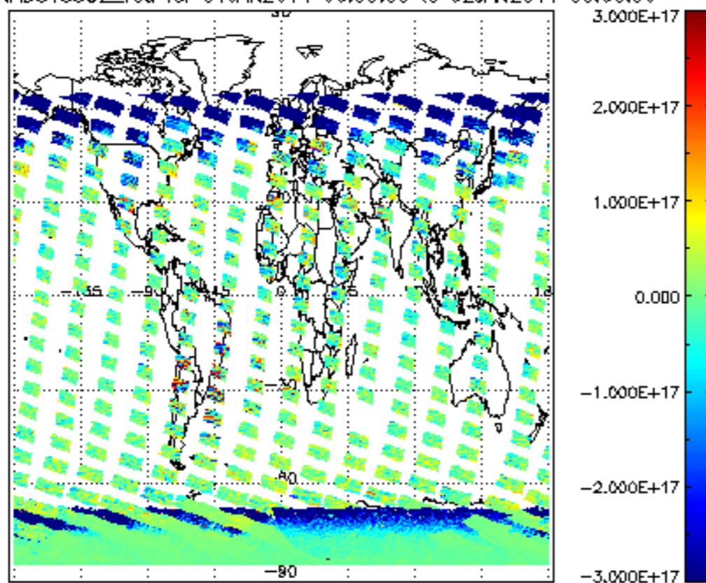
SCIOL2P_NADUV5S02_vcd for 01JAN2011 00:00:00 to 02JAN2011 00:00:00
