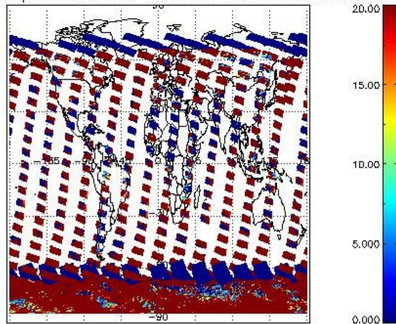
cLopt_depth for 01JAN2011 00:00:00 to 02JAN2011 00:00:00
