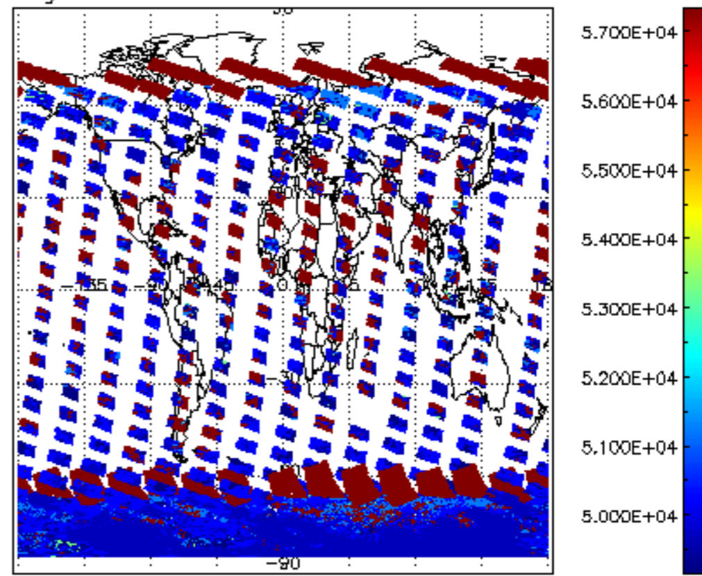
cloud_flags for 01JAN2011 00:00:00 to 02JAN2011 00:00:00
