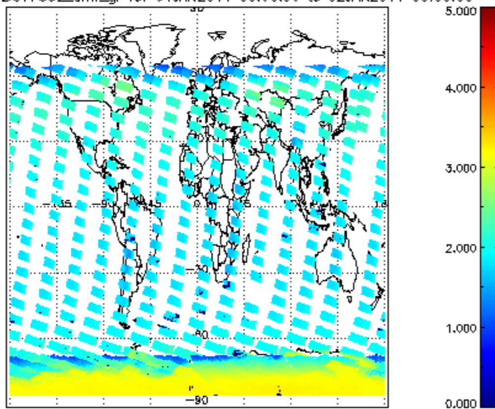
SCIOL2P_NADUV7S02_amf_gr for 01JAN2011 00:00:00 to 02JAN2011 00:00:00
