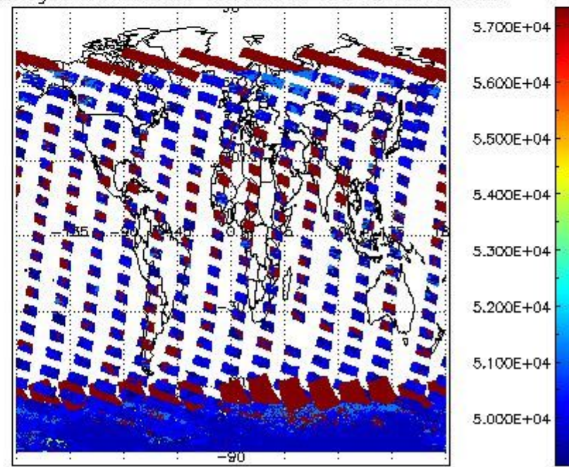
cloud_flags for 01JAN2011 00:00:00 to 02JAN2011 00:00:00
