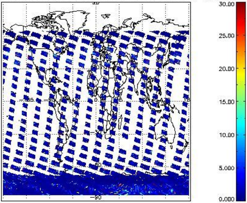
SCIOL2P_NADUV7S02_vcd_err for 01JAN2011 00:00:00 to 02JAN2011 00:00:00
