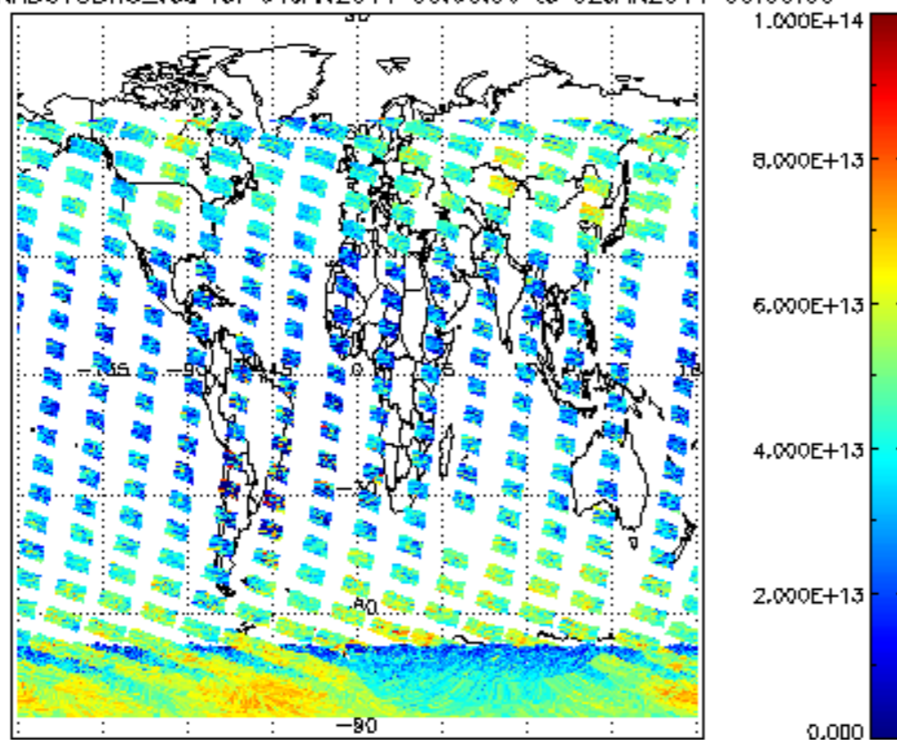
SCIOL2P_NADUV3BRO_vcd for 01JAN2011 00:00:00 to 02JAN2011 00:00:00
