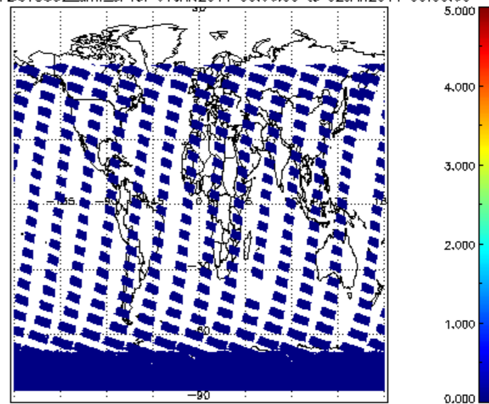
SCIOL2P_NADUV5S02_amf_cl for 01JAN2011 00:00:00 to 02JAN2011 00:00:00
