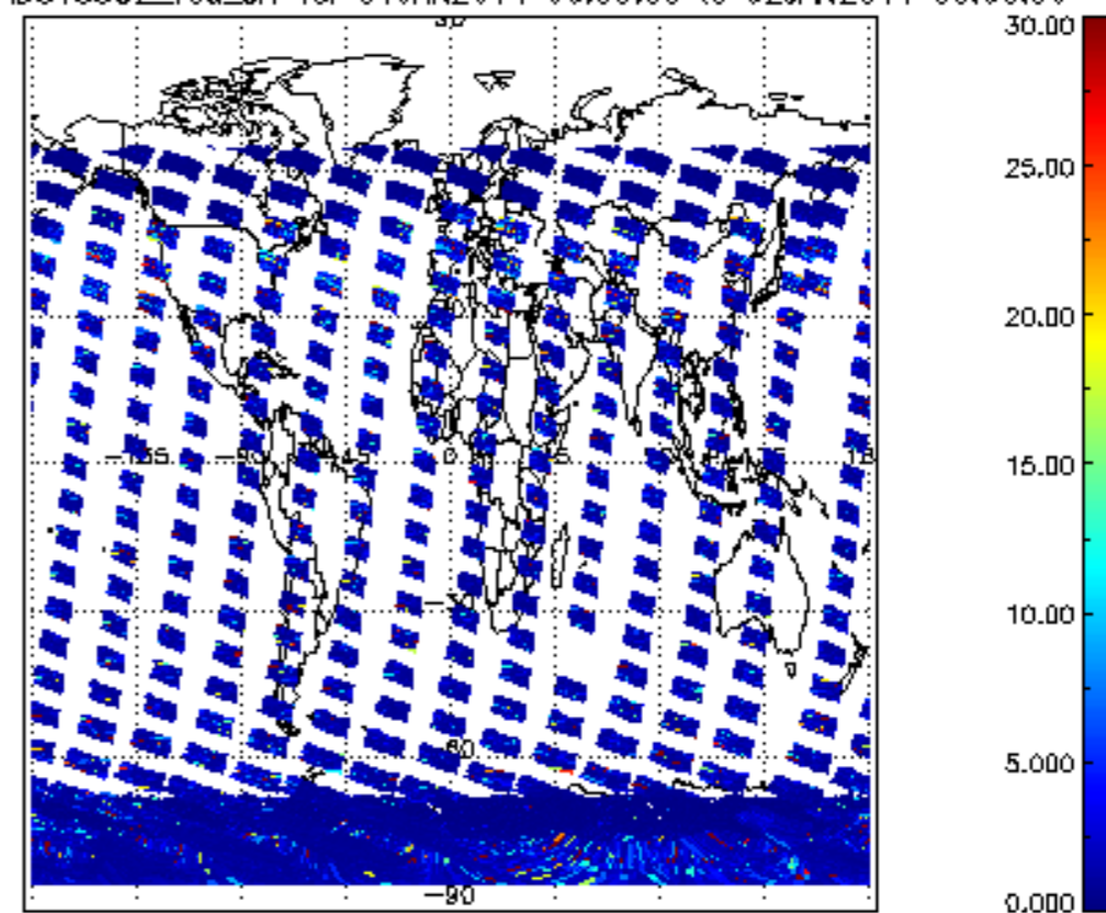
SCIOL2P_NADUV5S02_vcd_err for 01JAN2011 00:00:00 to 02JAN2011 00:00:00
