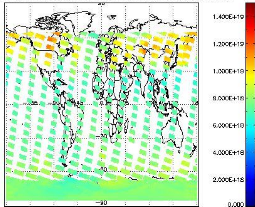
SCIOL2P_NADUV003_vcd for 01JAN2011 00:00:00 to 02JAN2011 00:00:00
