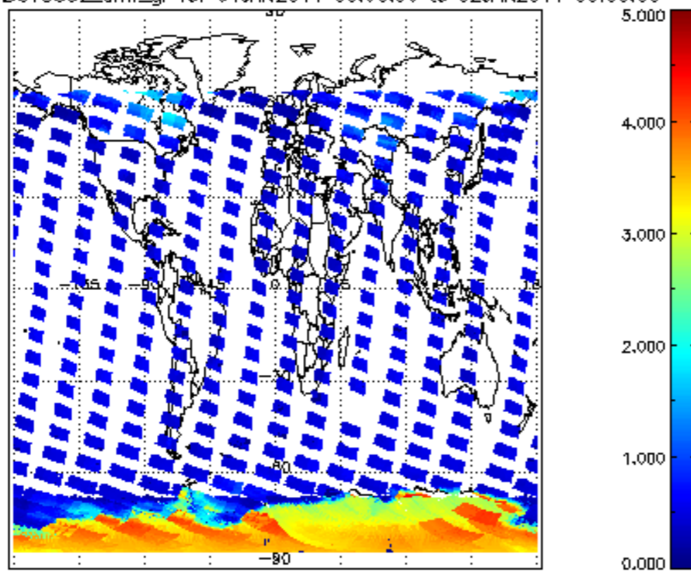
SCIOL2P_NADUV5S02_amf_gr for 01JAN2011 00:00:00 to 02JAN2011 00:00:00
