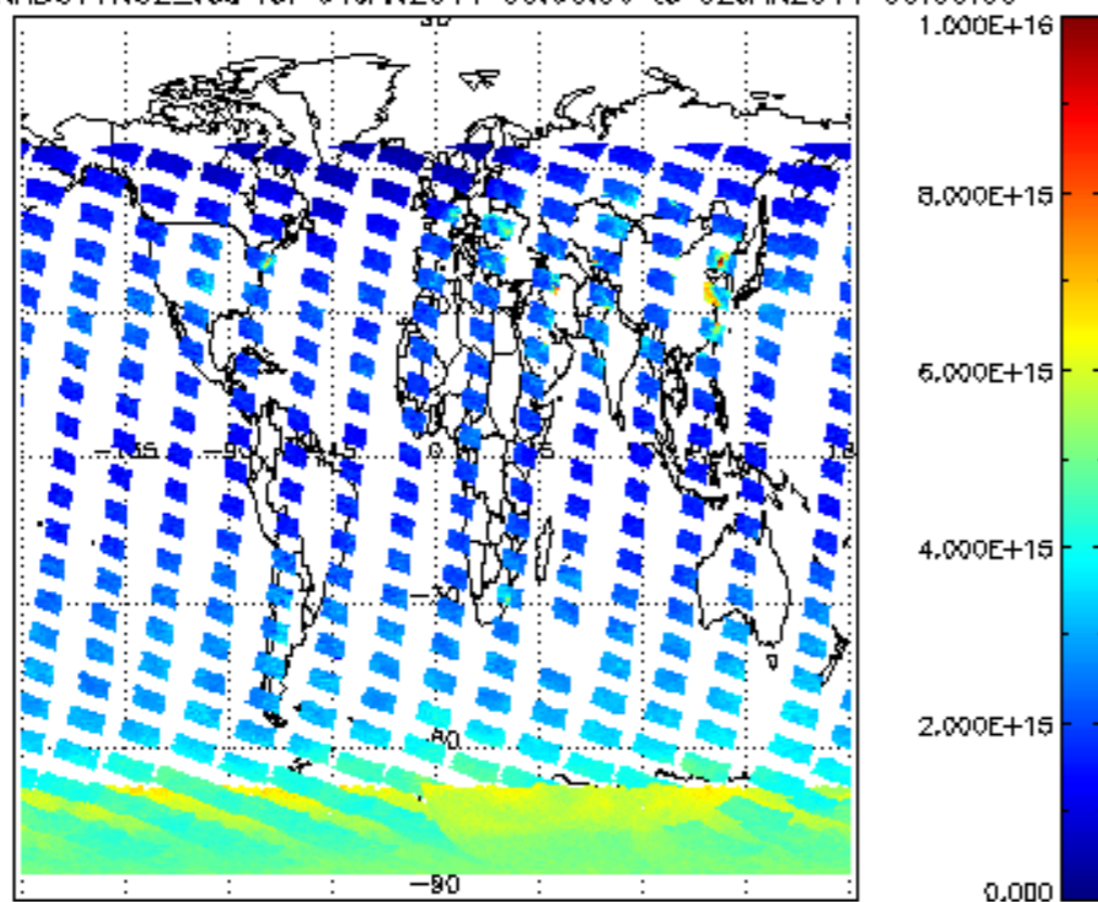
SCIOL2P_NADUV1NO2_vcd for 01JAN2011 00:00:00 to 02JAN2011 00:00:00
