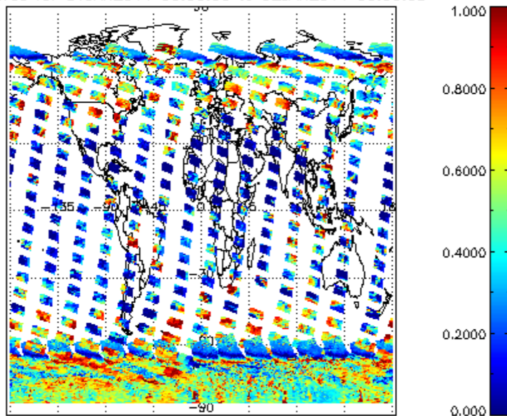
cL_frac for 01JAN2011 00:00:00 to 02JAN2011 00:00:00
