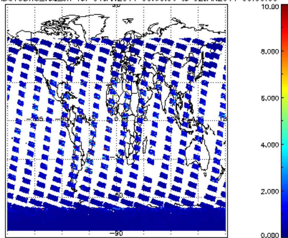
SCIOL2P_NADUV3BRO_vcd_err for 01JAN2011 00:00:00 to 02JAN2011 00:00:00
