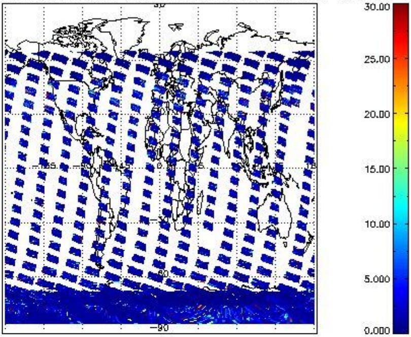
SCIOL2P_NADUV5SO2_vcd_err for 01JAN2011 00:00:00 to 02JAN2011 00:00:00
