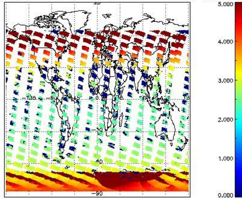
SCIOL2P_NADUV3BRO_amf_cl for 01JAN2011 00:00:00 to 02JAN2011 00:00:00
