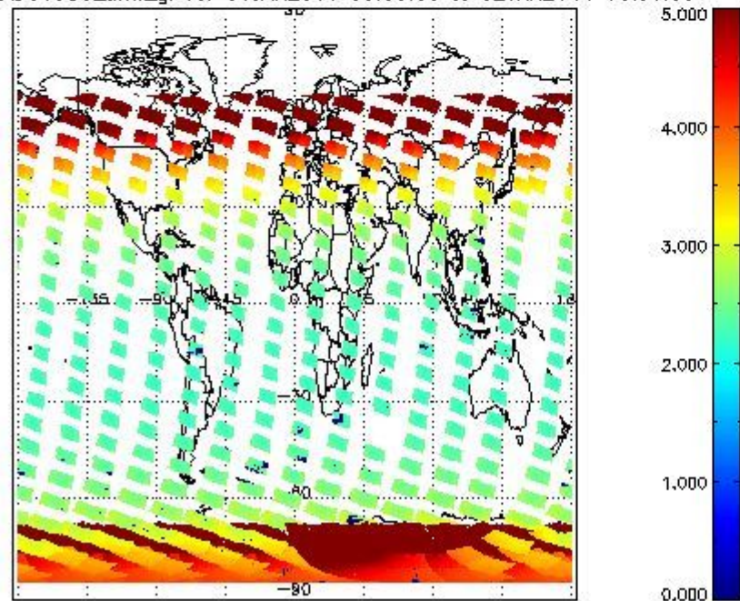
SCIOL2P_NADUV003_amf_gr for 01JAN2011 00:00:00 to 02JAN2011 00:00:00
