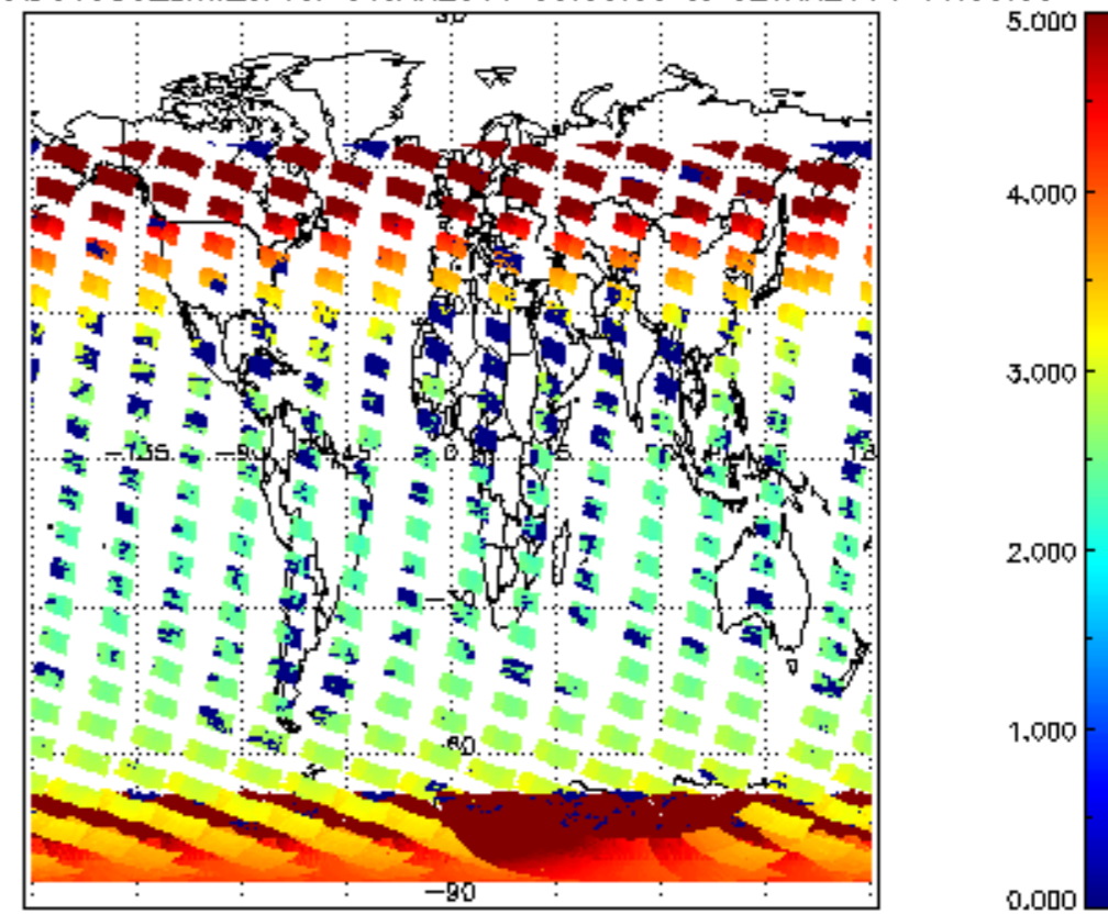
SCIOL2P_NADUV003_amf_cl for 01JAN2011 00:00:00 to 02JAN2011 00:00:00
