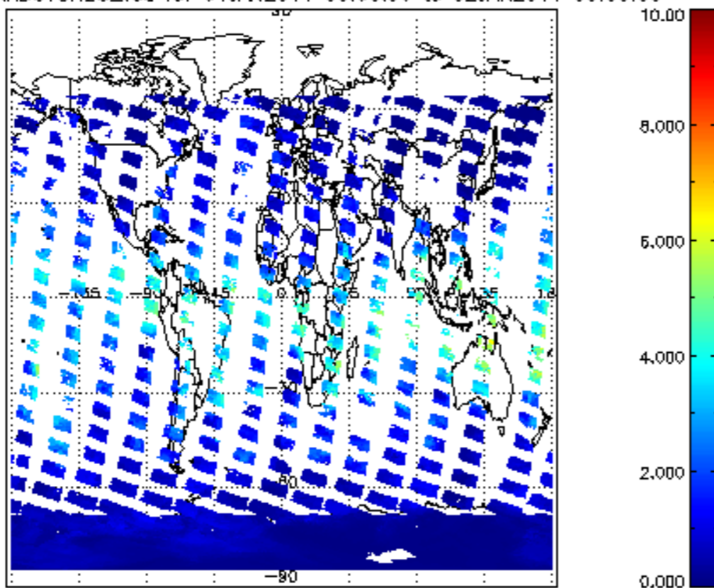
SCIOL2P_NADUV8H20_vcd for 01JAN2011 00:00:00 to 02JAN2011 00:00:00
