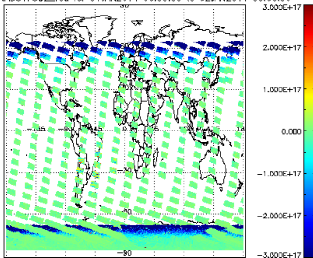
SCIOL2P_NADUV7S02_vcd for 01JAN2011 00:00:00 to 02JAN2011 00:00:00
