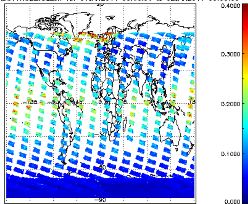
SCIOL2P_NADUV1NO2_vcd_err for 01JAN2011 00:00:00 to 02JAN2011 00:00:00
