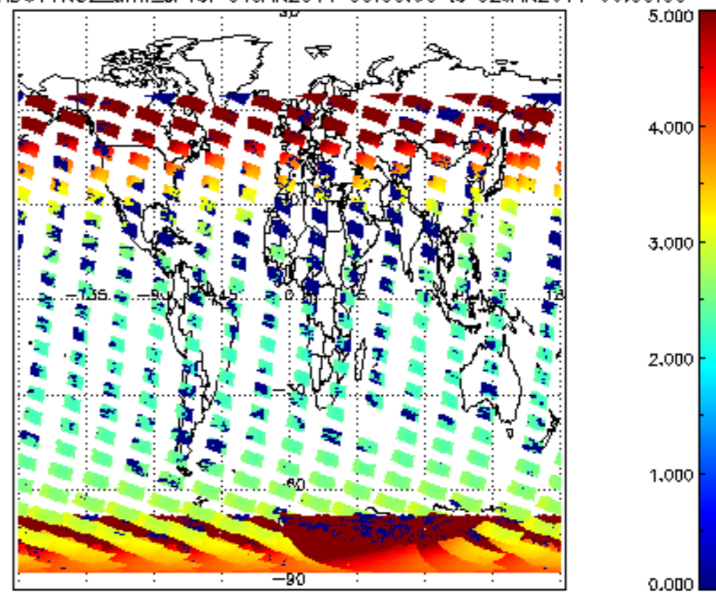
SCIOL2P_NADUV1NO2_amf_cl for 01JAN2011 00:00:00 to 02JAN2011 00:00:00
