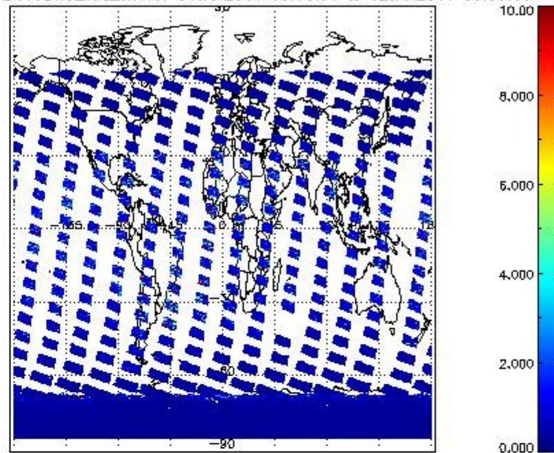
SCIOL2P_NADUV3BRO_vcd_err for 01JAN2011 00:00:00 to 02JAN2011 00:00:00
