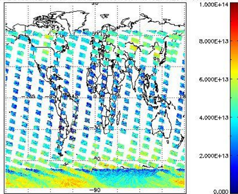
SCIOL2P_NADUV3BRO_vcd for 01JAN2011 00:00:00 to 02JAN2011 00:00:00
