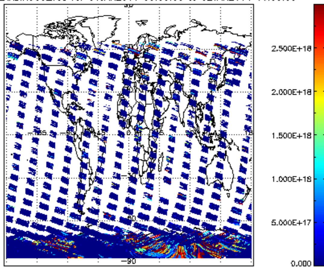
SCIOL2P_NADIR3CO_vcd for 01JAN2011 00:00:00 to 02JAN2011 00:00:00
