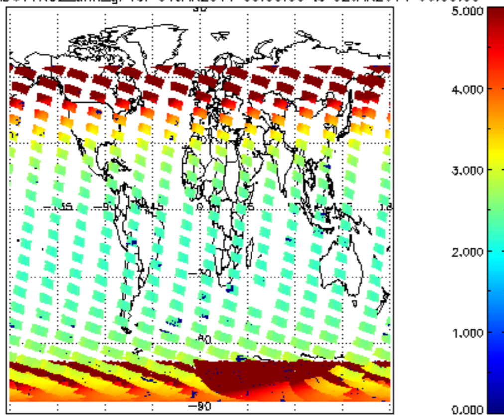
SCIOL2P_NADUV1NO2_amf_gr for 01JAN2011 00:00:00 to 02JAN2011 00:00:00
