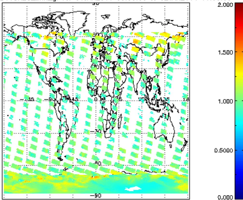
SCIOL2P_NADUV8H20_amf_gr for 01JAN2011 00:00:00 to 02JAN2011 00:00:00
