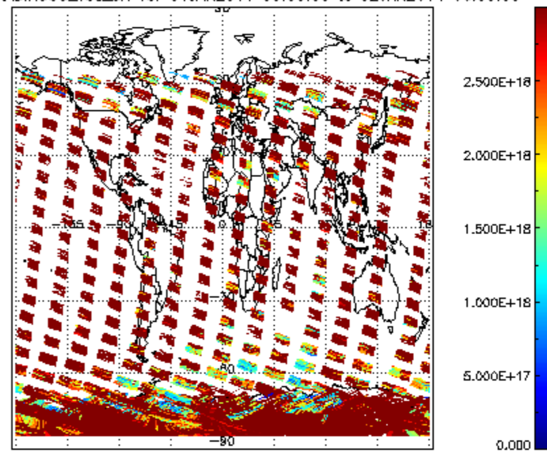
SCIOL2P_NADIR3CO_vcd_err for 01JAN2011 00:00:00 to 02JAN2011 00:00:00
