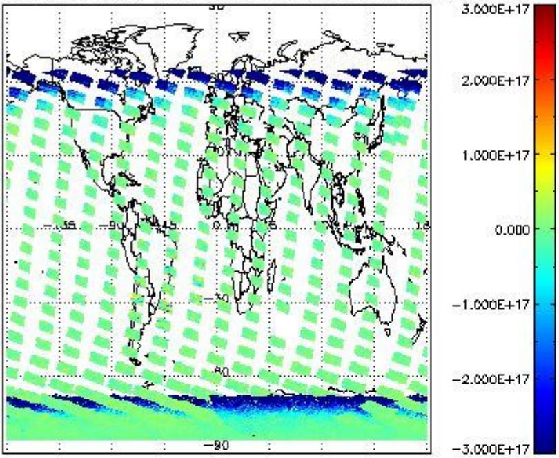
SCIOL2P_NADUV7S02_vcd for 01JAN2011 00:00:00 to 02JAN2011 00:00:00
