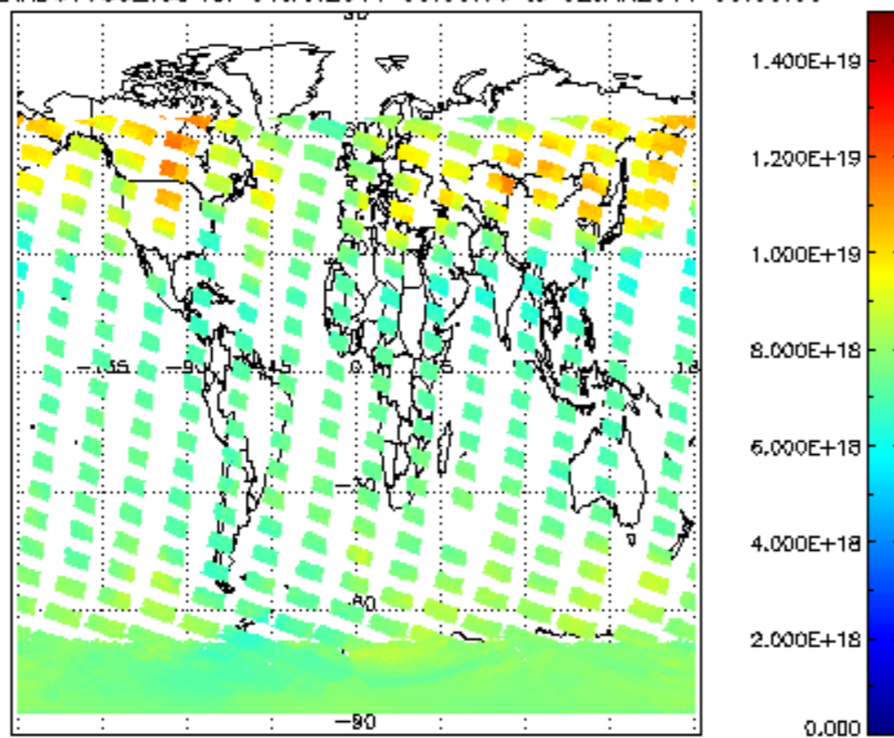
SCIOL2P_NADUV003_vcd for 01JAN2011 00:00:00 to 02JAN2011 00:00:00
