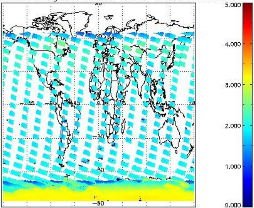
SCIOL2P_NADUV7S02_amf_gr for 01JAN2011 00:00:00 to 02JAN2011 00:00:00
