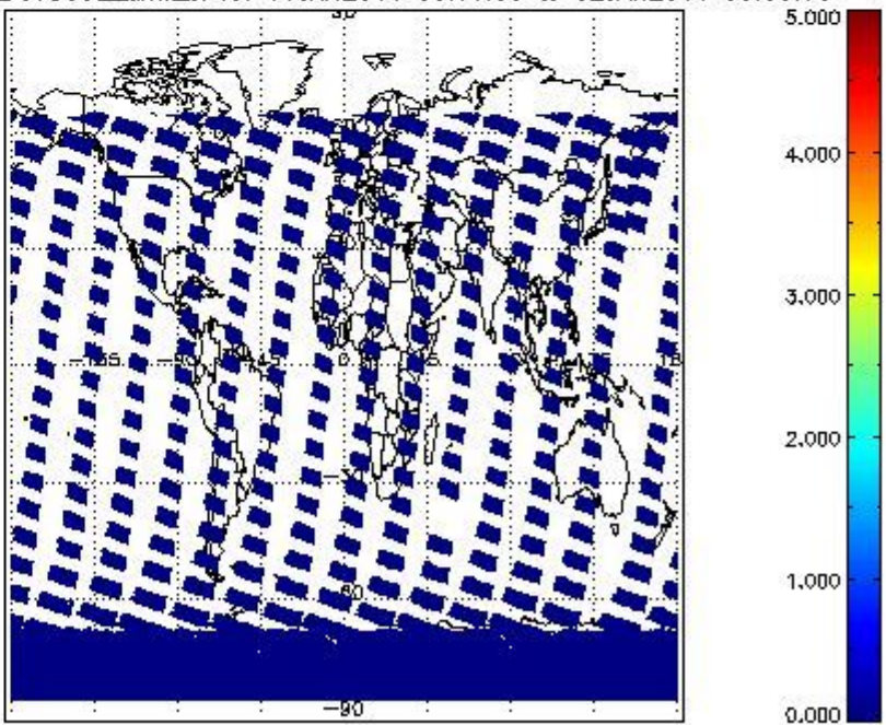
SCIOL2P_NADUV5SO2_amf_cl for 01JAN2011 00:00:00 to 02JAN2011 00:00:00
