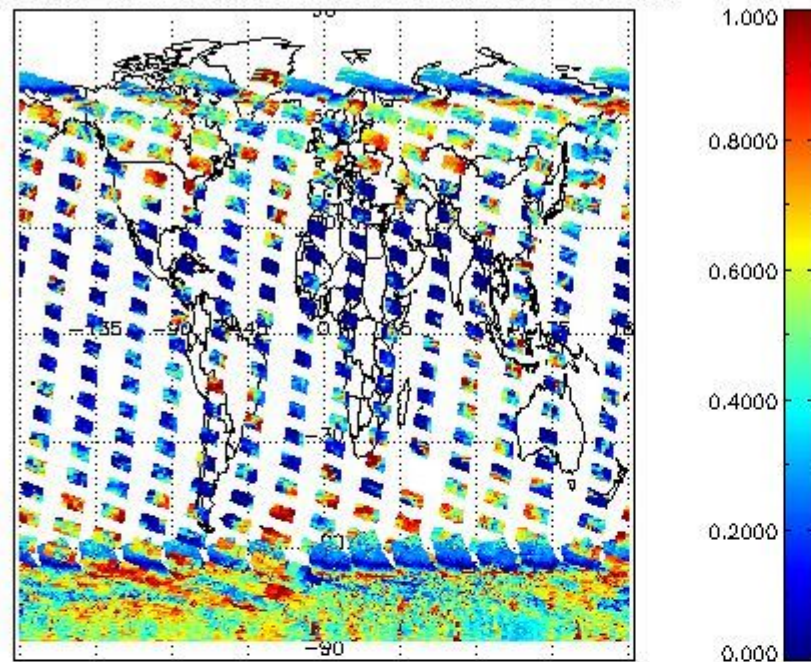
cL_frac for 01JAN2011 00:00:00 to 02JAN2011 00:00:00
