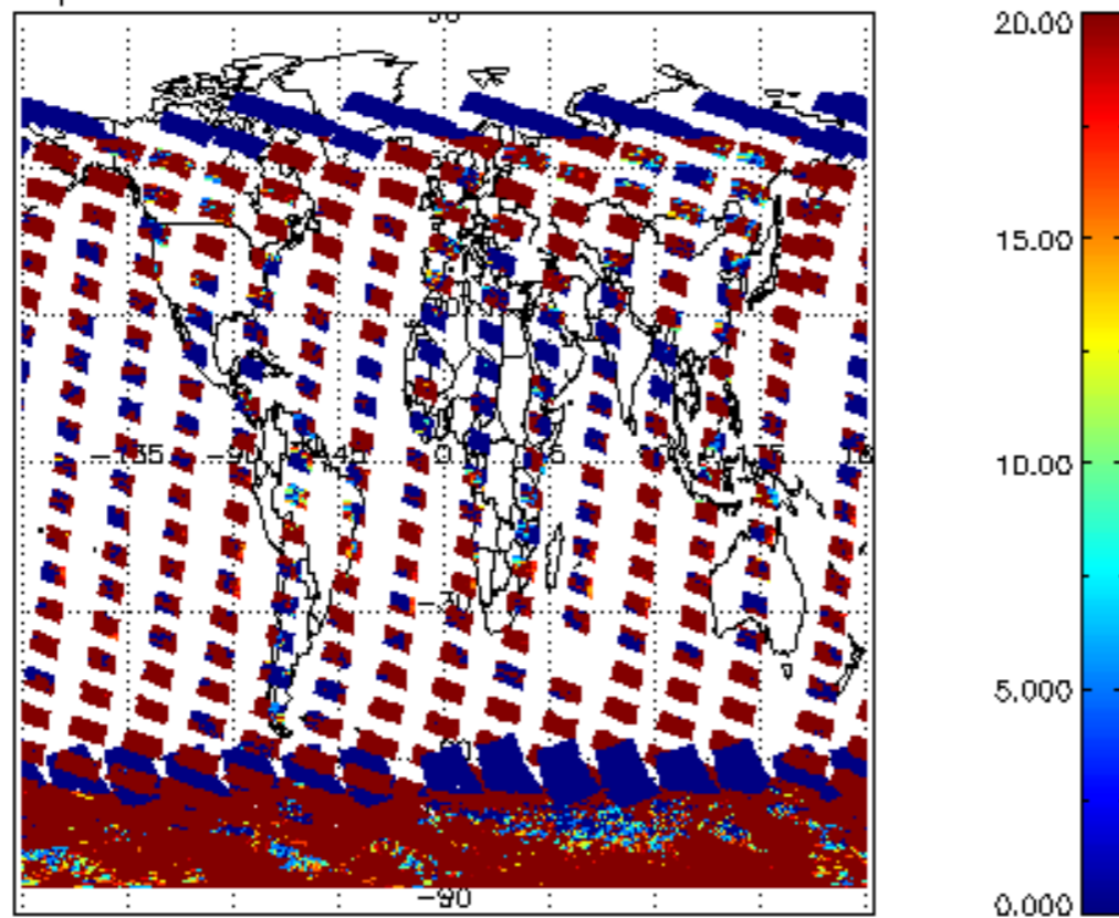
cLopt_depth for 01JAN2011 00:00:00 to 02JAN2011 00:00:00
