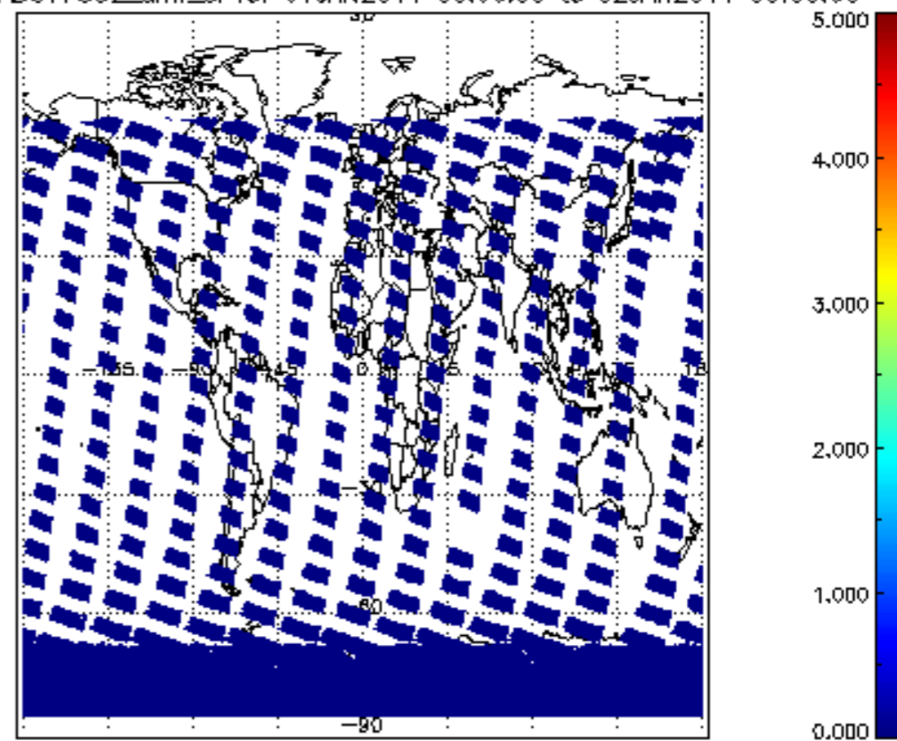
SCIOL2P_NADUV7S02_amf_cl for 01JAN2011 00:00:00 to 02JAN2011 00:00:00
