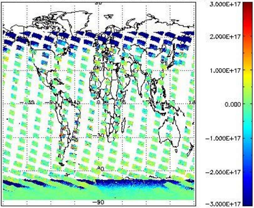
SCIOL2P_NADUV5SO2_vcd for 01JAN2011 00:00:00 to 02JAN2011 00:00:00
