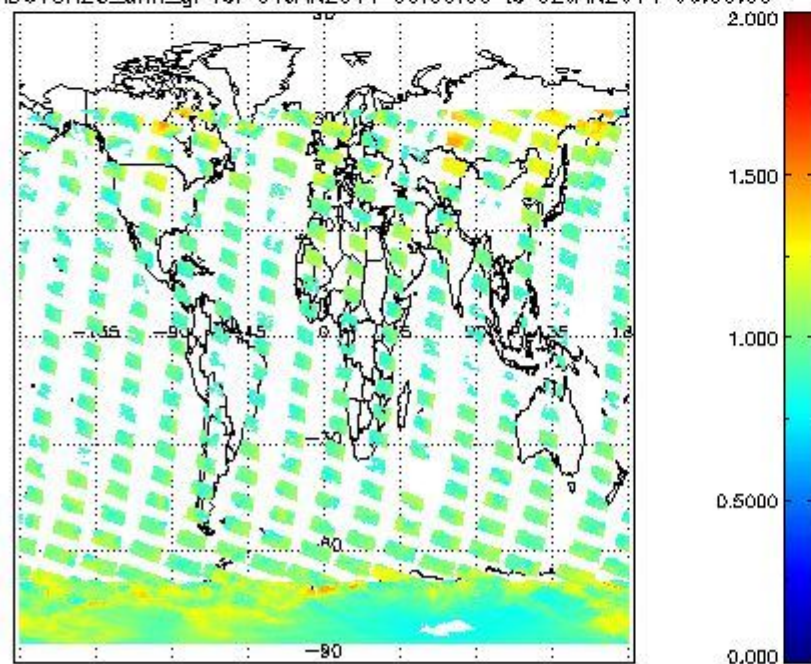
SCIOL2P_NADUV8H20_amf_gr for 01JAN2011 00:00:00 to 02JAN2011 00:00:00
