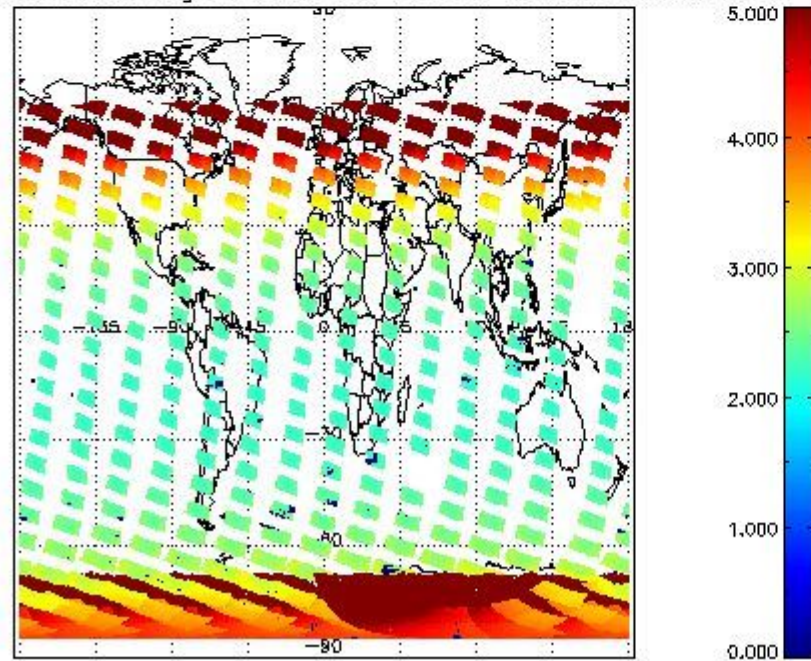
SCIOL2P_NADUV3BRO_amf_gr for 01JAN2011 00:00:00 to 02JAN2011 00:00:00
