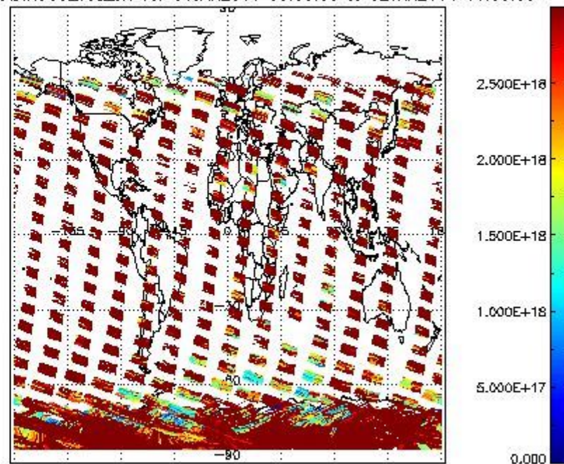
SCIDL2P_NADIR3CO_vcd_err for 01JAN2011 00:00:00 to 02JAN2011 00:00:00
