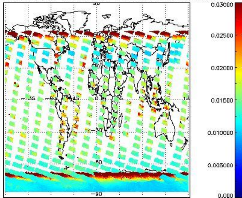
SCIOL2P_NADUV003_vcd_err for 01JAN2011 00:00:00 to 02JAN2011 00:00:00
