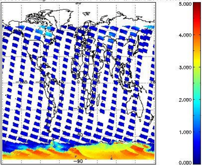
SCIOL2P_NADUV5SO2_amf_gr for 01JAN2011 00:00:00 to 02JAN2011 00:00:00
