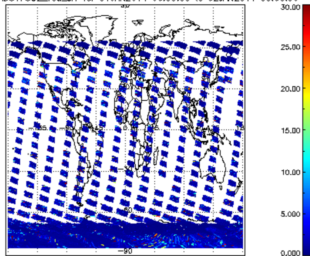
SCIOL2P_NADUV7S02_vcd_err for 01JAN2011 00:00:00 to 02JAN2011 00:00:00
