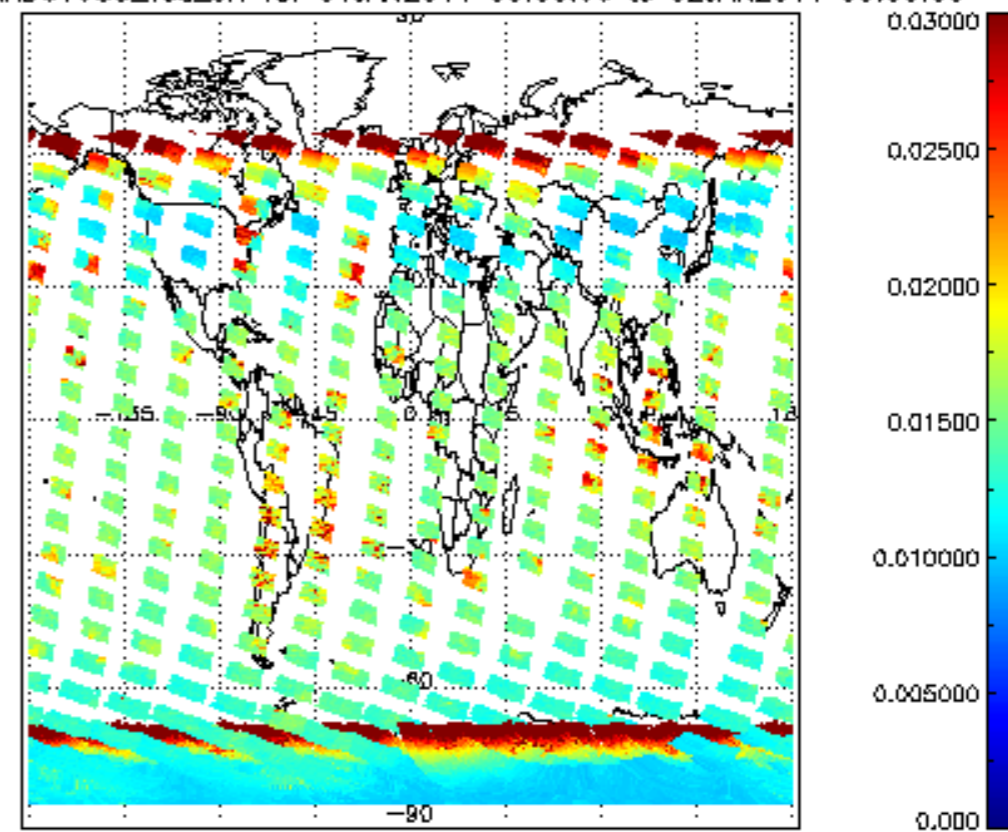
SCIOL2P_NADUV003_vcd_err for 01JAN2011 00:00:00 to 02JAN2011 00:00:00
