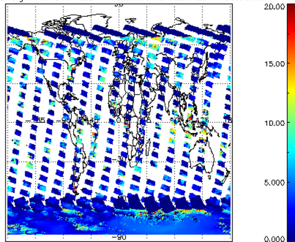
cL_top_height for 01JAN2011 00:00:00 to 02JAN2011 00:00:00
