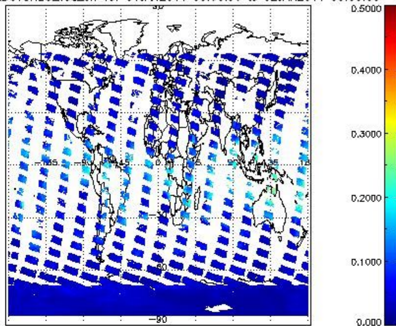
SCIOL2P_NADUV8H20_vcd_err for 01JAN2011 00:00:00 to 02JAN2011 00:00:00
