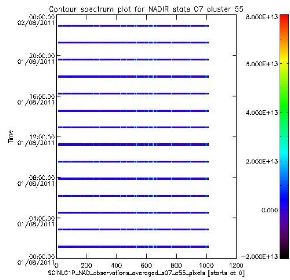
sciamachy_i1b_source_packet_report_SCIA_7_04_U_20110801_8.PNG
