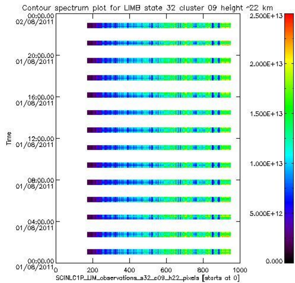
sciamachy_i1b_source_packet_report_SCIA_7_04_U_20110801_12.PNG
