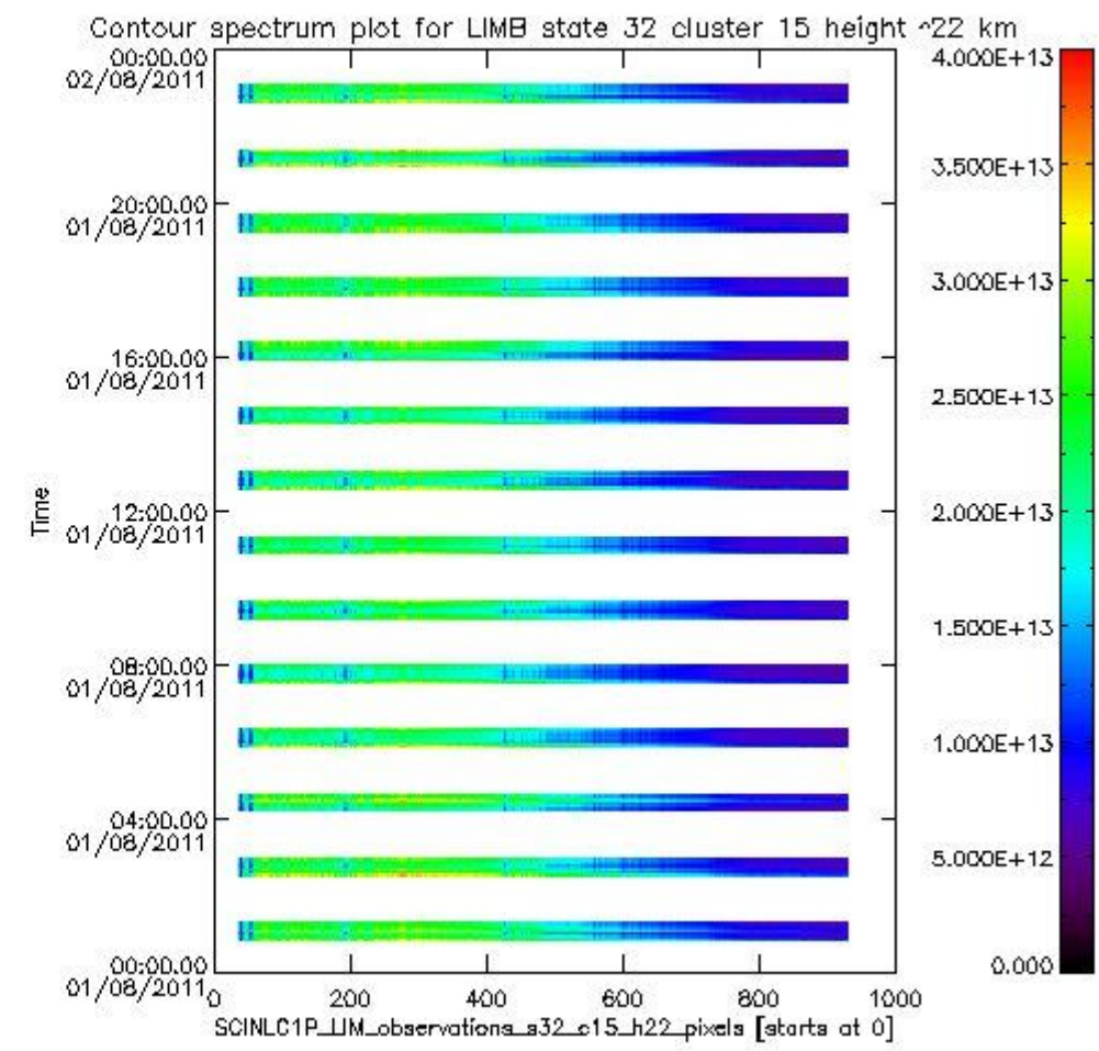
sciamachy_i1b_source_packet_report_SCIA_7_04_U_20110801_16.PNG
