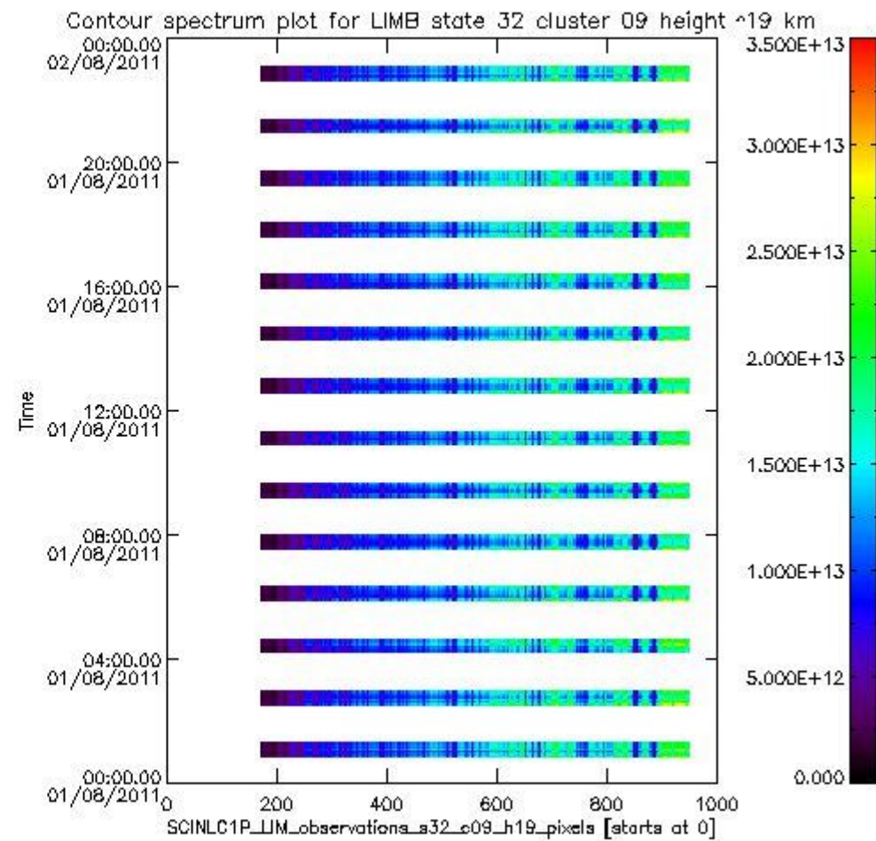
sciamachy_i1b_source_packet_report_SCIA_7_04_U_20110801_10.PNG
