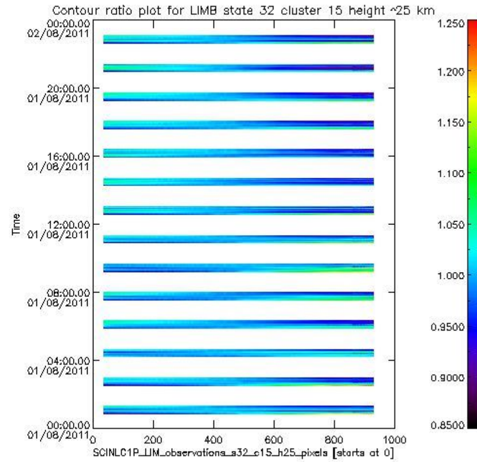
sciamachy_11b_source_packet_report_SCIA_7_04_U_20110801_19.PNG
