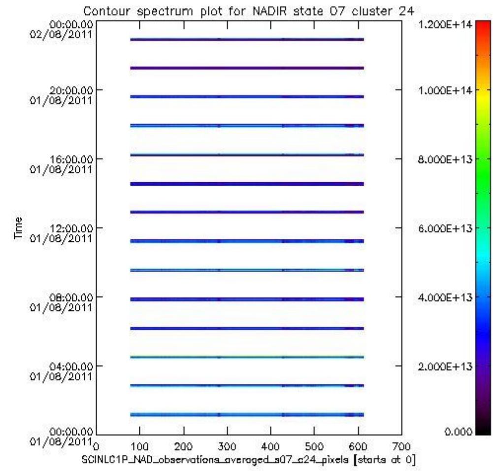
sciamachy_i1b_source_packet_report_SCIA_7_04_U_20110801_6.PNG
