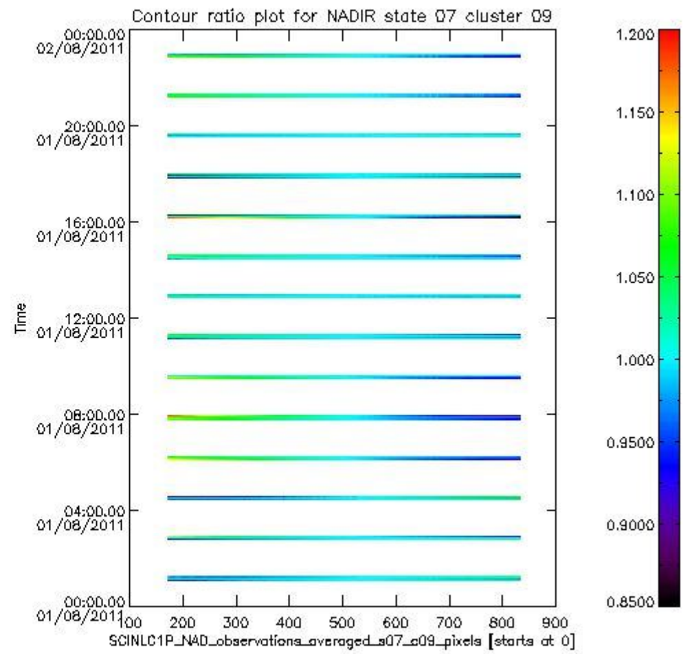
sciamachy_i1b_source_packet_report_SCIA_7_04_U_20110801_3.PNG
