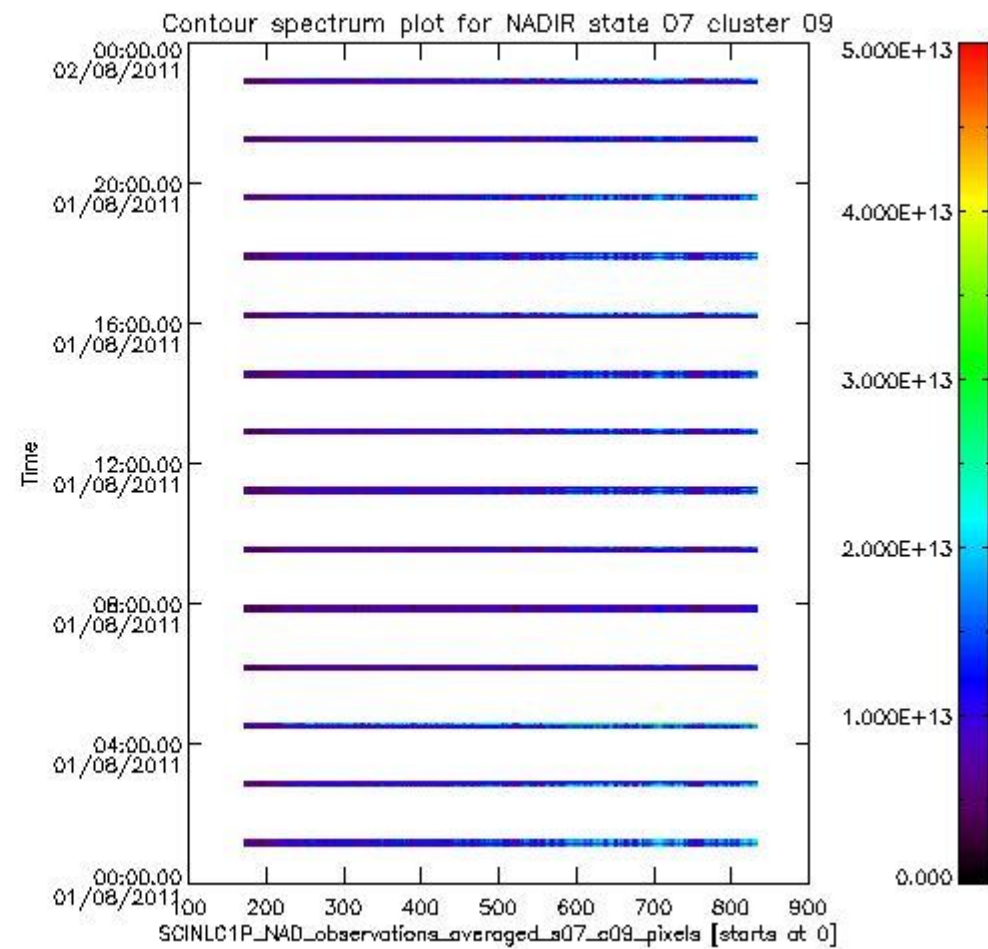
sciamachy_i1b_source_packet_report_SCIA_7_04_U_20110801_2.PNG
