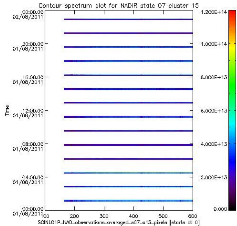
sciamachy_i1b_source_packet_report_SCIA_7_04_U_20110801_4.PNG
