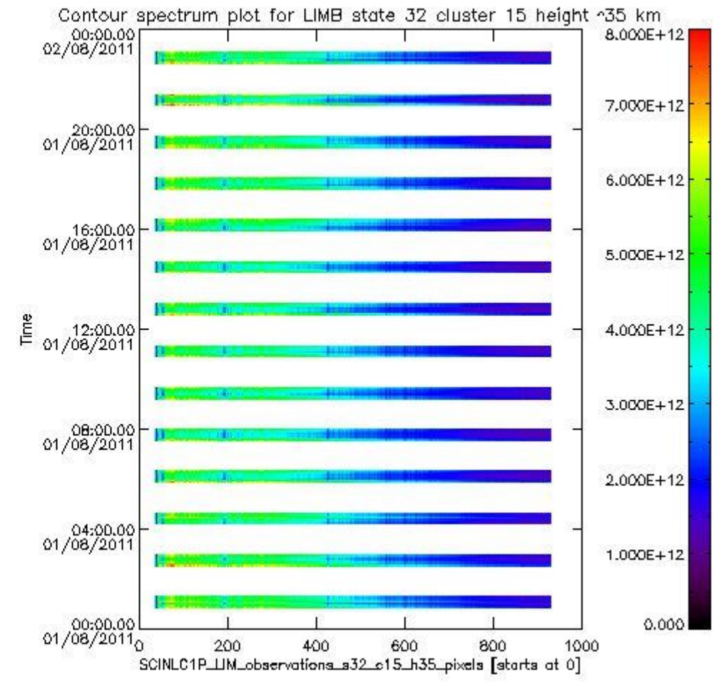
sciamachy_11b_source_packet_report_SCIA_7_04_U_20110801_20.PNG
