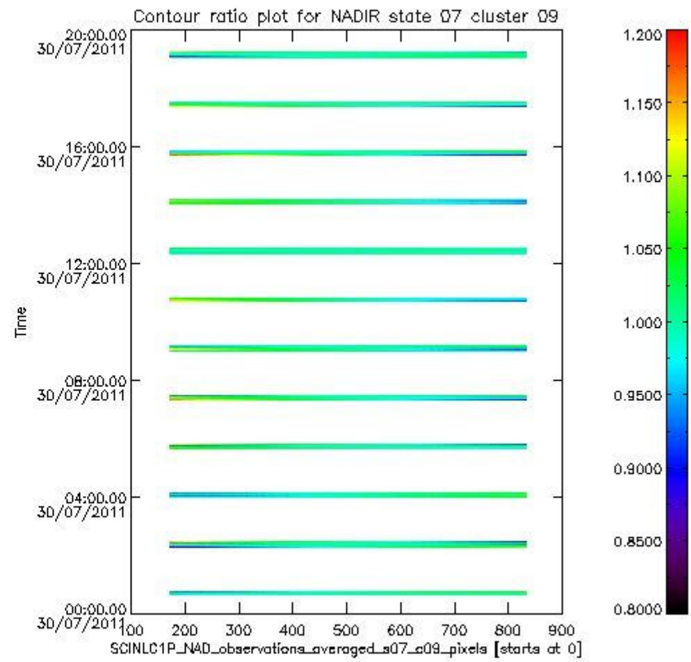
sciamachy_i1b_source_packet_report_SCIA_7_04_U_20110730_3.PNG
