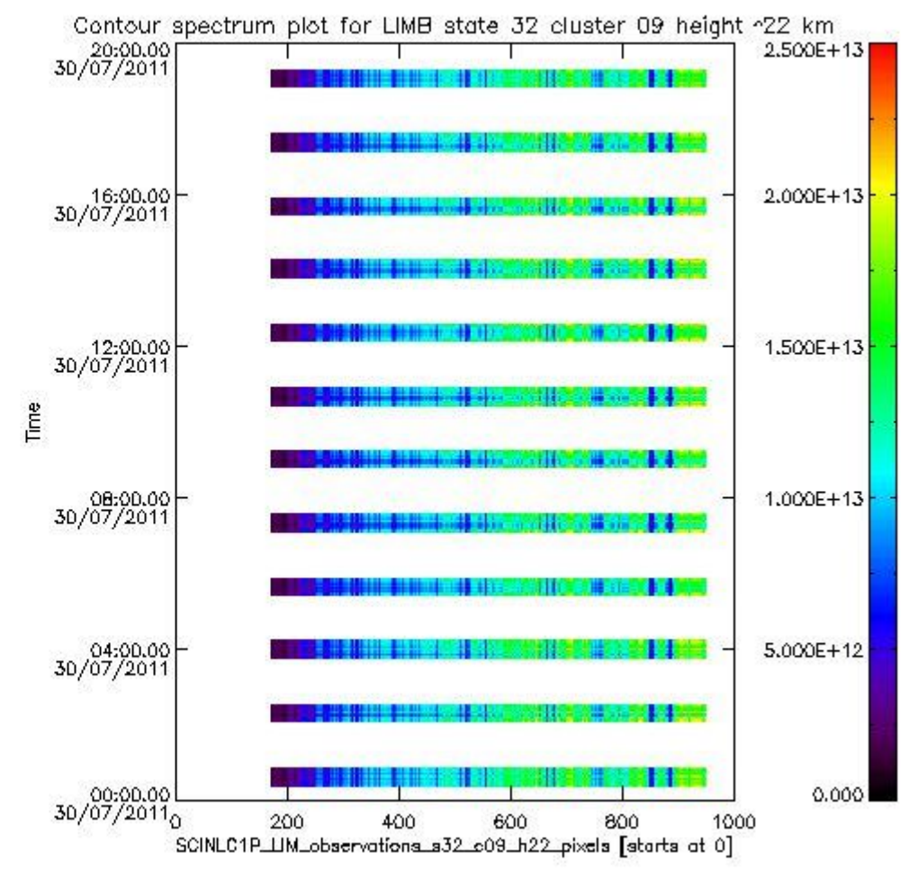
sciamachy_i1b_source_packet_report_SCIA_7_04_U_20110730_12.PNG
