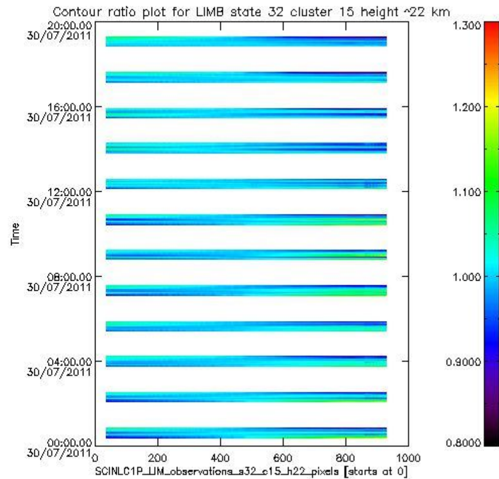
sciamachy_11b_source_packet_report_SCIA_7_04_U_20110730_17.PNG
