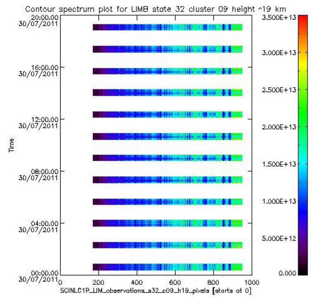
sciamachy_i1b_source_packet_report_SCIA_7_04_U_20110730_10.PNG
