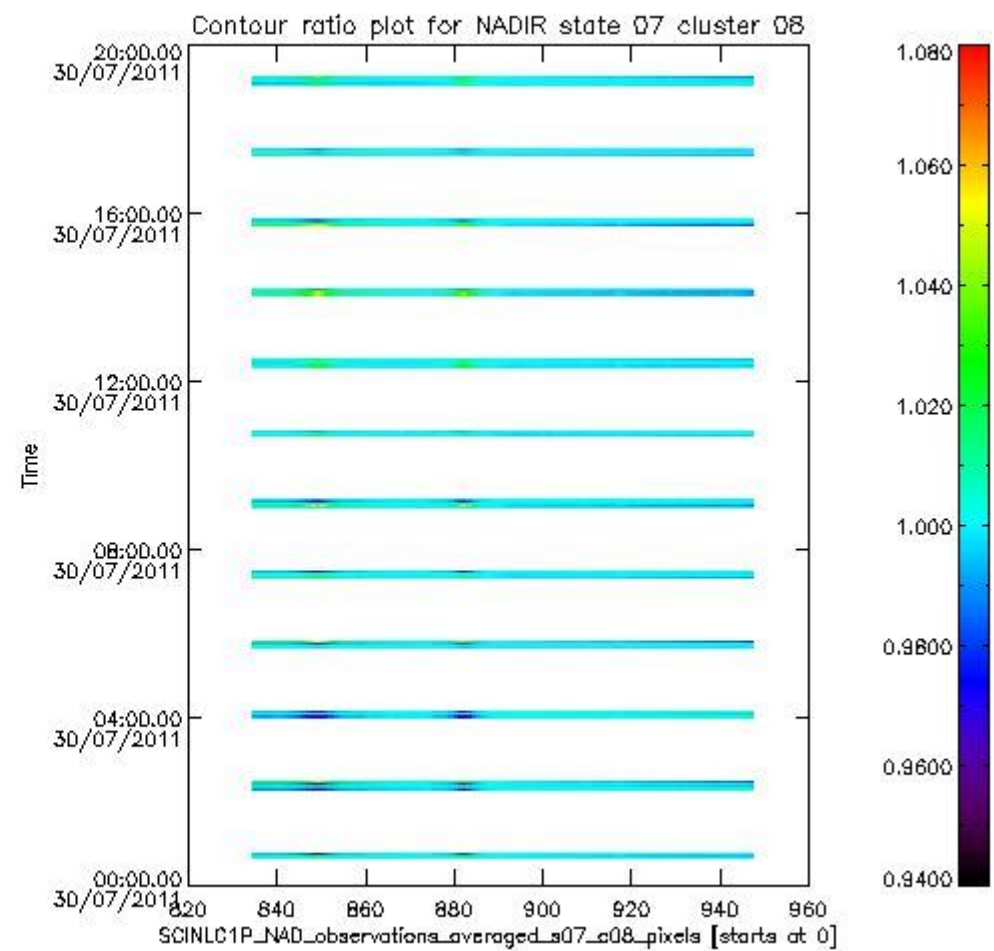
sciamachy_i1b_source_packet_report_SCIA_7_04_U_20110730_1.PNG
