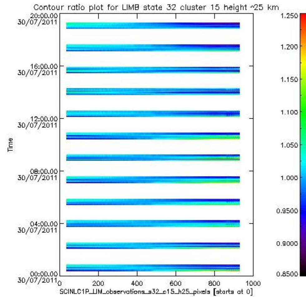
sciamachy_11b_source_packet_report_SCIA_7_04_U_20110730_19.PNG
