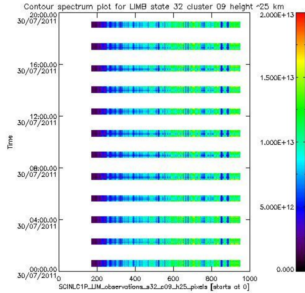
sciamachy_l1b_source_packet_report_SCIA_7_04_U_20110730_14.PNG
