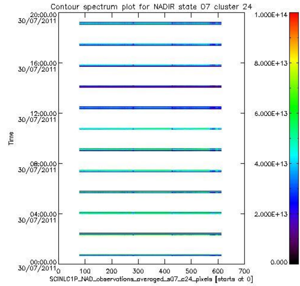
sciamachy_i1b_source_packet_report_SCIA_7_04_U_20110730_6.PNG
