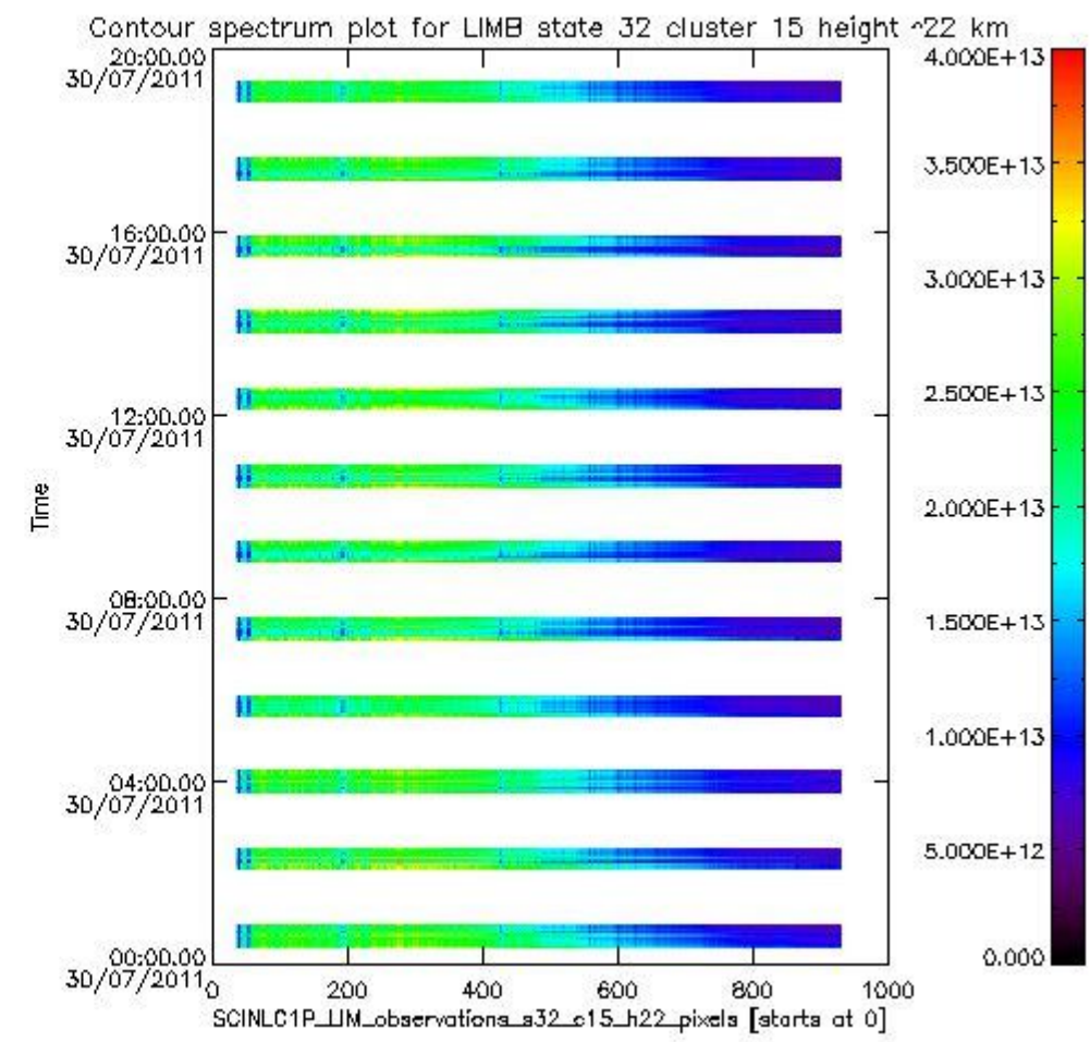
sciamachy_i1b_source_packet_report_SCIA_7_04_U_20110730_16.PNG
