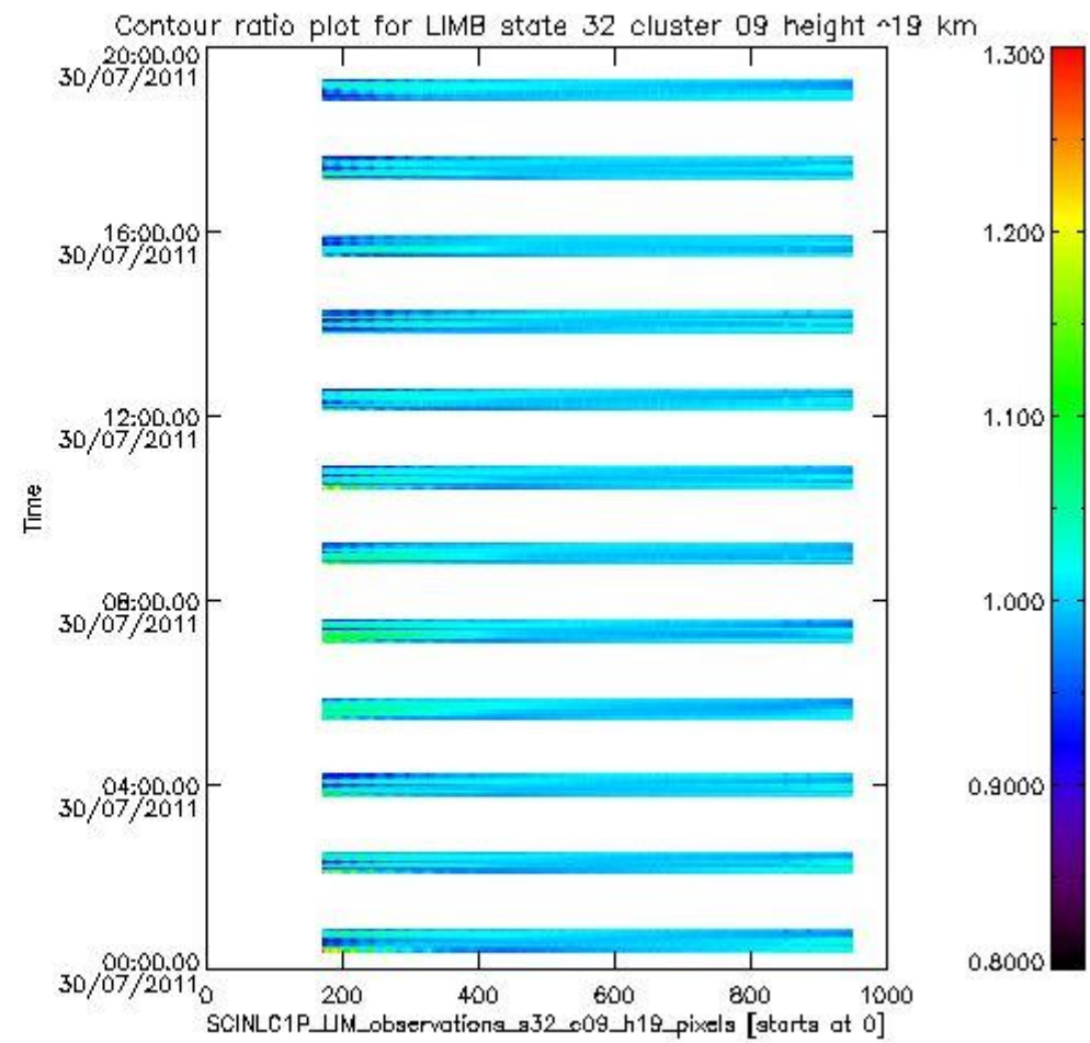
sciamachy_i1b_source_packet_report_SCIA_7_04_U_20110730_11.PNG
