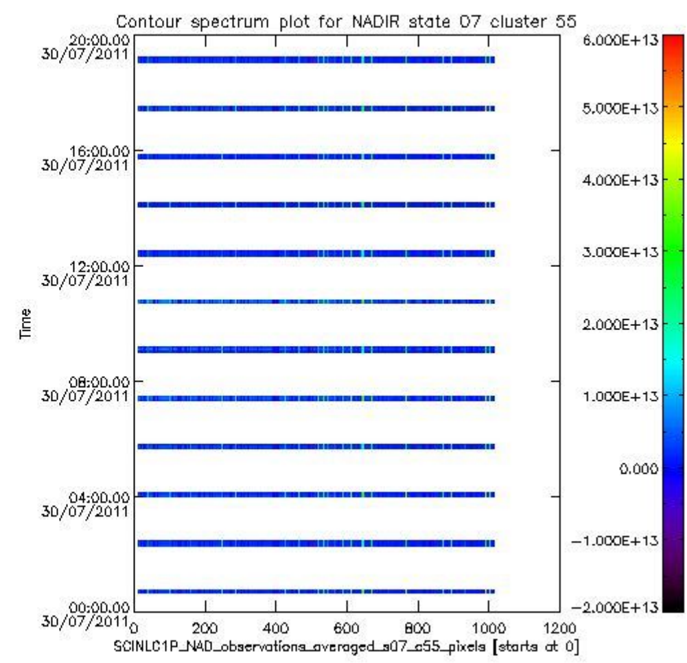
sciamachy_i1b_source_packet_report_SCIA_7_04_U_20110730_8.PNG
