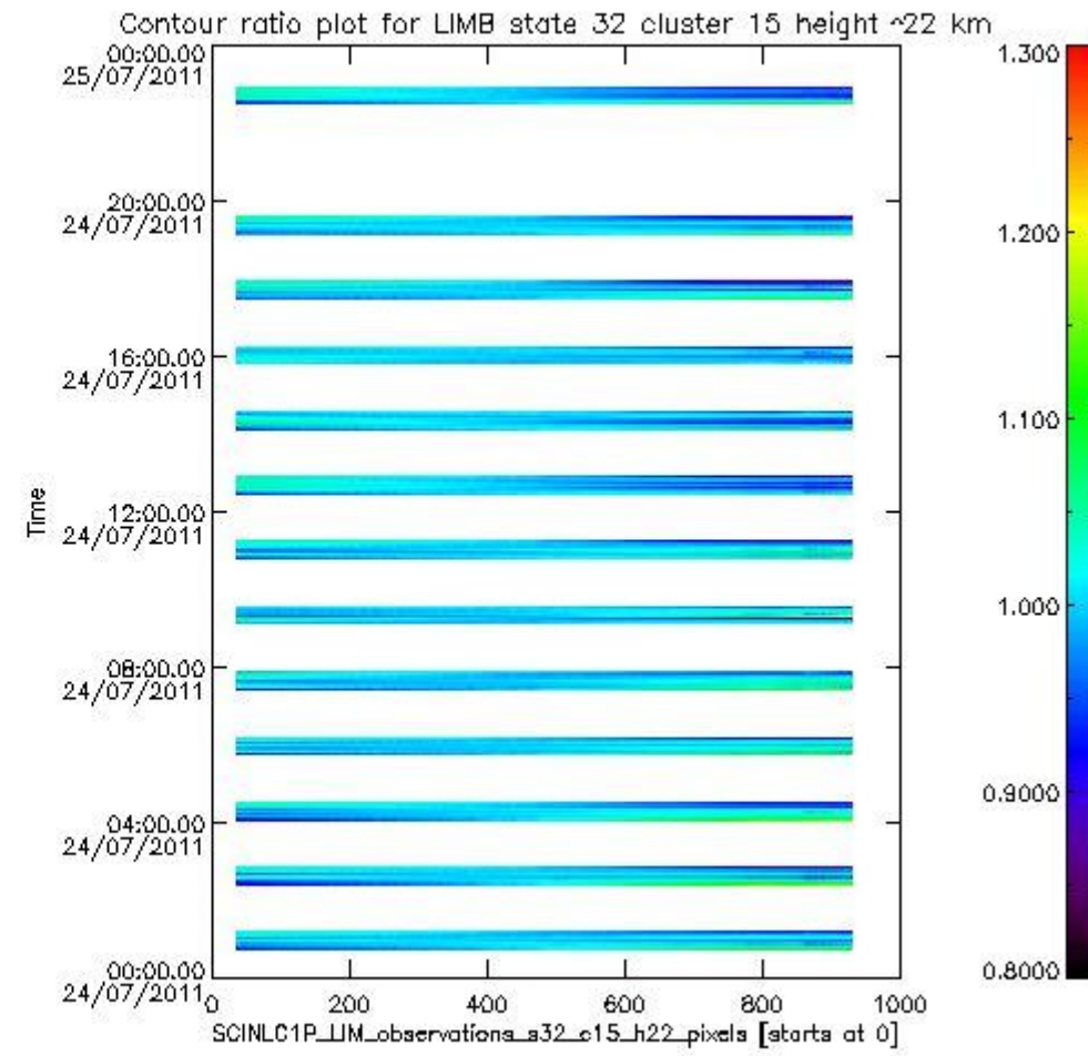
sciamachy_11b_source_packet_report_SCIA_7_04_U_20110724_17.PNG
