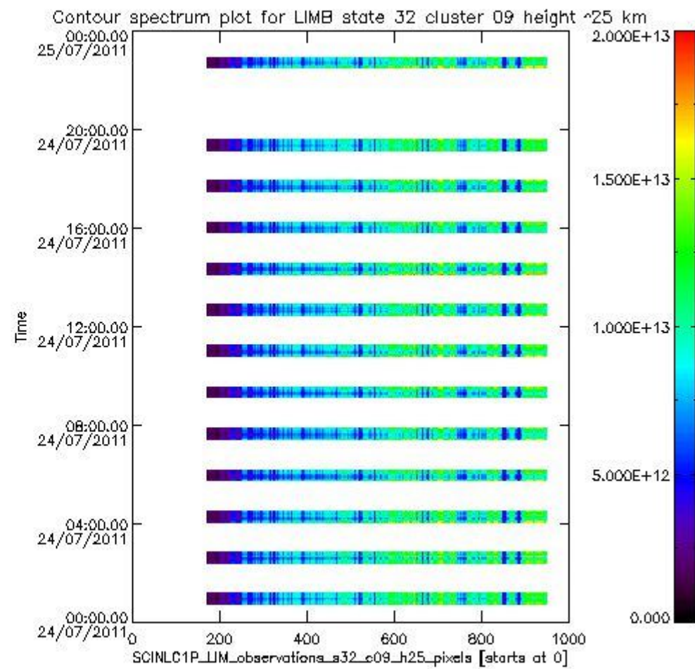
sciamachy_l1b_source_packet_report_SCIA_7_04_U_20110724_14.PNG
