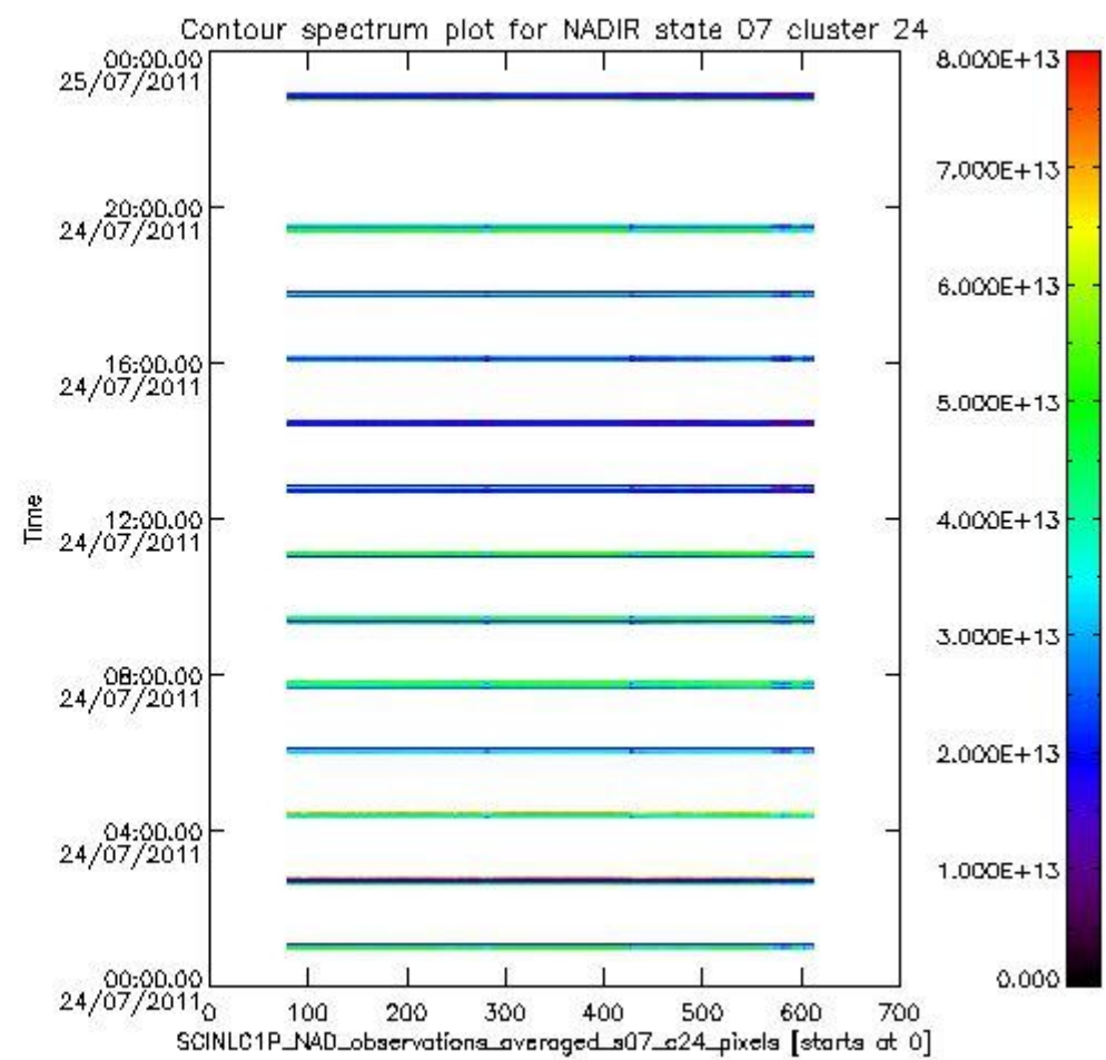
sciamachy_i1b_source_packet_report_SCIA_7_04_U_20110724_6.PNG
