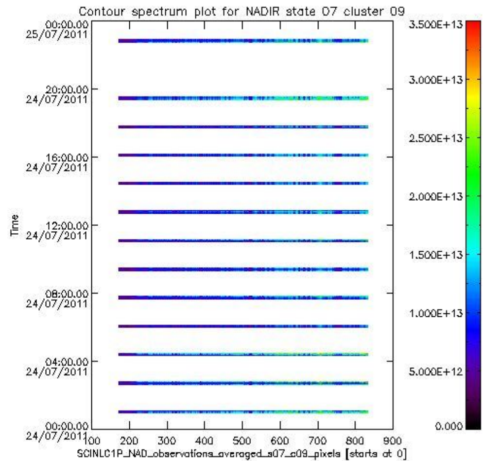
sciamachy_i1b_source_packet_report_SCIA_7_04_U_20110724_2.PNG
