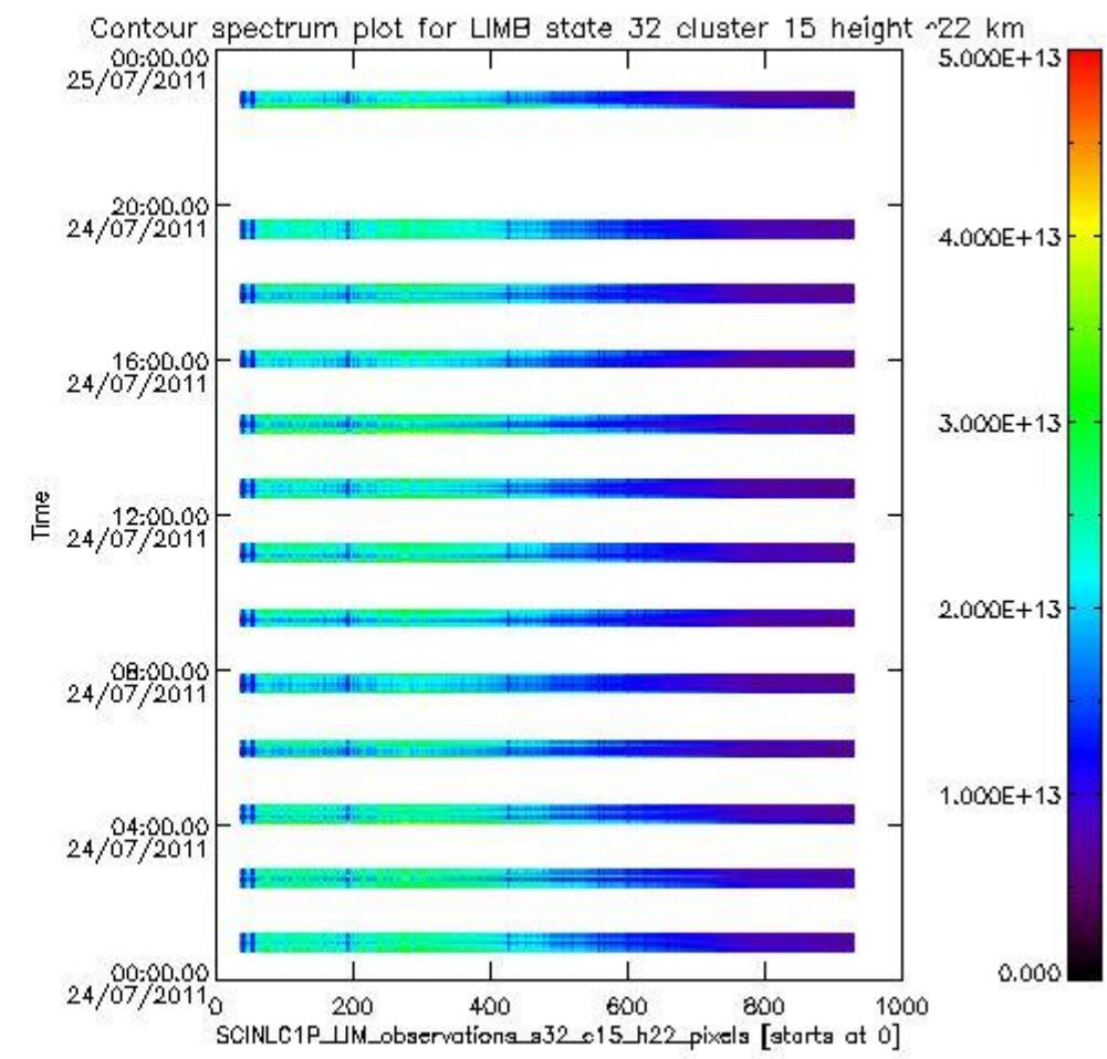
sciamachy_i1b_source_packet_report_SCIA_7_04_U_20110724_16.PNG
