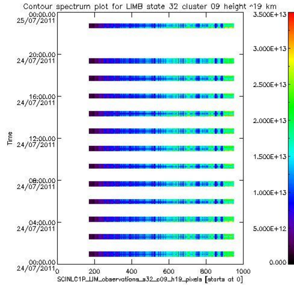
sciamachy_i1b_source_packet_report_SCIA_7_04_U_20110724_10.PNG
