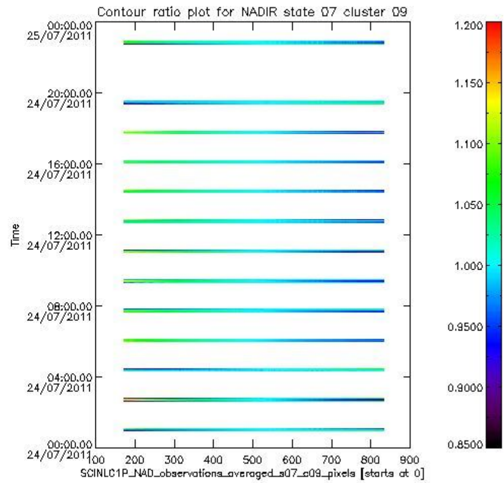
sciamachy_i1b_source_packet_report_SCIA_7_04_U_20110724_3.PNG
