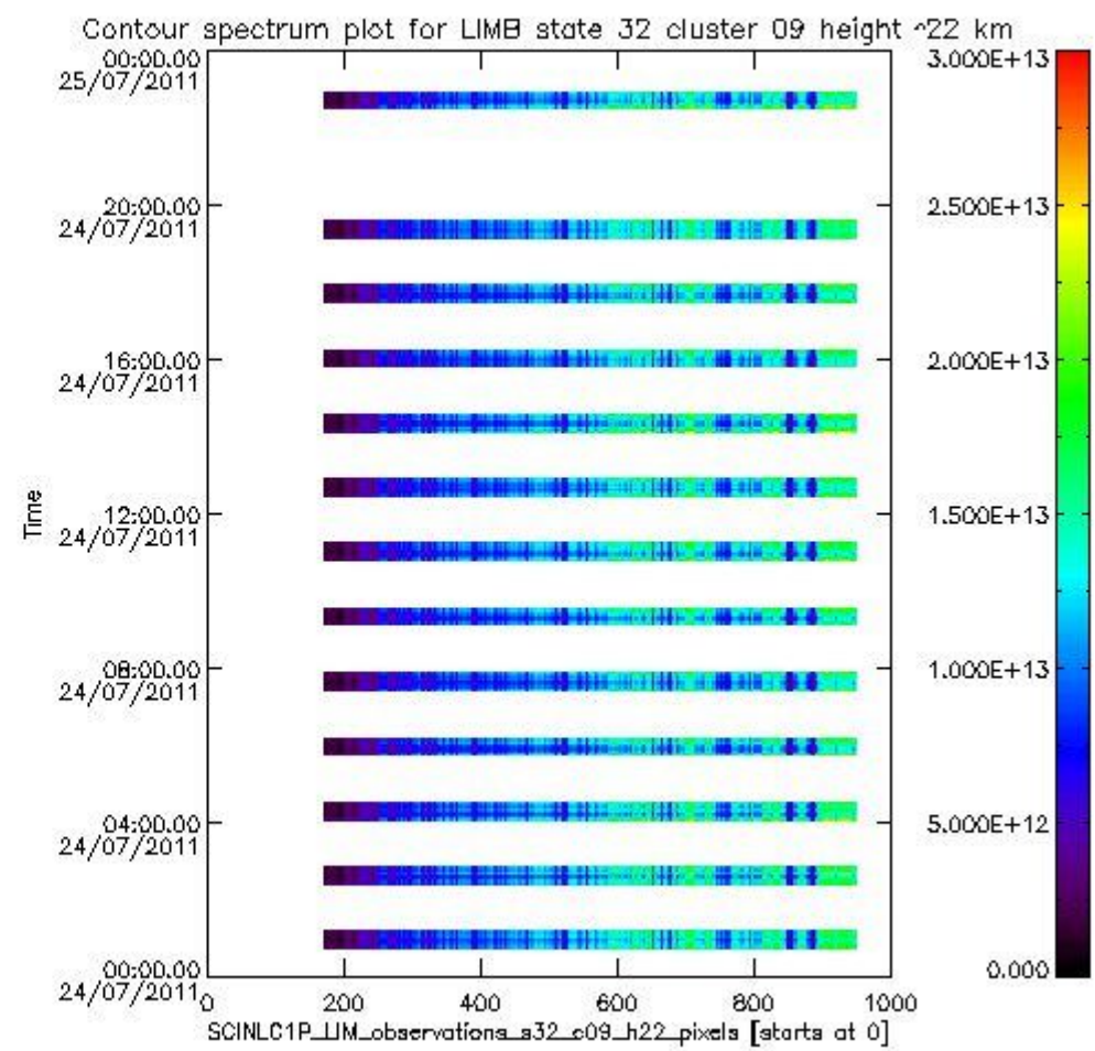
sciamachy_i1b_source_packet_report_SCIA_7_04_U_20110724_12.PNG
