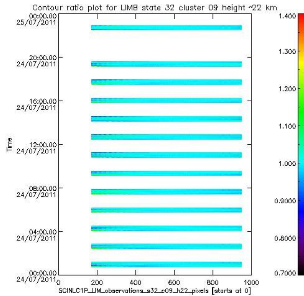
sciamachy_l1b_source_packet_report_SCIA_7_04_U_20110724_13.PNG
