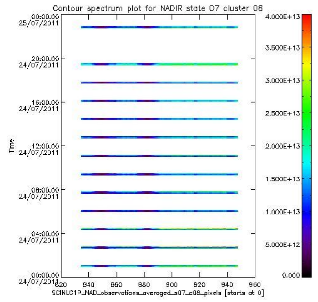
sciamachy_i1b_source_packet_report_SCIA_7_04_U_20110724_0.PNG
