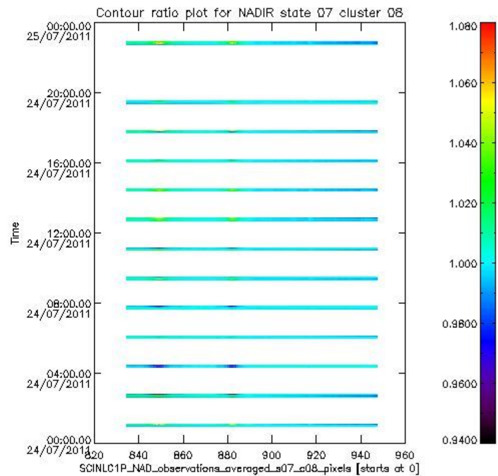
sciamachy_i1b_source_packet_report_SCIA_7_04_U_20110724_1.PNG
