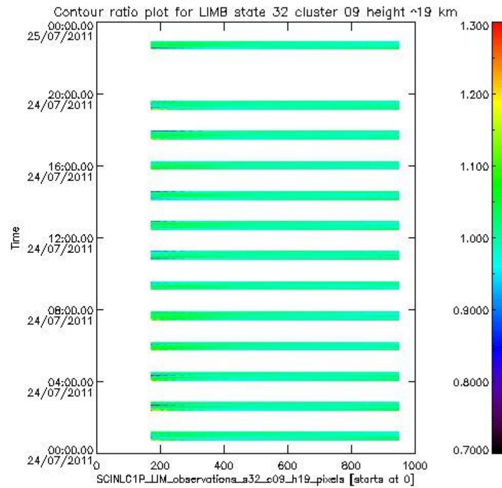
sciamachy_l1b_source_packet_report_SCIA_7_04_U_20110724_11.PNG
