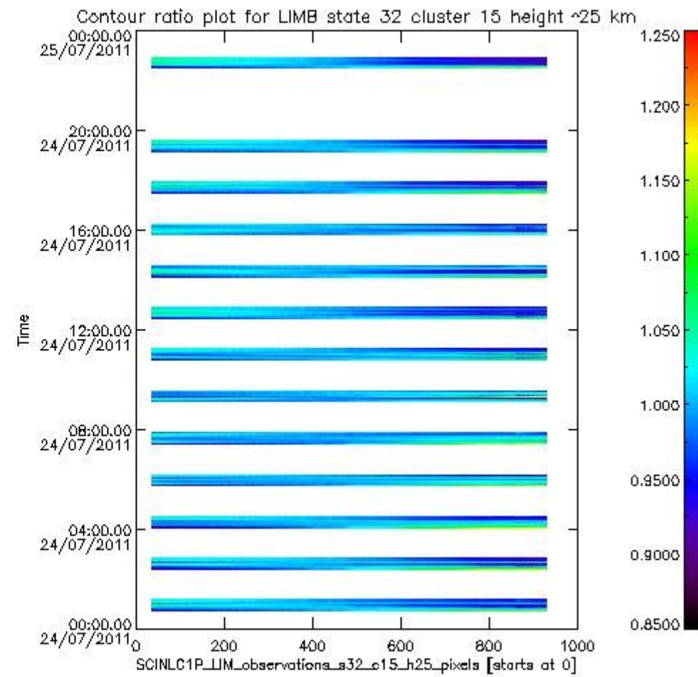
sciamachy_11b_source_packet_report_SCIA_7_04_U_20110724_19.PNG
