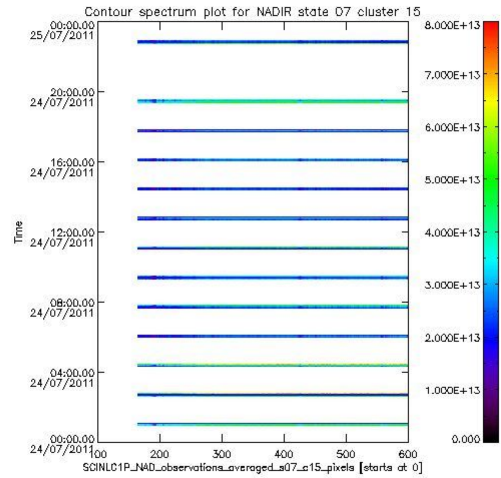
sciamachy_i1b_source_packet_report_SCIA_7_04_U_20110724_4.PNG
