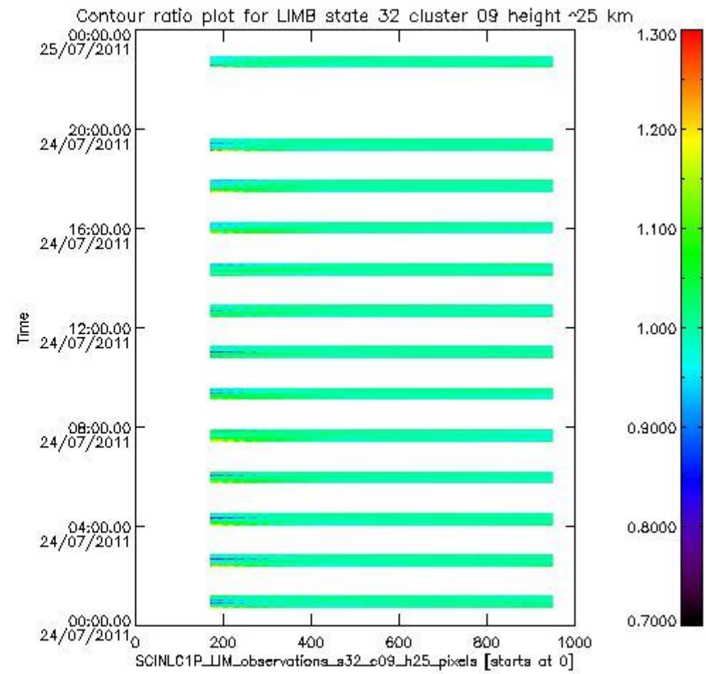
sciamachy_l1b_source_packet_report_SCIA_7_04_U_20110724_15.PNG
