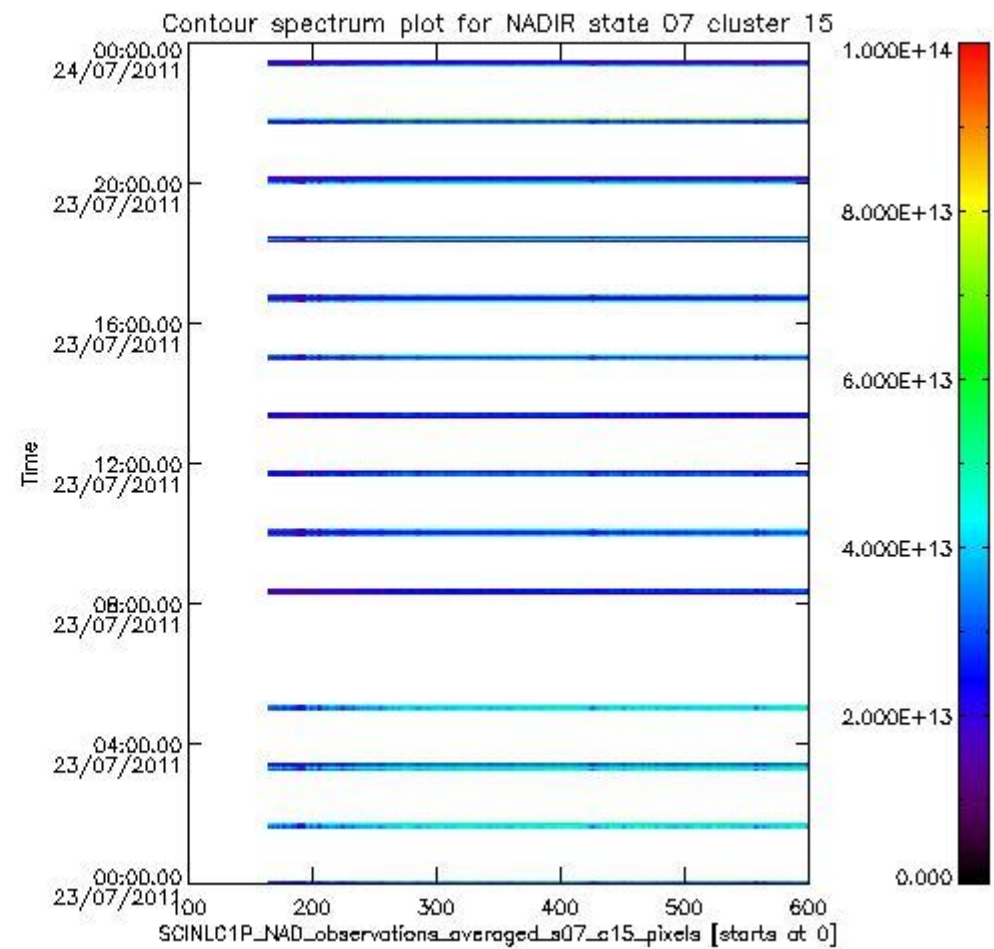
sciamachy_i1b_source_packet_report_SCIA_7_04_U_20110723_4.PNG
