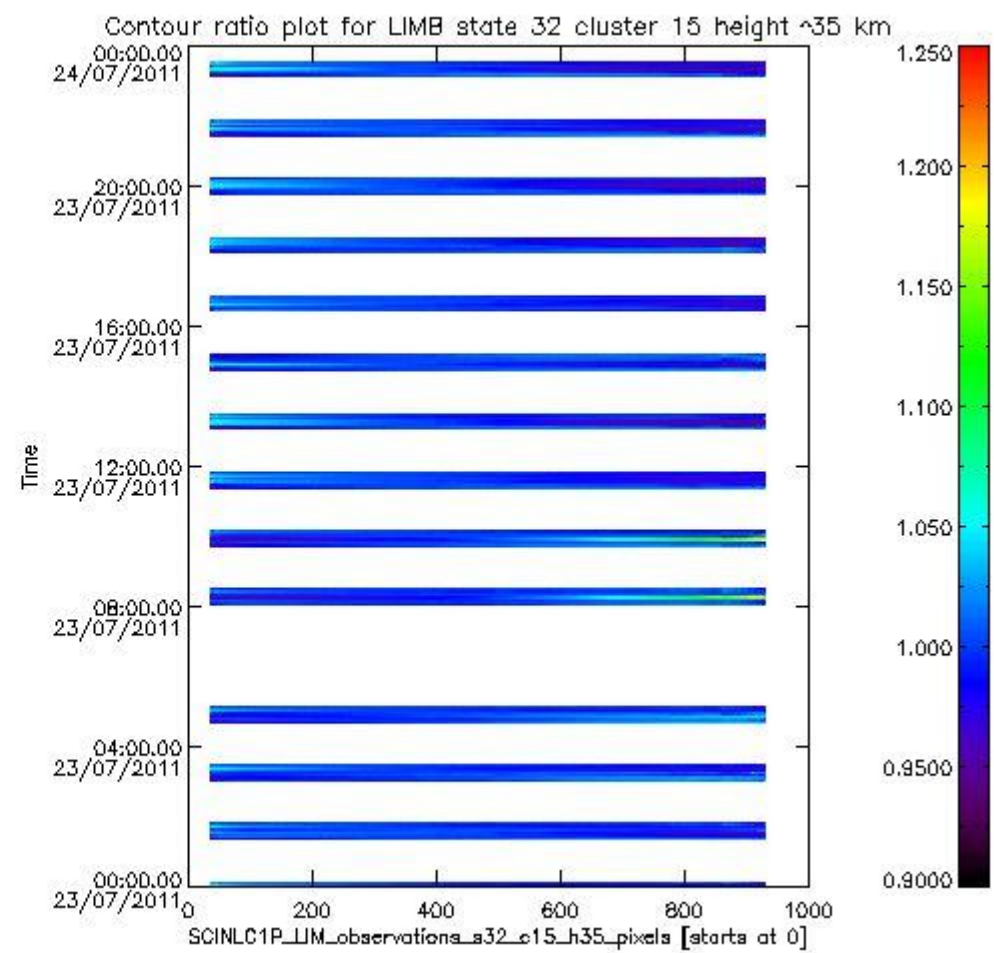
sciamachy_i1b_source_packet_report_SCIA_7_04_U_20110723_21.PNG
