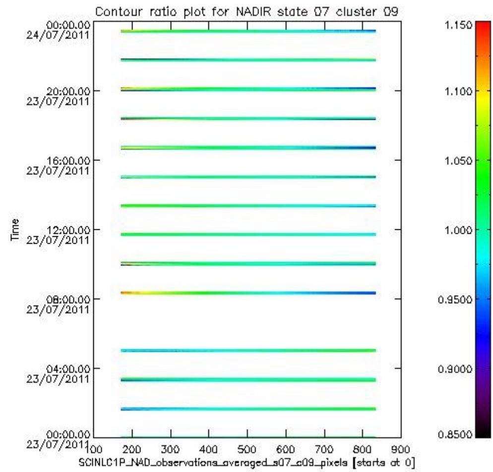
sciamachy_i1b_source_packet_report_SCIA_7_04_U_20110723_3.PNG
