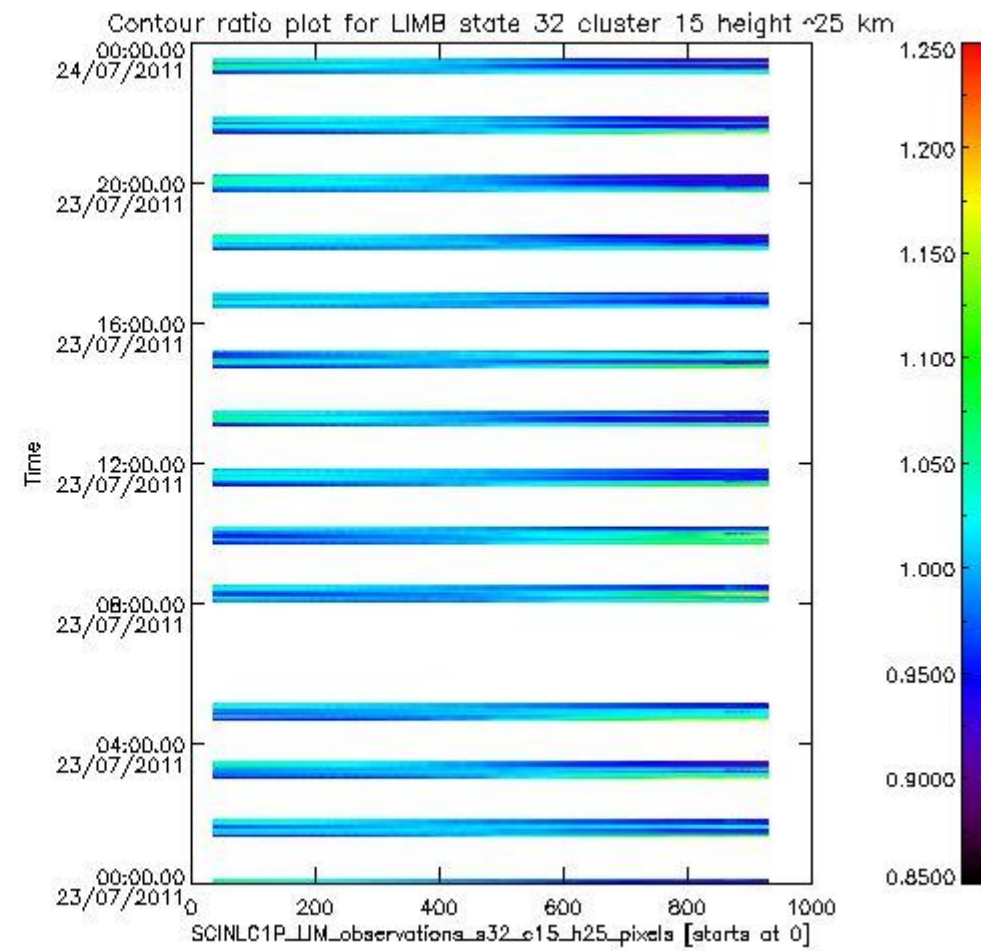
sciamachy_11b_source_packet_report_SCIA_7_04_U_20110723_19.PNG
