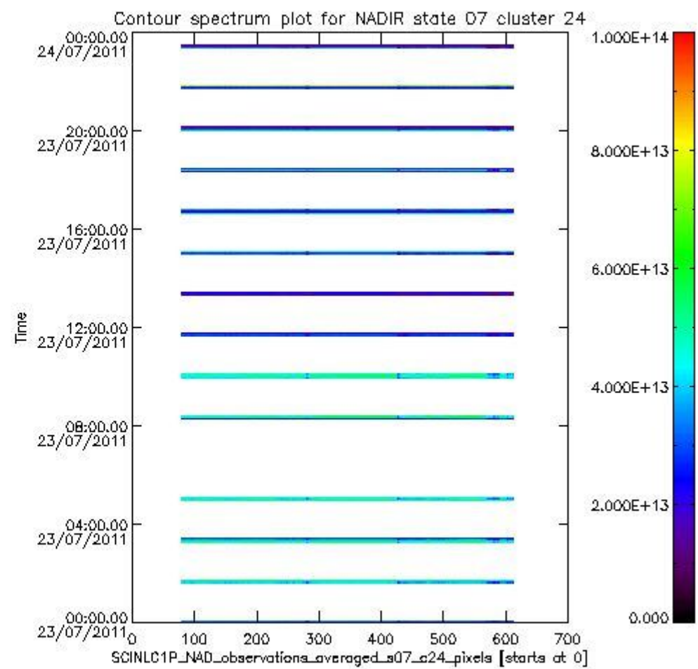
sciamachy_i1b_source_packet_report_SCIA_7_04_U_20110723_6.PNG
