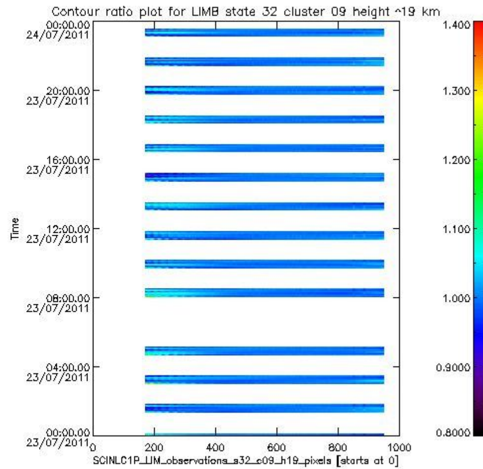
sciamachy_i1b_source_packet_report_SCIA_7_04_U_20110723_11.PNG
