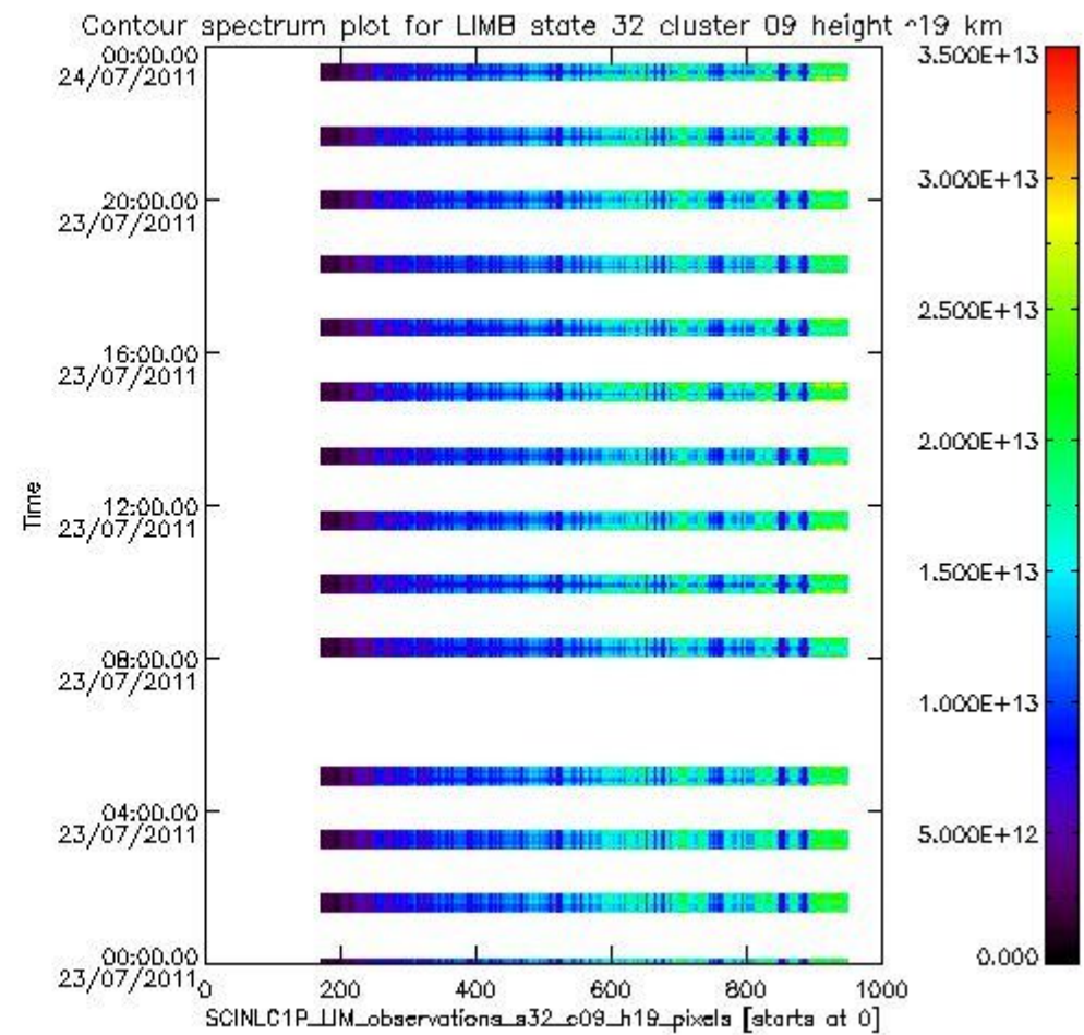
sciamachy_i1b_source_packet_report_SCIA_7_04_U_20110723_10.PNG
