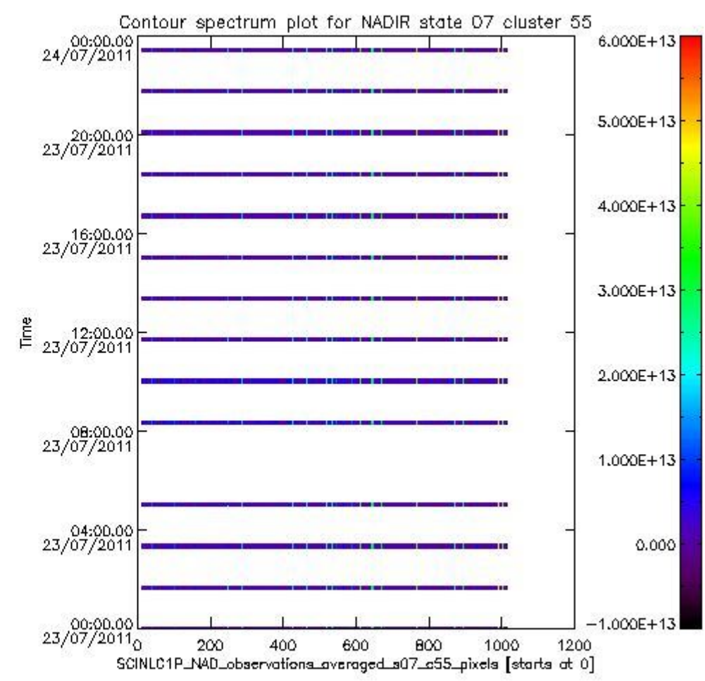
sciamachy_i1b_source_packet_report_SCIA_7_04_U_20110723_8.PNG
