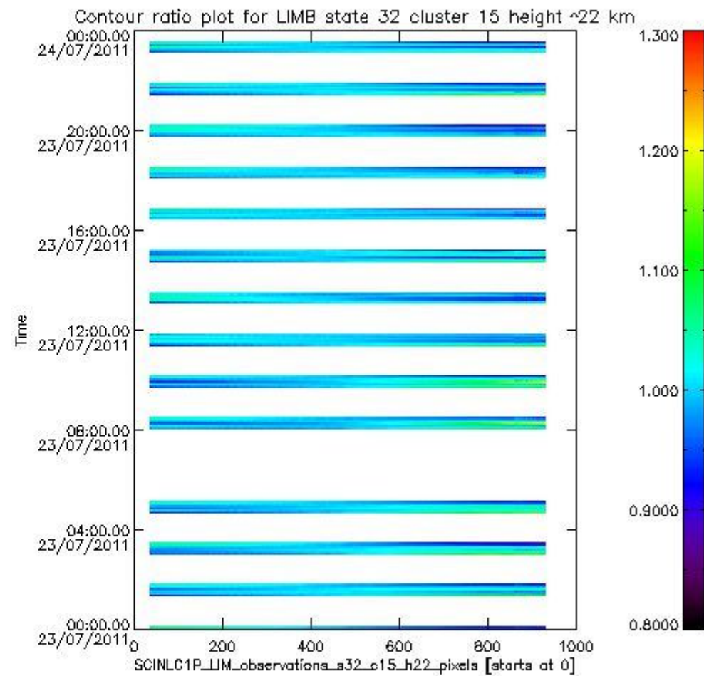
sciamachy_11b_source_packet_report_SCIA_7_04_U_20110723_17.PNG
