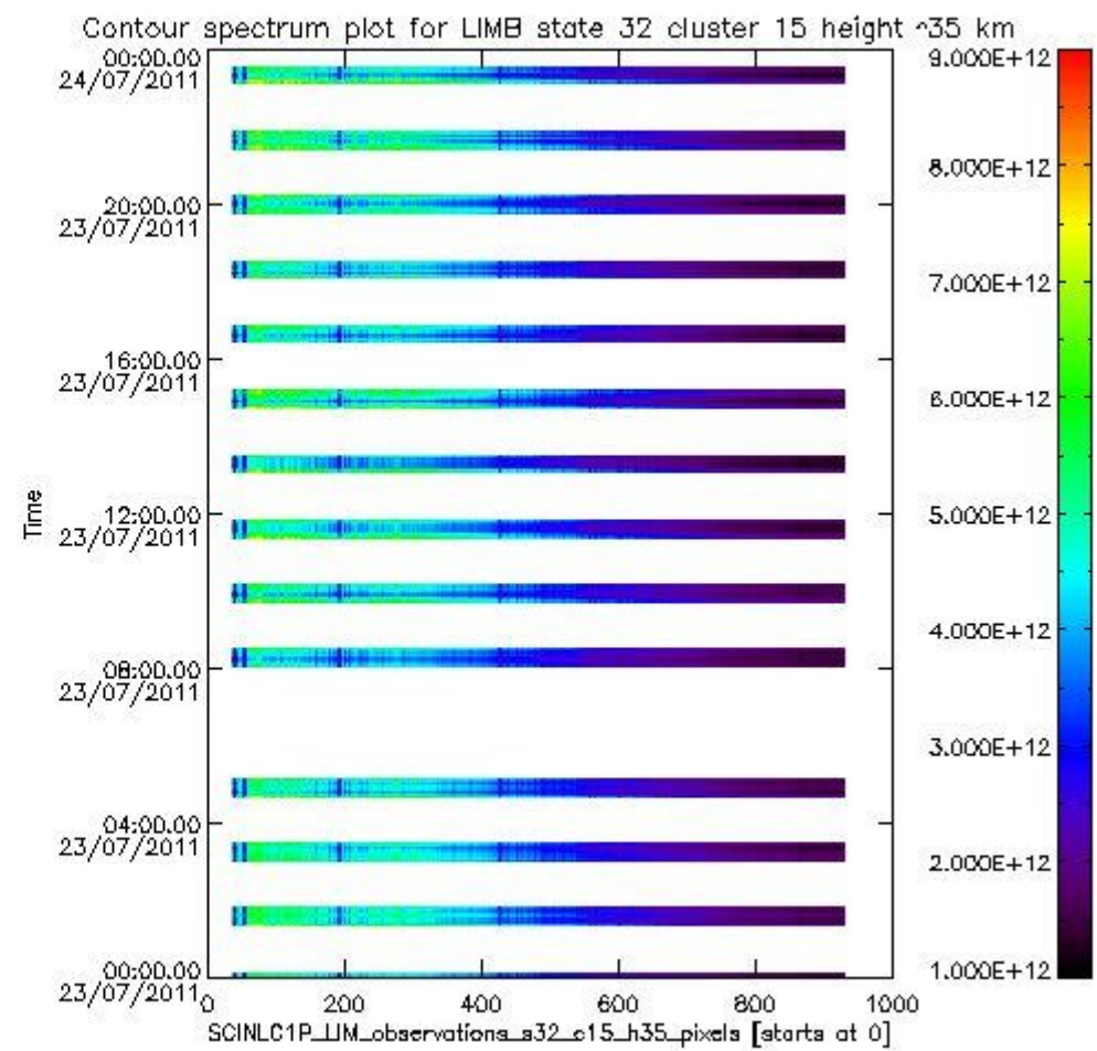
sciamachy_11b_source_packet_report_SCIA_7_04_U_20110723_20.PNG
