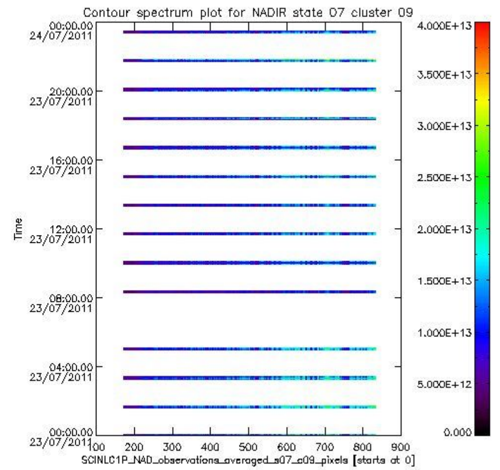
sciamachy_i1b_source_packet_report_SCIA_7_04_U_20110723_2.PNG
