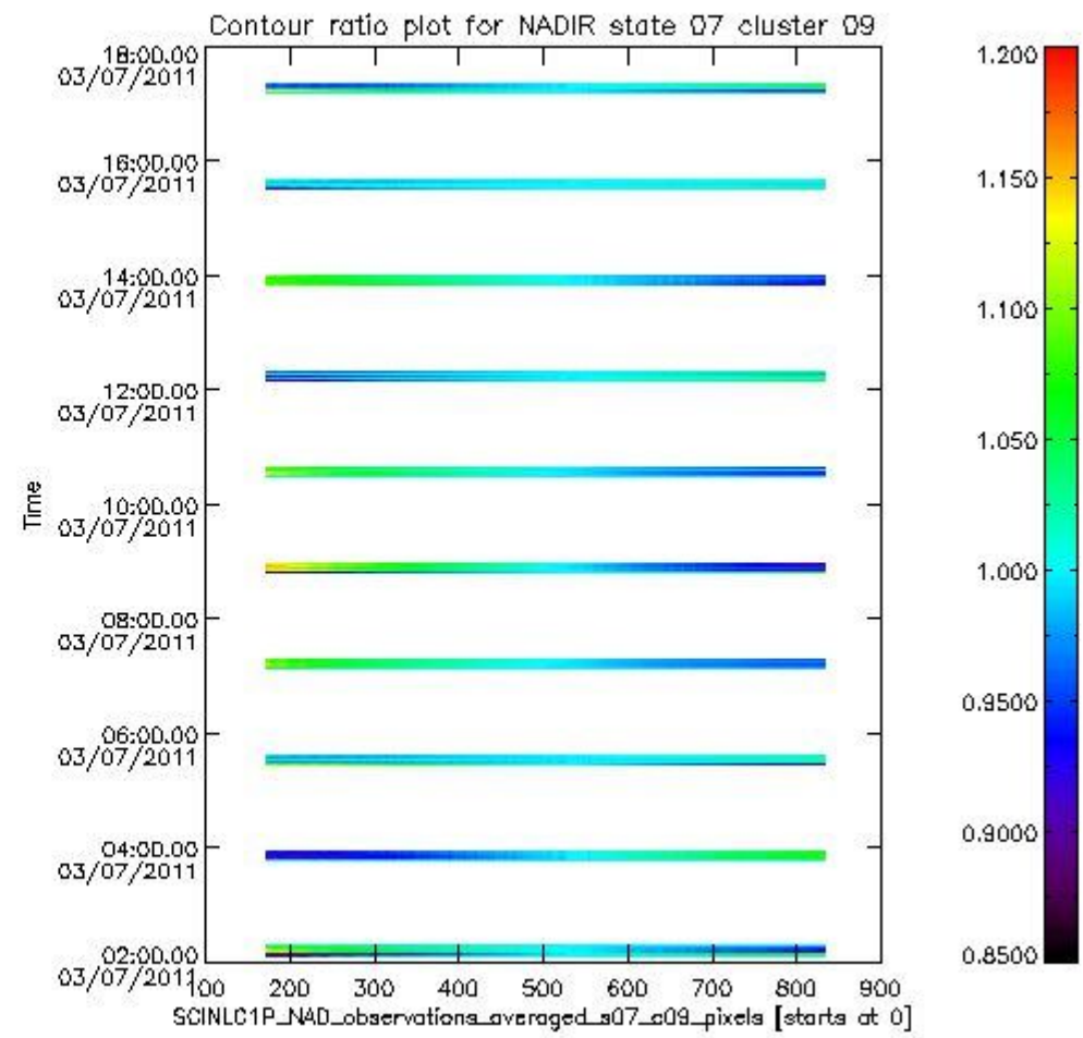
sciamachy_i1b_source_packet_report_SCIA_7_04_U_20110703_3.PNG
