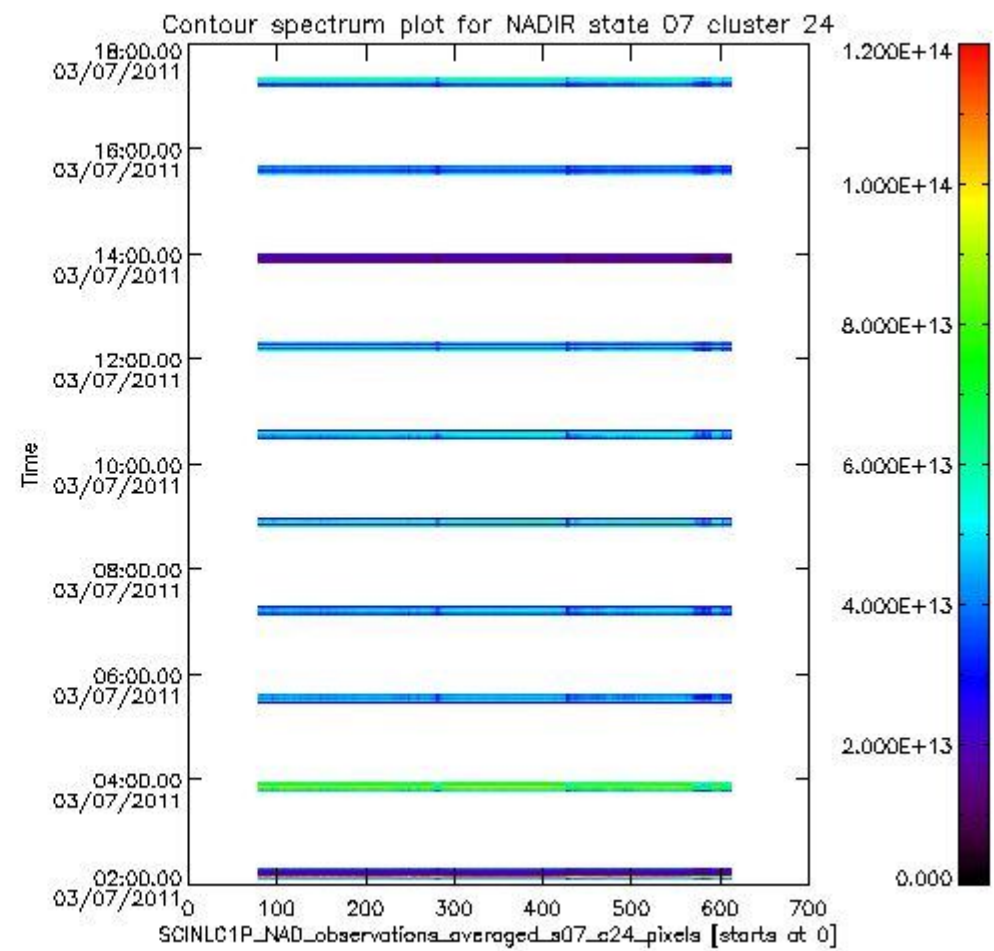
sciamachy_i1b_source_packet_report_SCIA_7_04_U_20110703_6.PNG
