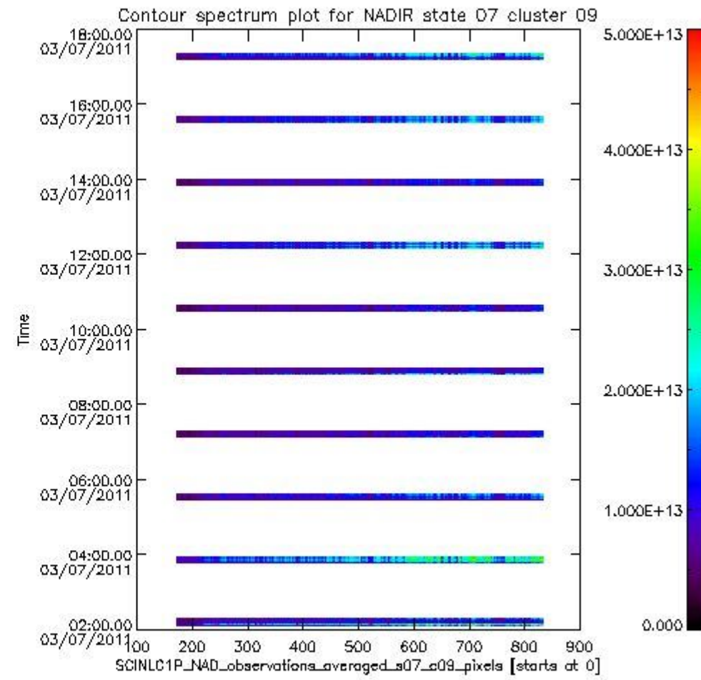
sciamachy_i1b_source_packet_report_SCIA_7_04_U_20110703_2.PNG
