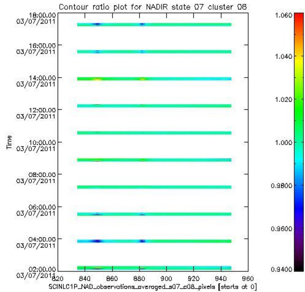
sciamachy_i1b_source_packet_report_SCIA_7_04_U_20110703_1.PNG
