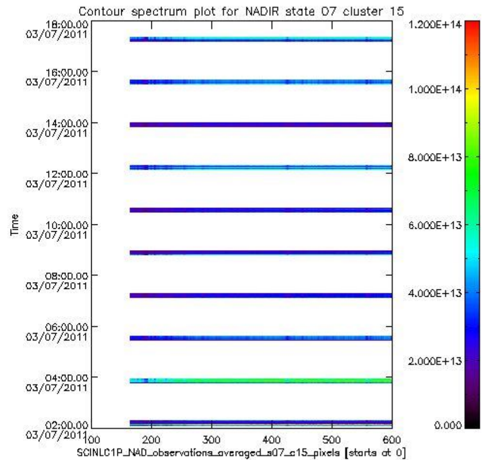
sciamachy_i1b_source_packet_report_SCIA_7_04_U_20110703_4.PNG
