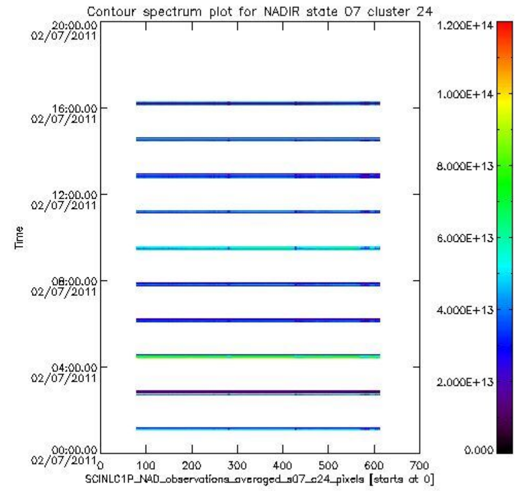
sciamachy_i1b_source_packet_report_SCIA_7_04_U_20110702_6.PNG
