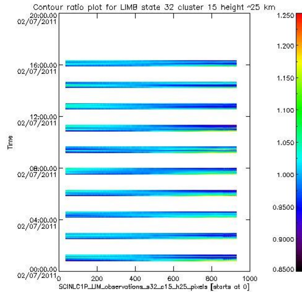
sciamachy_11b_source_packet_report_SCIA_7_04_U_20110702_19.PNG
