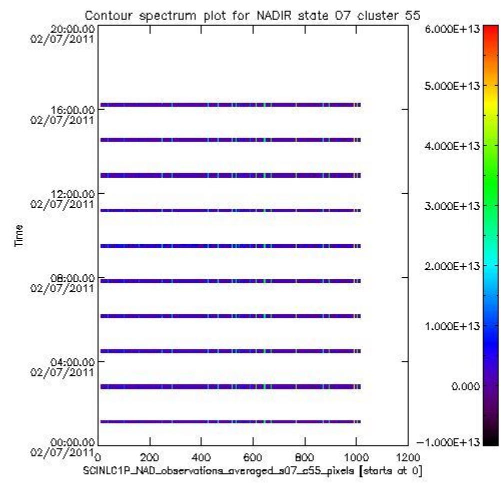
sciamachy_i1b_source_packet_report_SCIA_7_04_U_20110702_8.PNG
