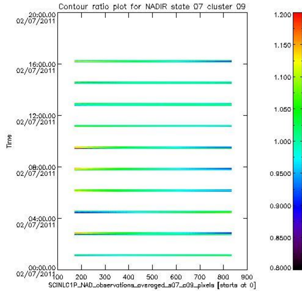
sciamachy_i1b_source_packet_report_SCIA_7_04_U_20110702_3.PNG
