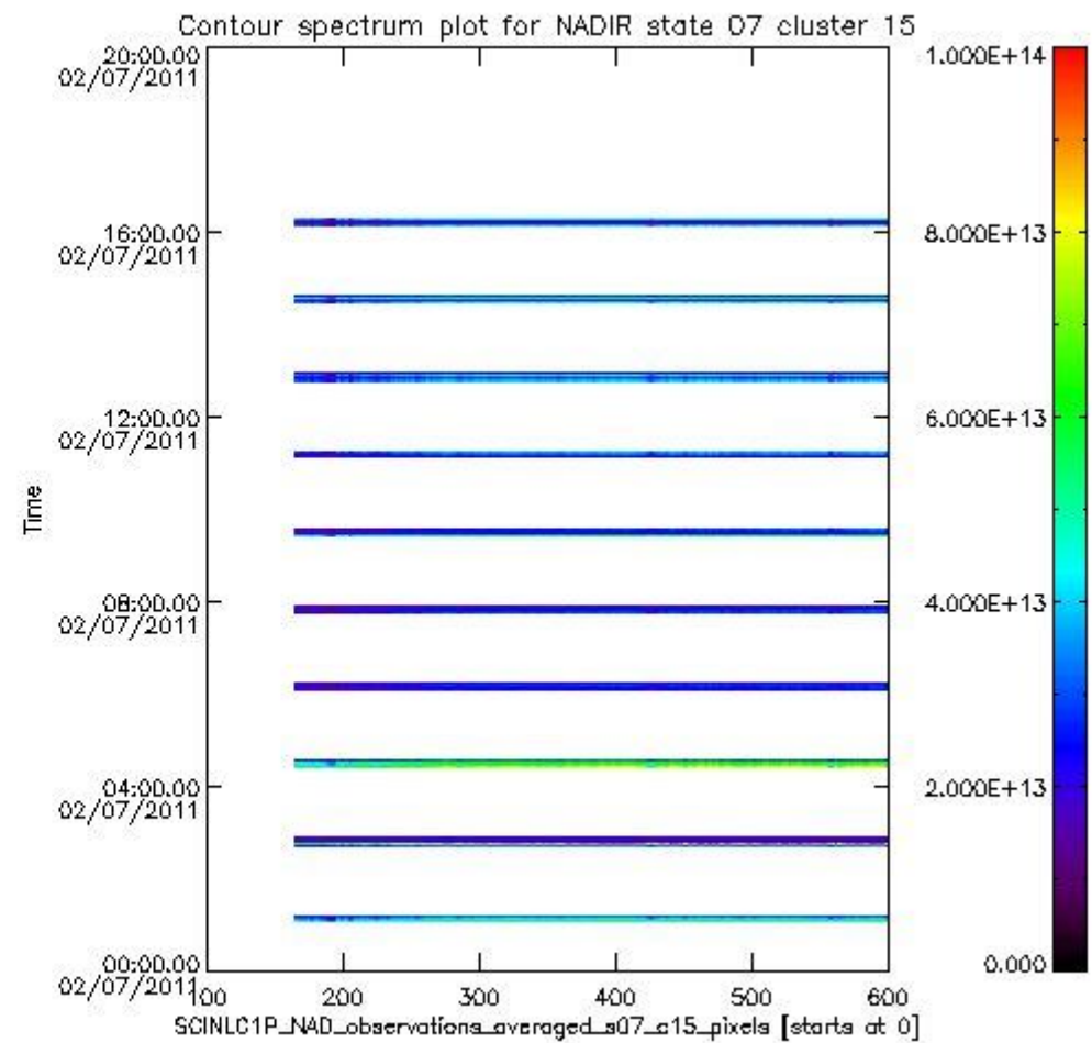
sciamachy_i1b_source_packet_report_SCIA_7_04_U_20110702_4.PNG
