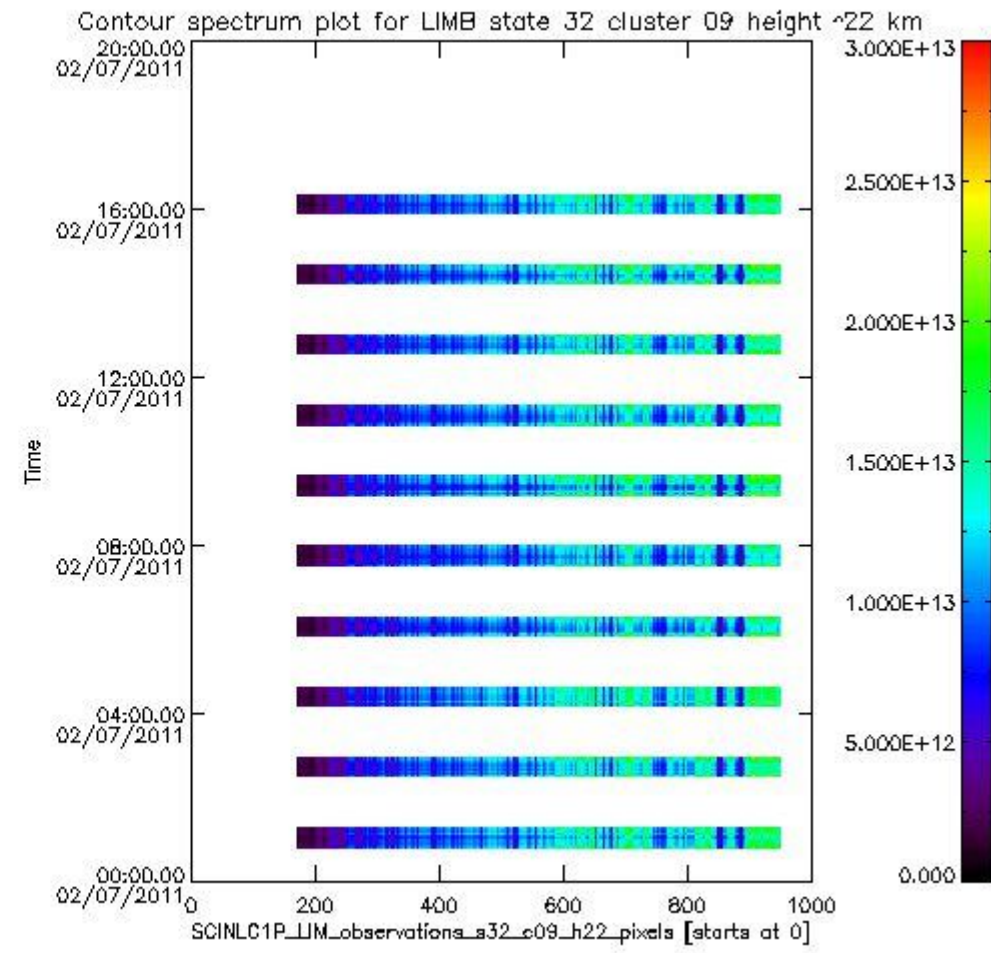
sciamachy_i1b_source_packet_report_SCIA_7_04_U_20110702_12.PNG
