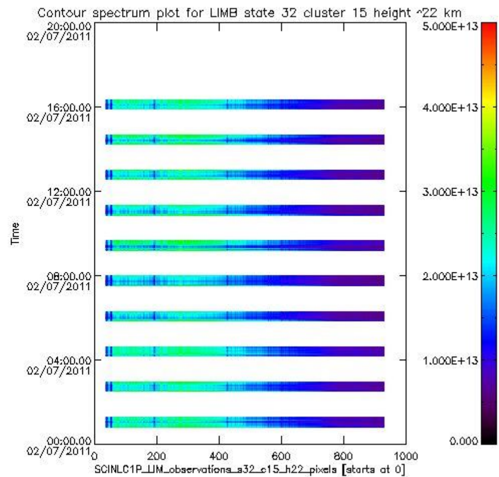
sciamachy_i1b_source_packet_report_SCIA_7_04_U_20110702_16.PNG
