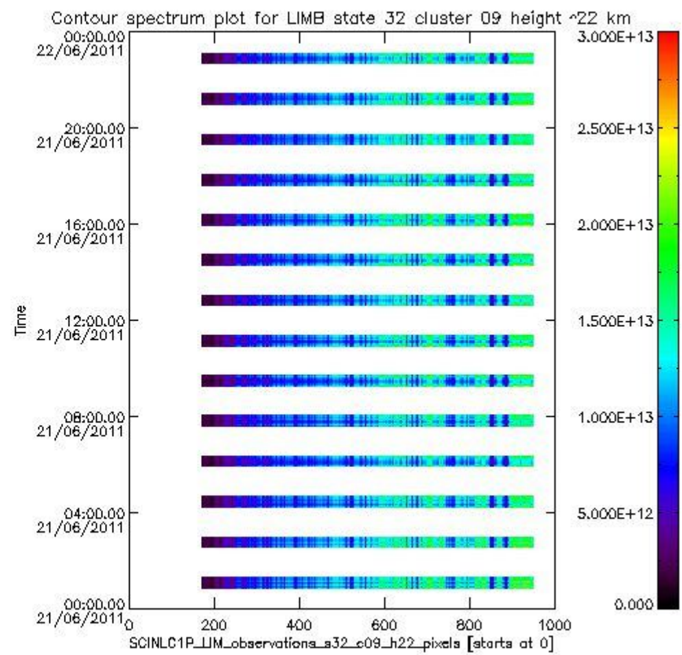
sciamachy_i1b_source_packet_report_SCIA_7_04_U_20110621_12.PNG
