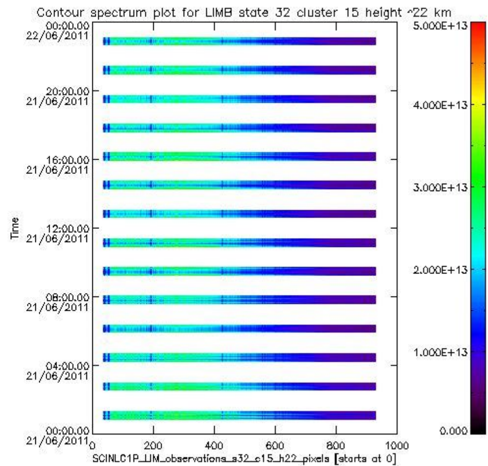
sciamachy_i1b_source_packet_report_SCIA_7_04_U_20110621_16.PNG
