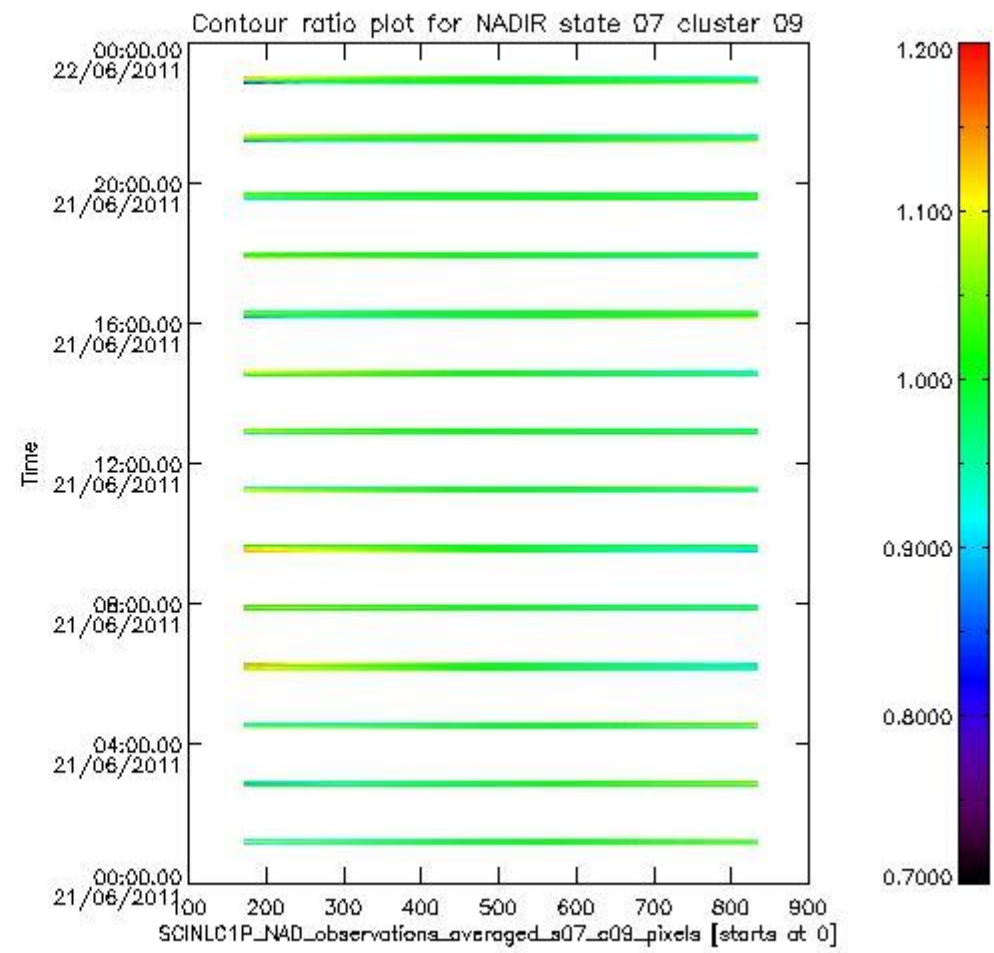
sciamachy_i1b_source_packet_report_SCIA_7_04_U_20110621_3.PNG
