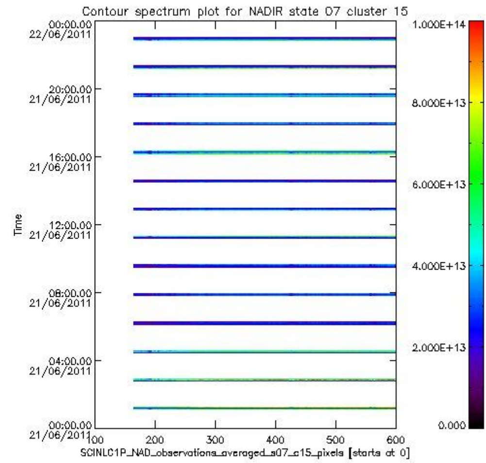
sciamachy_i1b_source_packet_report_SCIA_7_04_U_20110621_4.PNG
