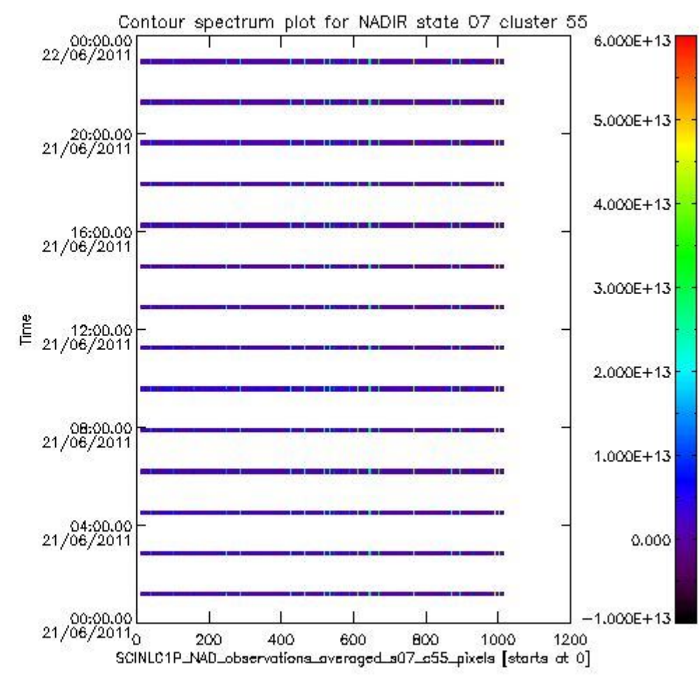
sciamachy_i1b_source_packet_report_SCIA_7_04_U_20110621_8.PNG
