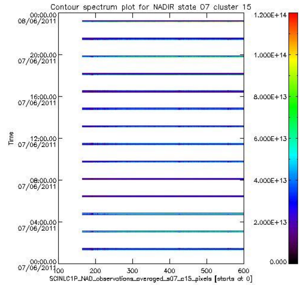
sciamachy_i1b_source_packet_report_SCIA_7_04_U_20110607_4.PNG
