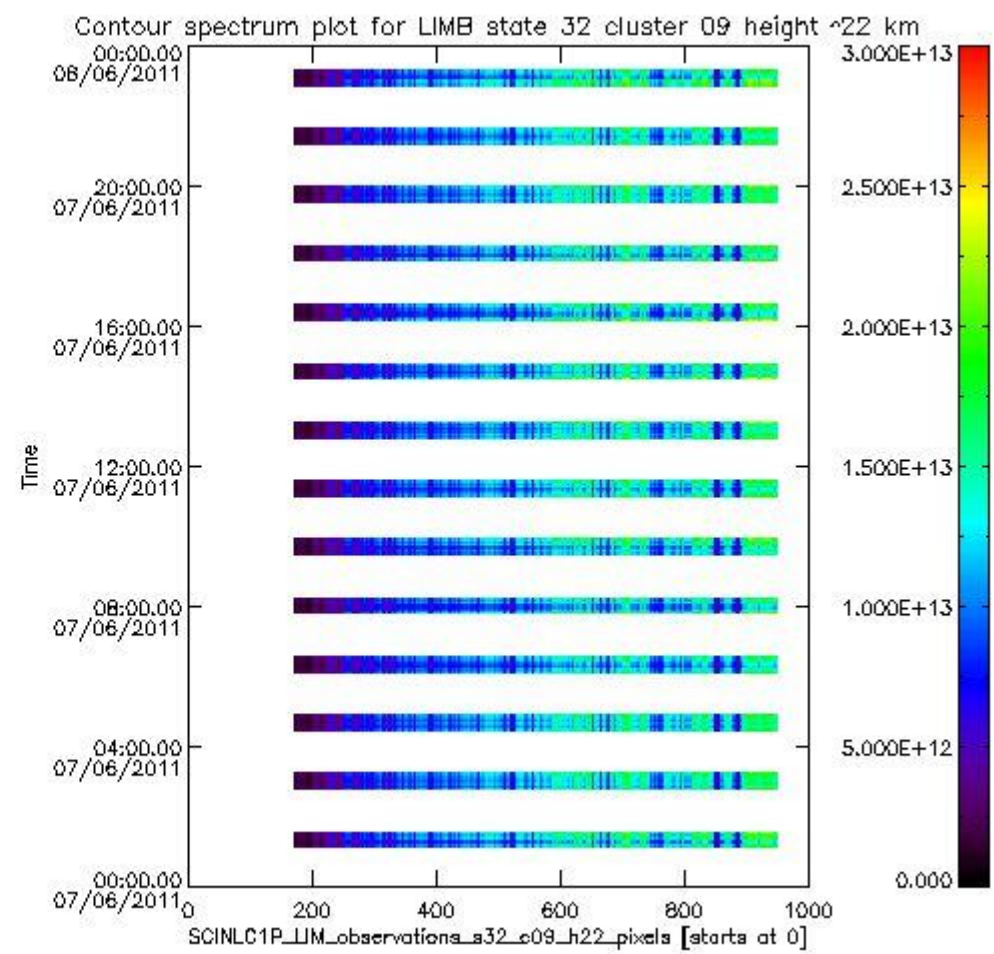
sciamachy_i1b_source_packet_report_SCIA_7_04_U_20110607_12.PNG
