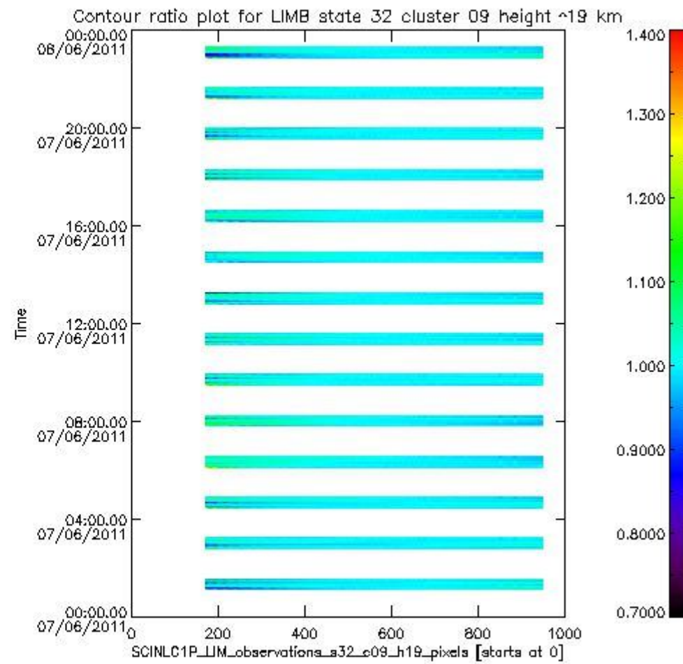
sciamachy_i1b_source_packet_report_SCIA_7_04_U_20110607_11.PNG
