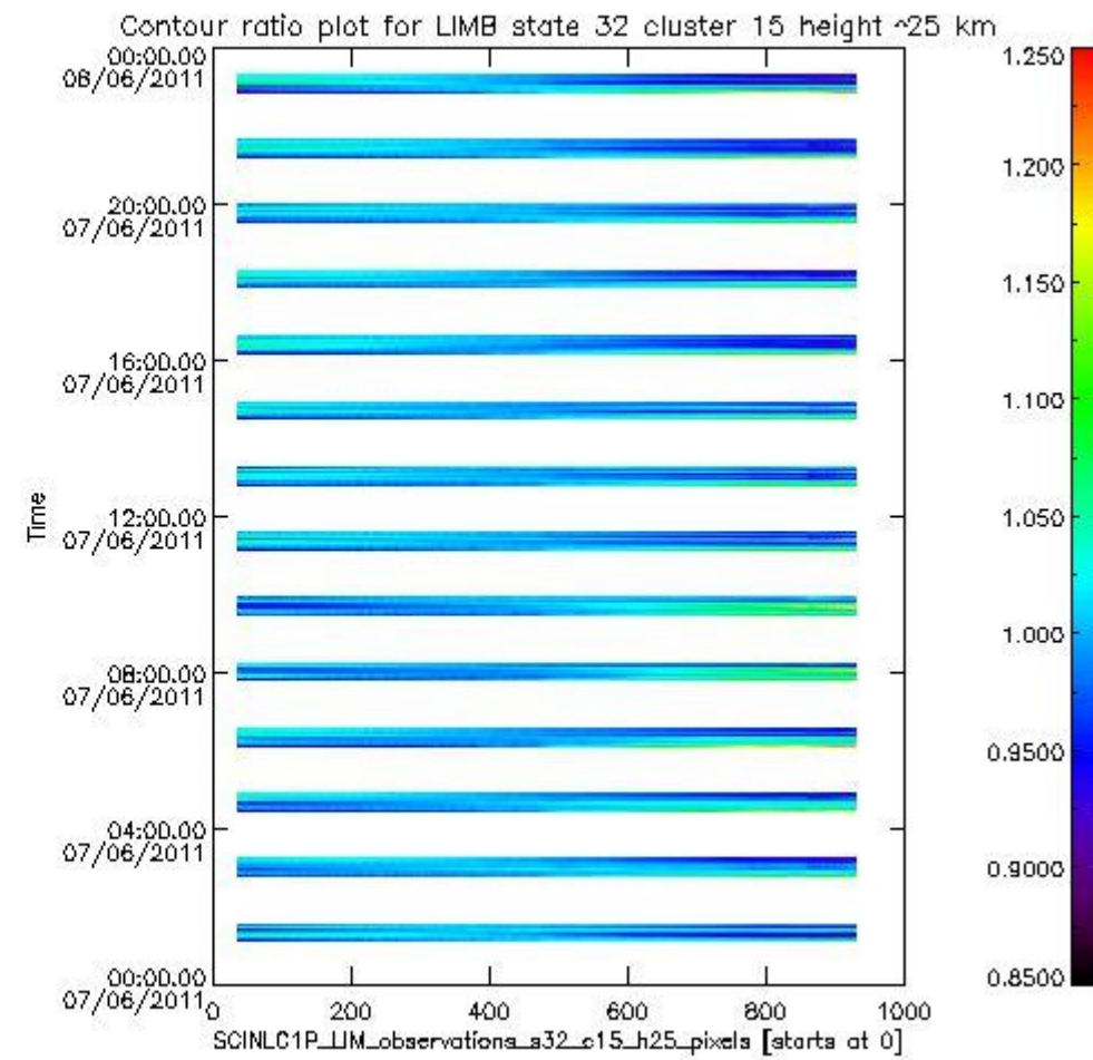
sciamachy_11b_source_packet_report_SCIA_7_04_U_20110607_19.PNG
