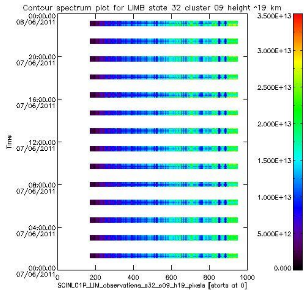
sciamachy_i1b_source_packet_report_SCIA_7_04_U_20110607_10.PNG
