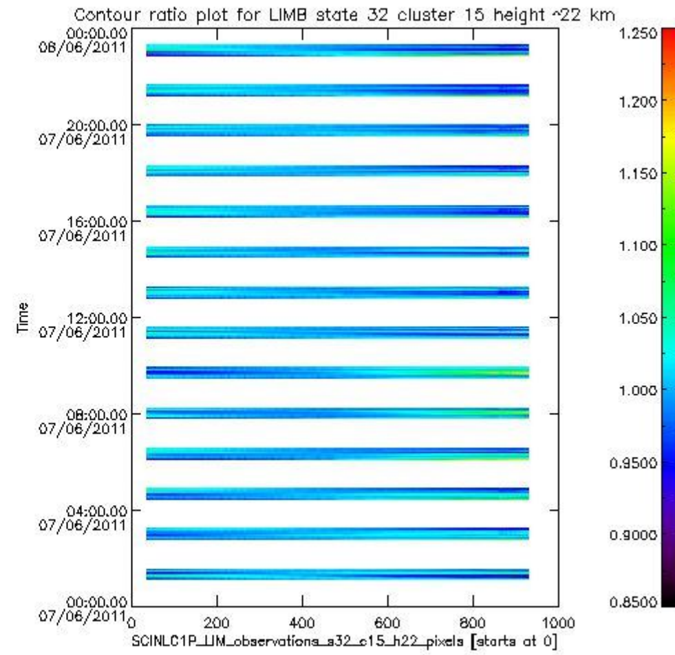
sciamachy_11b_source_packet_report_SCIA_7_04_U_20110607_17.PNG
