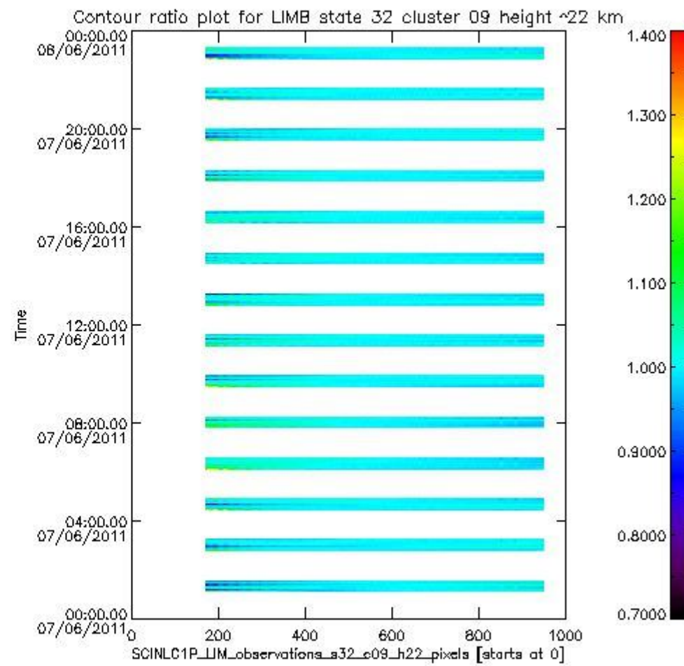
sciamachy_l1b_source_packet_report_SCIA_7_04_U_20110607_13.PNG
