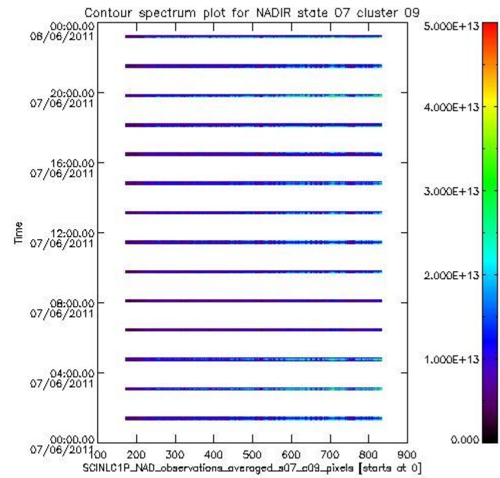
sciamachy_i1b_source_packet_report_SCIA_7_04_U_20110607_2.PNG
