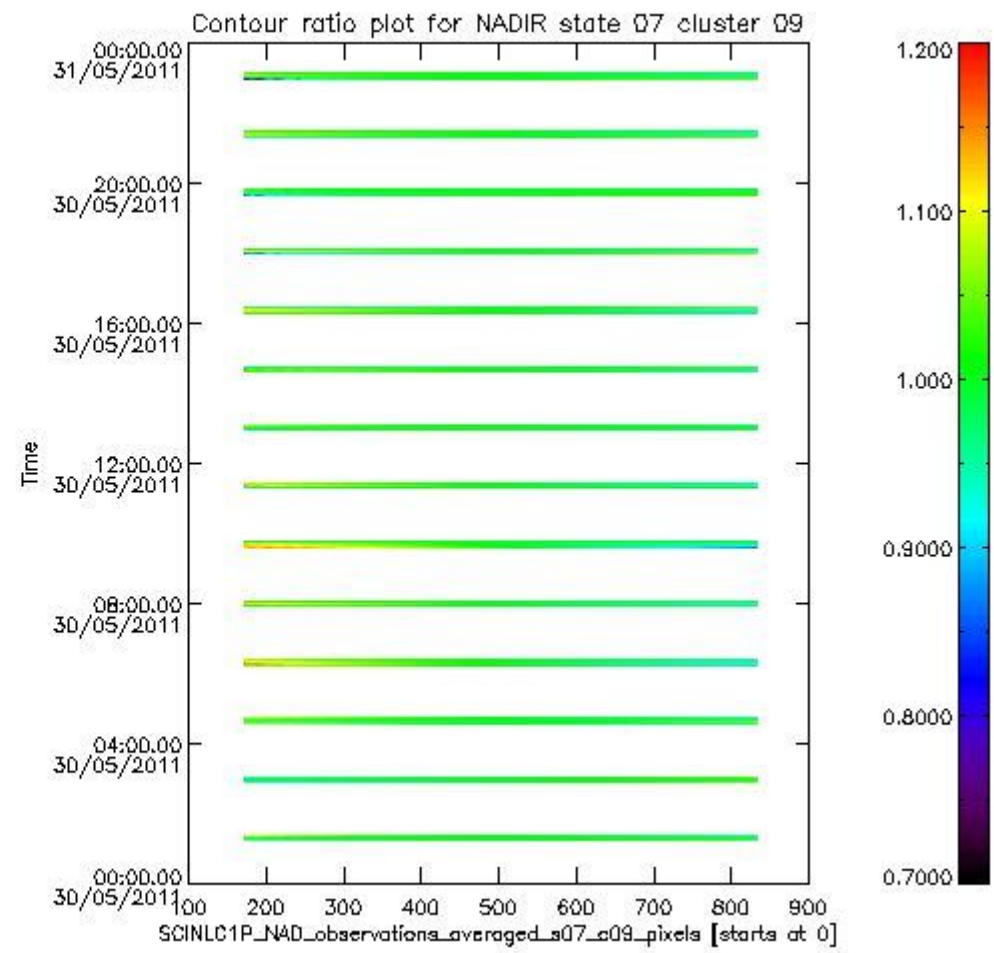
sciamachy_i1b_source_packet_report_SCIA_7_04_U_20110530_3.PNG
