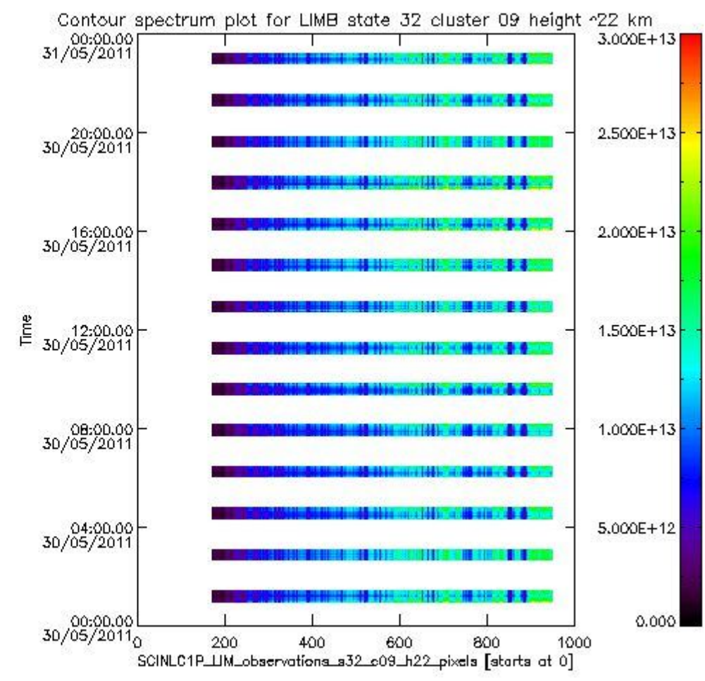
sciamachy_i1b_source_packet_report_SCIA_7_04_U_20110530_12.PNG
