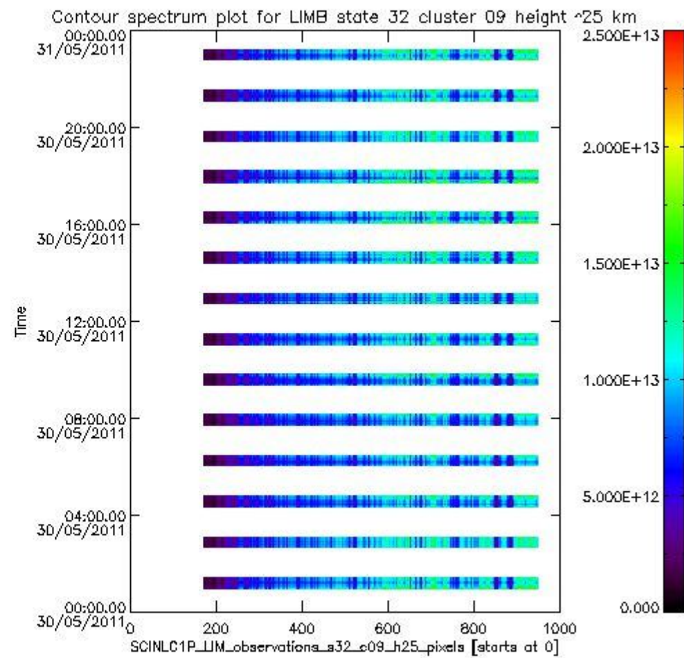
sciamachy_i1b_source_packet_report_SCIA_7_04_U_20110530_14.PNG
