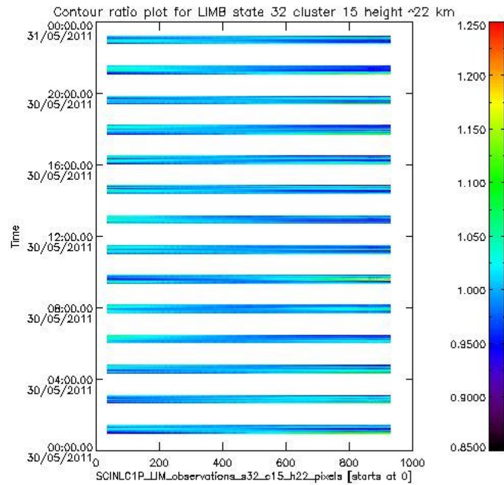
sciamachy_11b_source_packet_report_SCIA_7_04_U_20110530_17.PNG
