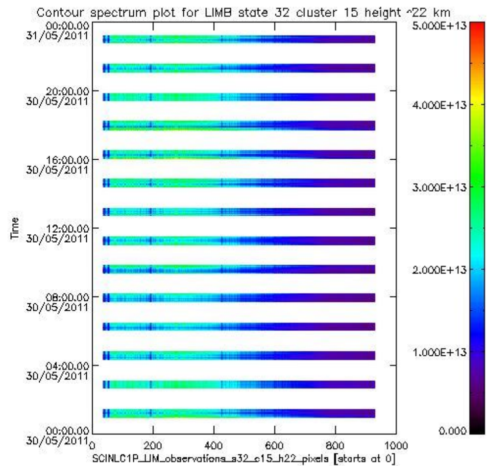
sciamachy_i1b_source_packet_report_SCIA_7_04_U_20110530_16.PNG
