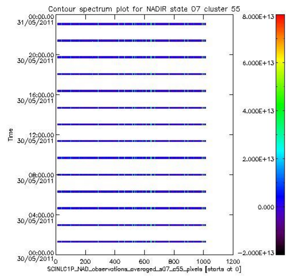
sciamachy_i1b_source_packet_report_SCIA_7_04_U_20110530_8.PNG
