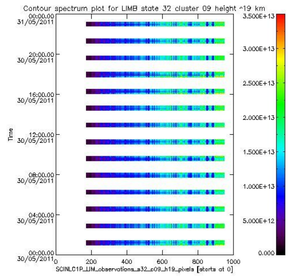
sciamachy_i1b_source_packet_report_SCIA_7_04_U_20110530_10.PNG
