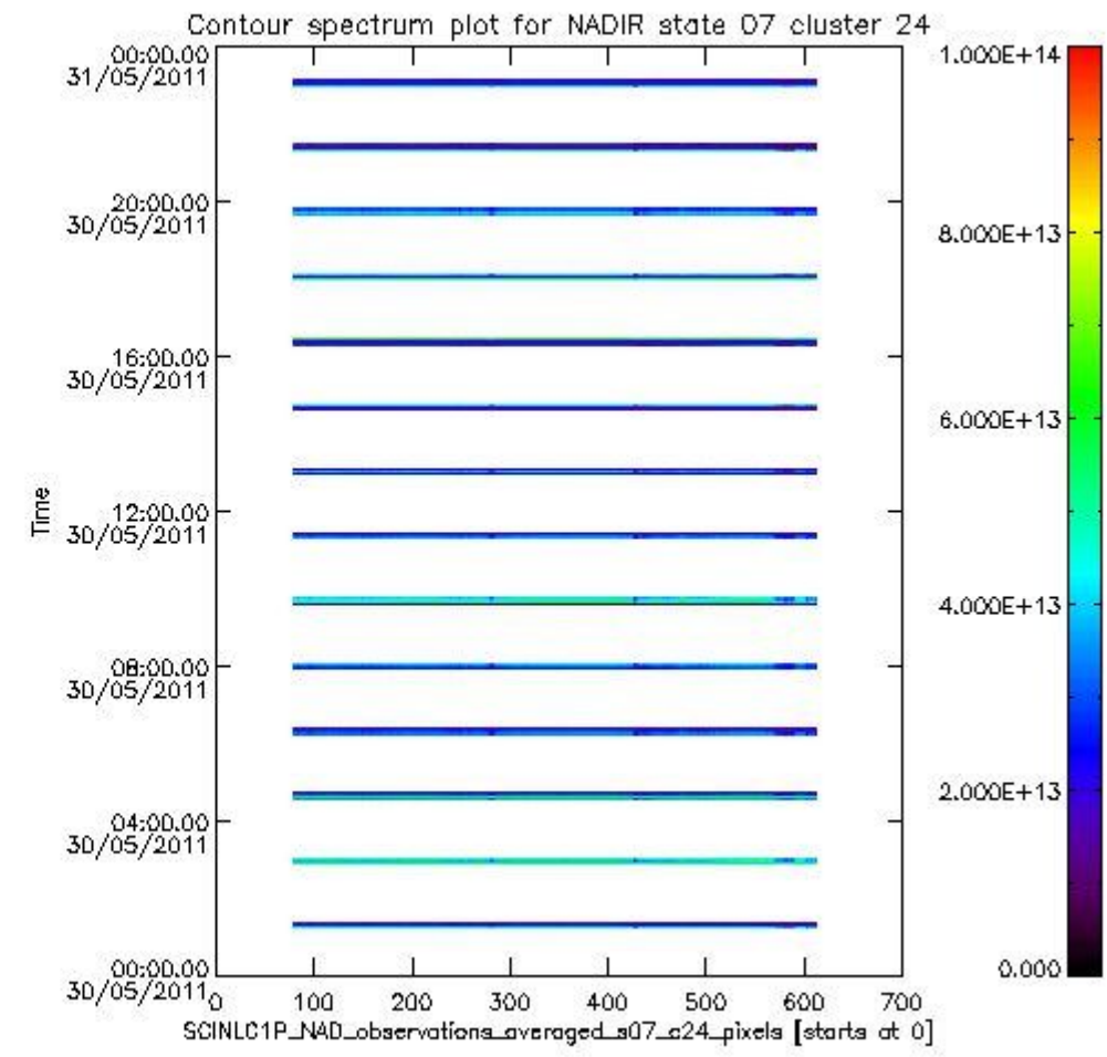
sciamachy_i1b_source_packet_report_SCIA_7_04_U_20110530_6.PNG
