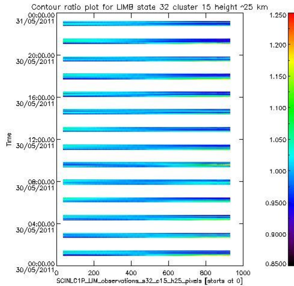
sciamachy_11b_source_packet_report_SCIA_7_04_U_20110530_19.PNG
