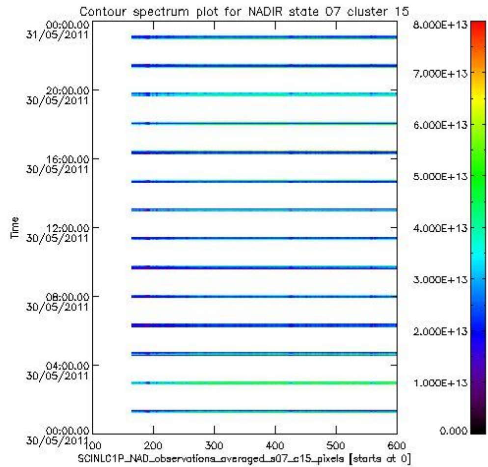
sciamachy_i1b_source_packet_report_SCIA_7_04_U_20110530_4.PNG
