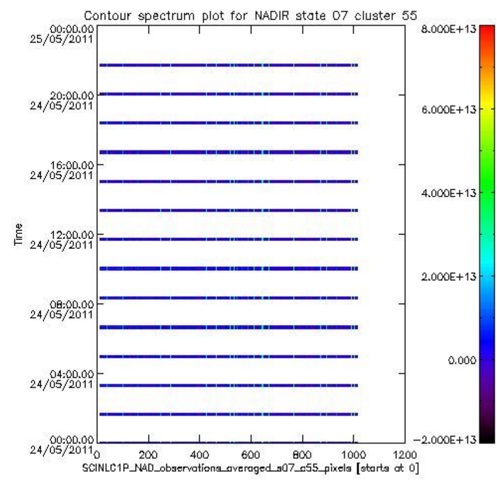
sciamachy_i1b_source_packet_report_SCIA_7_04_U_20110524_8.PNG
