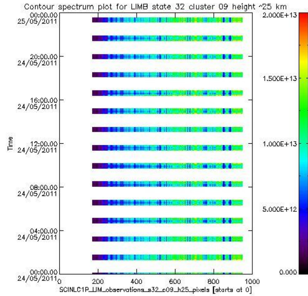
sciamachy_l1b_source_packet_report_SCIA_7_04_U_20110524_14.PNG
