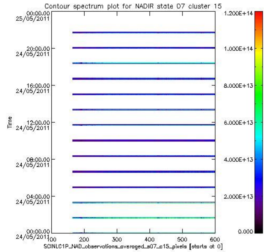
sciamachy_i1b_source_packet_report_SCIA_7_04_U_20110524_4.PNG
