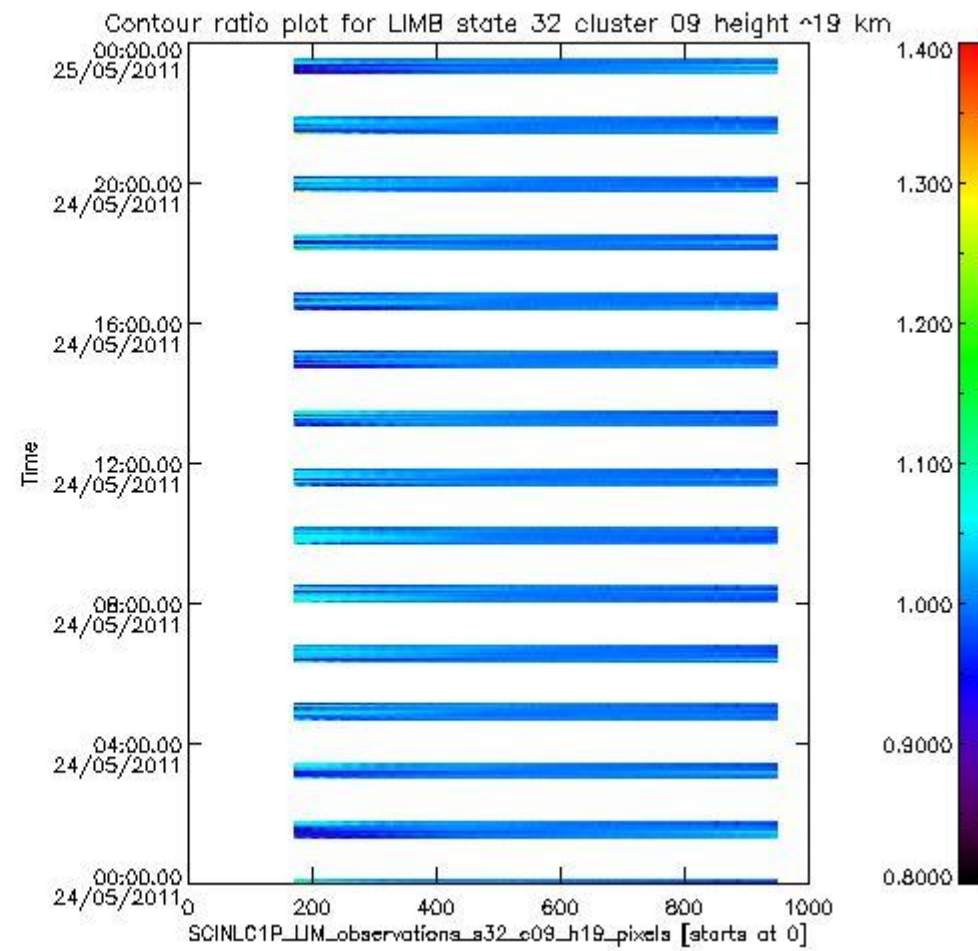
sciamachy_i1b_source_packet_report_SCIA_7_04_U_20110524_11.PNG
