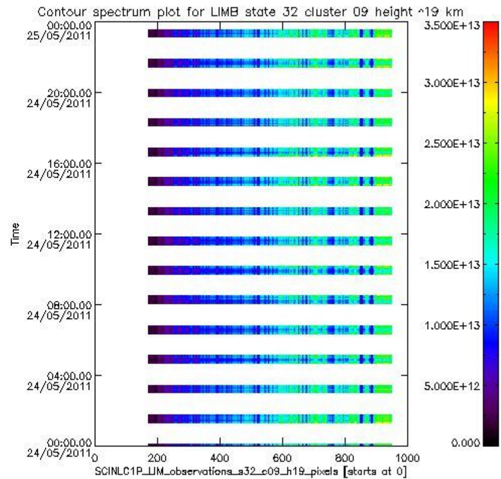
sciamachy_l1b_source_packet_report_SCIA_7_04_U_20110524_10.PNG
