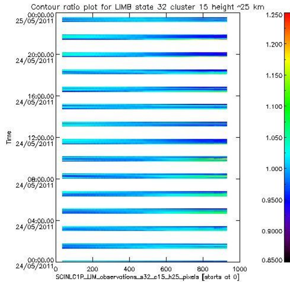
sciamachy_11b_source_packet_report_SCIA_7_04_U_20110524_19.PNG
