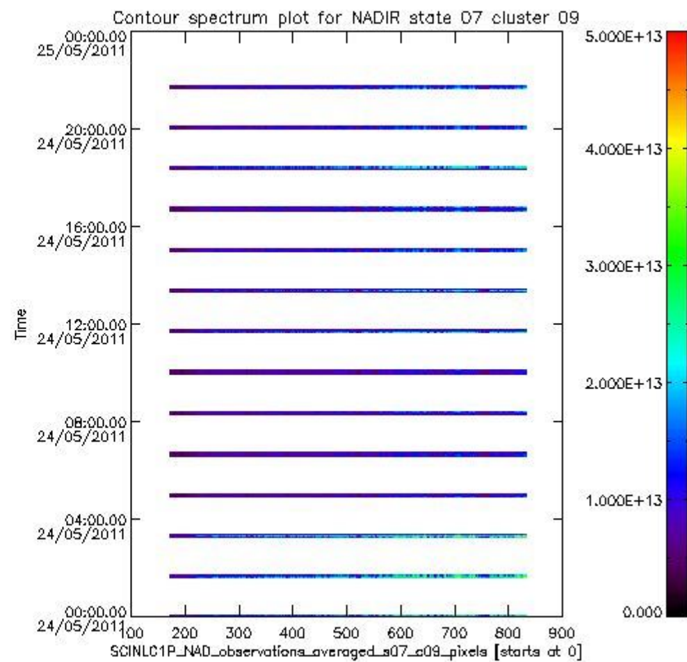
sciamachy_i1b_source_packet_report_SCIA_7_04_U_20110524_2.PNG
