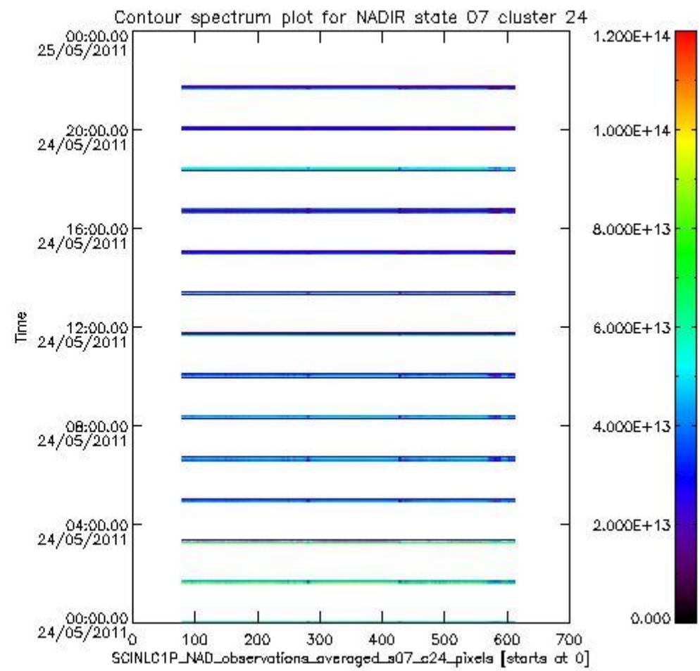
sciamachy_i1b_source_packet_report_SCIA_7_04_U_20110524_6.PNG
