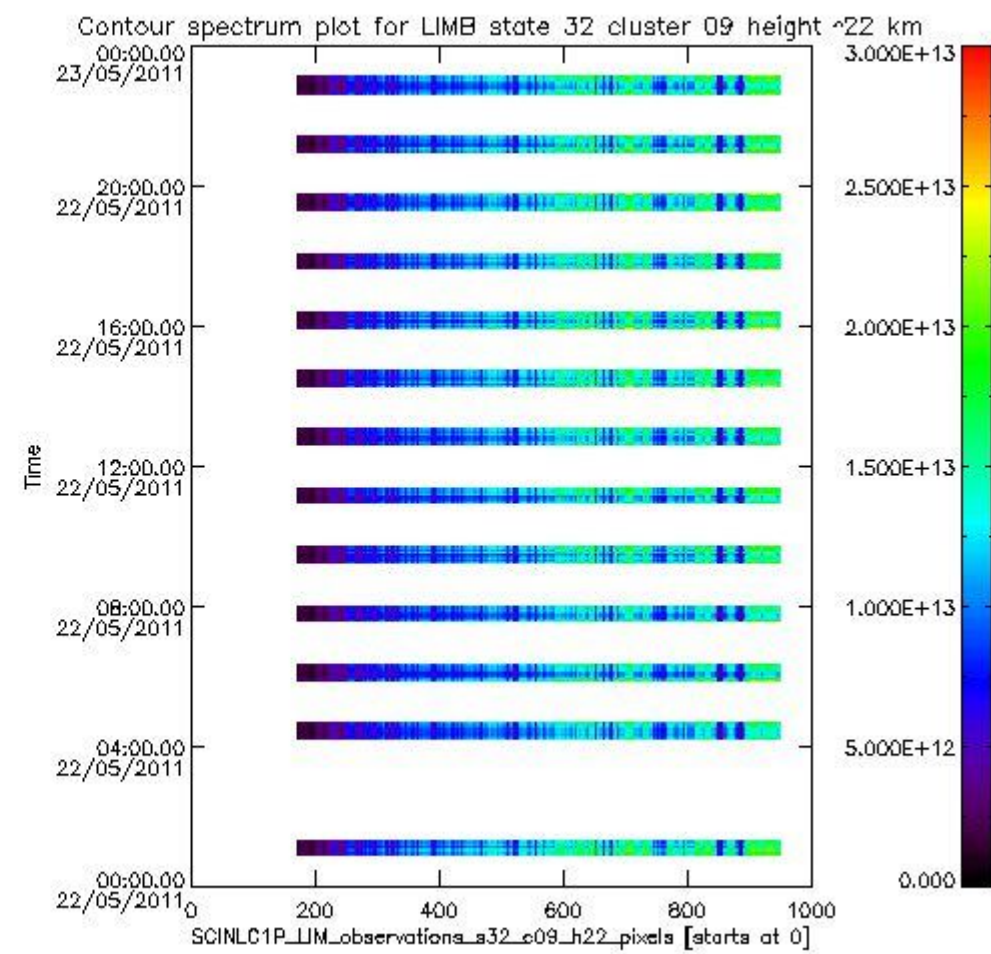
sciamachy_i1b_source_packet_report_SCIA_7_04_U_20110522_12.PNG
