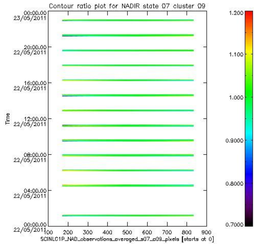
sciamachy_i1b_source_packet_report_SCIA_7_04_U_20110522_3.PNG
