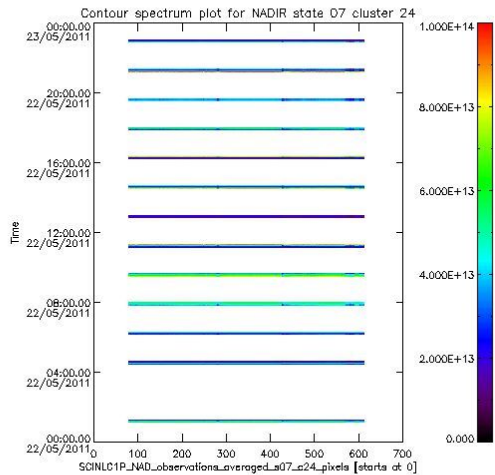
sciamachy_i1b_source_packet_report_SCIA_7_04_U_20110522_6.PNG
