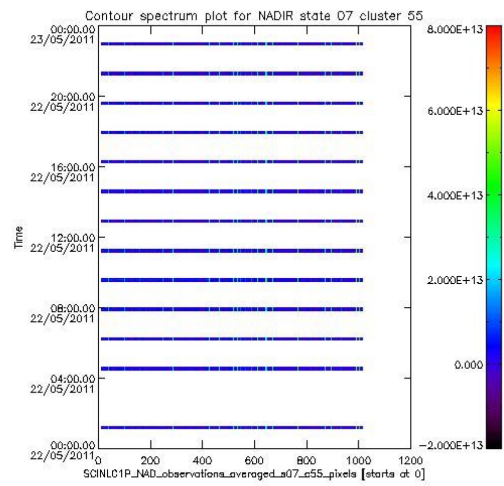
sciamachy_i1b_source_packet_report_SCIA_7_04_U_20110522_8.PNG
