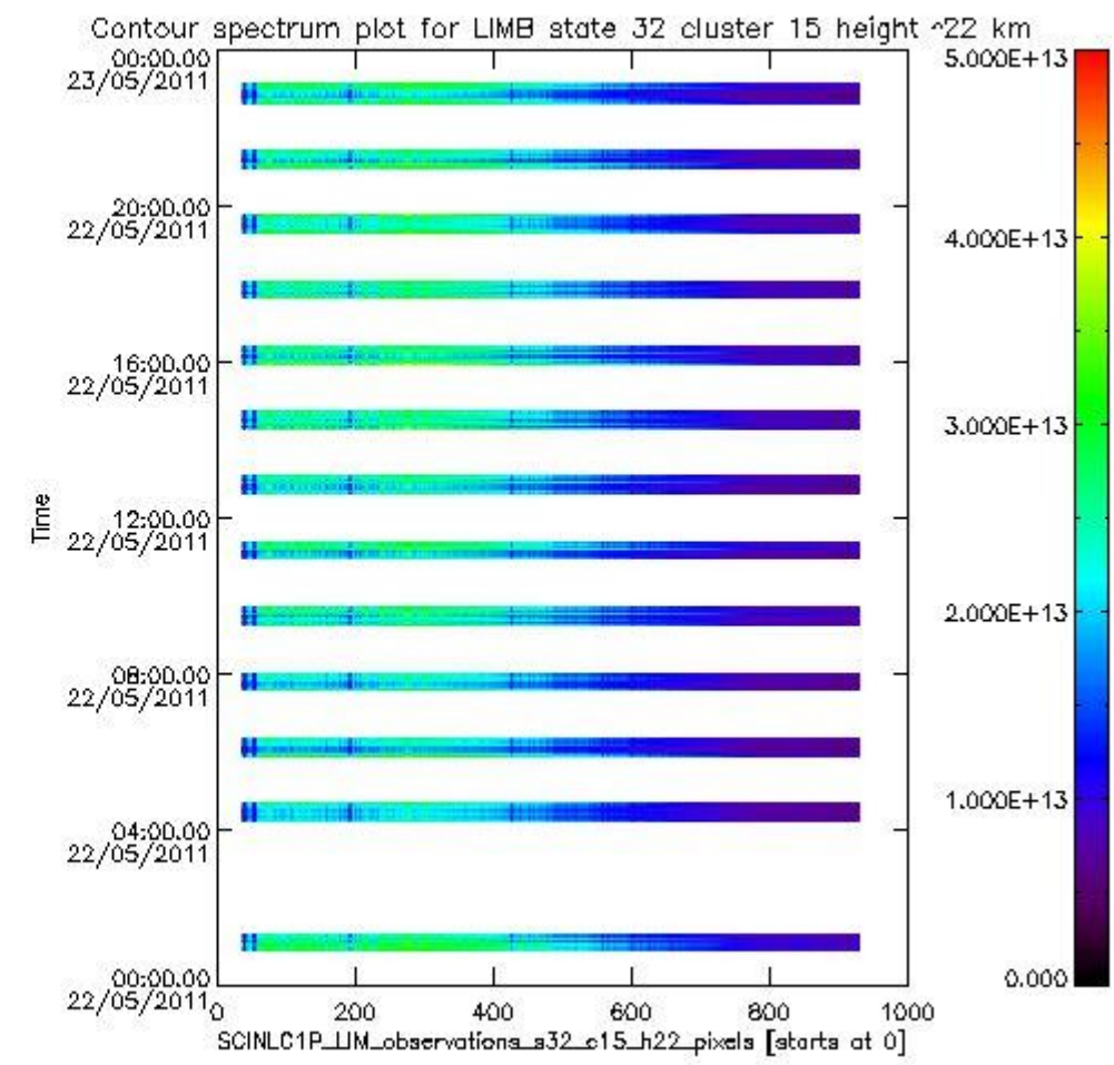
sciamachy_i1b_source_packet_report_SCIA_7_04_U_20110522_16.PNG
