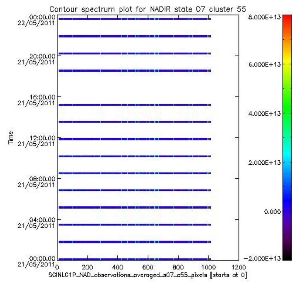
sciamachy_i1b_source_packet_report_SCIA_7_04_U_20110521_8.PNG
