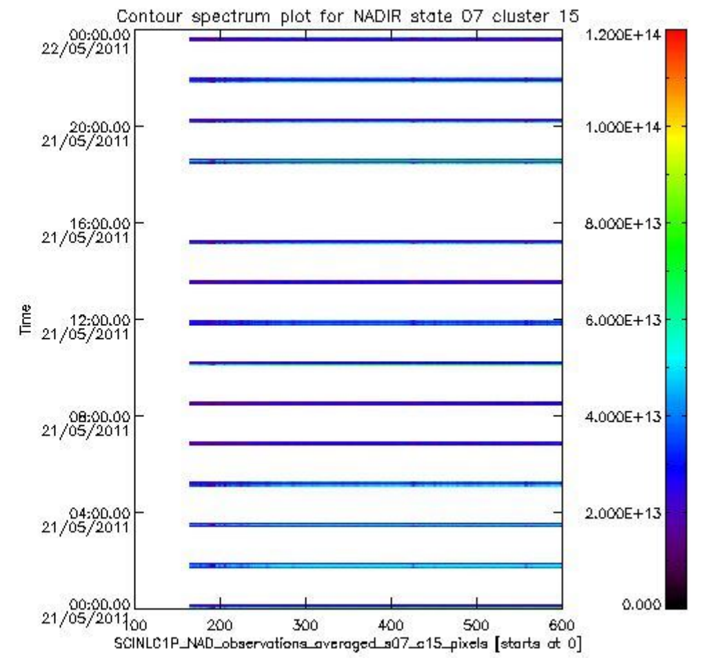
sciamachy_i1b_source_packet_report_SCIA_7_04_U_20110521_4.PNG
