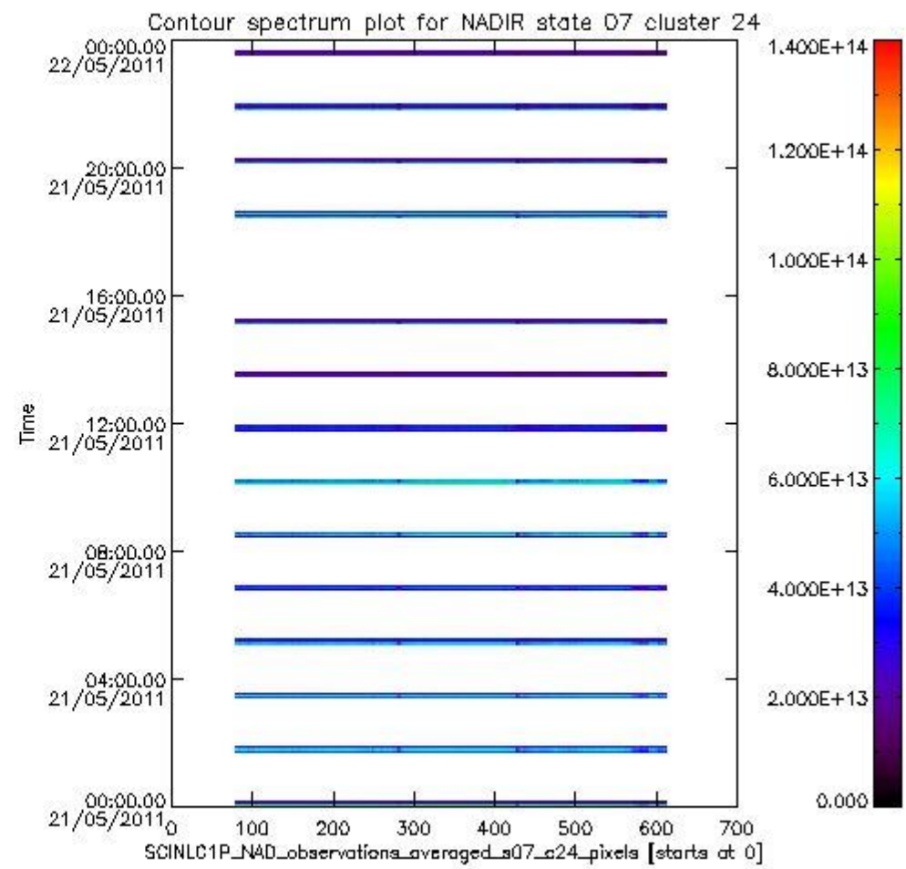
sciamachy_i1b_source_packet_report_SCIA_7_04_U_20110521_6.PNG
