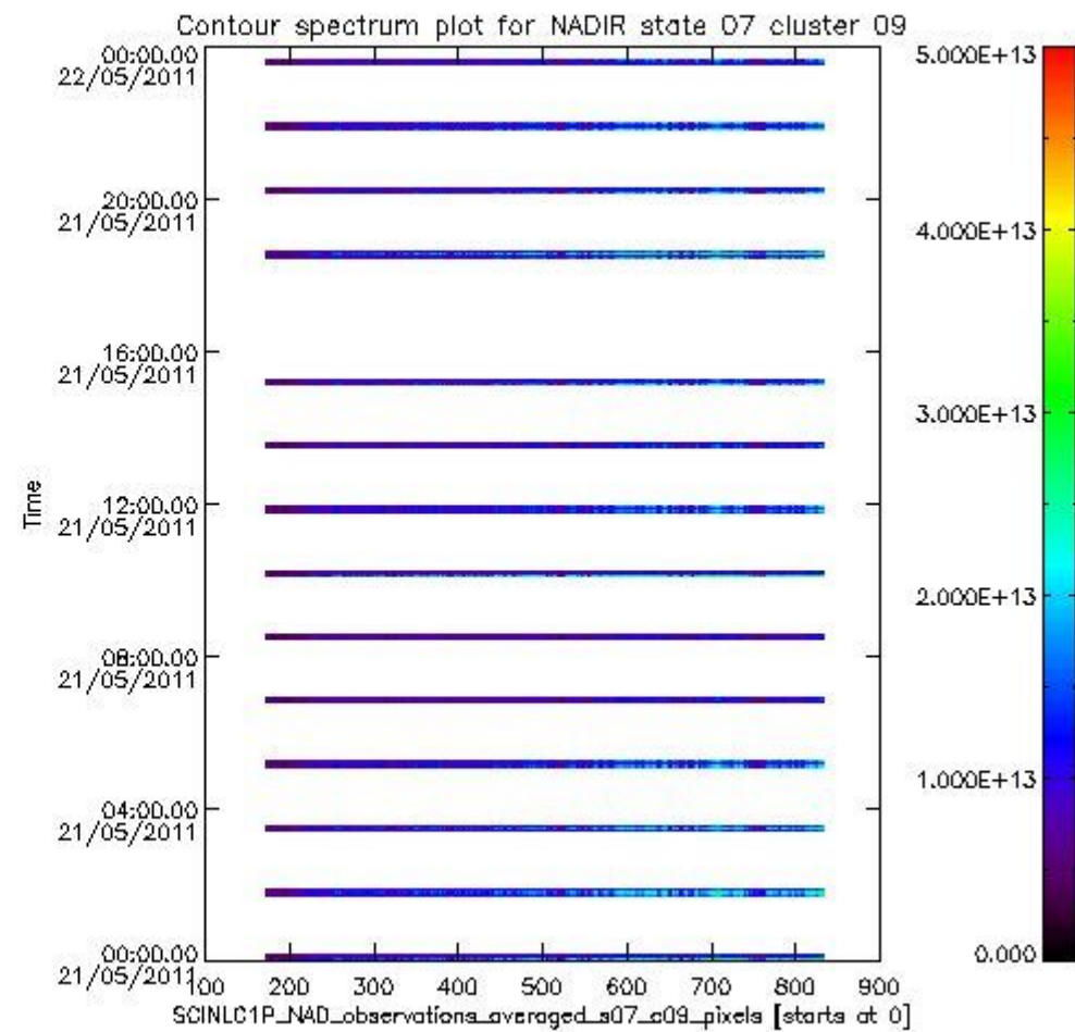
sciamachy_i1b_source_packet_report_SCIA_7_04_U_20110521_2.PNG
