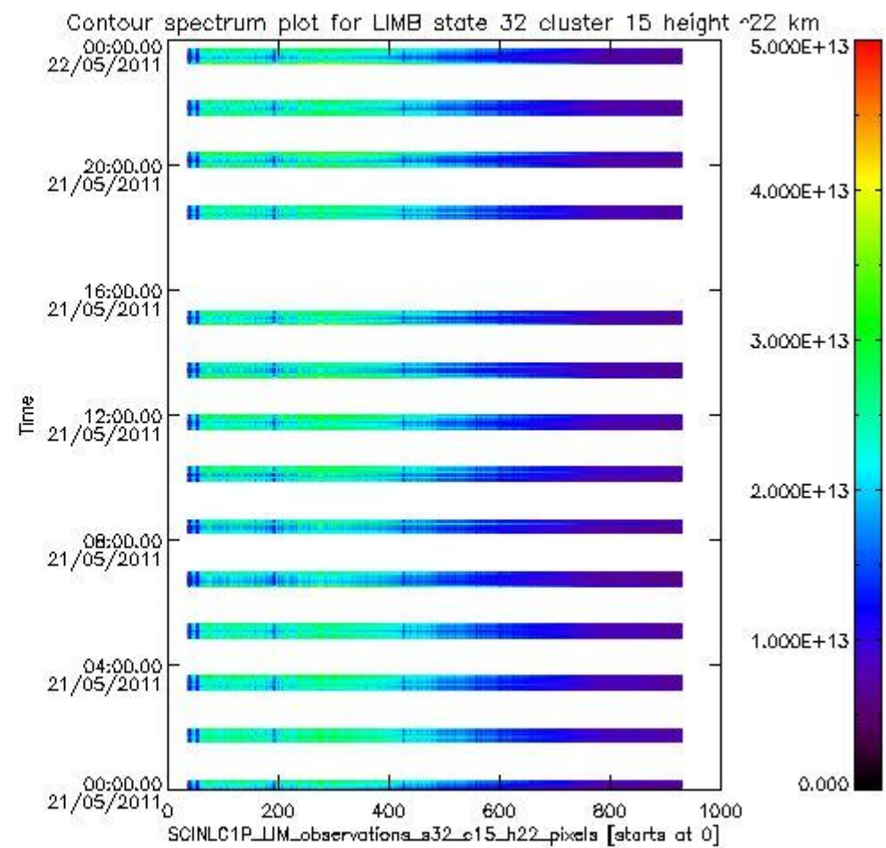
sciamachy_i1b_source_packet_report_SCIA_7_04_U_20110521_16.PNG
