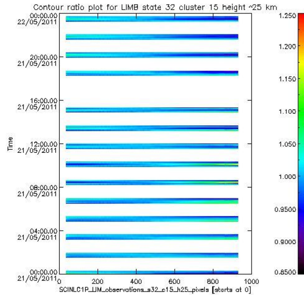
sciamachy_11b_source_packet_report_SCIA_7_04_U_20110521_19.PNG
