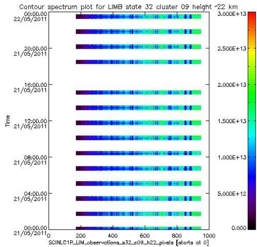
sciamachy_i1b_source_packet_report_SCIA_7_04_U_20110521_12.PNG
