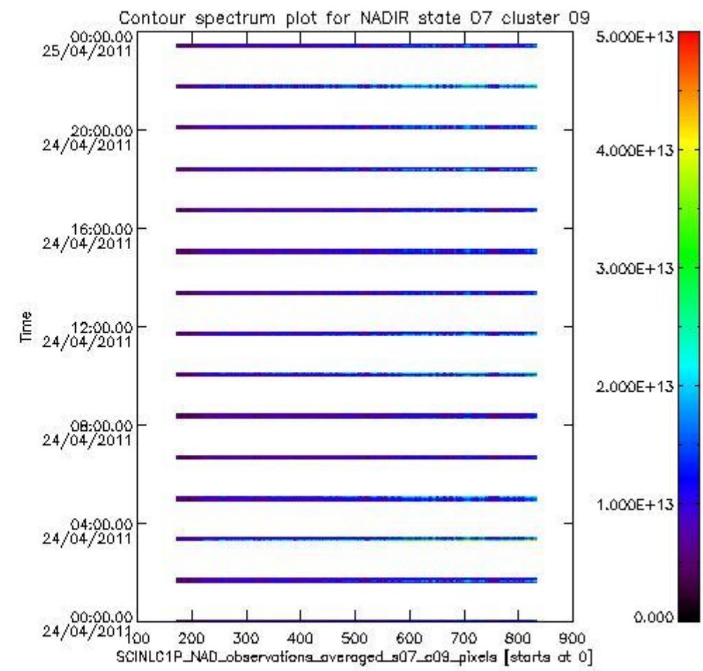
sciamachy_i1b_source_packet_report_SCIA_7_04_U_20110424_2.PNG
