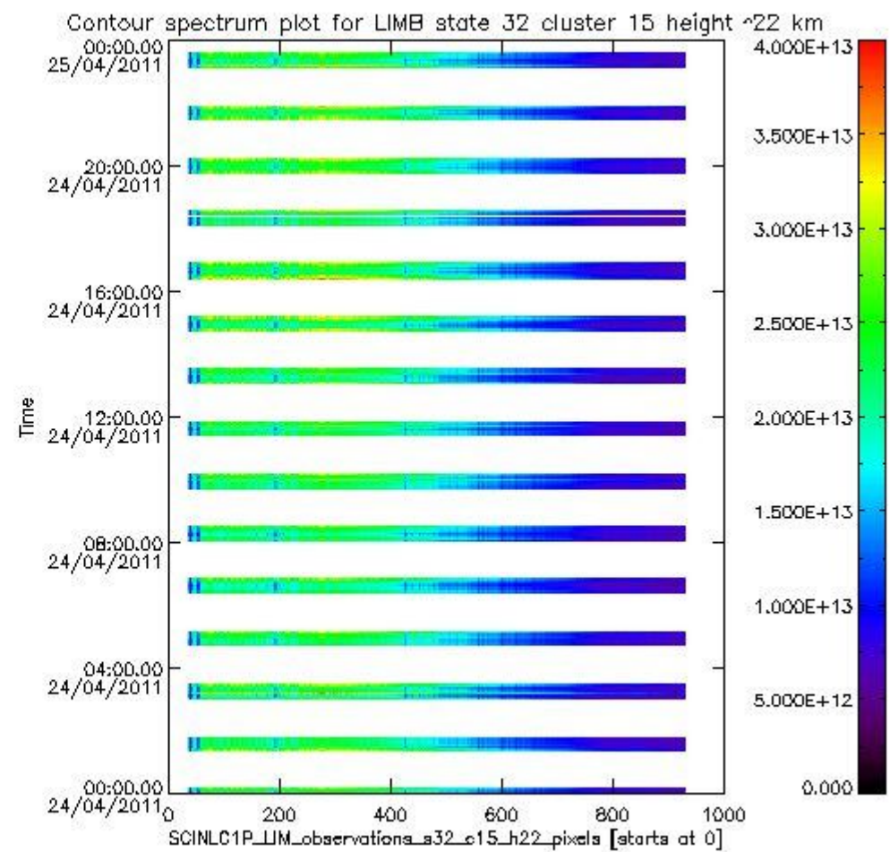
sciamachy_i1b_source_packet_report_SCIA_7_04_U_20110424_16.PNG
