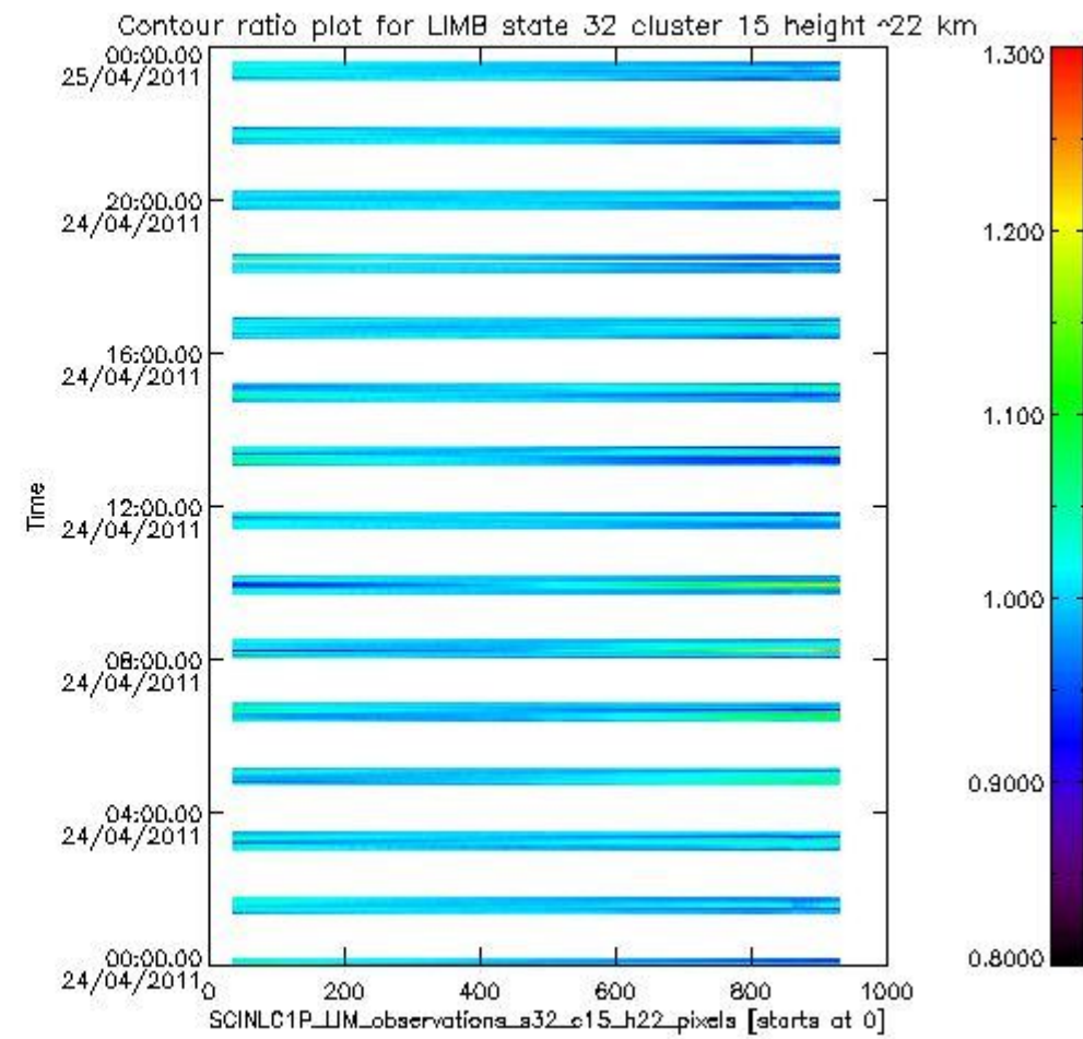
sciamachy_11b_source_packet_report_SCIA_7_04_U_20110424_17.PNG
