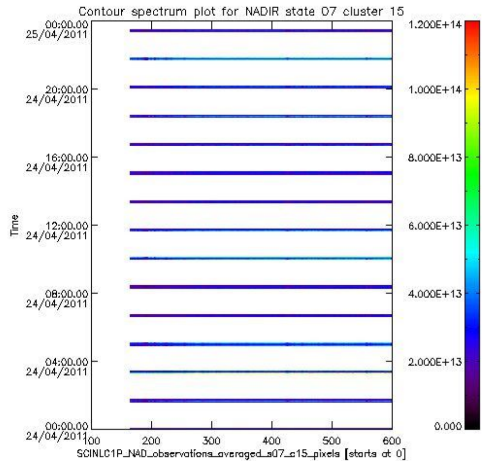
sciamachy_i1b_source_packet_report_SCIA_7_04_U_20110424_4.PNG
