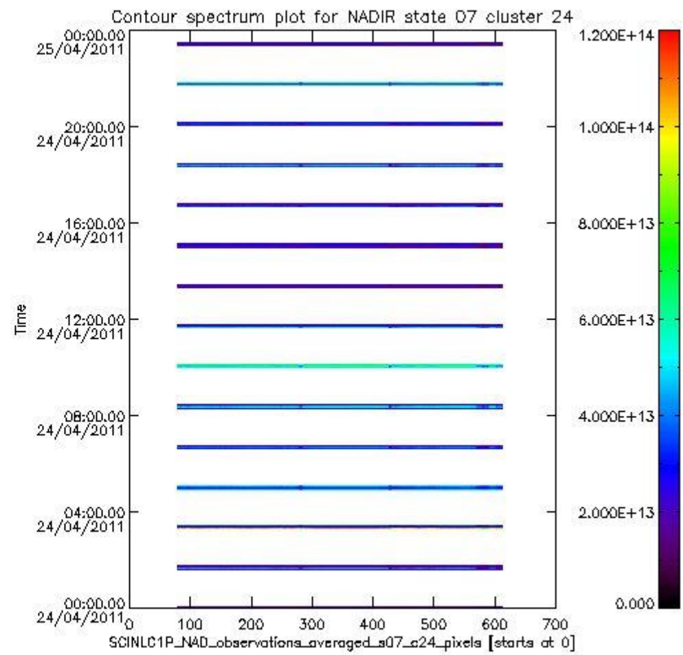
sciamachy_i1b_source_packet_report_SCIA_7_04_U_20110424_6.PNG
