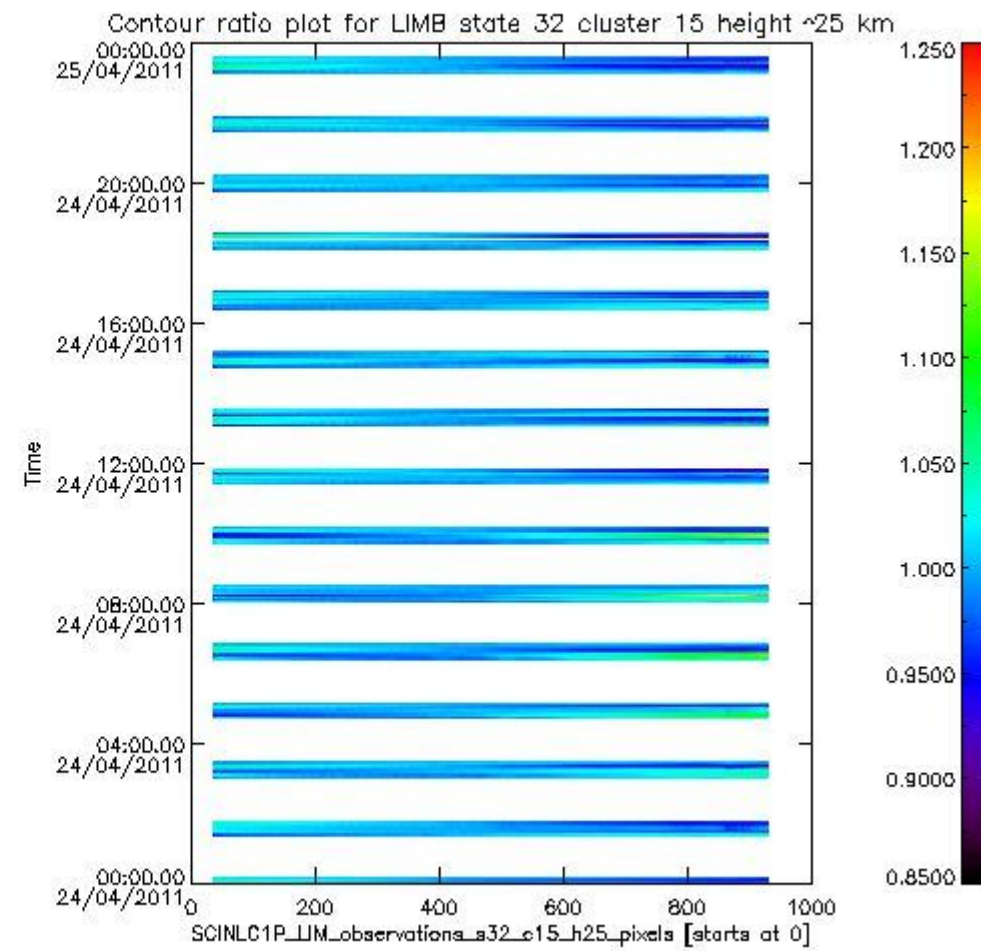
sciamachy_11b_source_packet_report_SCIA_7_04_U_20110424_19.PNG
