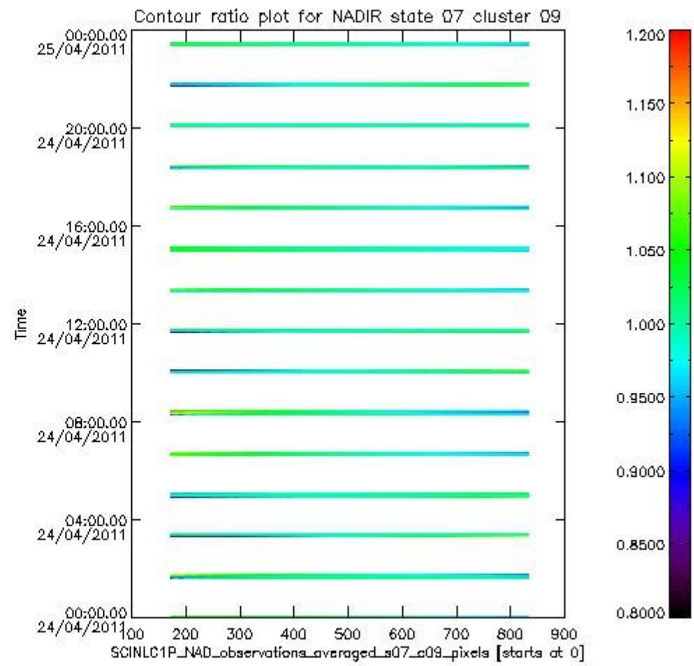
sciamachy_i1b_source_packet_report_SCIA_7_04_U_20110424_3.PNG
