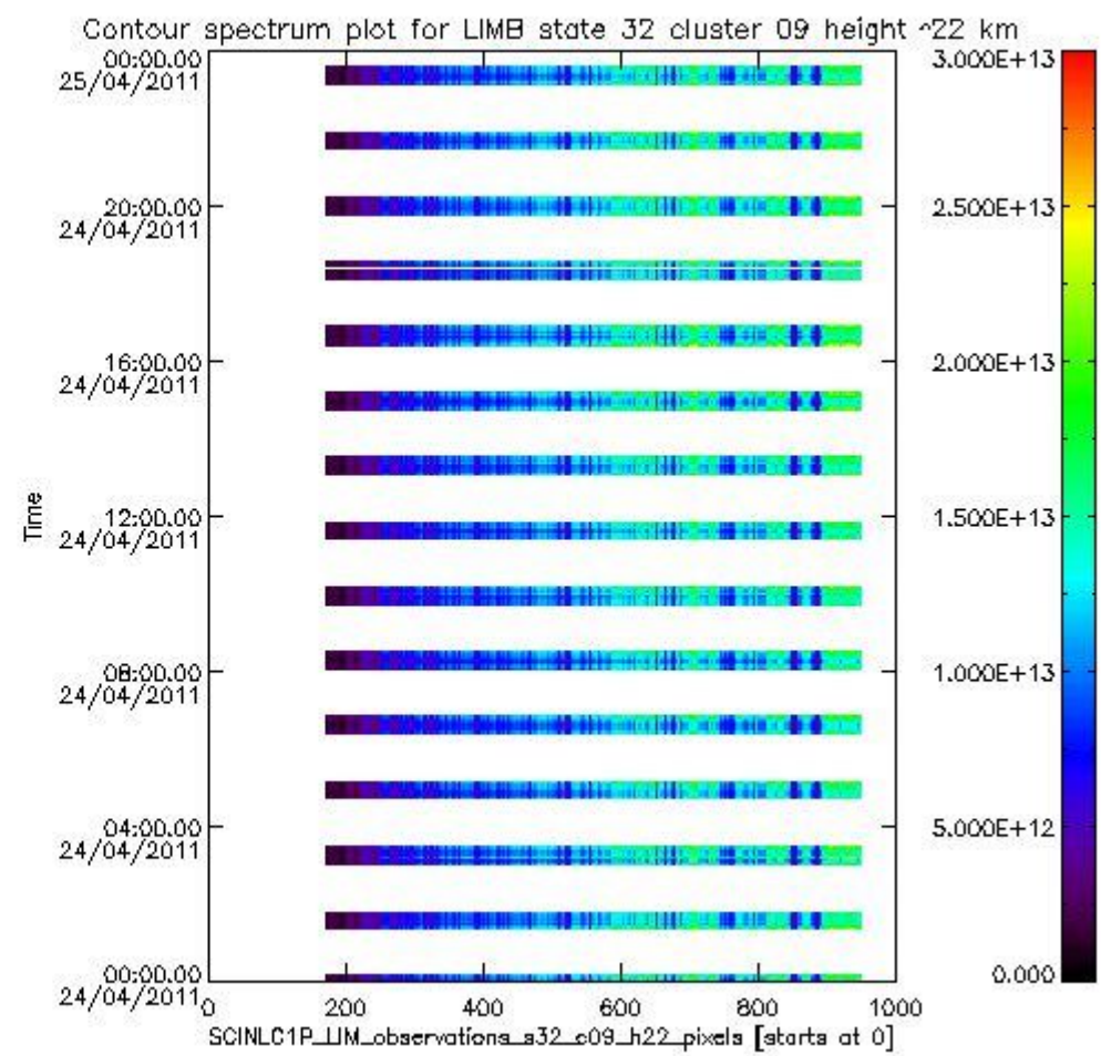
sciamachy_i1b_source_packet_report_SCIA_7_04_U_20110424_12.PNG
