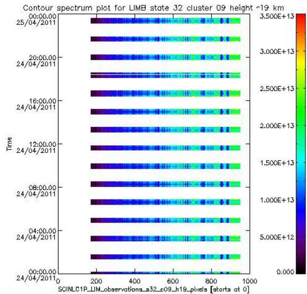
sciamachy_i1b_source_packet_report_SCIA_7_04_U_20110424_10.PNG
