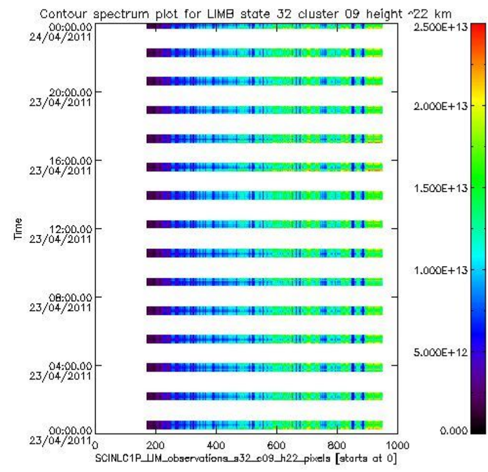
sciamachy_i1b_source_packet_report_SCIA_7_04_U_20110423_12.PNG
