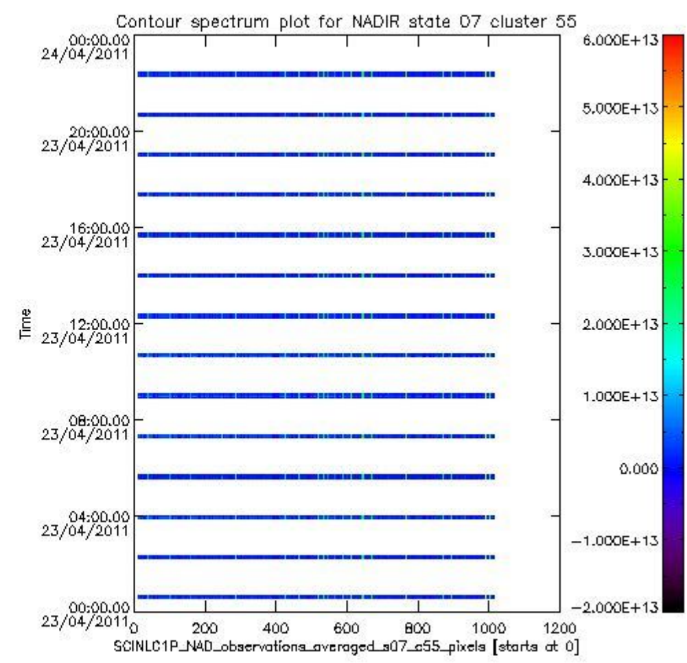
sciamachy_i1b_source_packet_report_SCIA_7_04_U_20110423_8.PNG
