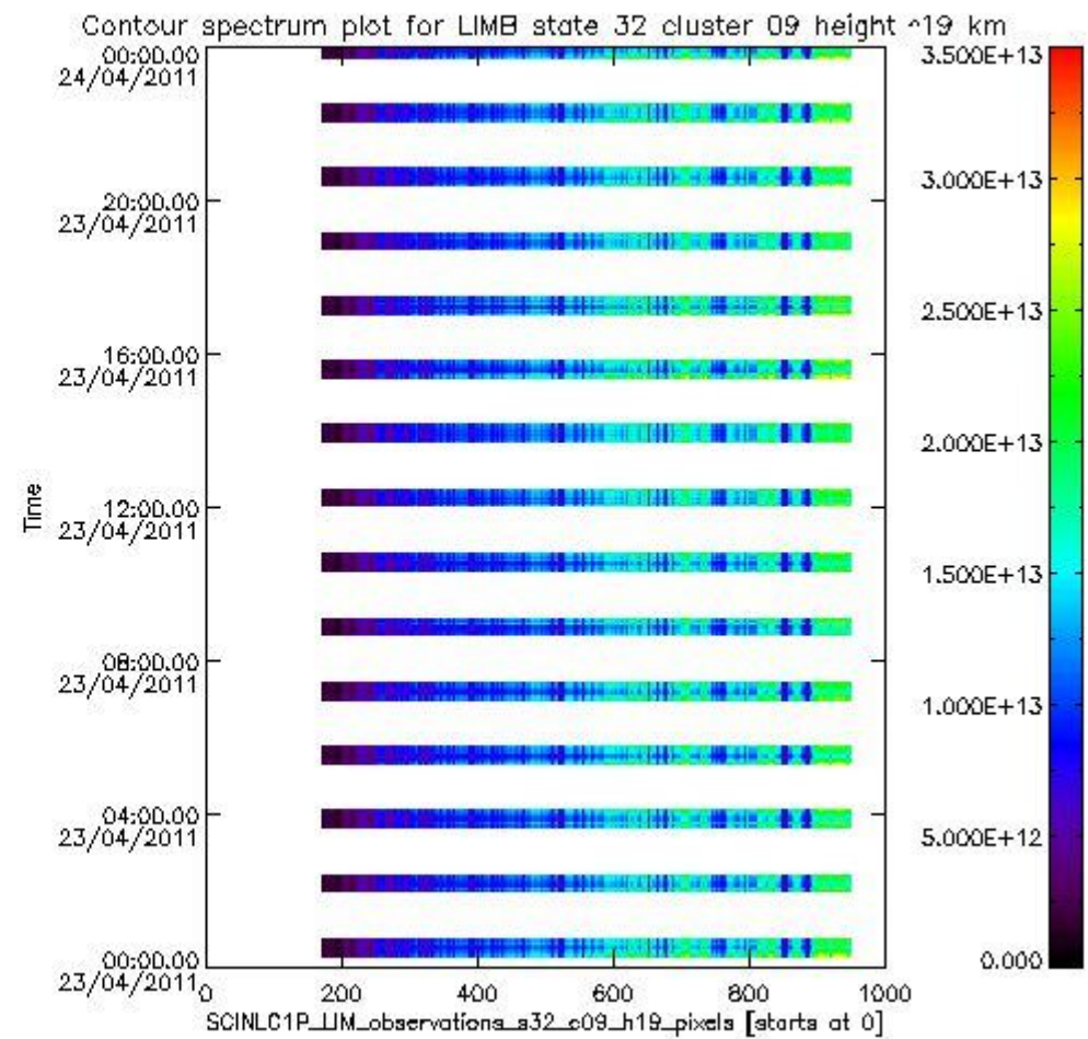
sciamachy_i1b_source_packet_report_SCIA_7_04_U_20110423_10.PNG
