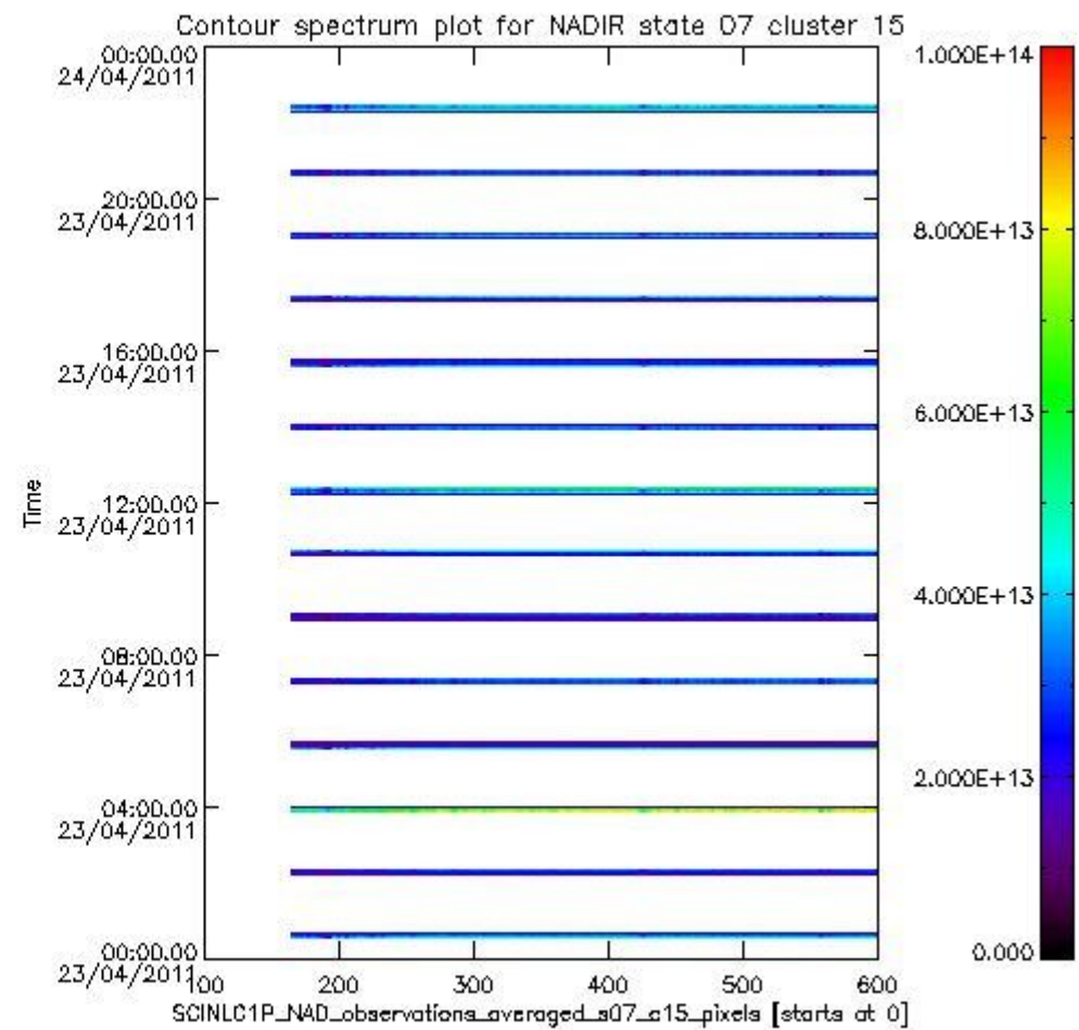
sciamachy_i1b_source_packet_report_SCIA_7_04_U_20110423_4.PNG
