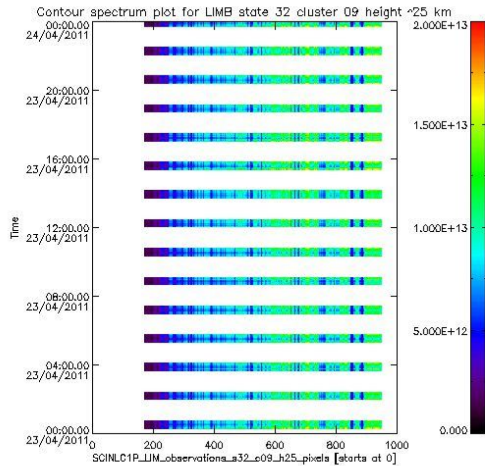
sciamachy_i1b_source_packet_report_SCIA_7_04_U_20110423_14.PNG
