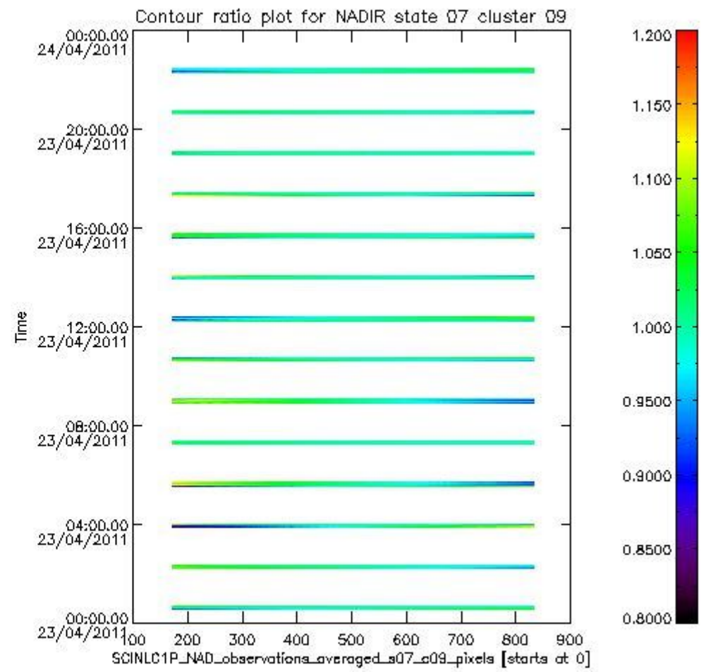
sciamachy_i1b_source_packet_report_SCIA_7_04_U_20110423_3.PNG
