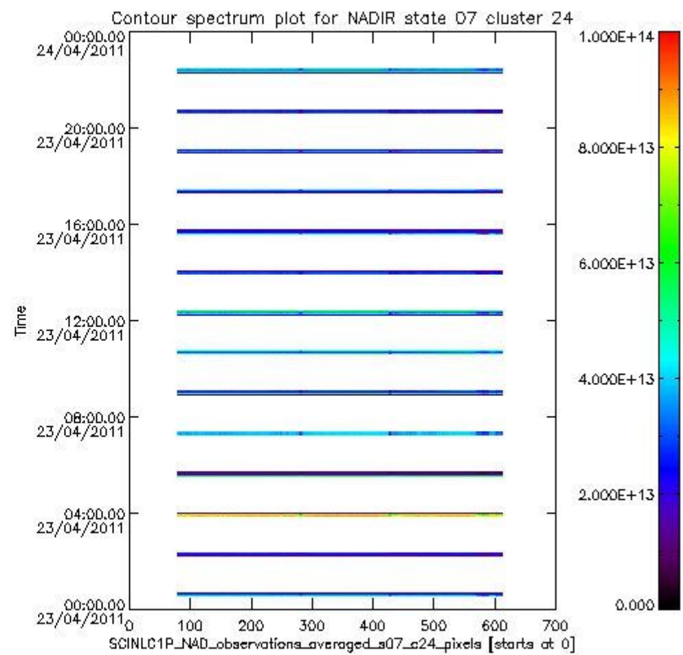
sciamachy_i1b_source_packet_report_SCIA_7_04_U_20110423_6.PNG
