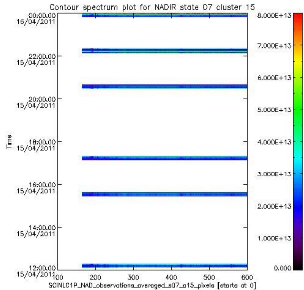
sciamachy_i1b_source_packet_report_SCIA_7_04_U_20110415_4.PNG
