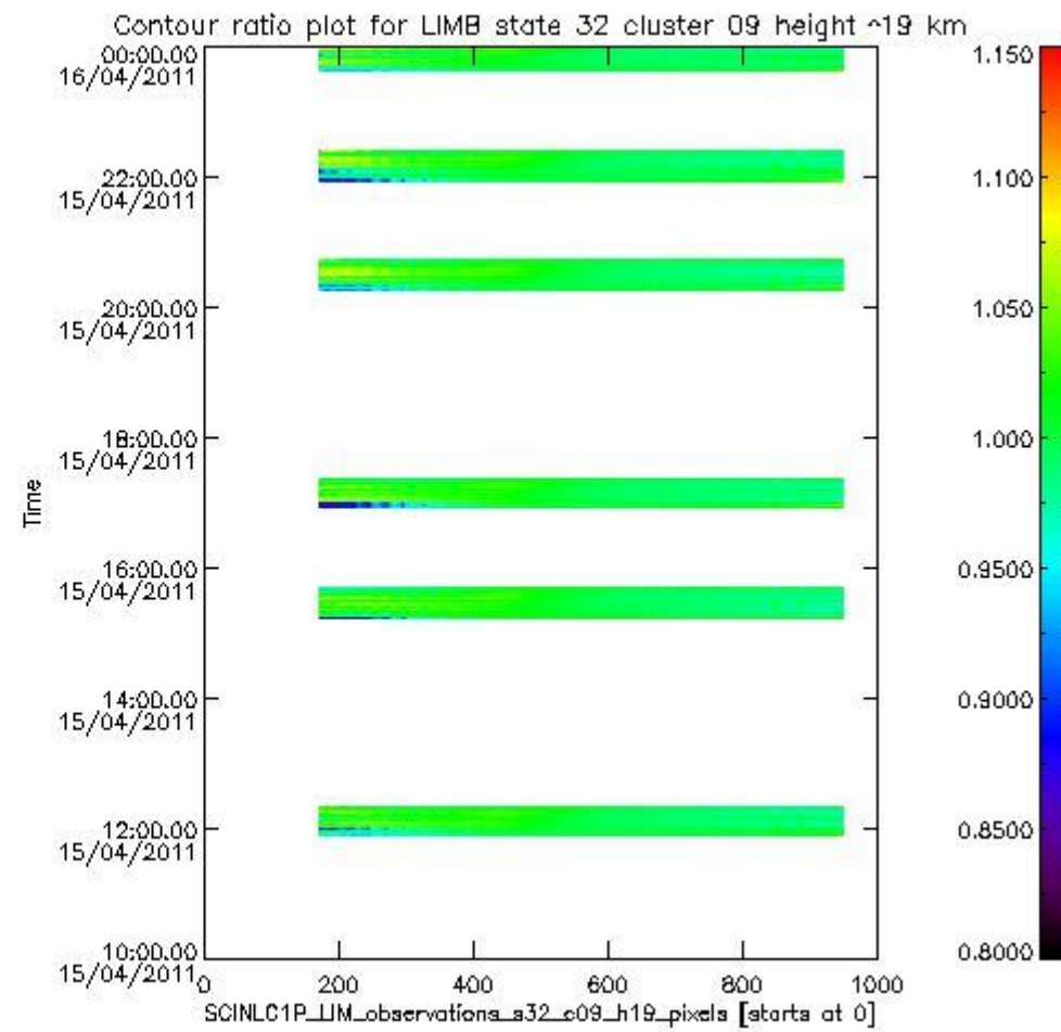
sciamachy_i1b_source_packet_report_SCIA_7_04_U_20110415_11.PNG
