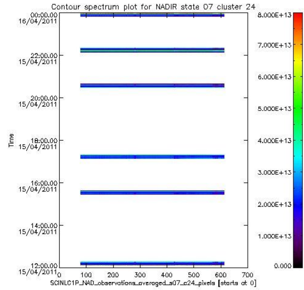
sciamachy_i1b_source_packet_report_SCIA_7_04_U_20110415_6.PNG
