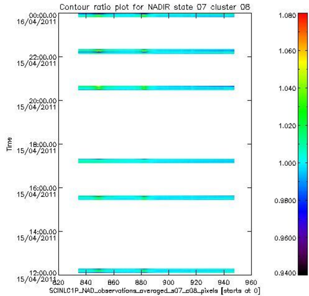
sciamachy_i1b_source_packet_report_SCIA_7_04_U_20110415_1.PNG
