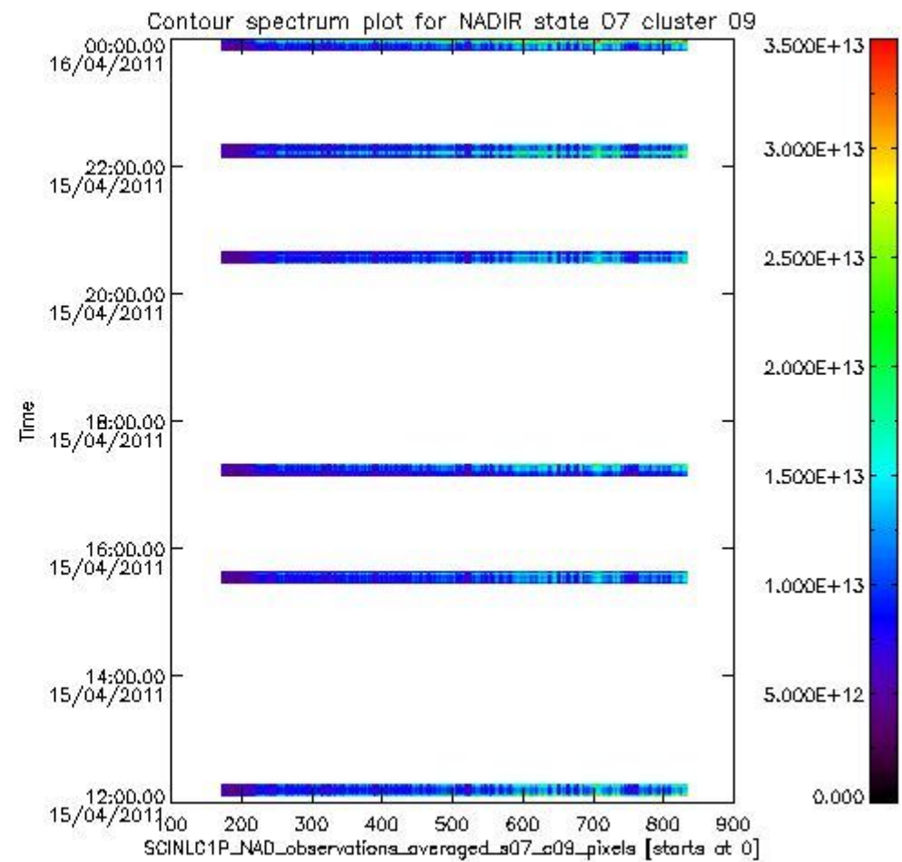
sciamachy_i1b_source_packet_report_SCIA_7_04_U_20110415_2.PNG
