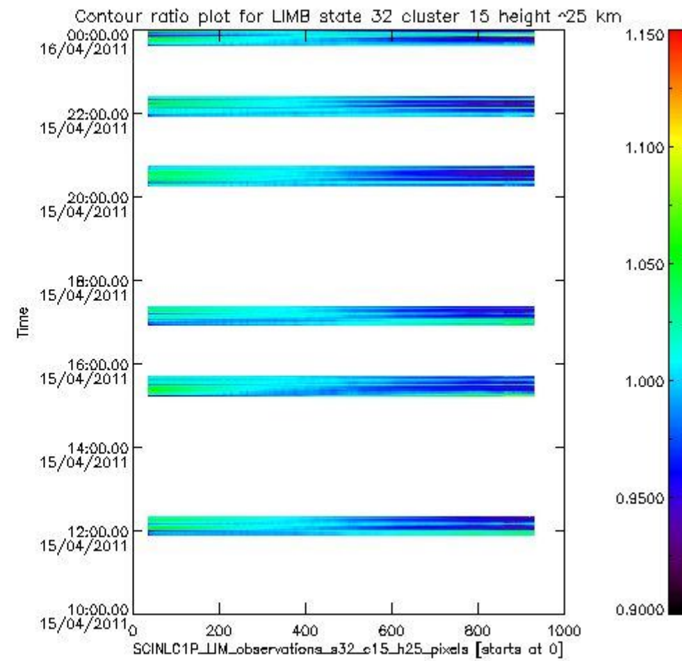
sciamachy_11b_source_packet_report_SCIA_7_04_U_20110415_19.PNG
