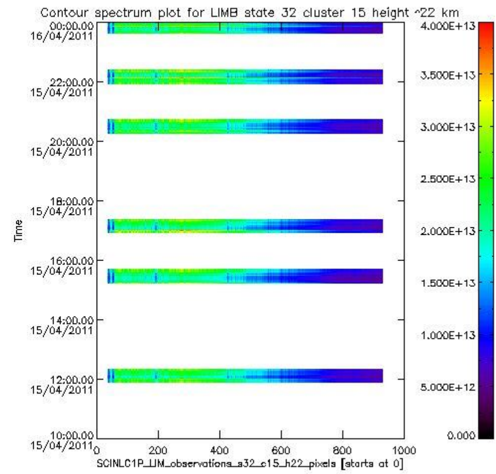
sciamachy_i1b_source_packet_report_SCIA_7_04_U_20110415_16.PNG
