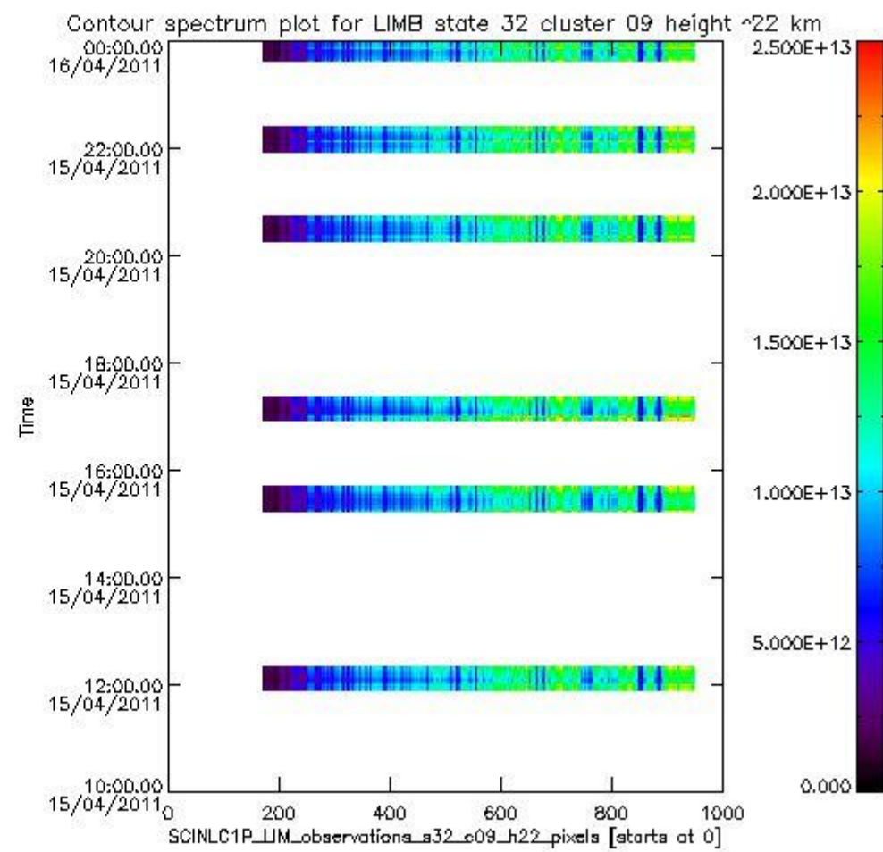
sciamachy_i1b_source_packet_report_SCIA_7_04_U_20110415_12.PNG
