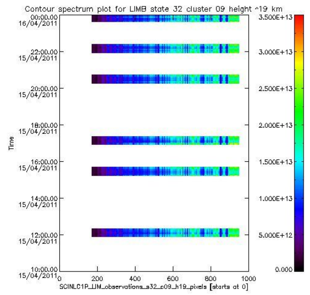
sciamachy_i1b_source_packet_report_SCIA_7_04_U_20110415_10.PNG
