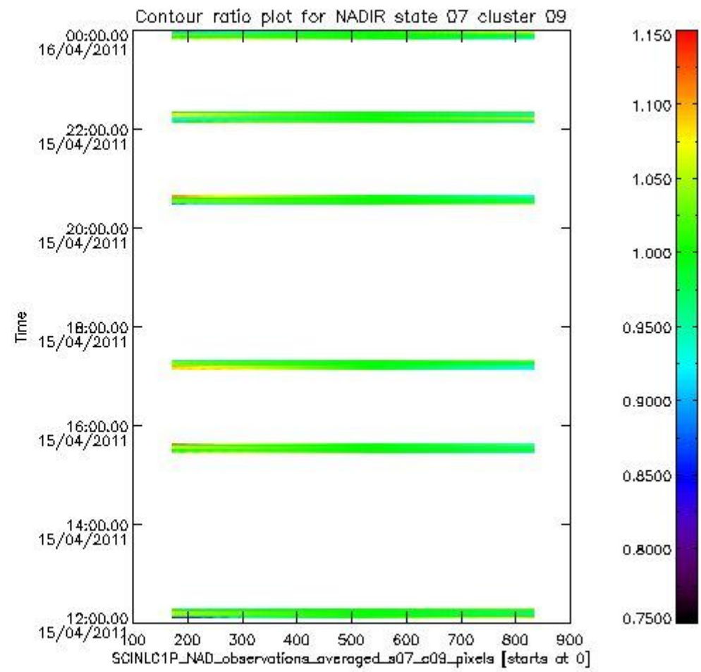
sciamachy_i1b_source_packet_report_SCIA_7_04_U_20110415_3.PNG
