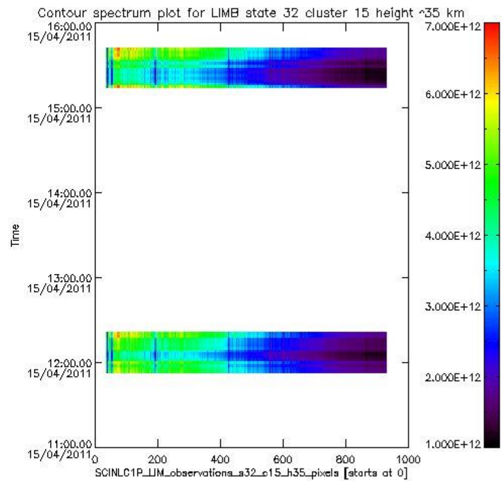
sciamachy_11b_source_packet_report_SCIA_7_04_U_20110415_20.PNG
