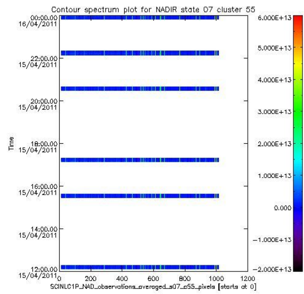
sciamachy_i1b_source_packet_report_SCIA_7_04_U_20110415_8.PNG
